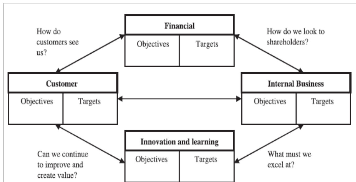
Figure 3: BSC Framework
