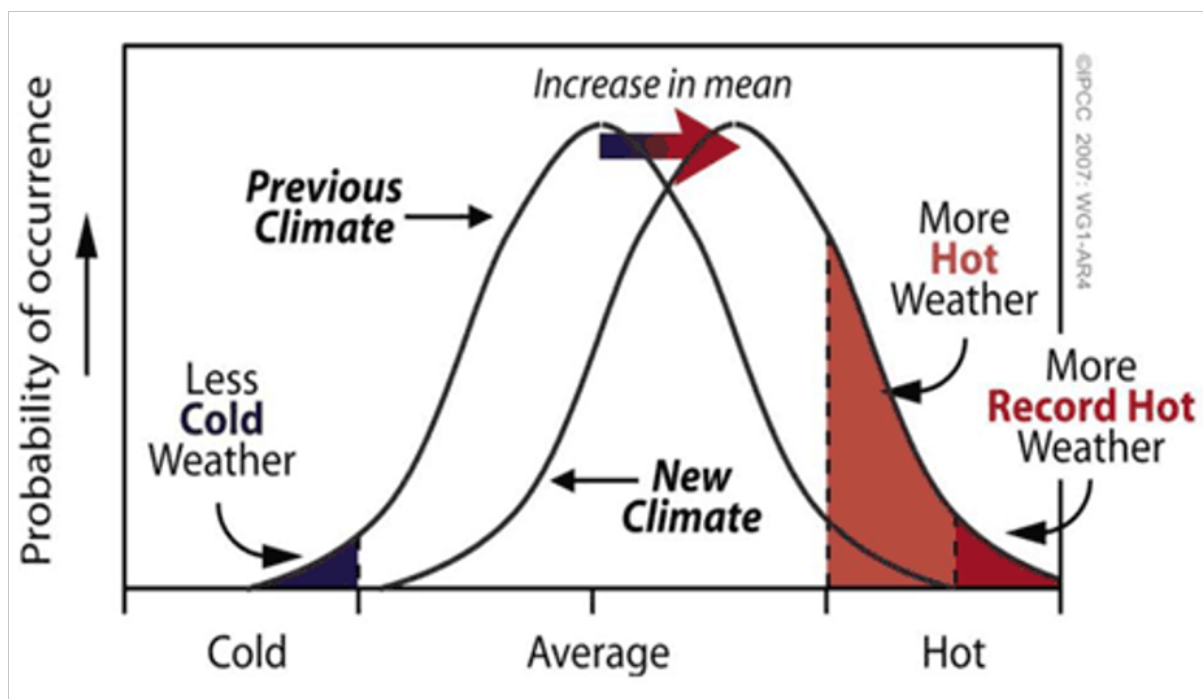
Figure 2.2: Demonstration of how a shift in average temperature influences the frequency of extreme heat. Source: IPCC (2007)
