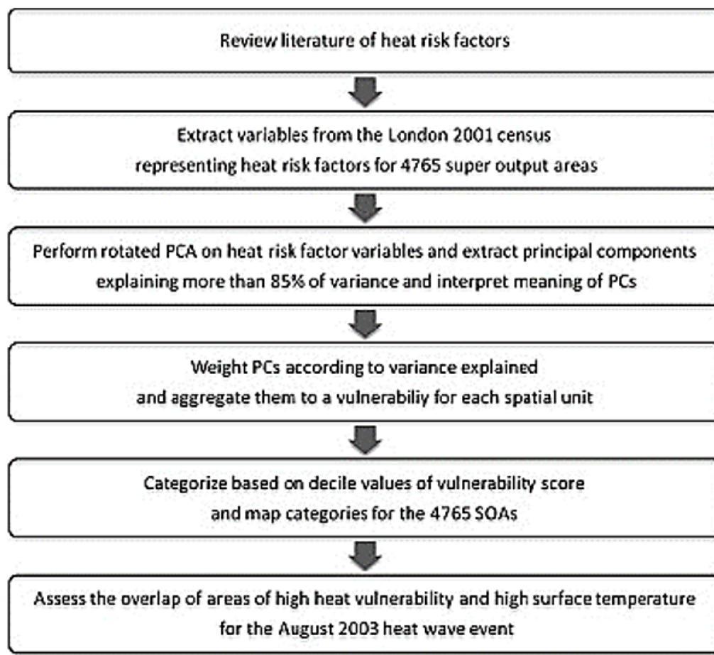
Figure 3.2: Example methodology applied in the development of the Heat Vulnerability Index. Source: Wolf and McGregor (2013)
