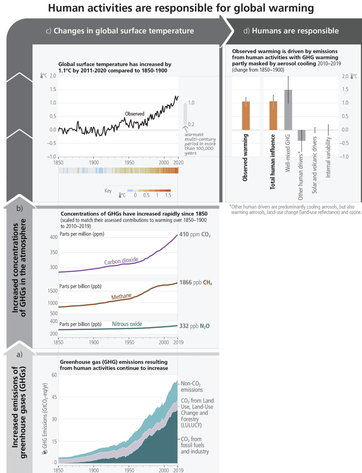
Figure 2.1: The causal chain from emissions to resulting warming of the climate system. a) Emissions of greenhouse gases (GHG) have increased rapidly over recent decades; b) These emissions have led to increases in the atmospheric concentrations of several GHGs, including CO 2 , CH 4 and N 2 O; c) The global surface temperature increased by around 1.1°C since 1850/1900 to 2020; and d) Formal detection and attribution
