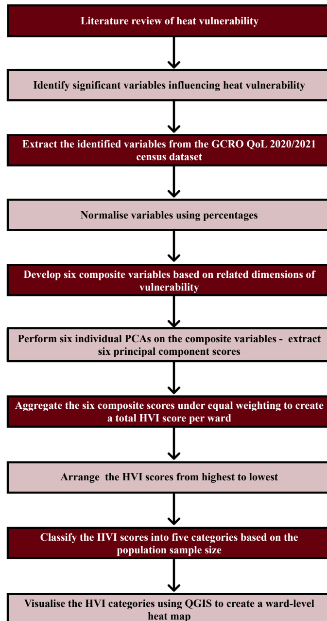
Figure 3.7: Figurative illustration of the step-by-step process of the Heat Vulnerability Index method.
