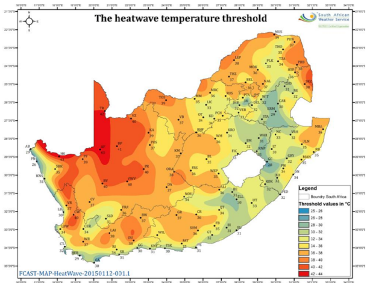
Figure 2.10: Heatwave temperature thresholds across South Africa. Source: South African Weather Service (n.d)
