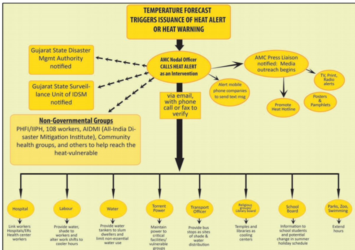
Figure 2.7: Communication plan activated by Ahmedabad Municipal Corporation's Nodal Officer in response to a heat alert or warning. Source: Ahmedabad Municipal Corporation (2016)
