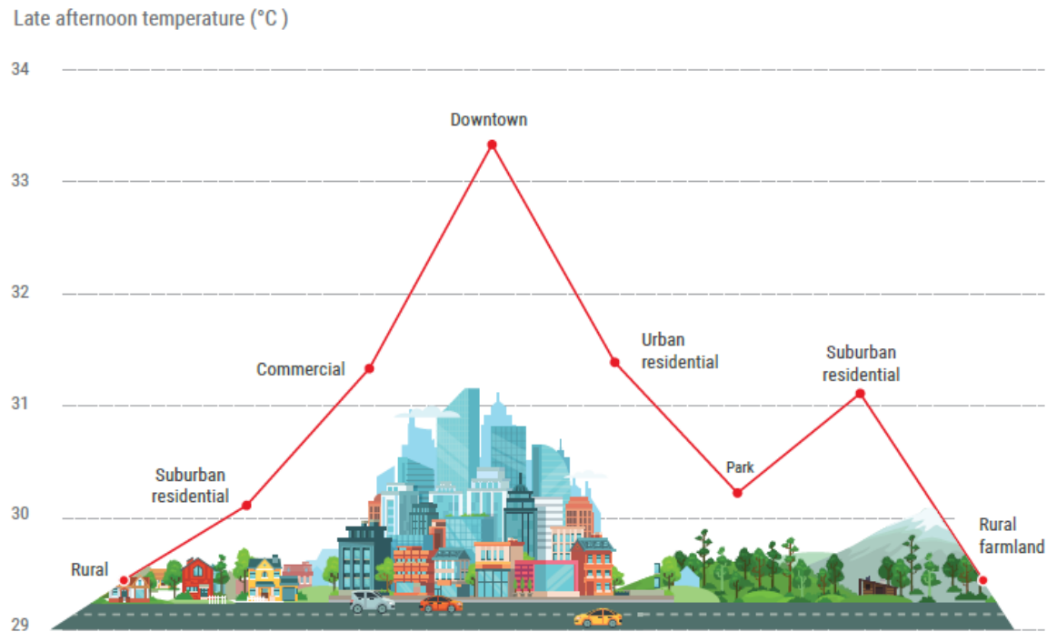
Figure 2.4: Urban Heat Island profile adapted from Heat Island Group, Lawrence Berkeley National Laboratory. Source: Puley (2022)
