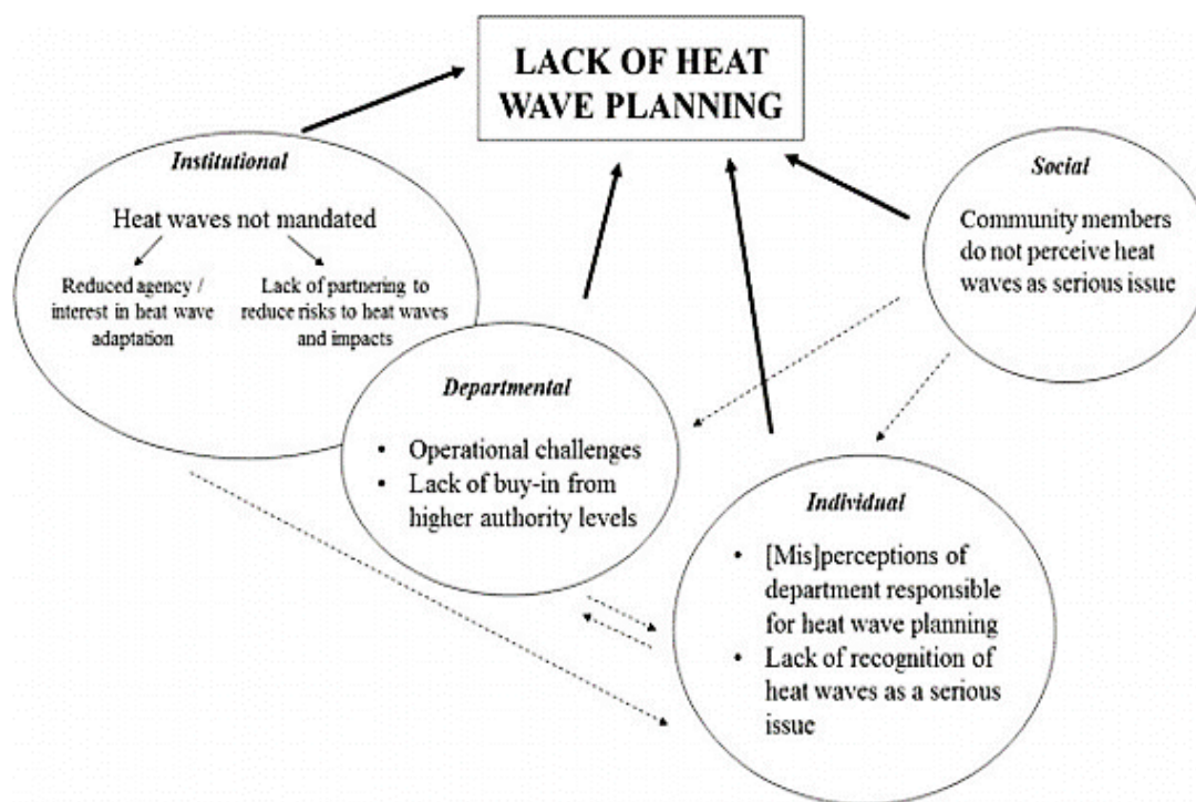
Figure 2.16: Inter-related individual, social and institutional settings of extreme heat and heatwave planning within the Environmental Health Department. Source: Nana et al. (2019)
