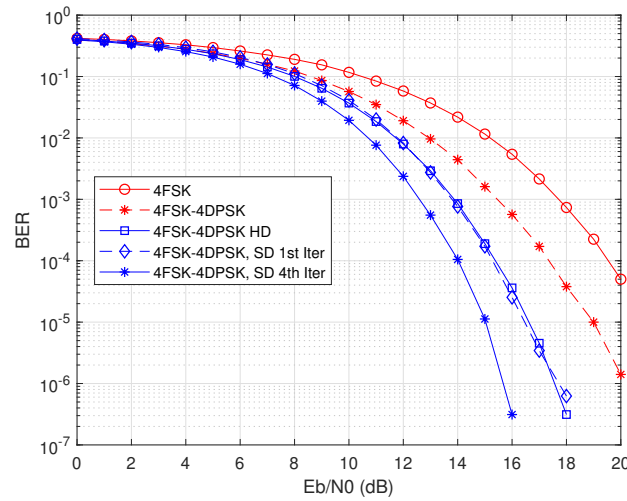
FIGURE 5.6: BER performance comparing permutation coded OFDM-4FSK-4DPSK scheme with the uncoded scheme in PLC, \frac{\sigma_G}{\sigma_I} = 0.1 , L = 4 , |C| = 4 .
