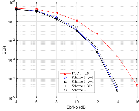
FIGURE 6.11: Schemes 1 & 3 with Viterbi decoding of PTC codewords for R_C = 1/4 , M = 4 and A = 0.1 in PLC channel.
