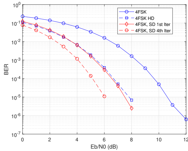
FIGURE 5.3: BER performance comparing permutation coded OFDM-4FSK scheme with the uncoded scheme in AWGN, L = 4 , |C| = 4 .
