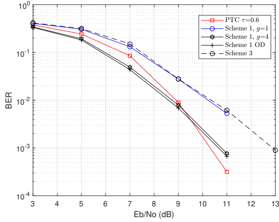
FIGURE 6.9: Schemes 1 & 3 with Viterbi decoding of PTC codewords for R_C = 2/3 , M = 4 and A = 0.1 in PLC channel.
