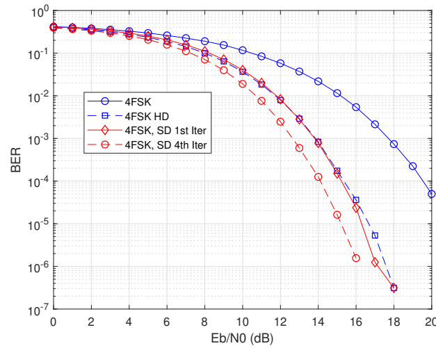
FIGURE 5.4: BER performance comparing permutation coded OFDM-4FSK scheme with the uncoded scheme in PLC, \frac{\sigma_G}{\sigma_I} = 0.1 , L = 4 , |C| = 4 .
