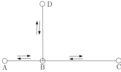
FIGURE 2.2: PLC network illustrating multipath model in the branches.
