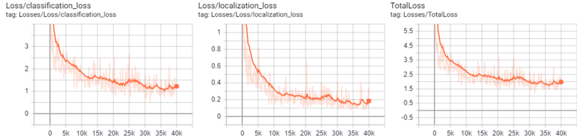
(c) SSD Group C Loss Graphs (from left to right) Classification loss, Localisation loss, and Total loss
