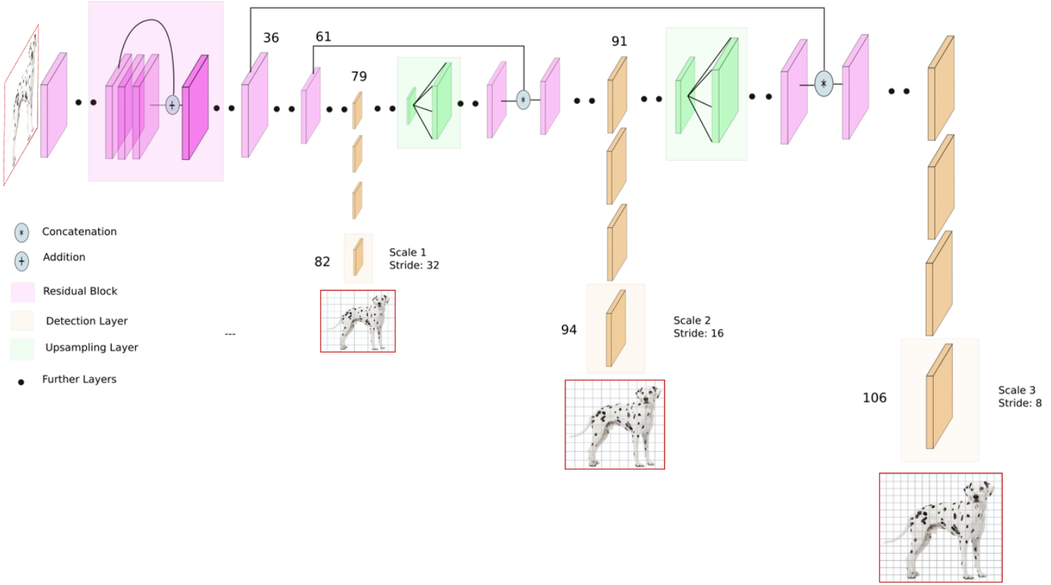
Figure 3.12: YOLOv3 Network Architecture [Jing et al. 2020]
