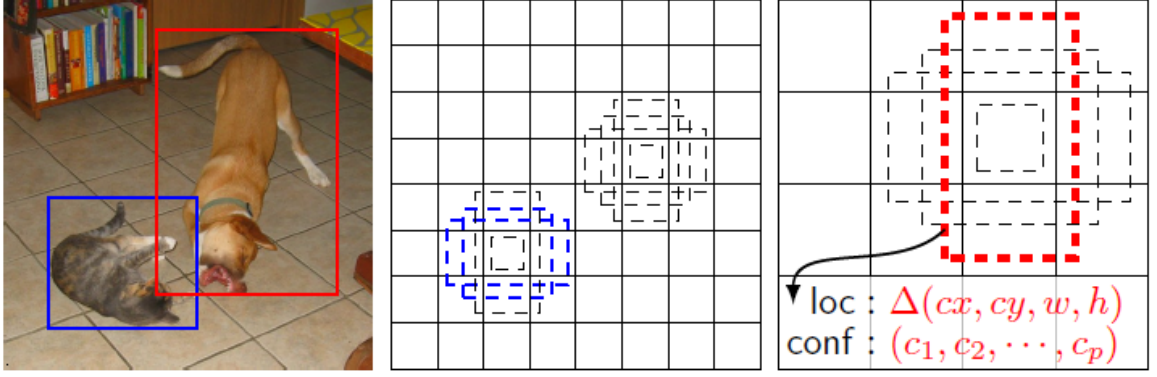
Figure 3.5: Input image of a cat and dog within their own ground truth box, alongside an 8 x 8 and a 4 x 4 feature map with default boxes predicting the localization and classification output. The blue boxes correspond to the cat, while the red corresponds to the dog [Liu et al. 2016]
