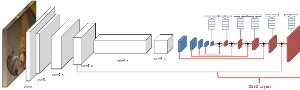
Figure 3.7: Structure of DSSD with additional deconvolutional layers [Fu et al. 2017]
