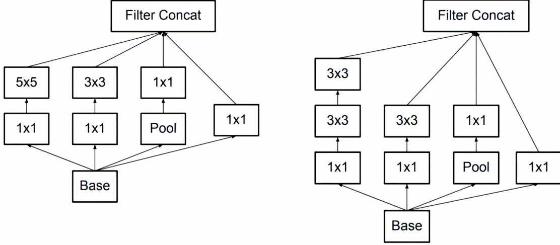
Figure 2.5: Inception model version 1 (left); Inception model version 2 (right) [Szegedy et al. 2016].
