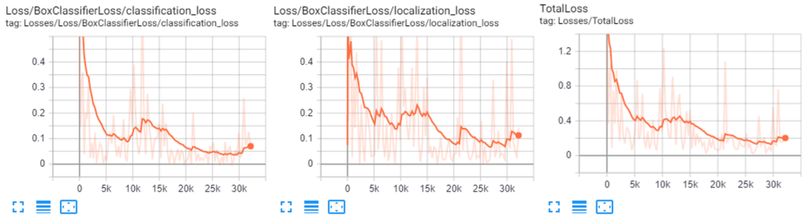
(c) Faster R-CNN Group C Loss Graphs (from left to right) Classification loss, Localisation loss, and Total loss
