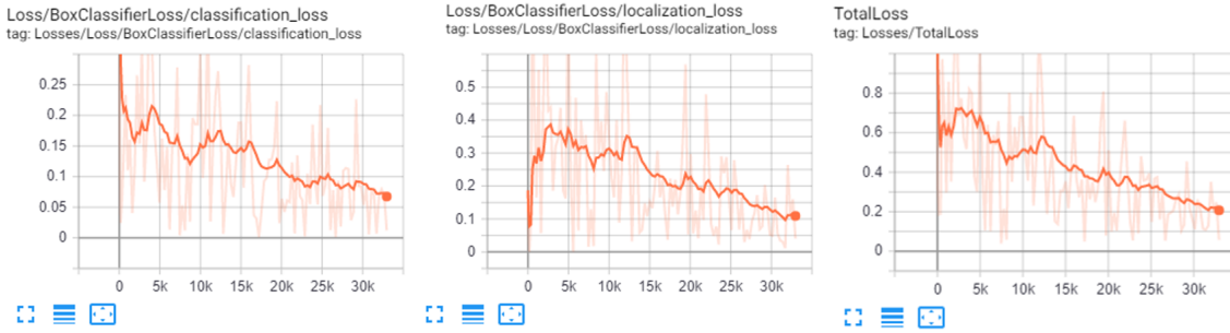
(c) RFCN Group C Loss Graphs (from left to right) Classification loss, Localisation loss, and Total loss
