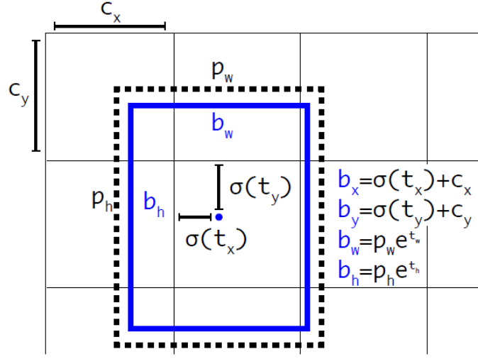
Figure 3.11: Bounding box location predictions [Redmon and Farhadi 2017]
