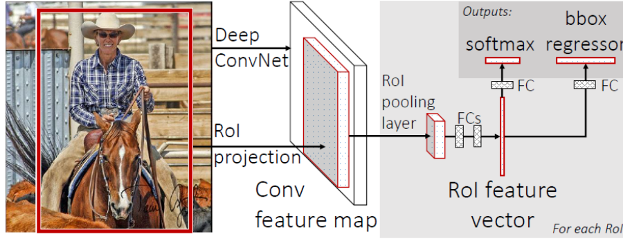
Figure 4.2: Fast R-CNN Architecture [Girshick 2015]
