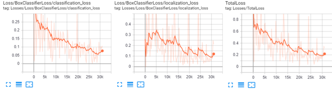
(a) RFCN Group A Loss Graphs (from left to right) Classification loss, Localisation loss, and Total loss
