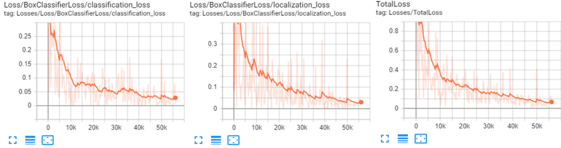
(e) Faster R-CNN Group E Loss Graphs (from left to right) Classification loss, Localisation loss, and Total loss
