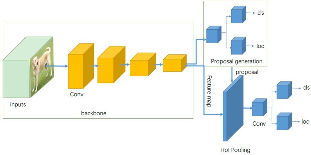
Figure 4.1: Two-stage object detector architecture. Inputs images are fed into a sequence of convolutional layers ( Conv ) represented by the yellow cubes. Feature maps are then generated and passed into the Region Proposal network. The blue cubes represent convolutional layers in this network from which classification ( cls ) and localisation ( loc ) are predicted. [Jiao et al. 2019]
