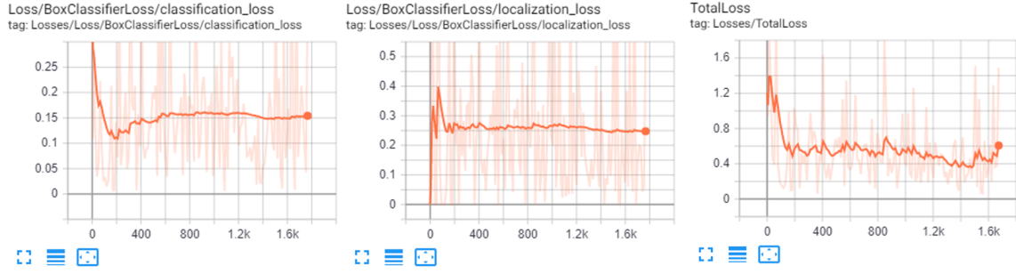
(d) Faster R-CNN Group D Loss Graphs (from left to right) Classification loss, Localisation loss, and Total loss
