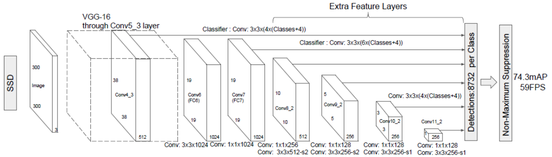
Figure 3.4: SSD structure with an input image of size 300 \times 300 \times 3 [Liu et al. 2016]
