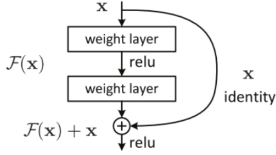
Figure 2.4: Residual Learning - shortcut connection [He et al. 2016].
