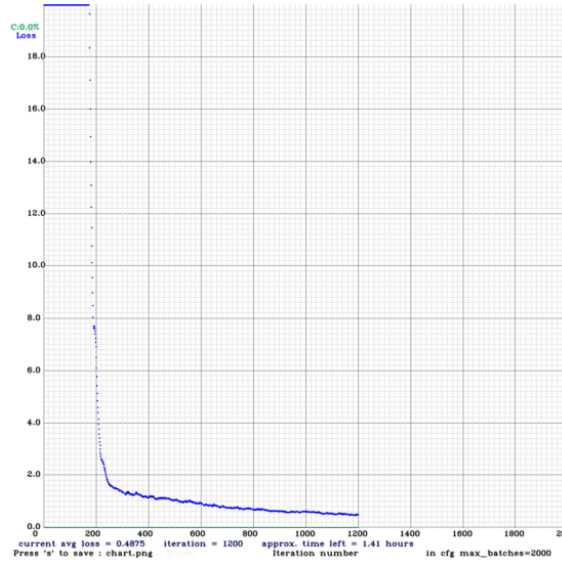
(e) YOLO Group E Loss Graphs
