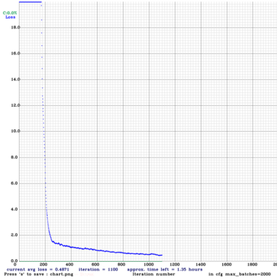
(c) YOLO Group C Loss Graphs
