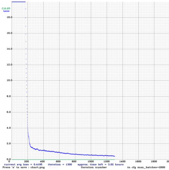
(a) YOLO Group A Loss Graphs
