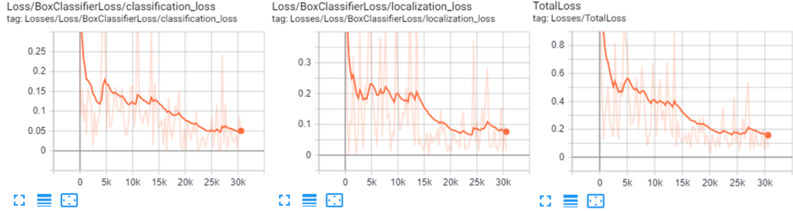
(a) Faster R-CNN Group A Loss Graphs (from left to right) Classification loss, Localisation loss, and Total loss
