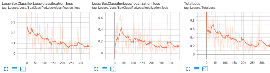
(b) RFCN Group B Loss Graphs (from left to right) Classification loss, Localisation loss, and Total loss
