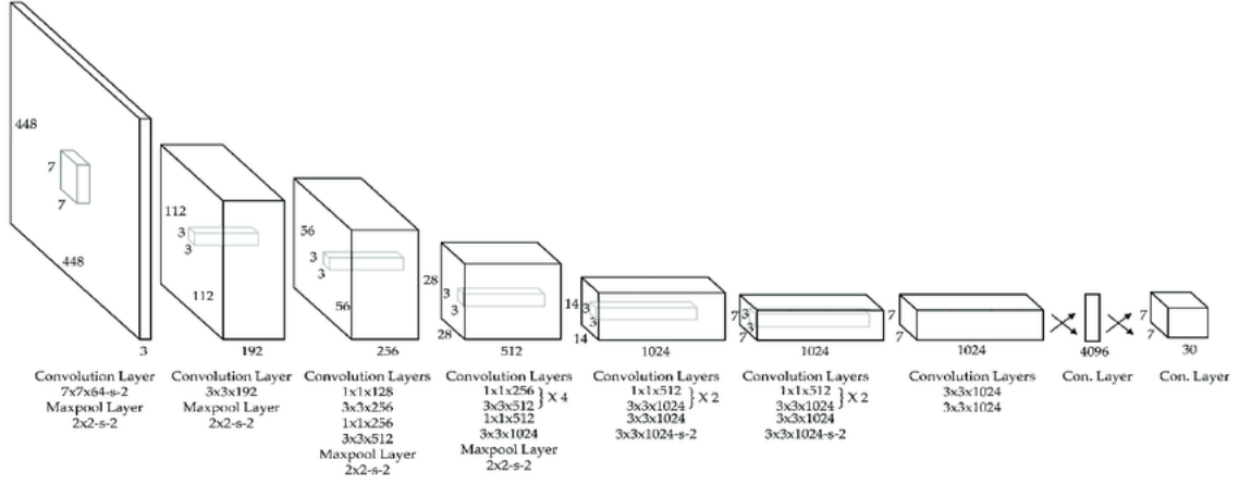
Figure 3.9: YOLO network design [Geethapriya et al. 2019]
