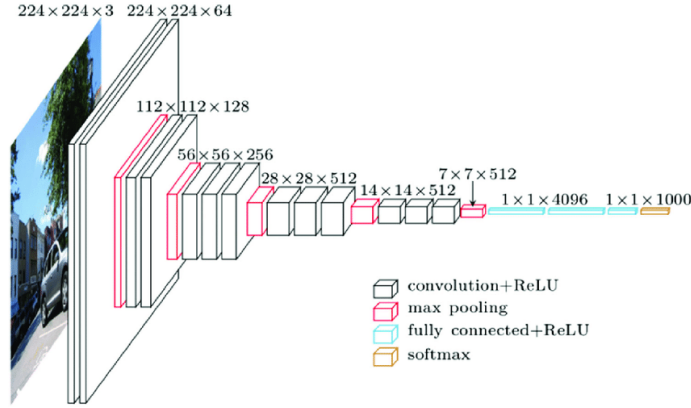
Figure 2.3: VGG16 architectural design [Nash et al. 2018].
