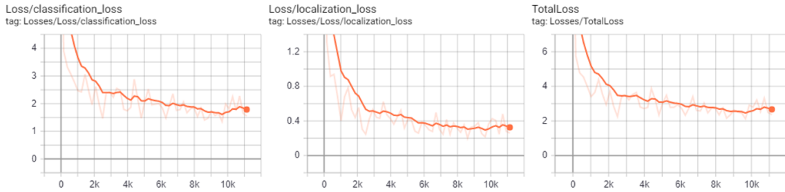
(d) SSD Group D Loss Graphs (from left to right) Classification loss, Localisation loss, and Total loss
