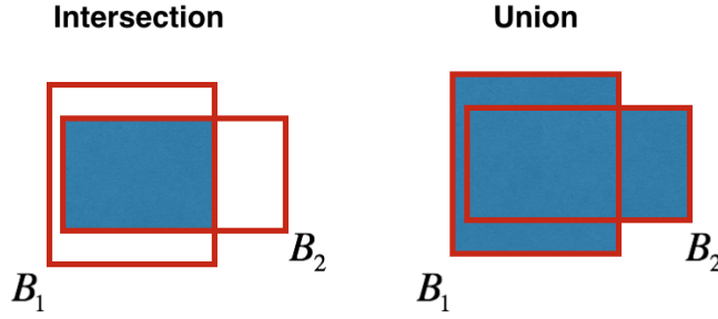
Figure 3.1: Example of B_1 \cap B_2 (left) vs. B_1 \cup B_2 (right)
