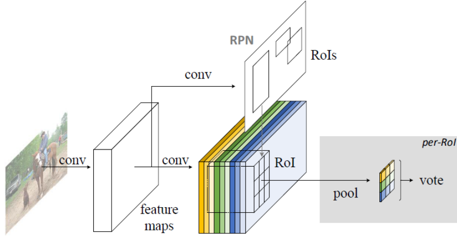
Figure 4.4: Architecture of RFCN from end-to-end [Dai et al. 2016]
