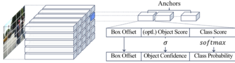
Figure 3.3: Output tensor structure [Noh et al. 2018]
