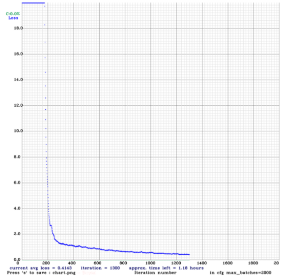
(b) YOLO Group B Loss Graphs
