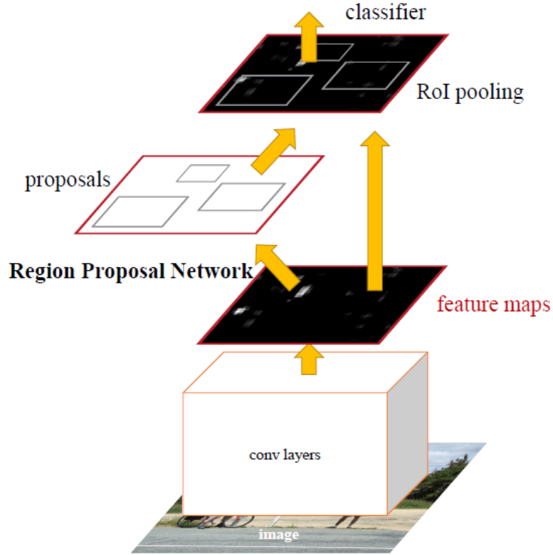
Figure 4.3: Faster R-CNN network consisting of convolutional layers and the RPN [Ren et al. 2015a]
