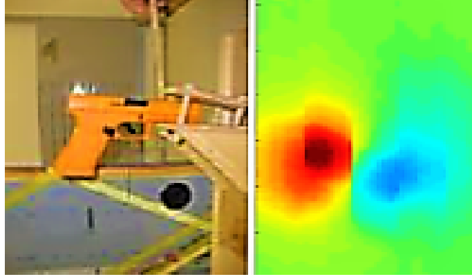
Figure 2.2: Replica-gun sample with equivalent electromagnetic image [Alqubaa and Tian 2012].
