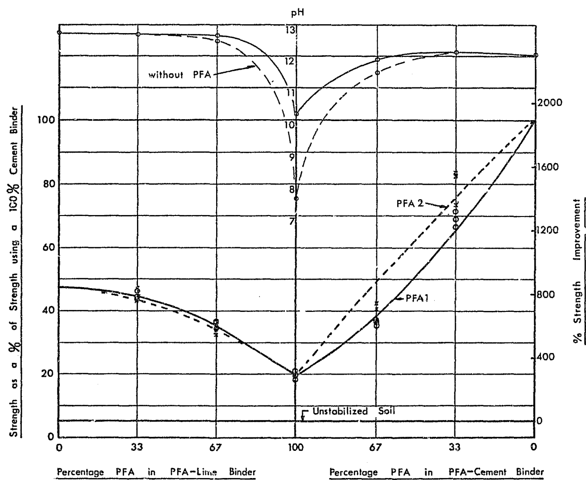
FIG 4.10 Relation between Strength and Binder Composition - SOIL D (Overall binder content = 9%)
