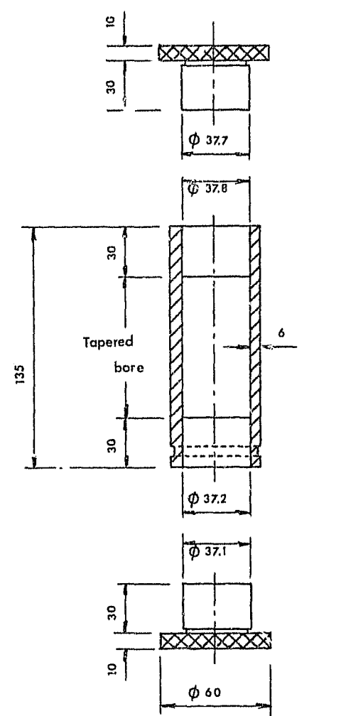
Tapered Cylindrical Mould with End Plugs
