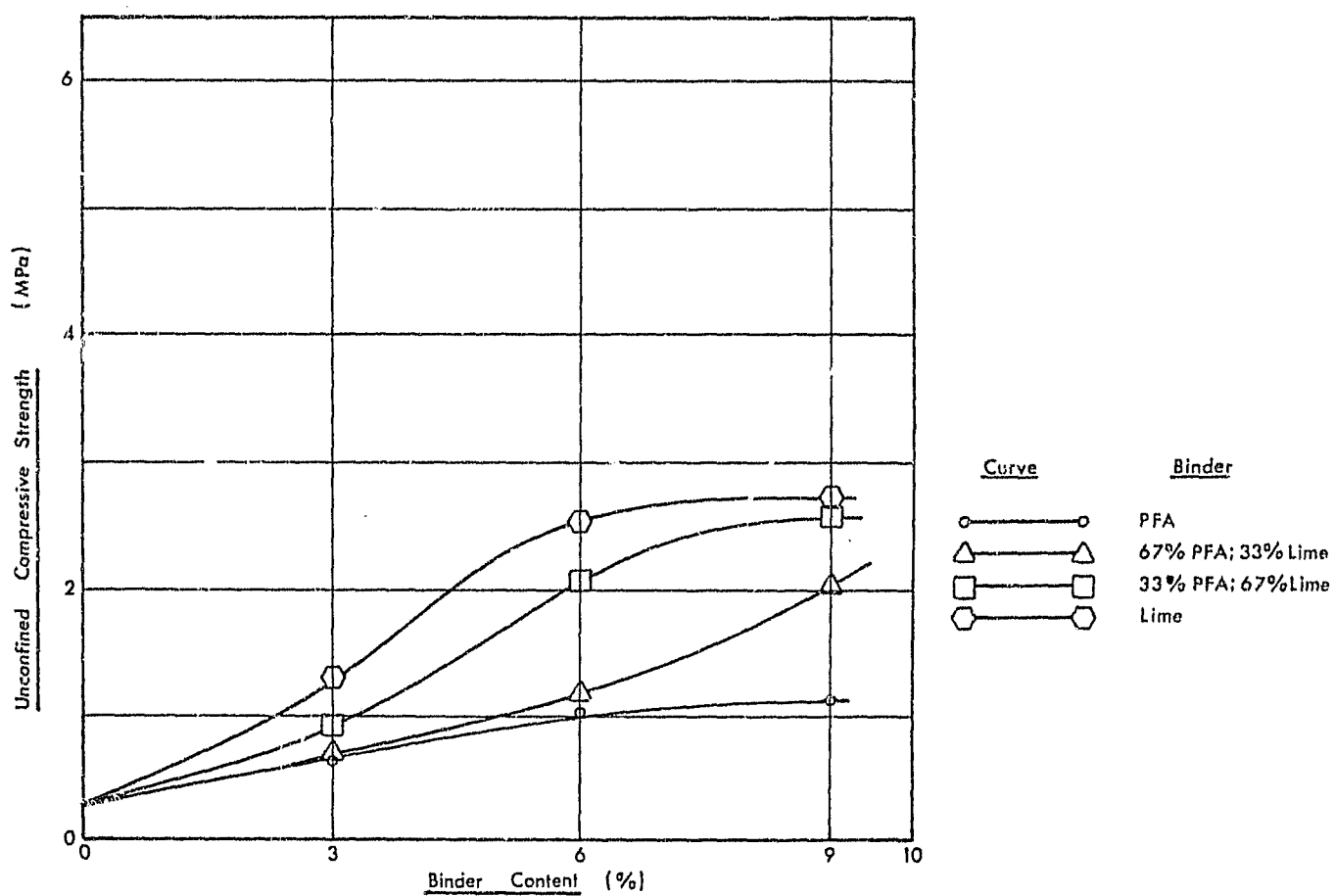
FIG 4.14 The effect of Binder Content on Strength PFA / Lime Binders (Soil D)
