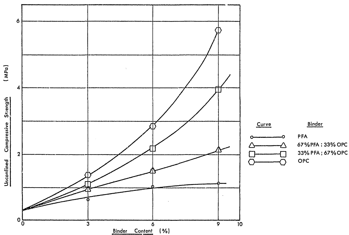
FIG 4.13 The effect of Binder Content on Strength - PFA / OPC Binders (Soil D)
