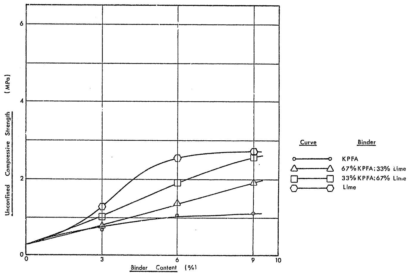
FIG 4.16 The effect of Binder Content on Strength (Soil D) KPFA / Lime Binders
