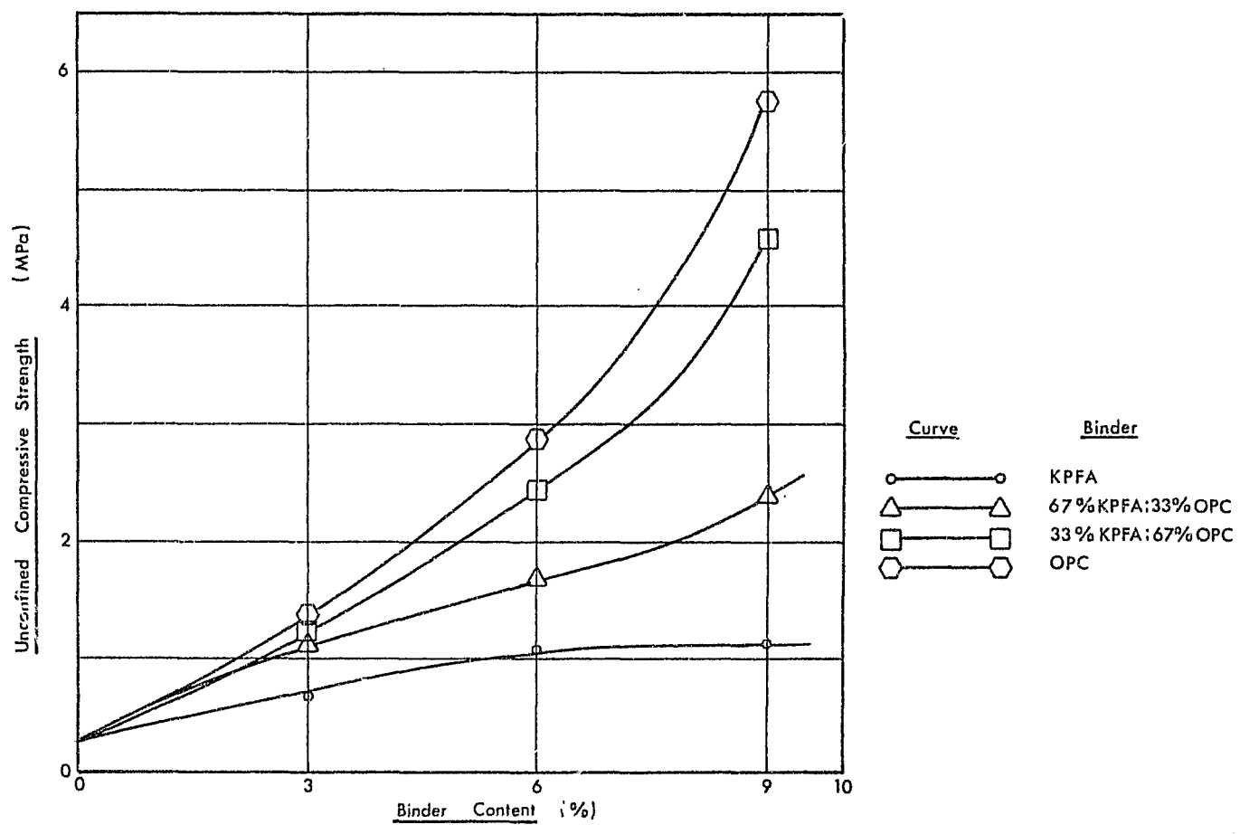
FIG 4.15 The effect of Binder Content on Strength KPFA / OPC Binders (Soil D)
