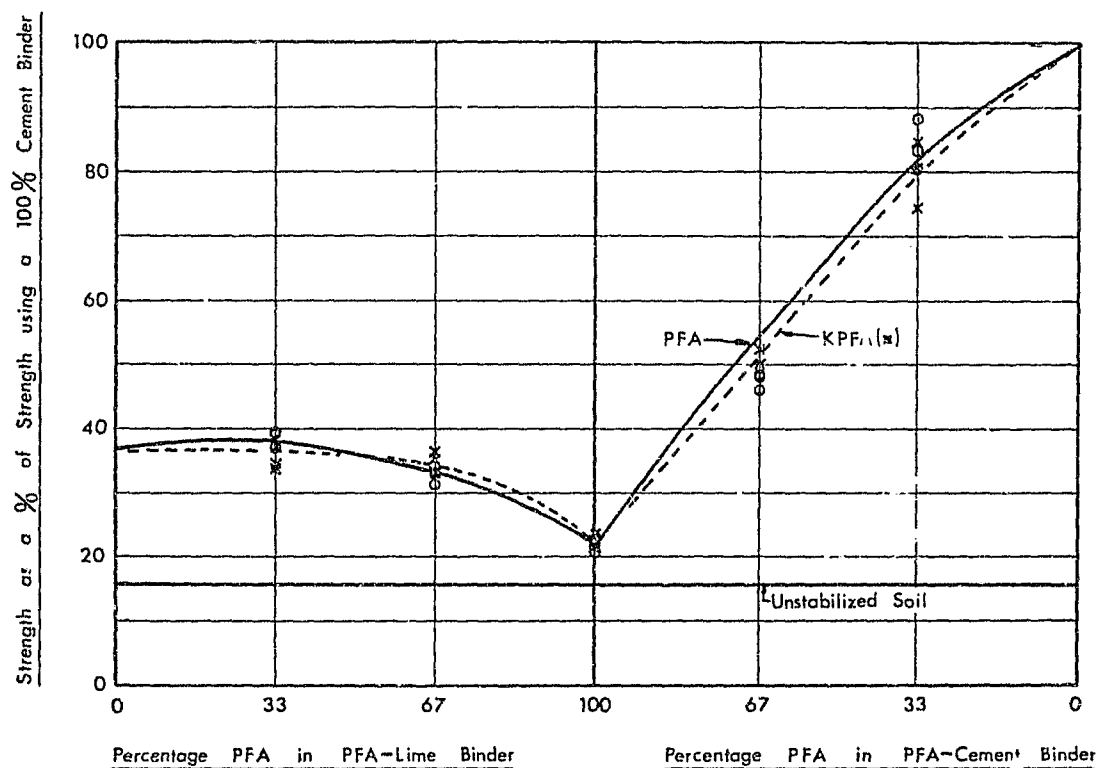
FIG 4.3 Relation between Strength and Binder Composition - SOIL A (Overall binder content = 3%)
