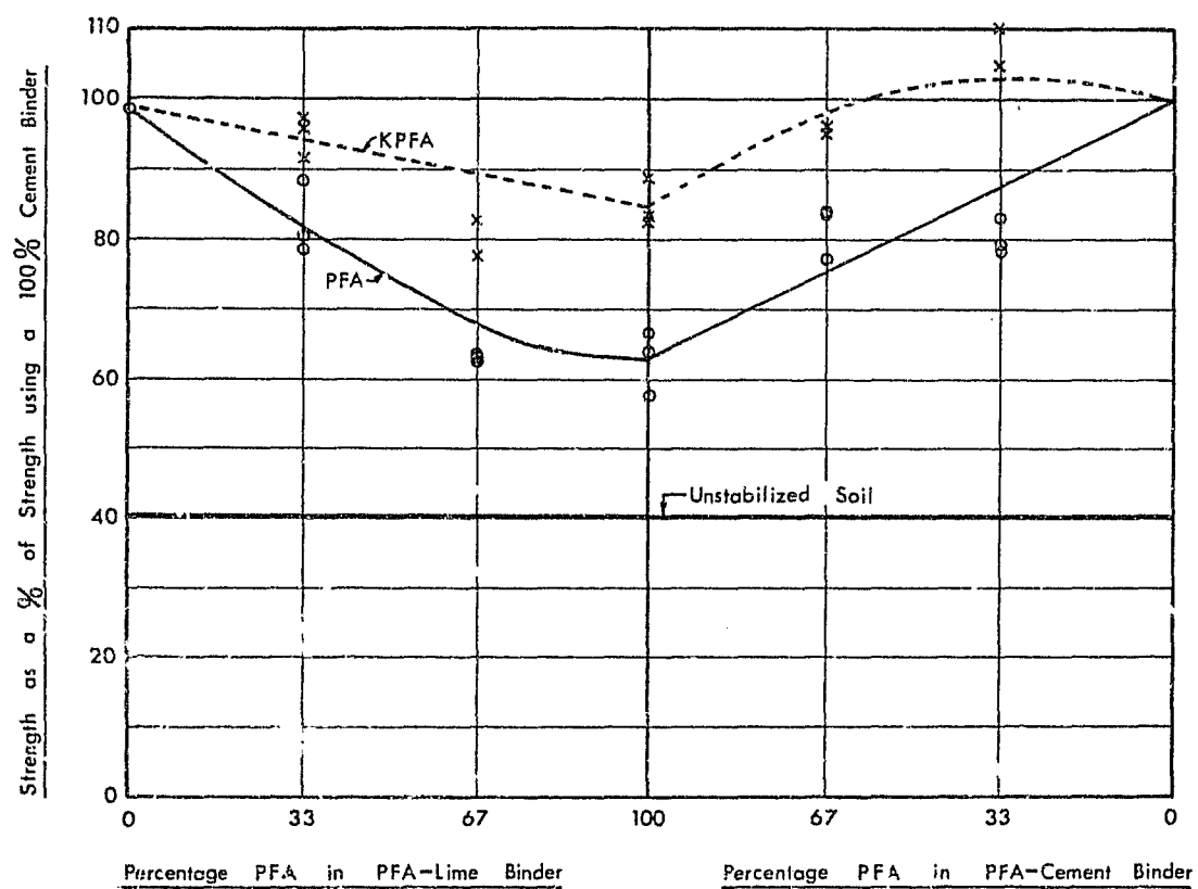
FIG 4.4 Relation between Strength and Binder Composition - SOIL B (Overall binder content = 3%)
