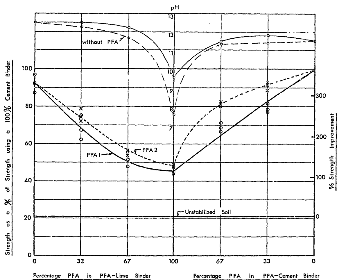
FIG 4.5 Relation between Strength and Binder Composition - SOIL D (Overall binder content = 3%)
