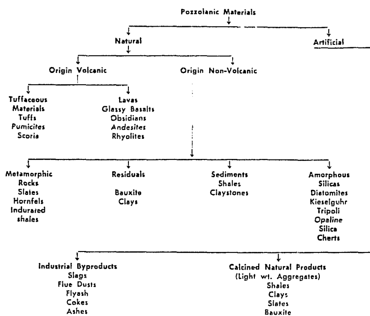
FIG 1.1 Classification of Pozzolans (after Croft 8 )
