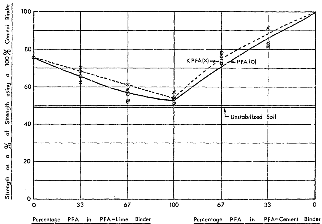
FIG 4.5 Relation between Strength and Binder Composition - SOIL C (Overall binder content = 3%)
