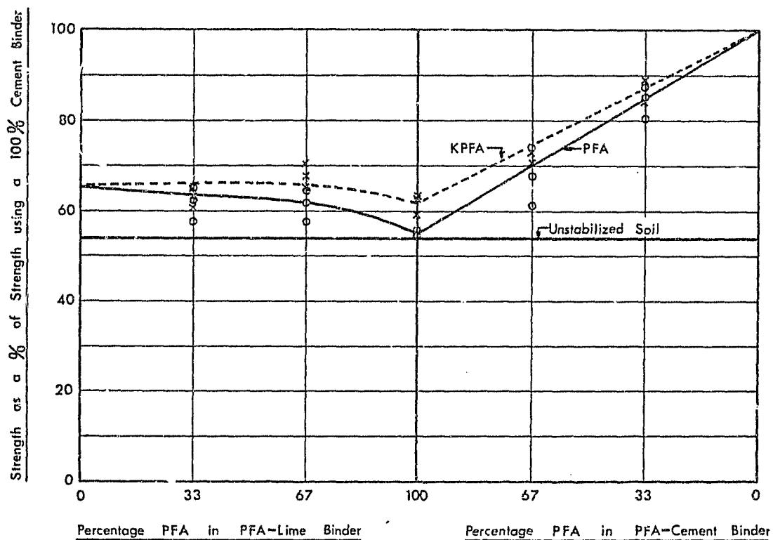
FIG 4.7 Relation between Strength and Binder Composition - SOIL E (Overall binder content = 3%)
