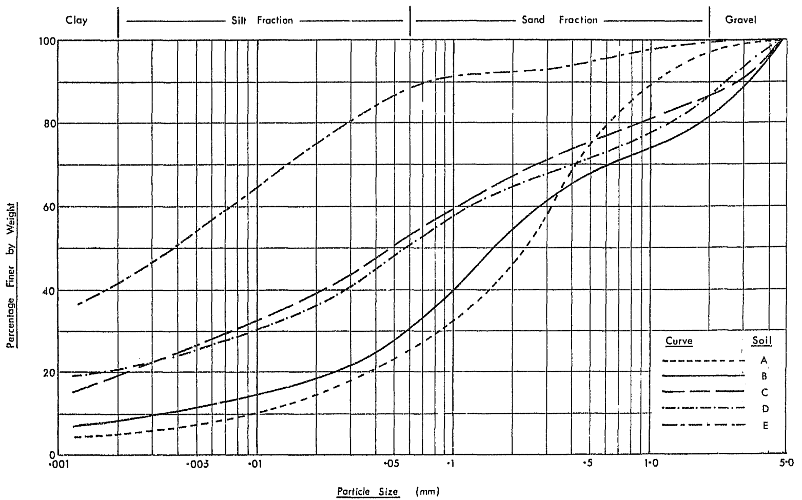
FIG 2.1 Grading curves for the Soils
