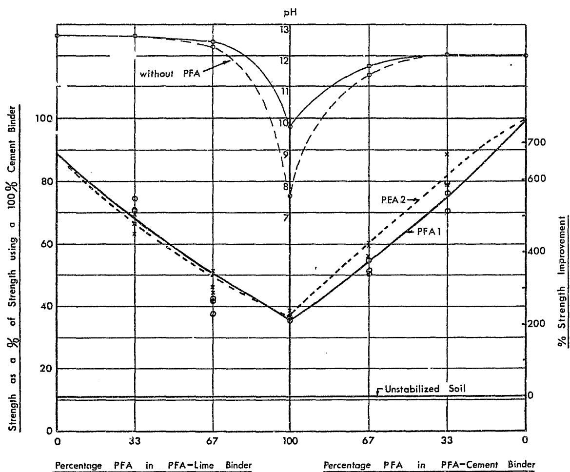
FIG 4.9 Relation between Strength and Binder Composition - SOIL D (Overall binder content = 6%)
