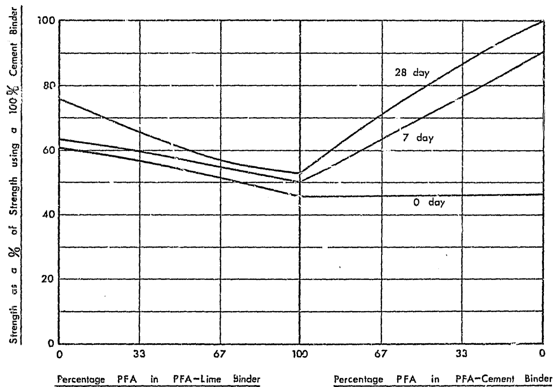
FIG 4.8 Relation between Strength and Binder Composition - SOIL C (Overall binder content = 3%)
