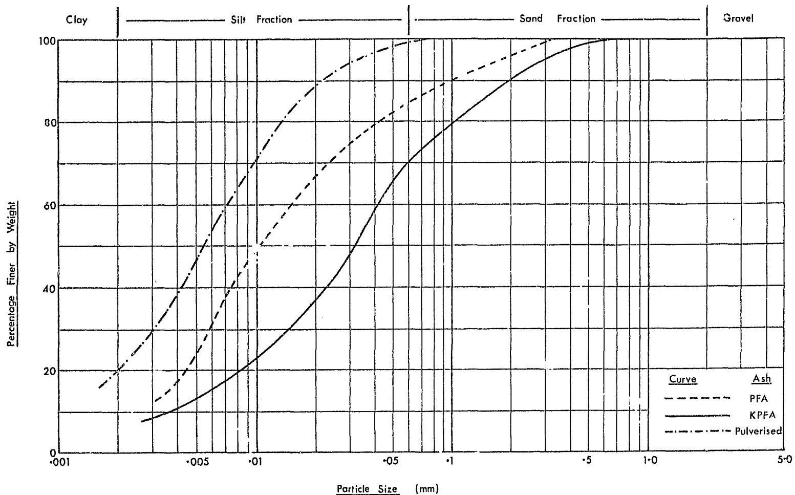
FIG 3.1 Grading curves for the Ashes
