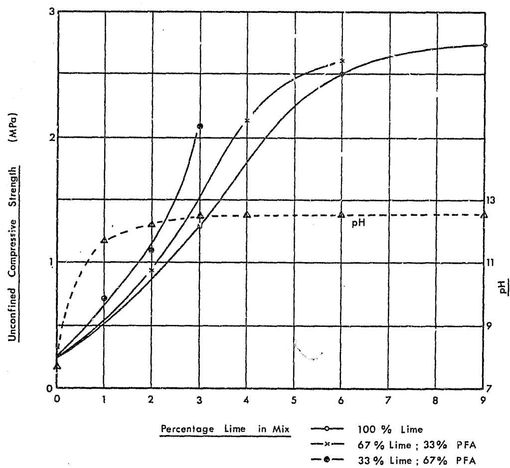
FIG 4.17 The effect of Lime Content on Strength
