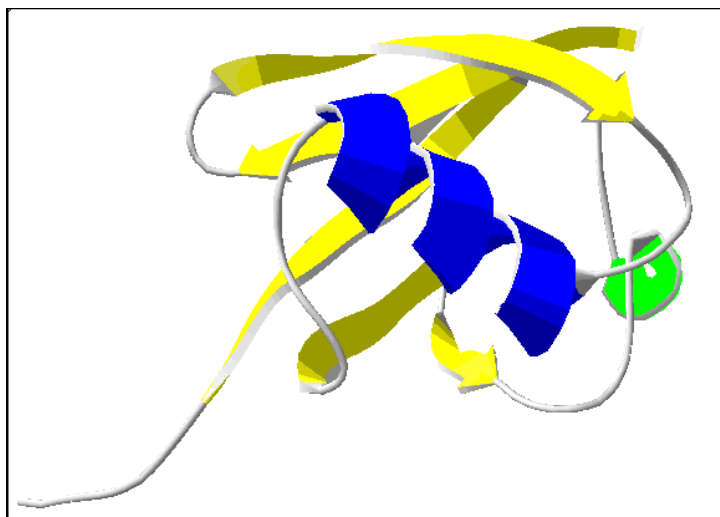
Figure 8. The native structure of ubiquitin. Ubiquitin consists of three and a half turns of \alpha -helix (blue), a short piece of 3_{10} -helix (green), seven reverse turns (white strands), and a five stranded mixed \beta -sheet (yellow), (Vijay-Kumar et al., 1987).
