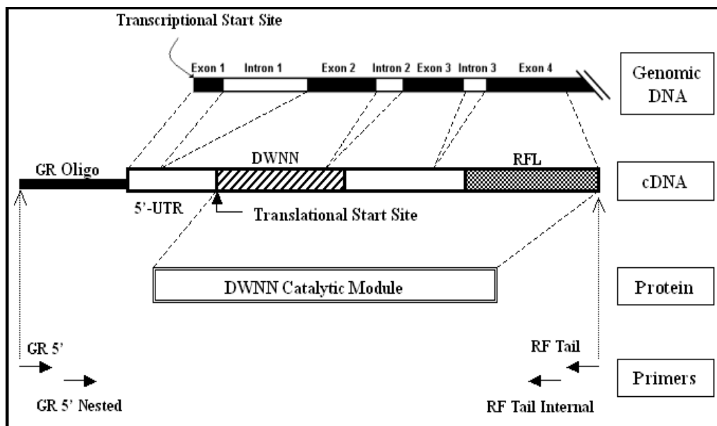
Figure 13. The 5' region of the SNAMA gene that is ultimately translated into the DWNN catalytic module. The GeneRacer™ (GR) oligo along with primers used during transcriptional start site determination are also shown.
