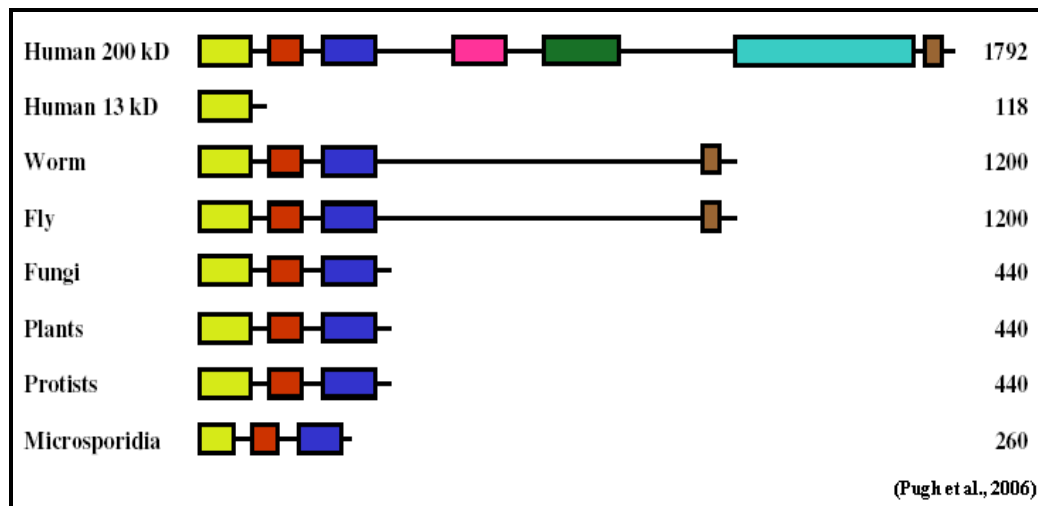
Figure 5. The domain structure of the RbBP6 family of proteins. The highly conserved DCM of the RbBP6 superfamily is shown by the DWNN domain (yellow), zinc finger motif (red) and RING finger motif (blue). Both the DCM and DWNN domain are expressed as individual polypeptides. Human RbBP6 contains additional domains that include the Rb-binding domain (green) and p53-binding domain (light blue) (Pugh et al., 2006).
