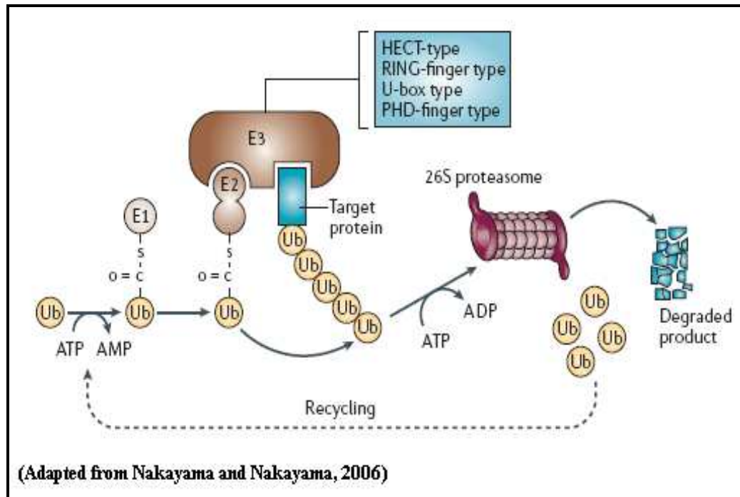
Figure 9. Degradation of proteins via the ubiquitin-proteasome pathway. Ubiquitin is transferred to the ubiquitin activating enzyme (E1) in an ATP-dependent manner. The ubiquitin is then transferred to an ubiquitin conjugating enzyme (E2). The ubiquitin ligase binds both the E2 and the target protein, thus allowing for the covalent attachment of the ubiquitin molecule to the target protein. Ubiquitin molecules are then added in succession until a chain of 4 or more residues is reached, at which point the target protein is transported to the 26S proteasome for degradation.
