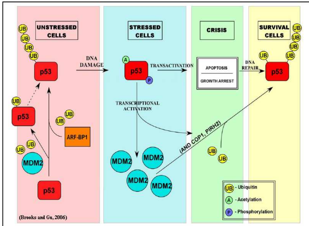
Figure 3. Regulation of p53 and Mdm2 during cell survival and apoptosis. In normal cells under no stress, extremely low levels of p53 are evident due to ubiquitination and degradation of p53 by E3 specific ligases such as Mdm2. Upon cell stress through DNA damage, p53 becomes stabilized and activated by post-translational modifications (Brooks and Gu, 2006).
