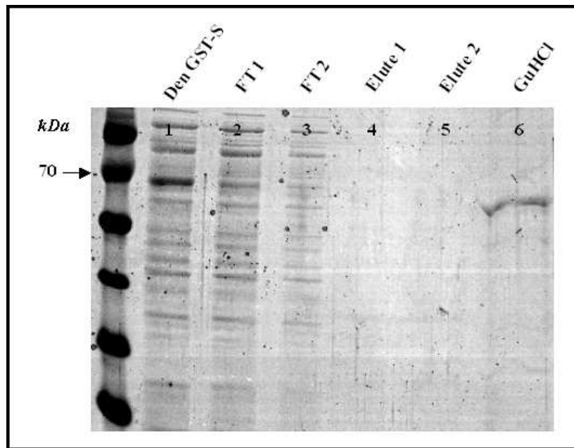
Figure 15. His-tag purification of denatured recombinant SNAMA protein. Denatured SNAMA protein was present amongst contaminating protein (lane 1). Ni +2 affinity chromatography under denaturing conditions was performed as described in the manufacturers protocol. Pure GST-SNAMA fusion protein was unexpectedly eluted using GuHCl (lane 6) rather than elution buffer in the step before (lanes 4 and 5). Note that the GST-SNAMA fusion protein appears smaller in size due to the gel being scewed.
