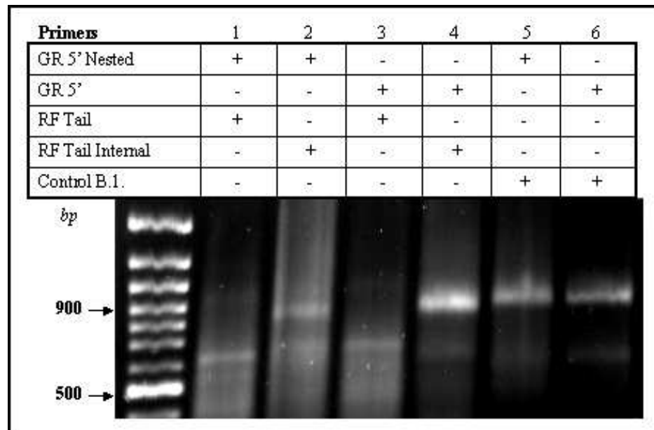
Figure 10. 5' Rapid amplification of cDNA ends using Drosophila RNA. Two distinct fragments of different size were amplified when 5' RACE was performed on Drosophila RNA from adults. The smaller fragment was between 650 and 700 bp in size while the larger was between 800 and 850 bp. Different combinations of primers resulted in slight variations in DNA fragment size and band intensities. A positive control using HeLa RNA and the Control B.1 primer resulted in the amplification of a fragment approximately 900 bp in size as expected (lanes 5 and 6).
