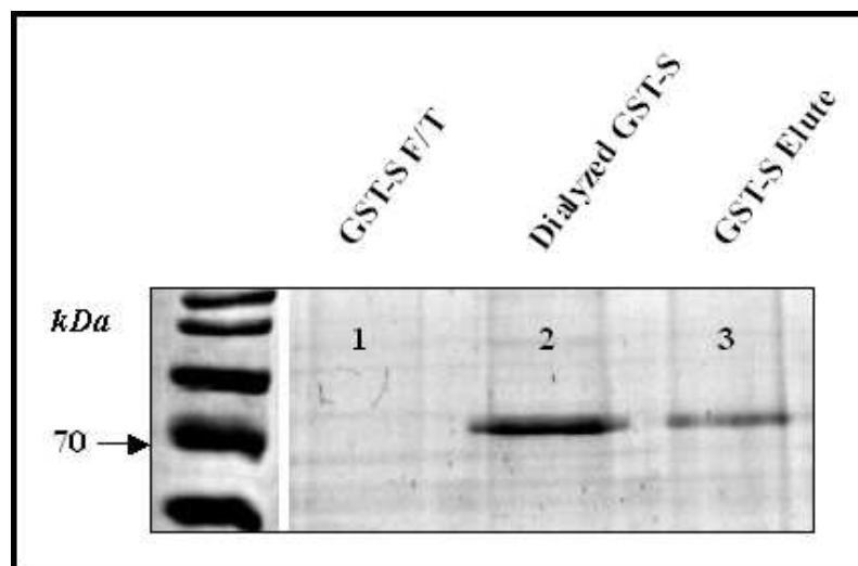
Figure 18. Glutathione affinity chromatography of refolded GST-S protein. The GST-S protein was eluted during the elution wash using glutathione (lane 3), with no protein present in the flow through wash (lane 1). The dialyzed GST-S protein sample prior to loading onto the glutathione agarose column can be seen in lane 2.
