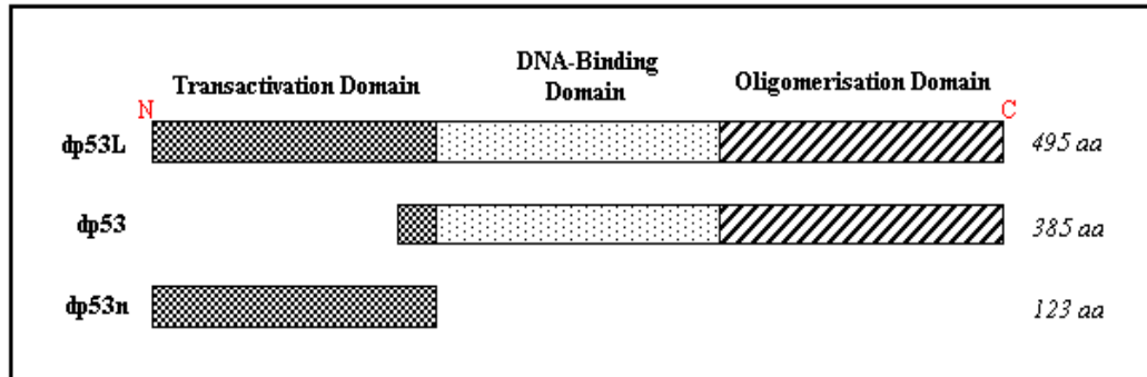
Figure 2. Drosophila melanogaster p53 isoforms: dp53L, dp53, and dp53n. dp53 is a N-terminally truncated isoform of an internal promoter and is identical to that first published. dp53L is initiated at exon A, 580 bp upstream of the internal promoter, and contains the conserved N-terminal domain FxxψW. This domain is not found within dp53 and is required to activate gene transcription. The third isoform, dp53n, is a splice variant of dp53L with no slicing of intron B (Bourdon et al., 2005).
