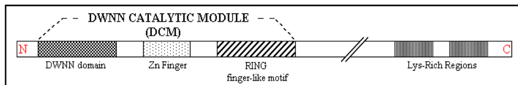
Figure 4. Schematic representation of the Drosophila SNAMA protein. SNAMA contains a highly conserved N-terminal region known as the DWNN Catalytic Module (DCM) encompassing a DWNN domain, Zn finger, and RING finger-like motif.
