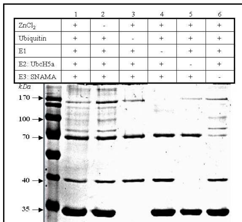
Figure 21. The dependence of SNAMA E3 activity on key ubiquitination factors. Ubiquitin conjugation assays using SNAMA E3 were performed in the absence of each of the key players involved in ubiquitination including E1, E2, ubiquitin, or zinc ions. Ubiquitination does not occur in the absence of ubiquitin, E1 or E2 (lanes 3, 4 and 5 respectively). However, ubiquitination takes place in the absence of zinc ions (lane 2). Poly-ubiquitin chains of 2 to 3 molecules and the Ubc5a-Ub complex still form in the absence of the E3 (SNAMA) as is indicated by the three additional peptides of approximately 70 kDa, 75 kDa, and 100 kDa (lane 6).
