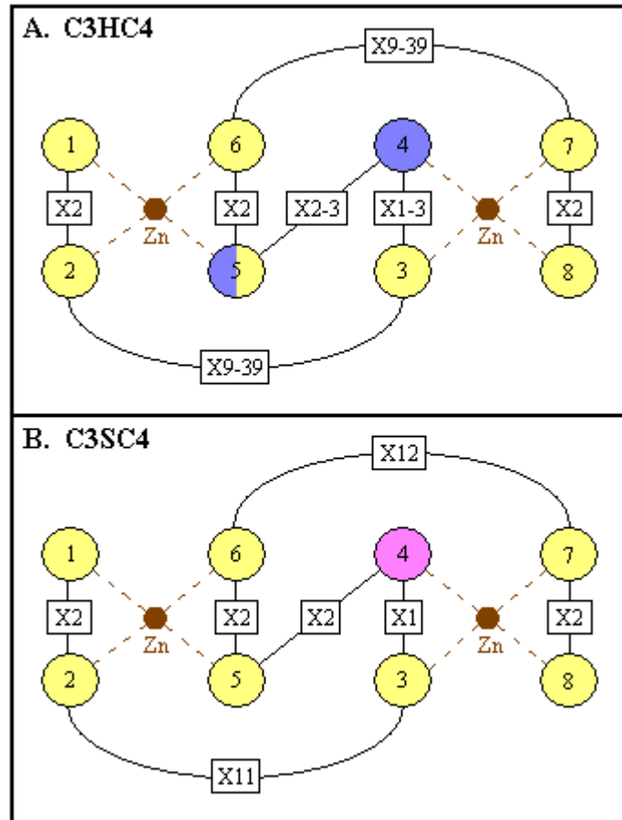
Figure 7. The “cross-brace” structure of RING finger motifs. (A) The classical C3HC4 RING finger, where two zinc ions are co-ordinated by cysteine residues (yellow spheres) and a histidine residue (blue sphere). (B) The uncharacteristic C3SC4 RING finger-like motif found within the DCM of SNAMA. Two zinc ions are co-ordinated by cysteine residues and a serine residue (pink sphere), (Mather et al., 2005).
