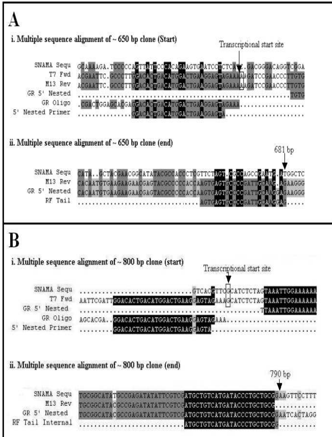
Figure 12. Multiple sequence alignment of cloned 5' RACE products. (A) Alignment of the 650-700 bp clone shows a fragment 681 bp in size that does not have a significant alignment with the SNAMA sequence. In contrast, the alignment shows that the RF Tail primer binds completely to the fragment. (B) Alignment of the 800-850 bp clone shows a fragment of 790 bp that aligns completely with SNAMA and the RF Tail primer.
