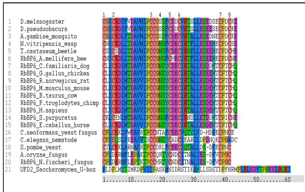
Figure 23. Multiple alignment of RING finger motifs from the RbBP6 superfamily. Orthologues of the SNAMA RFL motif were generated from the BlastP bioinformatic tool followed by alignment of the sequences using ClustalX. The conserved cysteine residues involved in the formation of the cross-brace structure of the RING finger are numbered at the top of the sequences. The conserved histidine in the fourth ligand has been substituted in all the RFL motifs of the RbBP6 family of protein. The classical U-box protein, Ufd2, was also included in the alignment.
