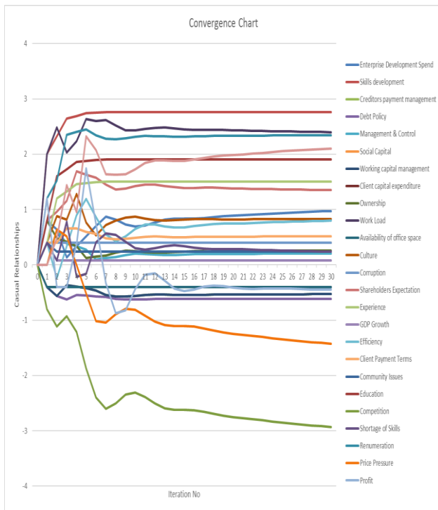
Figure 10: FCM Convergence Charts
