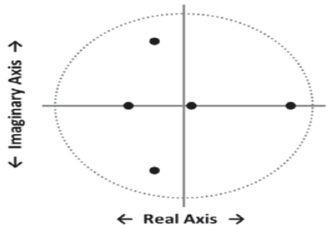
Figure 5 : Eigenvalues of a stable system (Stacey, 2016)
