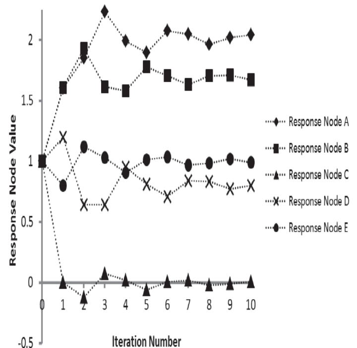
Figure 6 : FCM Simulation of a stable system (Stacey, 2016)
