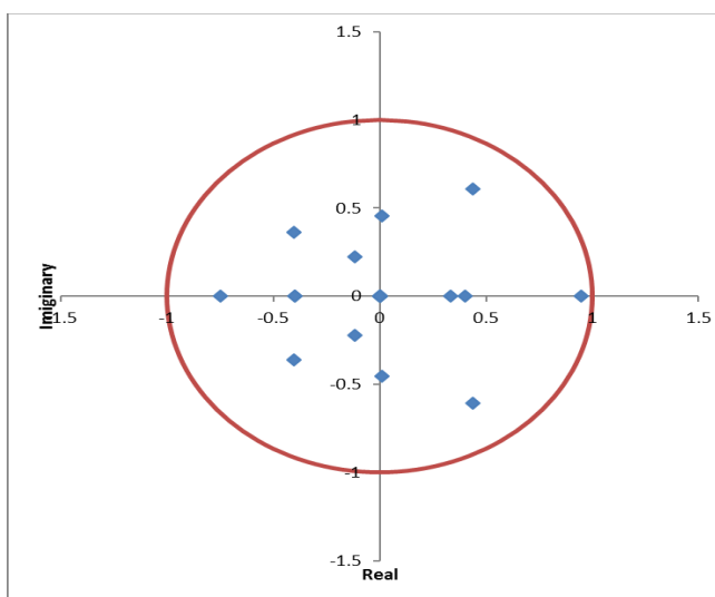
Figure 11 : Argand diagram of eigenvalues
