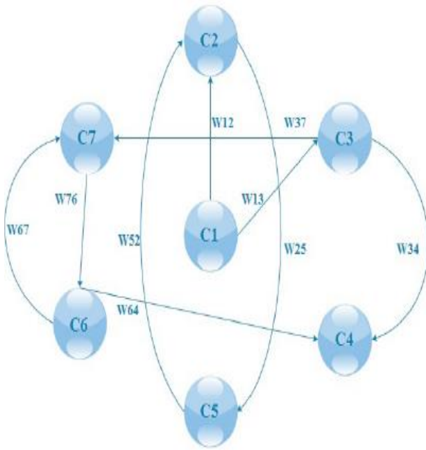
Figure 1: Simple Fuzzy Cognitive Map (Vergini & Groumpos, 2016)
