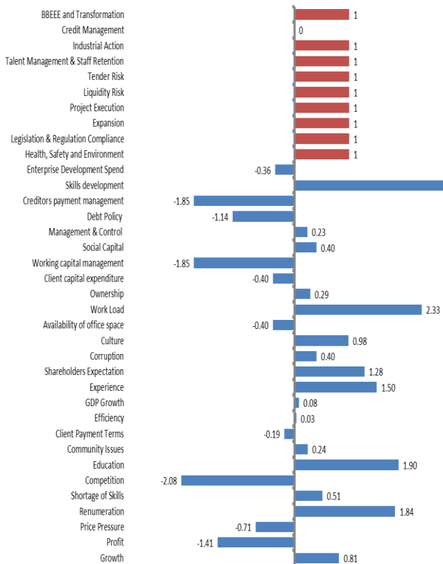
Figure 13: Scenario 3 – Credit Management switched inactive (0)
