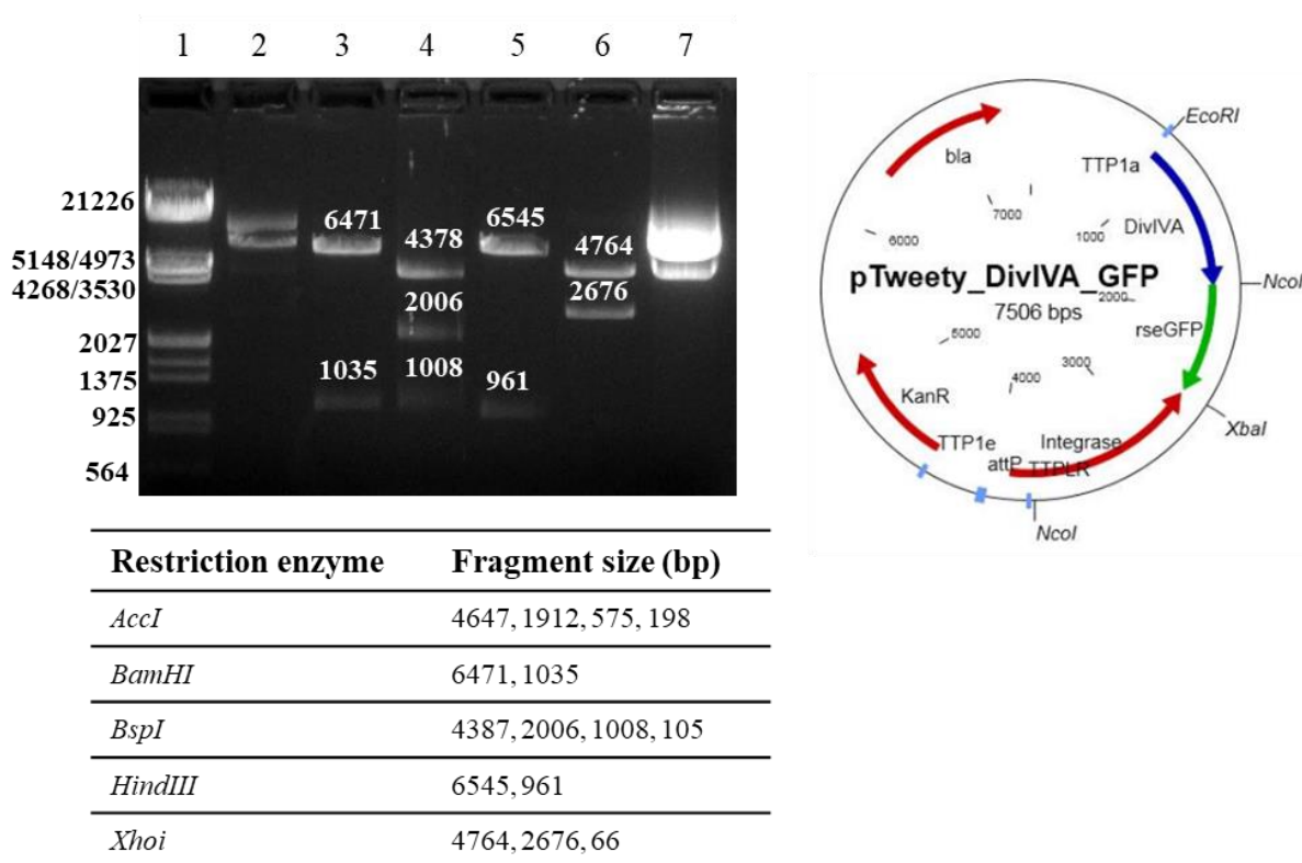
Figure 3.3.5. PTweety_DivIV_GFP restriction mapping to confirm plasmid integrity. 1- Molecular weight marker III, 2- AccI , 3- BamHI , 4- BspHI , 5- HindIII , 6- XhoI , 7-uncut plasmid. With the exception of AccI , all restriction enzymes produced expected band sizes. It appeared that AccI did not cut the DNA.
