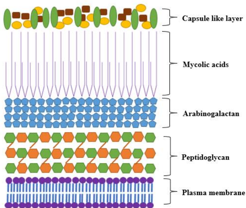
Figure 1.4. Schematic diagram representing the mycobacterial cell wall. Green oval shapes represent capsule proteins; yellow and brown represent capsule polysaccharides. Branch-like structures in pink represent mycolic acids, and blue pentagons represent arabinogalactan. Green and orange hexagons represent the N -acetylglucosamine and N -acetylmuramic acid components of the PG respectively. The orange lines represent the crosslinks between PG residues, and the purple circle and blue lines represent the phospholipid bilayer of the plasma membrane. Adapted from Squeglia et al. (2018).
