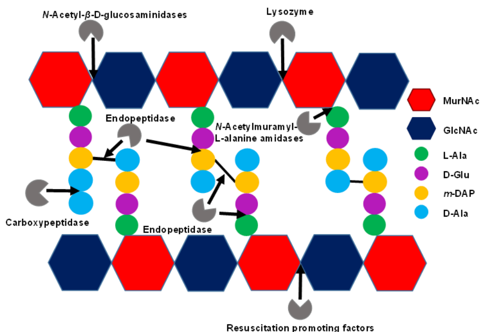
Figure 1.9. Various PG hydrolases and their cleavage locations on the PG molecule. Image adapted from Vollmer et al. (2008).
