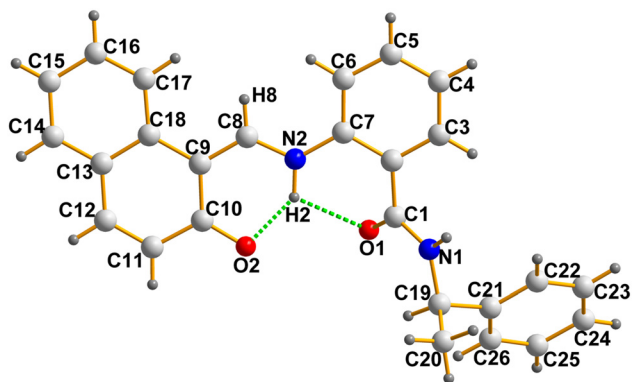
Figure 4: The structure of the (R) -sirtinol molecule.
