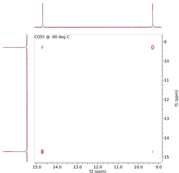
Figure 3: COSY correlation between 14.72 and 9.30 ppm at -90^{\circ}\text{C} .
