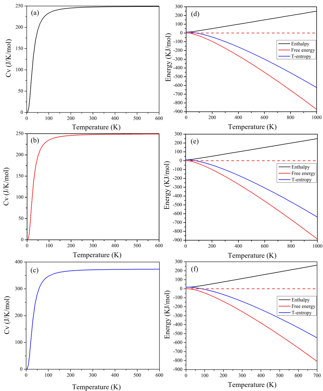
Figure 6.14: Temperature dependence of heat capacity of (a) \text{Cs}_2\text{Pb}_2\text{I}_3\text{Br}_3 , (b) \text{Cs}_2\text{Pb}_2\text{I}_5\text{Br} and (c) \text{Cs}_3\text{Pb}_3\text{IBr}_8 perovskites and their (d) - (e) enthalpy, temperature entropy, and free energy.
