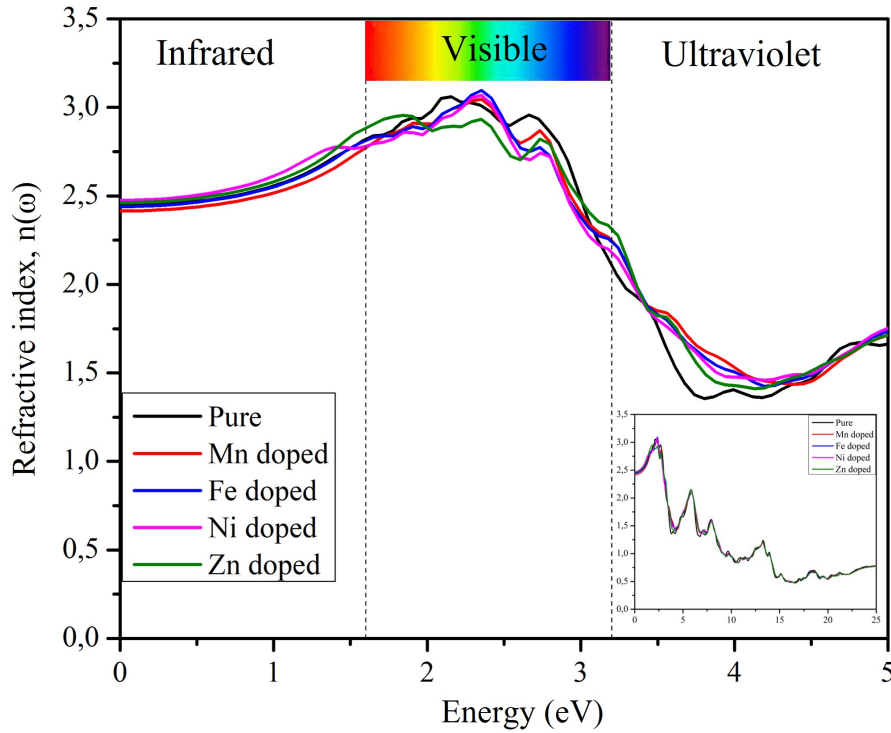
Figure 5.7: The calculated refractive index, n(\omega) for the undoped CsPbI 3 and TM doped perovskites.
