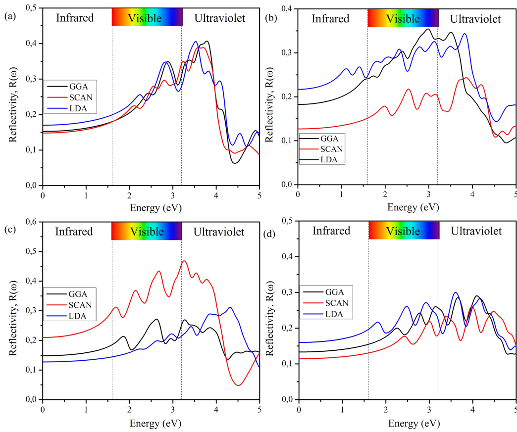
Figure 4.8: Calculated reflectivity R(\omega) of (a) \text{CsPbI}_3 , (b) \text{CsPbI}_2\text{Br} , (c) \text{CsPbIBr}_2 and (d) \text{CsPbBr}_3 compounds obtained using LDA, GGA-PBE and SCAN meta-GGA.
