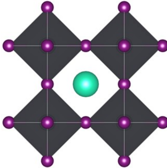
Figure 4.1: The constructed cubic polyhedron crystal structure of CsPbI 3 . The perovskites CsPbI 2 Br, CsPbIBr 2 , and CsPbBr 3 were constructed by replacing the I - ion with the Br - ion.
