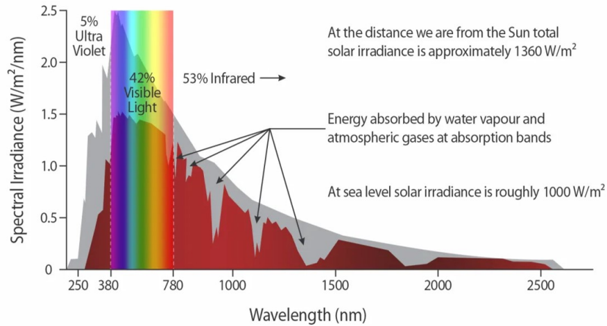
Figure 2.5: The solar radiation spectrum versus wavelength [38].
