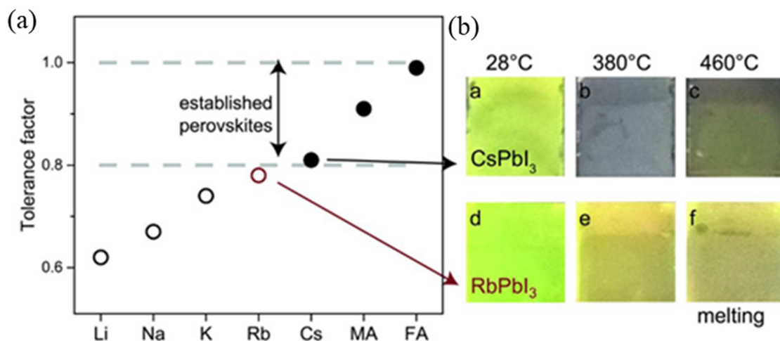
Figure 2.3: (a) The tolerance factor and different melting temperature of CsPbI 3 (○) and RbPbI 3 perovskites [46].
