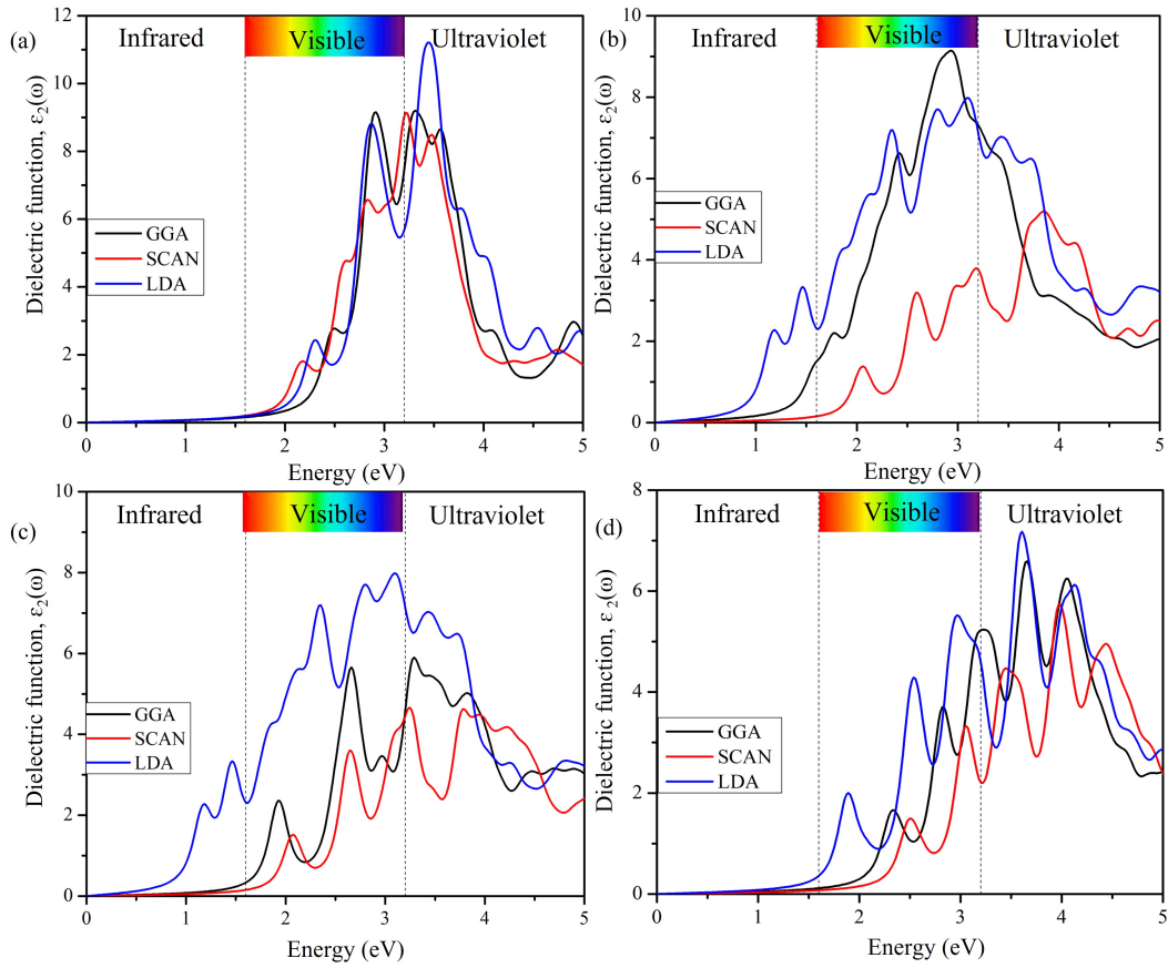
Figure 4.5: Calculated imaginary dielectric function \epsilon_2(\omega) of (a) \text{CsPbI}_3 , (b) \text{CsPbI}_2\text{Br} , (c) \text{CsPbIBr}_2 and (d) \text{CsPbBr}_3 compounds obtained using LDA, GGA-PBE and SCAN meta-GGA.
