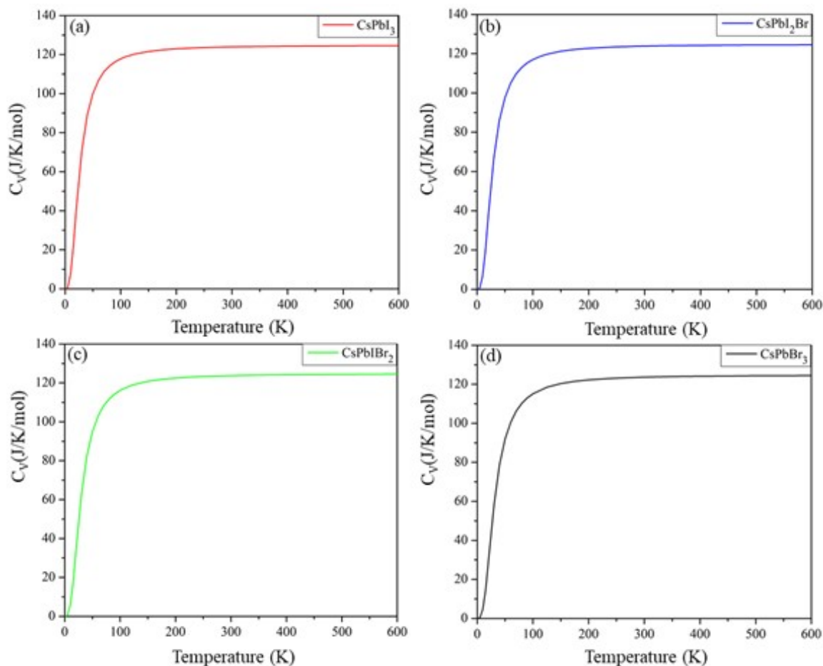
Figure 4.11: Temperature dependence of heat capacity of (a) \text{CsPbI}_3 , (b) \text{CsPbI}_2\text{Br} , (c) \text{CsPbBr}_2\text{I} and (d) \text{CsPbBr}_3 perovskites obtained using GGA-PBE and LDA the functionals.
