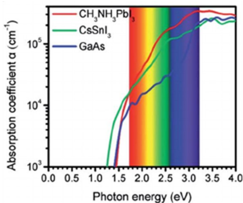
Figure 2.4: Optical absorption coefficient comparison for \text{CH}_3\text{NH}_3\text{PbI}_3 , \text{CsSnI}_3 and GaAs solar cell materials [52].
