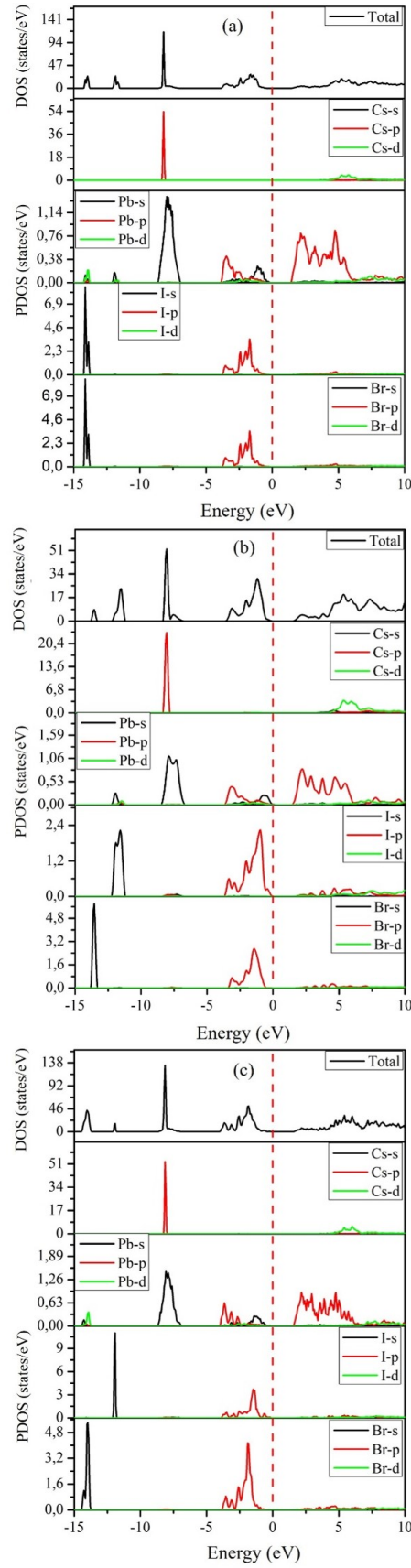
Figure 6.6: The calculated total and partial density of states for the predicted structures (a) \text{Cs}_2\text{Pb}_2\text{I}_3\text{Br}_3 , (b) \text{Cs}_2\text{Pb}_2\text{I}_5\text{Br} and (c) \text{Cs}_3\text{Pb}_3\text{IBr}_8 .
