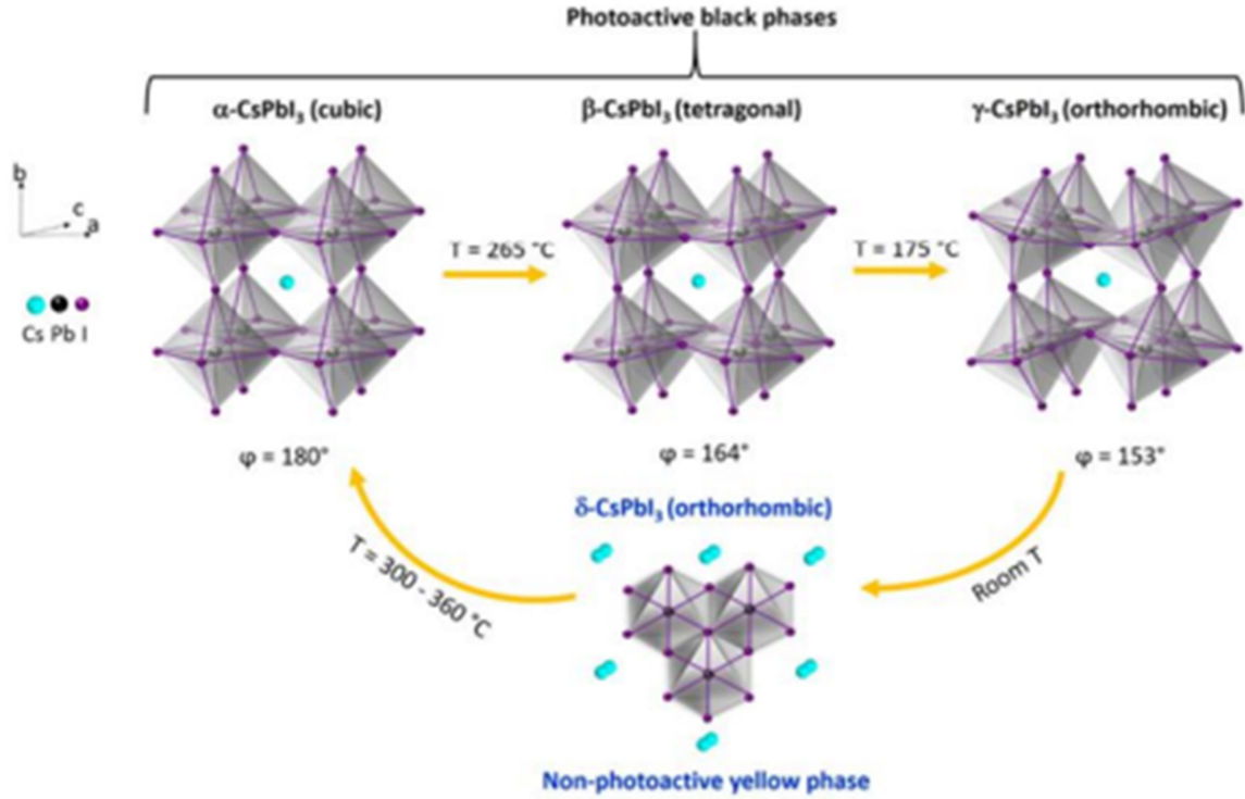
Figure 2.2: Schematic illustration of crystalline structure of \text{CsPbI}_3 and its polymorphic phase transition [37].
