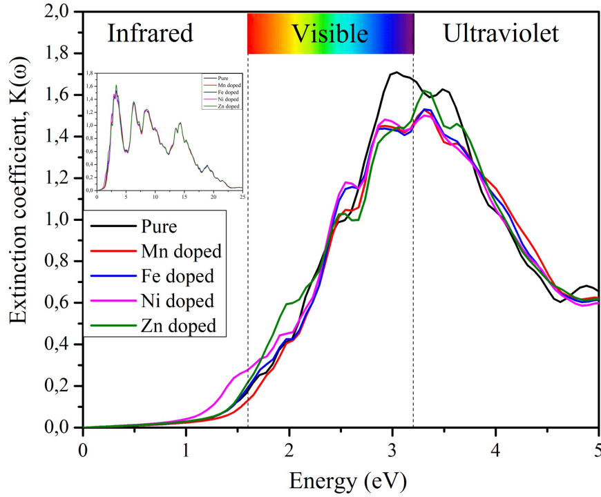
Figure 5.8: The calculated extinction coefficient of undoped \text{CsPbI}_3 and TM doped perovskites
