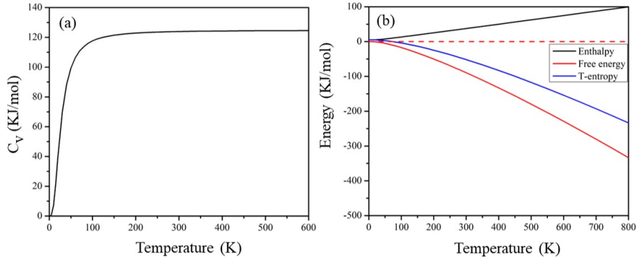
Figure 5.12: The calculated heat capacity, enthalpy, entropy and free energy against temperature for \text{CsPbI}_3 perovskite.
