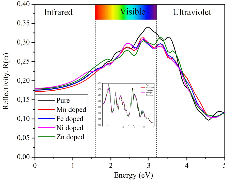
Figure 5.9: The calculated reflectivity, R(\omega) of undoped CsPbI 3 and TM doped perovskites.
