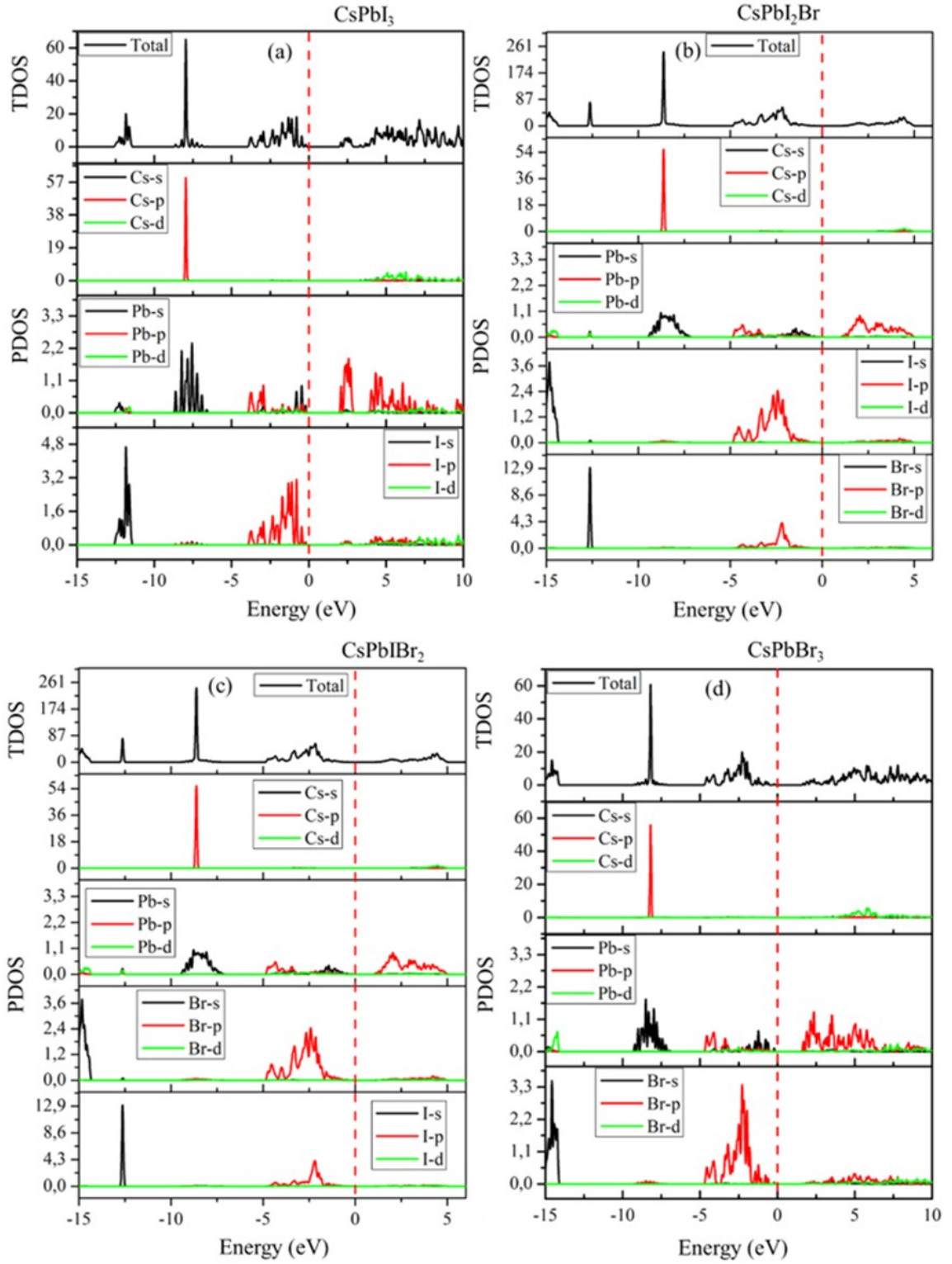
Figure A.2: Total and partial density of states for (a) CsPbI 3 , (b) CsPbI 2 Br, (c) CsPbIBr 2 and (d) CsPbBr 3 perovskites using LDA.
