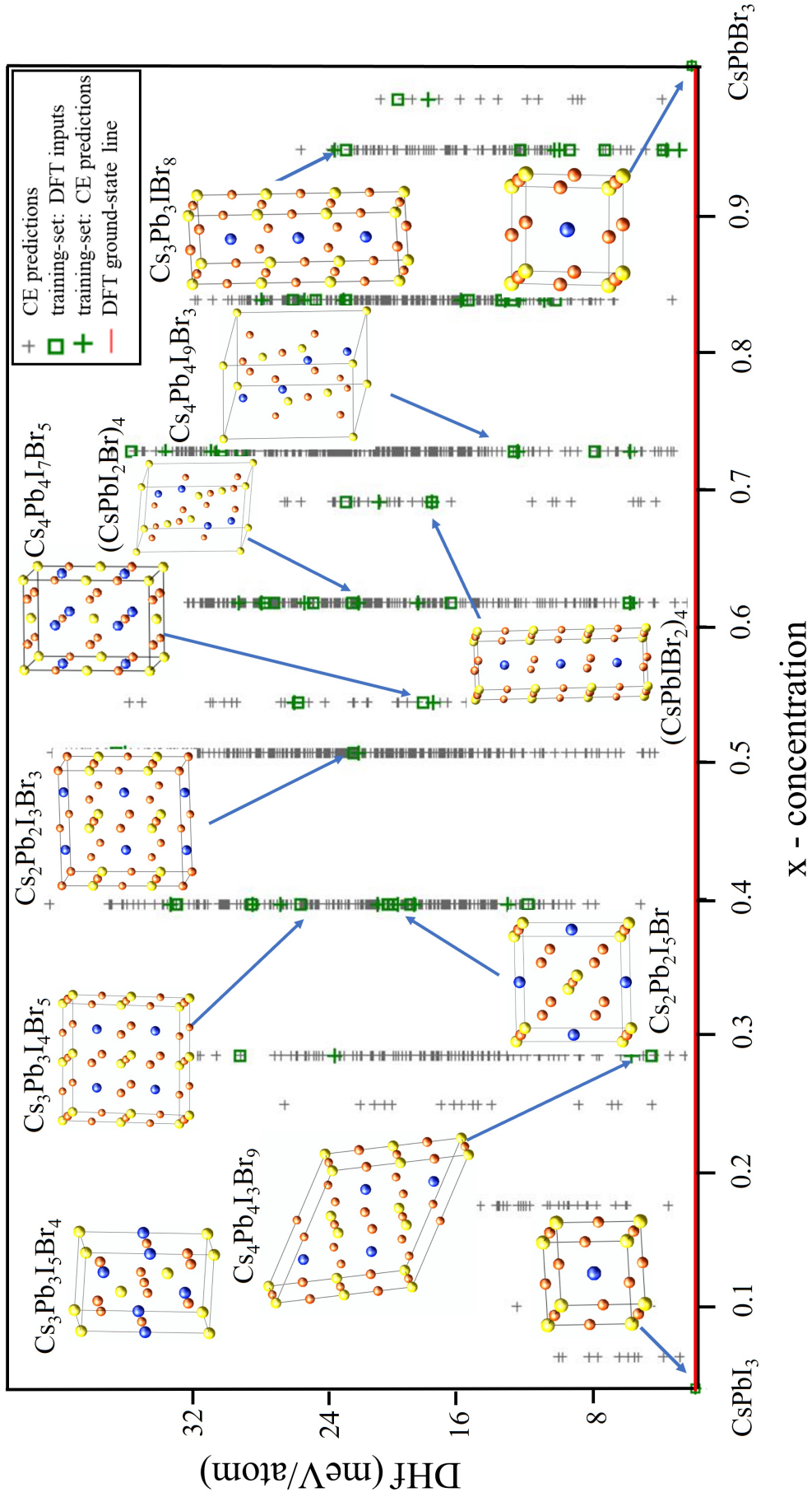
Figure 6.1: Ground state diagram of \text{CsPb(IBr)}_3 .
