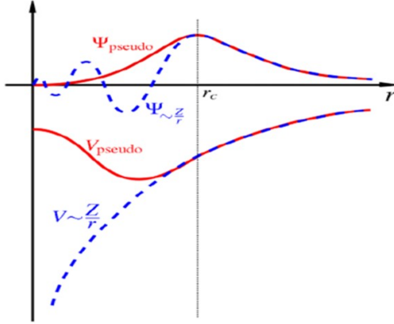
Figure 3.1: Pseudopotentials and pseudo wavefunctions [131].
