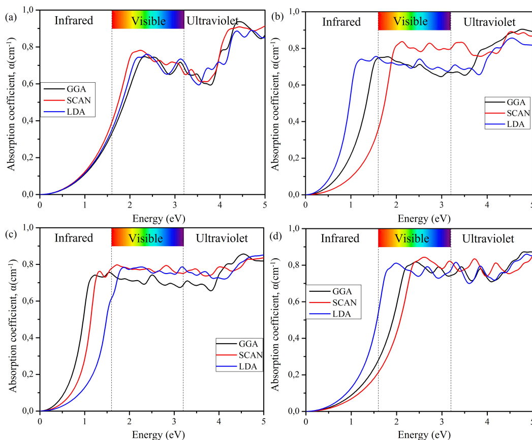
Figure 4.9: Calculated absorption coefficient \alpha(\omega) of (a) \text{CsPbI}_3 , (b) \text{CsPbI}_2\text{Br} , (c) \text{CsPbIBr}_2 and (d) \text{CsPbBr}_3 compounds obtained using LDA, GGA-PBE and SCAN meta-GGA.
