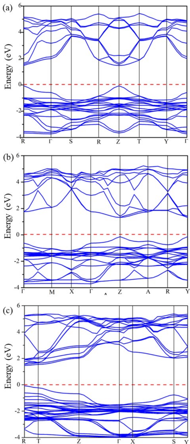
Figure 6.5: The calculated band structures of the predicted (a) \text{Cs}_2\text{Pb}_2\text{I}_3\text{Br}_3 , (b) \text{Cs}_2\text{Pb}_2\text{I}_5\text{Br} and (c) \text{Cs}_3\text{Pb}_3\text{IBr}_8 structures.
