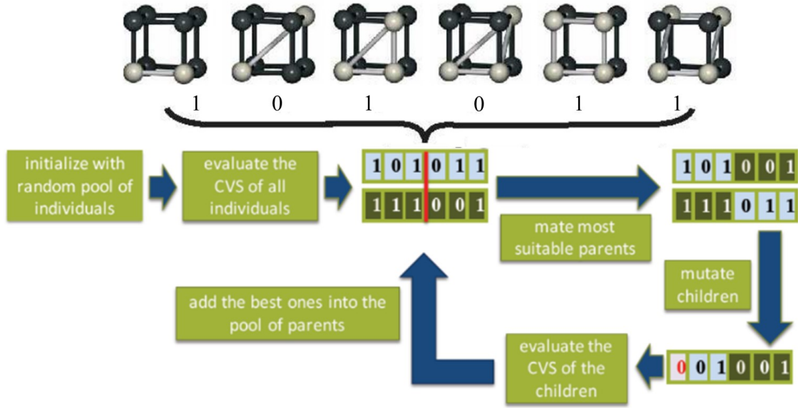
Figure 3.2: Illustration of genetic algorithm approach [139].
