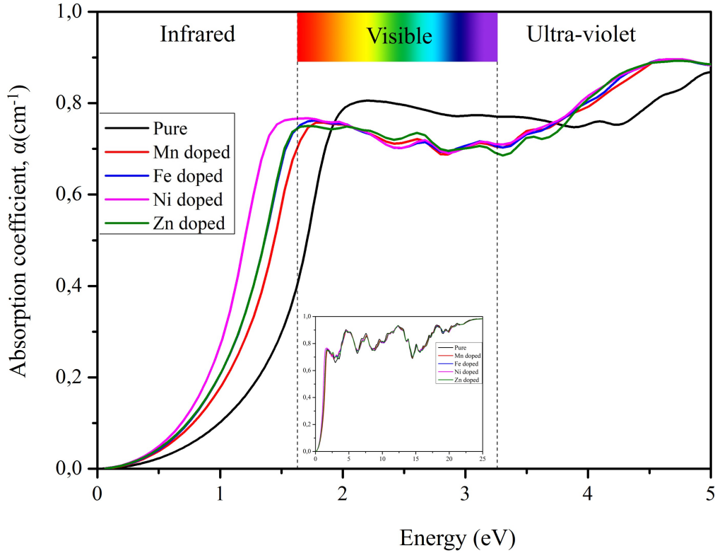
Figure 5.11: The calculated optical absorption coefficient, \alpha(\omega) of the undoped CsPbI 3 and TM doped perovskites.
