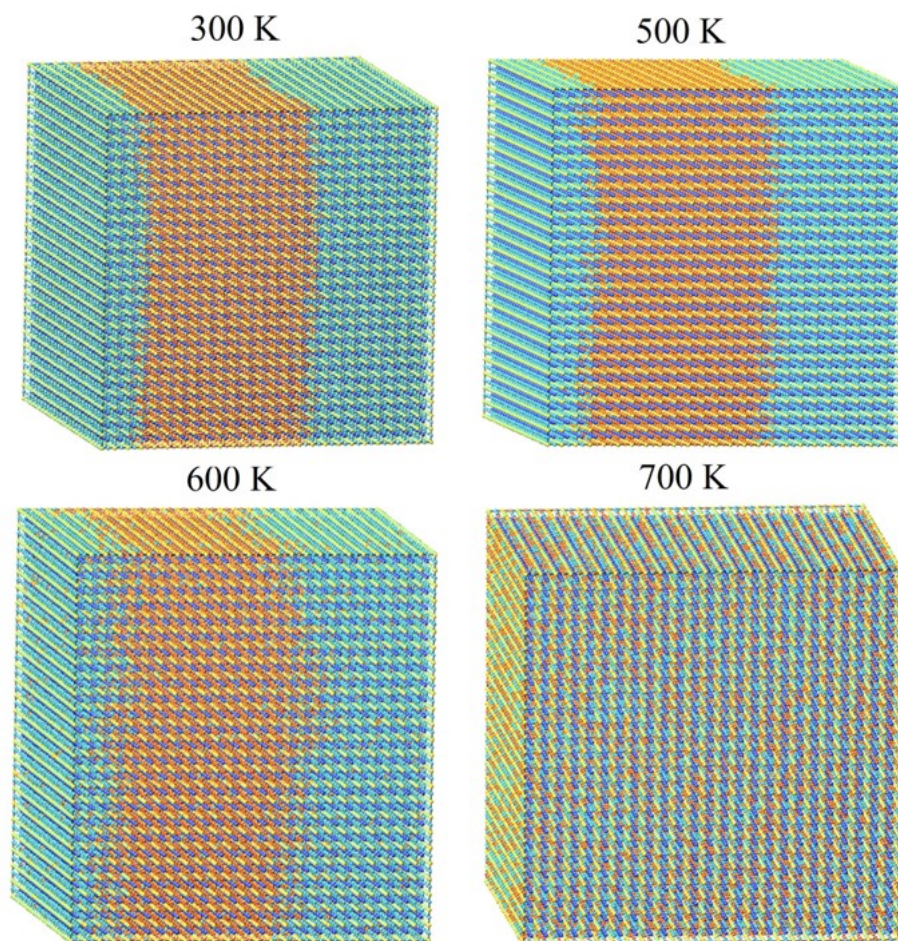
Figure 6.3: Monte Carlo simulation cells of \text{CsPbI}_{0.5}\text{Br}_{0.5} at different temperature. Blue and orange balls are I and Br atoms.
