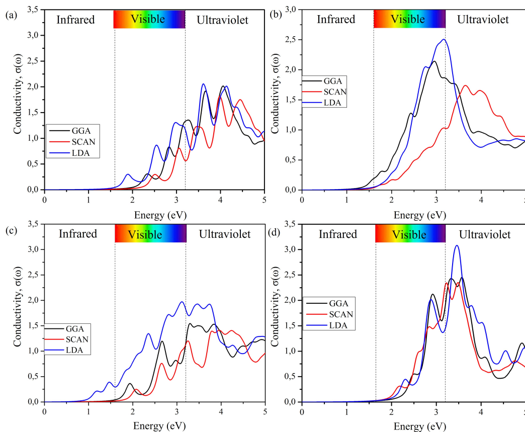
Figure 4.10: Calculated optical conductivity \sigma(\omega) of (a) \text{CsPbI}_3 , (b) \text{CsPbI}_2\text{Br} , (c) \text{CsPbIBr}_2 and (d) \text{CsPbBr}_3 compounds obtained using LDA, GGA-PBE and SCAN meta-GGA.
