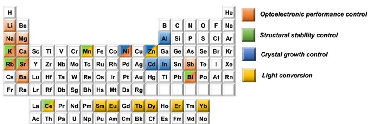
Figure 2.9: Different doping elements and their functions in tailoring lead halide perovskites [85].
