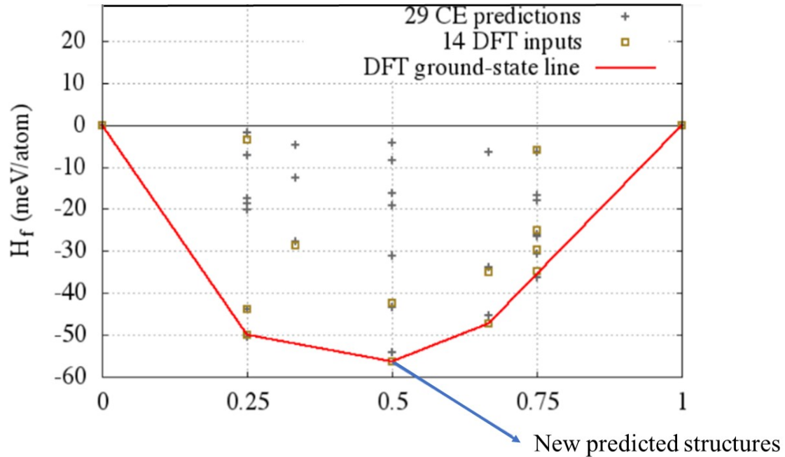
Figure 3.3: Binary groundstate diagram illustrating miscible constituent [139].
