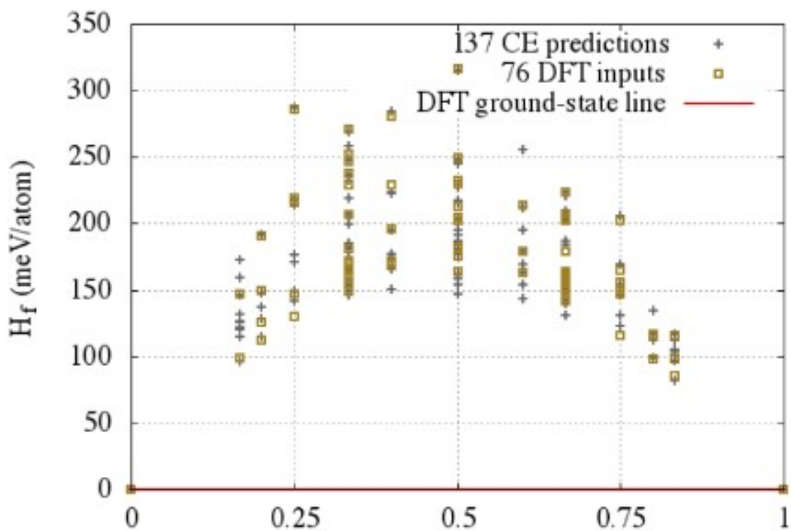
Figure 3.4: Binary groundstate diagram illustrating miscibility gap [139].
