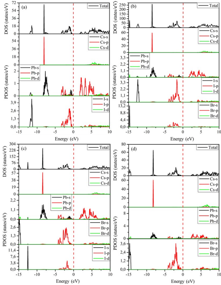
Figure 4.3: Total and partial density of states for (a) \text{CsPbI}_3 , (b) \text{CsPbI}_2\text{Br} , (c) \text{CsPbIBr}_2 and (d) \text{CsPbBr}_3 perovskites obtained using SCAN meta-GGA.
