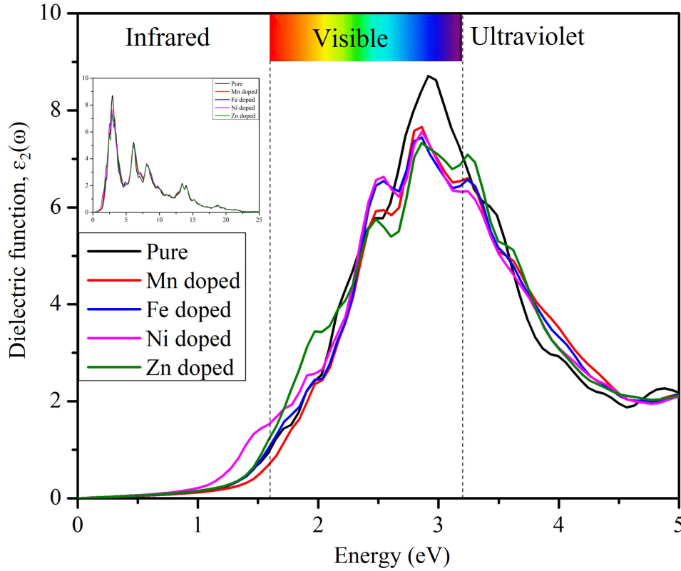
Figure 5.6: The calculated imaginary part of the dielectric function, \epsilon_2(\omega) for undoped \text{CsPbI}_3 and TM doped perovskites.
