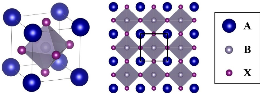
Figure 5.1: The constructed polyhedron unit cell (left) and supercell cubic perovskite crystal structure with A-cation (blue), B-cation (grey) and X-anions (magenta).
