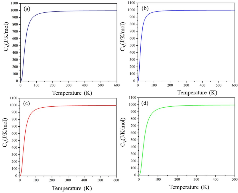
Figure 5.13: The calculated heat capacity against temperature for \text{CsPb}_{0.875}\text{TM}_{0.125}\text{I}_3 perovskite materials.
