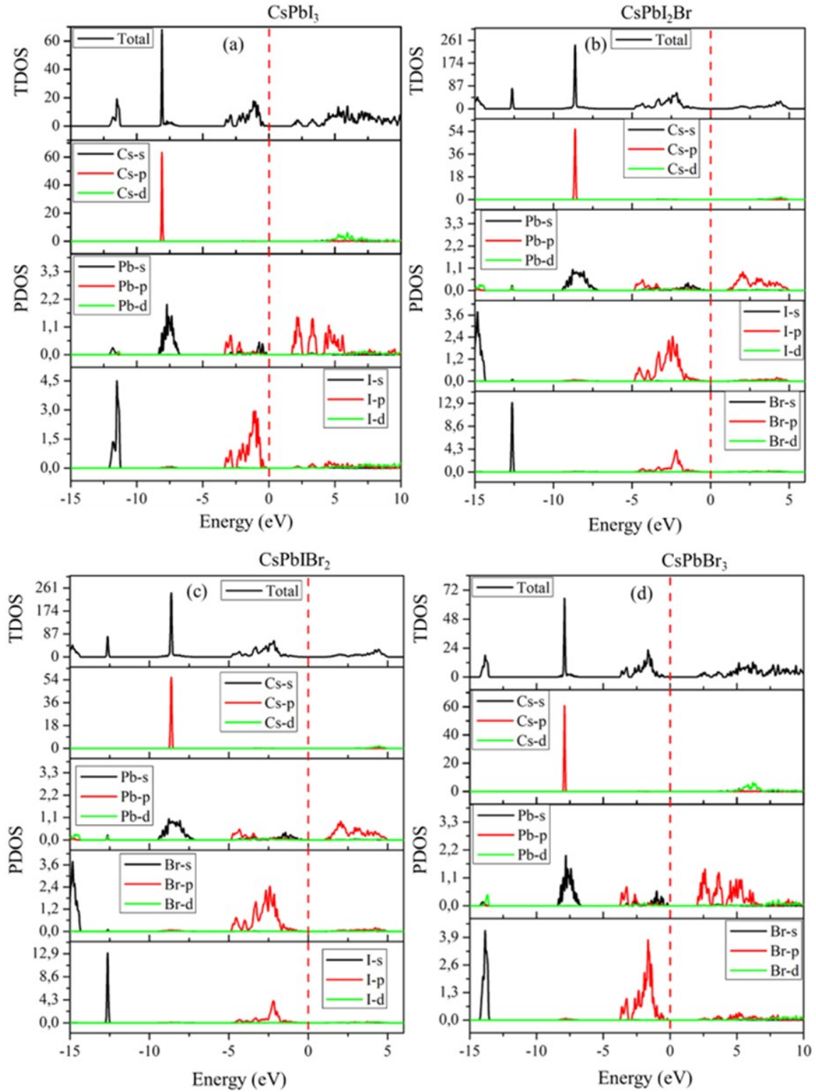
Figure A.1: Total and partial density of states for (a) \text{CsPbI}_3 , (b) \text{CsPbI}_2\text{Br} , (c) \text{CsPbIBr}_2 and (d) \text{CsPbBr}_3 perovskites using GGA.
