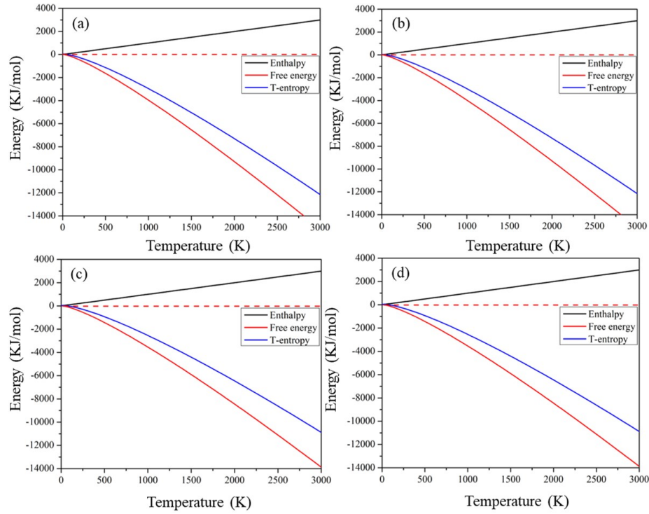
Figure 5.14: The calculated enthalpy, entropy and free energy against temperature for \text{CsPb}_{0.875}\text{TM}_{0.125}\text{I}_3 perovskite materials.
