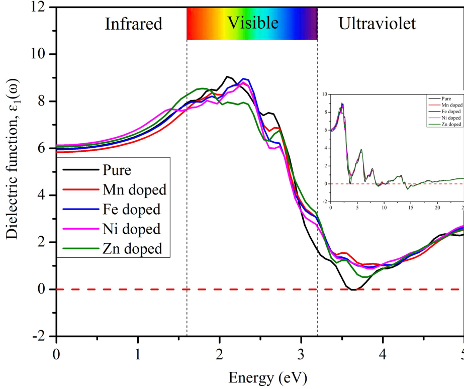
Figure 5.5: The calculated real part of the dielectric function, \epsilon_1(\omega) for undoped CsPbI 3 and TM doped perovskites.
