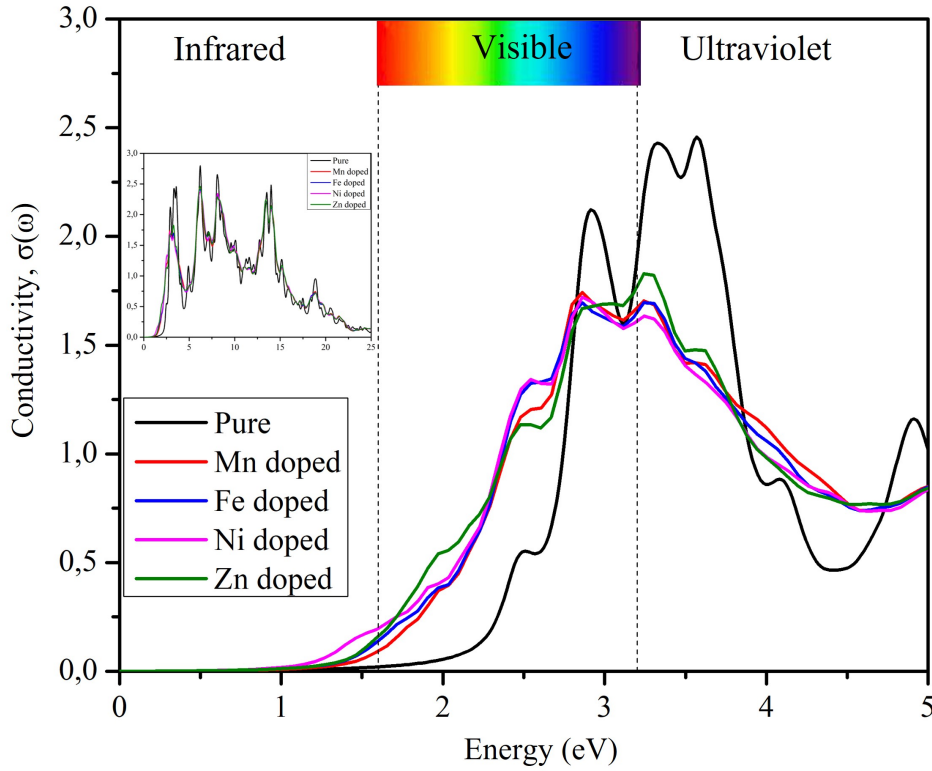
Figure 5.10: The calculated conductivity, \sigma(\omega) of undoped \text{CsPbI}_3 and TM doped perovskites using GGA-PBE functional.
