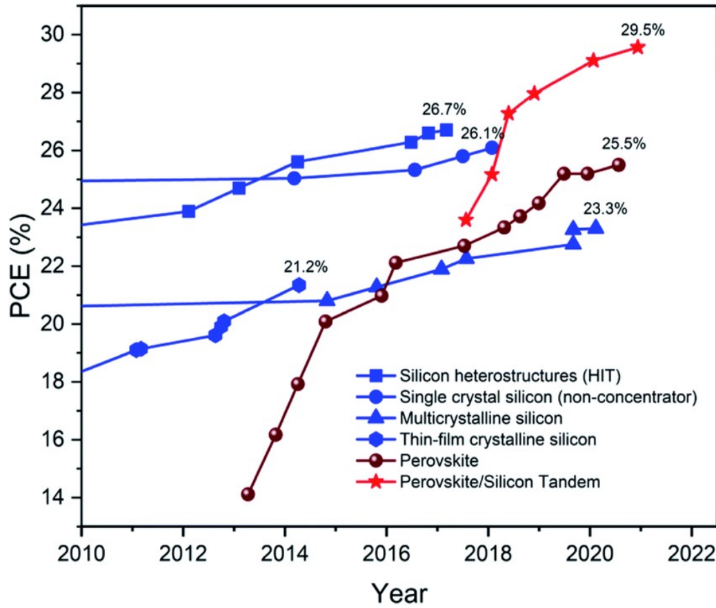
Figure 2.7: Efficiency graph for silicon, perovskite, and tandem silicon-perovskite devices during the past ten years. Information extracted from the US NREL's efficiency graph [65].
