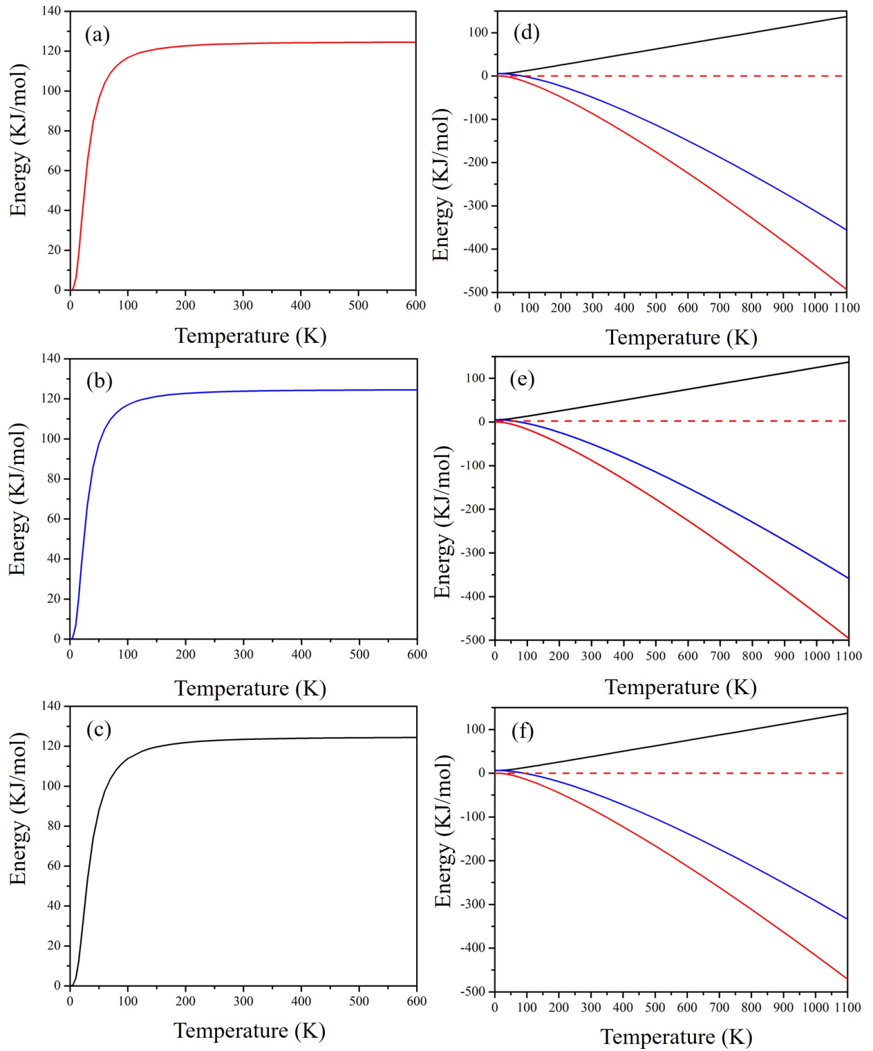
Figure 4.13: Temperature dependence of heat capacity of (a) \text{CsPbI}_3 , (b) \text{CsPbI}_2\text{Br} and (c) \text{CsPbBr}_3 perovskites and their (d) - (e) enthalpy, temperature entropy, and free energy using SCAN functional.
