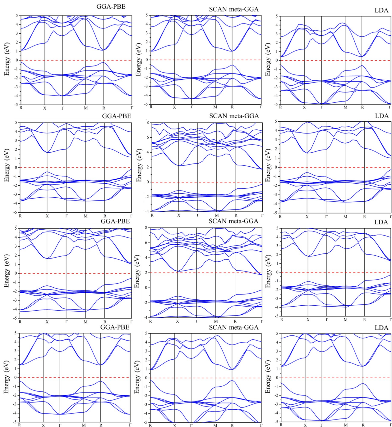
Figure 4.2: Band structures of (a) \text{CsPbI}_3 , (b) \text{CsPbI}_2\text{Br} , (c) \text{CsPbIBr}_2 and (d) \text{CsPbBr}_3 perovskites obtained using three functionals.
