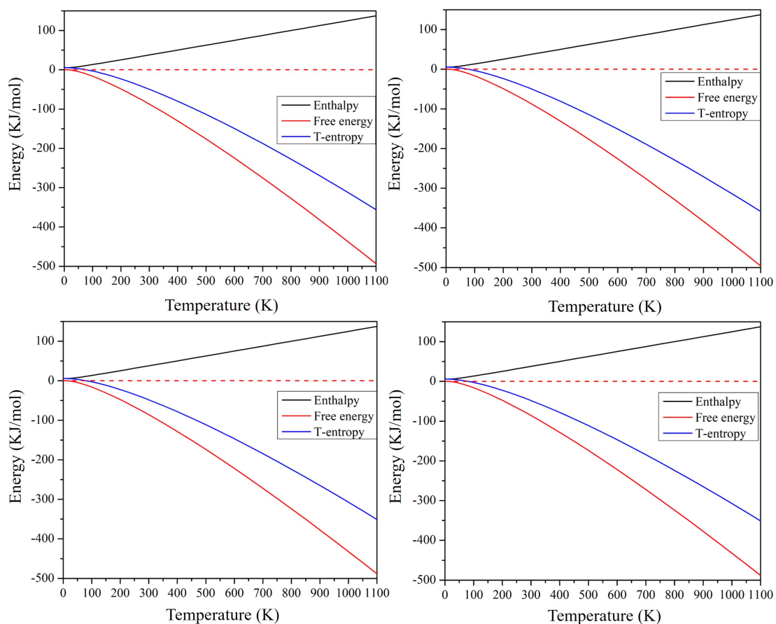
Figure 4.12: Temperature dependence of thermodynamic properties, that is, enthalpy, temperature entropy, and free energy of (a) \text{CsPbI}_3 , (b) \text{CsPbI}_2\text{Br} , (c) \text{CsPbBr}_2\text{I} and (d) \text{CsPbBr}_3 perovskites obtained using GGA-PBE.
