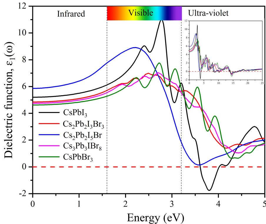
Figure 6.7: The calculated real \epsilon_1(\omega) dielectric function of the predicted structures (a) \text{Cs}_2\text{Pb}_2\text{I}_3\text{Br}_3 , (b) \text{Cs}_2\text{Pb}_2\text{I}_5\text{Br} and (c) \text{Cs}_3\text{Pb}_3\text{IBr}_8 .
