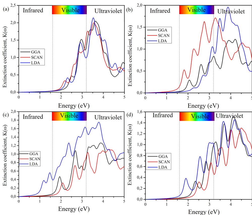
Figure 4.7: Calculated extinction coefficient K(\omega) of (a) \text{CsPbI}_3 , (b) \text{CsPbI}_2\text{Br} , (c) \text{CsPbIBr}_2 and (d) \text{CsPbBr}_3 compounds obtained using LDA, GGA-PBE and SCAN meta-GGA.
