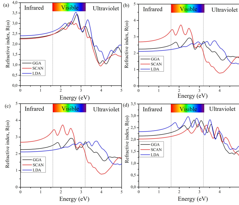
Figure 4.6: Calculated refractive index n(\omega) of (a) \text{CsPbI}_3 , (b) \text{CsPbI}_2\text{Br} , (c) \text{CsPbIBr}_2 and (d) \text{CsPbBr}_3 compounds obtained using LDA, GGA-PBE and SCAN meta-GGA.
