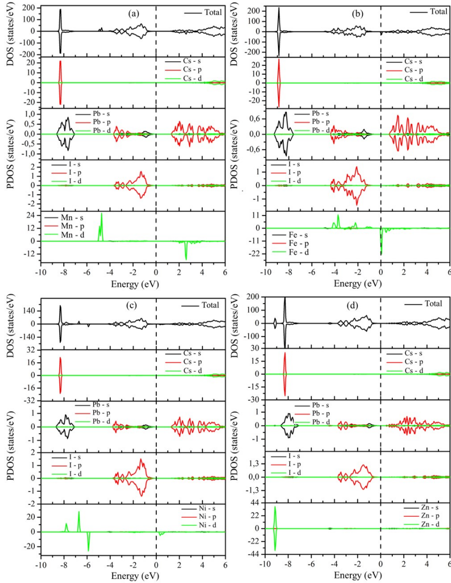
Figure 5.4: Total and partial density of states for (a) \text{CsPb}_{0.875}\text{Mn}_{0.125}\text{I}_3 , (b) \text{CsPb}_{0.875}\text{Fe}_{0.125}\text{I}_3 , (c) \text{CsPb}_{0.875}\text{Ni}_{0.125}\text{I}_3 , and (d) \text{CsPb}_{0.875}\text{Zn}_{0.125}\text{I}_3 perovskite materials.
