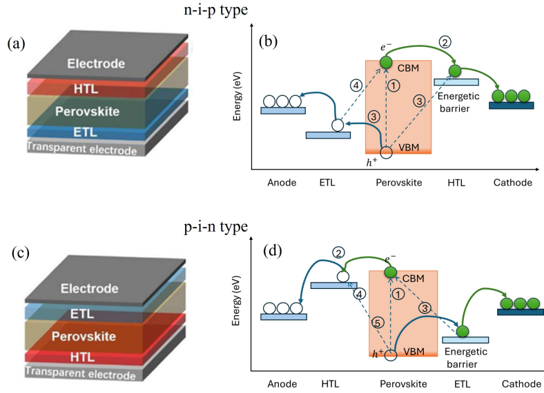
Figure 2.6: Device architecture of (a) n-i-p and (b) the charge transport process type PSCs, (c) p-i-n with (d) charge transport process in p-i-n type PSCs.
