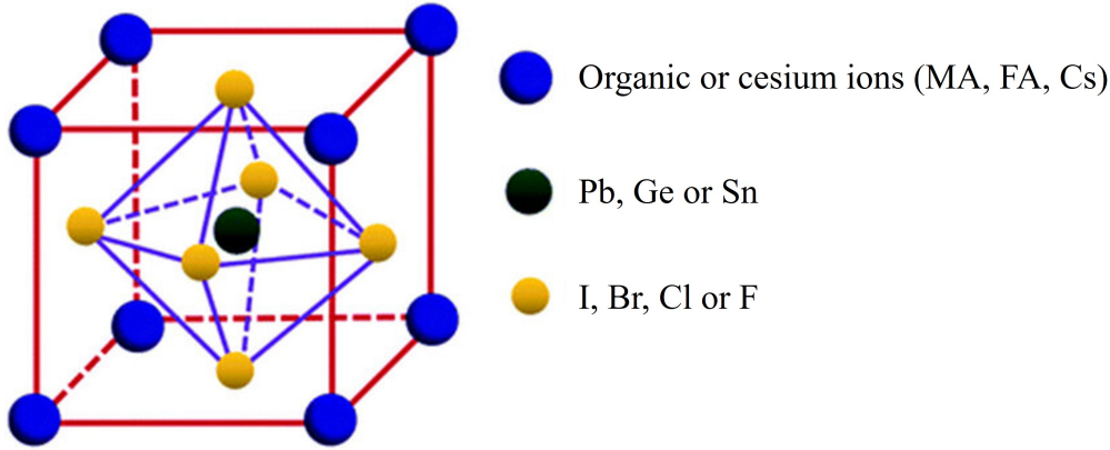
Figure 2.1: Cubic crystal structure of perovskite ABX_3 [19].
