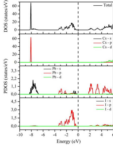
Figure 5.3: Total and partial DOS for undoped \text{CsPbI}_3 perovskite.
