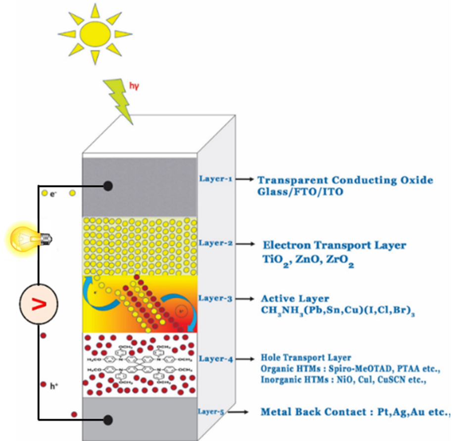
Figure 2.8: An illustration of perovskite solar cell layers [66].
