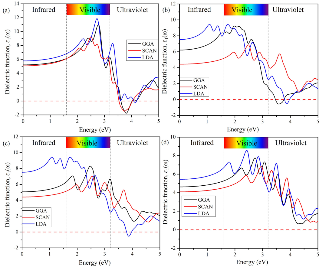
Figure 4.4: Calculated real part \epsilon_1(\omega) of (a) \text{CsPbI}_3 , (b) \text{CsPbI}_2\text{Br} , (c) \text{CsPbIBr}_2 and (d) \text{CsPbBr}_3 compounds obtained using LDA, GGA-PBE and SCAN meta-GGA.
