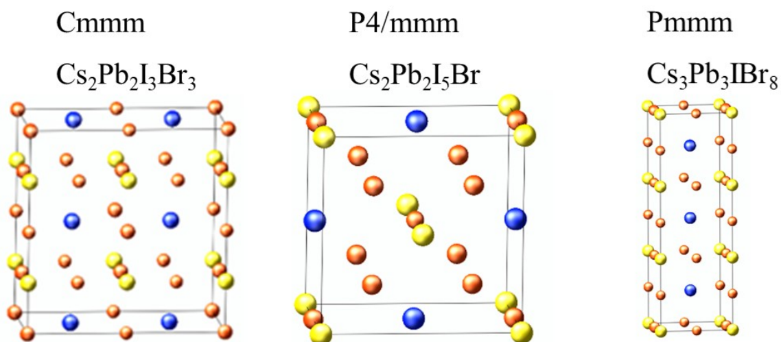
Figure 6.4: The cluster expansion predicted structure \text{Cs}_2\text{Pb}_2\text{I}_3\text{Br}_3 , \text{Cs}_2\text{Pb}_2\text{I}_5\text{Br} and \text{Cs}_3\text{Pb}_3\text{IBr}_8 .
