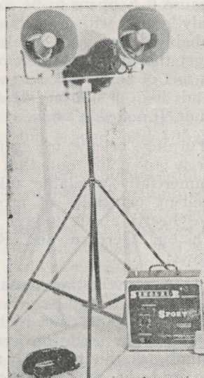
PORTABLE TRANSISTORISED AMPLIFIER FOR SCHOOL SPORTS MEETINGS, ETC.
