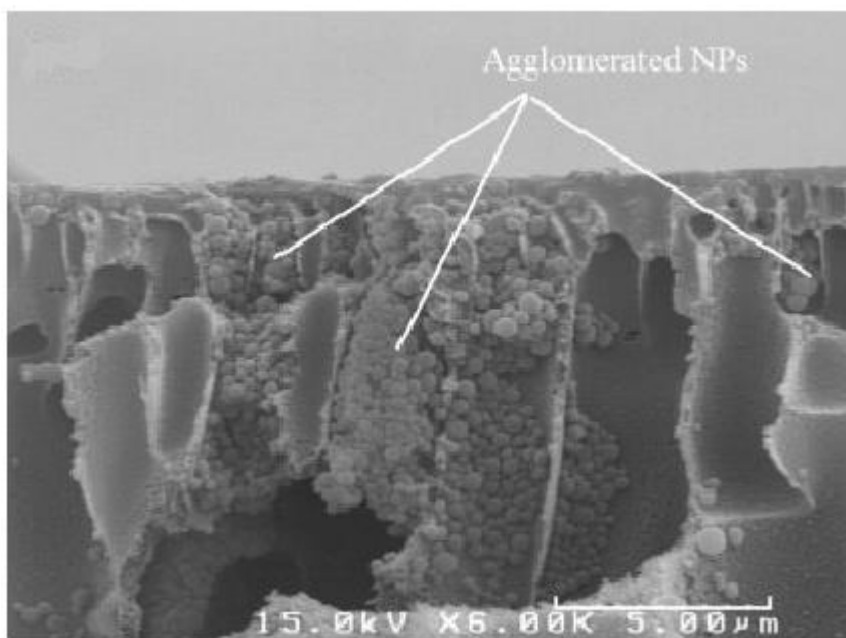
Figure 14 SEM cross-sectional image showing agglomeration in polyaniline/iron oxide nanoparticles modified polyethersulfone membrane (Daraei et al. 2012).
