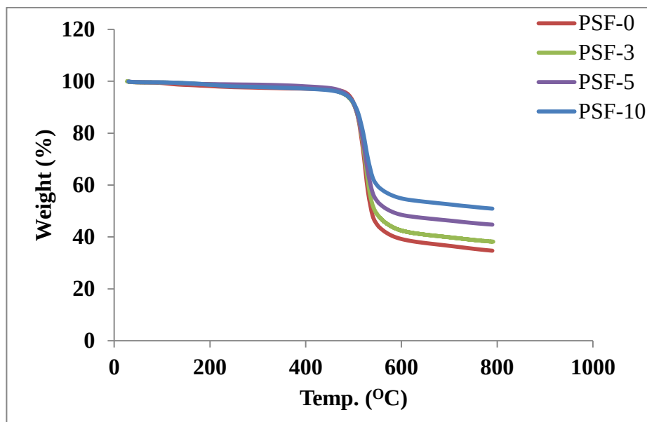
Figure 41 The TGA curve of the Co-modified and unmodified PSF membrane
