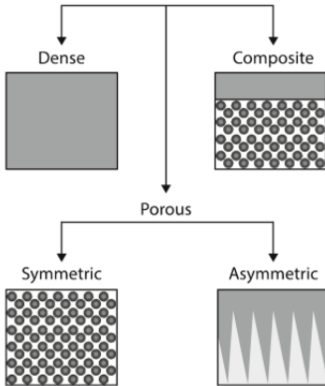
Figure 2 Classification of membranes according to structure (Bradley & Al-Shaeli 2017)
