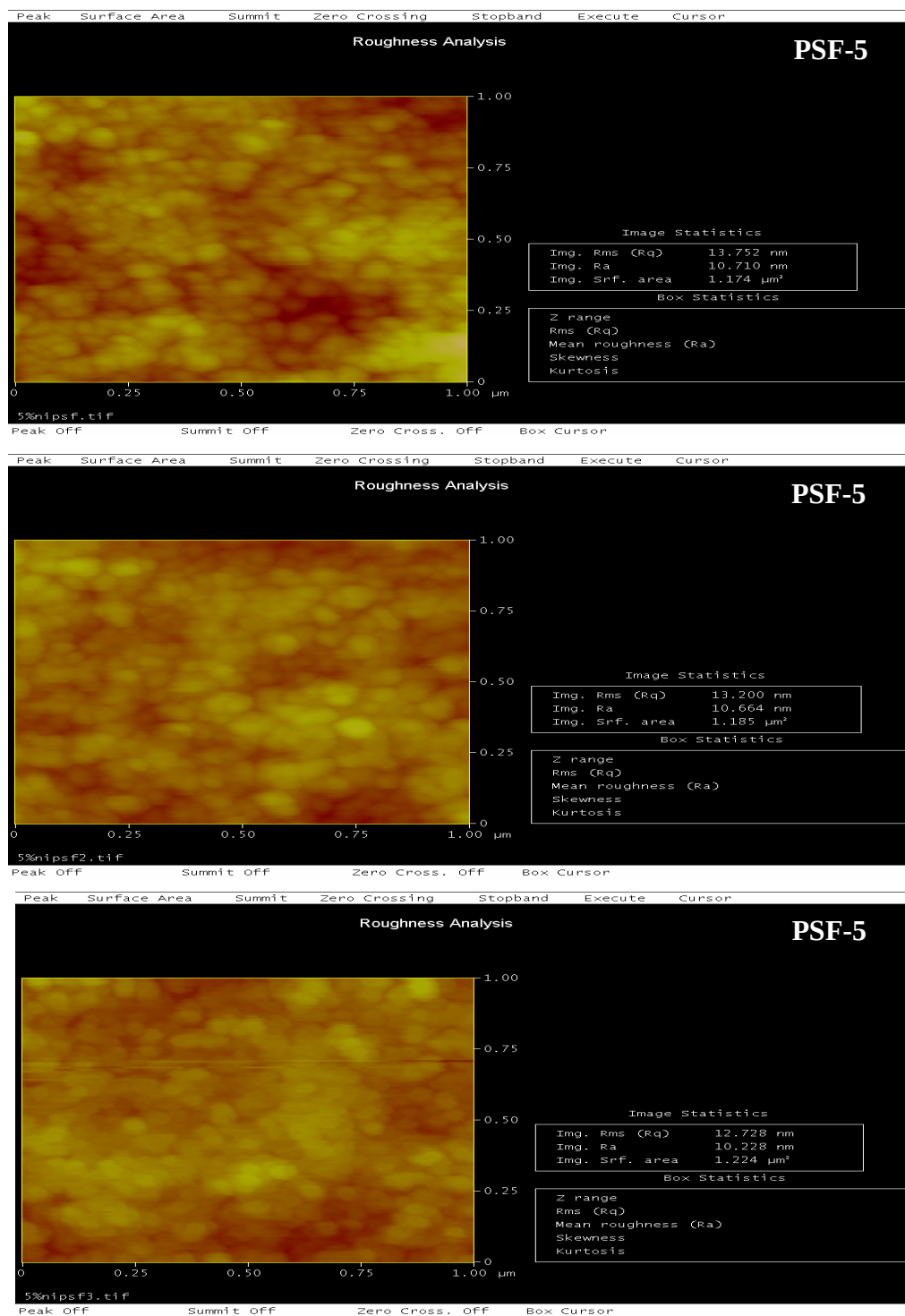
Figure 27 The 2D AFM images of the three different areas of the Ni modified PSF-5 membrane showing the quantitative roughness data of the membrane.
