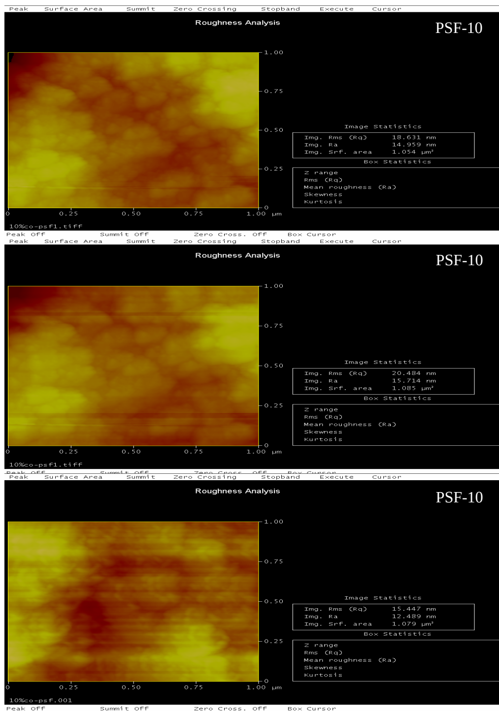
Figure 39 The 2D AFM image of the three different areas of the PSF-10 membrane.
