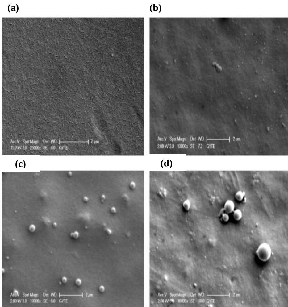
Figure 7 The SEM image of the outer surface of (a) Neutral-PSF, (b) 0.25wt% Ag-PSF (c) 0.5wt% Ag-PSF, and (d) 1.0wt% Ag-PSF modified membranes (Koseoglu-Imer et al. 2013)
