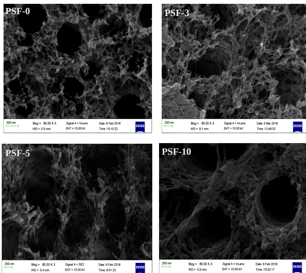
Figure 34 The SEM image inner structures of the Co-modified and unmodified PSF membranes
