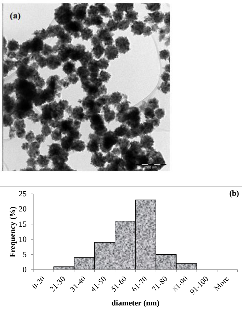
Figure 20 (a) TEM image and (b) size distribution of the Ni nanoparticles.
