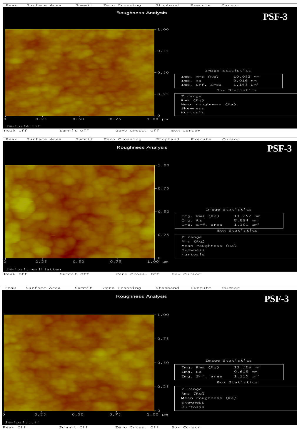
Figure 26 The 2D AFM images of the three different areas of the Ni modified PSF-3 membrane showing the quantitative roughness data of the membrane.
