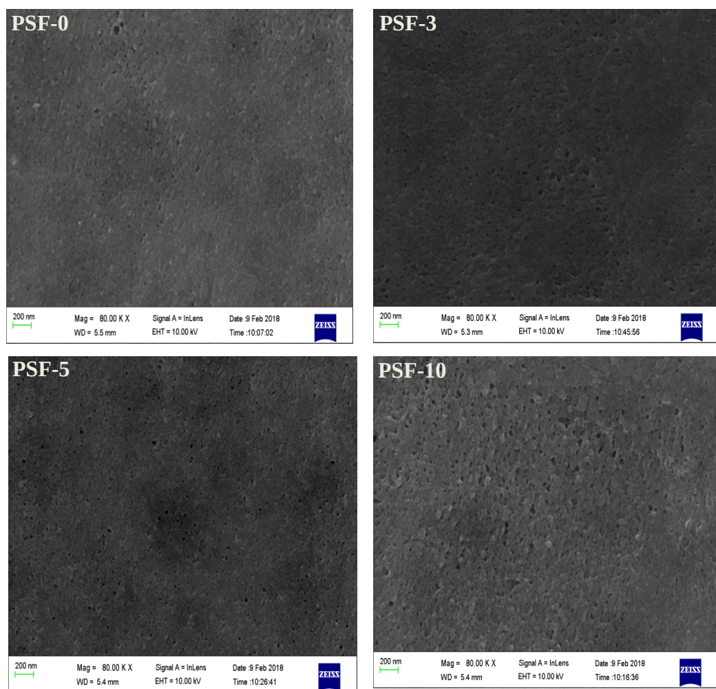
Figure 22 The SEM images of the top surface of the Ni-modified and unmodified PSF membranes
