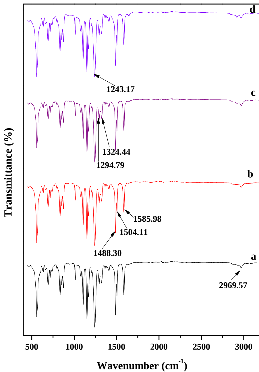
Figure 29 The FTIR spectra of (a) unmodified PSF-0, and the Ni modified (b) PSF-3, (c) PSF-5, and (d) PSF-10.
