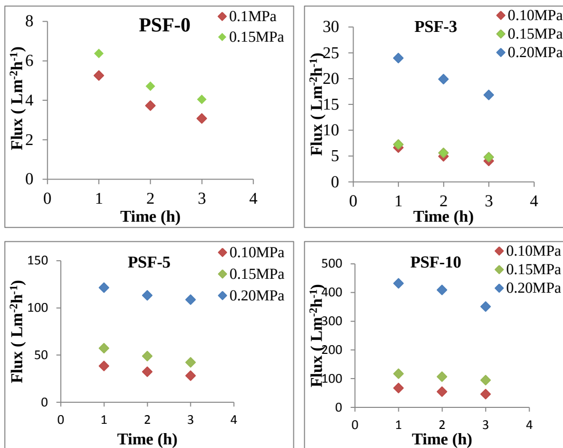
Figure 31 The flux of the Ni-modified and unmodified membranes at different pressures.
