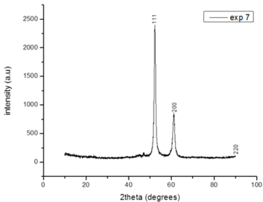
Figure 19 The XRD spectra of the Ni nanoparticles
