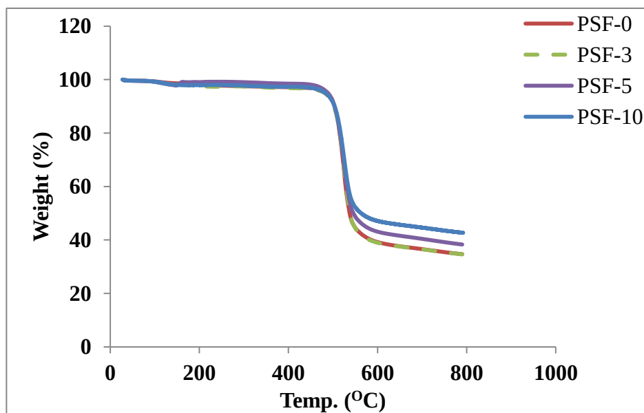
Figure 30 The TGA curve of the Ni-modified and unmodified PSF membranes.
