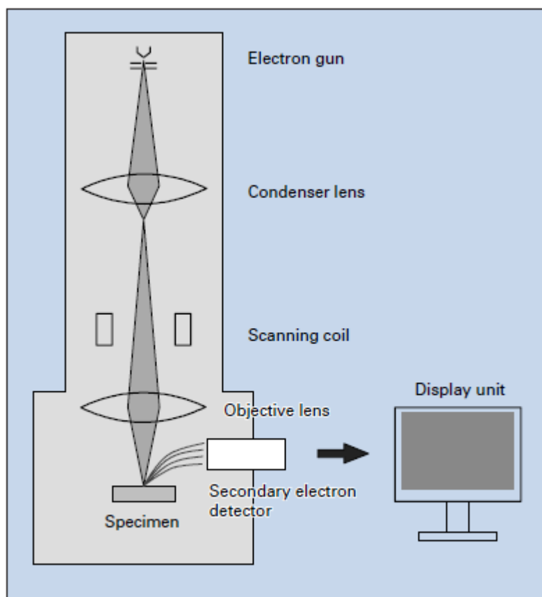
Figure 15 The basic components of SEM (JEOL)
