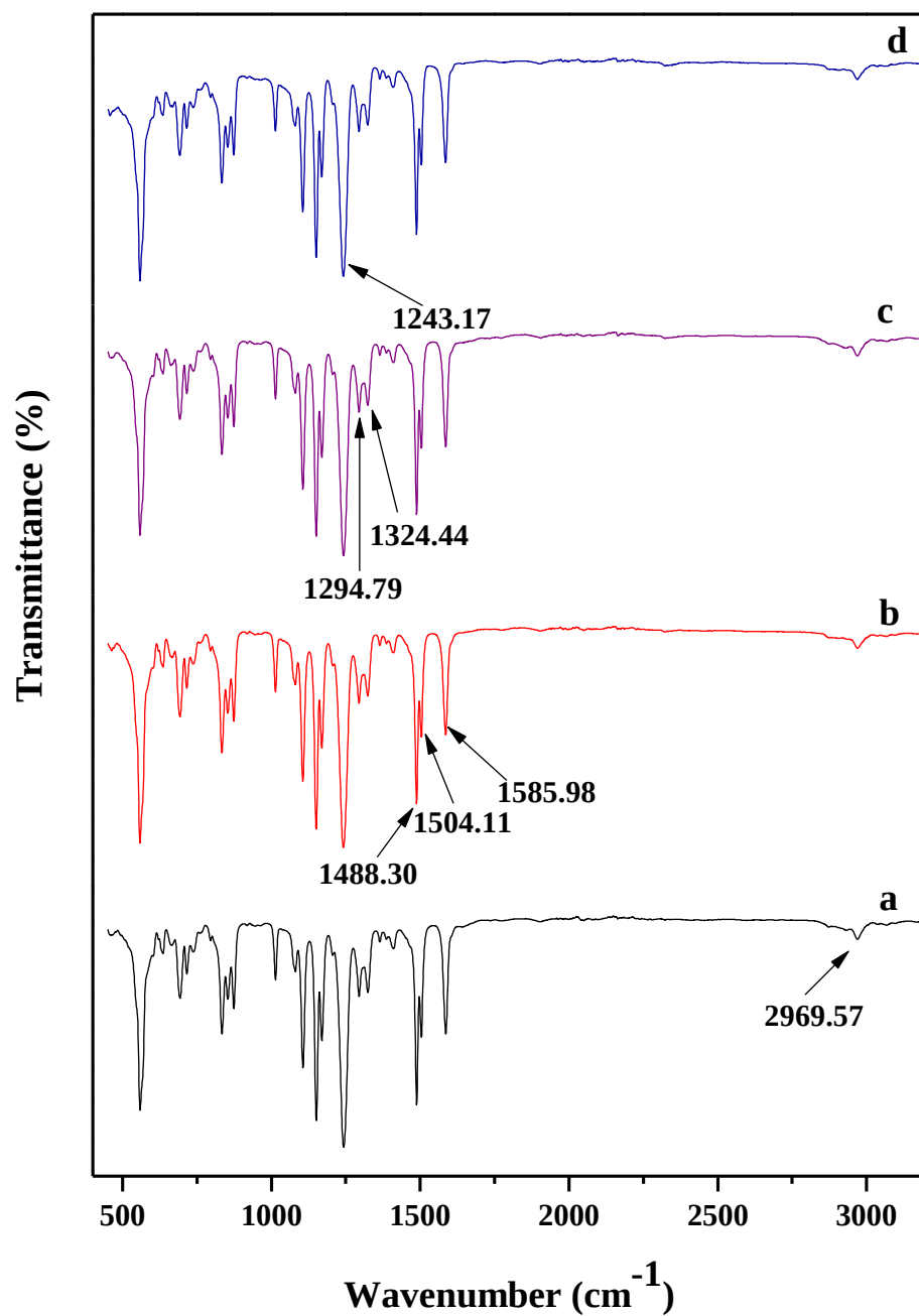
Figure 40 The FTIR spectra of (a) unmodified PSF-0, (b) Co modified PSF-3, (c) Co modified PSF-5, and (d) Co modified PSF-10.
