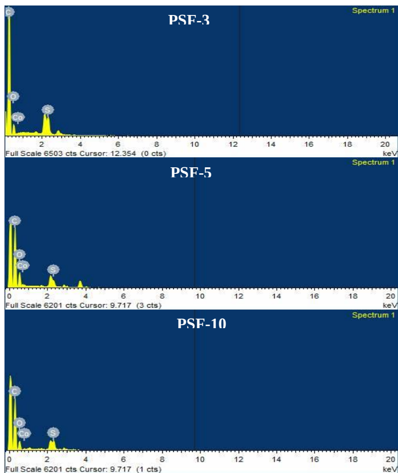
Figure 35 The EDX of the Co-modified PSF membranes
