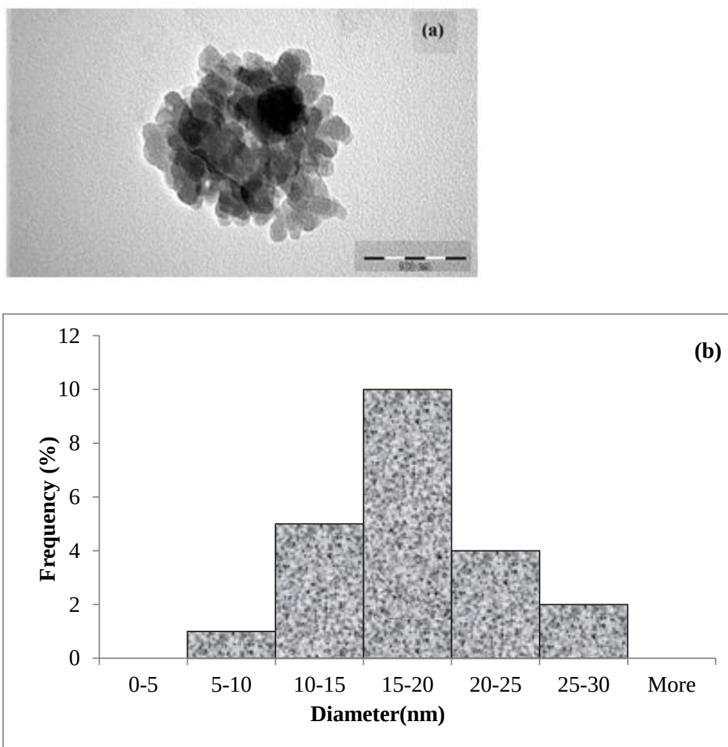
Figure 21 The TEM image (a), and size distribution (b), of the Co nanoparticles.
