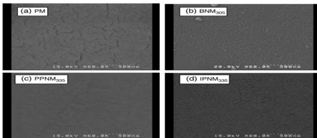
Figure 10 The SEM image of the (a) neutral polysulfone, (b) PSF membrane modified through blending method, (c) PSF membrane modified through photopolymerization, and (d) PSF membrane modified through interfacial polymerization (Homayoonfal et al. 2014).
