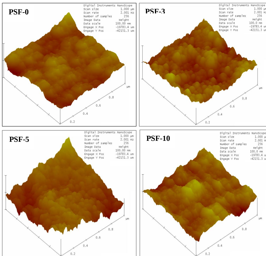
Figure 36 The 3D AFM image of the cobalt modified and unmodified PSF membranes.
