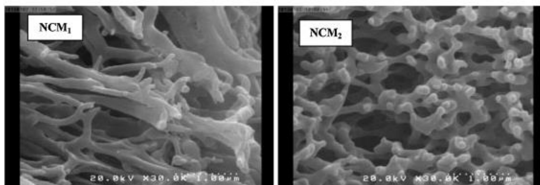
Figure 11 The SEM image of the 0.02wt% (denoted NCM 1 ), and 0.03wt% (denoted NCM 2 ) alumina-PSF nanocomposite membranes (Homayoonfal et al. 2015).
