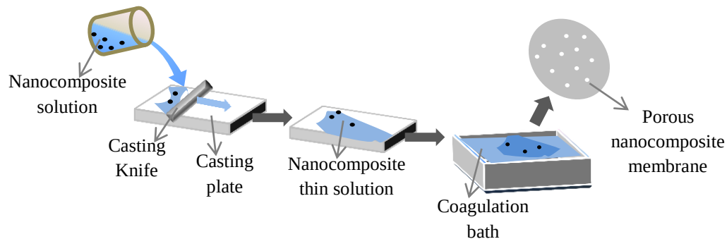
Figure 3 Schematic diagram of immersion precipitation.
