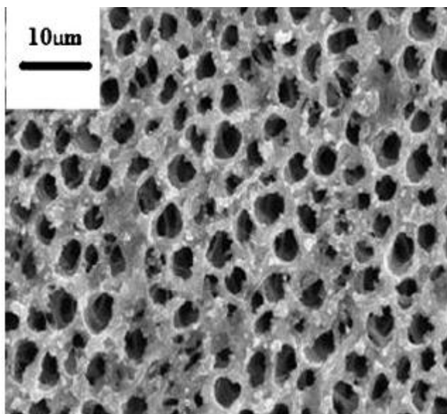
Figure 13 SEM image of the cobalt- modified polysulfone membrane (Phelane et al. 2014b).
