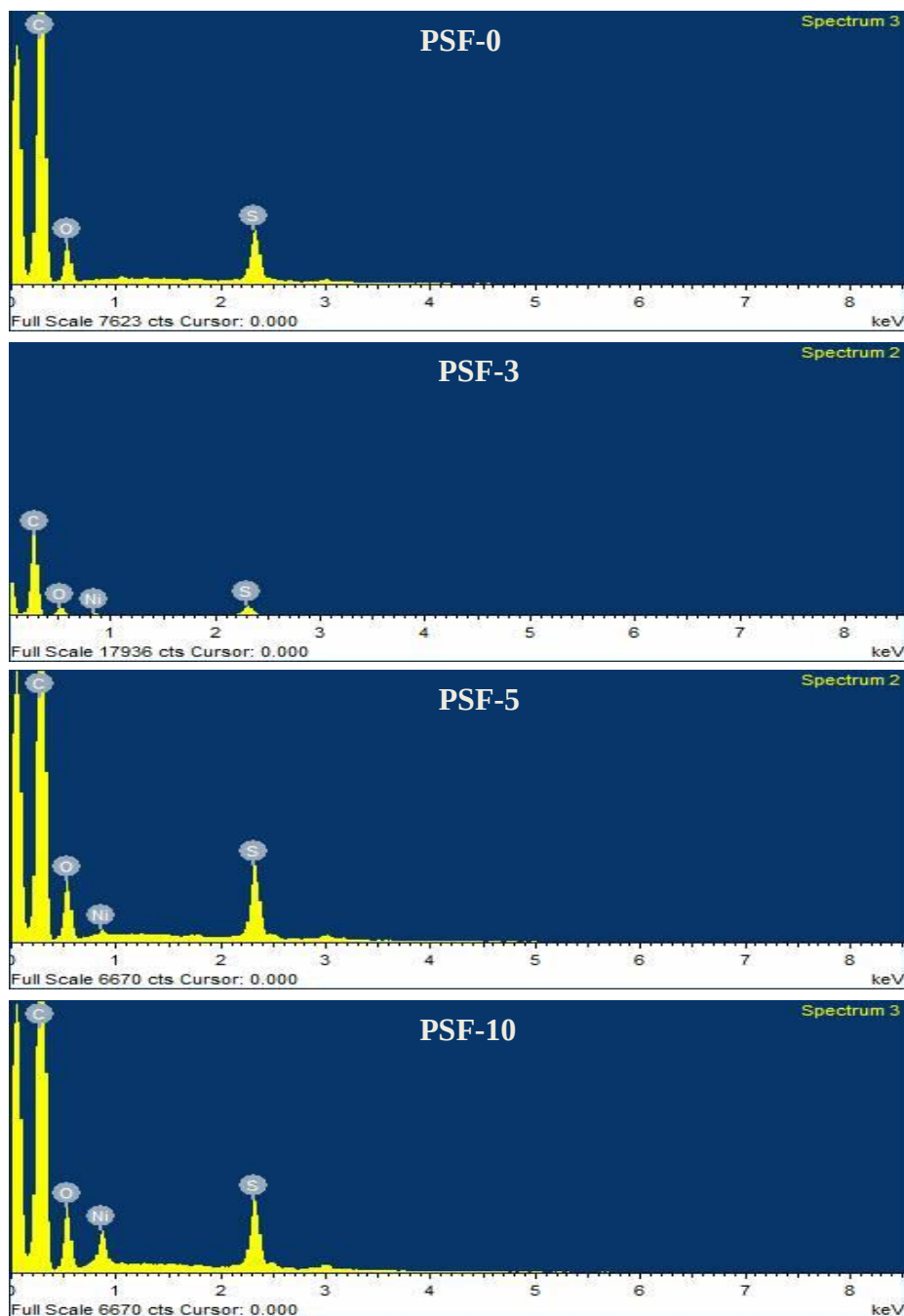
Figure 24 The EDX spectra of the Ni-modified and unmodified PSF membranes
