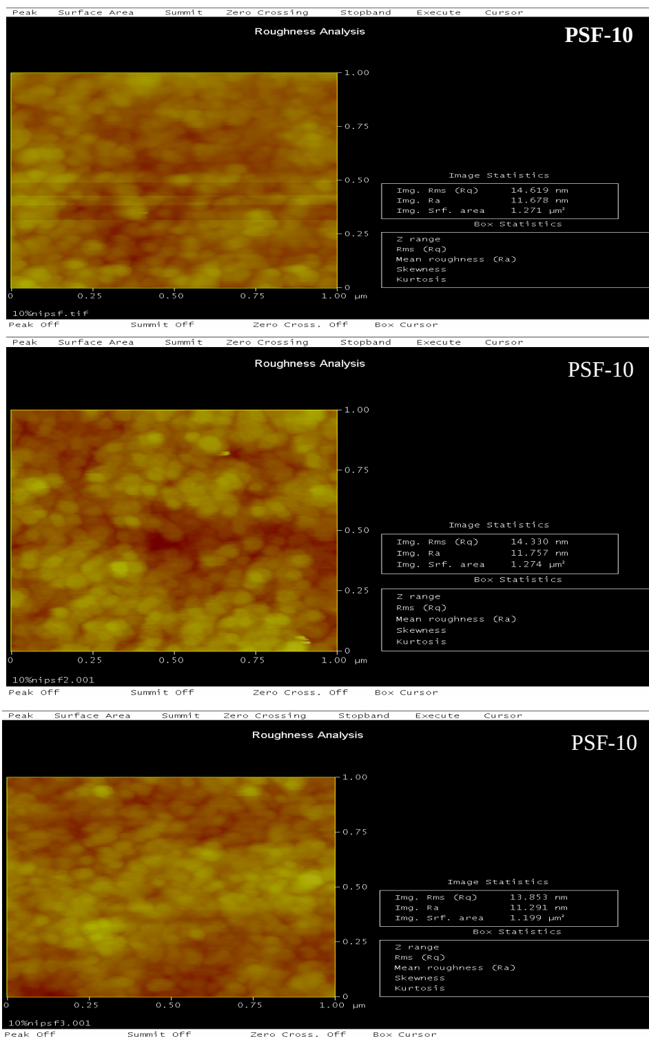
Figure 28 The 2D AFM image of the three different areas of the Ni modified PSF-10 membrane showing the quantitative roughness data of the membrane.
