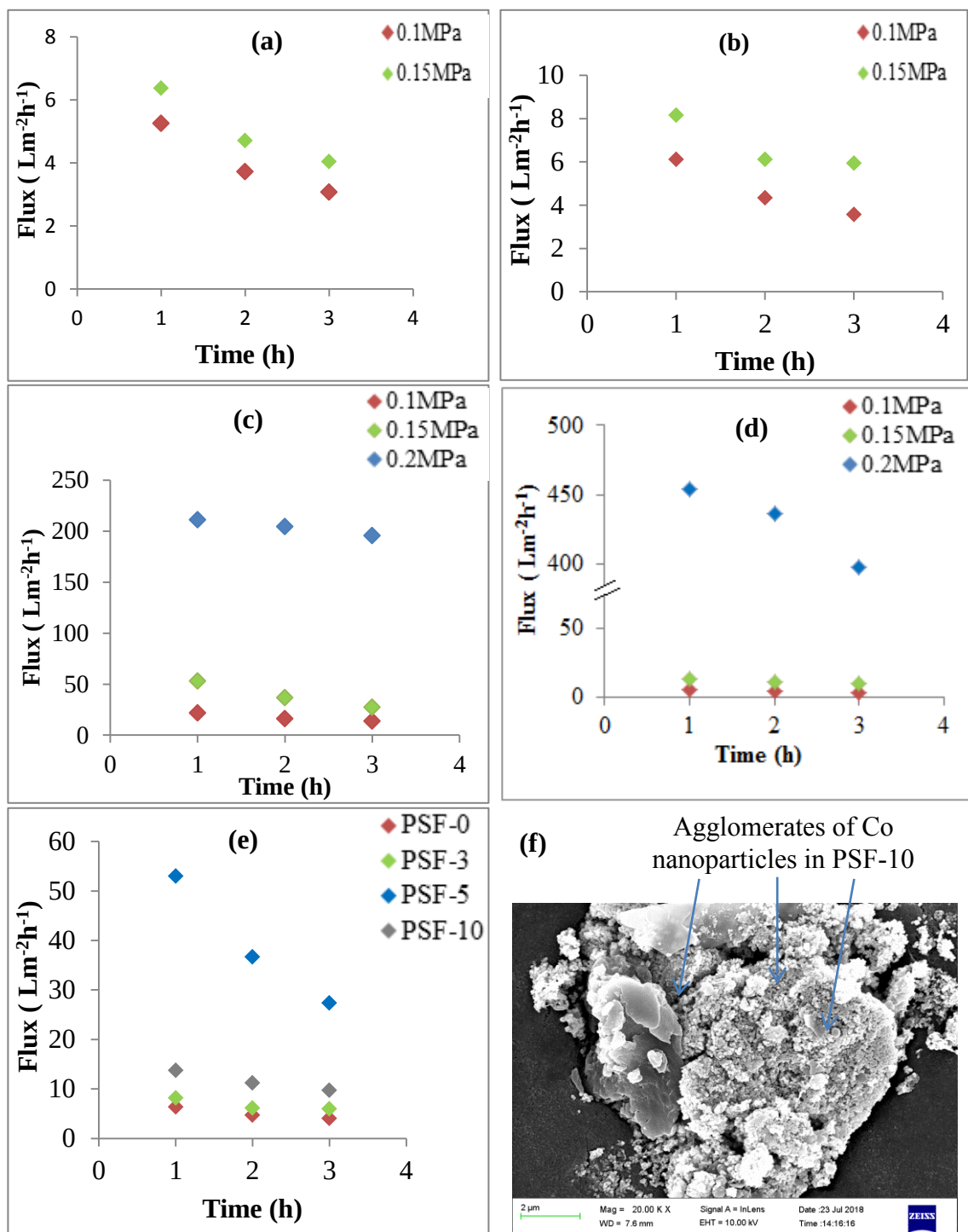
Figure 42 The flux of (a) unmodified PSF, (b) Co-modified PSF-3, (c) Co-modified PSF-5, (d) Co-modified PSF-10, (e) unmodified and modified Co-PSF membranes at 0.15MPa, and (f) agglomeration in PSF-10 membrane.
