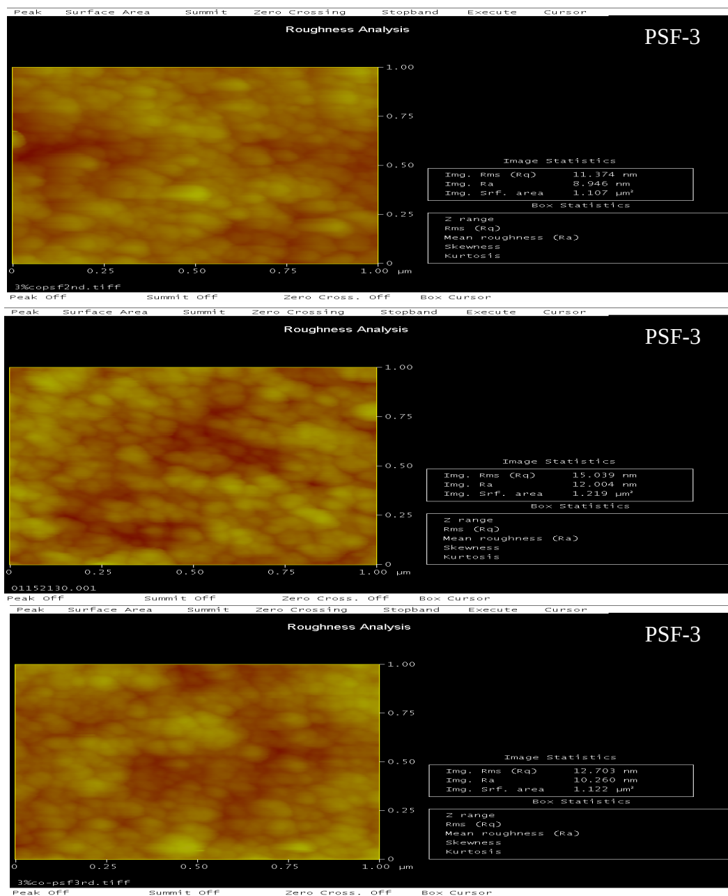
Figure 37 The 2D AFM image of the three different areas of the Co modified PSF-3 membrane.
