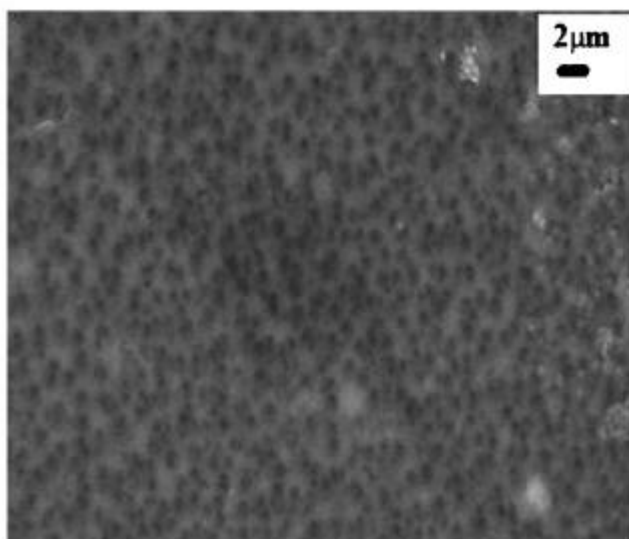
Figure 12 The SEM image of the PSF-Ni nanocomposite membrane showing uniform porosity (Phelane et al. 2014b)
