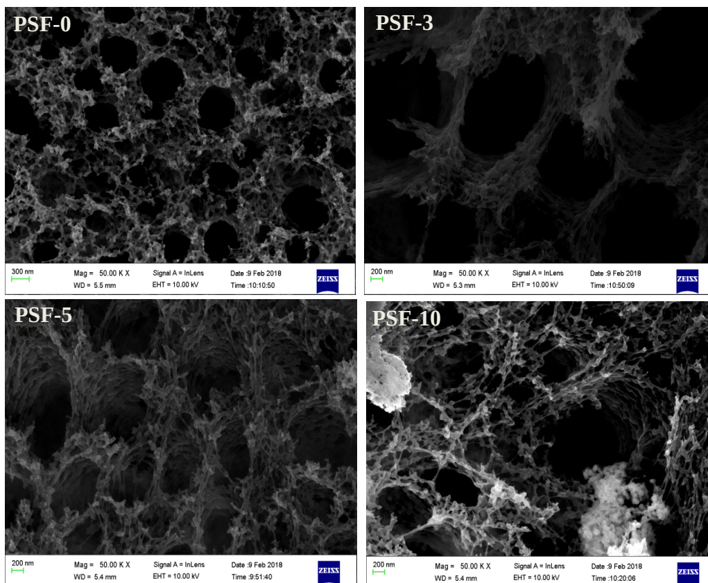
Figure 23 The SEM images of the inner structures of the Ni-modified and unmodified PSF membranes
