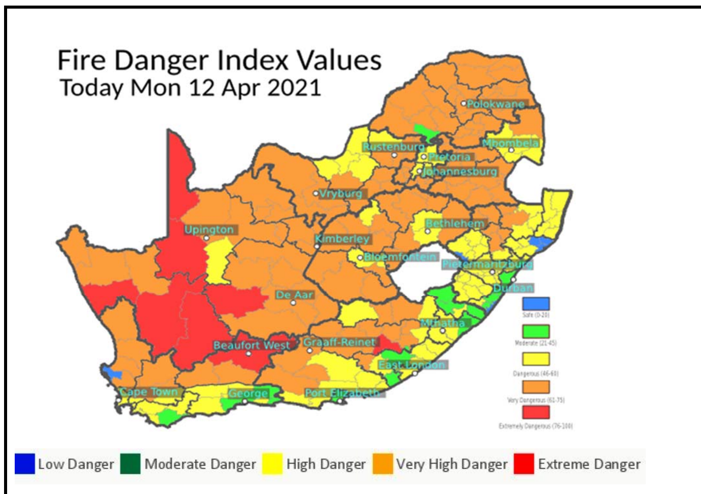
Figure. 2.7: Fire Danger Rating Index in South Africa.
