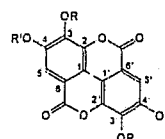
3 R, R' = \text{CH}_3 3,3',4-Tri- O -methylellagic acid 6 R = \text{CH}_3 , R' = \text{H} 3,3'-Di- O -methylellagic acid 7 R, R' = \text{H} Ellagic acid
