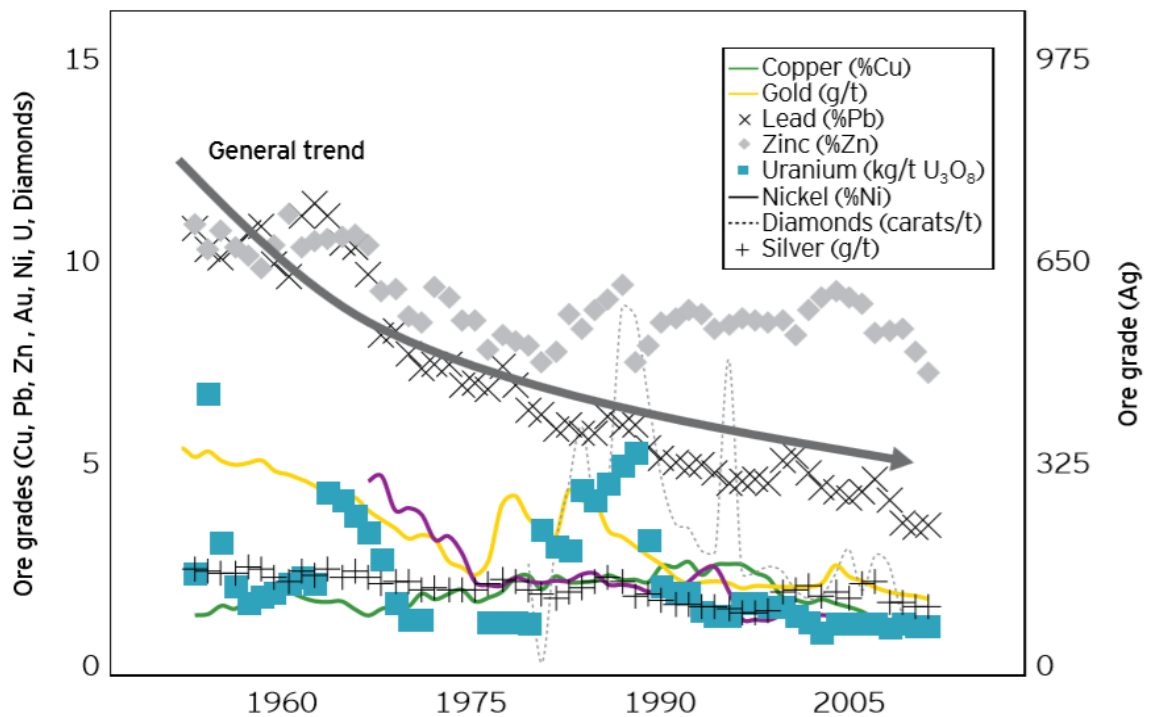
Figure 2.3: Showing declining grade of Copper, Lead, Zinc, Gold, Nickel, Uranium and Diamond Ores (Ernst & Young, 2017a)
