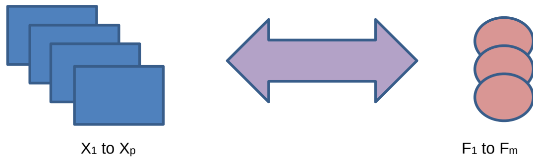
Figure 6: Graphical representation of Exploratory Factor Analysis (Stacey, 2015, p 29)
