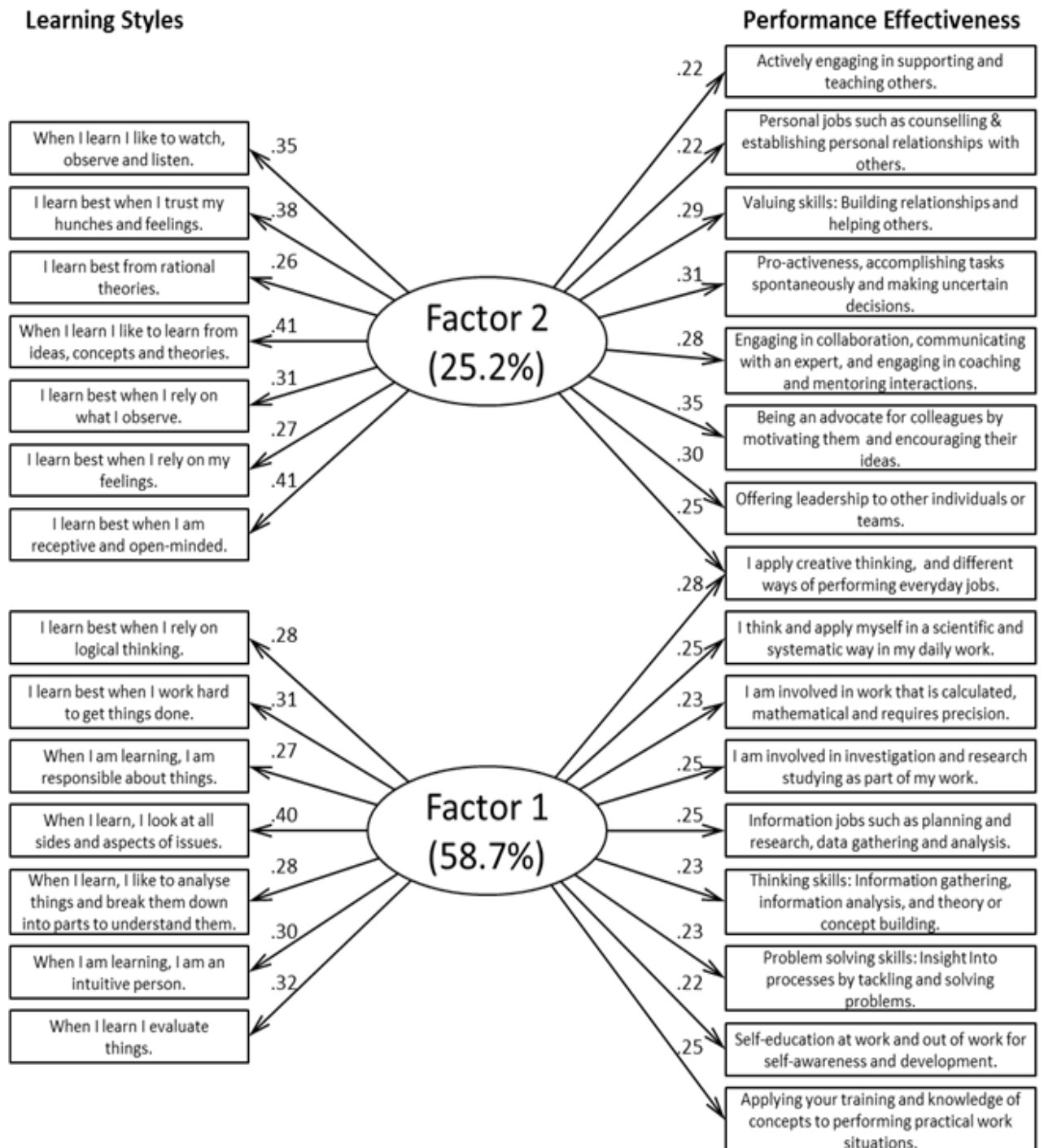
Figure 15: Inter-battery Factor Analysis representation of two factor solution
