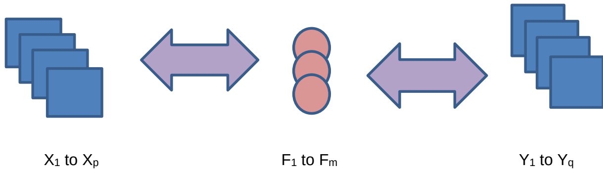
Figure 7: Graphical representation of Inter-battery Factor Analysis (Stacey, 2015, p 9)
