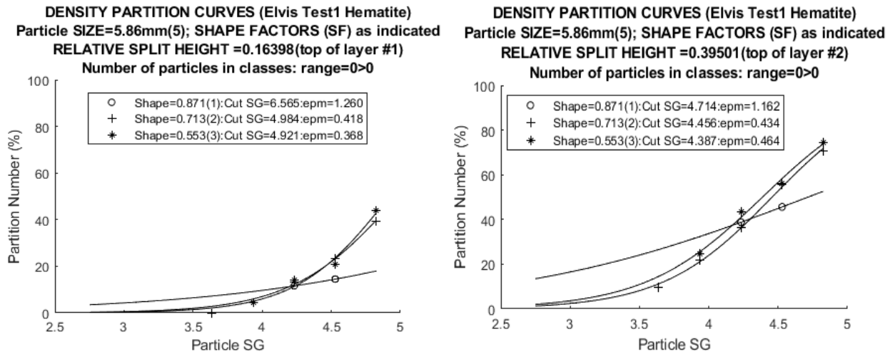
Figure 20: Effect of shape on partition curves for particles in size class 5 with 16% and 39% Yields (i.e., cutting the bed at the top of layers 1 and 2).
