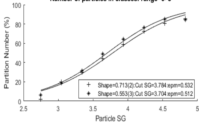
Figure 23: Effect of shape on density partition curves in size class 7 (3.94mm) for different yields.
