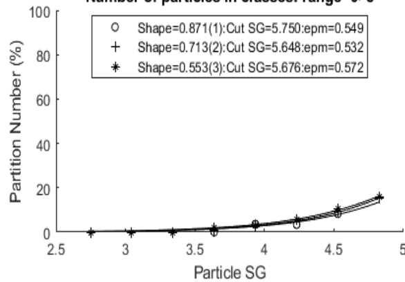
DENSITY PARTITION CURVES (Elvis Test1 Hematite) Particle SIZE=3.94mm(7); SHAPE FACTORS (SF) as indicated RELATIVE SPLIT HEIGHT =0.54091(top of layer #3) Number of particles in classes: range=0>8
