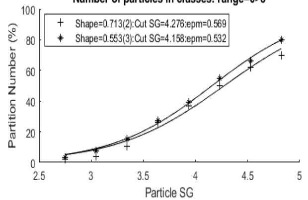
DENSITY PARTITION CURVES (Elvis Test1 Hematite) Particle SIZE=3.94mm(7); SHAPE FACTORS (SF) as indicated RELATIVE SPLIT HEIGHT =0.69237(top of layer #4) Number of particles in classes: range=0>8
