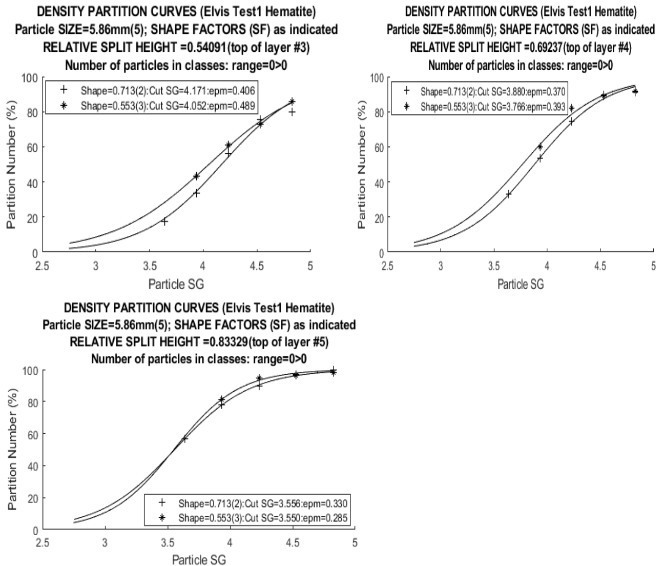
Figure 21: Effect of shape on partition curves in size class 5 (5.86mm) with 54%, 69% and 83% Yields (i.e., cutting the bed at the top of layers 3, 4 and 5).
