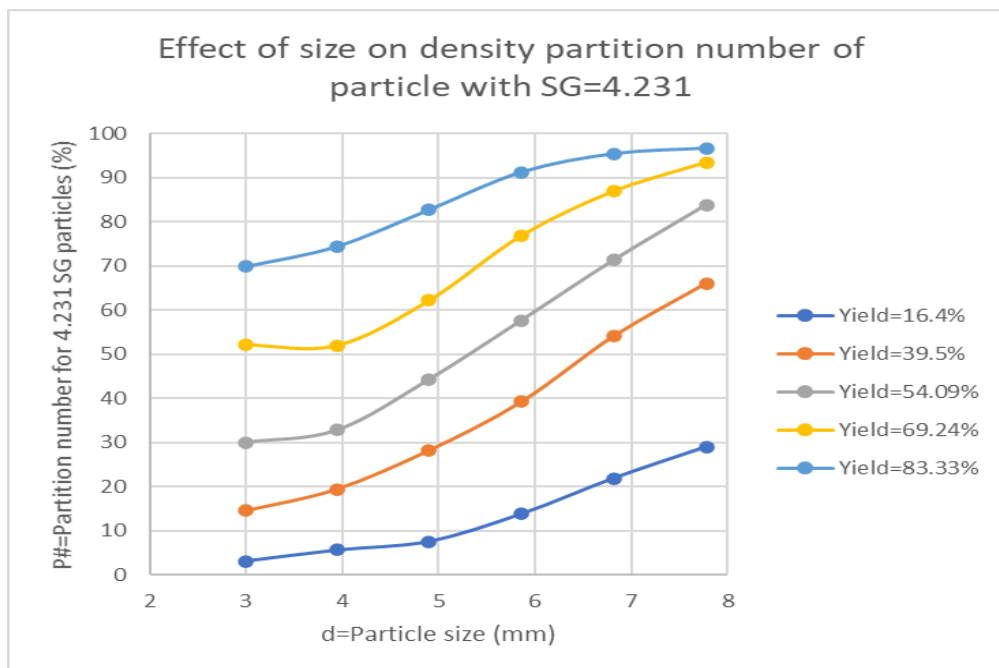
Figure 16: Graph showing the effect of particle size on density partition number of particles with SG=4.231
