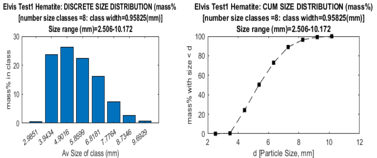
Figure 10: Size distribution graph.
