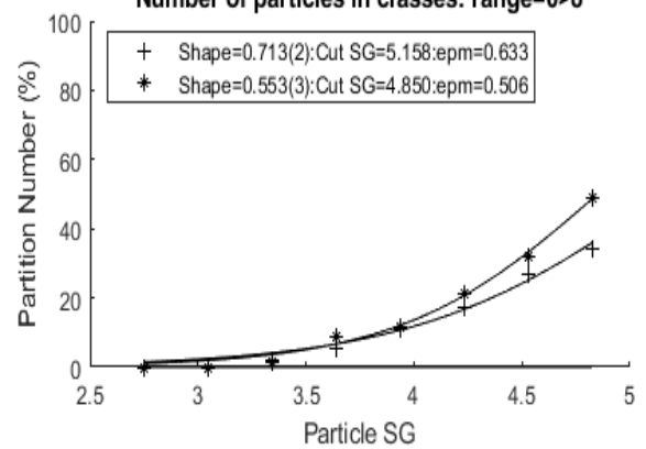
DENSITY PARTITION CURVES (Elvis Test1 Hematite) Particle SIZE=3.94mm(7); SHAPE FACTORS (SF) as indicated RELATIVE SPLIT HEIGHT =0.69237(top of layer #4) Number of particles in classes: range=0>8
