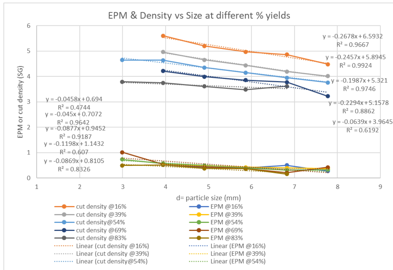
Figure 17: Effect of size on EPM & cut density at different %yield.
