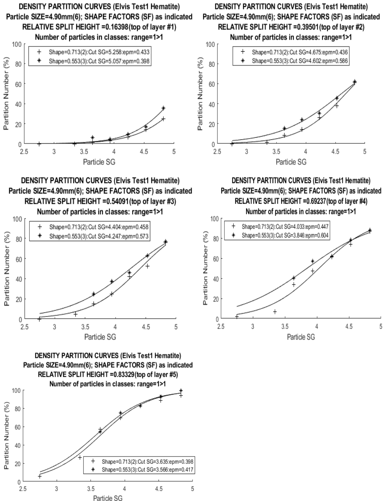
Figure 22: Effect of shape on density partition curves for size class 6 (4.9mm) particles for different yields.
