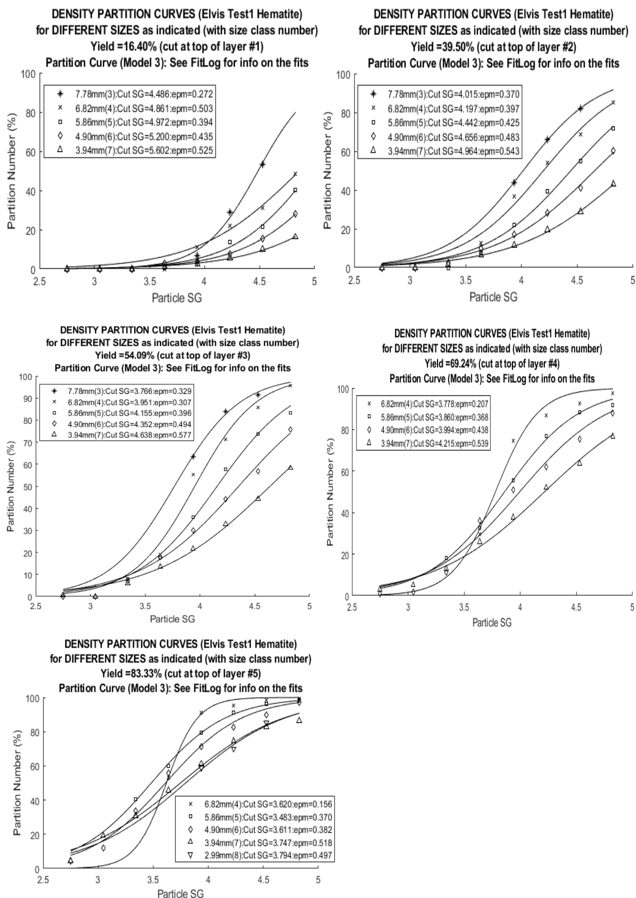
Figure 15: Density partition curves for different particle sizes for different yields.
