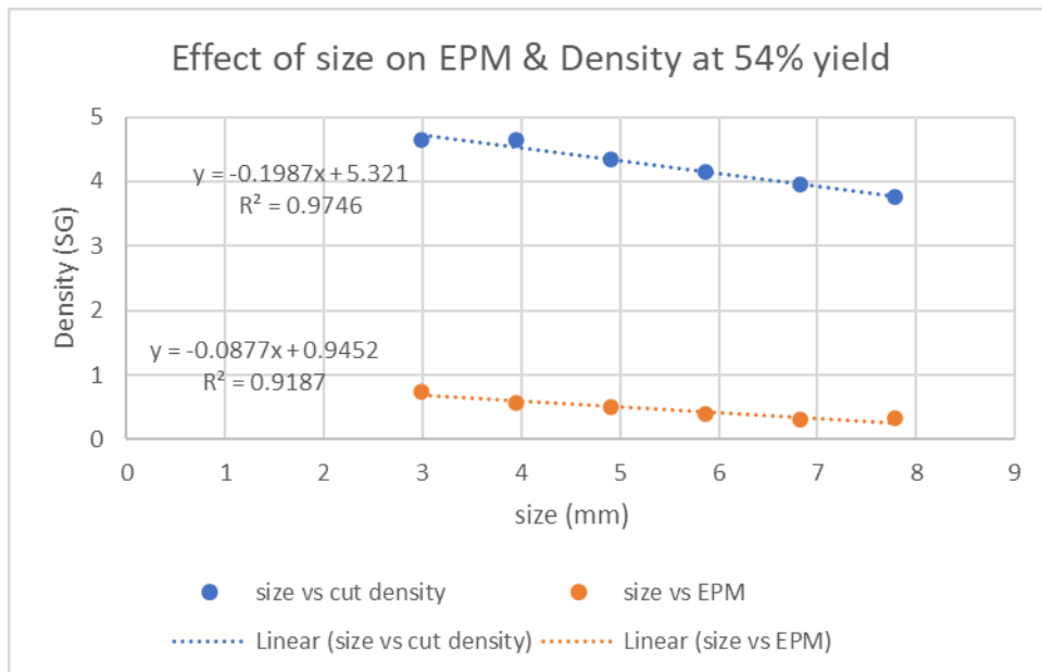
Figure 32: Effect of size on EPM and cut density at 54% yield.
