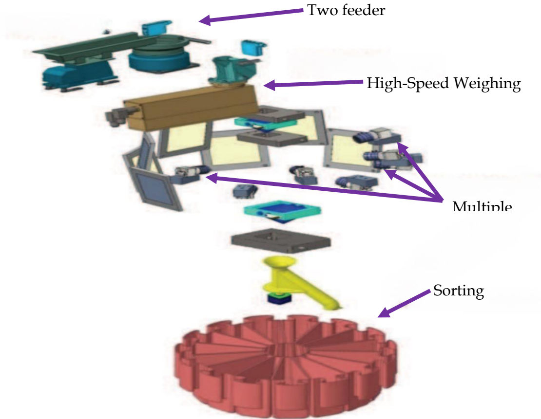
Figure 3: The multistage internal operations of the RhoVol device.
