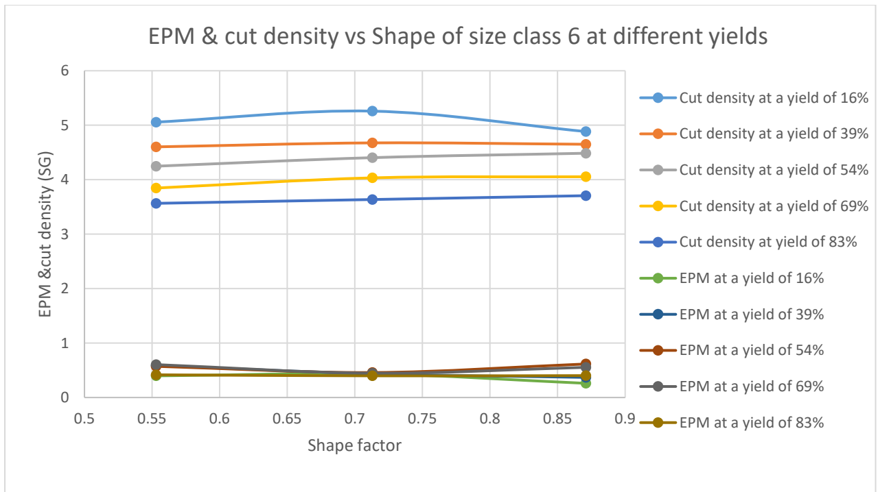
Figure 25: Effect of shape on EPM and cut density in size class 6 at different yields.
