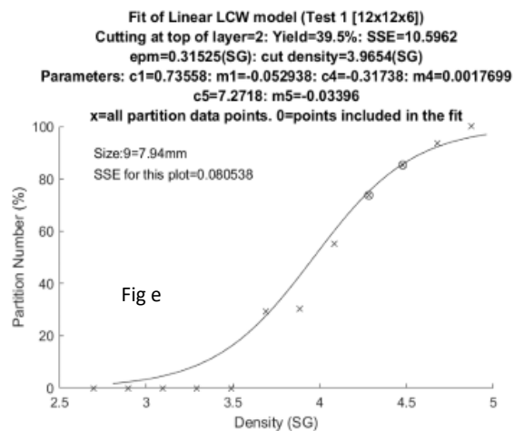
Figure 19: Example of fits of the overall linear model to the partition data. Crosses indicate partition numbers for all data points. Ringed crosses indicate which are 'reliable' because they are derived from classes with more than 50 particles.
