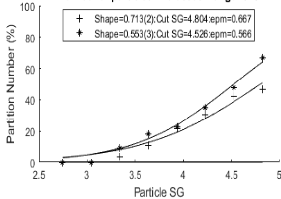
DENSITY PARTITION CURVES (Elvis Test1 Hematite) Particle SIZE=3.94mm(7); SHAPE FACTORS (SF) as indicated RELATIVE SPLIT HEIGHT =0.83329(top of layer #5) Number of particles in classes: range=0>8
