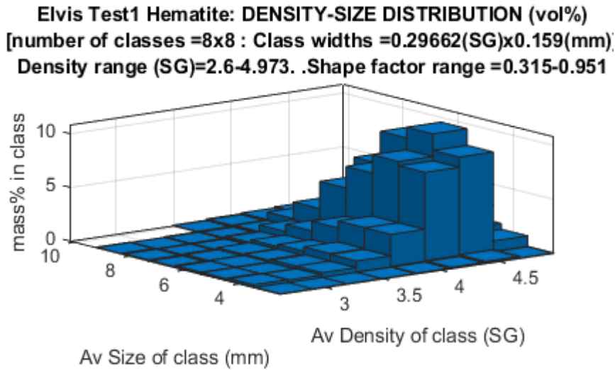
Figure 12: Density-Size 3D distribution.
