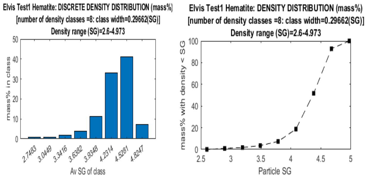
Figure 9: Density distribution graph.
