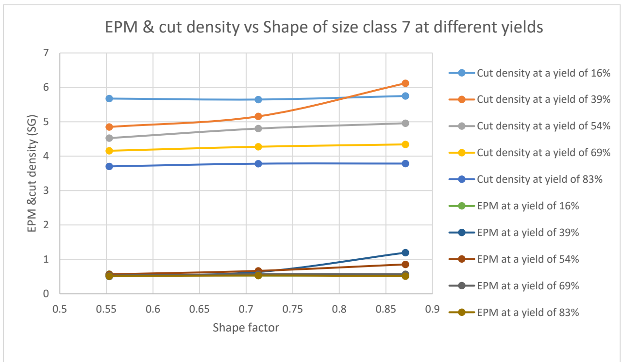
Figure 26: Effect of shape on EPM and cut density in size class 7 at different yields.
