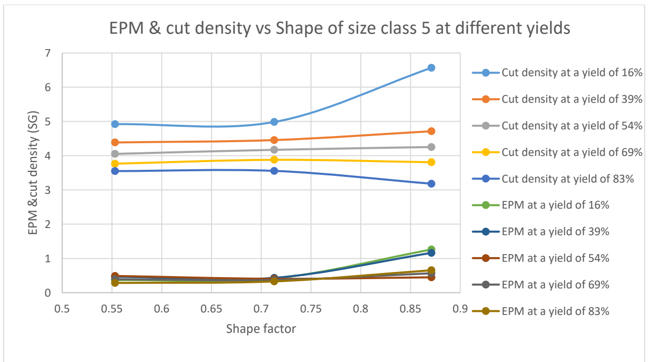
Figure 24: Effect of shape on EPM and cut density in size class 5 at different yields.
