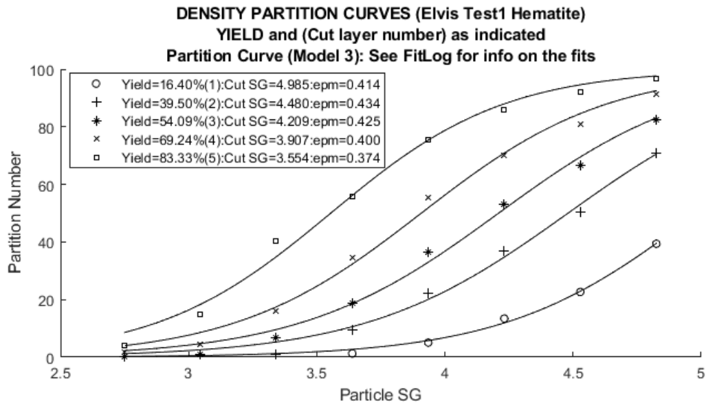
Figure 14: Density partition curve graph.
