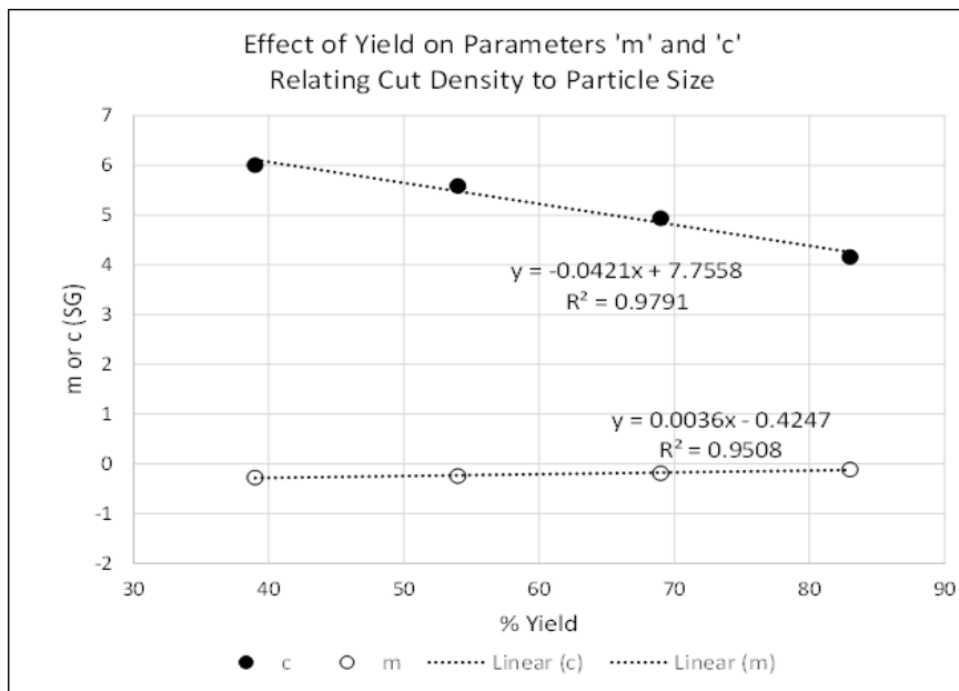
Figure 18: Effect of Yield on the linear fits of Cut density vs Particle size.
