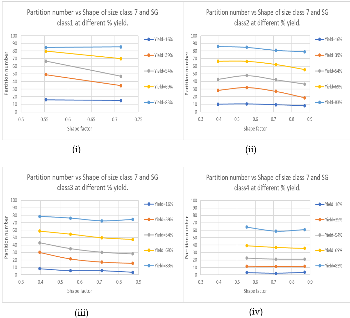
Figure 29: Effect of shape on size class 7 (3.94mm) and (i) SG class 1; (ii)SG class 2; (iii) SG class3; (iv) SG class 4 at different yields.
