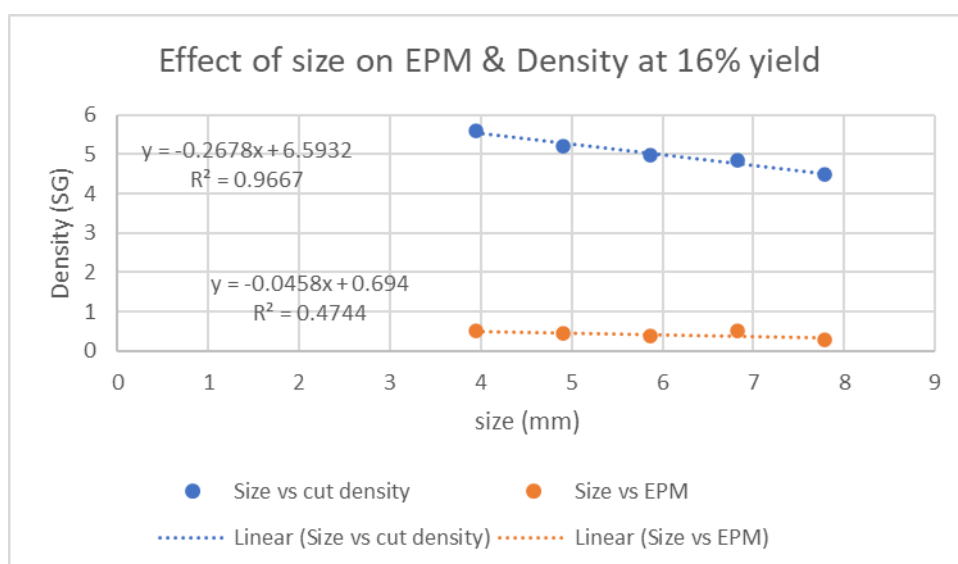
Figure 30: Effect of size on EPM and cut density at 16% yield.
