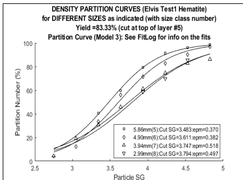
Figure 35: Partition Curves for different sizes.
