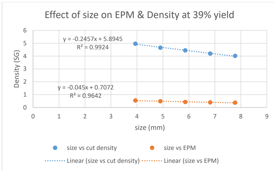
Figure 31: Effect of size on EPM and cut density at 39% yield.
