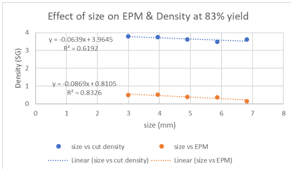
Figure 34: Effect of size on EPM and cut density at 83% yield.
