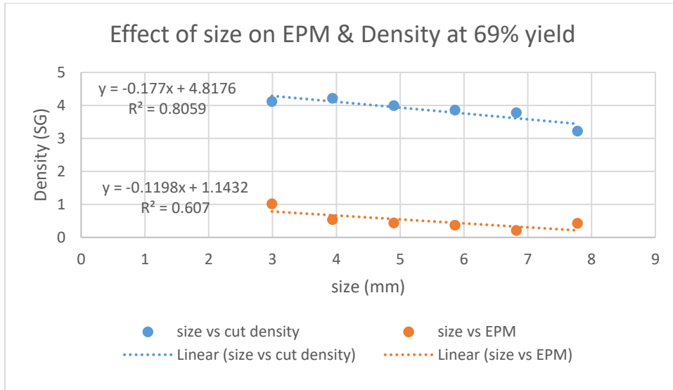
Figure 33:Effect of size on EPM and cut density at 69% yield.
