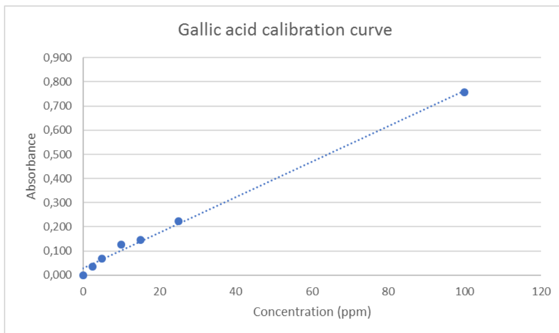
Figure 2.7 Gallic acid standard calibration curve
