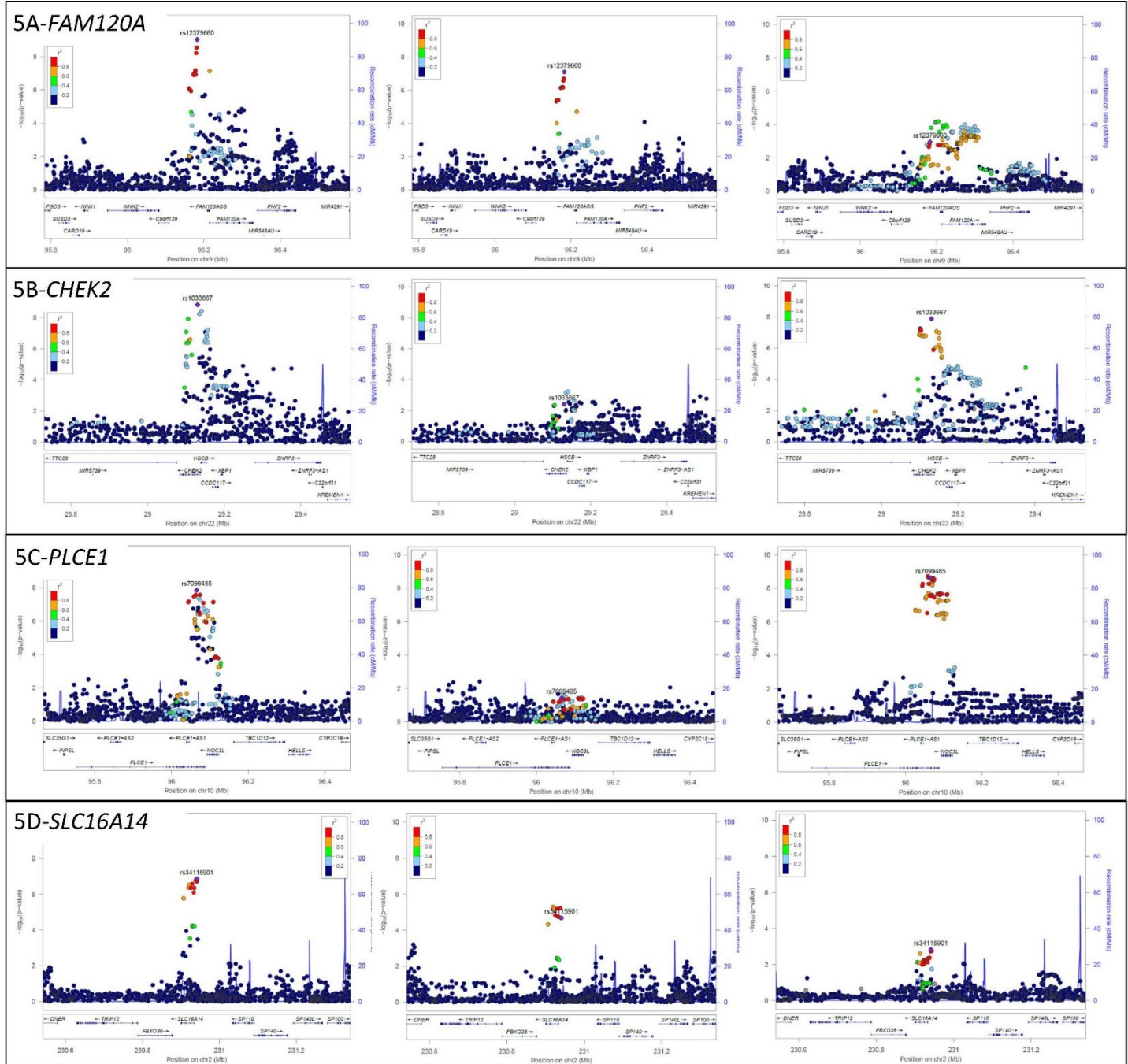
Figure 5.5. Meta-analysis Locus zoom plots.
