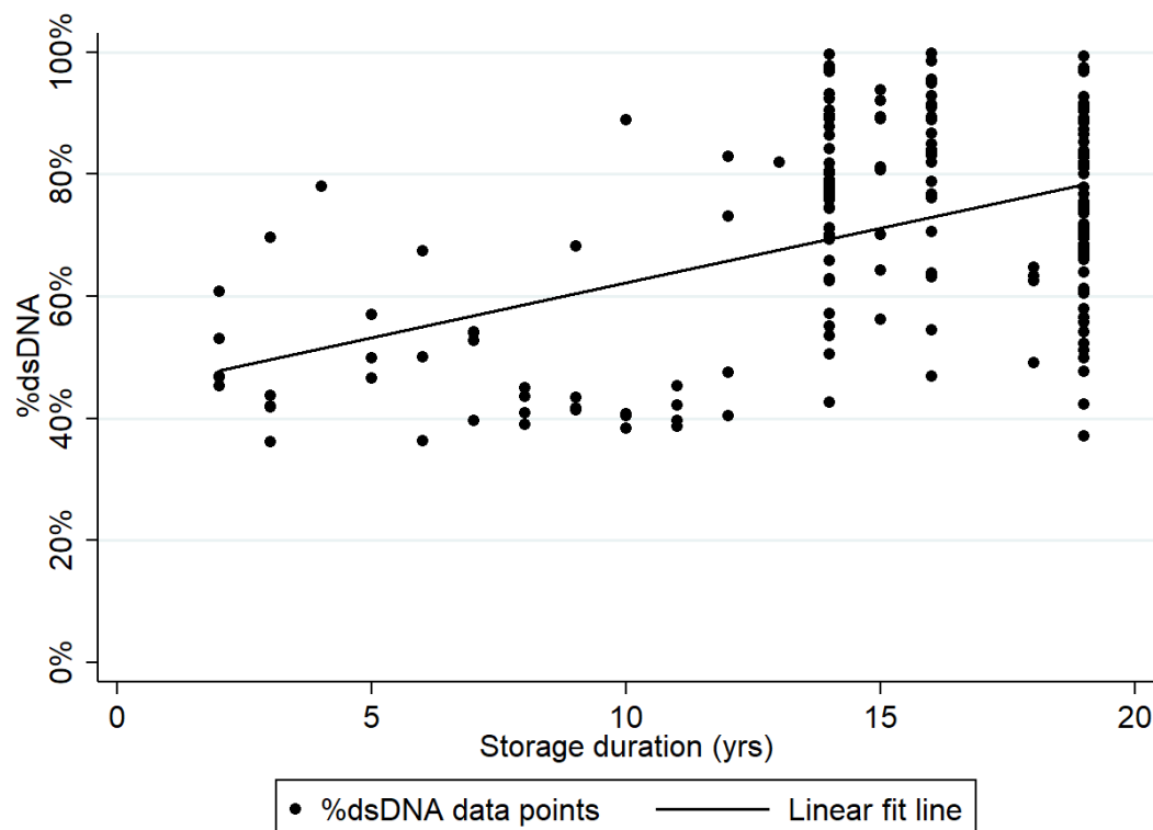
Figure 3.2. %dsDNA vs storage duration.
