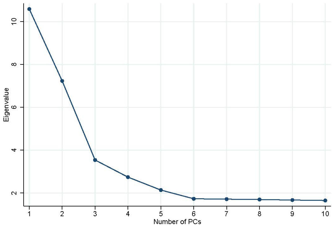
Supplementary figure 5.1. The eigenvalues for Principal component analysis of OSCC GWAS.
