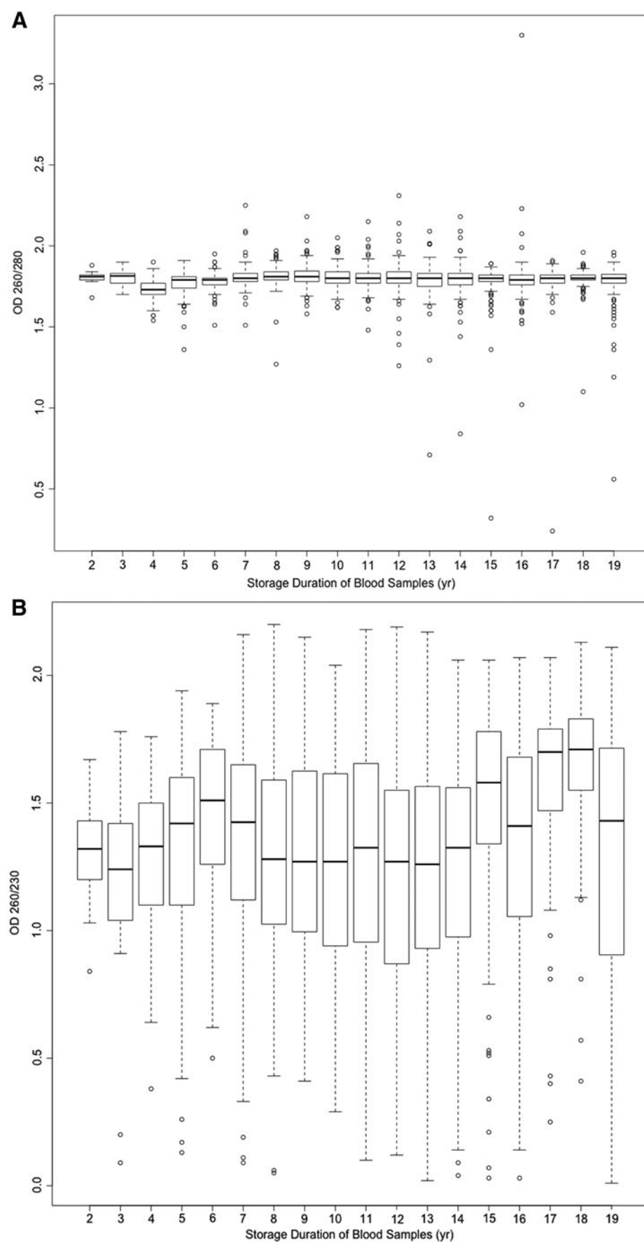
FIG. 4. (A) A260/280 ratio distribution of all samples across duration of blood sample storage. A260/280 ratios were measured by NanoDrop. (B) A260/230 ratio distribution of all samples across duration of blood sample storage. A260/230 ratios were measured by NanoDrop.
