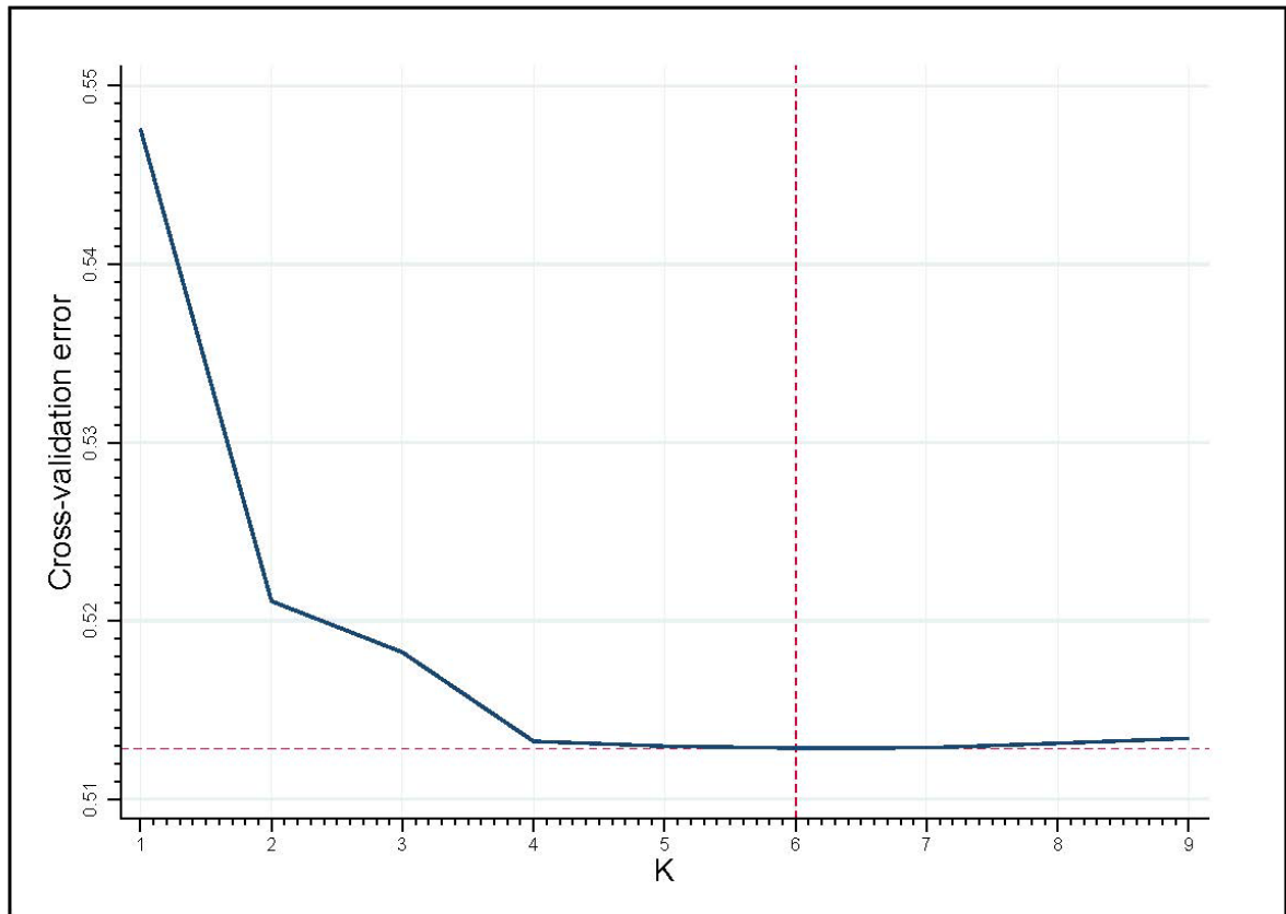
Supplementary figure 5.4. Cross-validation errors for Admixture analysis, for K=1 to K=9. Optimal K=6, with the lowest cross-validation error of 0.51286.
