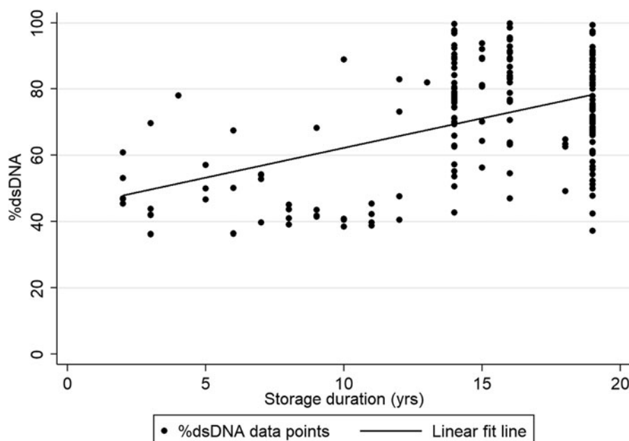
FIG. 3. %dsDNA versus storage duration. The linear fit line indicates that a positive trend exists between %dsDNA and the increase of storage duration. %dsDNA, percentage of double-stranded DNA.
