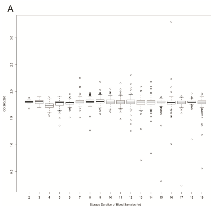
Figure 3.4. A260/280 ratios distribution of all samples across the duration of blood sample storage.
