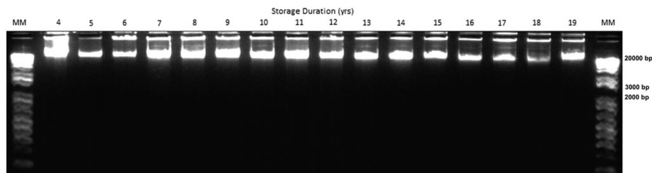
FIG. 1. Gel image showing integrity of genomic DNA from 4 to 19 years of blood sample storage. One representative sample was used from each year of storage (4–19 years). Two microliters of genomic DNA was resolved on 1.0% agarose gel with GelRed™ staining. GeneRuler™ 1 kb plus DNA Ladder MM was used for sizing reference. Electrophoresis was done at 8 V/cm for 45 minutes. MM, molecular marker.
