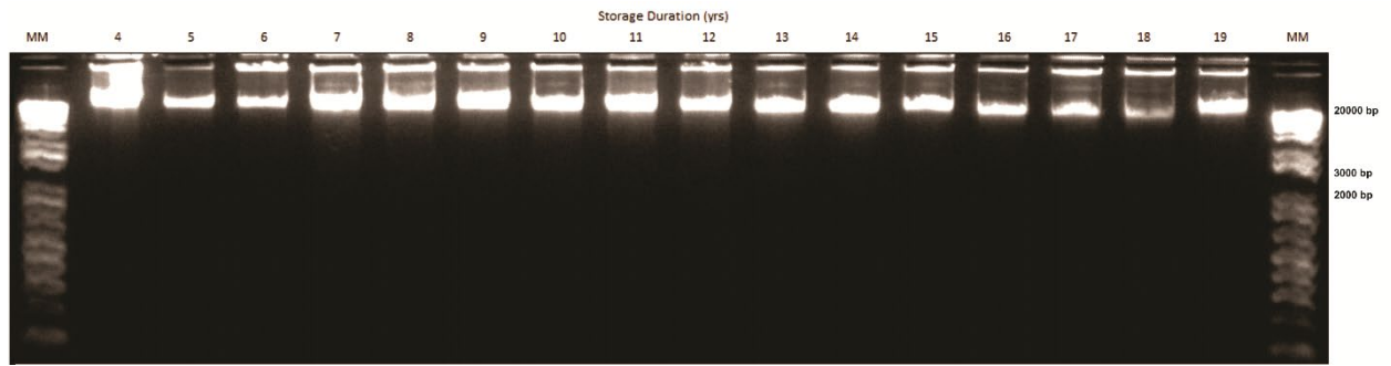
Figure 3.1. Gel image showing the integrity of genomic DNA from 4 years to 19 years of blood sample storage.
