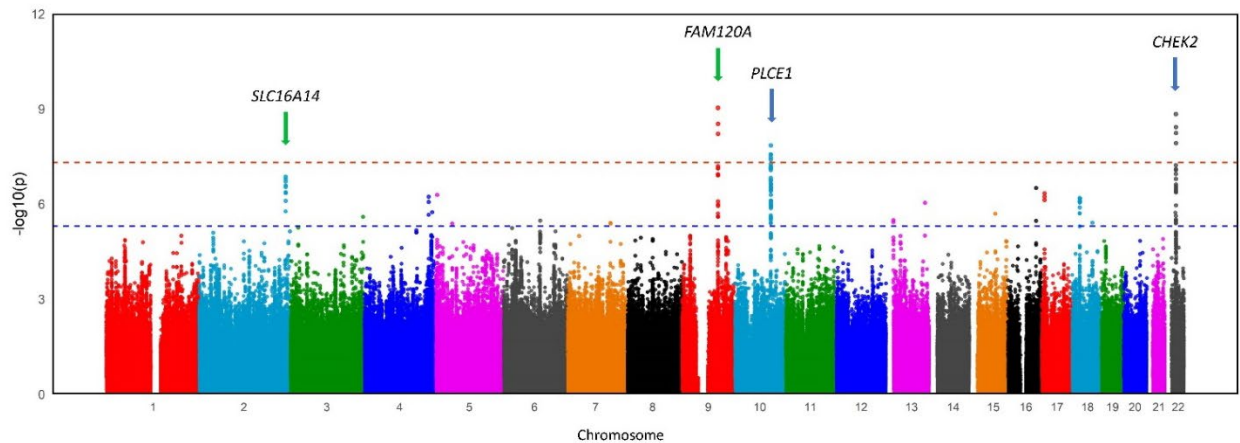
Figure 5.4. Meta-analysis Manhattan plot for African OSCC and Chinese OSCC.
