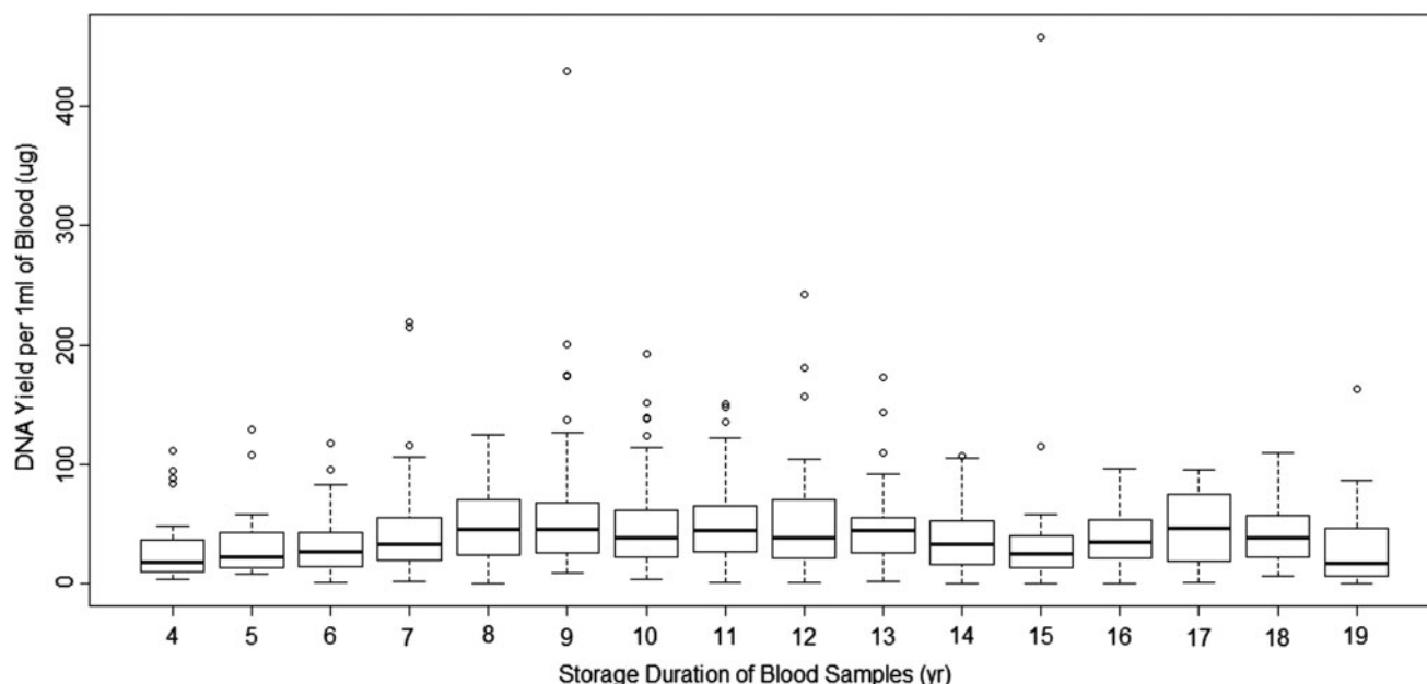
FIG. 2. Range and distribution of DNA yields per 1 mL of blood extracted from frozen whole blood stored over 4–19 years. Blood volume data were not available for 2 and 3 years of storage. No statistically significant difference in yield was observed across the duration of blood storage. DNA yields were measured by NanoDrop. TM
