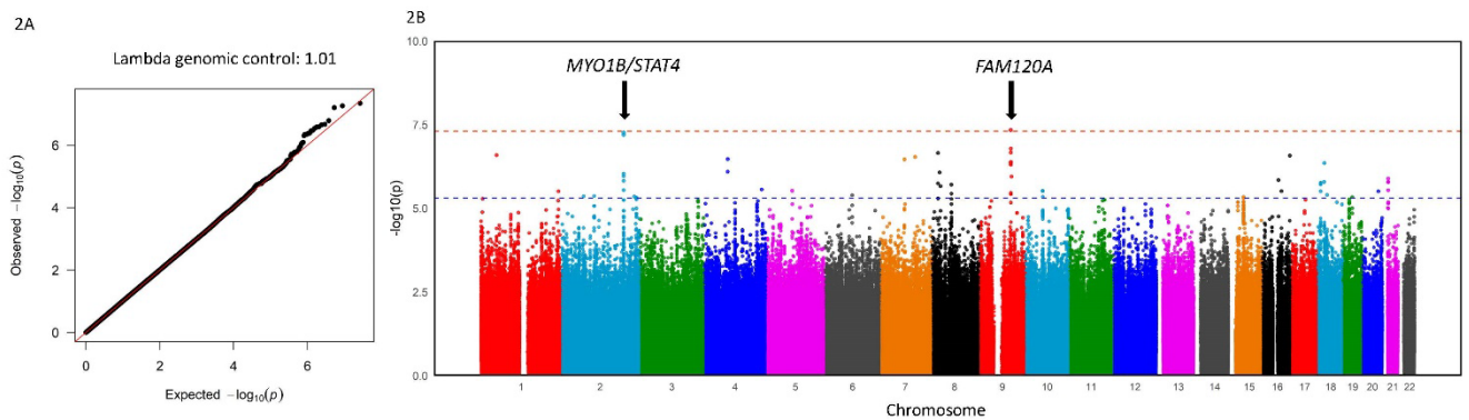
Figure 5.2. Quantile-Quantile and Manhattan plot of the African OSCC GWAS.
