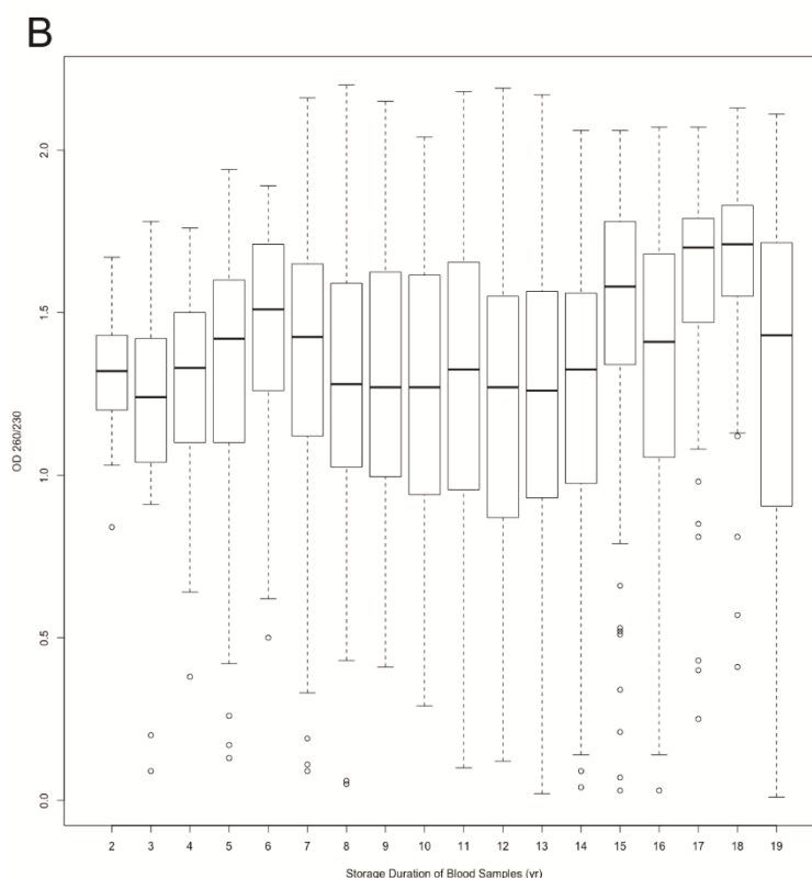
Figure 3.5. A260/230 ratios distribution of all samples across the duration of blood sample storage. A260/230 ratios were measured by NanoDrop.
