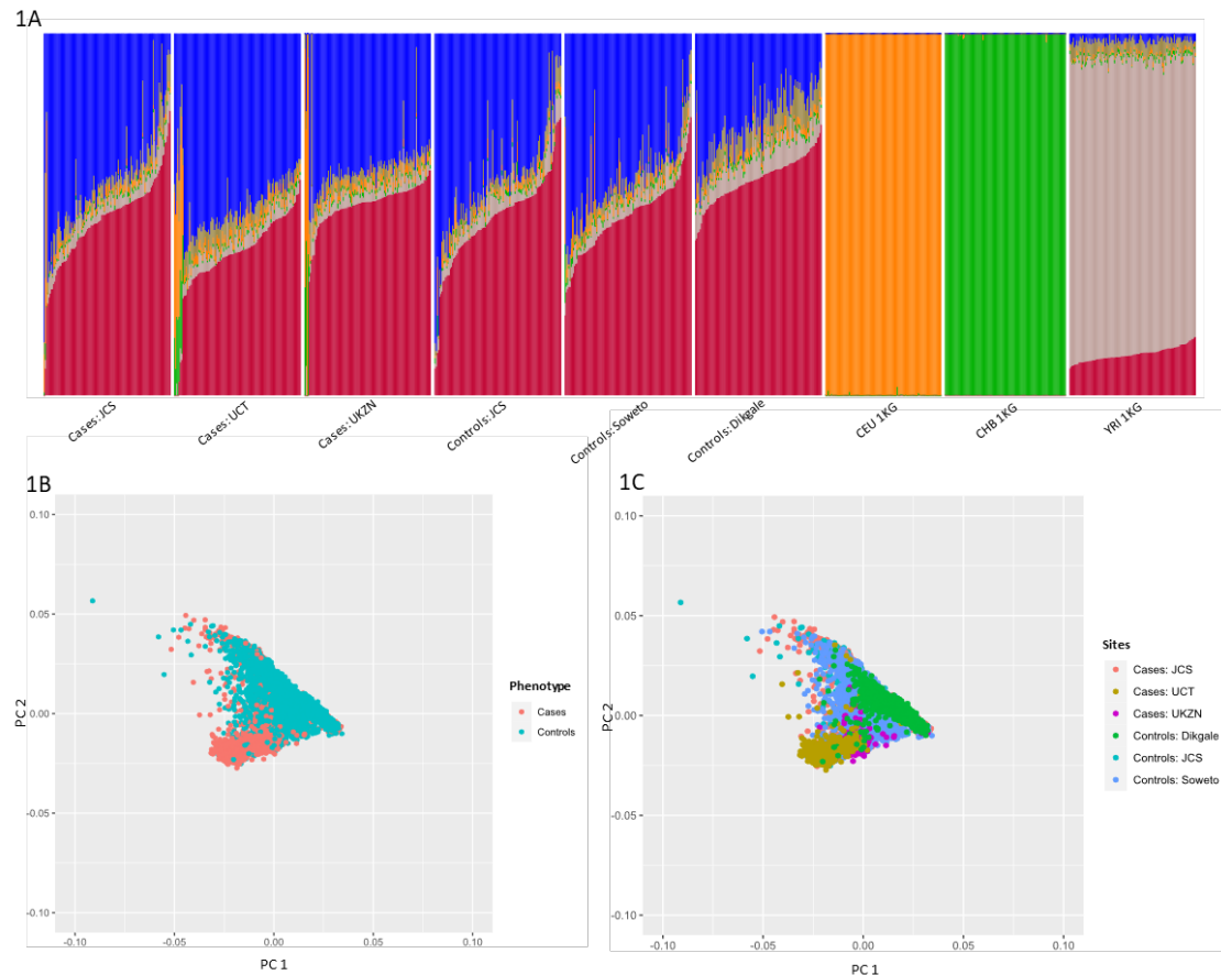
Figure 5.1. Admixture and Principal component plots of OSCC cases and controls.
