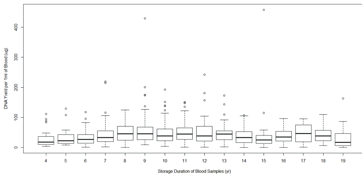
Figure 3.3. Range and distribution of DNA yields per 1ml of blood, extracted from frozen whole blood stored over 4 to 19 years.
