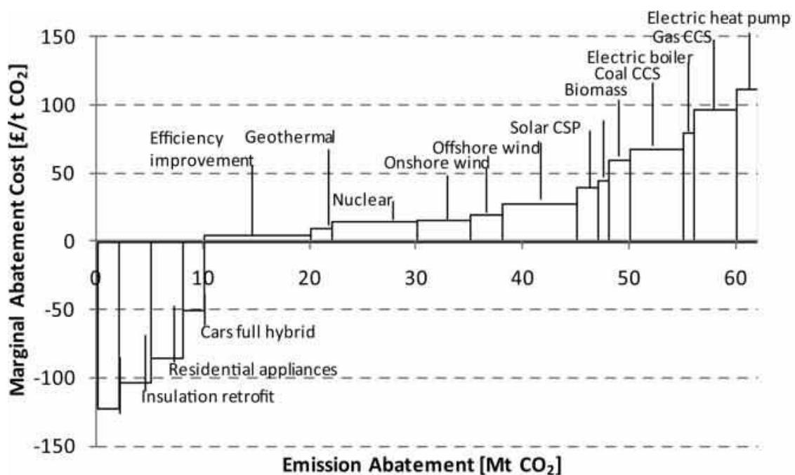
Fig. 9: Stylised example of a MACC curve (Kesicki and Ekins, 2011)
