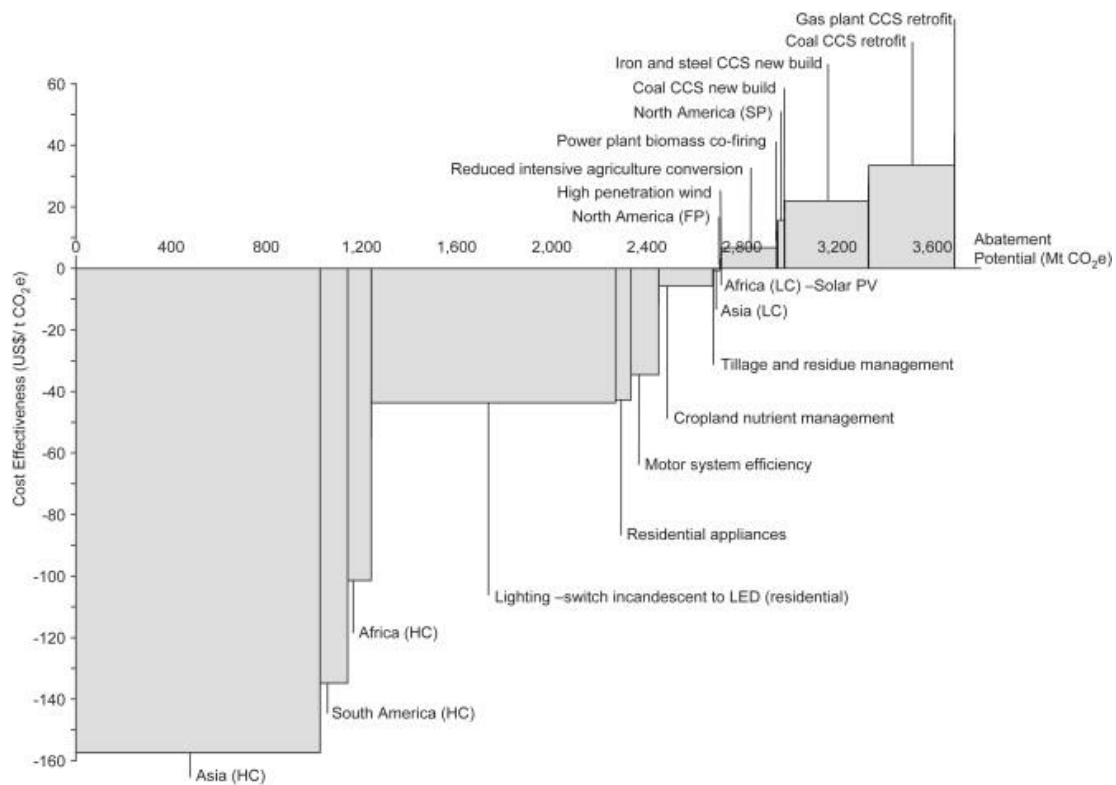
Fig. 8: The MACC of a range of carbon-abatement technologies and strategies for the world by 2030 (Pratt and Moran, 2010)
