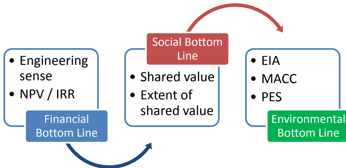
Fig. 10: TBL Workflow
