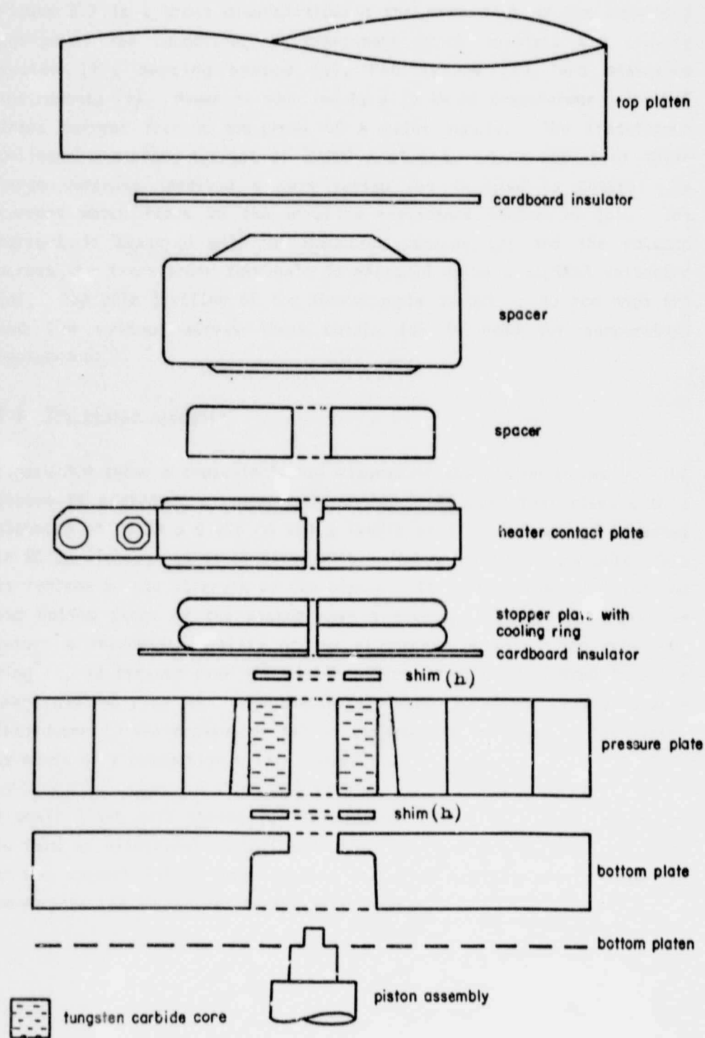
Fig. 3.6 The cylinder stack
