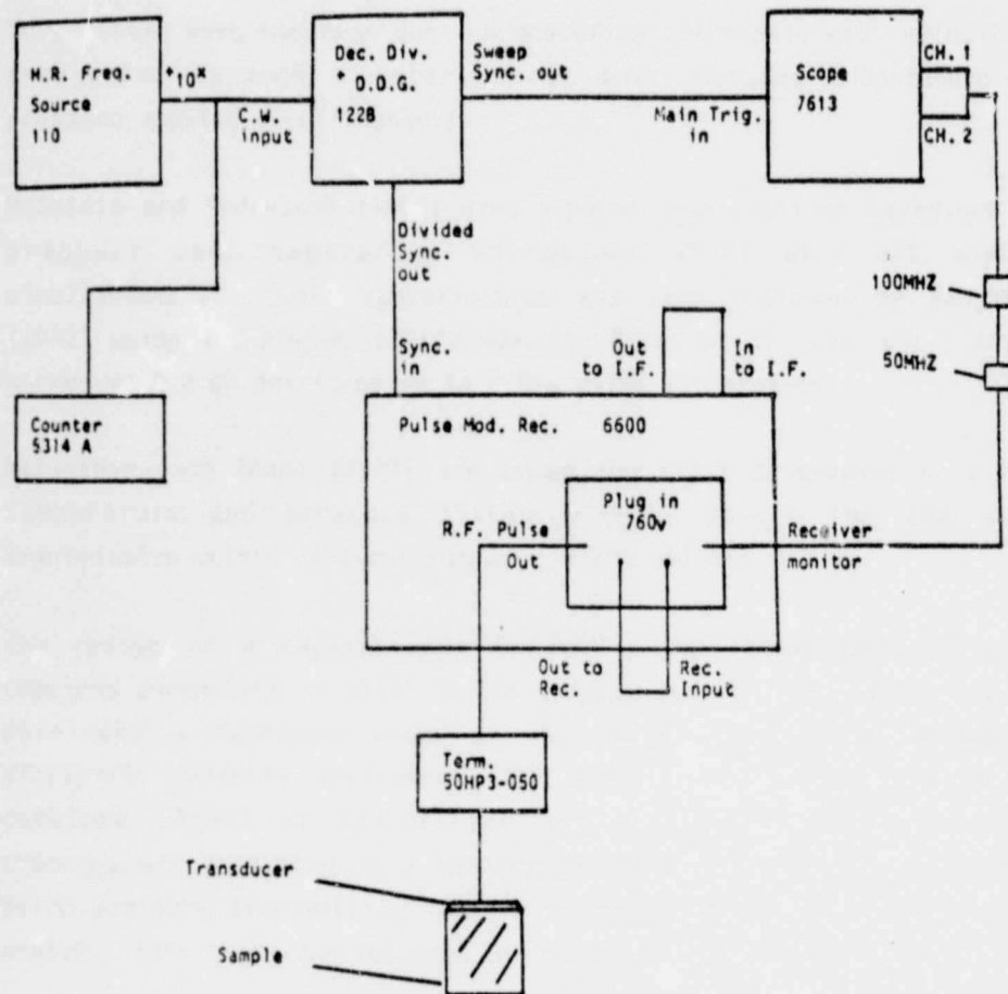
Fig. 3.3 Circuit diagram of the MATEC system
