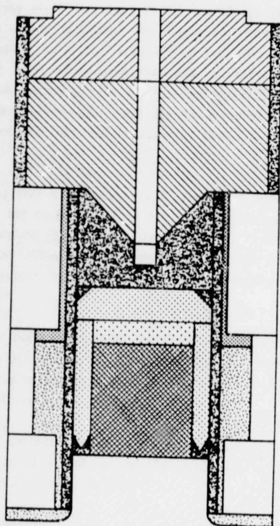
Fig. 3.9(b) Assembly diagram of capsule
