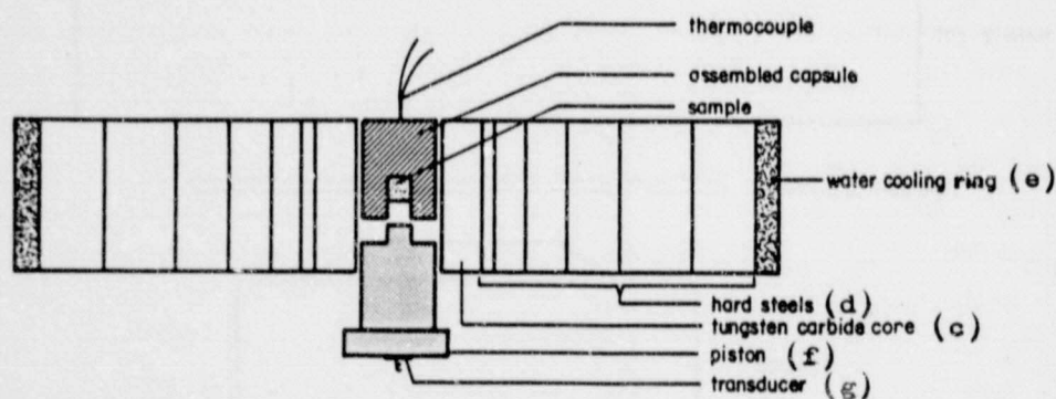
Fig. 3.5 Main components, capsule, piston and cylinder
