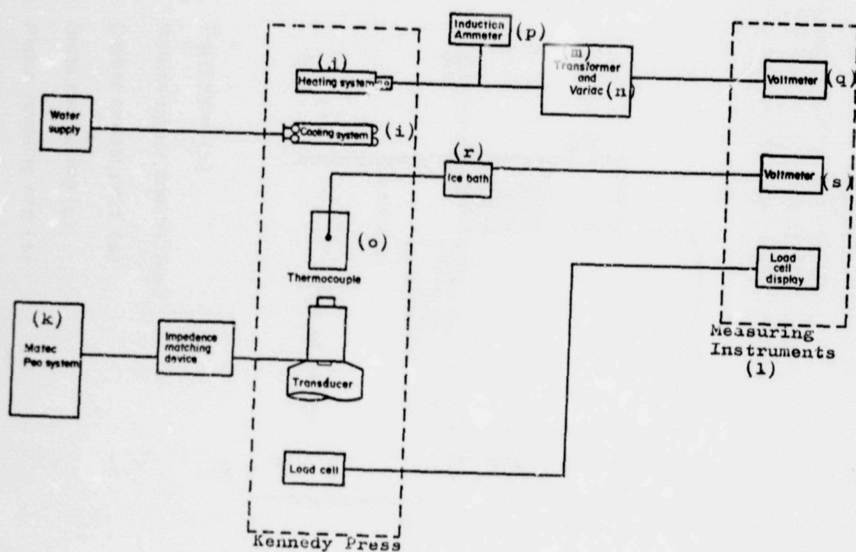
Fig. 3.7 Block diagram of the auxiliary equipment
