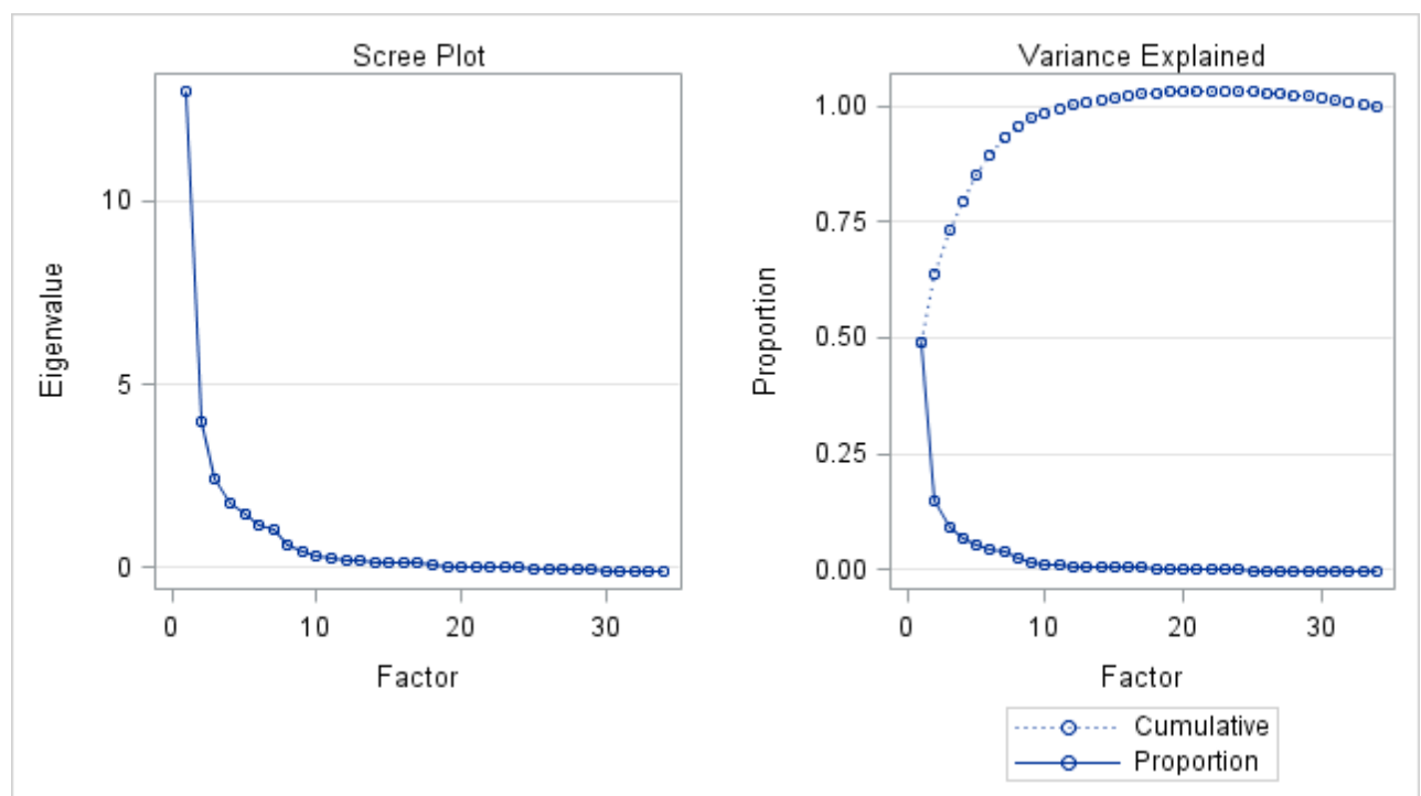
Figure 13: Scree plot showing factor structure.
