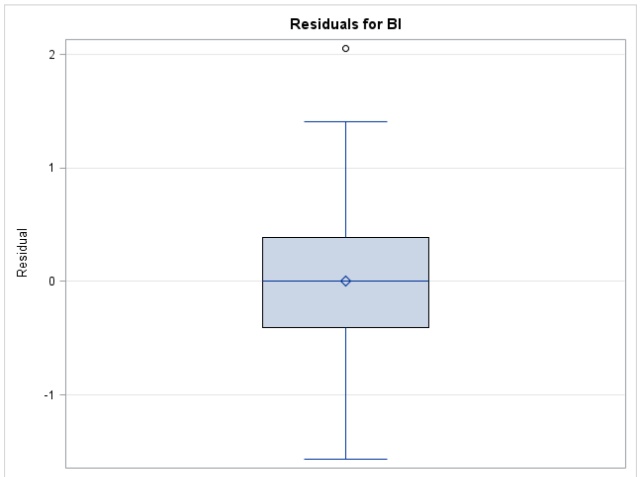
Figure 17: Residuals for BI.
