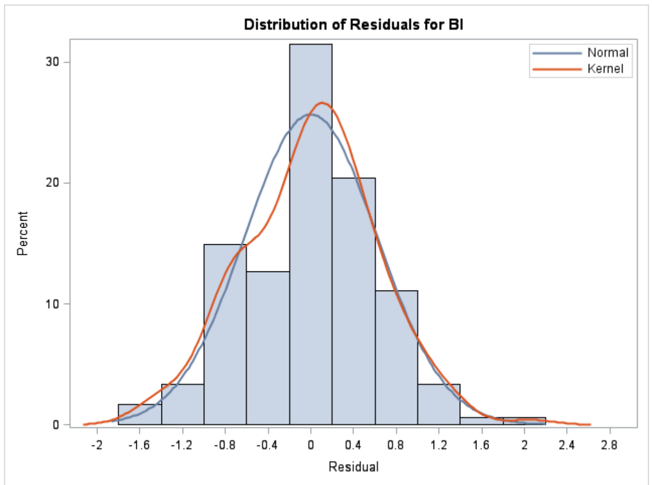
Figure 15: Distribution of Residuals for BI.
