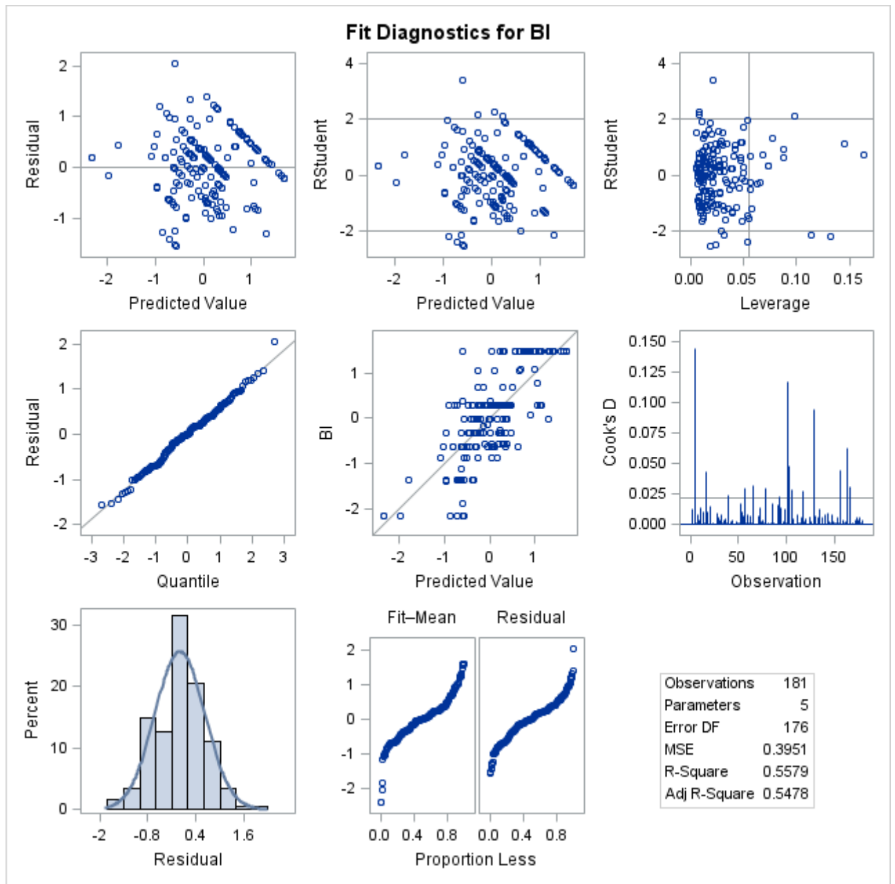
Figure 18: Fit diagnostics for BI.
