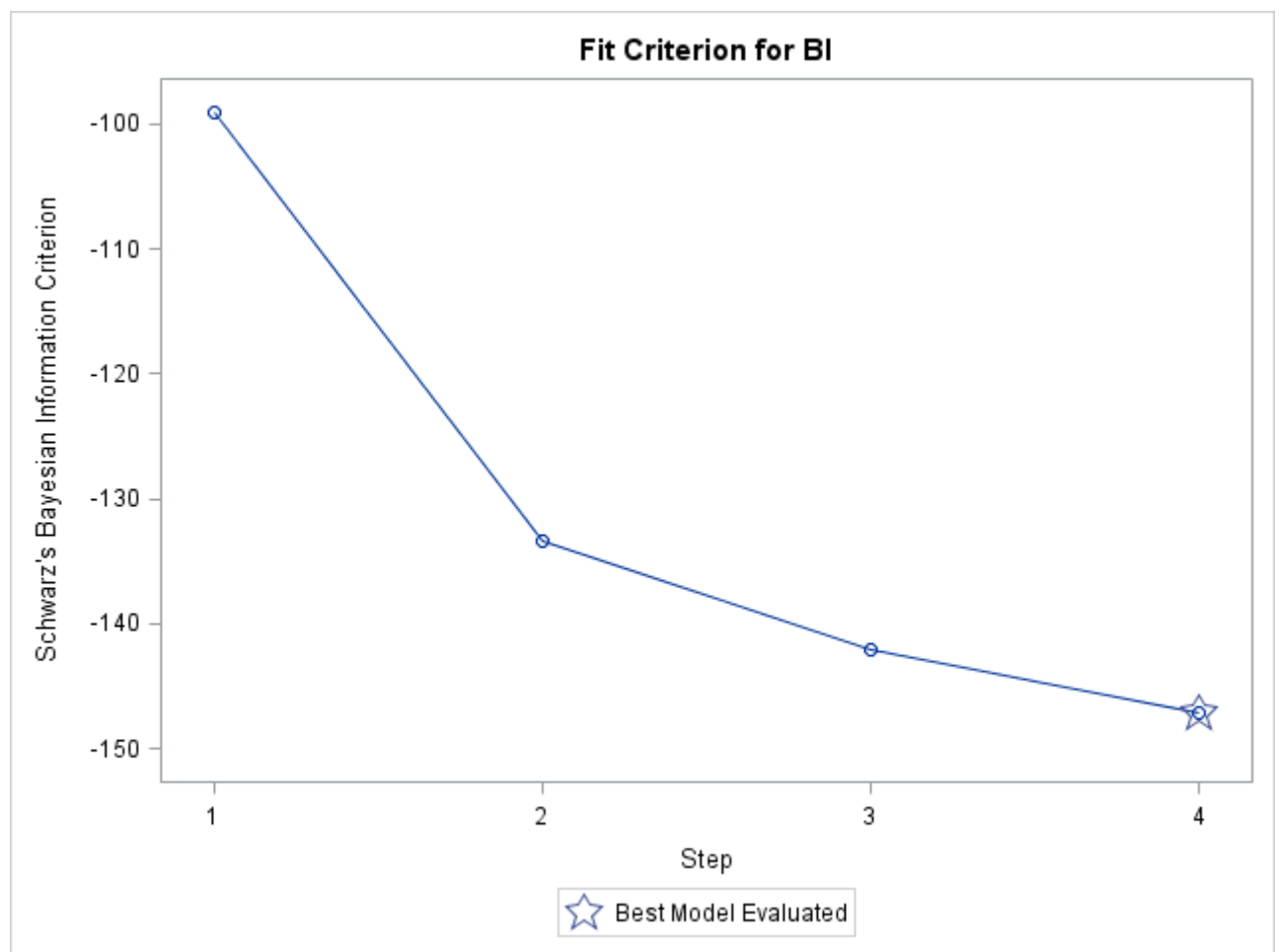
Figure 16: Fit Criterion for BI.
