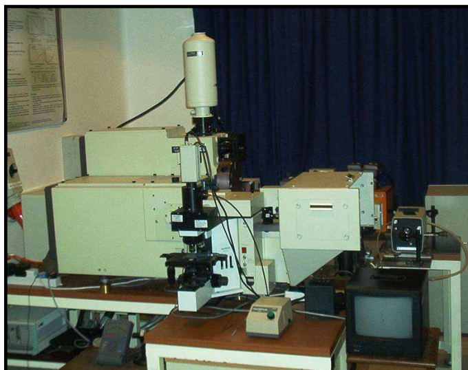
Figure 3.8: Image of Jobin-Yvon T64000 Raman spectrometer.
