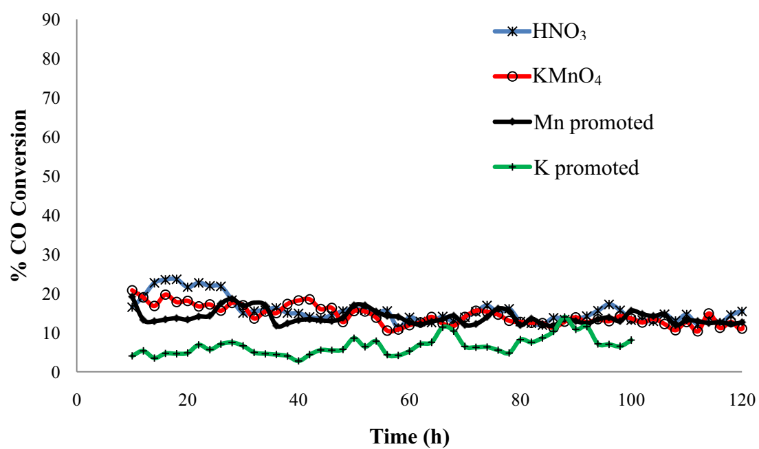
Figure B6: % CO conversion of 5 % Co/CS catalysts.
