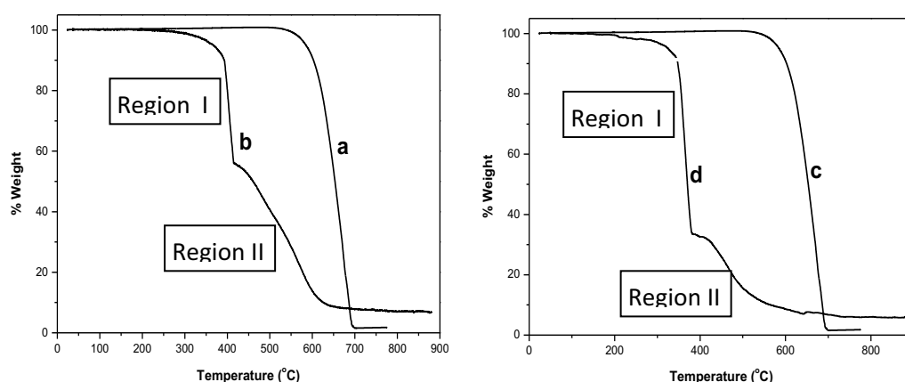
Figure 5.5: TGA profile run in air on the (a) HNO 3 functionalised CSs, (b) 5 % Co/CS catalysts functionalised by HNO 3 , (c) KMnO 4 functionalised CSs and (d) 5 % Co/CS catalysts functionalised by KMnO 4 .
