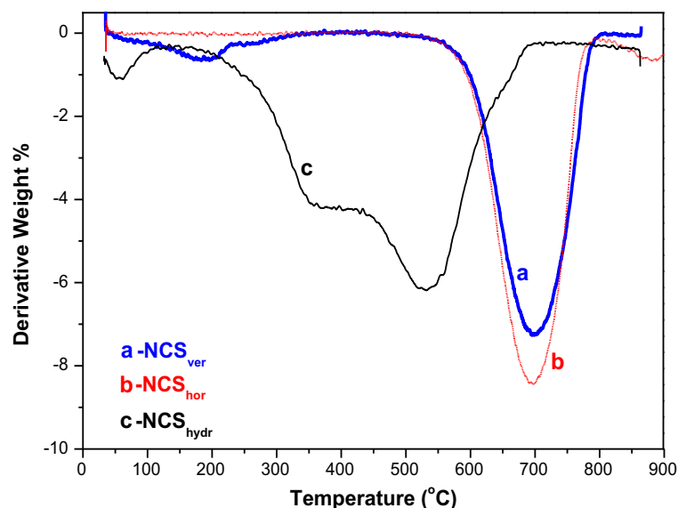
Figure 7.6: TGA profiles of as-synthesised (a) NCS ver (b) NCS hor and (c) NCS hydr run in air
