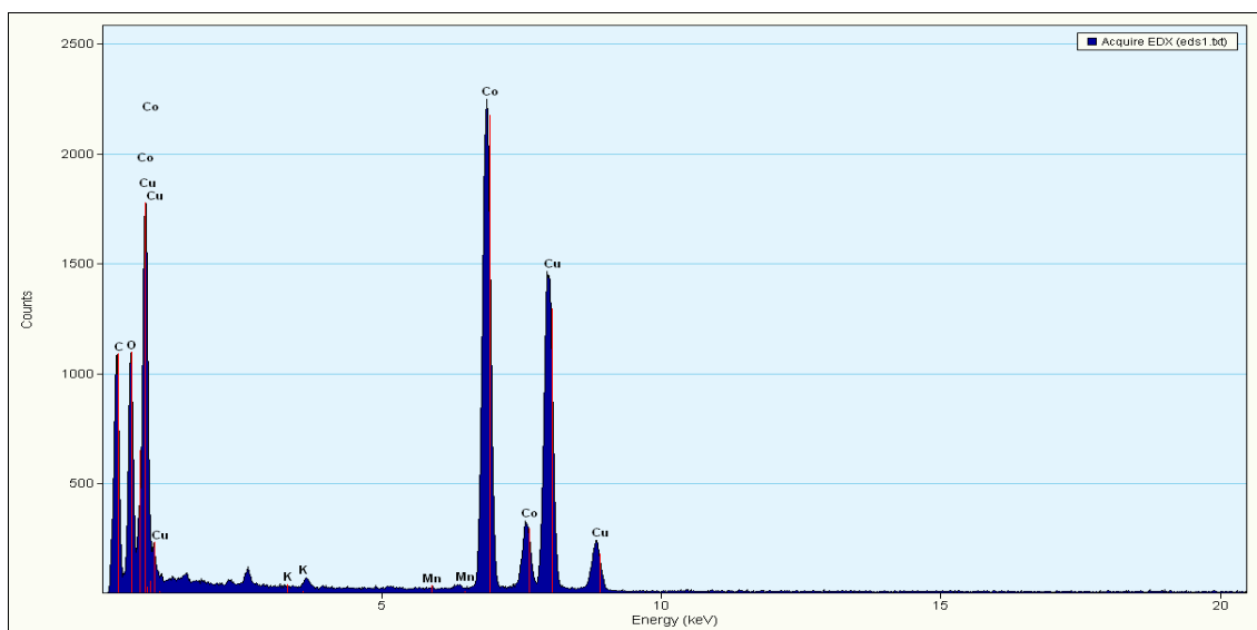
Figure 5.9: EDS spectrum of 5% Co/CS \text{KMnO}_4 .
