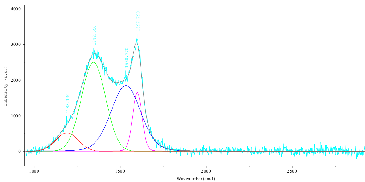
Figure C6: Raman spectra of CS hydr annealed at 800 °C under N 2 for 2.5 h.
