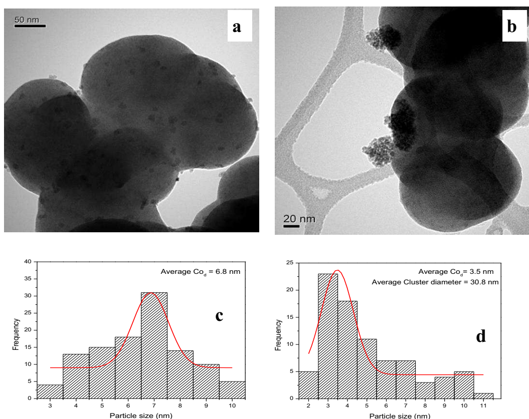
Figure 5.8: TEM images of (a) 5% Co/CS \text{KMnO}_4 functionalised and (b) 5% Co/CS \text{HNO}_3 functionalised catalysts.
