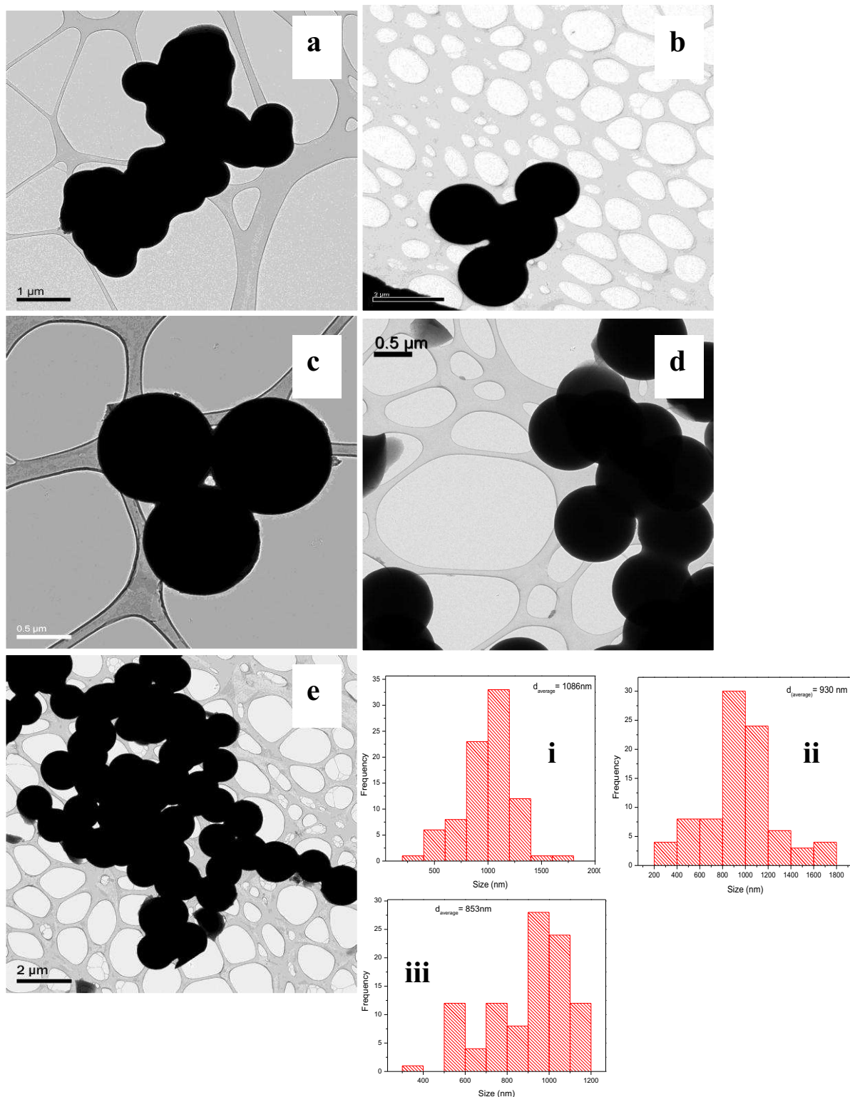
Figure 6.3: Effect of annealing temperature (a) 250, (b) 350, (c) 450, (d) 600 and (e) 800 °C for 2.5 h under N 2 gas and size distribution for (i) 250, (ii) 450 and 600 °C annealed CS hydr .
