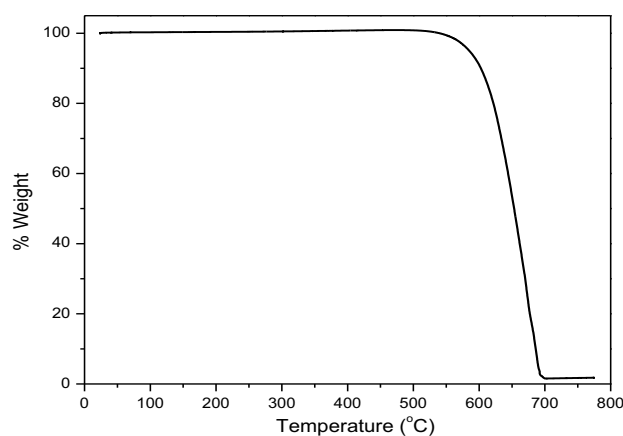
Figure 4.6: TGA of as-synthesised CSs run in air
