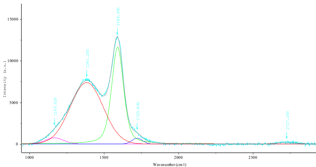
Figure C4: Raman spectra of CS hydr annealed at 450 °C under N 2 for 2.5 h.
