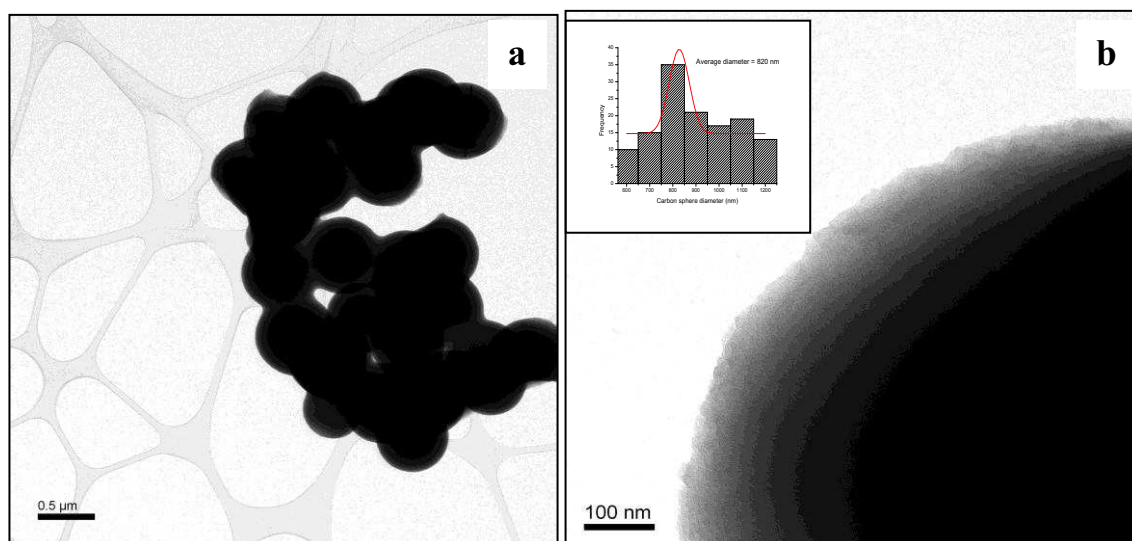
Figure 6.1: TEM images of as-prepared CS hydr (a) low magnification and (b) high magnification (insert: particle size distribution bar chart).
