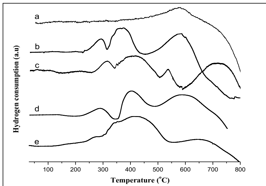
Figure 5.6: H 2 -TPR profiles of (a) As-synthesised CSs, (b) 5% Co/CS HNO 3 functionalised CS, (c) 5% Co/CS KMnO 4 functionalised CS, (d) 5% Co/ 0.05%K/ HNO 3 functionalised CS and (e) 5% Co/0.05%Mn/ HNO 3 functionalised CS.
