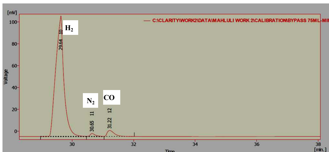
Figure 3.14: GC-TCD trace of syngas calibration H 2 (60%), N 2 (10%) and CO (30%)
