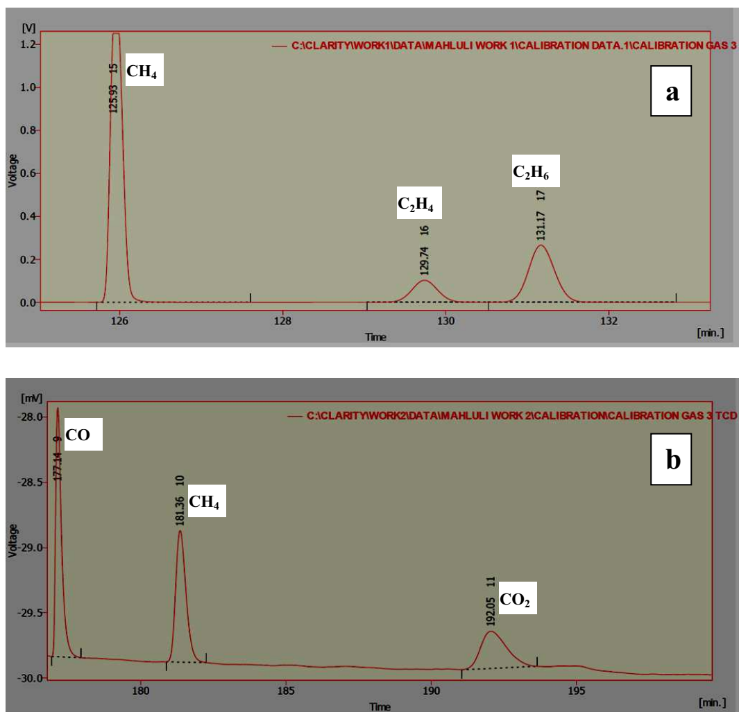
Figure 3.13: (a) GC-FID and (b) GC-TCD trace of calibration gas with CH 4 (2.5%), C 2 H 4 (0.2%), C 2 H 6 (0.5%), CO (10.0%), CO 2 (5.0%) and balance of Ar gas composition.
