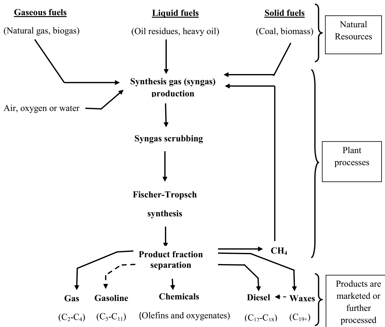
Figure 2.1: Industrial process overview for the production of fuels and chemicals by FTS [8].
