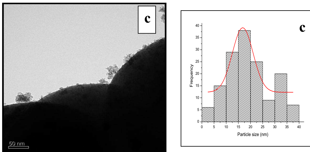
Figure 7.8: TEM images and particle size distribution for 5 % Fe supported on (a) NCS ver , (b) NCS hor and (c) NCS hydr
