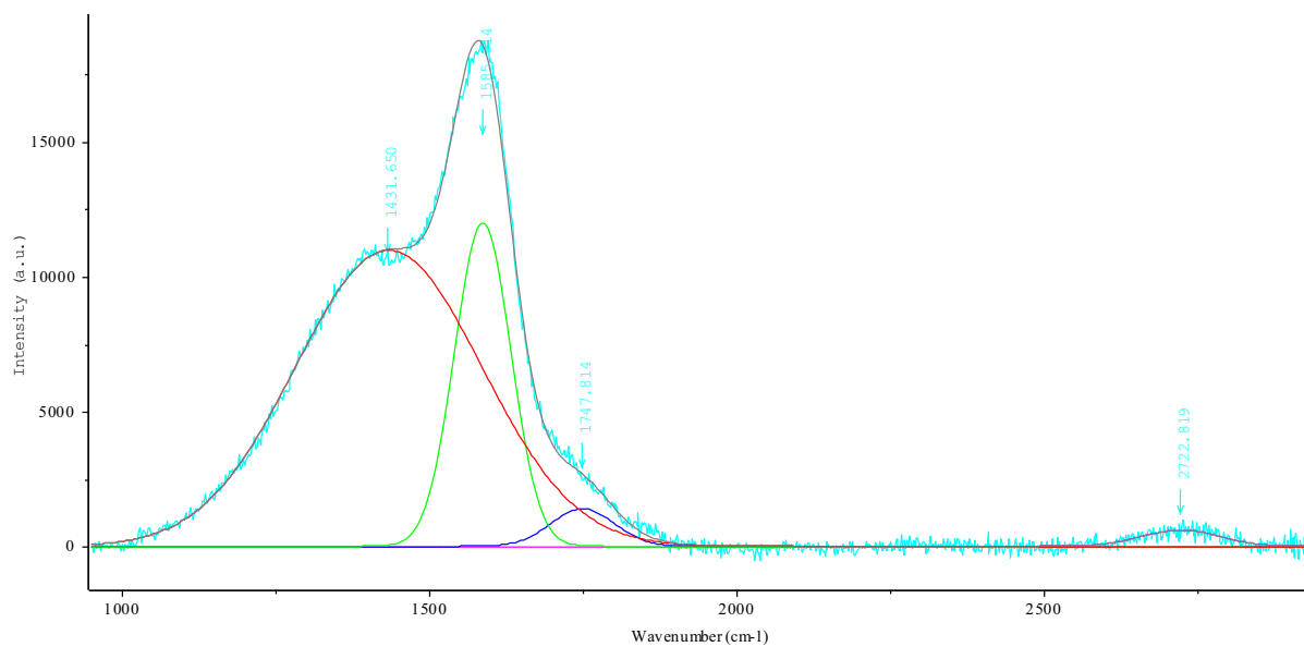
Figure C1: Raman spectra of CS hydr annealed at 250 °C under N 2 for 2.5 h.
