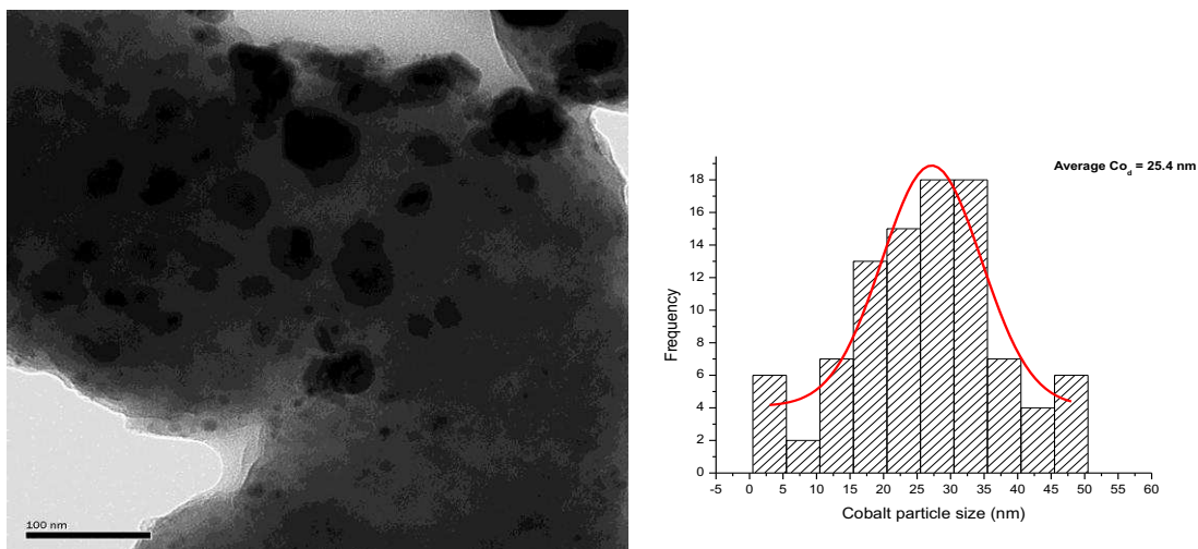
Figure 5.15: TEM images and particle size distribution of HNO 3 functionalised catalyst after 120 h on stream.
