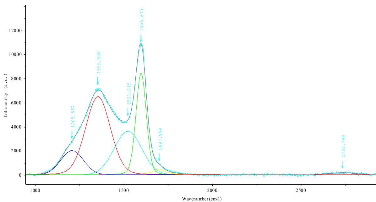
Figure C5: Raman spectra of CS hydr annealed at 600 °C under N 2 for 2.5 h.
