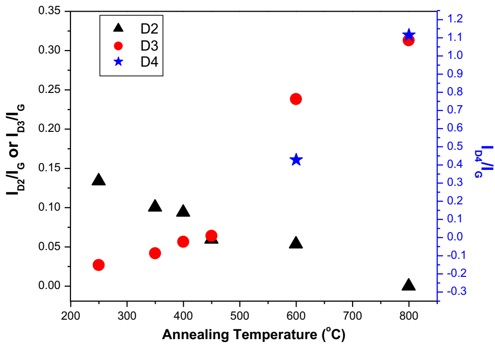
Figure 6.9: Effect of annealing temperature on I_{Di}/I_G -bands
