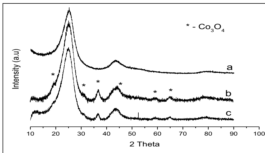
Figure 5.4: XRD patterns for (a) As-synthesised CSs, (b) 2.5% Co/CS HNO 3 functionalised CS, (c) 2.5% Co/CS KMnO 4 functionalised CS.
