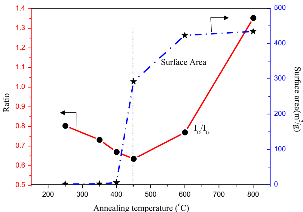
Figure 6.6: Effect of annealing temperature on surface area and crystallinity of CS_{hydr} .
