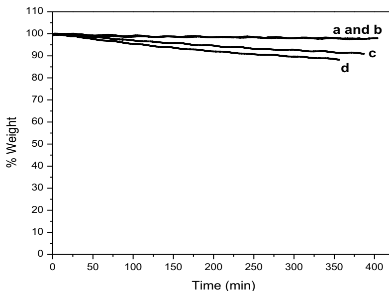
Figure B2: TGA profile of 5 % Co/CS run for 6 h under (a) air at 250 °C, (b) oxygen at 250 °C, (c) air at 300 °C and (d) oxygen at 300 °C.
