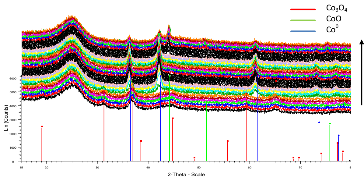
Figure B3: In-situ XRD patterns of reduction of \text{Co}_3\text{O}_4 phases in 5 % Co/CS \text{HNO}_3 catalyst at 350 °C for 24 h in 5 % \text{H}_2 (balance \text{N}_2 gas).
