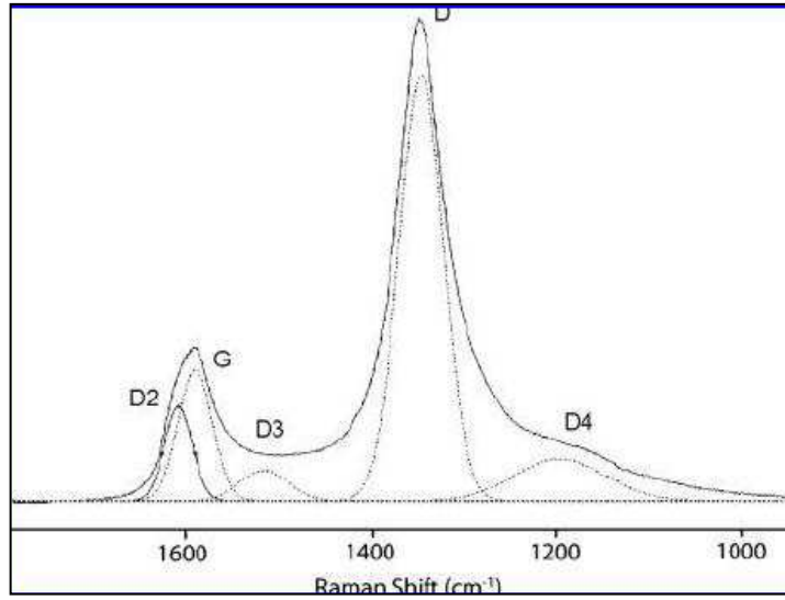
Figure 6.8: Example of computer deconvoluted G and D bands [12].
