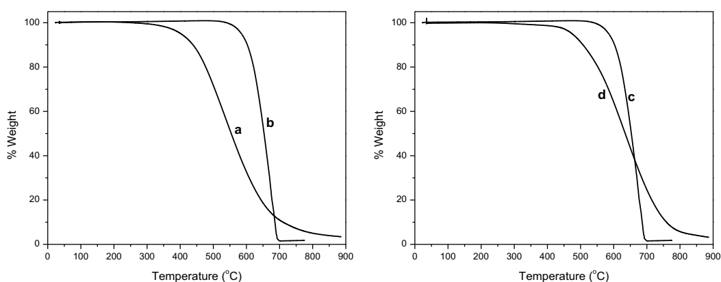
Figure 5.3: TGA profile run in air of (a) 5 % Co/CS catalysts functionalised by KMnO 4 . (b) KMnO 4 functionalised CSs, (c) HNO 3 functionalised CSs and (d) 5 % Co/CS catalysts functionalised by HNO 3 ,
