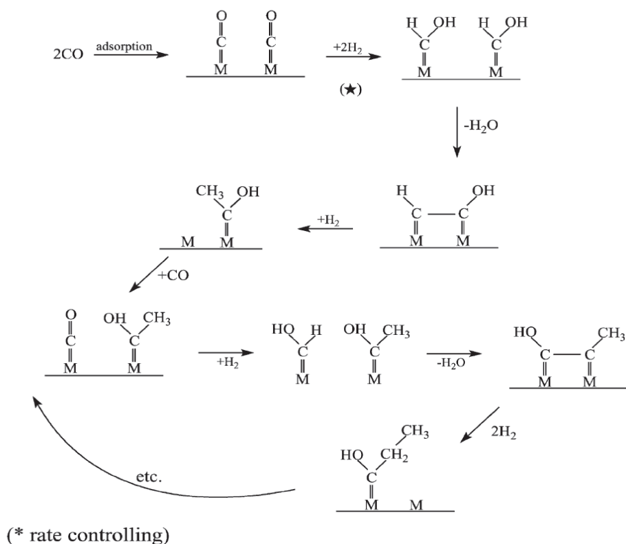
Figure 2.4: Schematic diagram showing the enol mechanism [23, 31]
