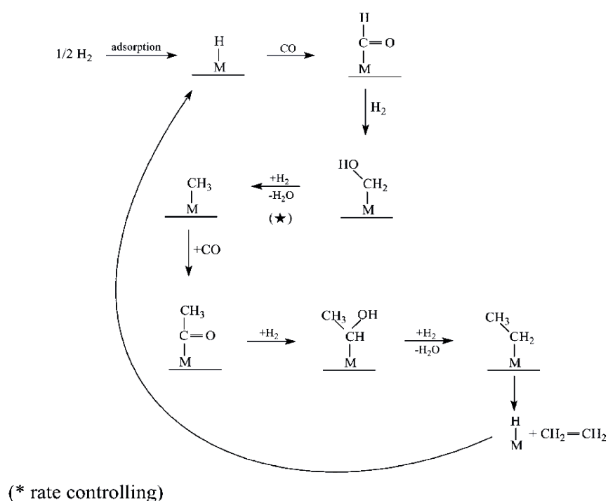
Figure 2.3: schematic diagram of the -CO insertion mechanism [23]
