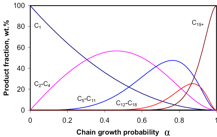
Figure 2.6: Theoretical product selectivity as a function of chain growth probability [47-48]
