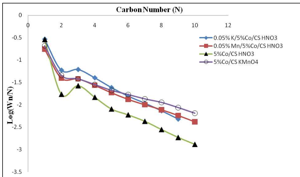
Figure 5.12: ASF distribution for (a) 5% Co/CS KMnO 4 , (b) 5% Co/CS HNO 3 , (c) 0.05% Mn/ 5 % Co/CS HNO 3 and (d) 0.05% K/ 5 % Co/CS HNO 3 .
