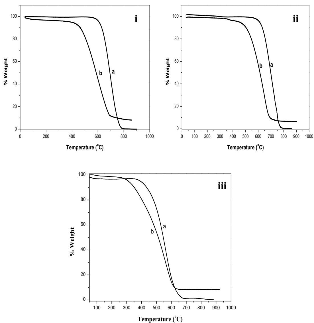
Figure 7.9: TGA profiles run in air of (a) as synthesised NCSs (b) 5% Fe catalyst supported on (i) NCS ver , (ii) NCS hor and (iii) NCS hydr .
