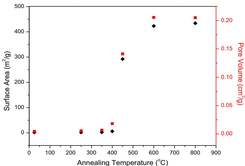
Figure 6.5: Effect of annealing temperature on surface area and pore volume.
