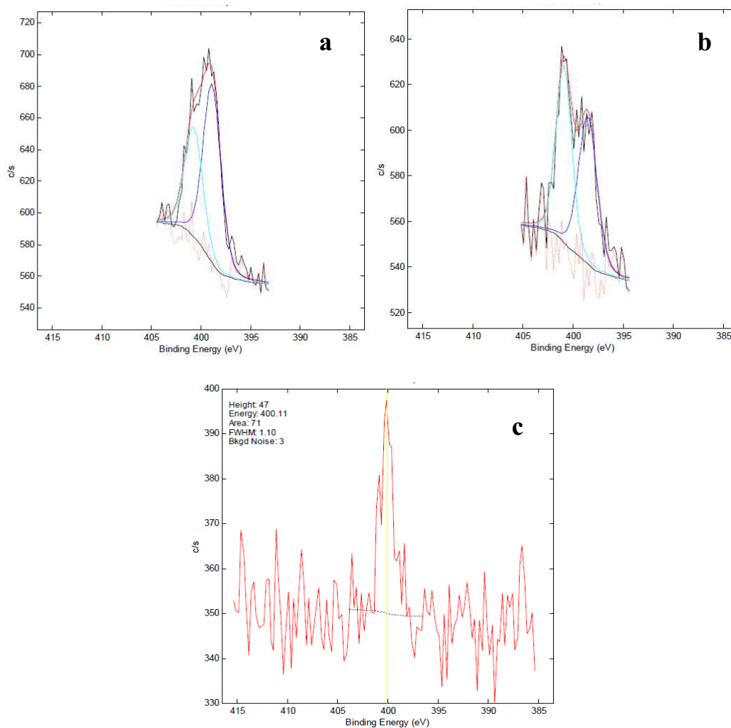
Figure 7.4: N1s spectrum of (a) NCS ver , (b) NCS hor and (c) NCS hydr
