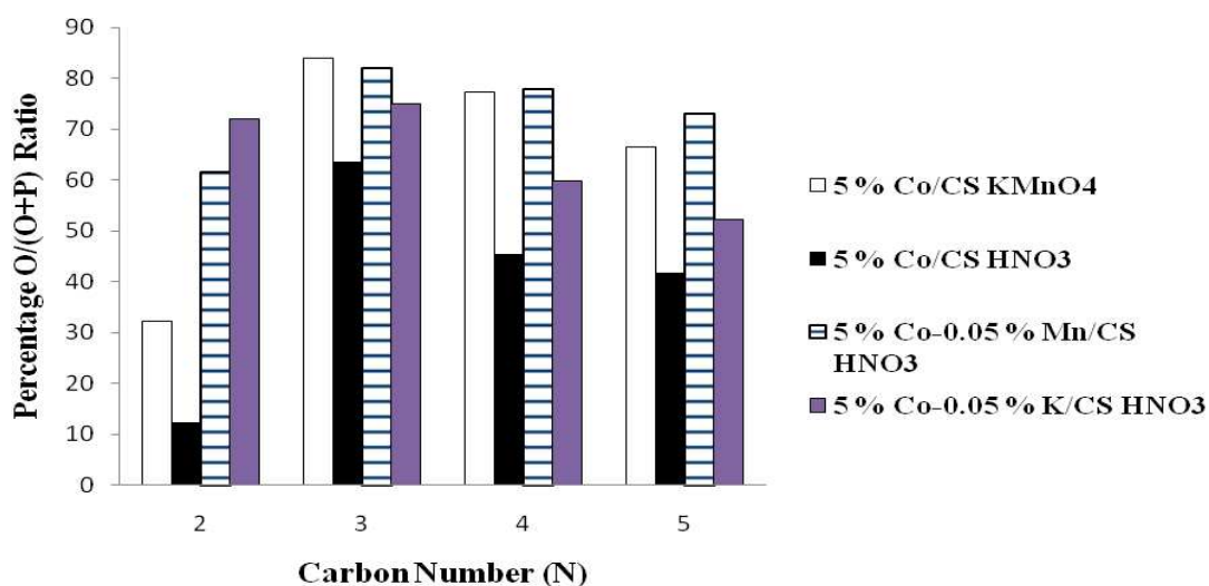
Figure 5.13: Olefin selectivity for 5% Co/CSs.
