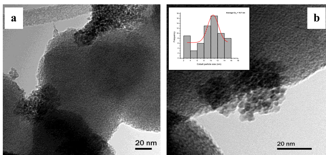
Figure 5.2 TEM images of 2.5 % Co/CS \text{KMnO}_4 functionalised catalysts
