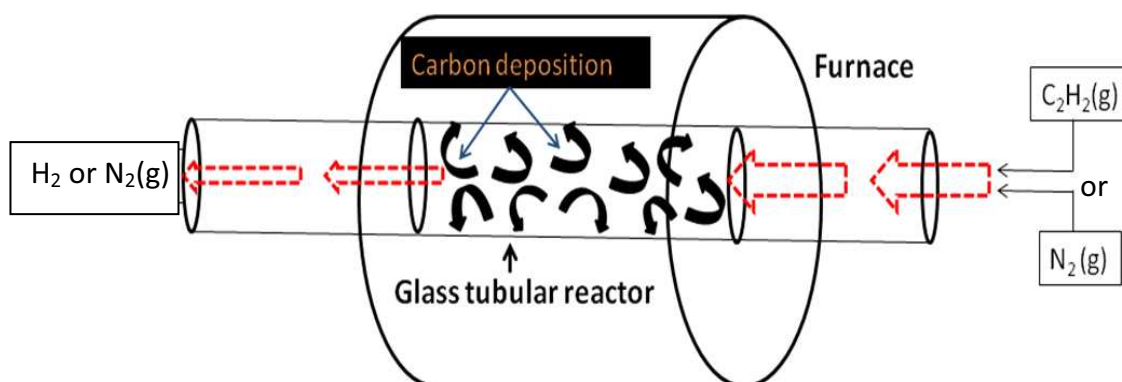
Figure 4.1: Schematic diagram of the chemical vapour deposition equipment and reaction.
