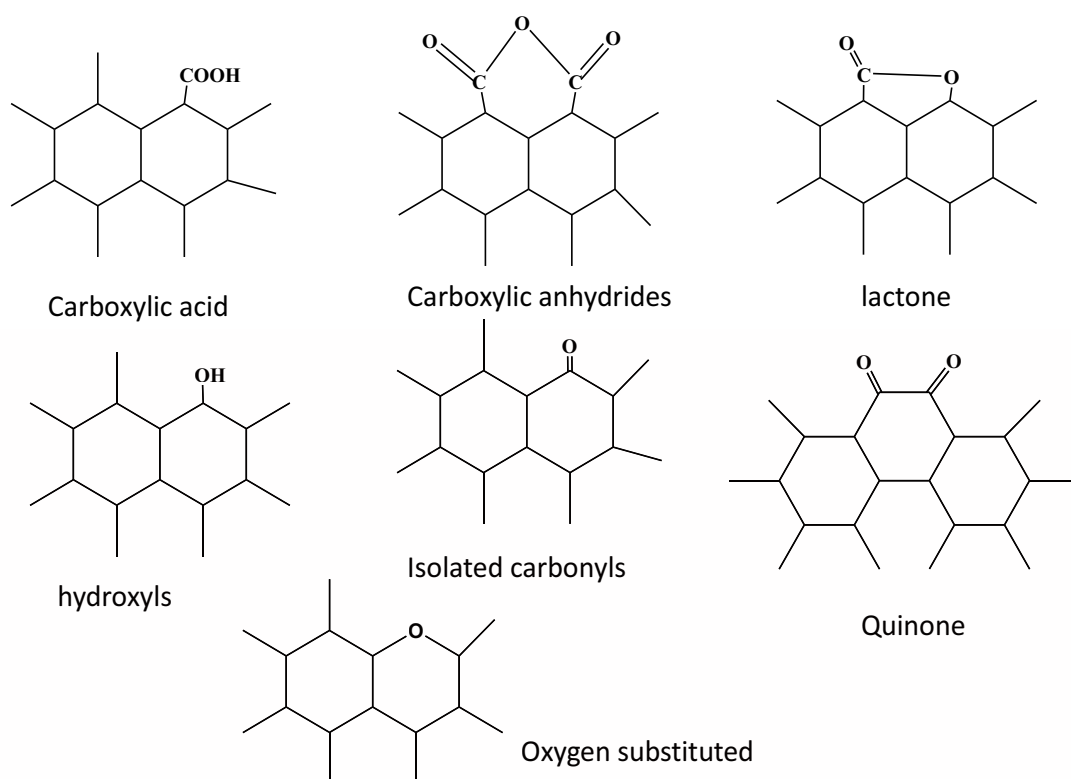
Figure 4.8: Possible surface functional groups found on CSs [6]
