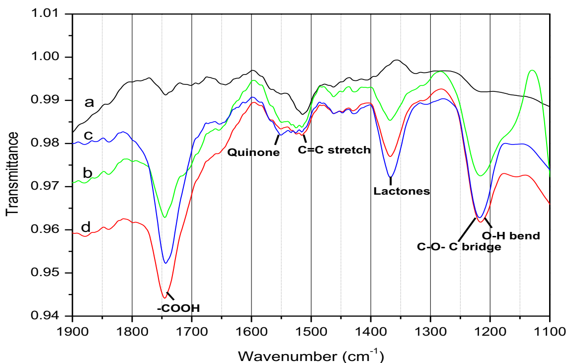
Figure 4.12: FTIR of (a) as-synthesised, CSs and 55 % \text{HNO}_3 functionalised CSs for (b) 96 h at room temperature (c) 24 h at 40 °C and (d) 2 h under reflux.
