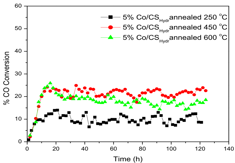
Figure C7: % CO conversion of 5% Co/CS hydr catalysts.
