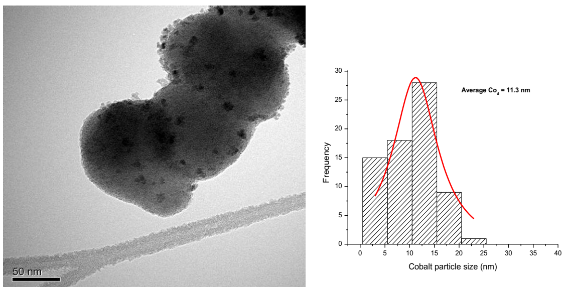
Figure 5.14: TEM images and particle size distribution of \text{KMnO}_4 functionalised catalyst after 120 h on stream.
