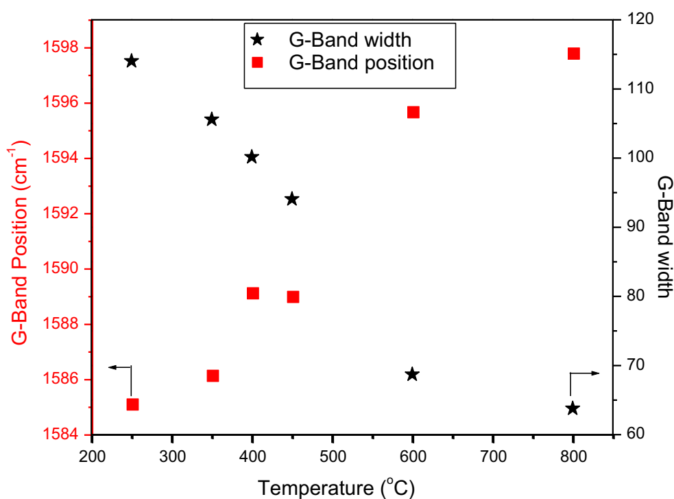
Figure 6.7: Effect of annealing temperature on G-bands
