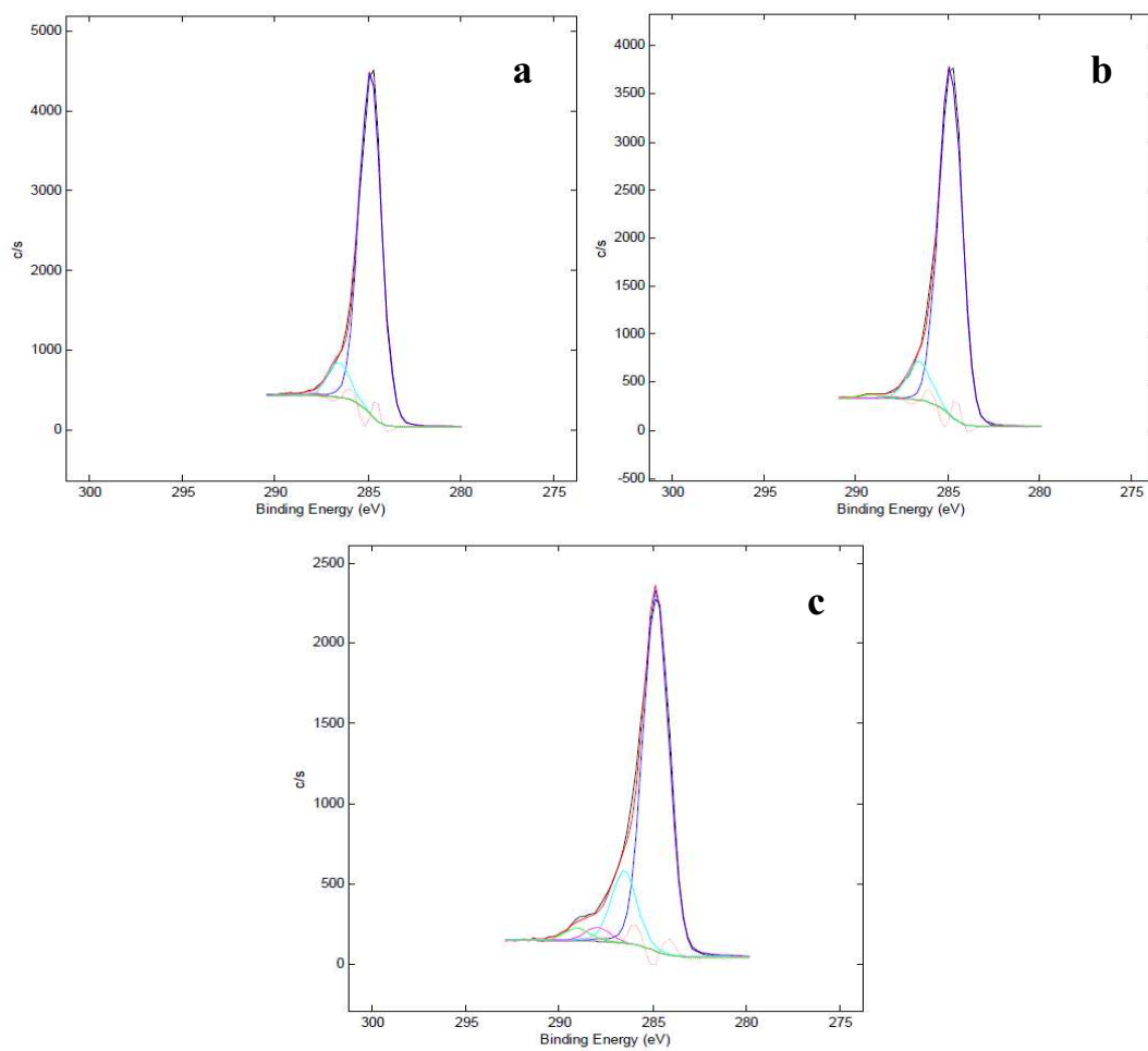
Figure 7.3: C1s spectrum of (a) NCS ver , (b) NCS hor and (c) NCS hydr
