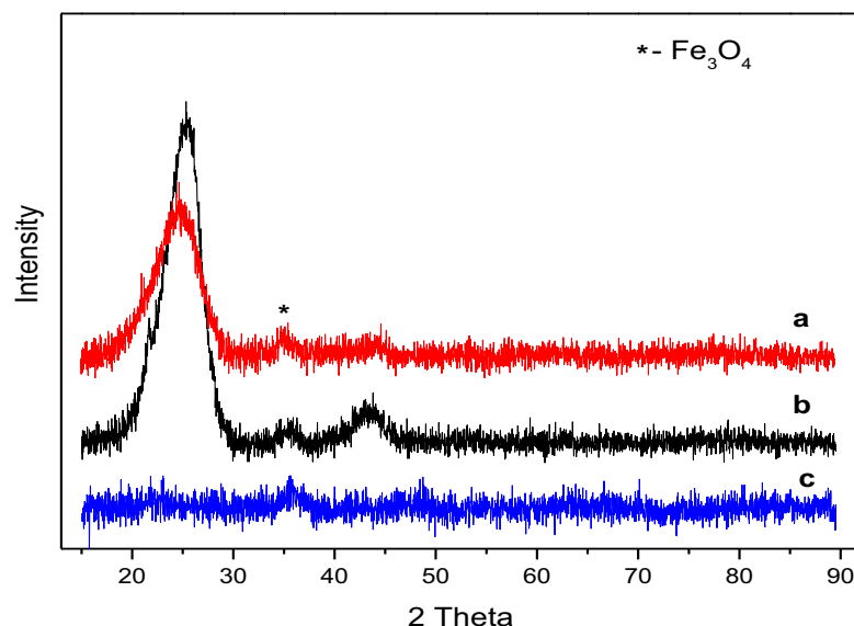
Figure 7.10: XRD patterns of (a) 5 % Fe/NCS ver (b) 5 % Fe/NCS hor (c) 5 % Fe/NCS hydr
