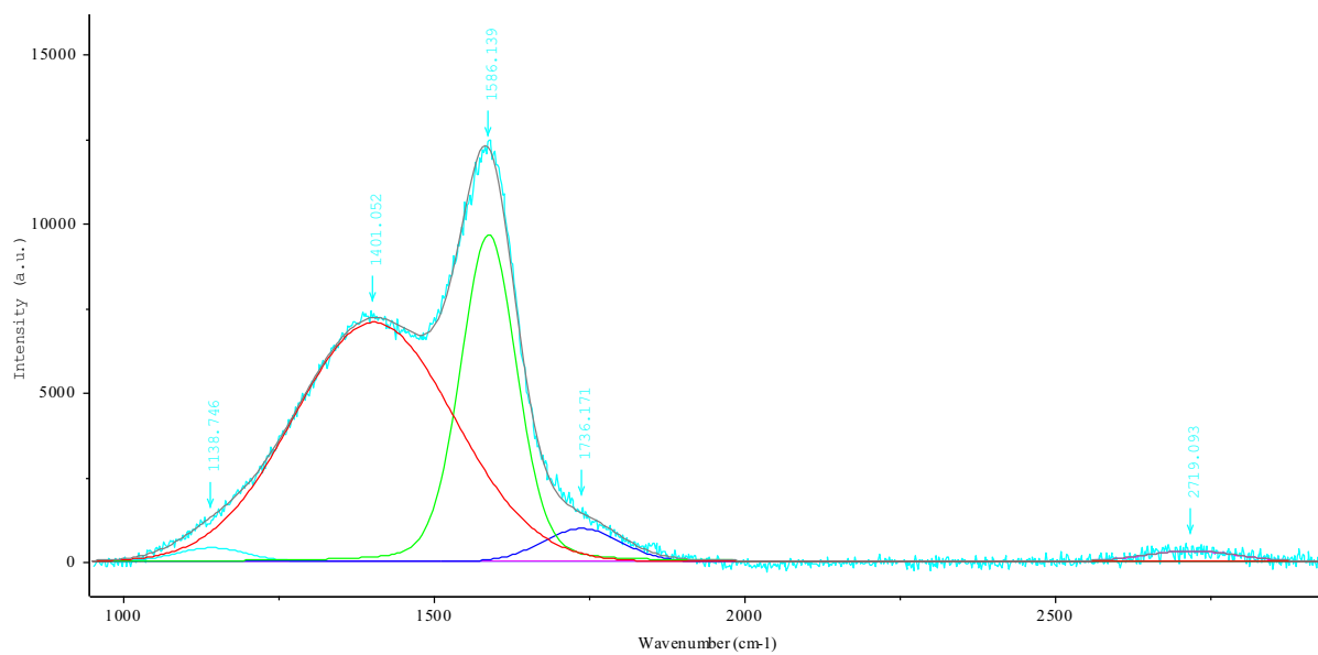
Figure C2: Raman spectra of CS hydr annealed at 350 °C under N 2 for 2.5 h.
