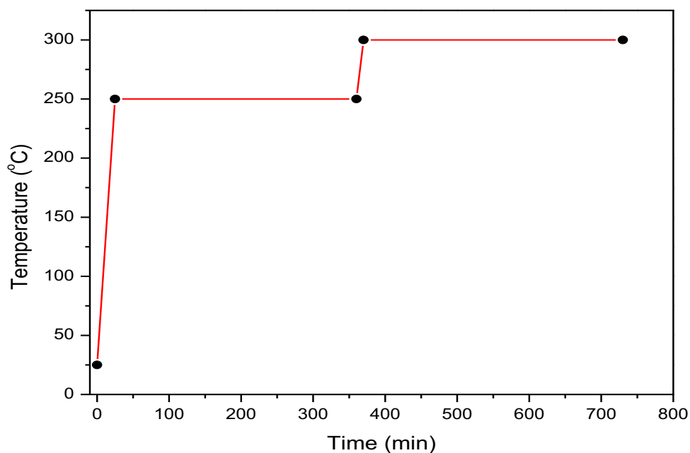
Figure B5: Temperature programme for the oxidation of \text{Co}^0 phases in 5 % Co/CS \text{HNO}_3 catalyst in air.
