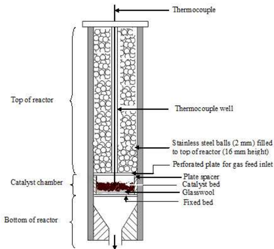
Figure 3.12: Schematic diagram of fixed bed reactor
