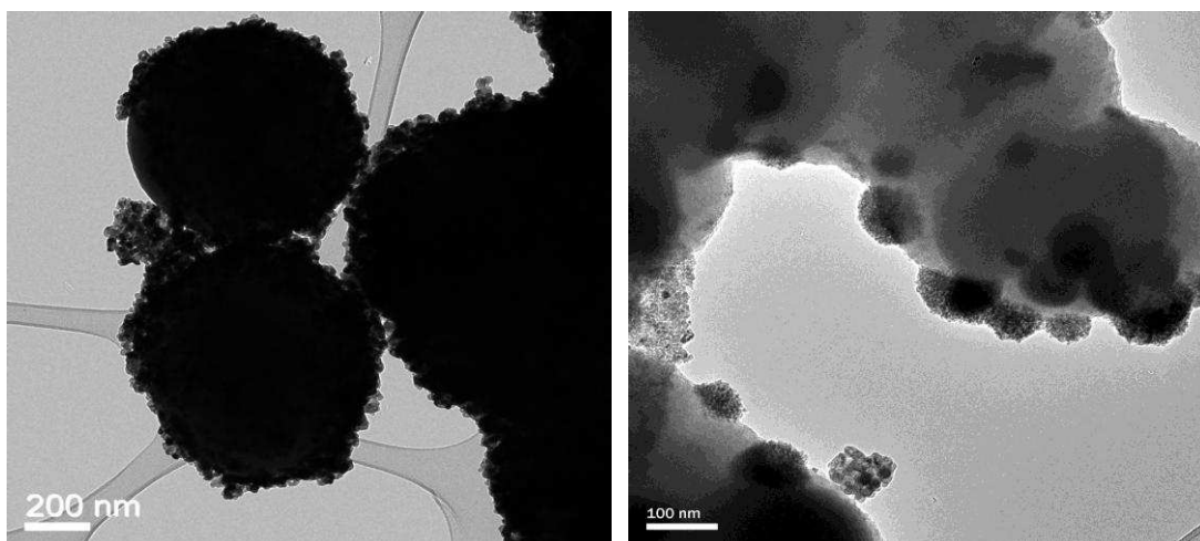
Figure 5.10: TEM images of (a) 10% Co/CS \text{KMnO}_4 functionalised catalyst (b) 10% Co/CS \text{HNO}_3 functionalised catalyst.
