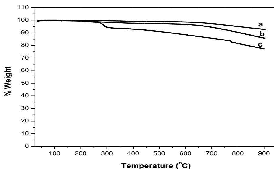
Figure 4.16: TGA profiles run in nitrogen gas: Effect of functionalising conditions of (a) 0.5 M \text{KMnO}_4 / 40 °C/ 4 h (b) 1 M \text{KMnO}_4 / 70 °C/ 4 h (c) 2 M \text{KMnO}_4 / 70 °C/ 4 h.
