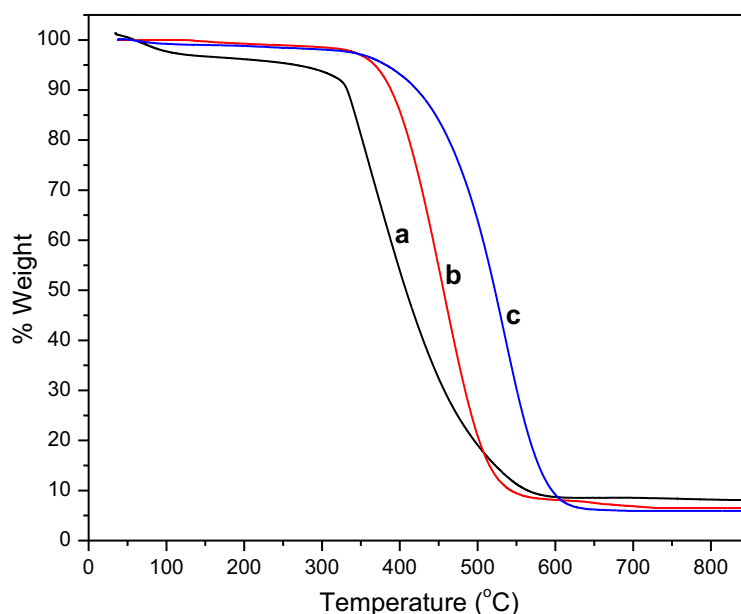
Figure 6.13: TGA profiles of (a) Co250CS hydr , (b) Co450CS hydr and (c) Co600CS hydr catalysts
