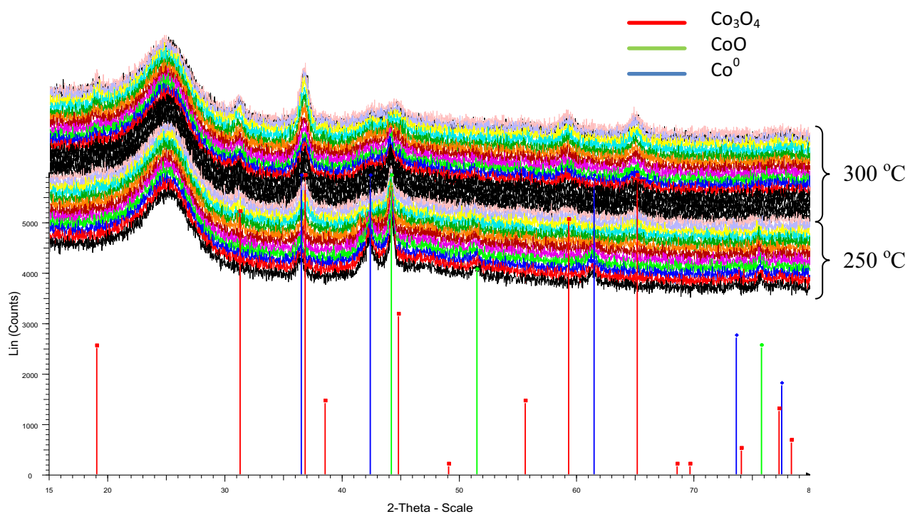
Figure B4: In-situ XRD patterns of oxidation of \text{Co}^0 phases in 5 % Co/CS \text{HNO}_3 catalyst in air.
