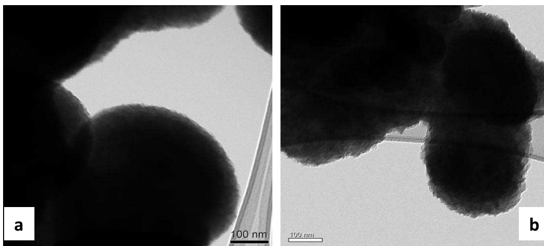
Figure 4.18: TEM image of CSs functionalised by (a) 0.5 M \text{KMnO}_4 / 40 °C/ 4 h (b) 2 M \text{KMnO}_4 / 70 °C/ 4 h.
