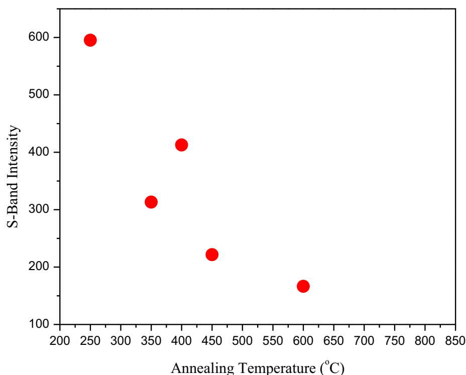
Figure 6.10: Effect of annealing temperature on S-bands
