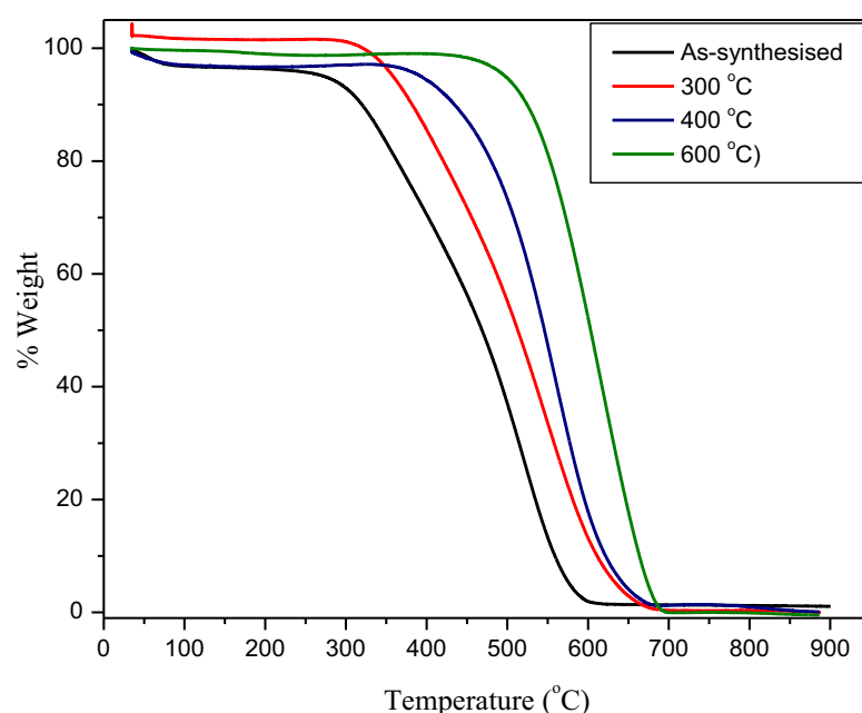
Figure 6.4: TGA profiles (under air) of as-synthesised and 300, 450 and 600 °C annealed \text{CS}_{\text{hydr}} samples (2.5 h heating).
