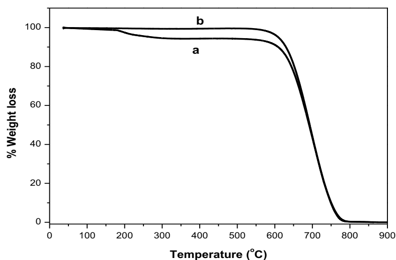
Figure 7.7: TGA profiles of NCS ver (a) before and (b) after annealing at 250 °C for 2 ½ h in N 2 gas.
