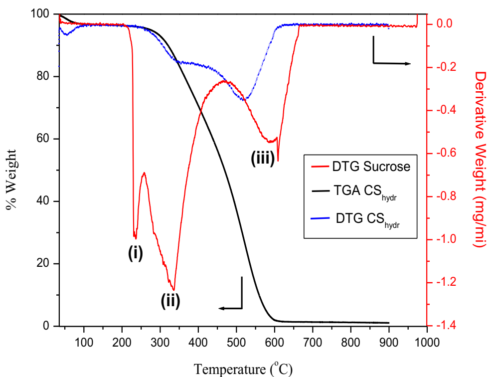
Figure 6.2: TGA and DTG profiles of as-synthesised \text{CS}_{\text{hydr}} and sucrose under air.
