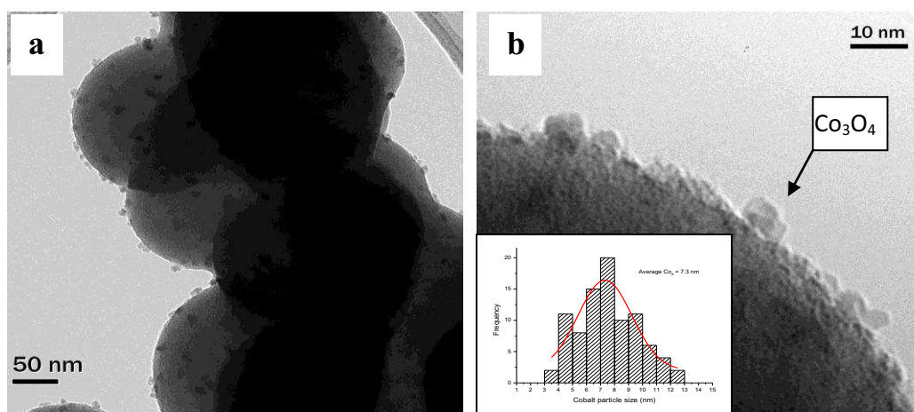
Figure 5.1 TEM images of 2.5 % Co/CS \text{KMnO}_4 functionalised catalysts
