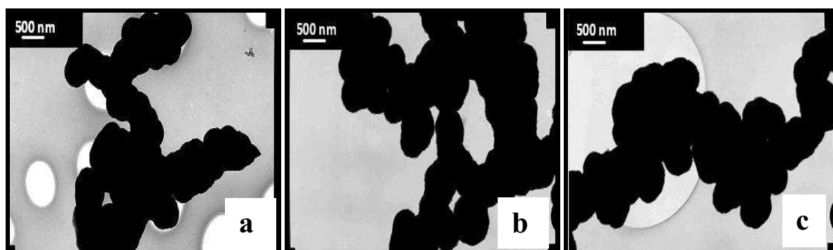
Figure 4.17: TEM images after functionalising with (a) 0.5 M \text{KMnO}_4 / 40 °C/ 4 h (b) 1 M \text{KMnO}_4 / 70 °C/ 4 h (c) 2 M \text{KMnO}_4 / 70 °C/ 4 h.
