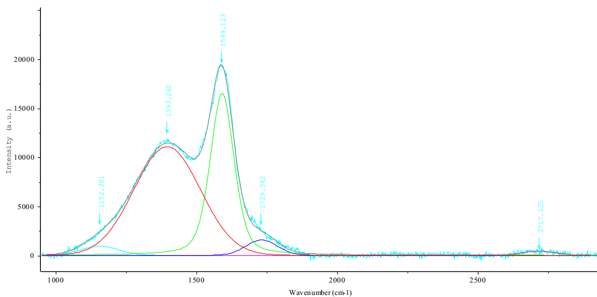
Figure C3: Raman spectra of CS hydr annealed at 400 °C under N 2 for 2.5 h.
