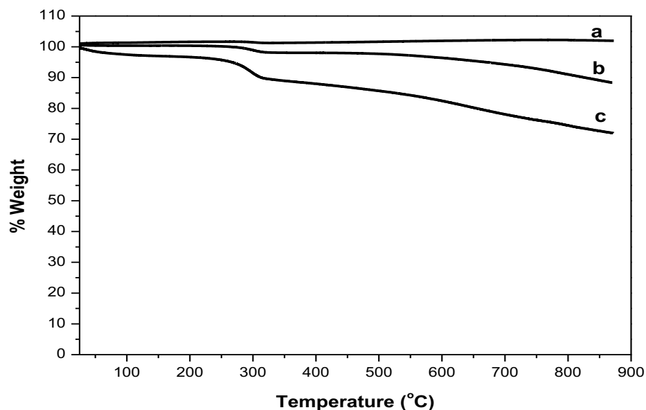
Figure 4.13: TGA profiles run in nitrogen: Effect of functionalising conditions: (a) 55 % HNO 3 / 40 °C/ 24 h (b) 55 % HNO 3 / reflux/ 2 h (c) 55 % HNO 3 / reflux/ 24 h.
