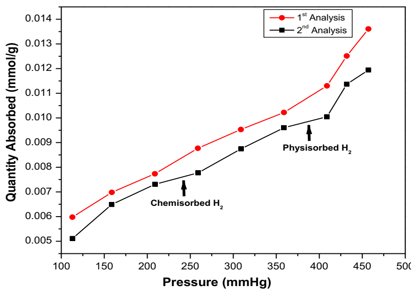
Figure B1: Adsorption isotherm of H 2 uptake during chemisorption analysis.
