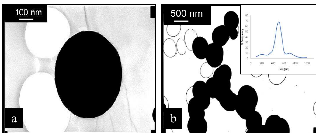
Figure 4.3: TEM images of as-synthesised CSs (a) single sphere and (b) accreted spheres (insert showing CSs diameter distribution).
