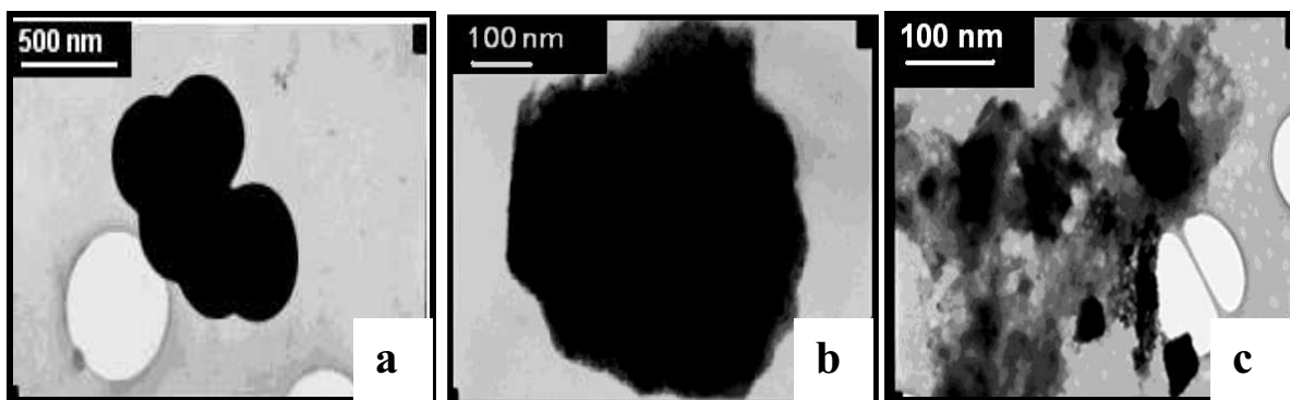
Figure 4.14: TEM images after functionalising of the CSs with (a) 55 % HNO 3 / 40 °C/ 24 h (b) 55 % HNO 3 / reflux/ 2 h (c) 55 % HNO 3 / reflux/ 24 h.
