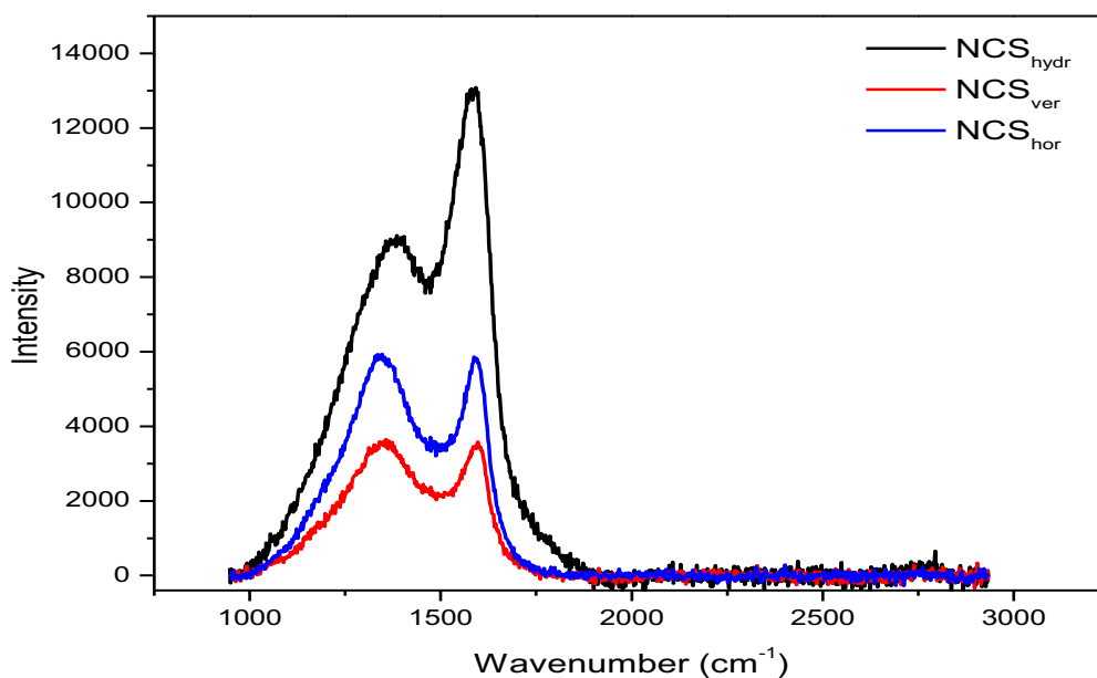
Figure 7.2: Raman spectra of NCSs.
