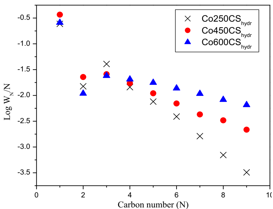
Figure 6.14: ASF plot of Co/CS hydr catalysts
