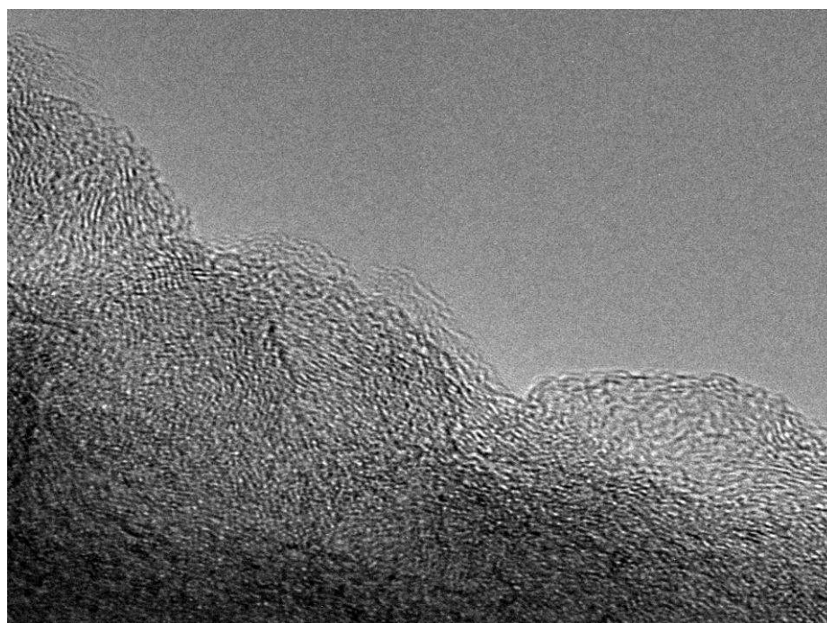
Figure 4.19: HRTEM image of CSs functionalised by 0.5 M \text{KMnO}_4 / 40 °C/ 4 h
