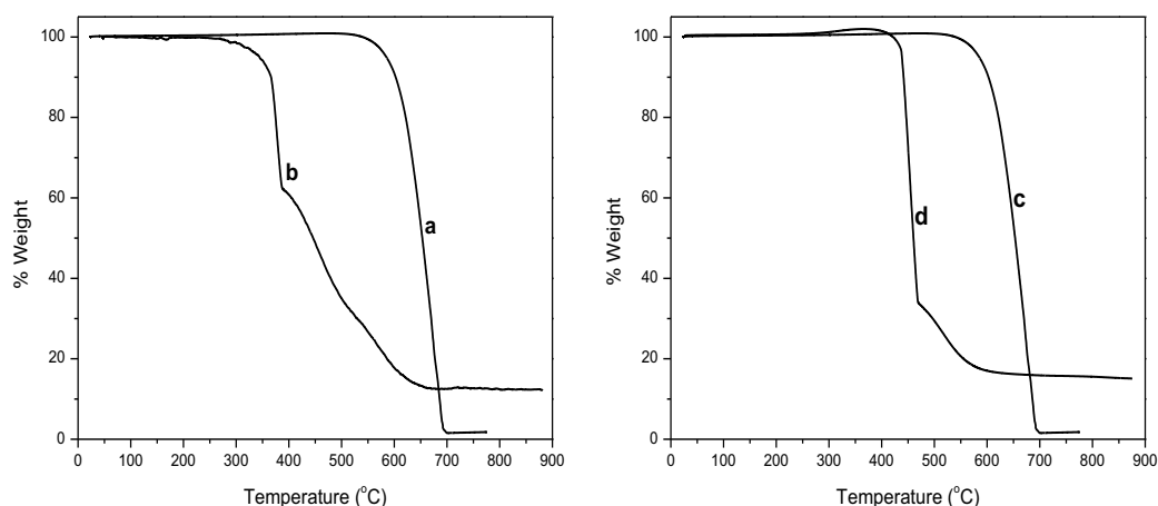
Figure 5.11: TGA profile run in air on the (a) \text{HNO}_3 functionalised CSs, (b) 10 % Co/CS catalysts functionalised by \text{HNO}_3 , (c) \text{KMnO}_4 functionalised CSs and (d) 10 % Co/CS catalysts functionalised by \text{KMnO}_4 .
