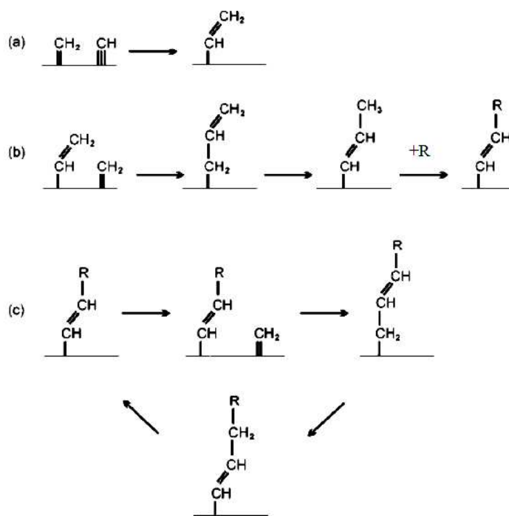
Figure 2.5: Schematic diagram of vinyl/alkenyl mechanism (a) chain initiation, (b) chain growth and methylene insertion, (c) chain propagation. [28]
