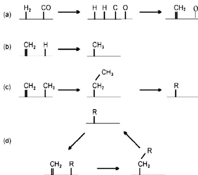
Figure 2.2: Schematic diagram of the alkyl mechanism showing (a) methylene formation, (b) chain initiation, (c) initial chain growth and (d) chain propagation [28].
