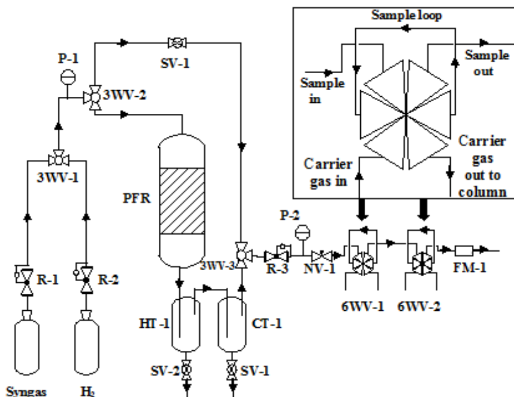
Figure 3.11: Flow sheet diagram of FT rig set up (insert: 6 way valve connecting to GC-FID and GC-TCD.)
