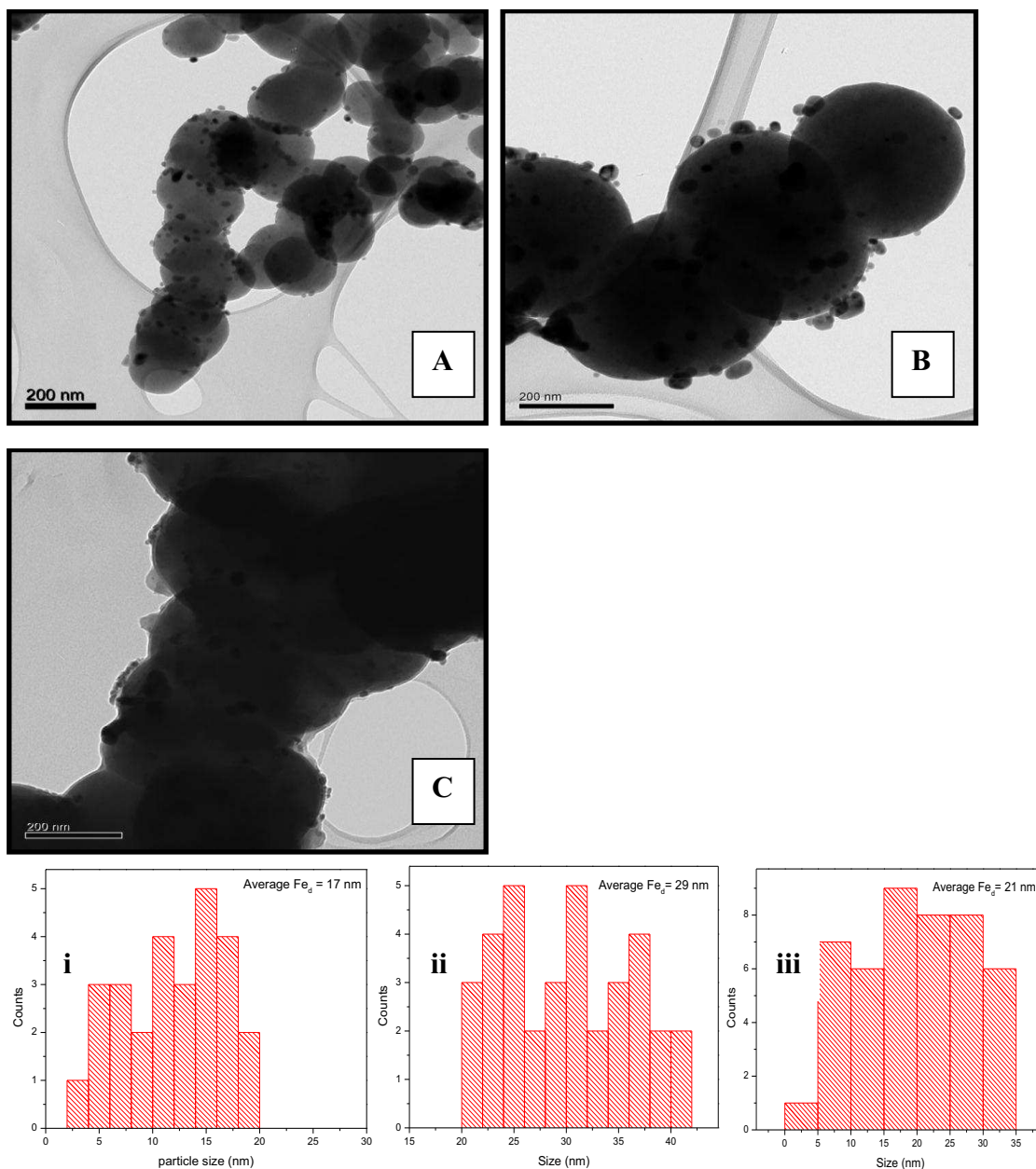
Figure 7.11: TEM images of (a) 5 % Fe/NCS ver (b) 5 % Fe/NCS hor (c) 5 % Fe/NCS hydr and size distribution of (i) 5 % Fe/NCS ver (ii) 5 % Fe/NCS hor (iii) 5 % Fe/NCS hydr after 120 h of FTS.
