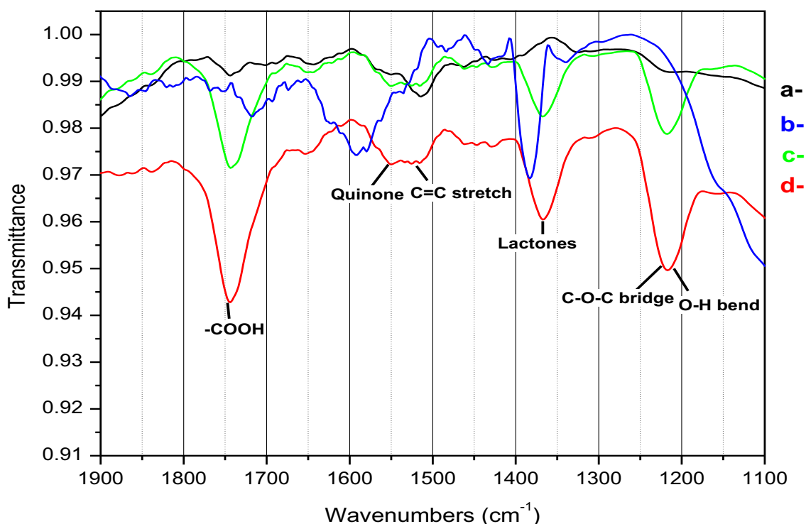
Figure 4.15: FTIR of (a) as-synthesised CSs (b) 0.5 M KMnO 4 / 4 h/ 25 °C (c) 1 M KMnO 4 / 4 h/ 40 °C and (d) 2 M KMnO 4 / 4 h/ 70 °C.
