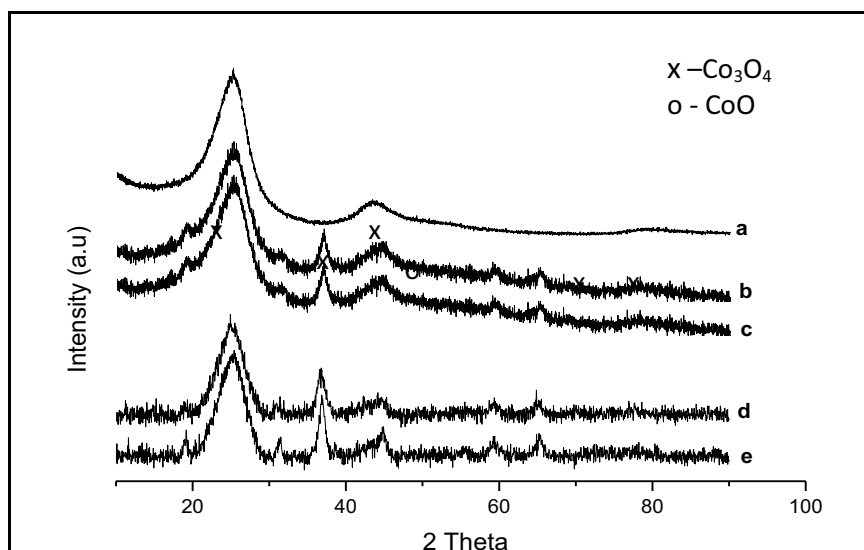
Figure 5.7: XRD patterns for (a) As-synthesised CSs, (b) 5% Co/CS HNO 3 functionalised CS, (c) 5% Co/CS KMnO 4 functionalised CS (d) 5% Co/0.05% K/CS HNO 3 functionalised CS, and (e) 5% Co/0.05% Mn HNO 3 functionalised CS.
