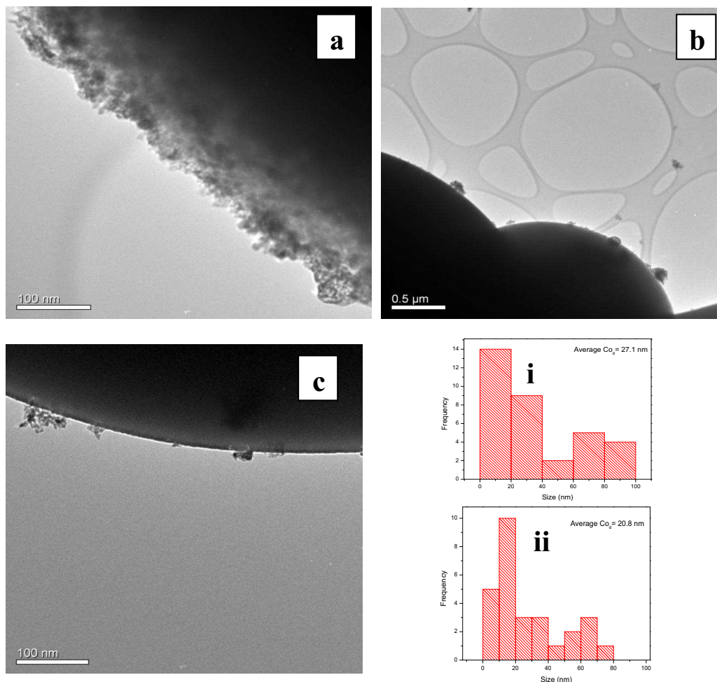
Figure 6.12: TEM images of (a) Co250CS hydr , (b) Co450CS hydr and (c) Co600CS hydr and Co particle size distribution of (i) Co450CS hydr and (ii) Co600CS hydr catalysts.
