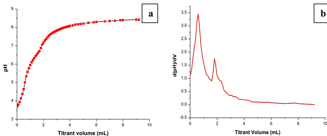
Figure 4.9: (a) Typical potentiometric titration curve of functionalised CSs and (b) the derivative graph.
