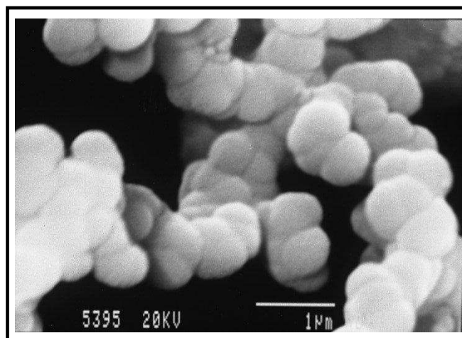
Figure 4.5: Shows SEM image of as-synthesised CSs.
