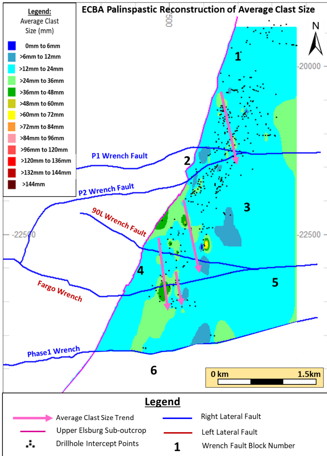
Figure 50: Palinspastic average clast size reconstruction for ECBA.
