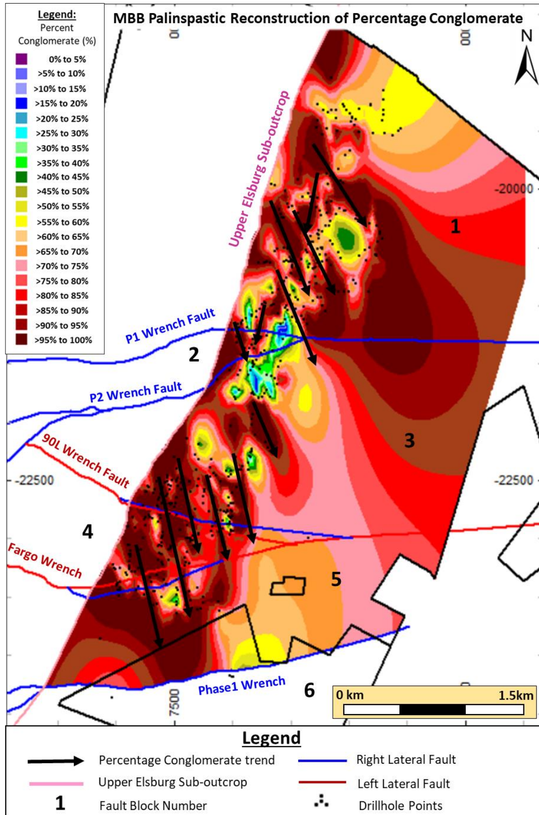
Figure 178: Palinspastic percentage conglomerate reconstruction for MBB.
