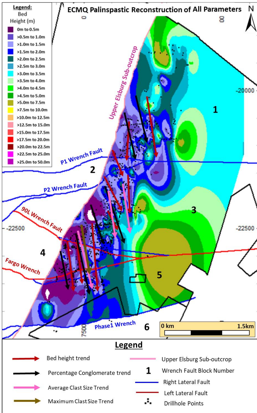
Figure 125: Palinspastic Reconstruction for the ECMQ - All Parameters
