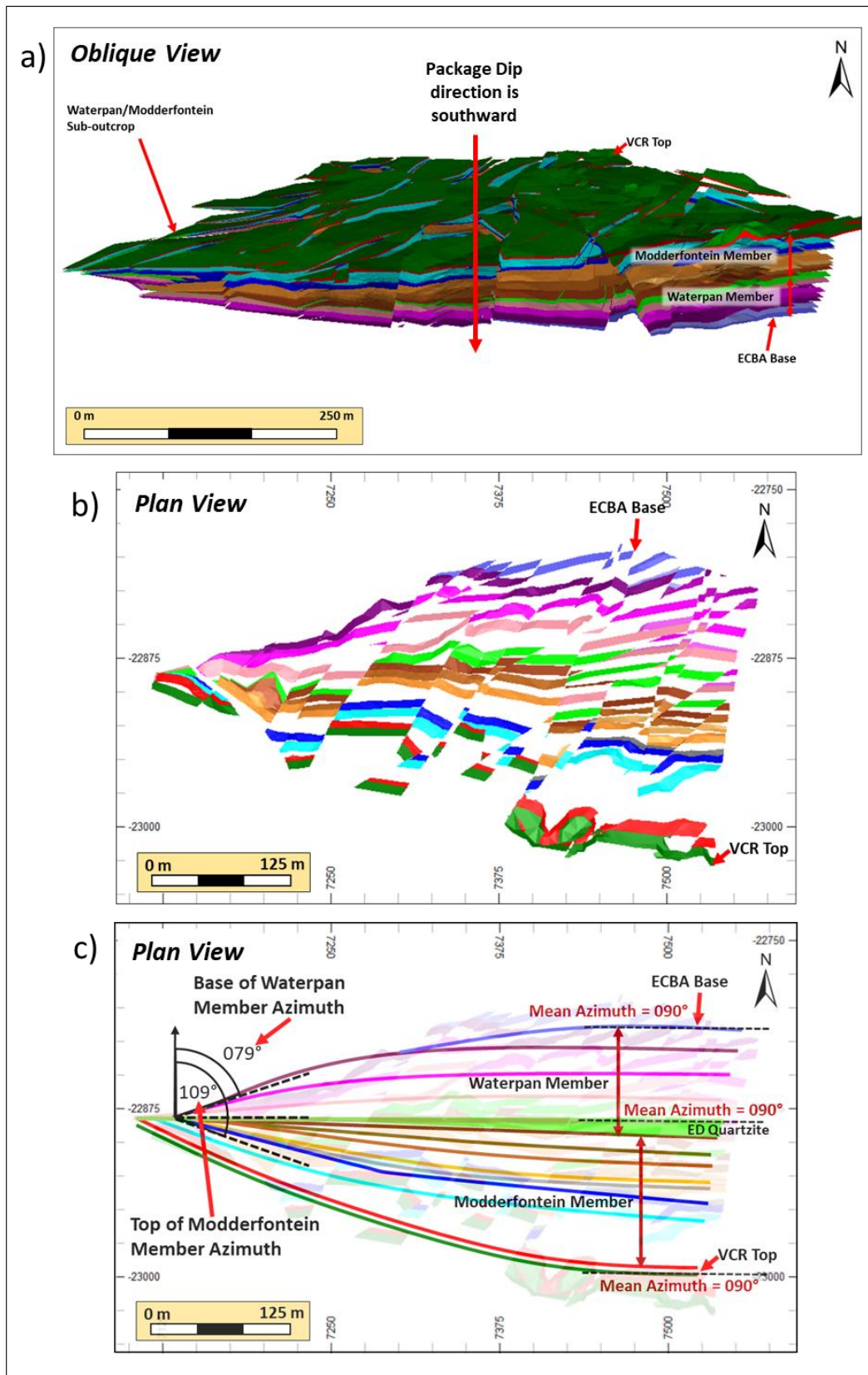
Figure 36: a) Oblique view of a section of the 3D model of the Waterpan (UE7) and Modderfontein (Elsburg Massives) sedimentary wedge and the overlying VCR, dipping towards the south. B) A horizontal section view through the Waterpan/Modderfontein 3D model presenting the complicated strike relationships. C) An interpreted bedding strike from the horizontal wedge slice depicted in b), showing the variation in strike at sub-outcrop and the near E-W strike attained towards the east.
