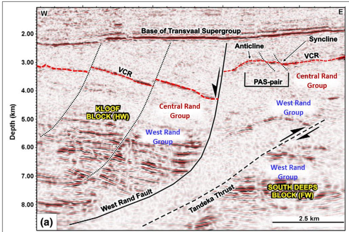
Figure 32: Interpreted seismic section across the listric West Rand Fault, showing the steeply dipping hanging wall (Kloof Block) and the blind Tandeka Thrust (modified after Manzi, 2013).
