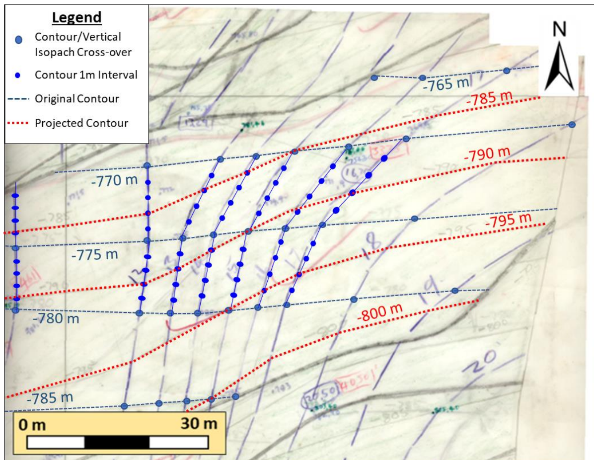
Figure 89: Projection and construction methodology of overlying or underlying beds to ensure accurate volumetrics (adapted from Obermeyer, 2004) (permission granted by Goldfields to reproduce).
