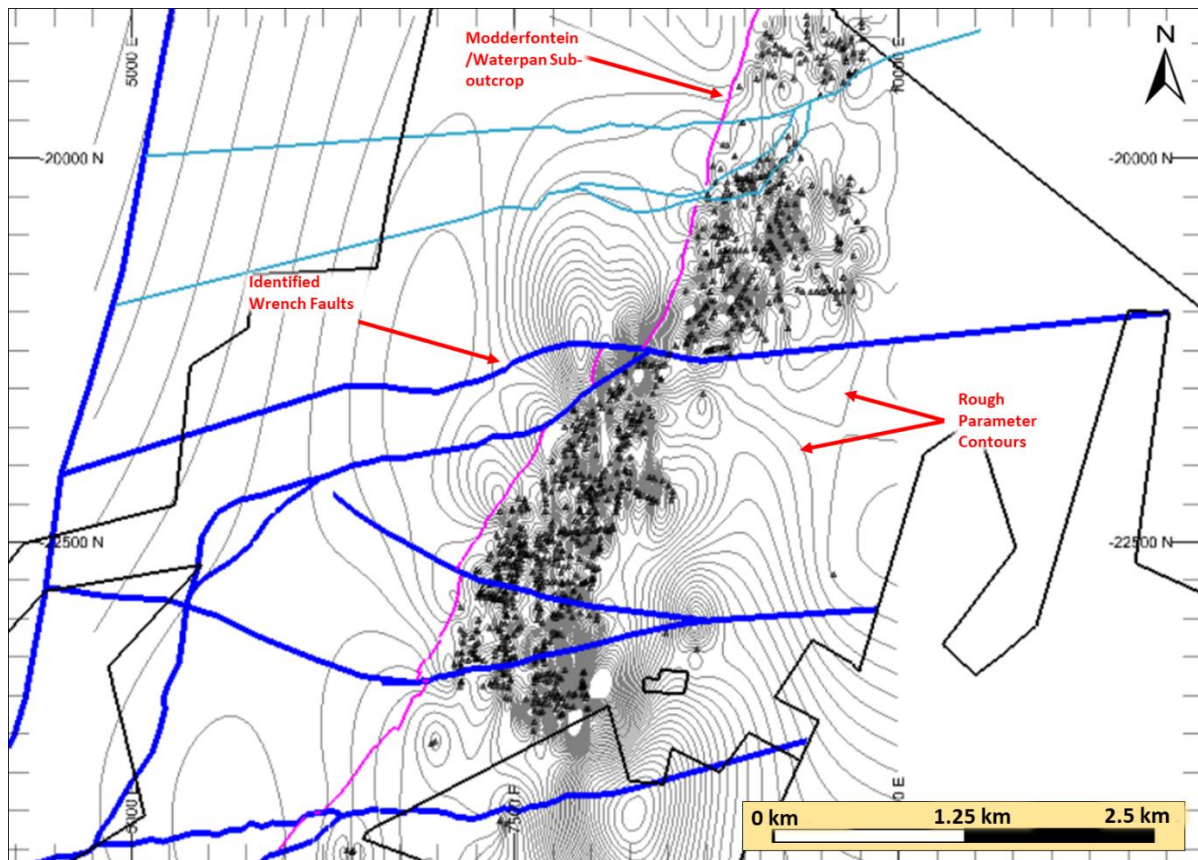
Figure 42: Rough contours for the ECB bed height in SDGM generated in Datamine Studio RM™ prior to palinspastic reconstruction.
