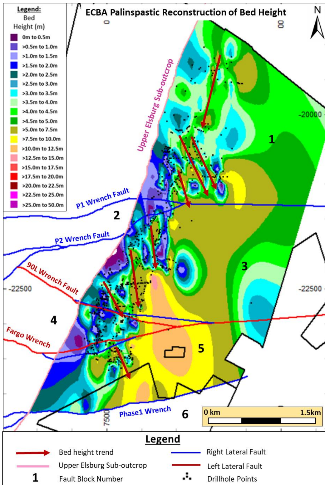
Figure 48: Palinspastic bed height reconstruction for ECBA.
