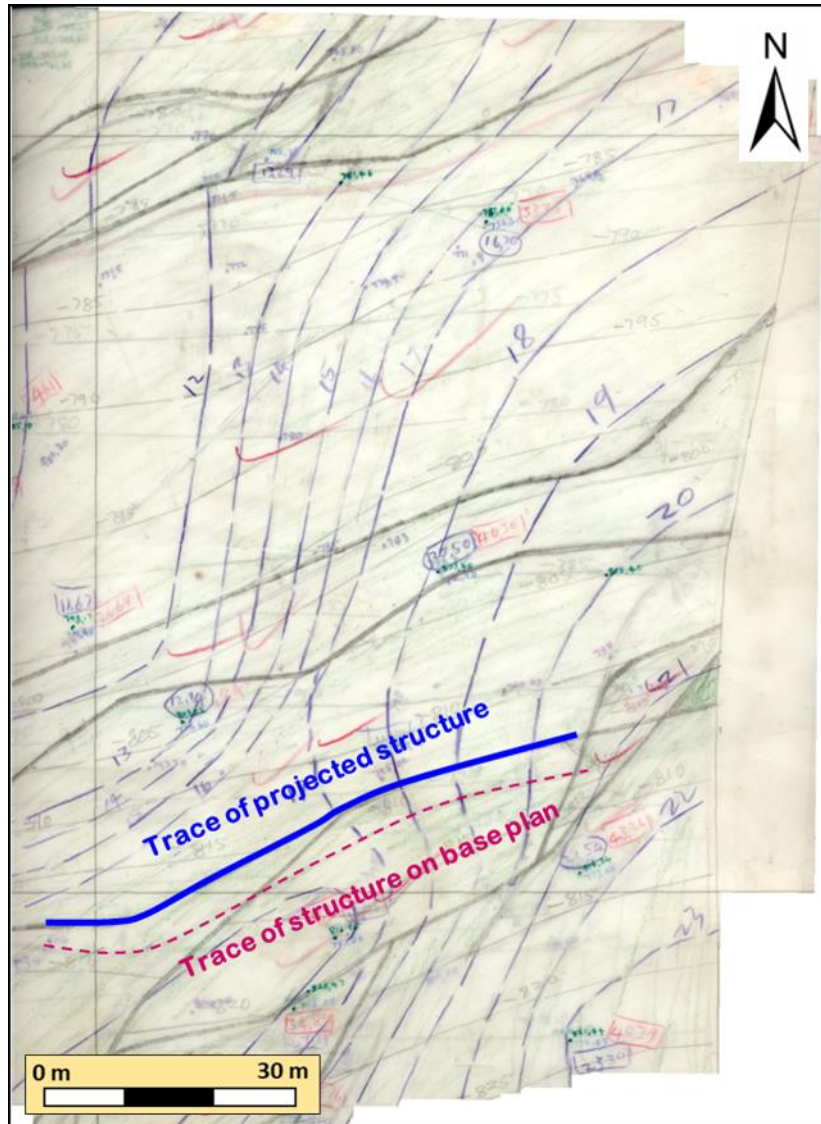
Figure 88: The vertical isopachs gave vertical projection distances between the base plan and the next projected plan. The horizontal off-sets of the faults were calculated by means of trigonometry and the resultant trace line plotted (modified after Obermeyer, 2004) (permission granted by Goldfields to reproduce).
