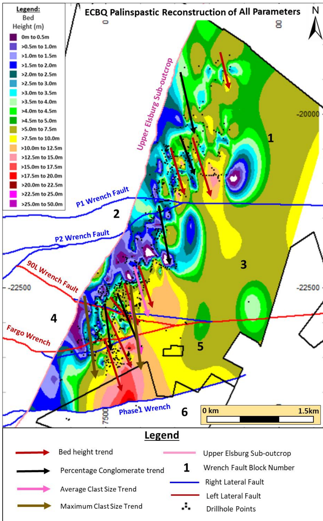
Figure 109: Palinspastic Reconstruction for the ECBQ - All Parameters
