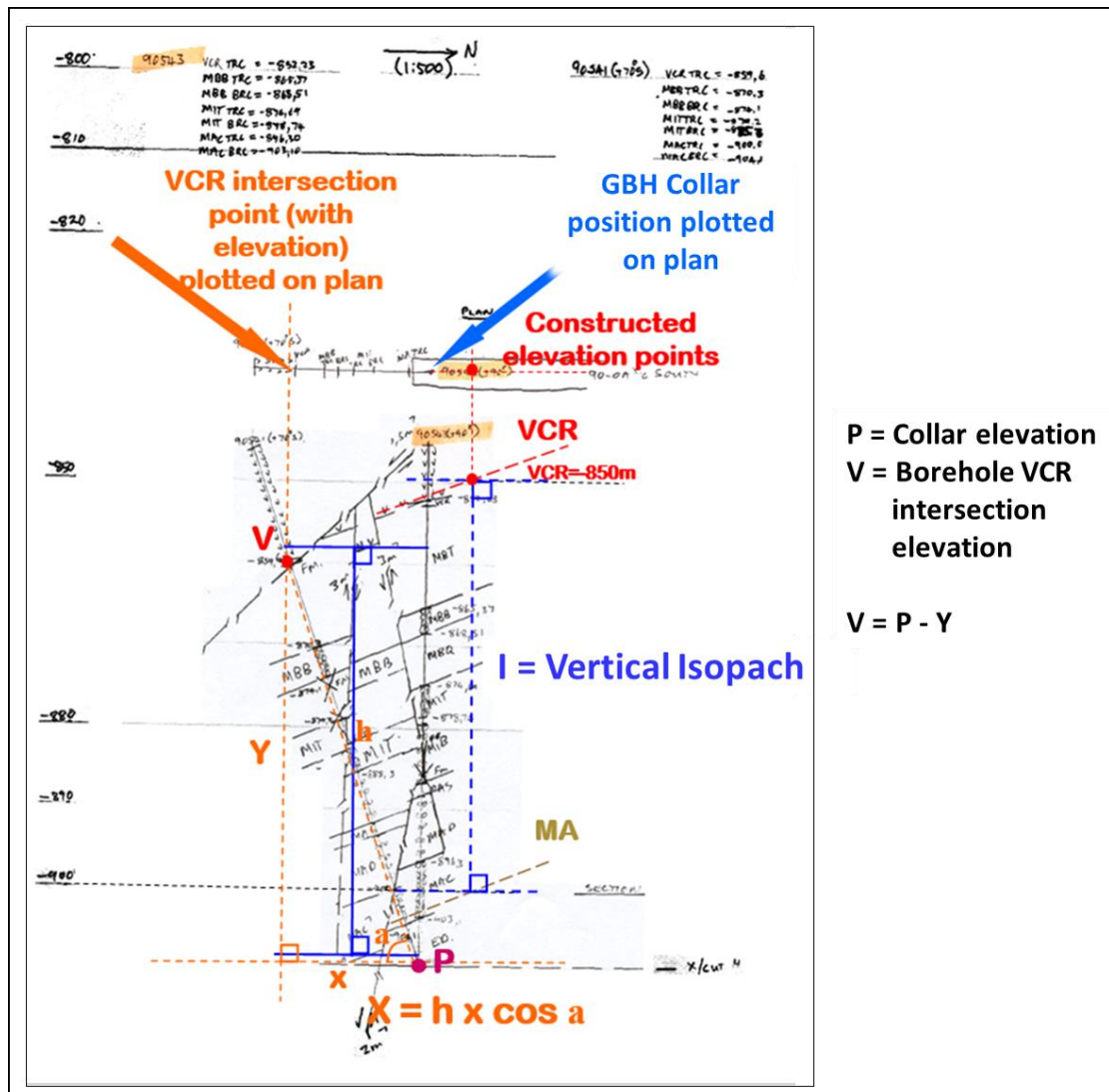
Figure 86: Vertical projection distances for structures and contours were calculated using the difference in elevations between the borehole intersections on the new plan and the base plan (modified from Obermeyer, 2004) (permission granted by Goldfields to reproduce).
