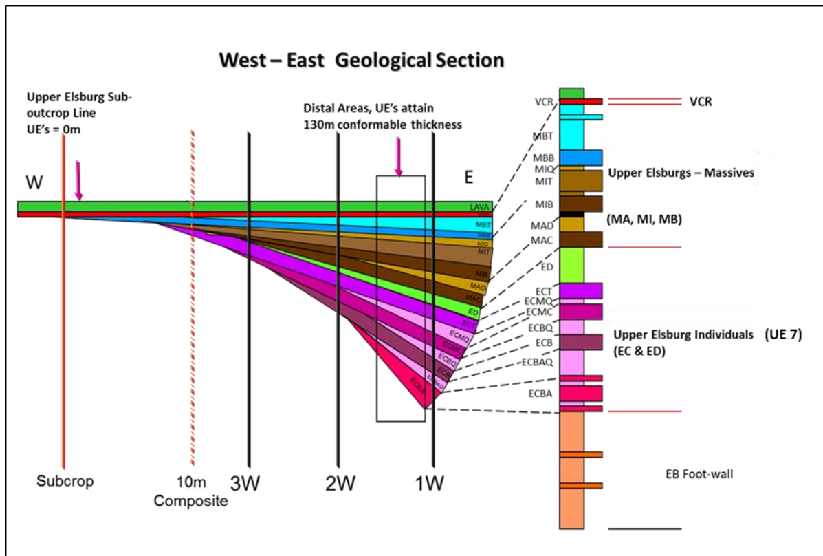
Figure 17: Schematic west to east section through the Upper Elsburgs at SDGM presenting their stratigraphic relationships and the stratigraphy as it is currently modelled (Obermeyer, 2005). The black vertical lines represent mining cross-cut positions relative to the stratigraphic make-up (permission granted by Goldfields to reproduce).
