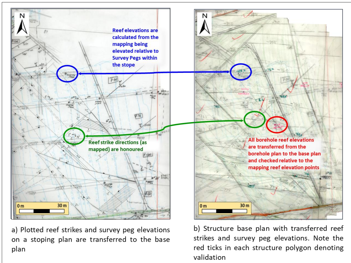
Figure 84: a) Measured and plotted reef strikes with peg elevations. b) Structure base plan with transferred reef strike and survey peg elevation data (Obermeyer, 2004b).
