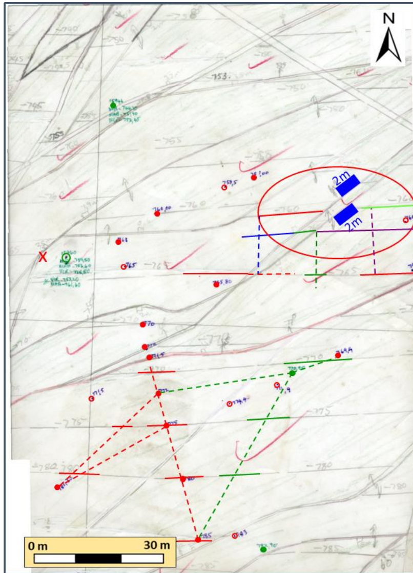
Figure 85: The strike of the reef contours was calculated as a set of simple 3-point problems, while neighbouring fault block contours were correlated by applying mapped throws to the bounding faults (Obermeyer, 2004) (permission granted by Goldfields to reproduce).
