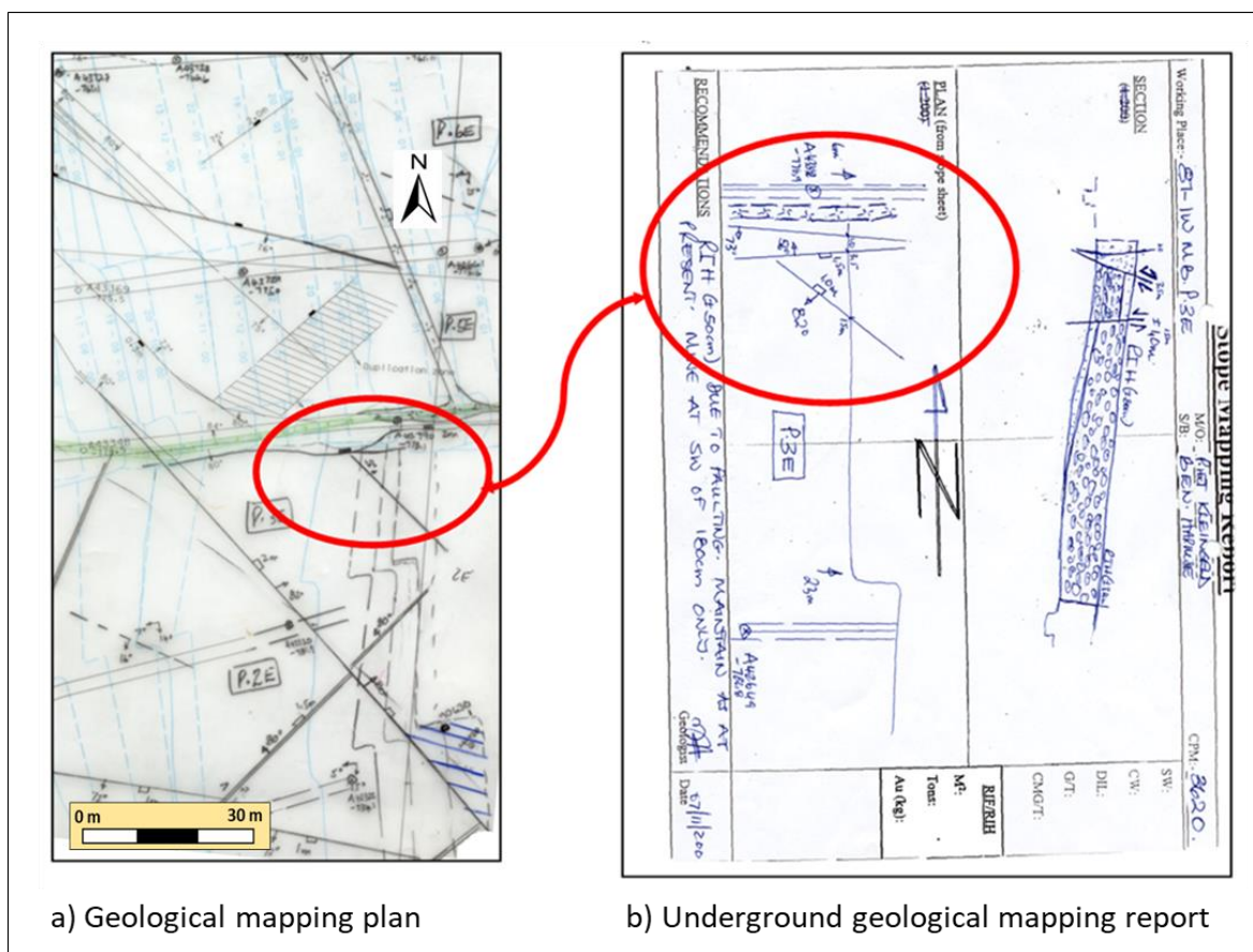
Figure 83: An example of a) a geological mapping plan and a corresponding b) underground mapping report showing some inconsistency in transfer of data (Obermeyer, 2004) (permission granted by Goldfields to reproduce).
