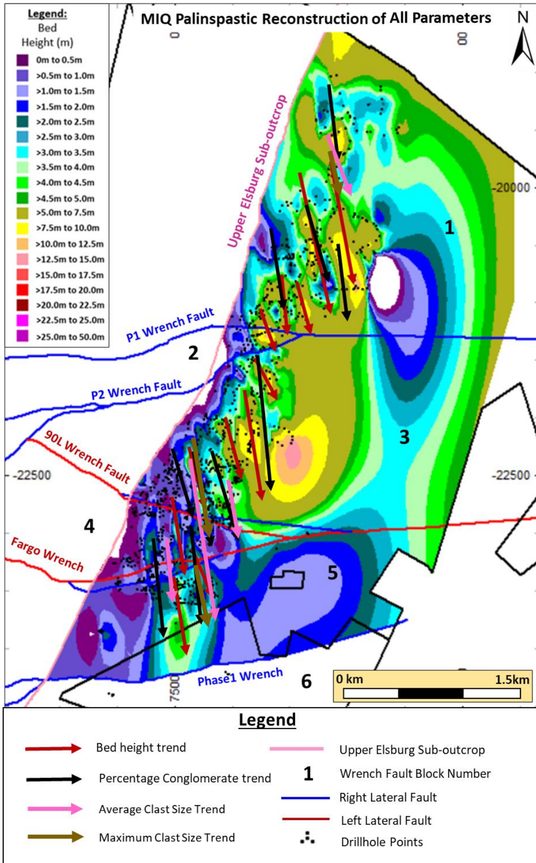
Figure 173: Palinspastic Reconstruction for the MIQ - All Parameters
