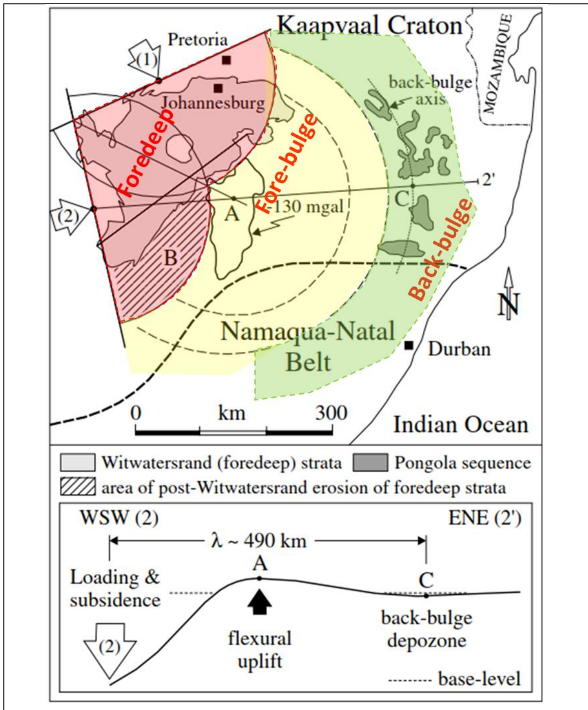
Figure 26: Partitioning of the Witwatersrand and Pongola basins into foredeep, forebulge and backbulge flexural provinces (modified after Catuneanu 2001).
