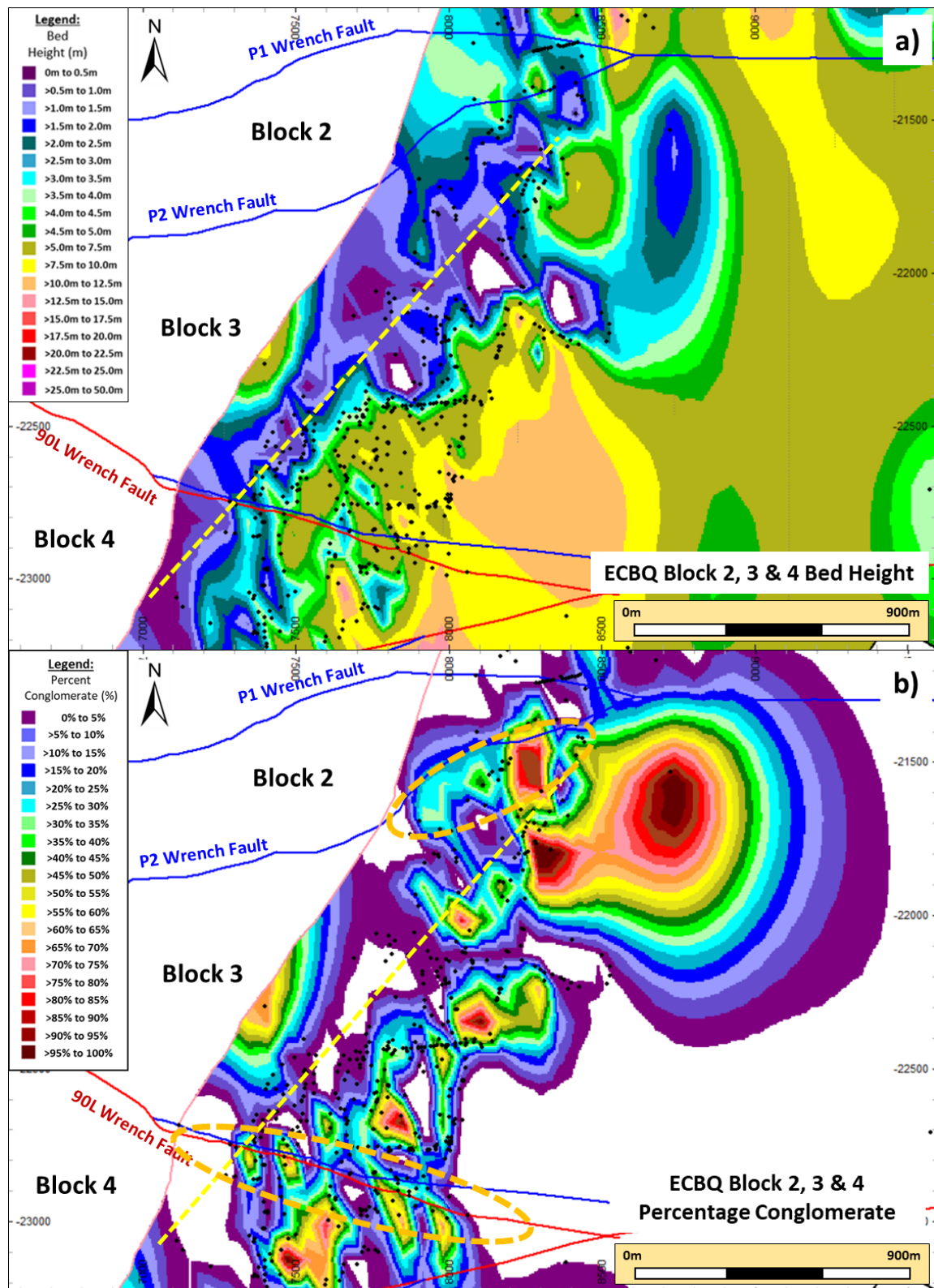
Figure 111: Enlarged Block 3 palinspastic reconstruction for a) bed height for ECBQ and b) for percentage conglomerate for ECBQ. Yellow line in a) and b) indicates a trend of lower bed height east of sub-outcrop with low percentage conglomerate. The yellow ellipse in b) indicates a trend along the strike of 90L Wrench of rapidly alternating nodes of high and low percentage conglomerate.
