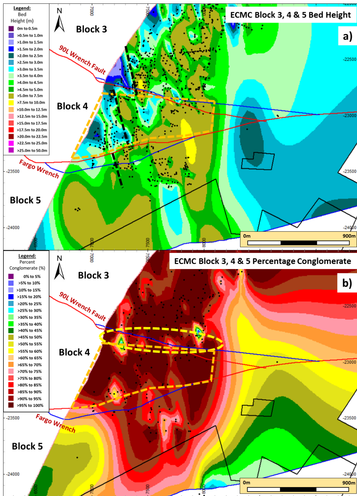
Figure 120: Enlarged Block 4 palinspastic reconstruction for a) bed height for ECMC and b) for percentage conglomerate for ECMC. Yellow polygon in a) and b) indicates zone of variable bed height and high percentage conglomerate. Yellow ellipse in b) indicates a trend along the strike of 90L Wrench of rapidly alternating nodes of high and low percentage conglomerate.
