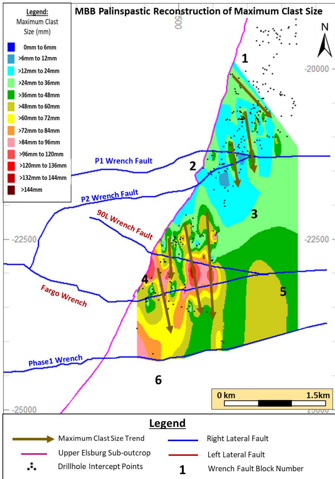
Figure 180: Palinspastic maximum clast size reconstruction for MBB.
