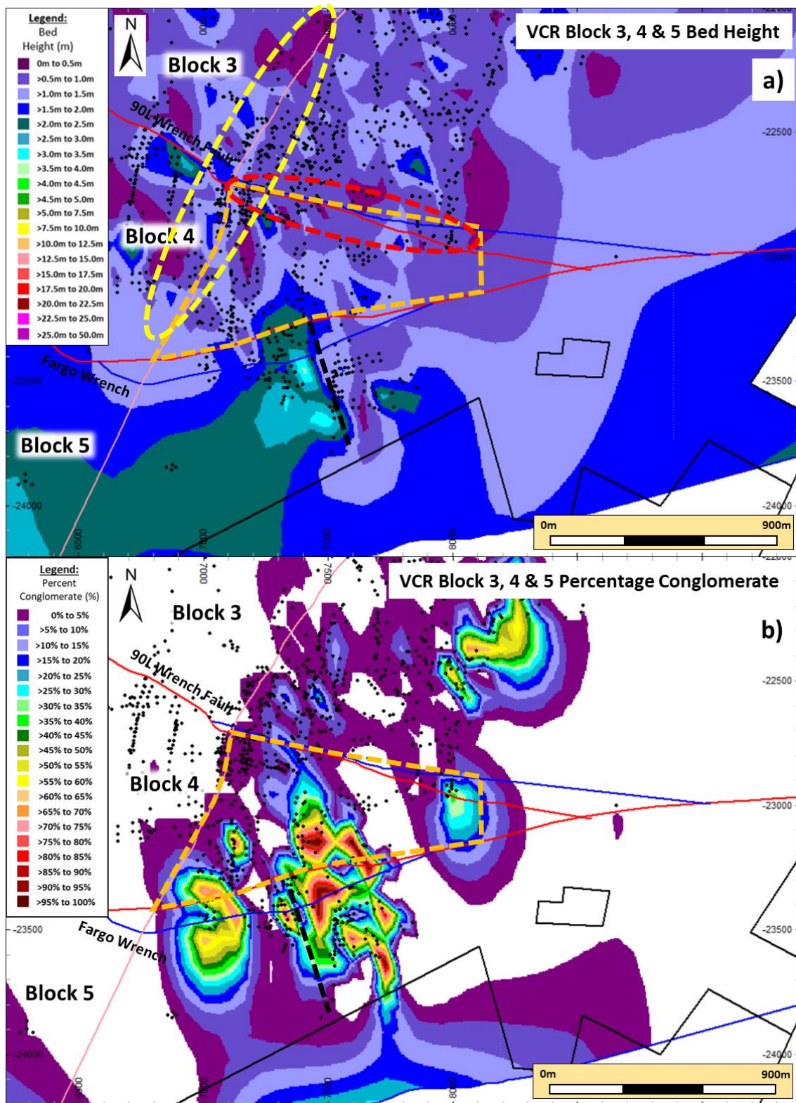
Figure 192: Enlarged Block 4 palinspastic reconstruction for a) bed height for VCR and b) for percentage conglomerate for VCR
