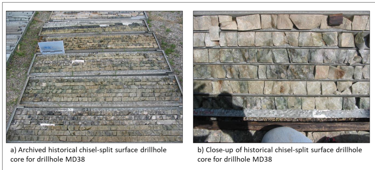
Figure 35: Historical archived split surface drillhole core from drillhole MD38 (modified after Muntingh et al., 2005) (permission granted by Goldfields to reproduce).
