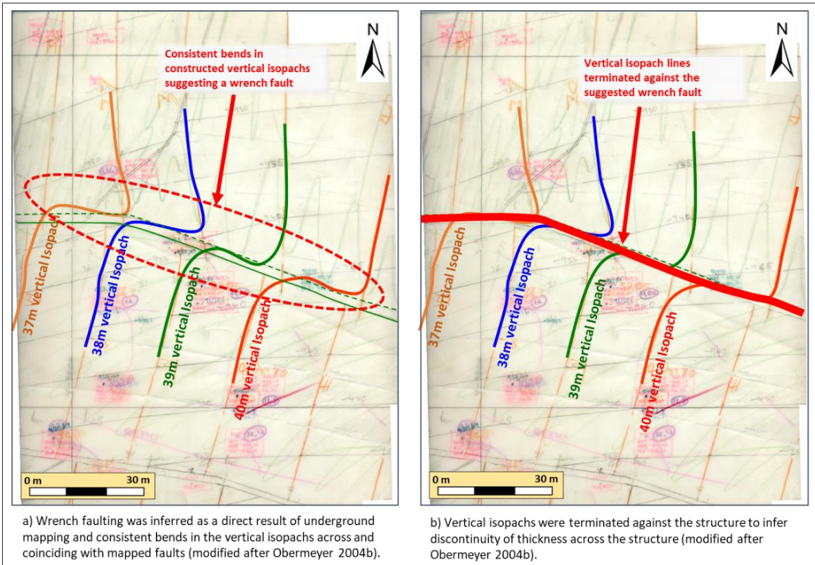
Figure 90: Identification and interpretation of wrench faults at SDGM (modified after Obermeyer, 2004) (permission granted by Goldfields to reproduce).
