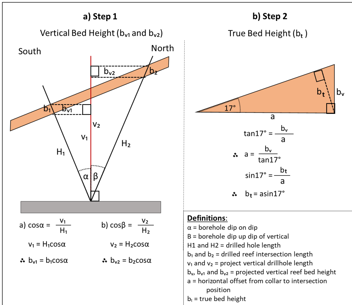
Figure 39: a) Standard trigonometric functions used to calculate vertical bed height ( b_{v1} or b_{v2} ). B) Trigonometric functions used to convert vertical bed height to true bed height ( b_t ) at a dip of 17^\circ .
