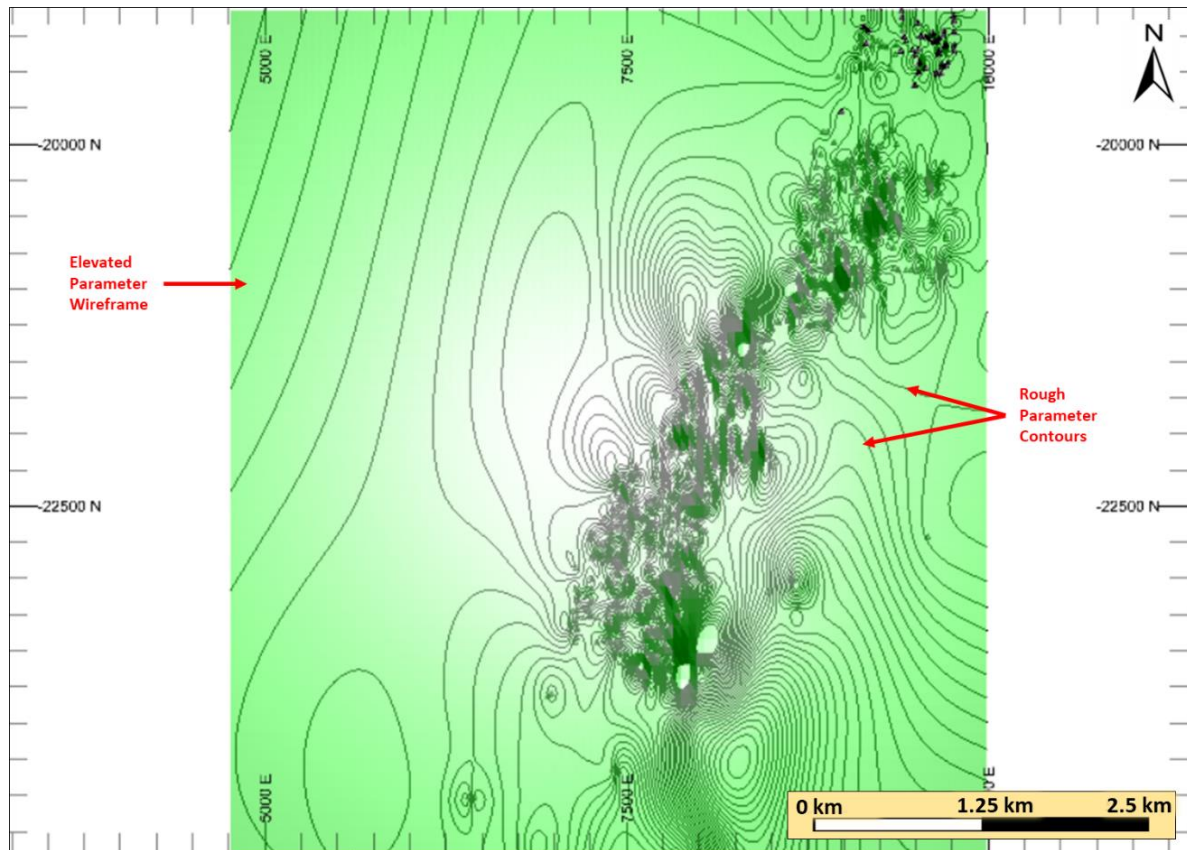
Figure 43: Rough contours for the ECB bed height with the automatically generated wireframe.
