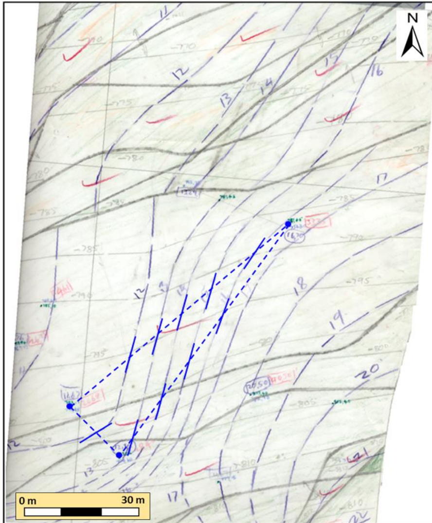
Figure 87: The vertical projection distances, calculated from the boreholes were transferred to the new plan, from the borehole plan as points. These points were triangulated and isolines, or vertical isopachs, were constructed (Obermeyer, 2004) (permission granted by Goldfields to reproduce).
