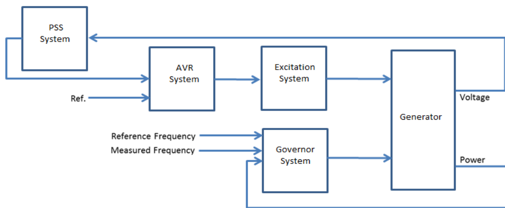
Figure 4.8 Edited plant model frame structure
