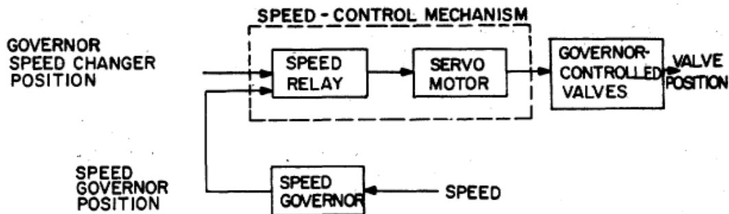
Figure 4.2 Mechanical-Hydraulic Speed governing system for steam turbine functional block diagram [13].
