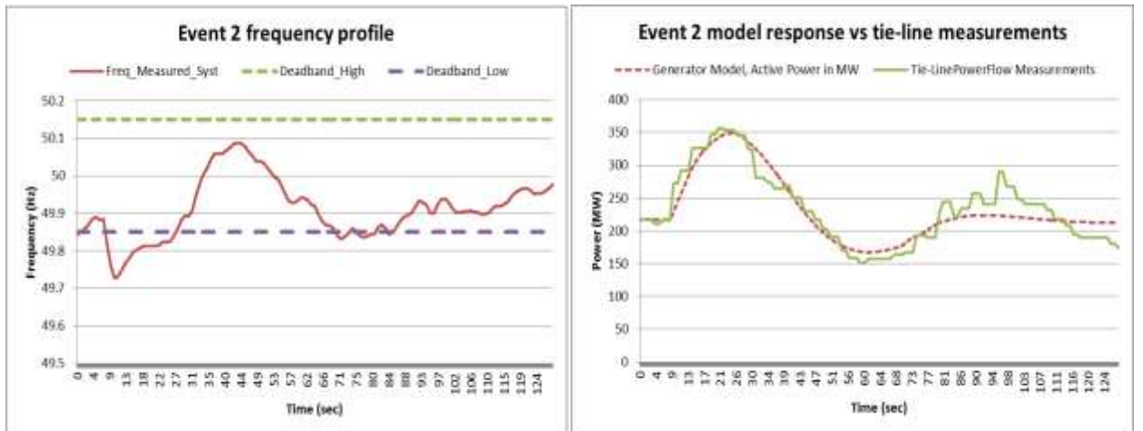
Figure 4.14 Event 2 TGOV5 governor model (with frequency dead band) simulation results
