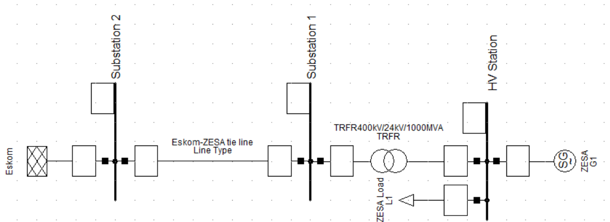
Figure 4.6 Grid used to tune generator to the mimic tie-line behaviour
