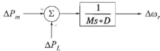
Figure A.0.4 Rotor dynamics transfer function [2]
