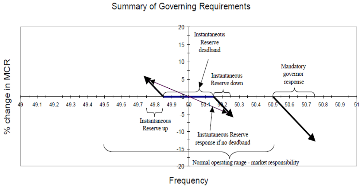
Figure B.0.1 Graphical representation of governing requirements [15]
