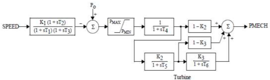
Figure 4.4 IEESG0 steam turbine model [14]
