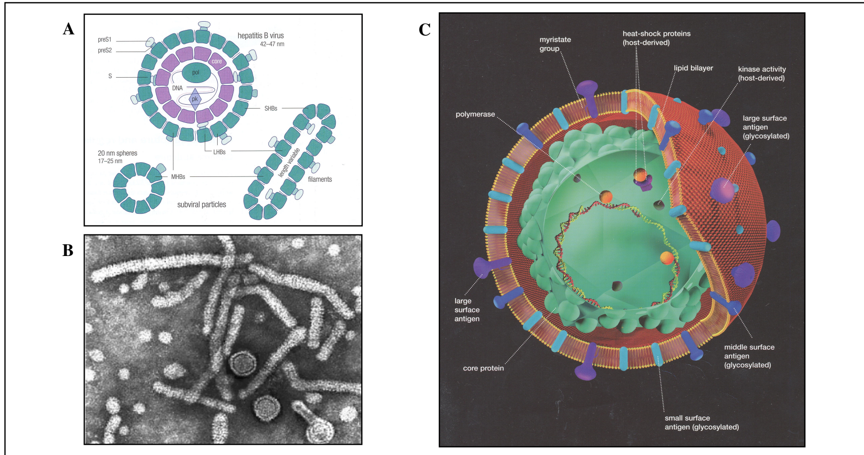
Figure 1.3 Structure of HBV virions and subviral particles. (A) Schematic model of a virion, 20 nm sphere, and filament [Kann, 2002]. (B) Electron micrograph showing Dane particles, spheres, and filaments in sera [Stannard, 2004]. (C) Three-dimensional representation of a Dane particle [Kann, 2002].
