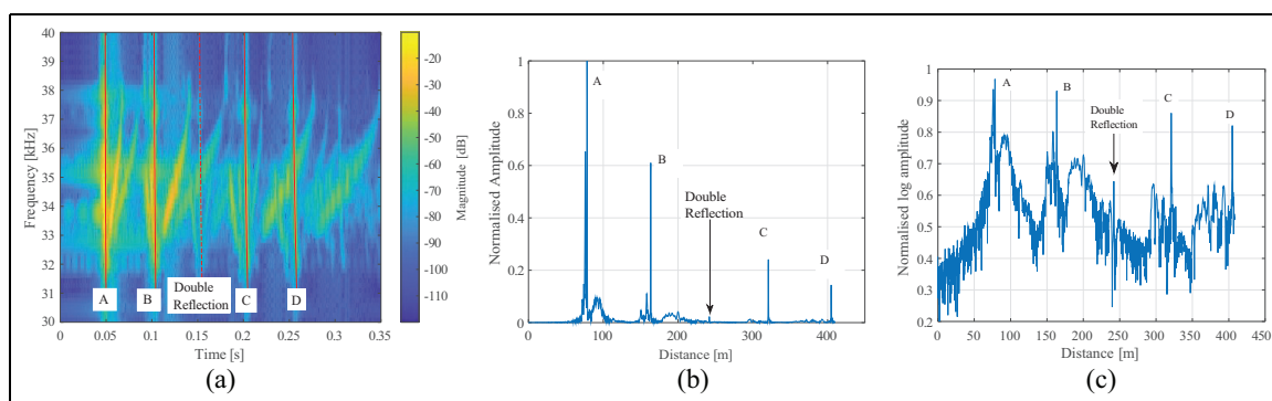
Figure 4. (a) Spectrogram of the simulated baseline signal for the experimental response and (b) & (c) the equivalent distance domain signals.
