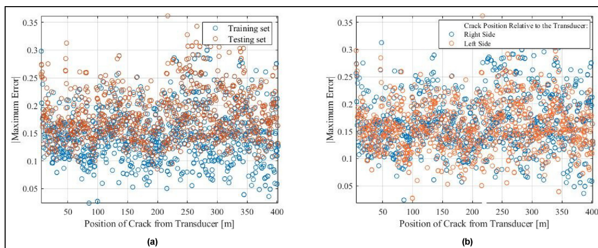
Figure 12. The VAE maximum absolute error for reconstructed response signals in (a) the training and testing sets and (b) samples located to the right and left of the transducer. VAE: variational autoencoder.
