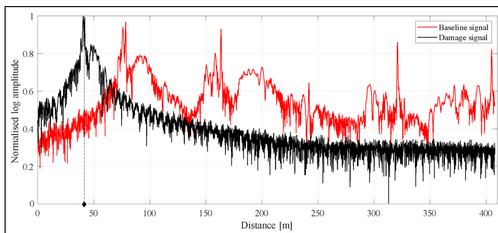
Figure 14. Damage signatures simulated using the procedure in the study by Ramatlo et al. 11 for a crack located at (•••) 41.375 m from the transducer on the left side.
