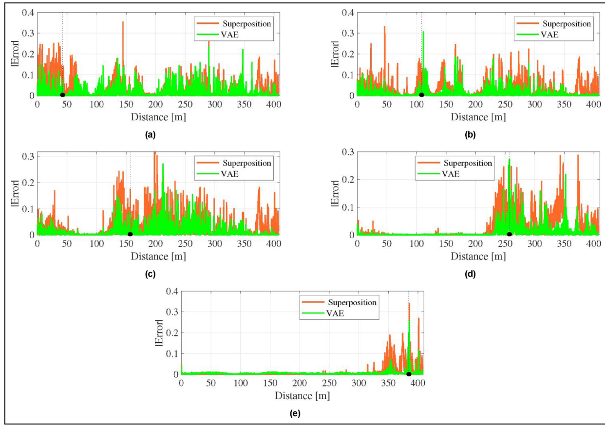
Figure 16. Absolute errors obtained from the VAE and superposition results for a crack located at (●···) (a) 41.375 m from the transducer on the left side, (b) 108.5 m from the transducer on the right side, (c) 154.8750 m from the transducer on the right side, (d) 253 m from the transducer on the left side and (e) 379.25 m from the transducer on the right side. VAE: variational autoencoder.
