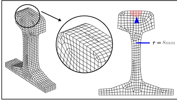
Figure 5. A hybrid model of the defect geometry with an 8 mm radius crack in the head of the rail.
