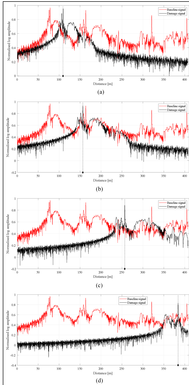
Figure A1. Damage signatures simulated using the procedure in Ramatlo et al. 11 for a crack located at (•••) (a) 108.5 m from the transducer on the right side, (b) 154.8750 m from the transducer on the right side, (c) 253 m from the transducer on the left side and (d) 379.25 m from the transducer on the right side.
