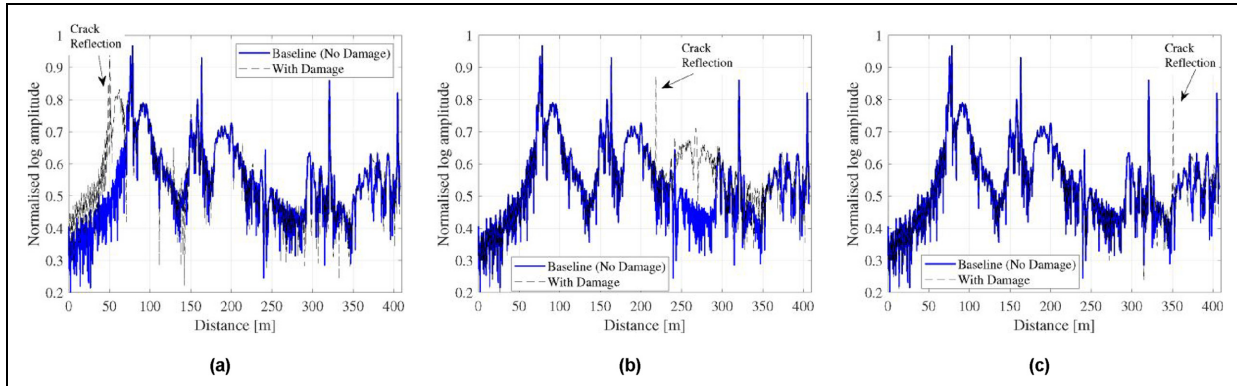
Figure 7. Virtual experimental response signals ( y_i ) containing damage reflections at user-specified distances of (a) 50 m, (b) 220 m and (c) 350 m.
