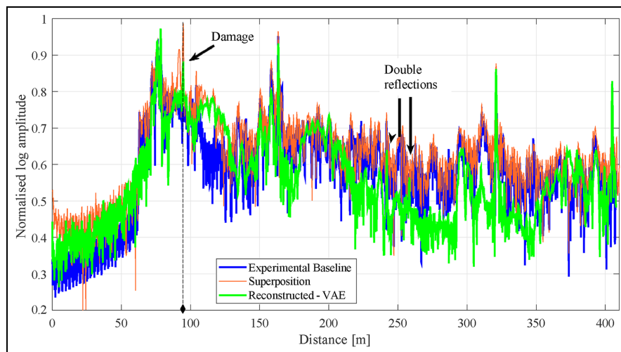
Figure 17. Inspection signal generated from a field experiment and a VAE model trained with virtual experimental signals. VAE: variational autoencoder.
