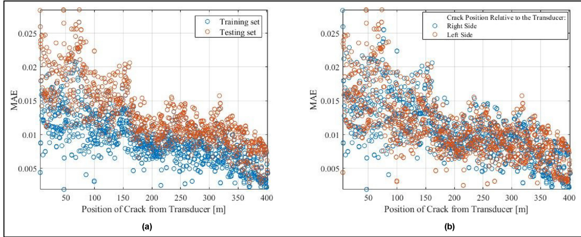
Figure 10. The VAE MAE for reconstructed response signals in (a) the training and testing sets and (b) samples located to the right and left of the transducer.
