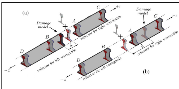
Figure 6. Digital models of the considered section of an operational rail with fake damage at specified distances d (a) between the transducer and weld B, and (b) between welds A and C.
