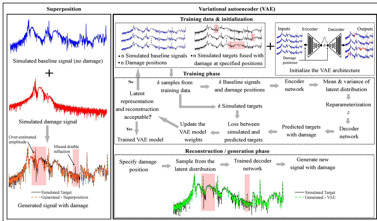
Figure 1. The generation of synthetic data containing damage signatures using the VAE and the superposition principle.
