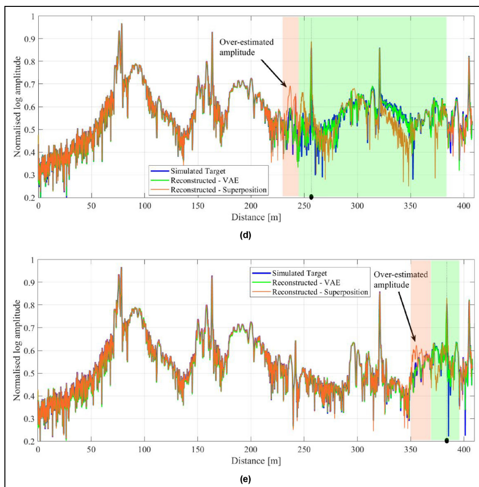
Figure 15. Response signals reconstructed from a VAE compared to superposition and the original target response for a crack located at (•••) (a) 41.375 m from the transducer on the left side, (b) 108.5 m from the transducer on the right side, (c) 154.8750 m from the transducer on the right side, and (d) 253 m from the transducer on the left side and (e) 379.25 m from the transducer on the right side. The area shaded in green and orange indicates the region over which the energy reflected from the damage in the superposition reconstructed response signals is significant. VAE: variational autoencoder.
