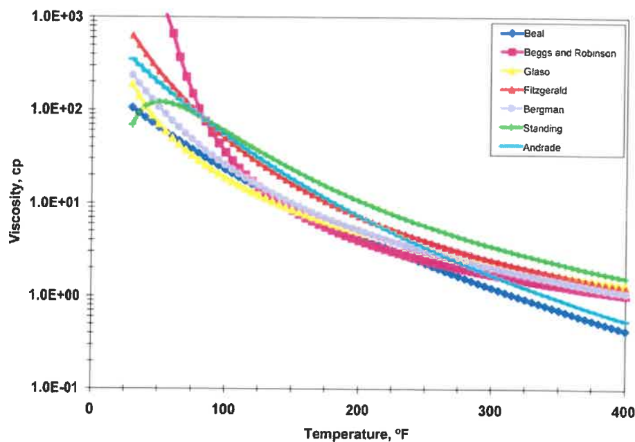
Figure 7: Viscosity models as a function of temperature (Macias-Salinas et al [2013]).
