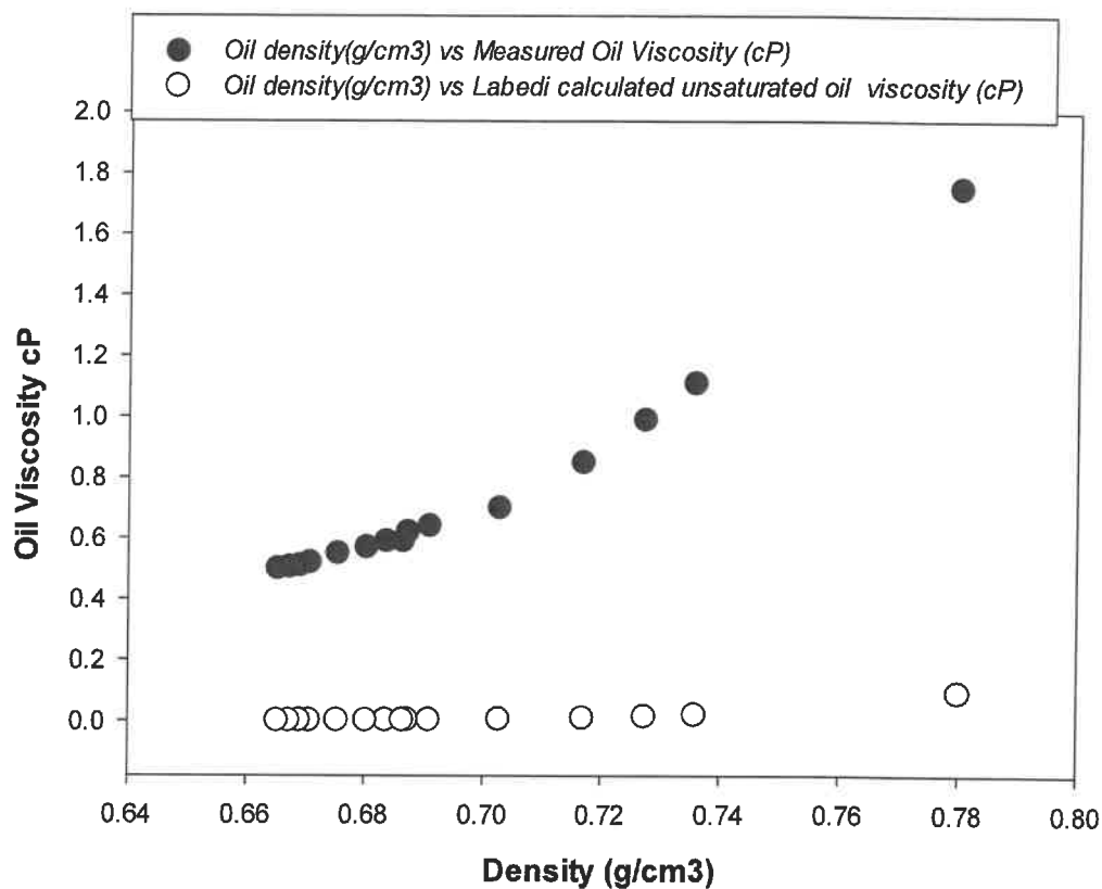
Figure 24: Relationship between Calculated Oil Viscosity and Measured Oil Viscosity.
