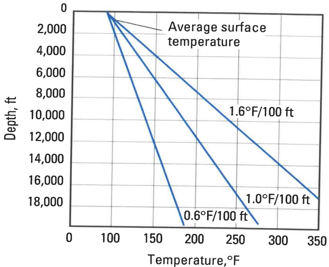
Figure 9: The relationship between reservoir depth and temperature
