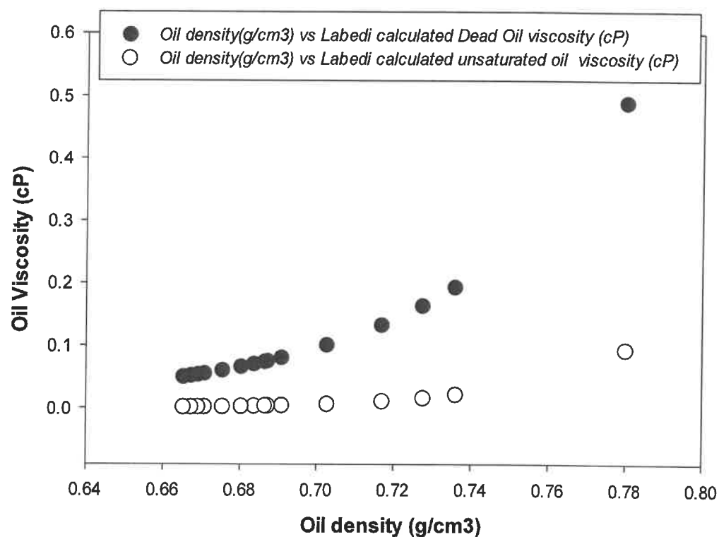
Figure 23: Trend graph (Viscosity vs Oil density ) using the Labedi model
