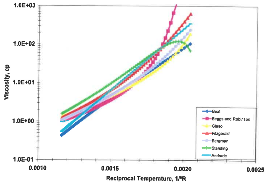
Figure 8: Area of applicability of the Andrade model in compared to other models (Macias-Salinas et al [2013]).
