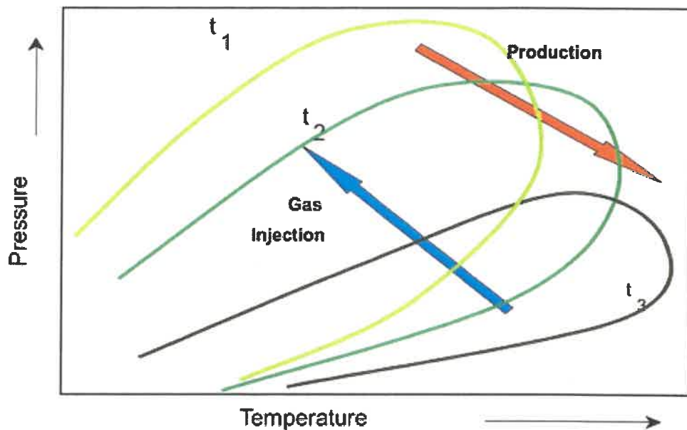
Figure 4: Pressure vs temperature during production and injection based on the different processing stages as shown in figure 1
