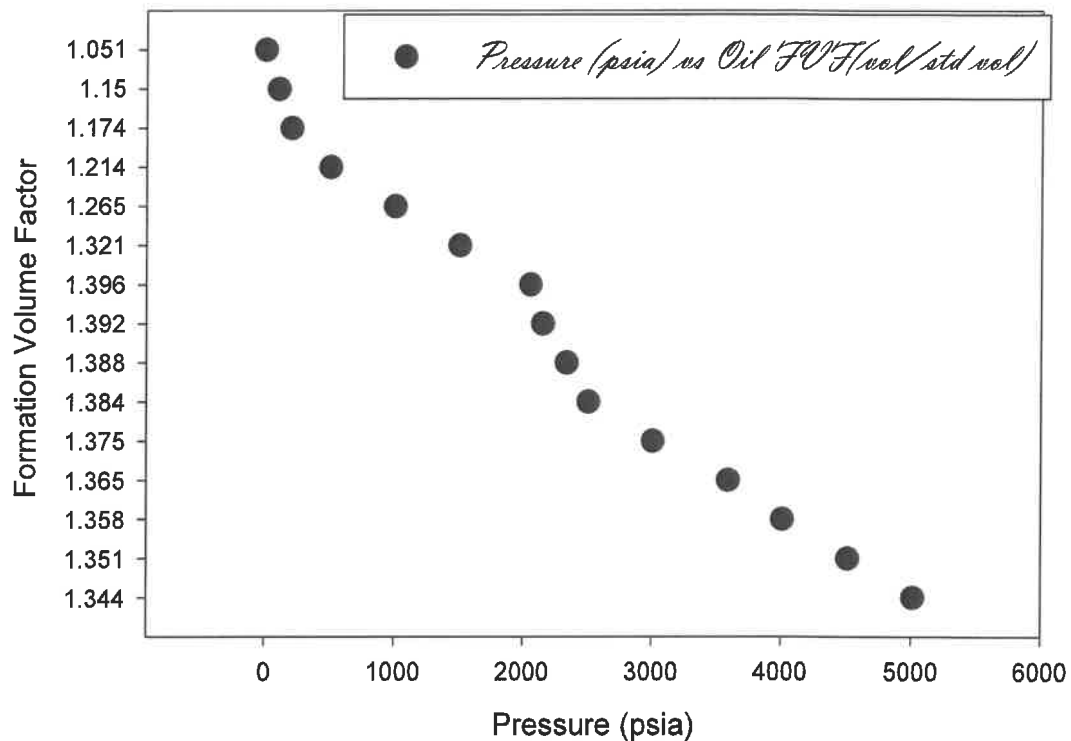
Figure 17: DL #1 Pressure – Formation Volume Factor
