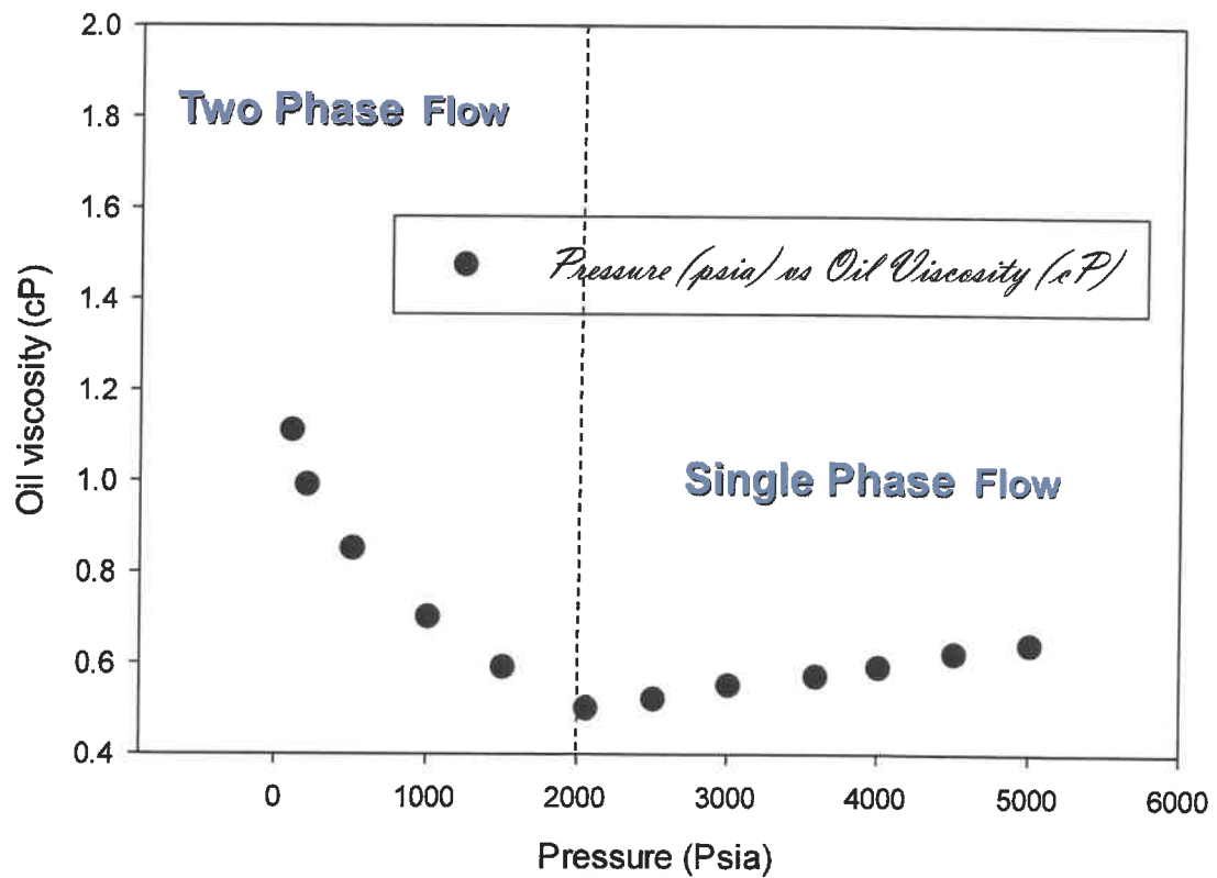
Figure 18: Viscosity of reservoir fluid vs Pressure
