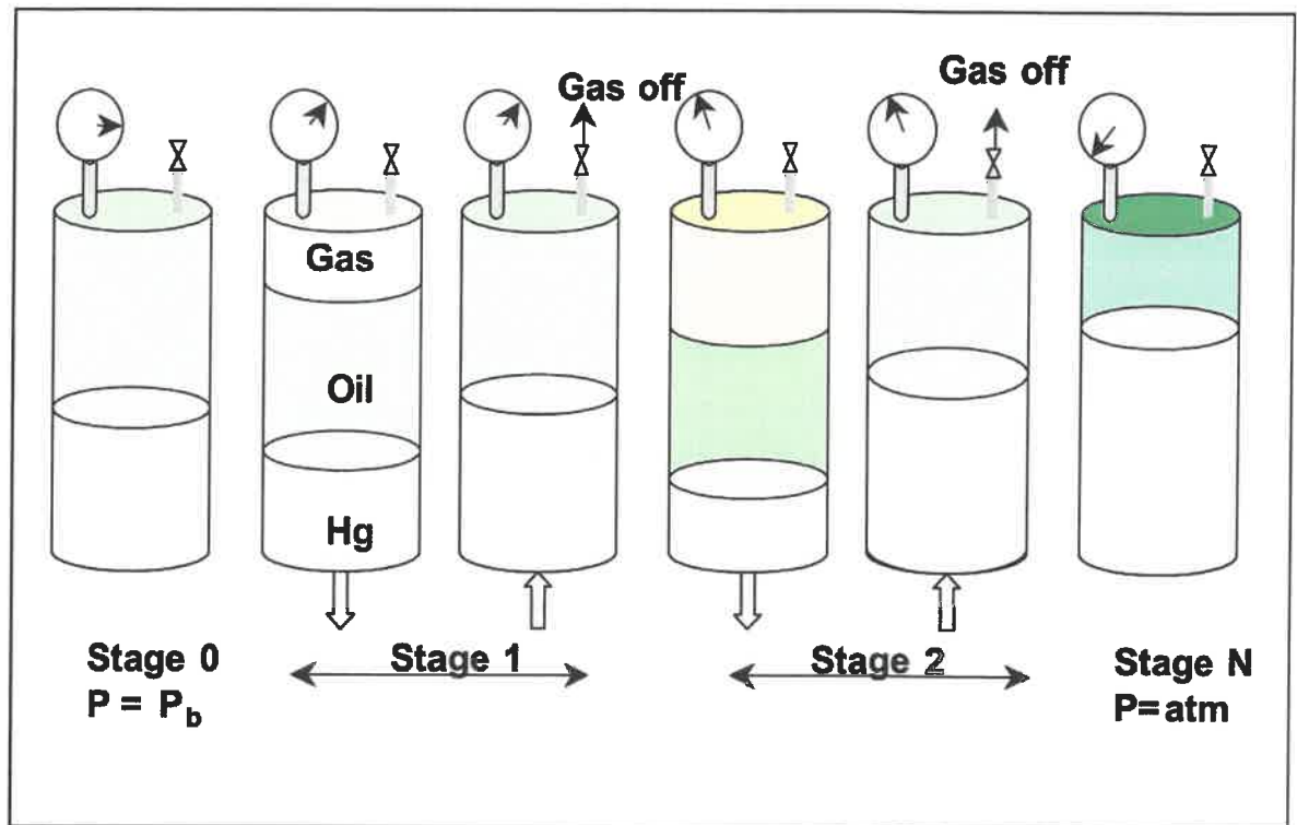
Figure 14: Illustration of the Differential Liberation Tests
