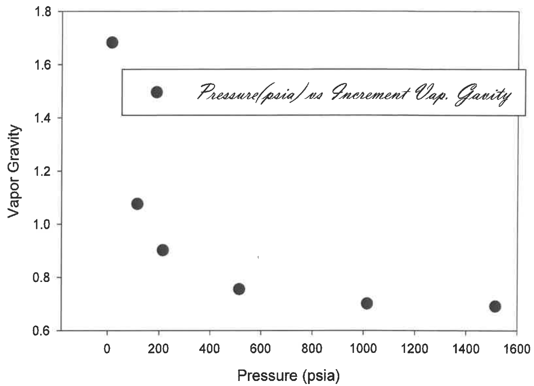
Figure 16: DL #1 Pressure Vapour Gravity
