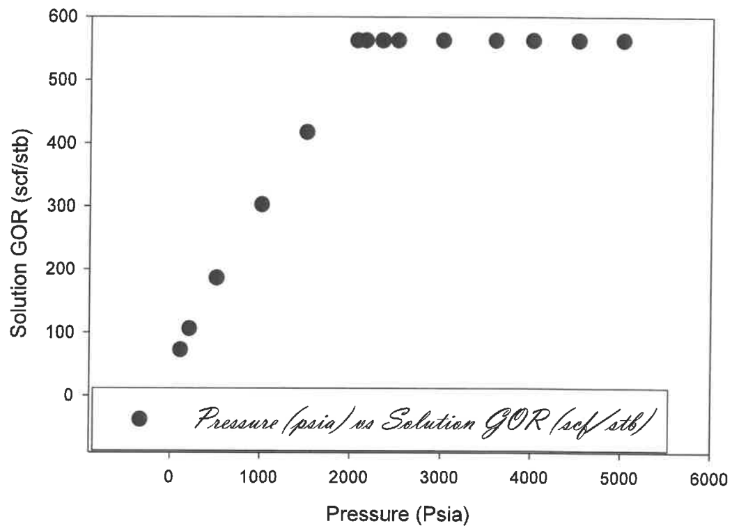
Figure 15: DL #1 Pressure - Oil Solution GOR
