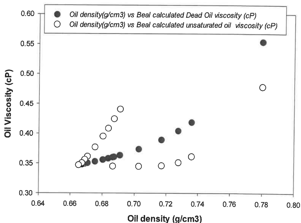
Figure 21: Trend graph (Viscosity vs Oil density ) using the Beal model
