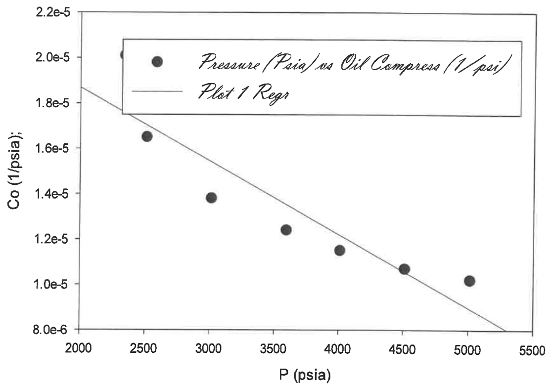
Figure 13: Illustration of the Pressure vs Oil compression
