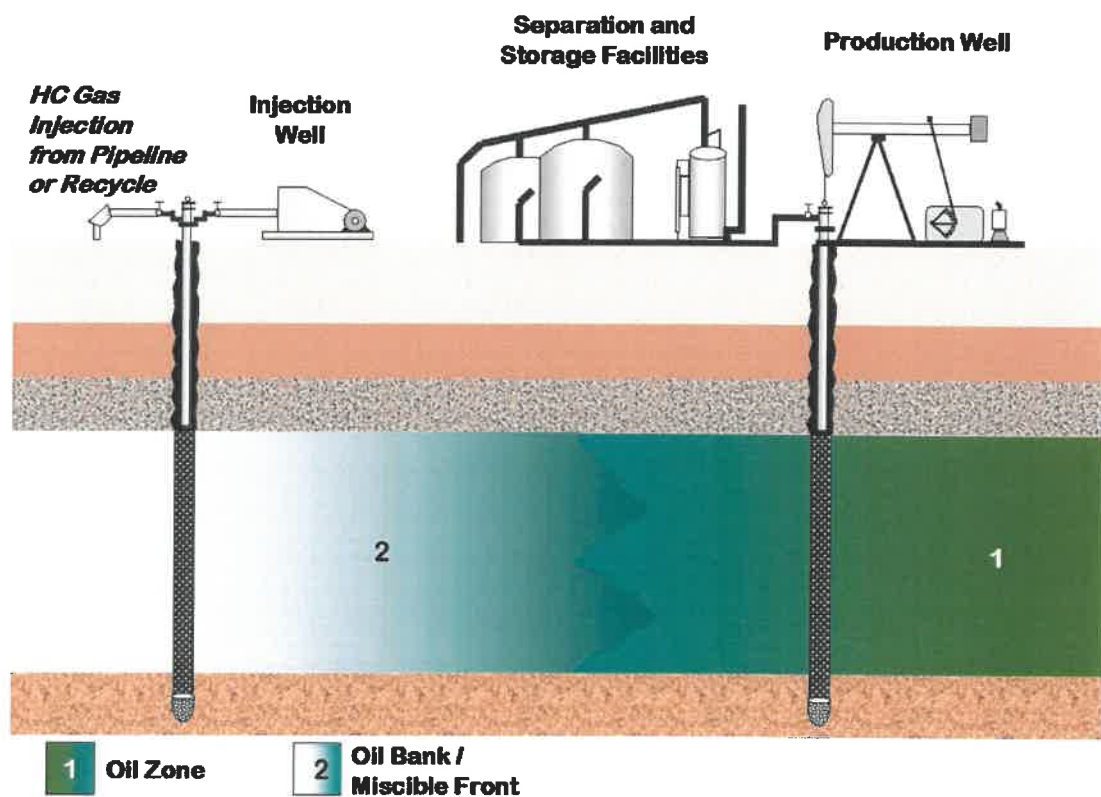
Figure 1: The various production processes of oil recovery
