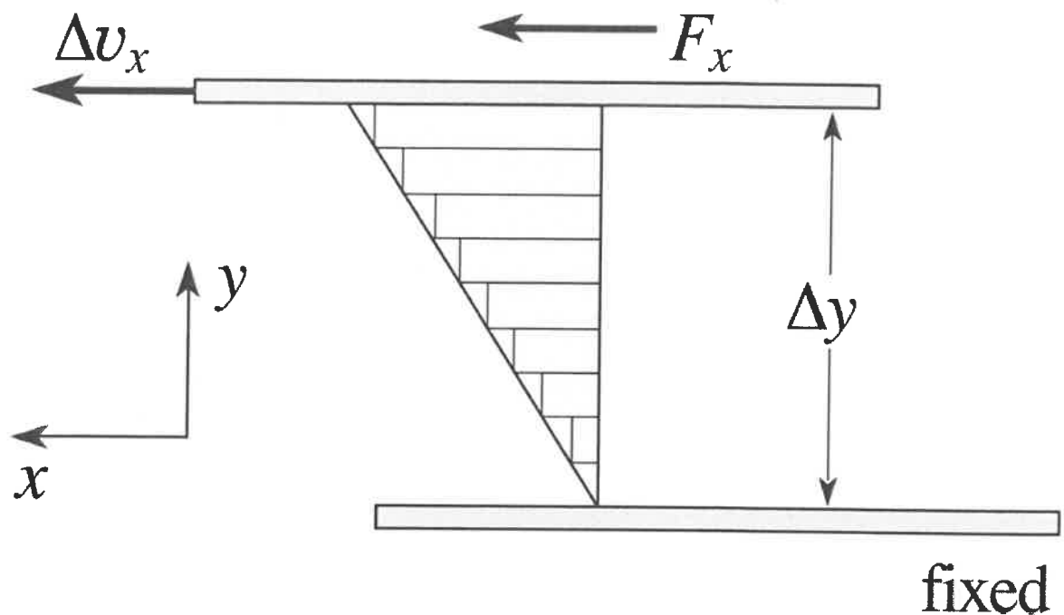
Figure 2: A fluid between two plates under a shear stress. F_x is the force acting on the top plate, V_x is the speed at which the top plate is moving as a result of the force applied and Y is the thickness between the top plate and the bottom plate.
