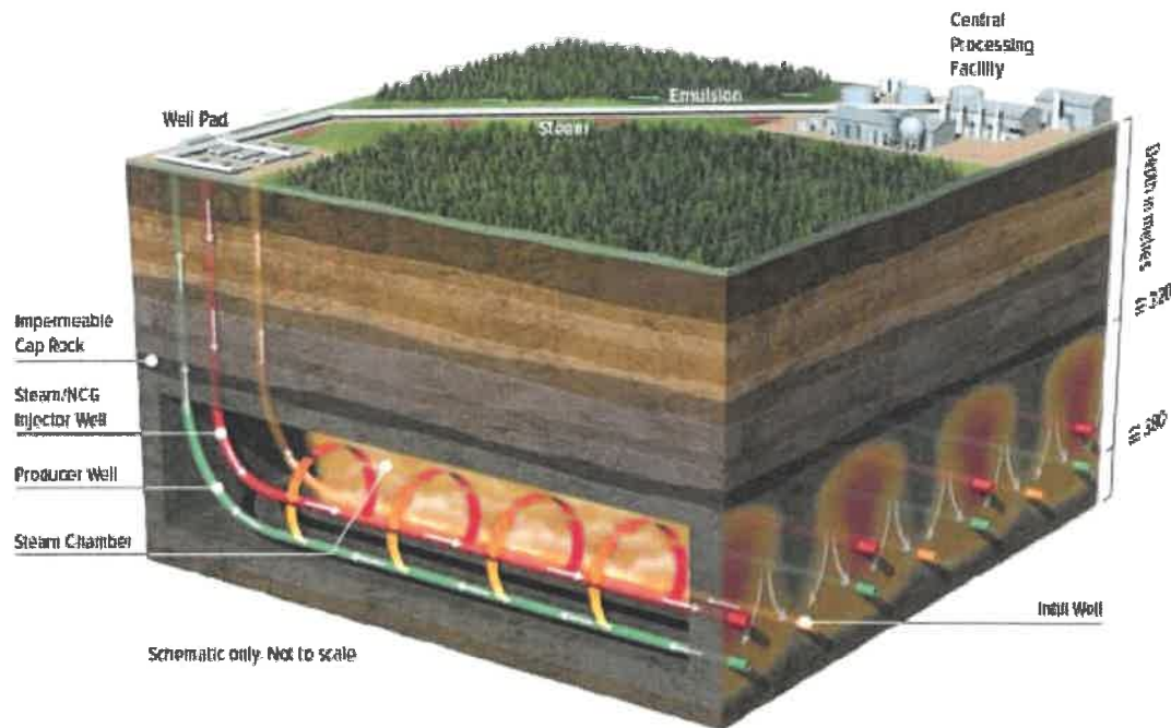
Figure 5: Illustration of the SAGD Process (source: https://www.megenergy.com/operations/steam-assisted-gravity-drainage-sagd )
