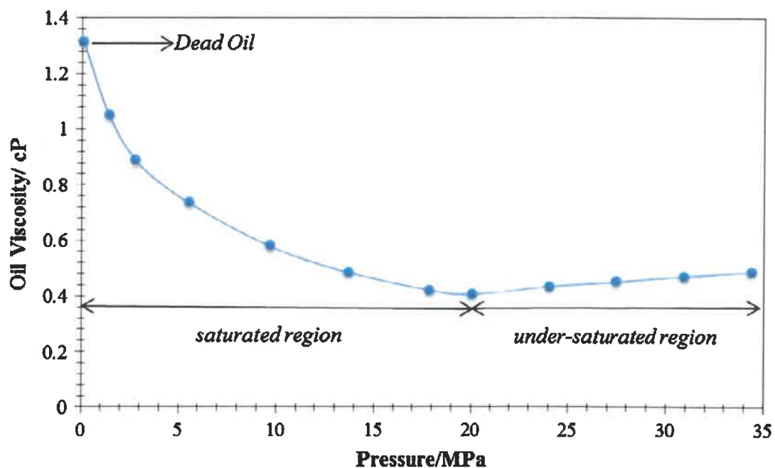
Figure 6: Viscosity curve as a function of pressure (Hemmati-Sarapardeh et al [2014])
