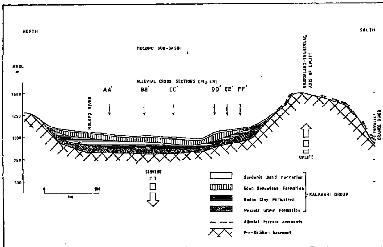
Figure 4.8 Longitudinal profile of the proto-Molopo after back-tilting and isostatic adjustments.
