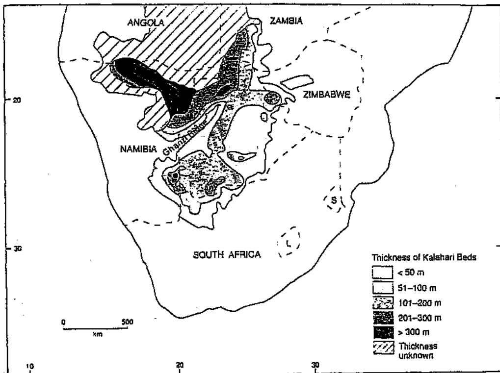
Figure 1.4 The thickness of the Kalahari Group sediments, after Thomas and Shaw (1991).
