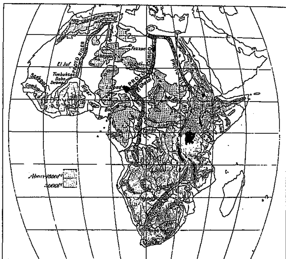
Figure 6.9 The proto-Orange as suggested by Schwarz (1919).
