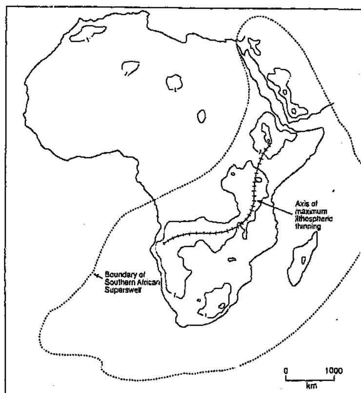
Figure 2.2 The Southern African Superswell (after Summerfield, 1996). Contours are drawn at 1 km intervals and are generalised from one-minute digital elevation data.
