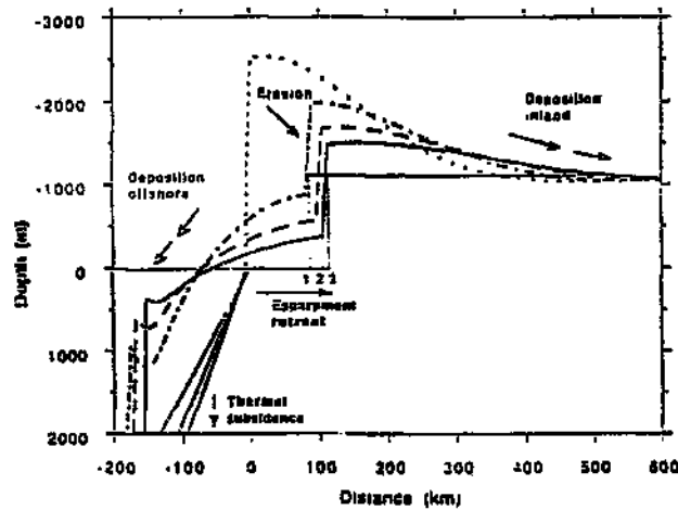
Figure 2.7 Evolution of the continuous plate model through time (after ten Brink and Stern, 1992). The initial uplift profile (heavy dotted line) is eroded by three erosional cycles, and the topography is allowed to rebound by regional isostasy after each cycle (other heavy lines).
