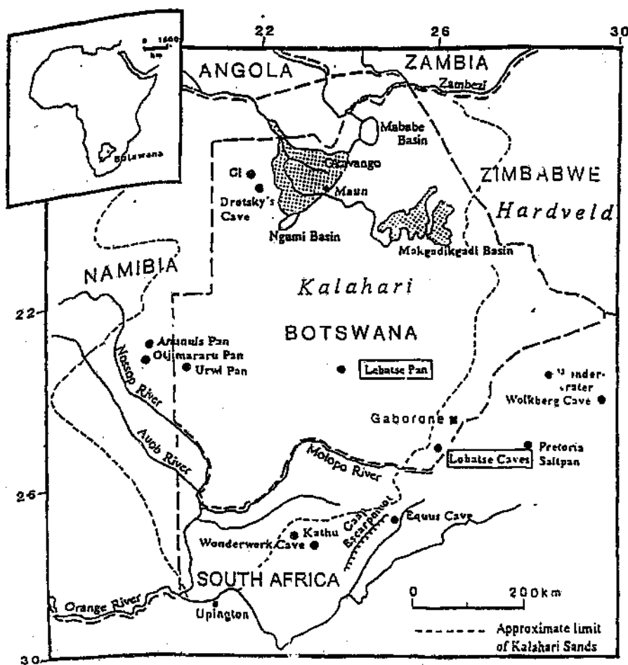
Figure 5.6 Map of central southern Africa showing the Lebatse Caves and the Lebatse Pan, and other sites of earlier palaeoclimatic studies (after Holmgren, 1995).
