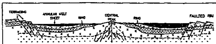
Figure 2.18 Schematic cross section through a complex impact structure (after Reimold and Gibson, 1996). Erosion is indicated by the lack of impact melt and/or fallback breccia on top of the central uplift region.
