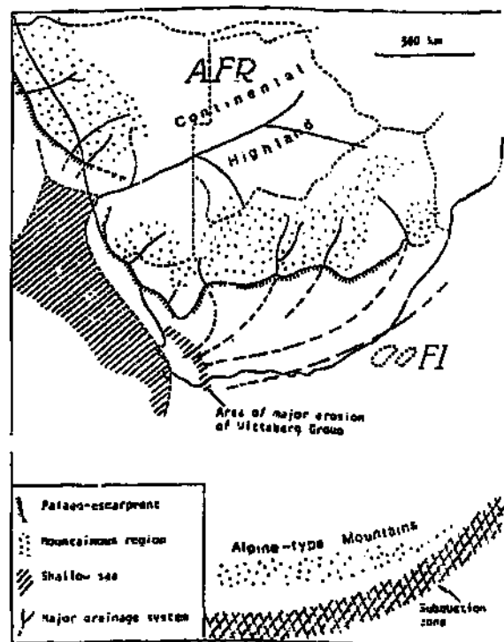
Figure 3.7 Schematic pre-glaciation palaeogeography of southern Africa (after Visser, 1987).
