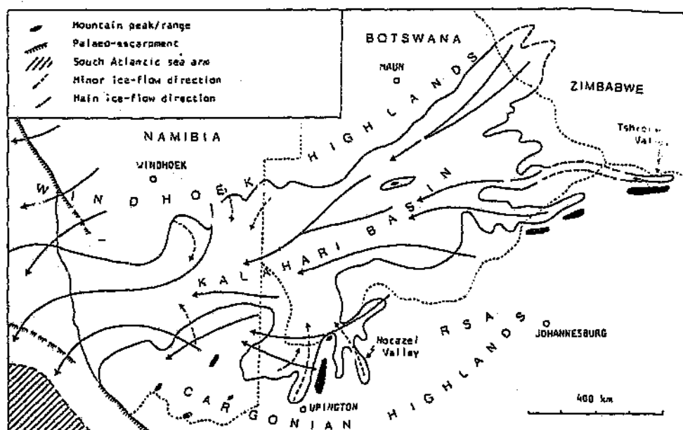
Figure 3.5 Outline of the Kalahari Basin during the Maximum glaciation (after Visser, 1987).
