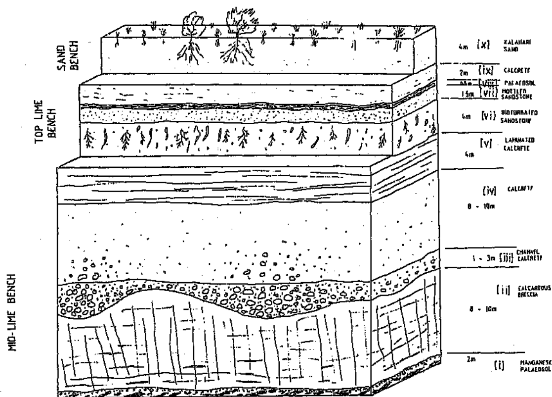
Figure 6.3 Overburden at the north wall of the Mamatwan mine (after Williams, 1993).
