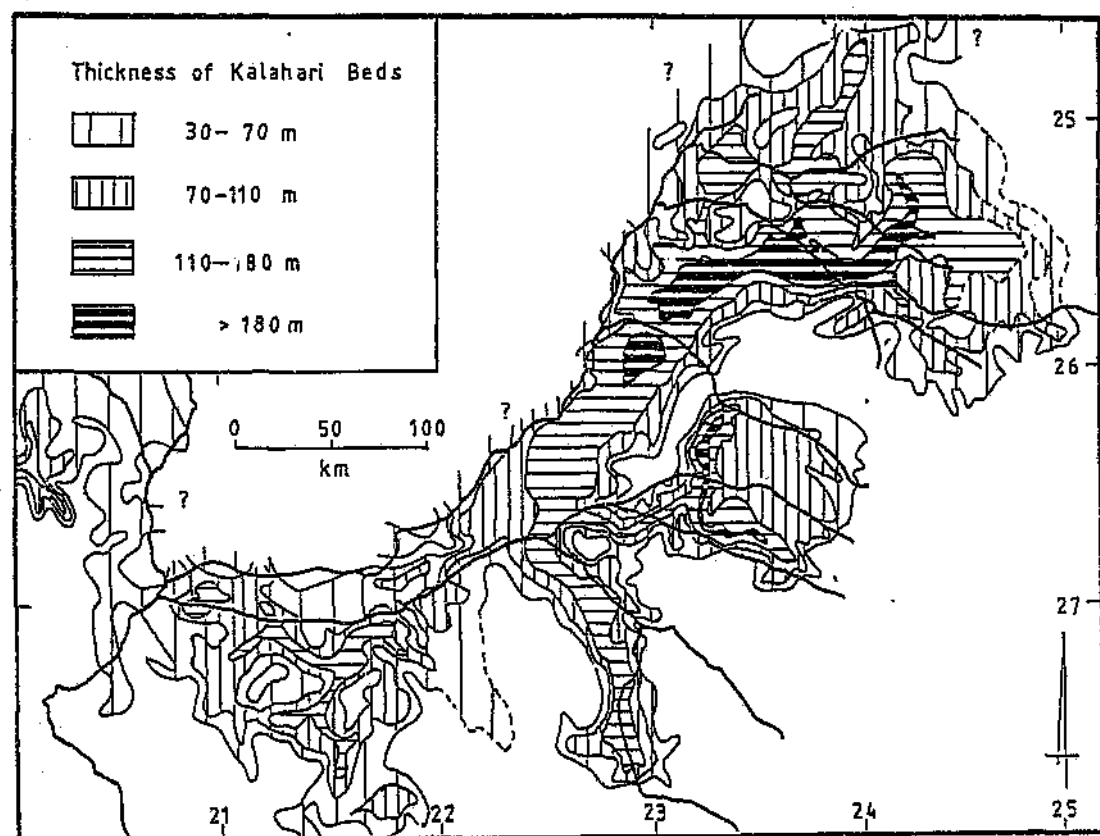
Figure 4.6 Thickness of the Kalahari Beds in the Molopo drainage area.
