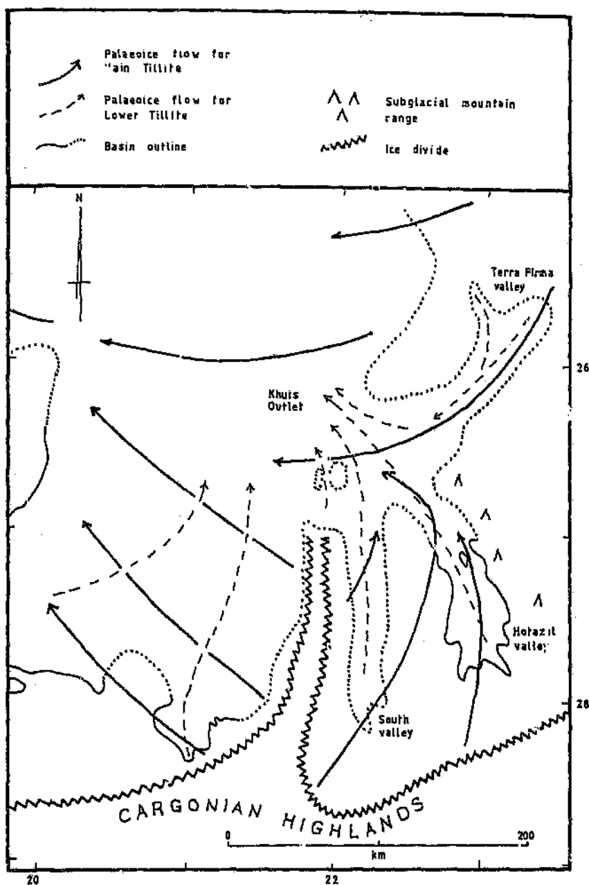
Figure 3.6 Palaeo-ice flow directions in the Molopo drainage area. Based on Visser (1983a).
