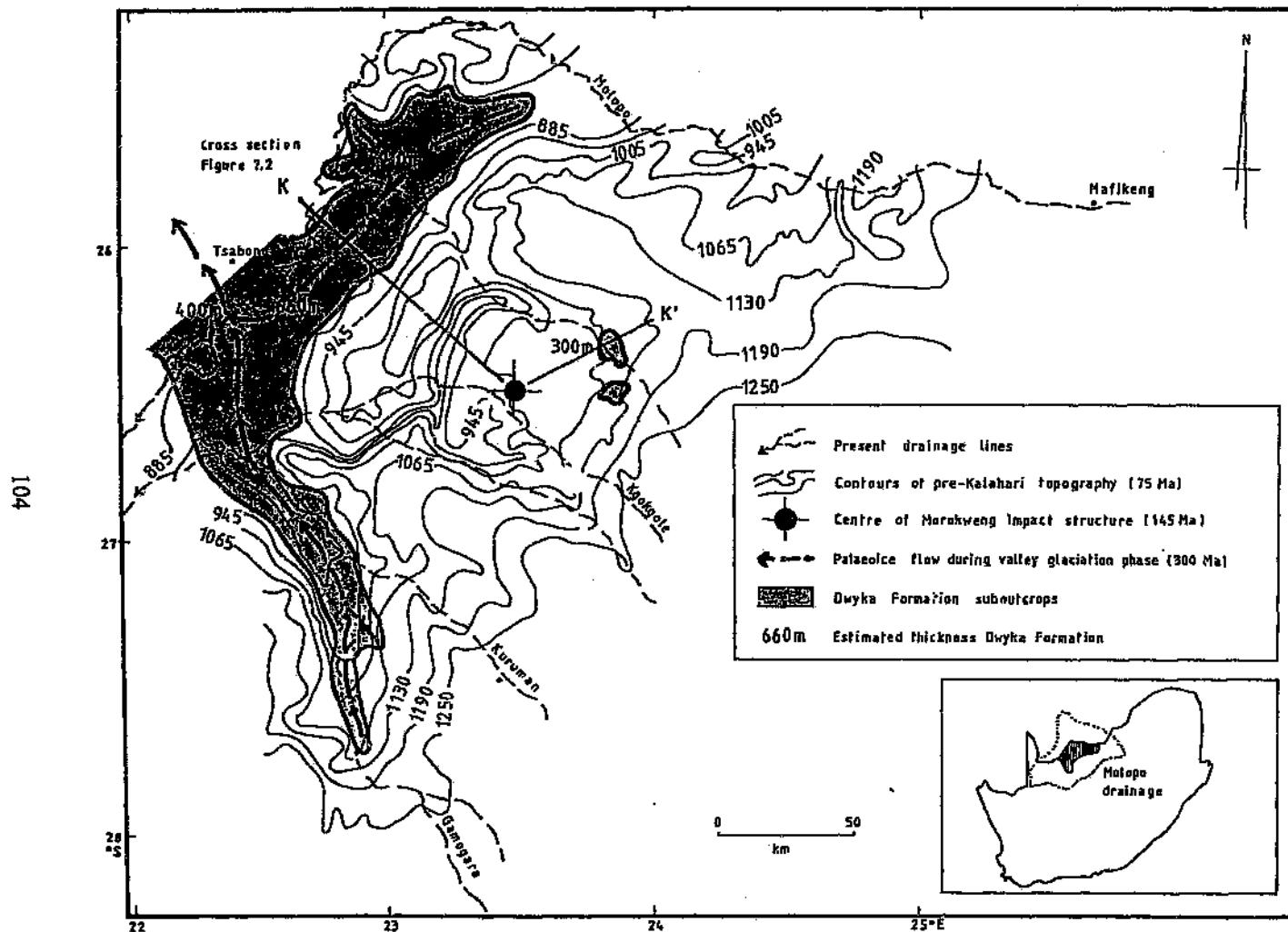
Figure 3.9 Pre-Kalahari topography and Dwyka Formation suboutcrops in relation with the Morokweng impact structure.
