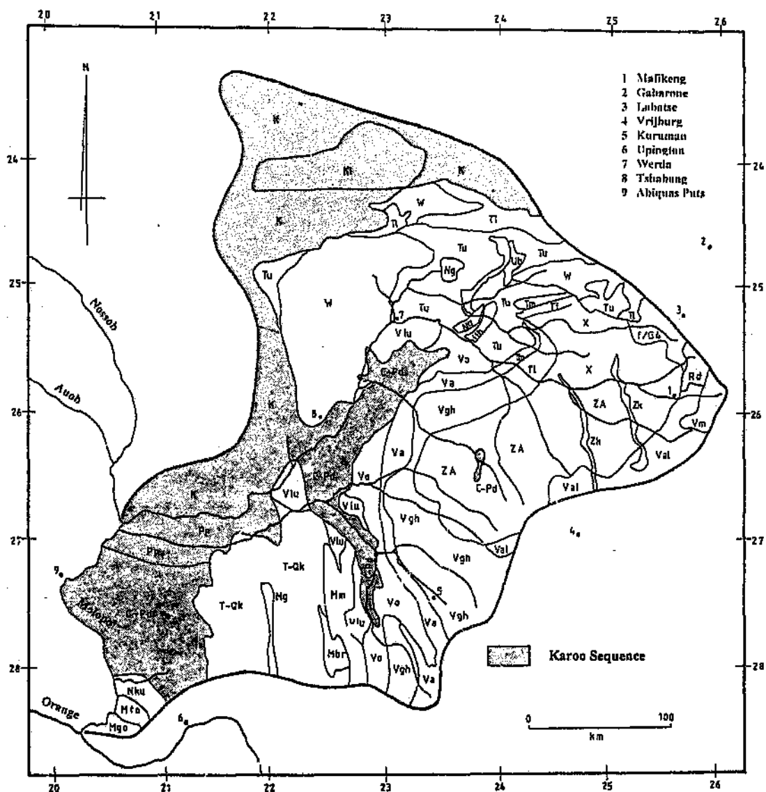
Figure 2.13 Pre-Kalahari geology, emphasising Karoo Sequence rocks in the Molopo drainage area. See table 2.1 for the legend.
