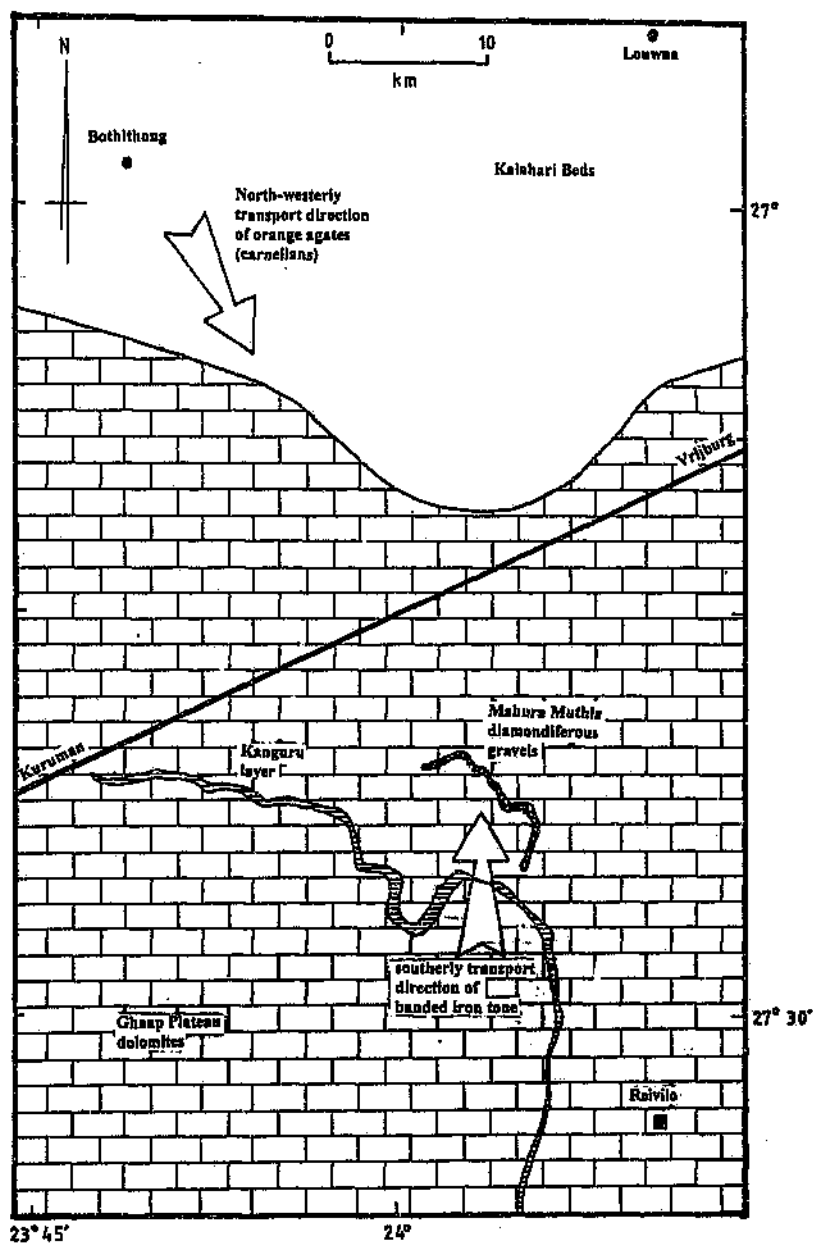
Figure 6.4 Mahura Muthla diamondiferous gravels on the Ghaap Plateau.
