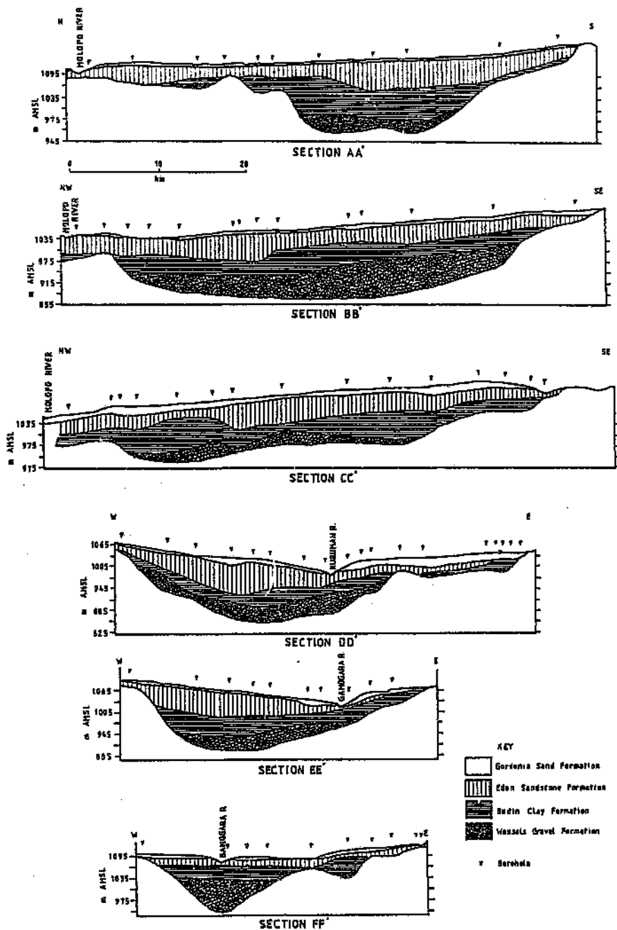
Figure 4.9 Cross sections of the sediment-filled proto-Molopo (modified after Smit, 1977).
