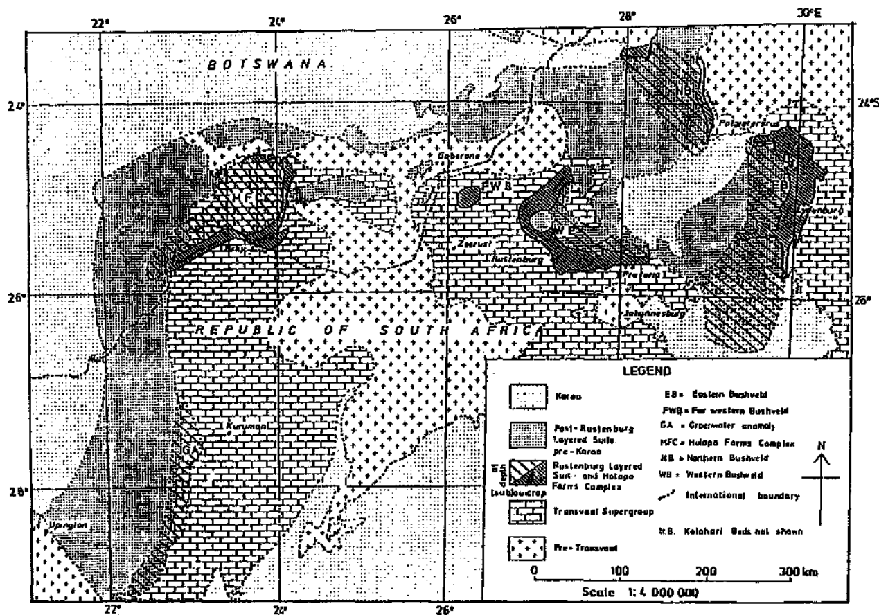
Figure 2.12 Geological sketch map showing extent of basic and ultrabasic rocks correlated with the Bushveld Complex (after Gould et al. , 1987).
