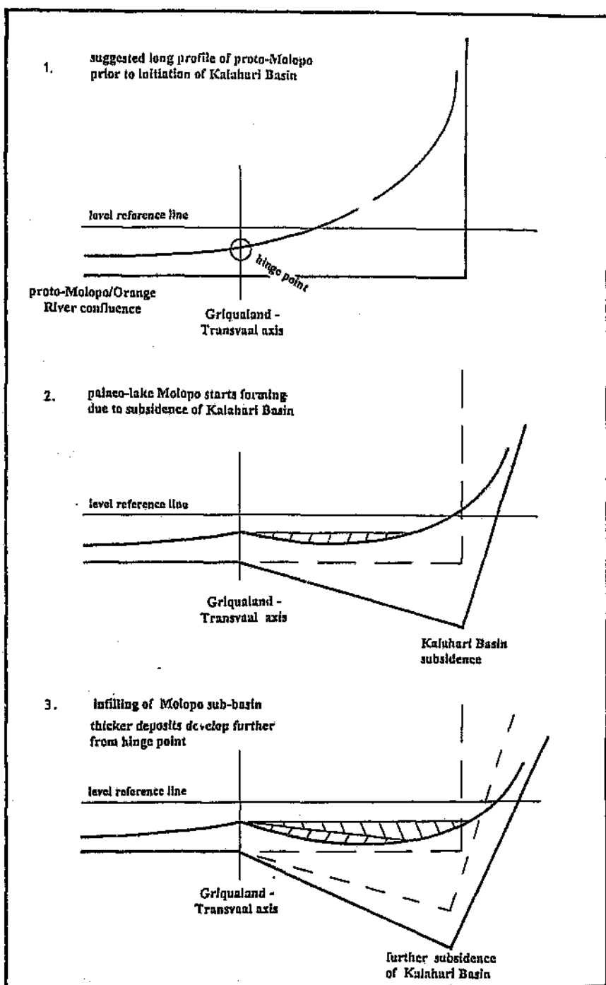
Figure 4.7 The back-tilting principle applied to the proto-Molopo.
