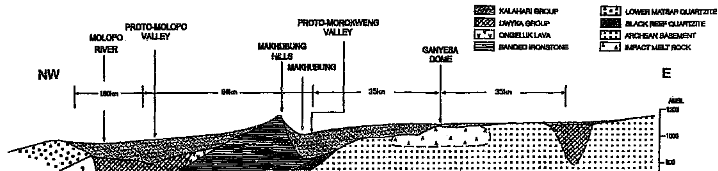
Figure 7.2 Schematic geological cross section through the Morokweng impact structure (after Reimold et al. , in press).
