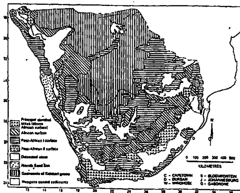
Figure 2.9 Simplified map of the principal cyclic landsurfaces of southern Africa (after Partridge, 1997b).
