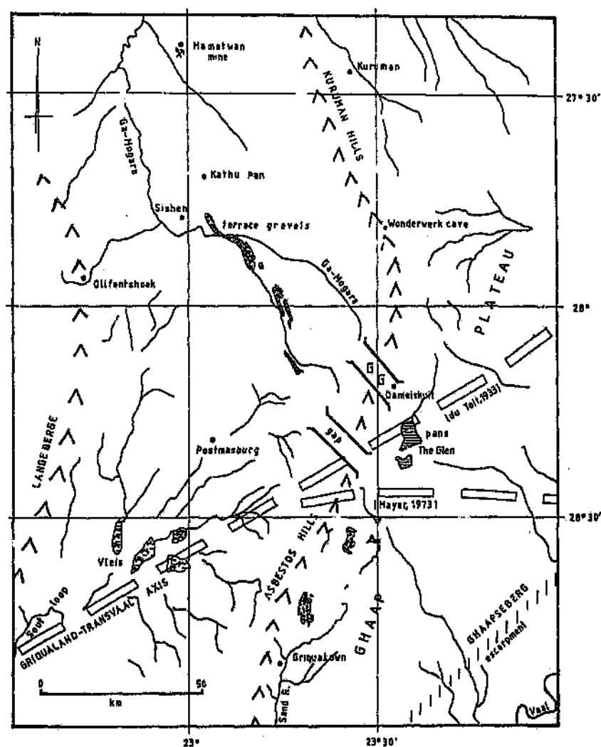
Figure 6.10 Palaeodrainage indicators in the Griqualand West study area.
