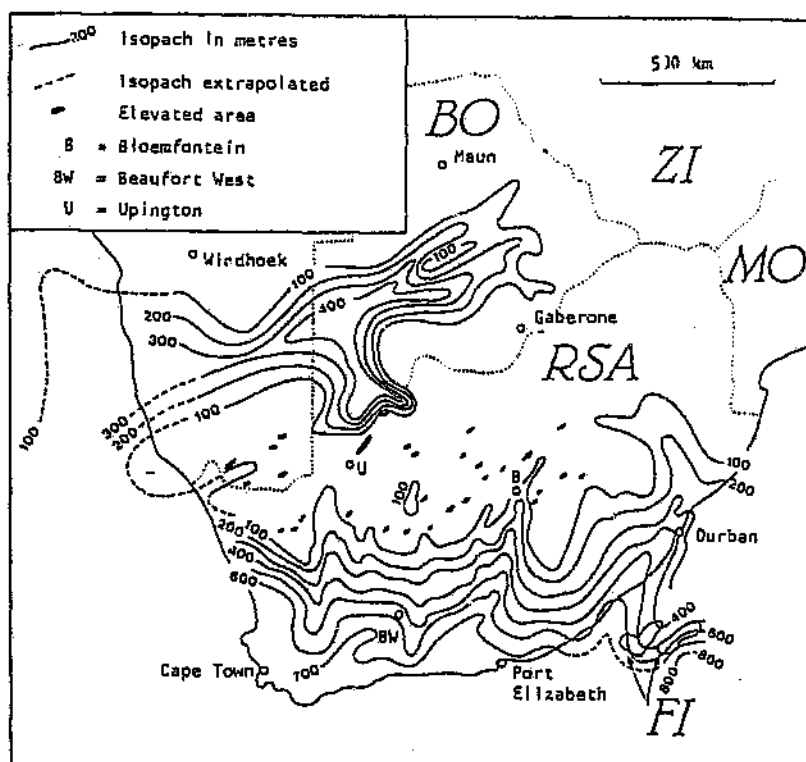
Figure 3.1 Isopach map of the glacial sequences in the Karoo and Kalahari Basins and on the Falkland Islands (after Visser, 1987).
