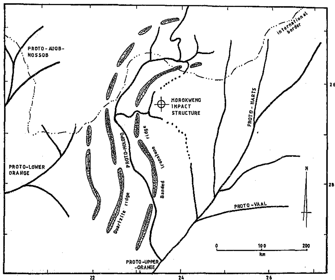
Figure 7.5 Late Cretaceous drainage.
