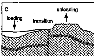
Figure 4.11 Diagrammatic representation of the principle of modelling denudational isostatic rebound for the Murray Basin (a, b, c) and distribution and magnitude (d) of loads (after Bishop and Brown, 1992).
