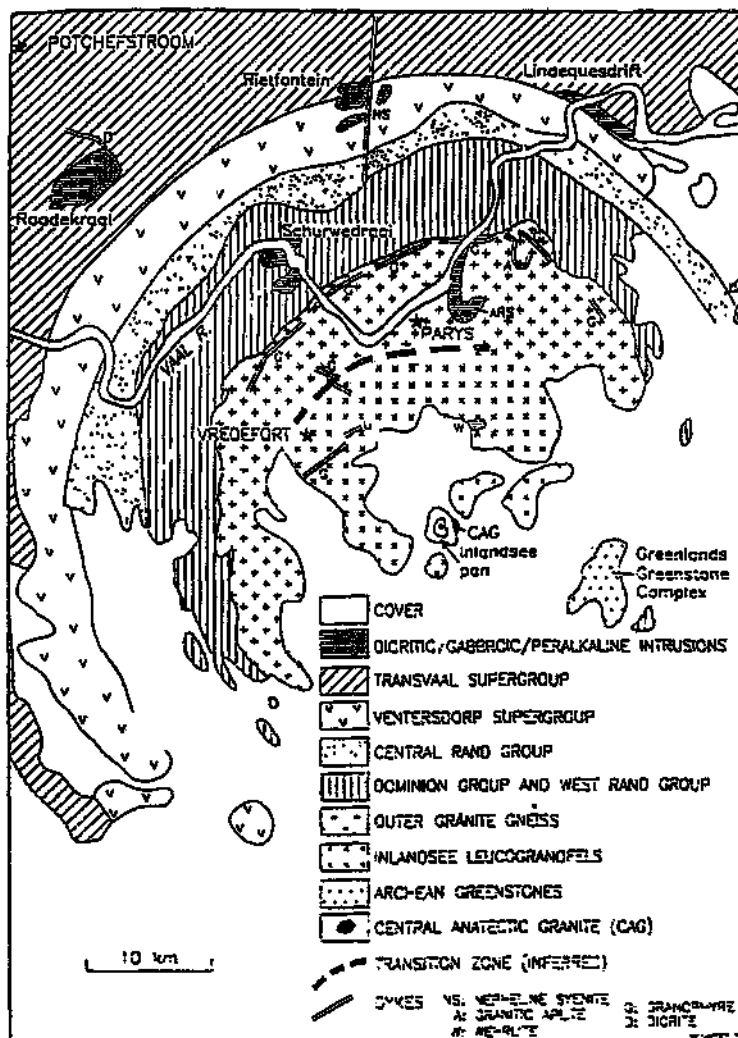
Figure 2.19 Schematic geological map of the Vredefort Dome (after Reimold and Gibson, 1996).
