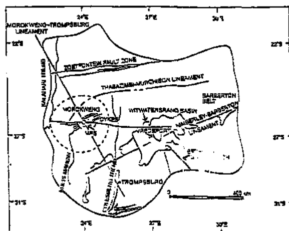
Figure 2.17 Kaapvaal province showing the Morokweng impact structure (after Corner et al. , 1997). MRS = Morokweng Ring Structure.
