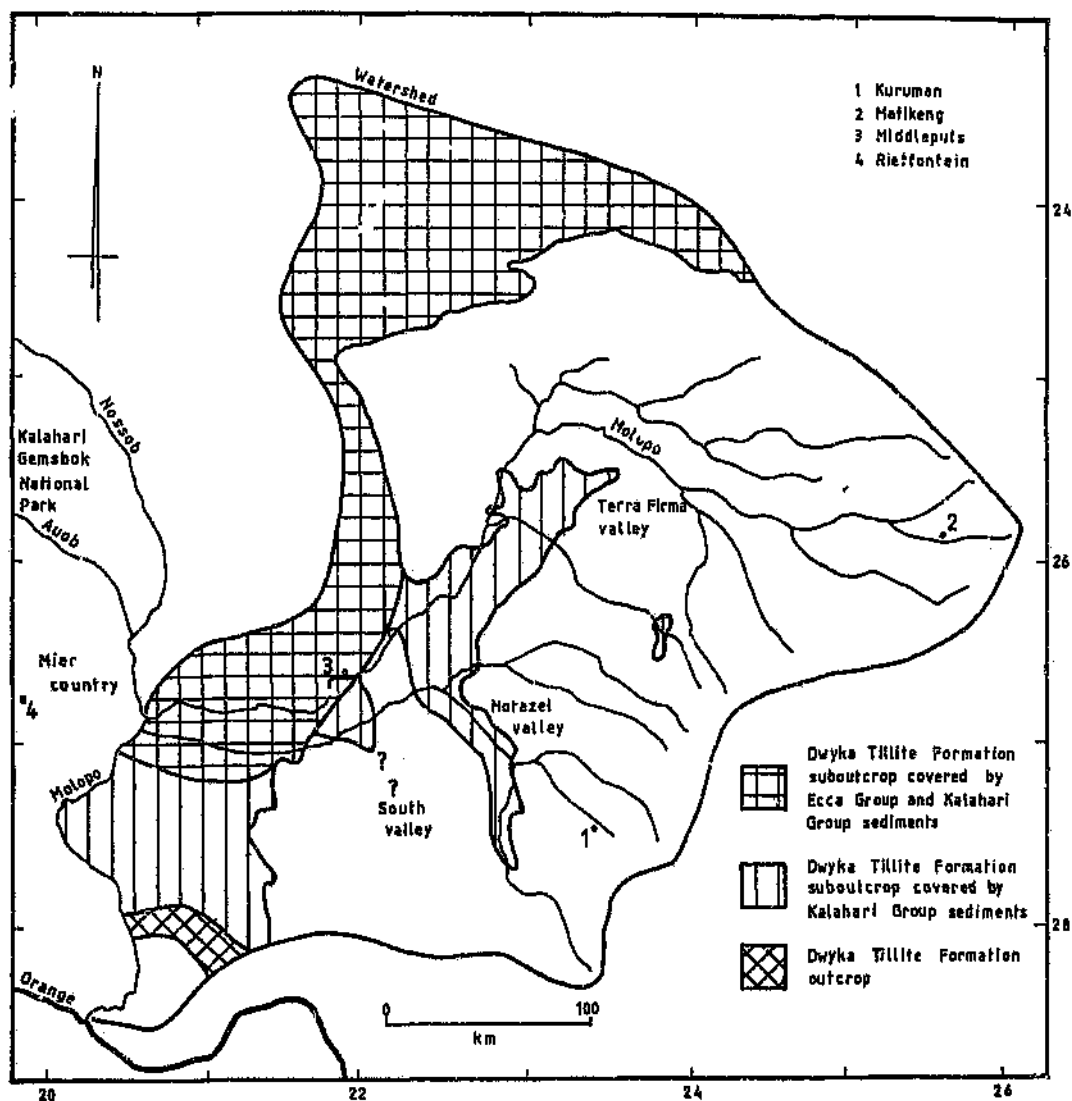
Figure 3.2 Dwyka Tillite Formation outcrops and suboutcrops in the Molopo drainage area. Based on the 1 : 1000 000 geological maps of South Africa and Botswana.
