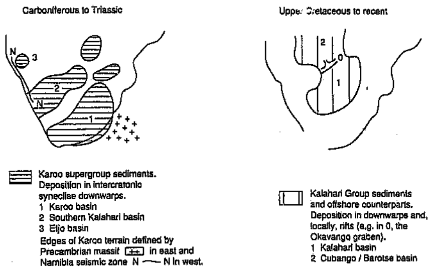
Figure 2.3 Sedimentary basins and deposits in southern Africa at two periods of the Phanerozoic (modified after Dingle et al. , 1983).
