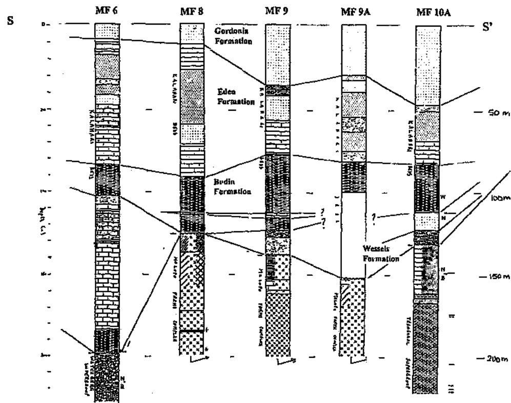
Figure 4.1 Graphic borehole logs across a pre-Kalahari palaeochannel. Based on data from Gould et al. (1989). See Fig. 4.3 for the location of the section.
