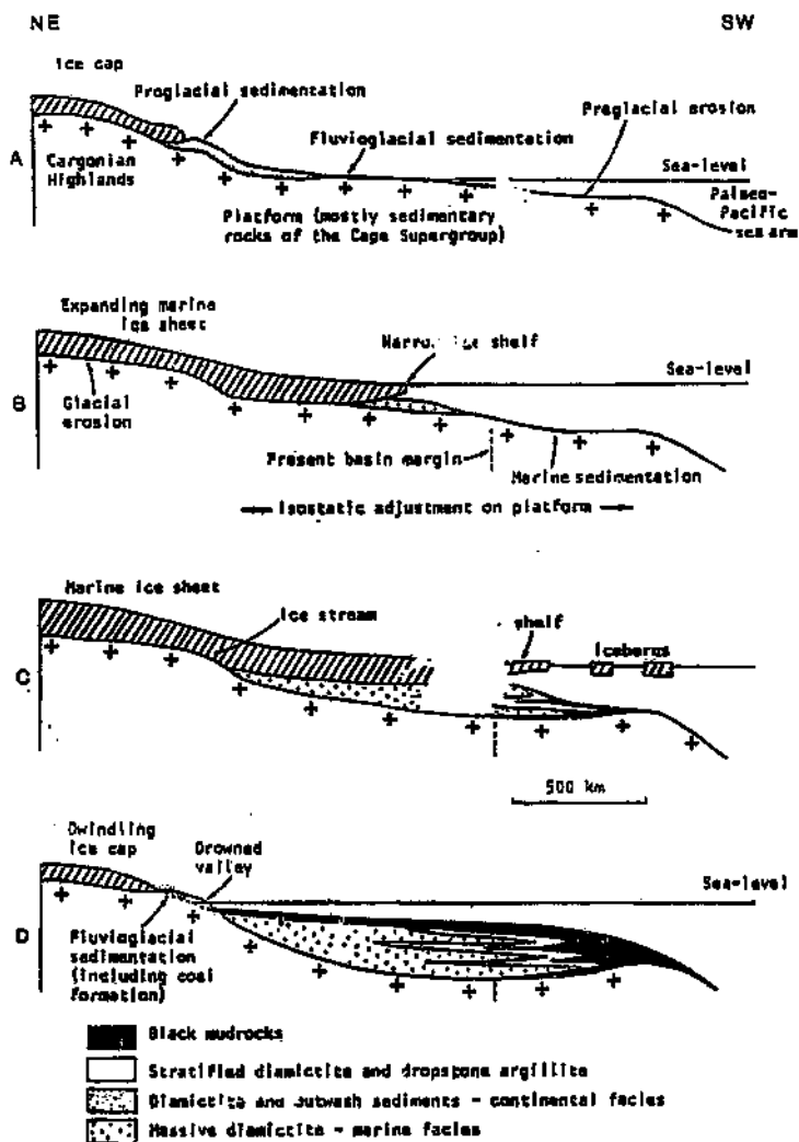
Figure 3.3 Stages in the growth and disintegration of the Permo-Carboniferous marine ice sheet in the Dwyka basin (after Visser, 1989).
