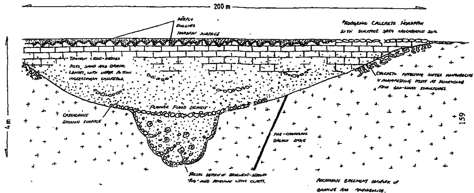
Figure 5.4 Schematic cross section of the Cainozoic deposits of a palaeovalley near Ramathlabama (after Brinn, 1991).
