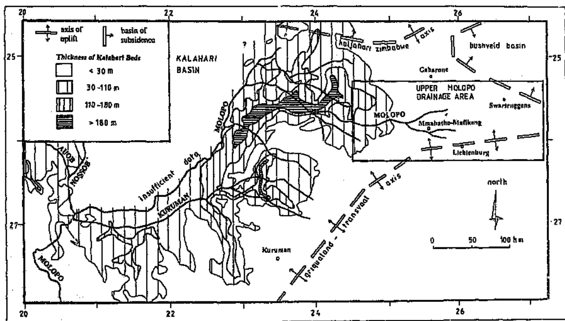
Figure 5.1 Proto-Molopo sedimentary sub-basin and tectonic structures (after Bootsman, 1997). Insert shows upper Molopo drainage area.
