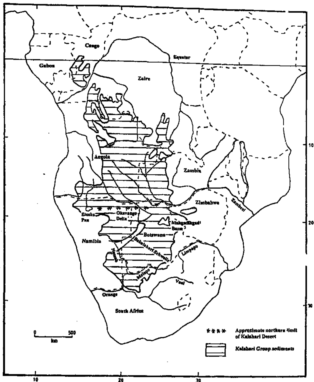
Figure 1.2 The mega-Kalahari, Kalahari Desert, and Bakalahari Schwelle . The shaded area is the mega-Kalahari; the Kalahari Desert corresponds to the part of the mega-Kalahari between the Orange River in the south and the Etosha-Okavango-Zambezi line in the north; the term Southern Kalahari refers to the area of the Kalahari Desert south of the Bakalahari Schwelle . Modified after Thomas and Shaw (1991).
