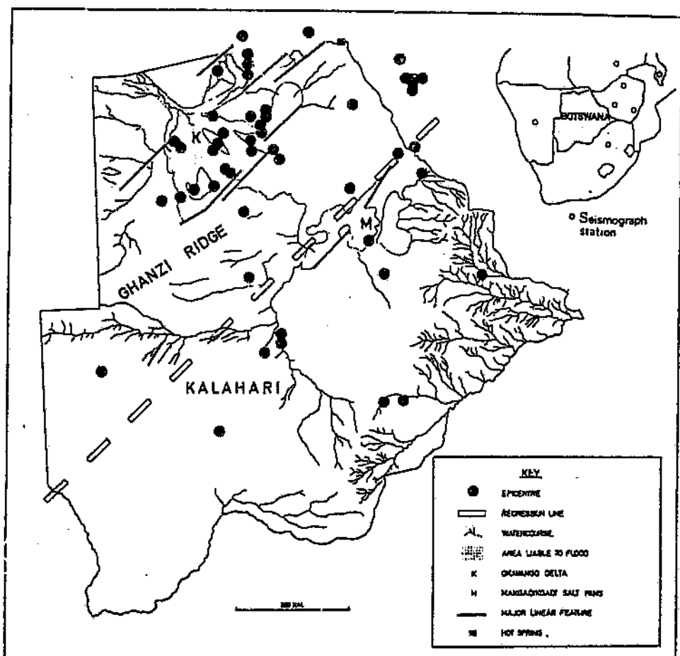
Figure 2.20 Earthquake centres in Botswana, September 1965 to August 1971 (after Reeves, 1973).
