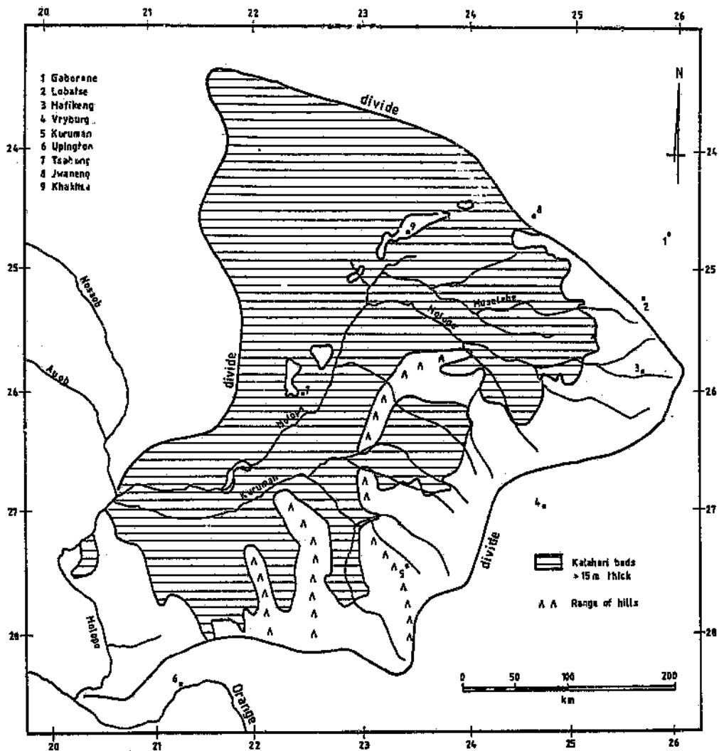
Figure 2.14 Distribution of Kalahari Beds (> 15 m) in the Molopo drainage area.
