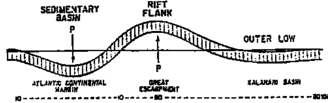
Figure 2.6 Continuous elastic plate model of southern Africa (after ten Brink and Stern, 1992)
