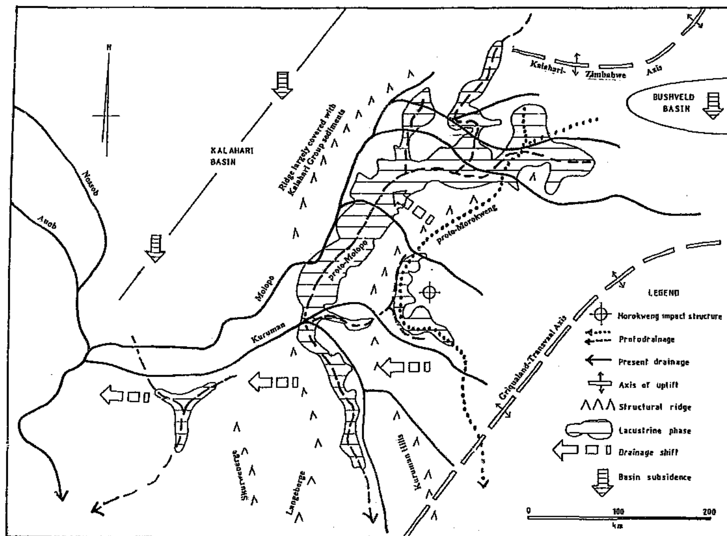
Figure 7.8 Synopsis of Molopo drainage shifts.
