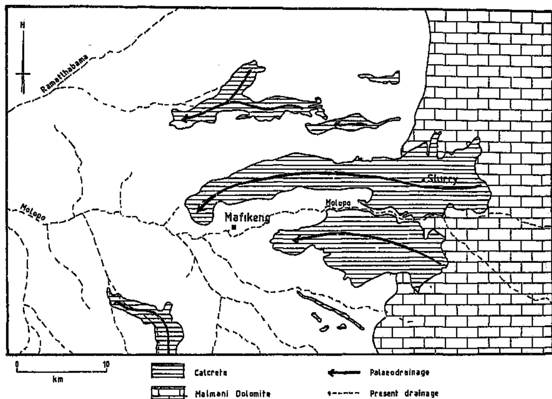
Figure 5.5 Calcrete tongues and palaeodrainage lines around Mafikeng.
