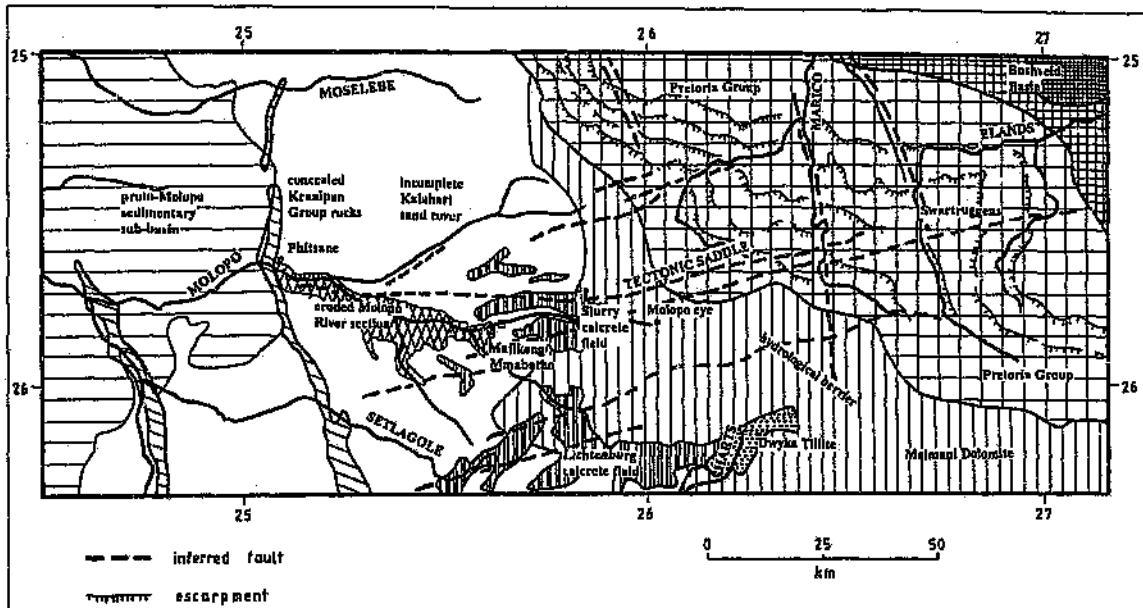
Figure 5.2 The upper Molopo drainage (after Bootsman, 1997).
