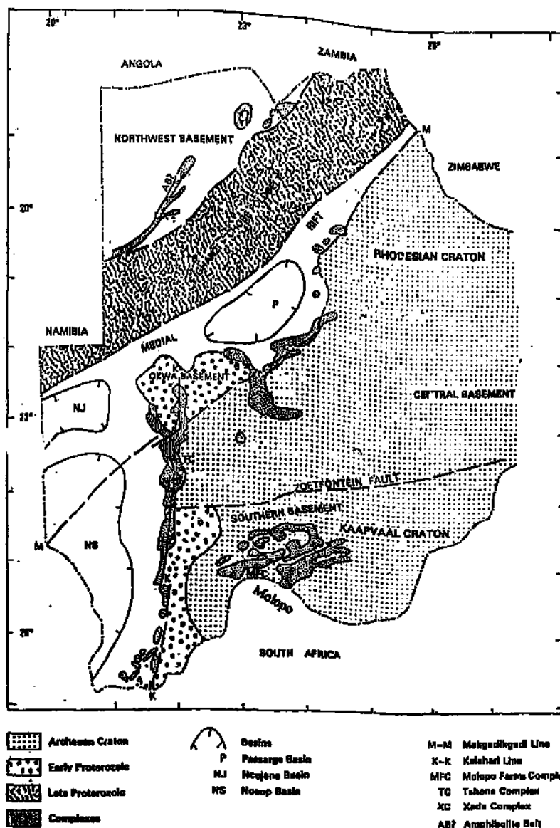
Figure 2.4 Synopsis of basement features in Botswana (after Meixner et al. , 1985).
