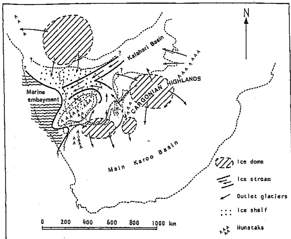
Figure 3.11 The ice extent during the Tses Glaciation (Early Permian) at its maximum and at an advanced stage of disintegration (after Visser, 1983a).
