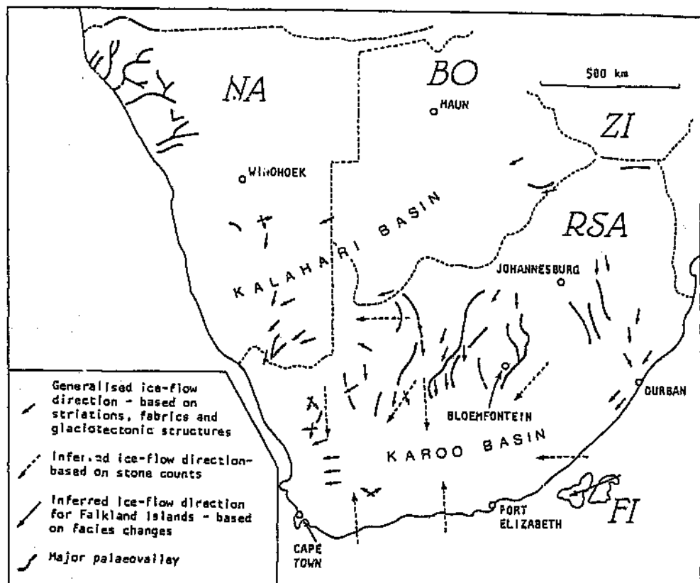
Figure 3.10 Major palaeovalleys in southern Africa (after Visser, 1987).
