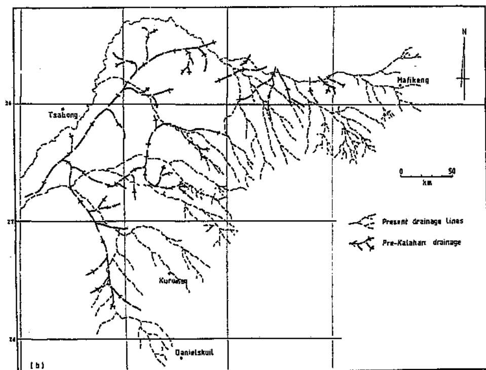
Figure 1.5 Pre-Kalahari surface contours (a) and pre-Kalahari drainage lines (b), after Smit (1977).
