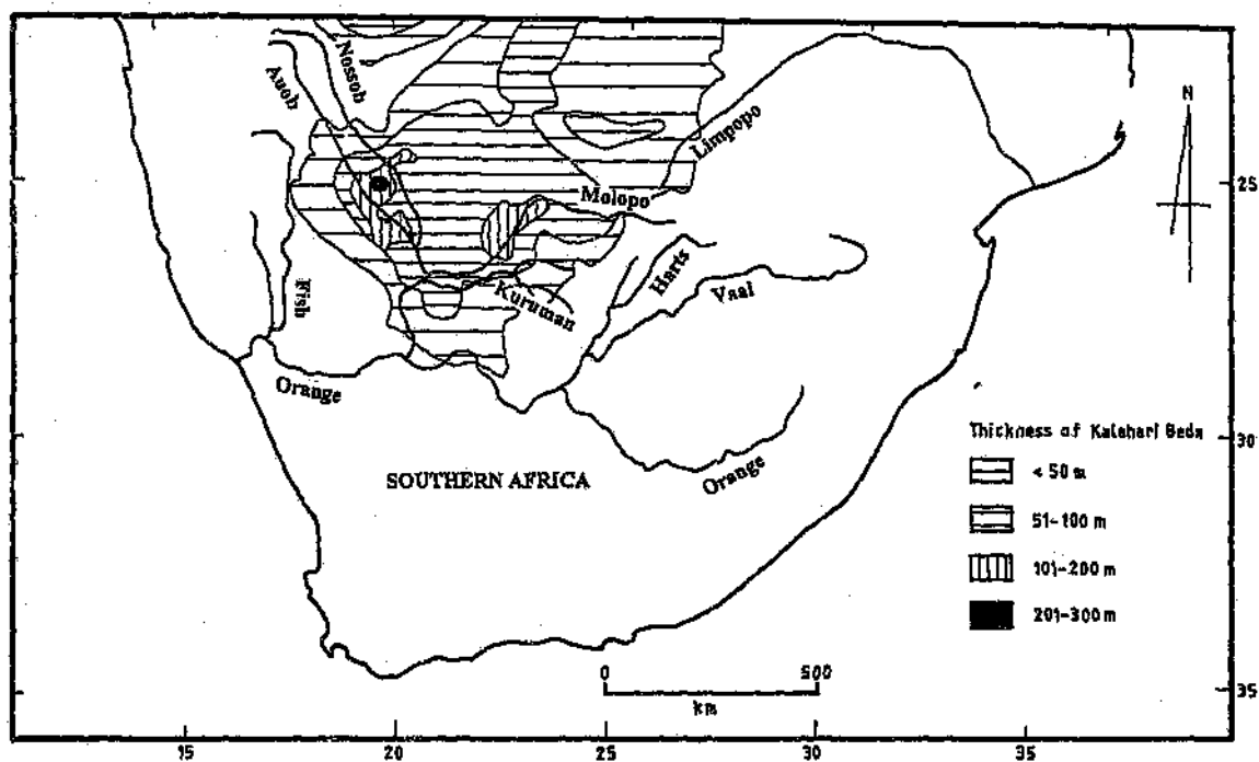
Figure 4.12 Southern Kalahari drainage and thickness of Kalahari Beds.
