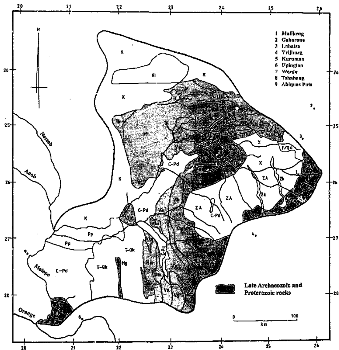
Figure 2.11 Pre-Kalahari geology, emphasising late Archaeozoic and Proterozoic rocks in the Molopo drainage area. See Table 2.1 for the legend.
