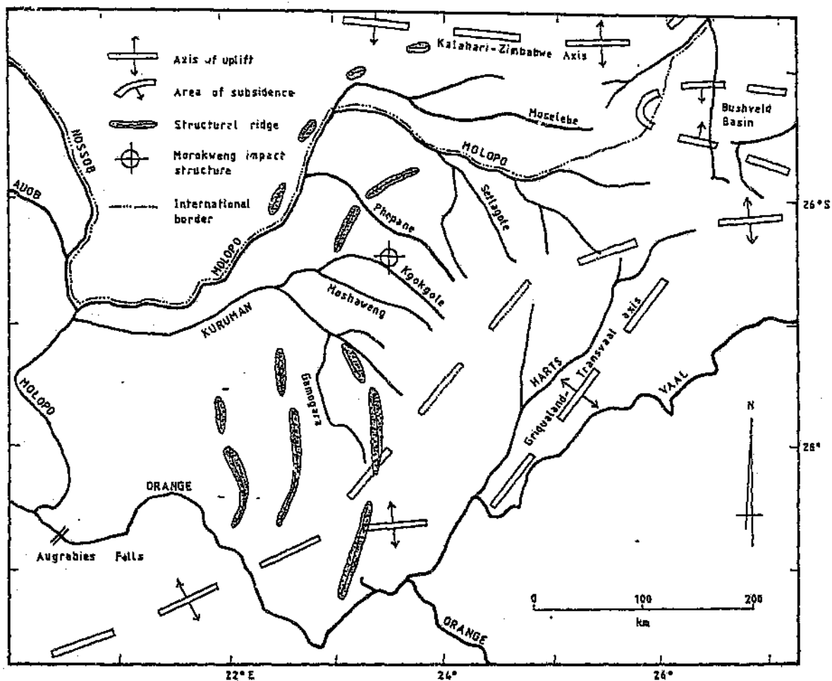
Figure 7.7 Late Tertiary drainage.
