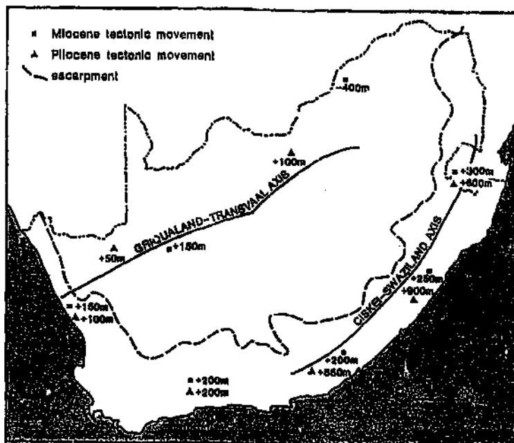
Figure 2.8 Axes of maximum uplift during the Miocene and Pliocene (after Moon and Dardis, 1988).
