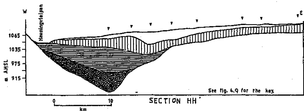
Figure 7.3 Alluvial cross section across a palaeovalley around the Morokweng impact structure near Heuningvlei. This represents the sediment-filled proto-Morokweng valley in Figure 7.2. Based on Smit (1977). See Figure 3.9 for the location of the cross section.
