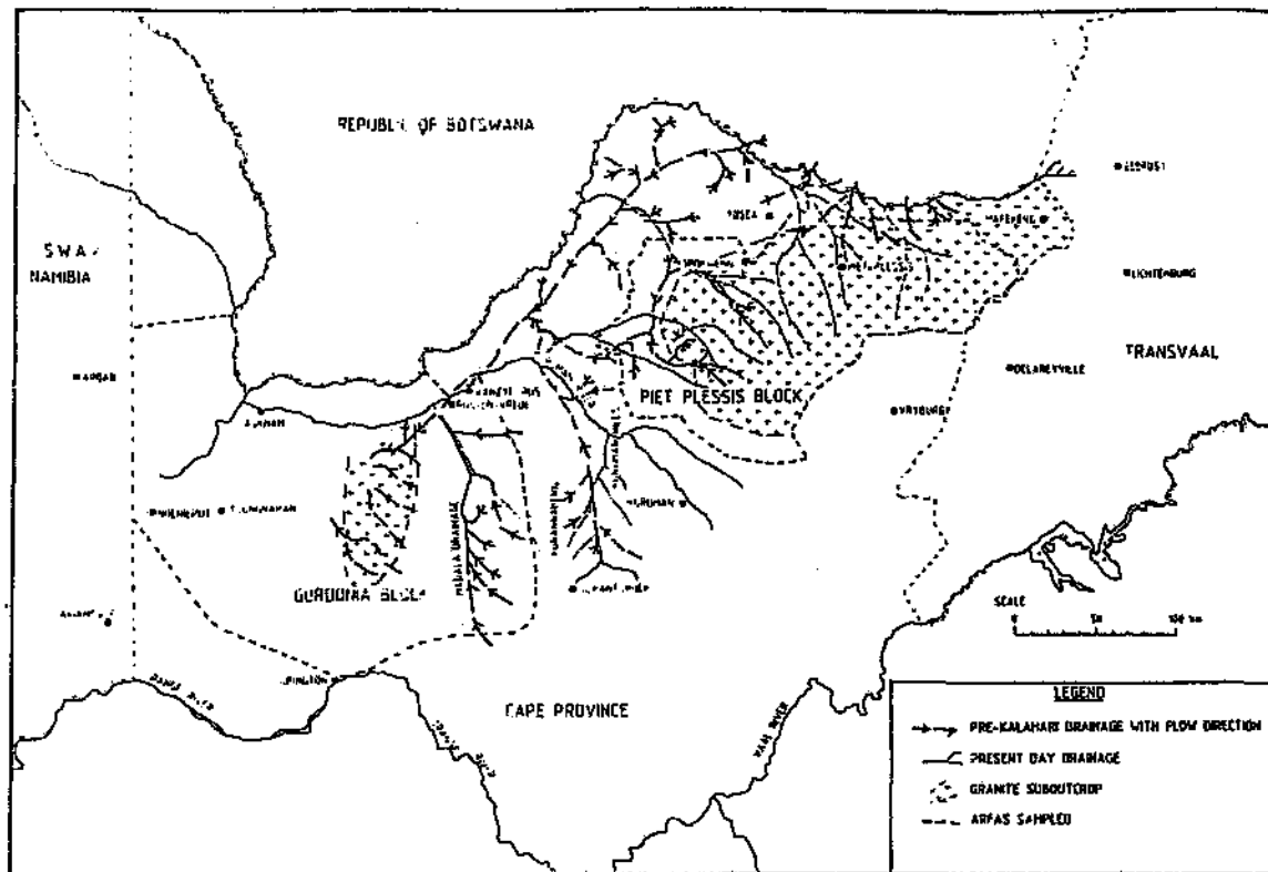
Figure 1.6 Pre-Kalahari drainage in the Molopo drainage according to Levin et al. (1985).
