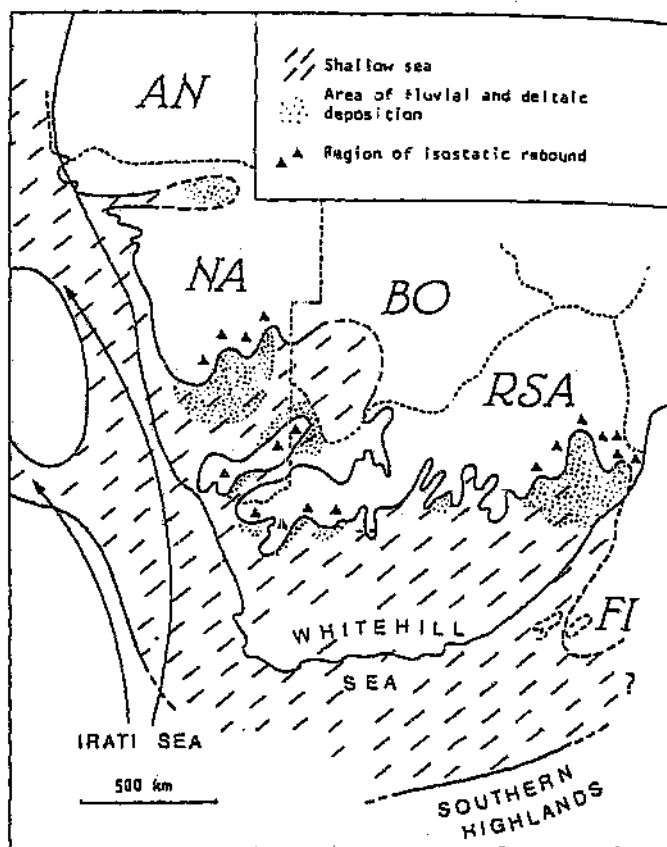
Figure 3.12 Distribution of post-glaciation seas over southern Africa (after Visser, 1987).
