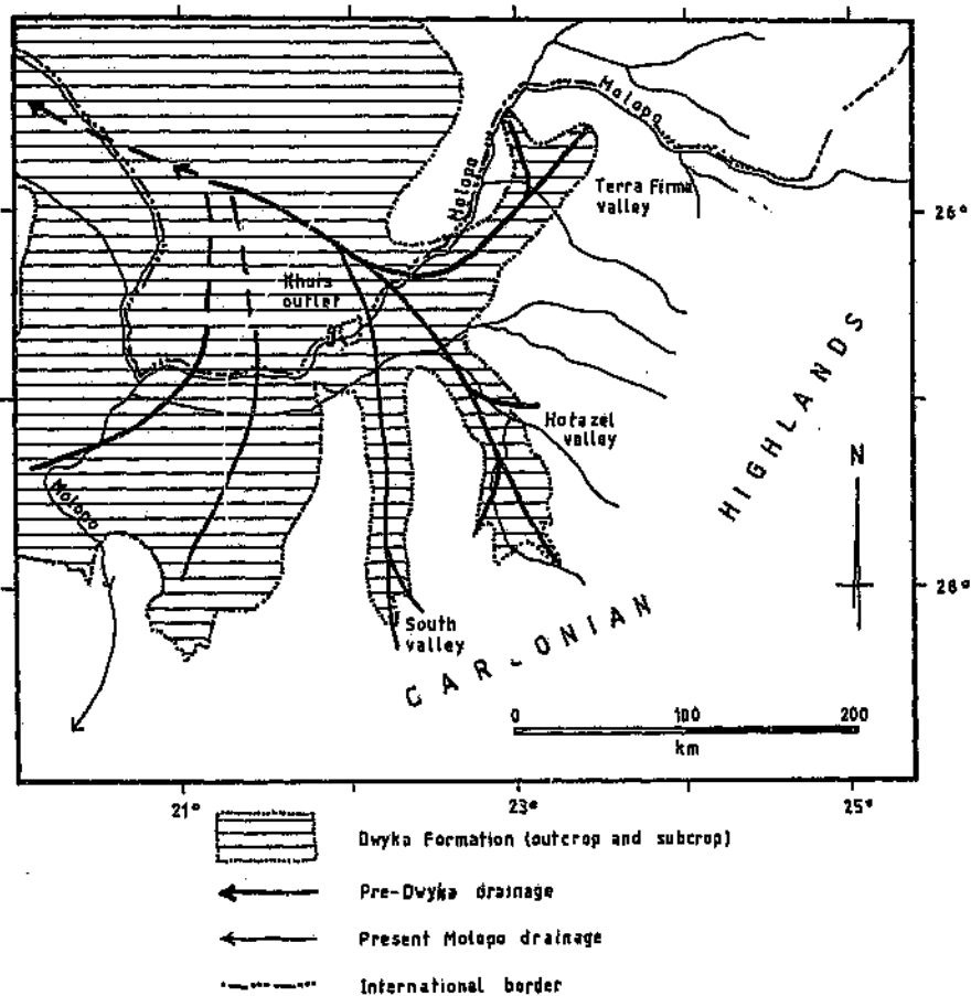
Figure 7.1 Pre-Dwyka palaeodrainage in the Molopo drainage area.
