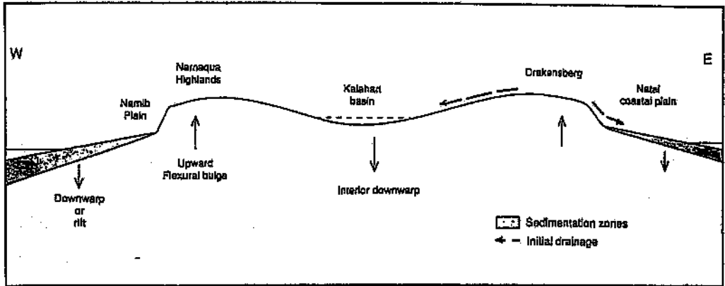
Figure 2.5 Schematic cross section of southern Africa following the splitting of Gondwana (after Thomas and Shaw, 1991).
