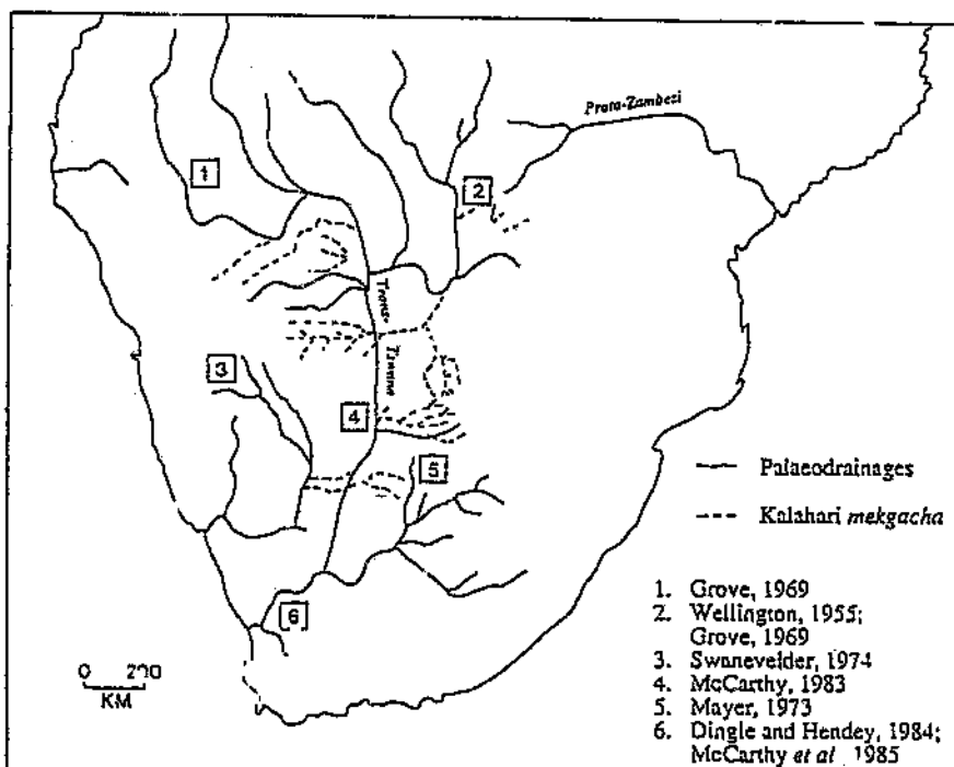
Figure 1.7 The course of the proposed Trans-Tswana palaeodrainage system plus the present courses of major mekgacha, after Dardis et al. (1988) and Nash (1992).
