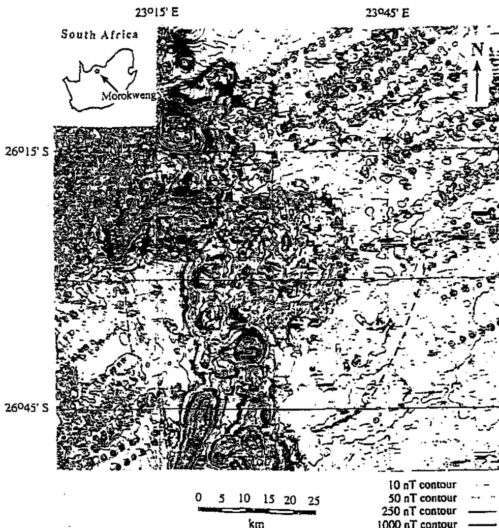
Figure 2.16 Aeromagnetic field across the Morokweng structure (after Hart et al. , 1997). Dashed line denotes the outer margin of the weakly magnetised halo.
