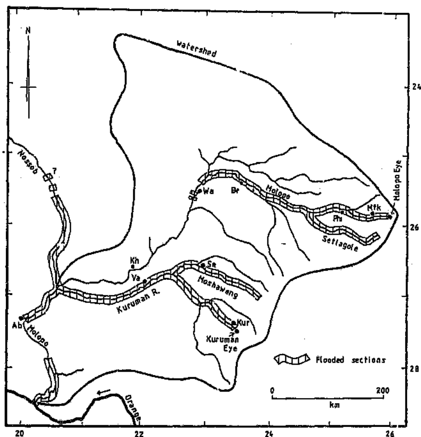
Figure 1.3 Most frequently reported flooded sections of the Molopo drainage in recent historical records. (Ab = Abiquas Put, Br = Bray, Kh = Khuis, Mfk = Mafikeng, Phi = Phitshane, Se = Severn, Va = Vanzijlsrus, Wa = Watersend Farm).
