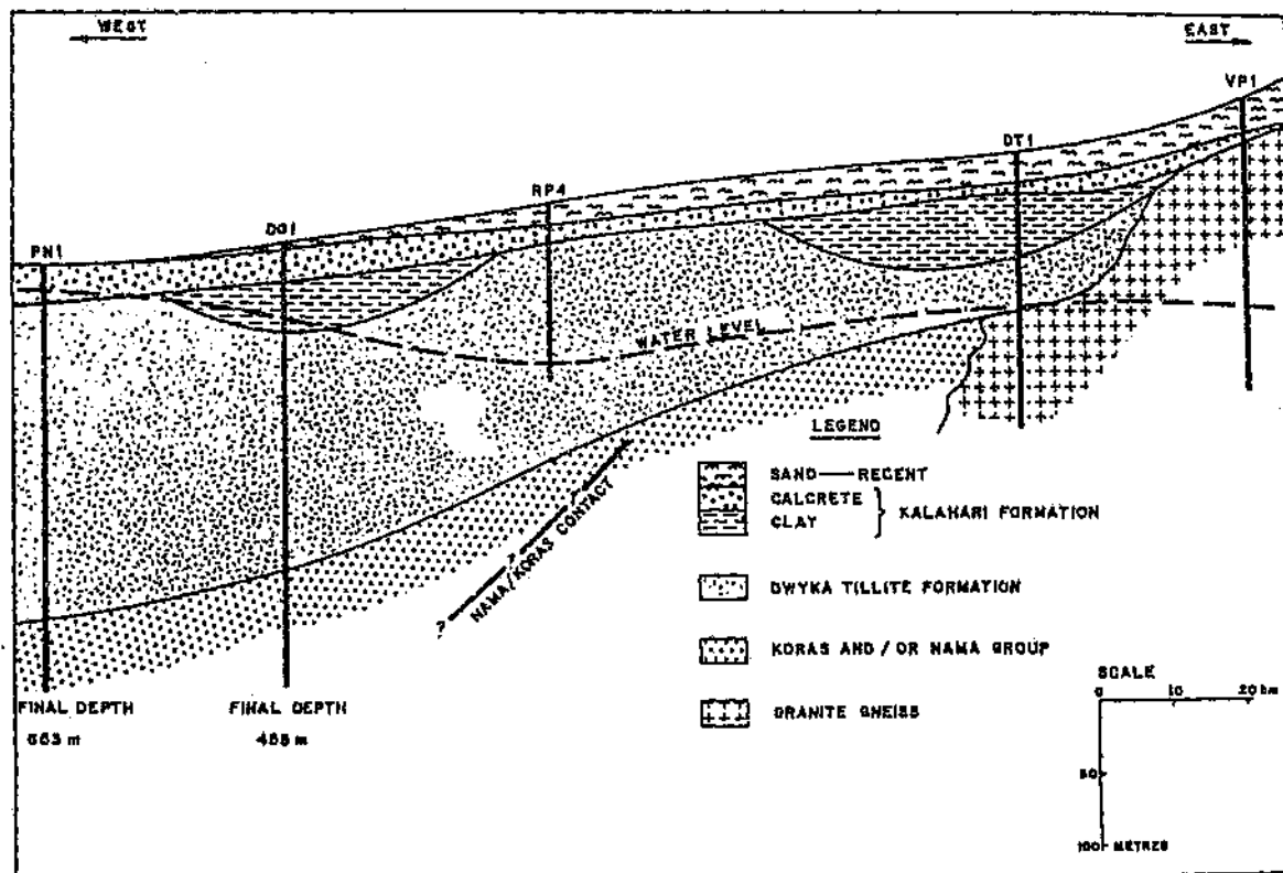
Figure 4.4 East-west geological profile in the area between the Orange and Kuruman Rivers (after Levin, 1980).
