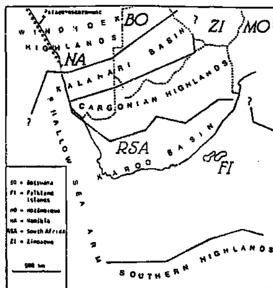
Figure 3.8 Geomorphic elements of part of south-western Gondwana during maximum glaciation (after Visser, 1987).
