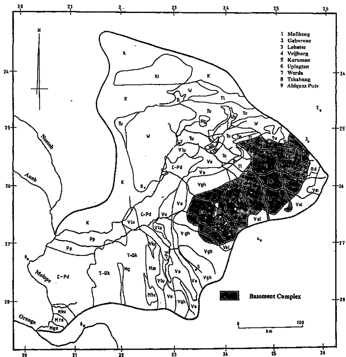
Figure 2.10 Pre-Kalahari geology, emphasising Basement Complex rocks in the Molopo drainage area. See Table 2.1 for the legend.
