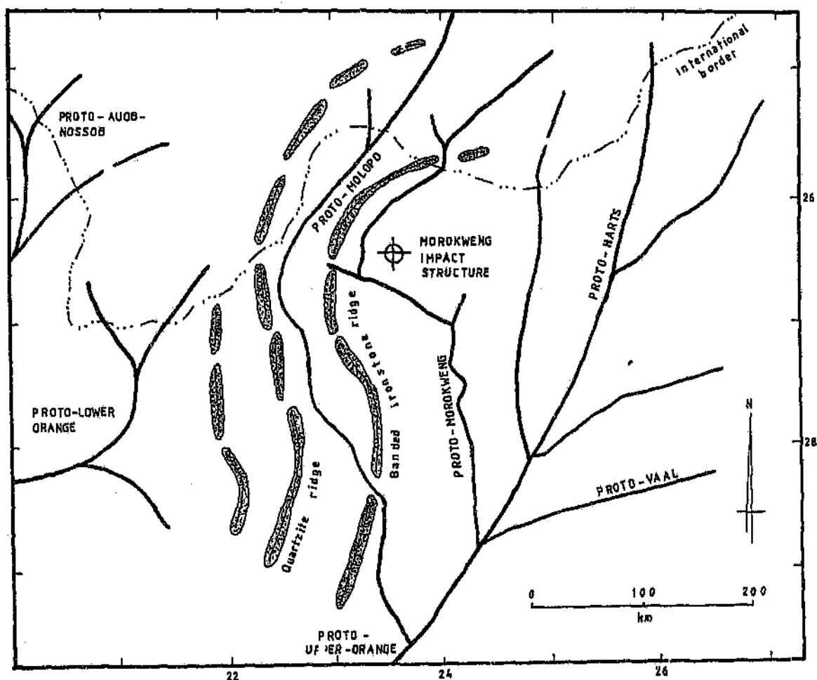
Figure 7.4 Middle to late Cretaceous drainage.
