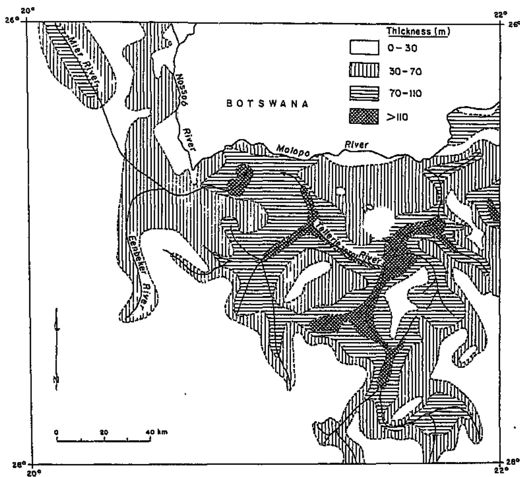
Figure 4.2 Isopach map of the Kalahari Group in Gordonia (after Botha et al. , 1986).
