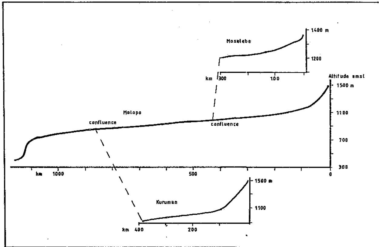
Figure 2. 22 Thalweg profiles of the Molopo, Moselebe, and Kuruman Rivers.
