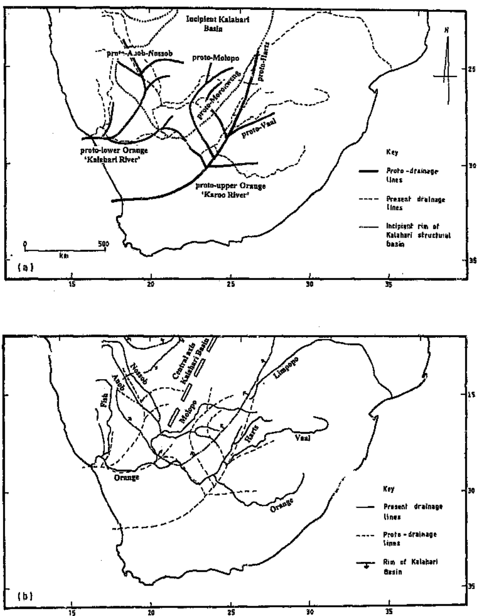
Figure 7.9 Palaeodrainage reconstructions for (a) late Cretaceous and (b) Quaternary. Karoo and Kalahari Rivers based on de Wit (1993).
