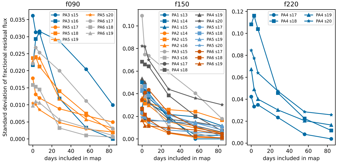
Figure A1. Standard deviation of the fractional residual flux of Uranus for every frequency and array. We bin the Uranus light curve (which has individual observation) into 3-, 7-, 28-, 56-, or 84-d bins and calculate the standard deviation. The standard deviation at zero days included in the map corresponds to the individual observations light curve, before binning.
