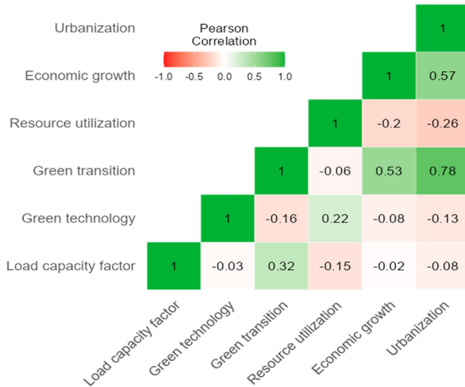
FIGURE 4 | Correlation heatmap.
