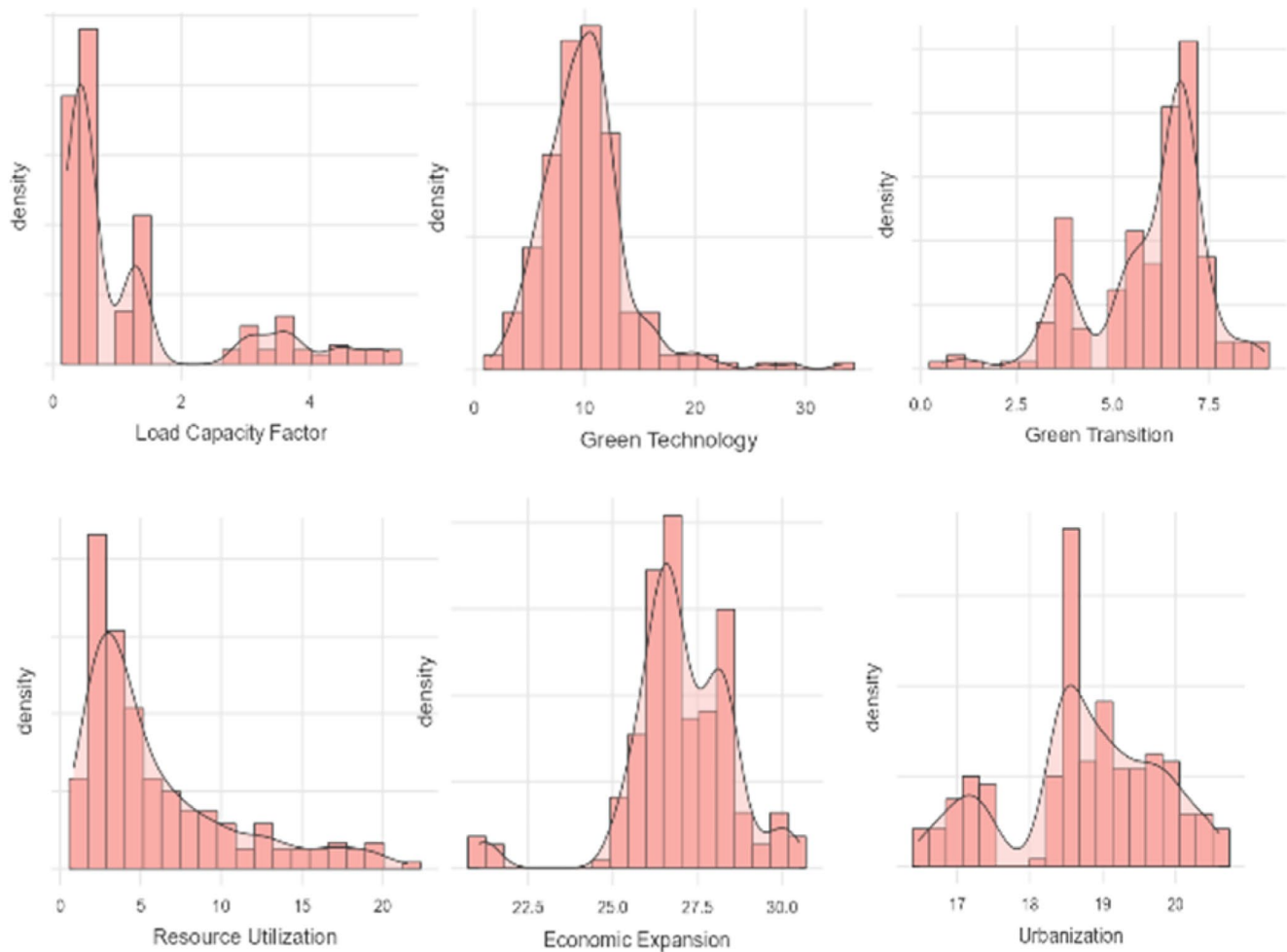
FIGURE 5 | Density plots.
