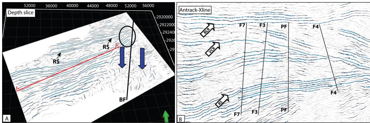
Figure 4.10 Resultant (a) depth slice at 5000 m and (b) antrack crossline (xline) extracted from the antrack volume. The depth slice shows the improved imaging of the Roodepoort shale and enhancement of fractures associated with the Bank Fault. The crossline shows the improved imaging of the Black Reef (BLR), Ventersdorp Contact Reef (VCR) and the Roodepoort shale (RS) horizons. The crossline also shows the improved mapping of faults to shallow depths (VCR and BLR levels).
