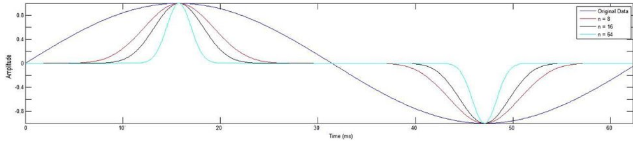
Figure 9 The seismic trace is sharpened by raising the cosine function to the n th power. Note the sharpened peaks as ' n ' value increases. The original data is shown in blue and the results of equation 7 with n = 8, 16 , and 64 are overlain.
