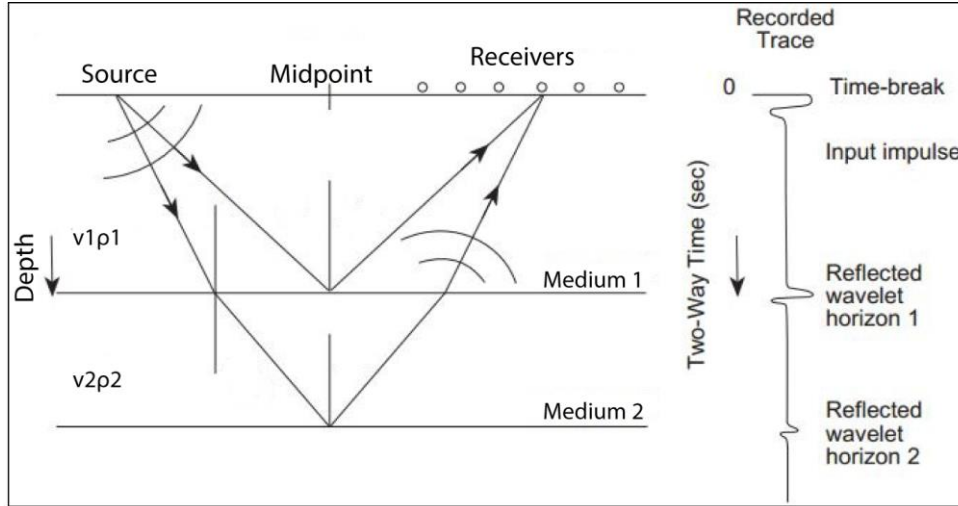
Figure 4.1 Schematic diagram of source-receiver geometry and the signal recorded by receivers. The diagram shows the reflection wave paths over a horizontal interface across which there is an acoustic impedance contrast, where v_2\rho_2 > v_1\rho_1 or v_2\rho_2 < v_1\rho_1 (after Salisbury and Snyder 2007). The two-way travel time increases with depth and v_1\rho_1 and v_2\rho_2 are the velocity and density for medium 1 and medium 2, respectively.
