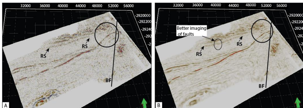
Figure 4.9 Depth slices at 5000 m showing (a) the amplitude display and (b) edge enhancement display.
