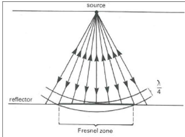
Figure 4.3 Fresnel zone (Kearey and Brooks 1991). The Fresnel zone is the area on a reflector where the energy of the incident ray is returned within a half-wavelength of the central ray. For seismic data with high signal-to-noise ratio the vertical resolution is defined by \lambda/8 and by \lambda/4 for data with low signal-to-noise where \lambda is the dominant wavelength of the data. Therefore, the wavelength is essentially the measure of the seismic resolution.
