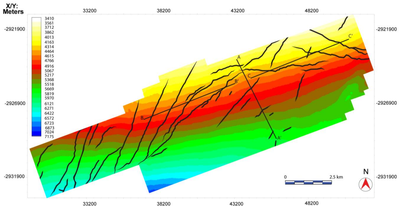
Fig. 6 Depth structural map of the Roodepoort shale derived from conventional picking. The map shows faults striking in various directions and the location of inline and crossline sections discussed in the main text.
