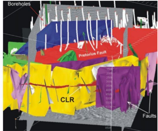
Figure 17 3D structural model of the Carbon Leader Reef model incorporating boreholes and faults.
