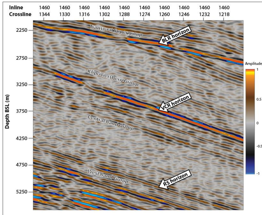
Figure 4.2 Seismic section (amplitude display) across the Mponeng gold mine showing the imaging of the reflective interface between the dolomites of the Transvaal Supergroup and the ultra-mafic to mafic lavas of the Klipriviersberg Group, which coincides with the Black Reef (BLR) horizon; the reflective interface of the Klipriviersberg lavas and the quartzites of the Central Rand Group, which coincides with the Ventersdorp Contact Reef (VCR) horizon; and the reflective boundary of the quartzites of the Central Rand Group and the chloritoid-rich shales of the West Rand Group, which coincides with the Roodepoort shale (RS) horizon.
