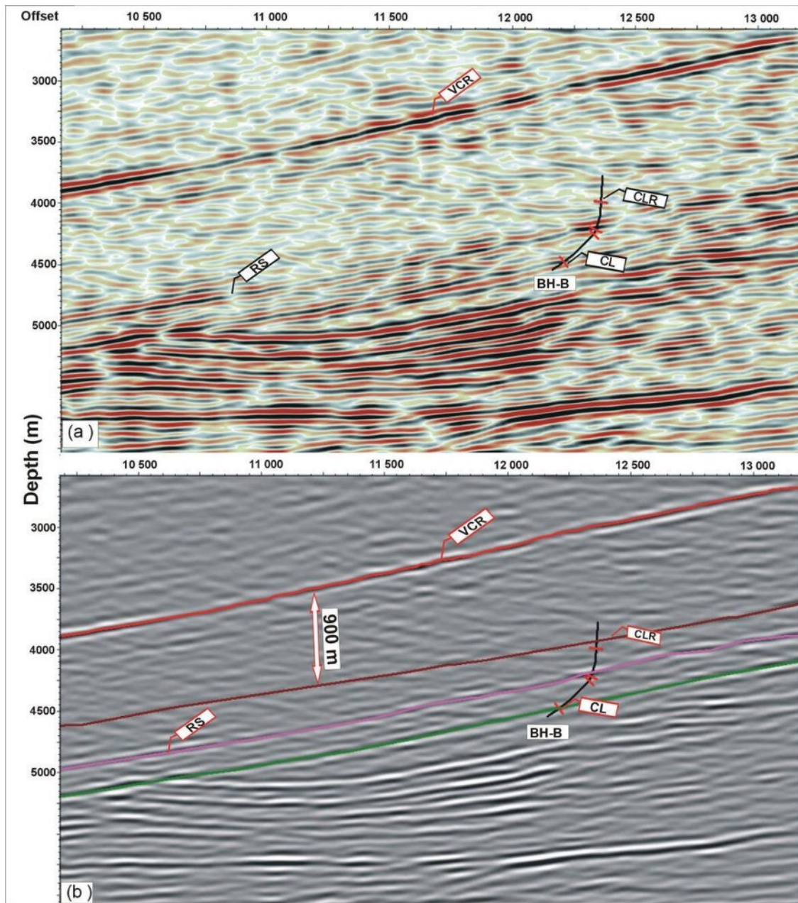
Figure 12 (a) Un-interpreted seismic section showing a good tie between seismic reflectors and the borehole. (b) Interpreted seismic section showing the derived CLR. RS: Roodepoort Shale, CL: Crown Lava.
