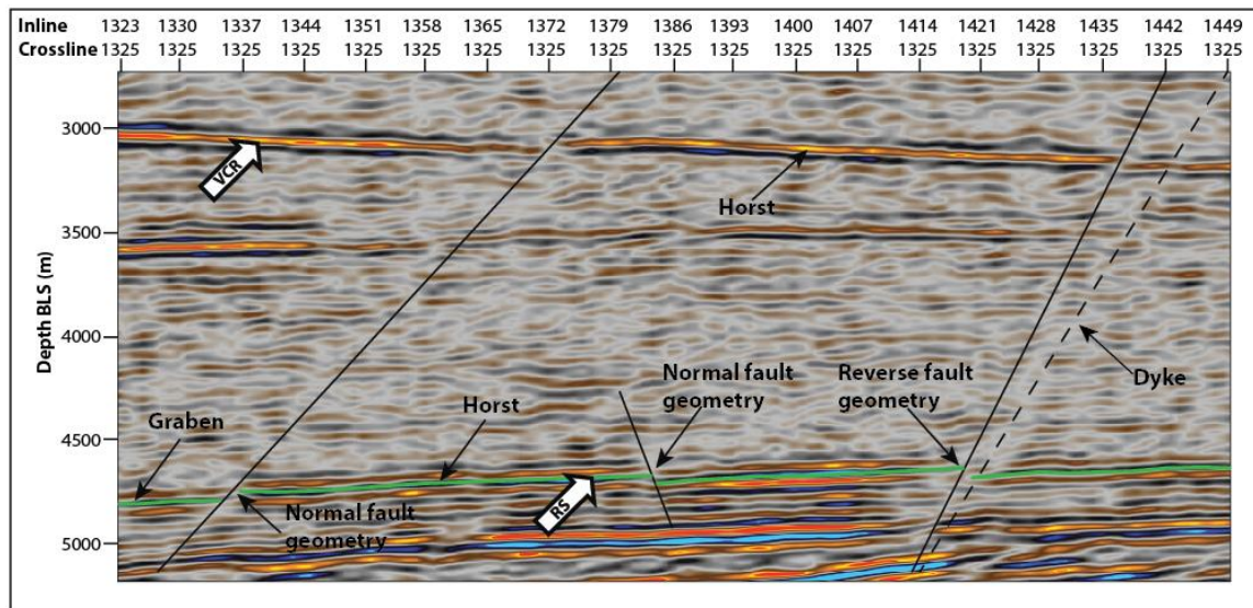
Figure 4.8 Amplitude display seismic section showing various types of faults across the survey areas. These faults crosscut the Roodepoort shale (RS) horizon at the top of the West Rand Group as well as the Ventersdorp Contact Reef (VCR) at the base of the Ventersdorp Supergroup. The seismic section also shows near vertical features (dykes) associated with highly attenuated seismic amplitudes.
