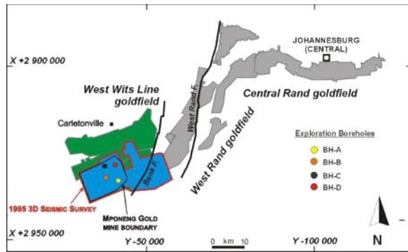
Figure 2 The location map showing the 3D seismic survey covering Mponeng Gold mine within the West Wits Line goldfields (modified after Dankert and Hein 2010).
