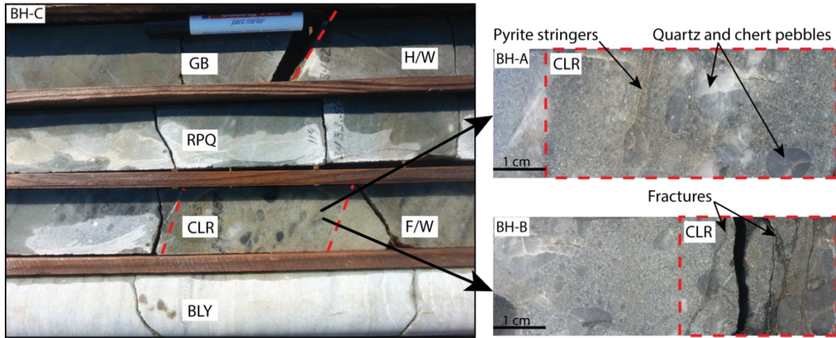
Figure 5 Borehole drill-core showing the CLR conglomerate and its hangingwall (Green Bar shale and Rice Pebble Quartzite) and footwall (Blyvooruitzicht Quartzite) lithostratigraphic units. Note that boreholes BH-A and BH-B show the poor development of the Carbon Leader Reef (CLR) conglomerate. GB: Green Bar shale, H/W: Hangingwall, RPQ: Rice Pebble Quartzite, CLR: Carbon Leader Reef, F/W: Footwall, BLY: Blyvooruitzicht Quartzite.
