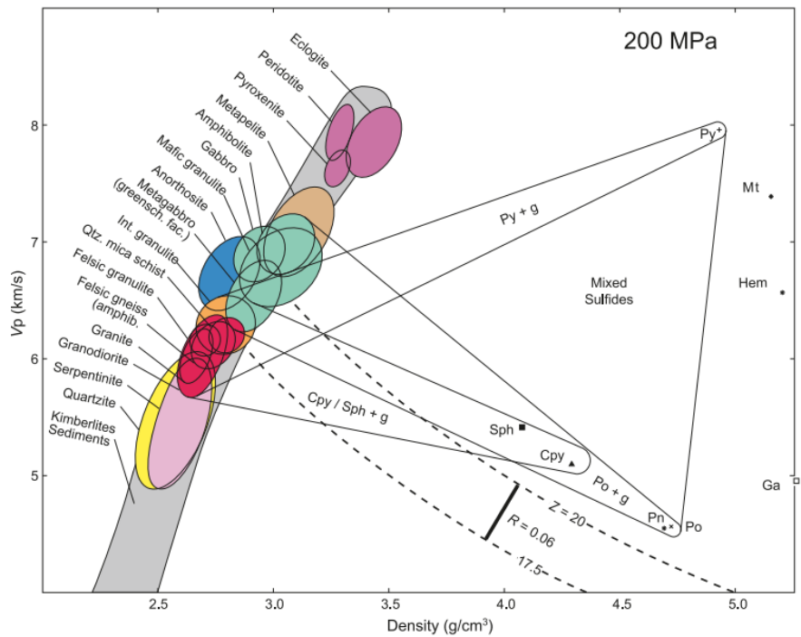
Figure 3.3 Nafe-Drake curve is a plot of compressional wave velocity ( V_p ) versus density for silicate rocks and sulphide ores. From the diagram it can be seen that quartzites usually have seismic velocities in the range of ~5 - 5.5 km/s and densities of ~2.5 g/cm 3 - 2.7 g/cm 3 (after Salisbury and Snyder 2007).
