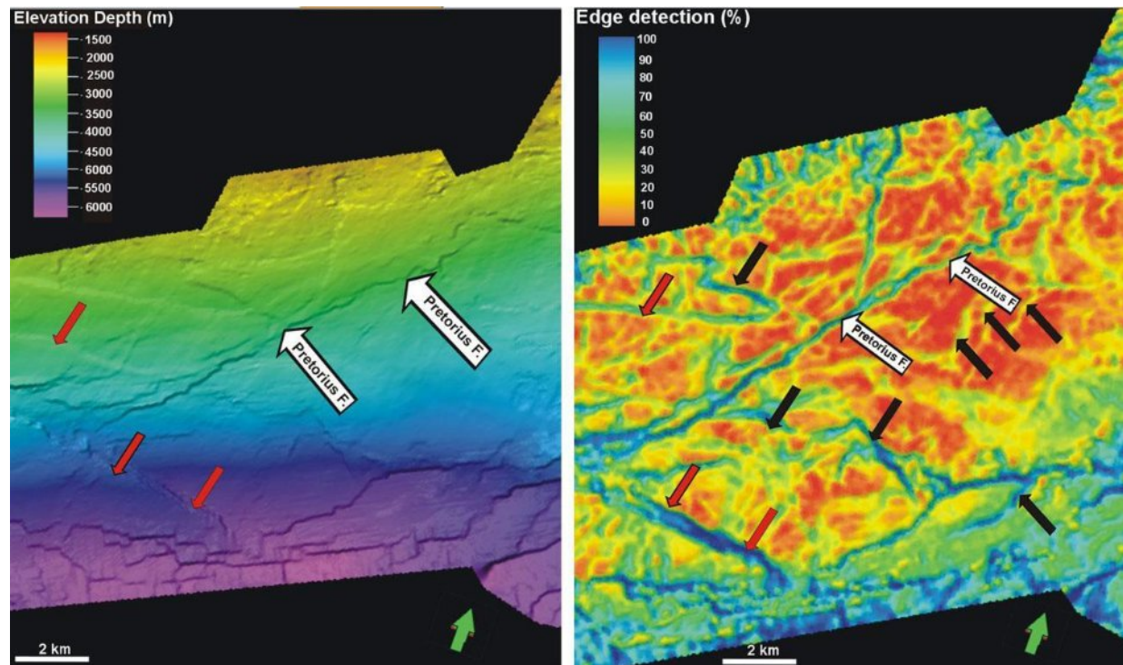
Figure 15 (a) Seismically imaged faults by smoothed conventional interpretation (picking). (b) High-resolution imaging of subtle features (faults and dykes, see black arrows) by an edge detection technique.
