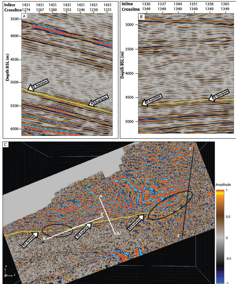
Figure 4.4 Conventional amplitude display seismic sections showing the correlation of the Roodepoort shale (RS) picks on the vertical sections represented by the (a) inline section and (b) crossline section and on the horizontal section represented by (c) the depth slice. The solid yellow lines represent areas where the confidence in picking was high due to the strong and continuous reflection of the horizon. The dashed yellow lines that are highlighted by the black circles in (c) show areas of structural complexity and low confidence in picking. Line A-A' and B-B' show the location of inline and crossline sections, respectively. F: Fault.
