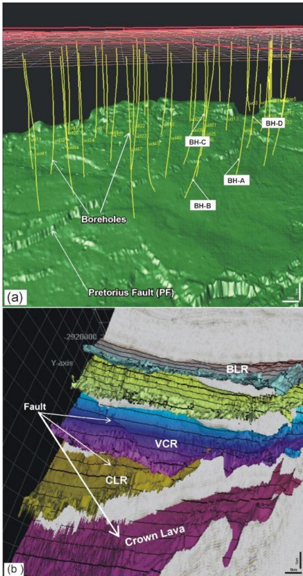
Figure 13 (a) CLR ore body integrated with exploration boreholes that intercept the CLR and the VCR. (b) 3D visualization of the interpreted seismic horizons used to derive the CLR horizon.
