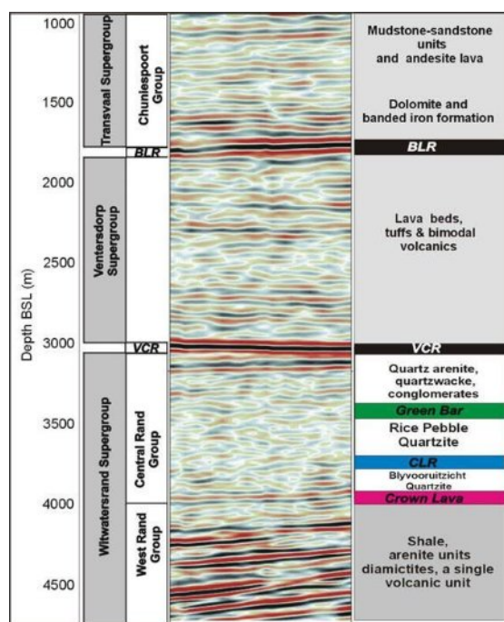
Figure 4 The summary of the stratigraphy of the West Wits Line goldfields (modified after Frimmel et al. 2005).
