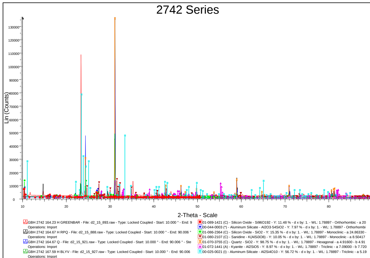
Figure 1: A stacked plot of the phase identification for the borehole GBH 2742 samples: 164.23 H GREENBAR, 164.67 H RPQ, 164.67 Q and 167.59 H BLYV. Phases are included at the bottom of the diagram. H: Heavy minerals; Q: Quartz.
