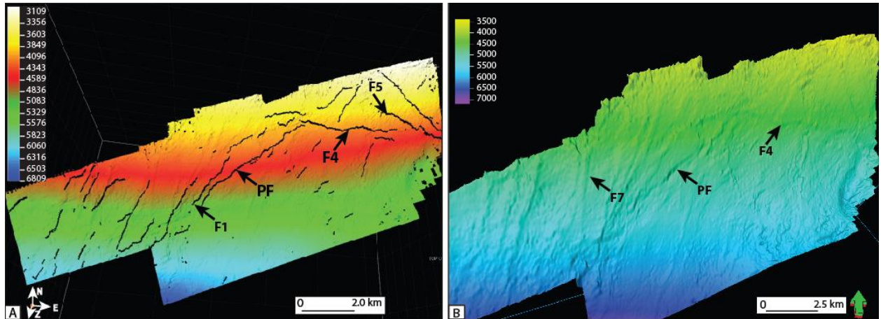
Figure 4.11 Roodepoort shale surface obtained from (a) conventional picking and (b) smoothed Roodepoort shale surface. The application of the smoothing operators has reduced the noise and spikes in the data.
