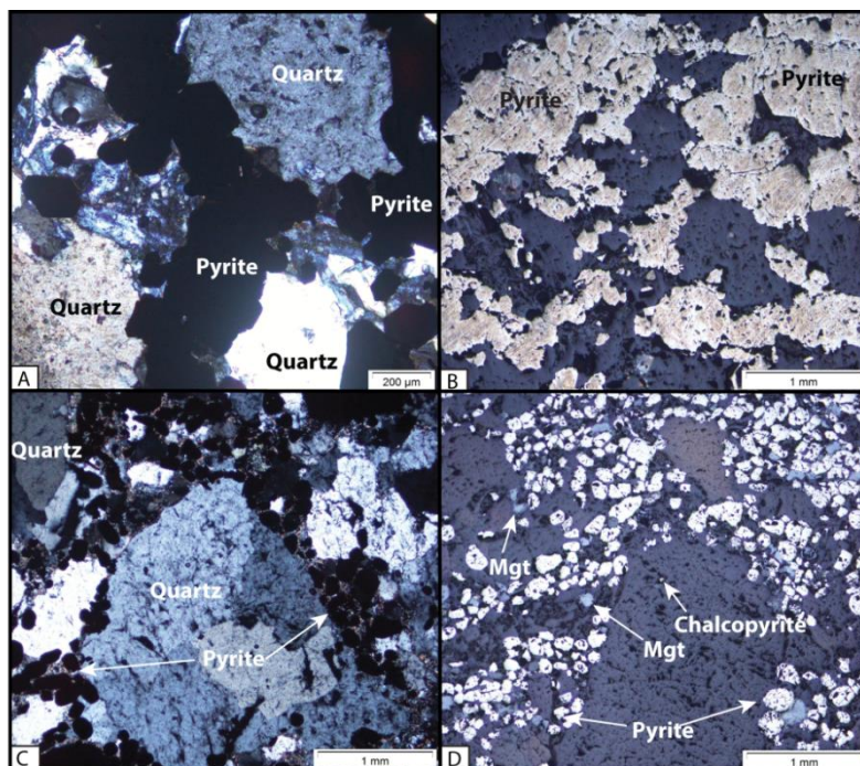
Figure 8 Thin sections and polished blocks of the Rice Pebble Quartzite and Carbon Leader Reef conglomerate from photo microscopy analysis. A and C show views of the thin sections in reflected light and B and D shows the polished blocks in reflected light.
