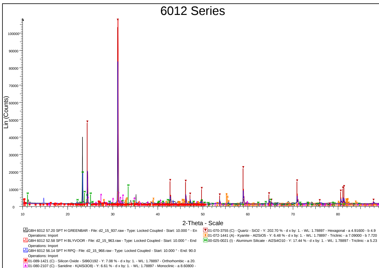
Figure 4: A stacked plot of the phase identification of the 6012 samples: 57.20 H GREENBAR, 52.58 SPT H BLYV and 56.14 H RPQ. Phases are included at the bottom of the diagram. H: Heavy minerals; Q: Quartz.
