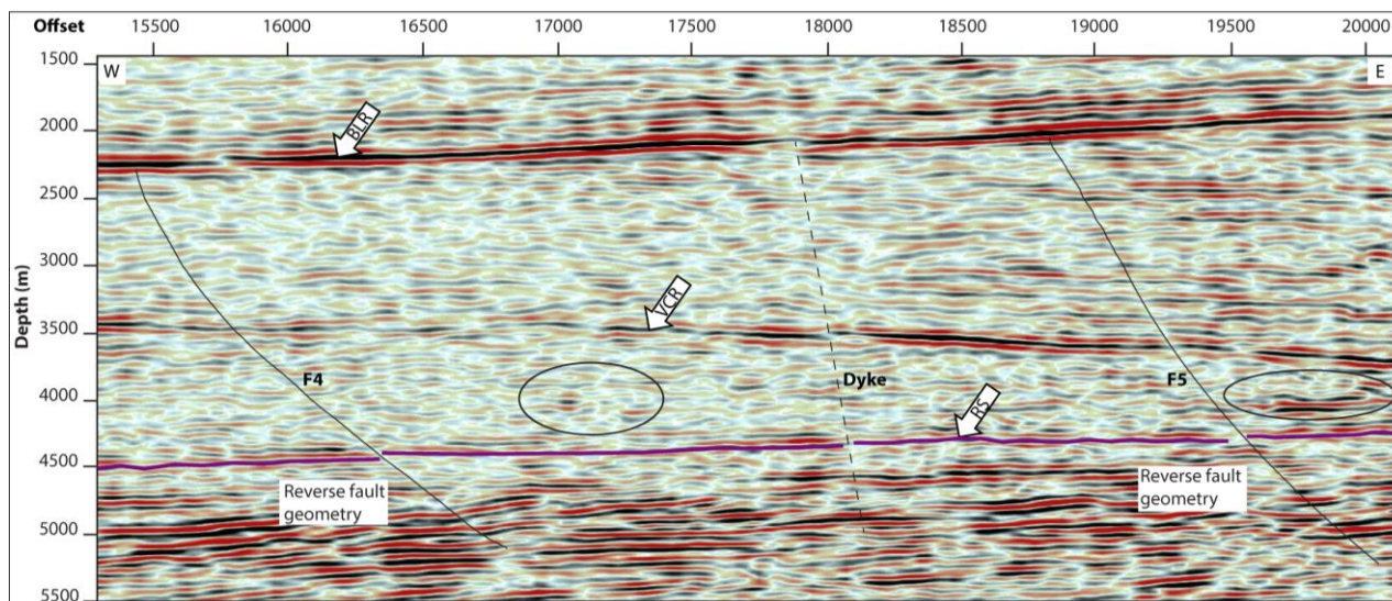
Fig. 8 Amplitude display seismic section (line C'-C'') showing the easterly dipping Fault 4 (F4) and Fault 5 (F5) cross-cutting the Roodepoort shale (RS) horizon at the top of the West Rand Group. The solid black lines highlight faults and the dotted lines show location of dykes in the stratigraphy. The circles encompass high amplitude areas that do not correspond to any horizon. Due to the low signal-to-noise of the amplitude display it is difficult to track faults and dykes up stratigraphy to the Ventersdorp Contact Reef (VCR) and the Black Reef (BLR) levels.
