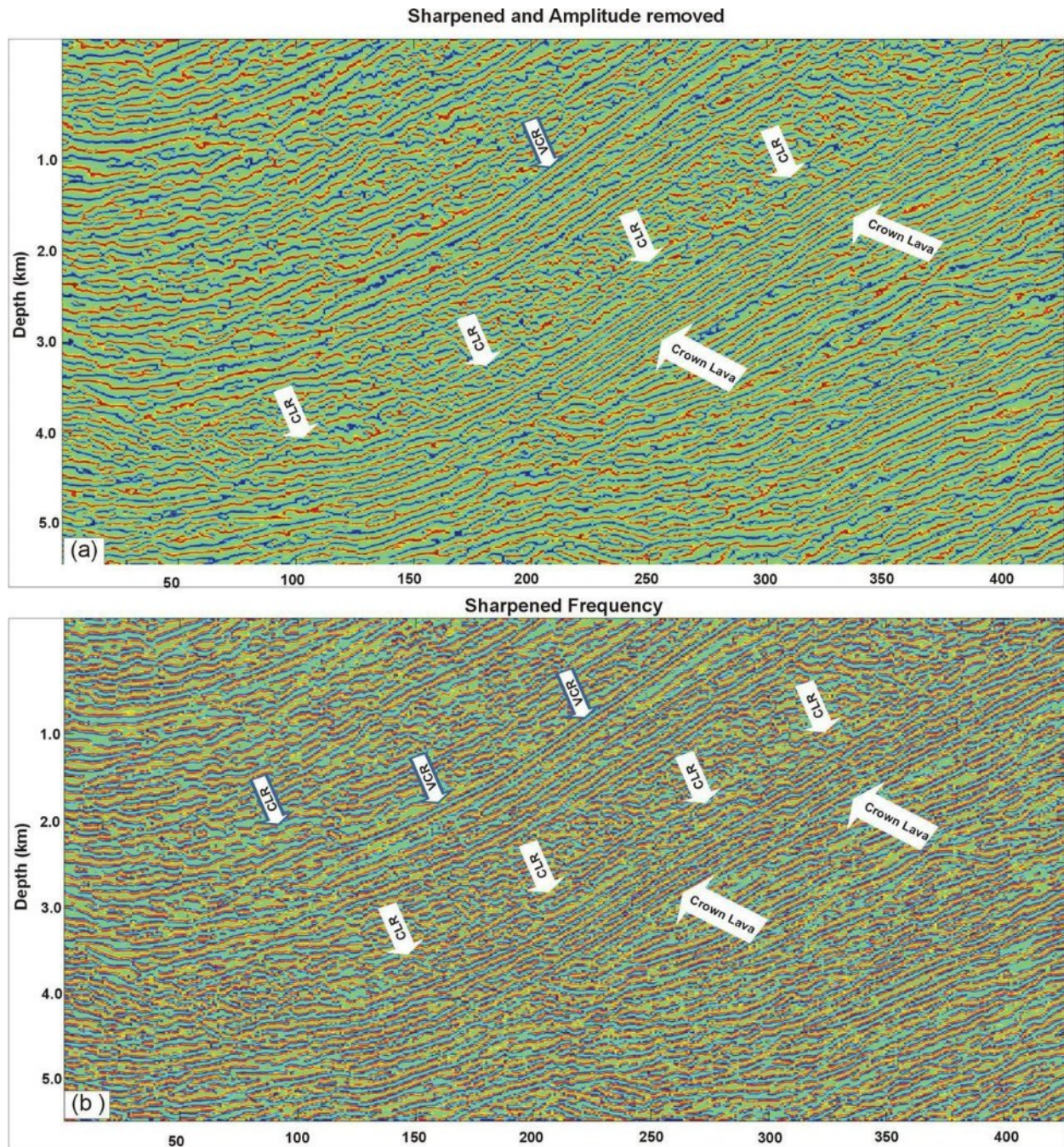
Figure 11 (a) Sharpened Instantaneous phase attribute shows a much improved enhancement of the CLR detection and its lateral continuity. (b) Identification of low amplitude events through the sharpened instantaneous frequency.
