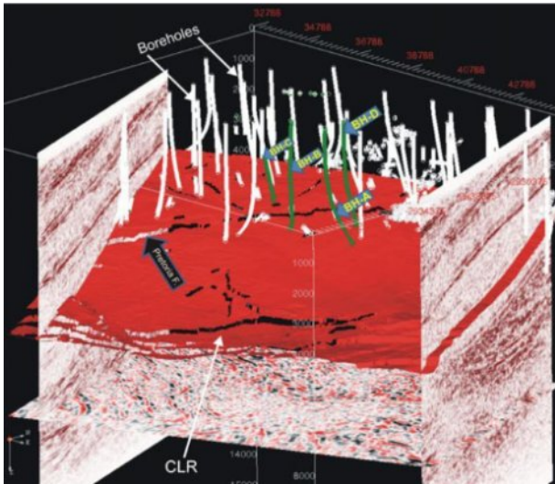
Figure 16 3D visualization of the 3D seismic data integrated with boreholes. The boreholes in green were used for physical property measurements.
