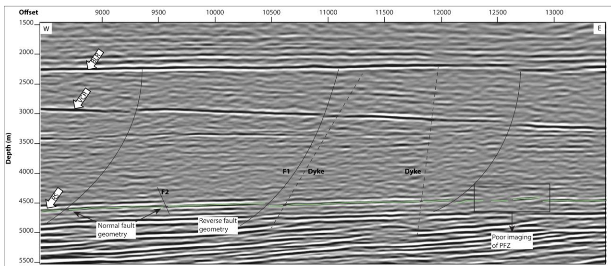
Fig. 7 Amplitude display seismic section (line B'-B'') showing the Pretorius Fault (PF), Fault 1 (F1), Fault 2 (F2) and Fault 3 (F3) cross-cutting the Roodepoort shale (RS) at the top of the West Rand Group. The solid lines indicate various faults while the dashed lines indicate dykes cross-cutting the stratigraphy. The oval shape highlights an area of high amplitude and the square shape encompasses a zone of the poorly imaged Pretorius Fault Zone (PFZ). Due to the low signal-to-noise of the amplitude display it is difficult to track faults and dykes up stratigraphy to the Ventersdorp Contact Reef (VCR) and the Black Reef (BLR) levels.
