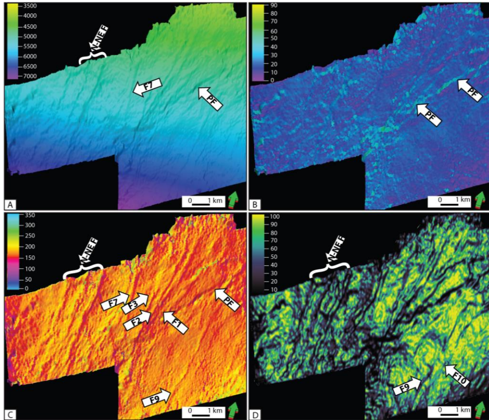
Fig. 12 Seismic attributes computed for the top of the West Rand horizon (block A). (a) The top of the West Rand smoothed surface (colour bar represents depth in metres). (b) Dip attribute display, showing the extent of the Pretorius Fault (PF) (colour bar given in degrees). (c) Azimuth attribute display, showing the enhancement of various faults on the western side of the RS surface (colour bar given in degrees). (d) The edge detection attribute display, clearly enhancing the north-northeast trending fault set and the north-south trending Fault 9 and Fault 10 ( (colour bar given in percentages). The north-northeast trending fault set consists of more than 3 faults: north-northeast Fault-set (N-NE F-set), Pretorius Fault (PF), Fault 1 (F1), Fault 2 (F2), Fault 3 (F3), Fault 7 (F7), Fault 9 (F9) and Fault 10 (F10).
