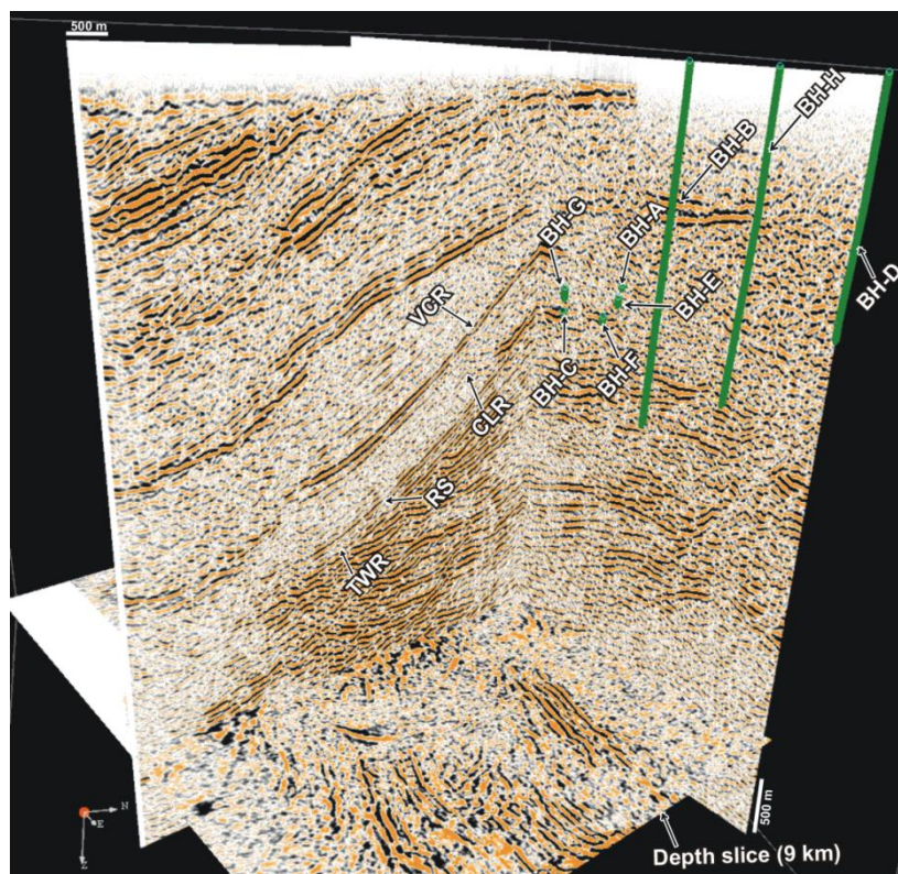
Figure 4 3D visualization of the migrated seismic volume (see 3D seismic block Fig. 2) covering Anglo Gold Ashanti Ltd and Sibanye Gold Ltd mines along the West Wits Line Goldfields, showing strong seismic reflectors and location of boreholes (BH-A to BH-H). VCR: Ventersdorp Contact Reef, TWR: Top of the West Rand, RS: Roodepoort shale, CLR: Carbon Leader Reef.
