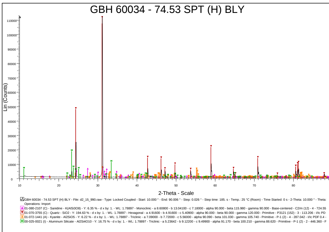
Figure 7: A plot of the phase identification sample 74.53 H BLY . Phases are included at the bottom of the diagram. H: Heavy minerals; Q: Quartz.
