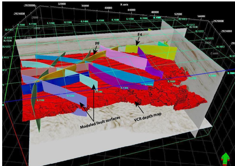
Fig. 14 3D structural model of the mining area incorporating the VCR ore body, second-order scale Pretorius Fault (PF) and subordinate faults.
