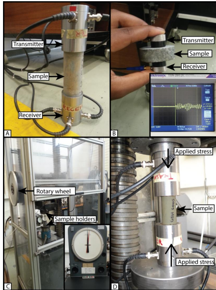
Figure 5.4 Ultrasonic velocity measurement apparatus at ambient (a and b) and elevated stresses (c and d). (a) Larger transducer (diameter=32 mm, 0.5 MHz) set used to measure seismic velocities for large samples (b) smaller transducer (diameter=16 mm, 0.5 MHz) set used to measure seismic velocities for smaller samples. (c) The uniaxial compressional loading is produced by hydraulic pistons that are driven by a computer controlled load holding pump. The induced load is monitored on a stress measuring gauge (insert in c). (d) The image shows the placement of the sample between the transducers positioned on pistons within the chamber.
