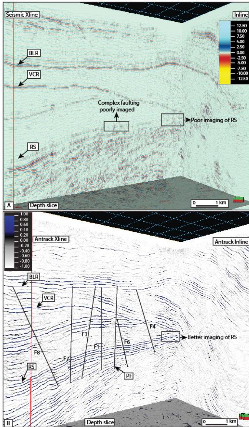
Fig. 9 Seismic inline, crossline (Xline) and depth slice showing the (a) regional continuity of the Black Reef (BLR), Ventersdorp Contact Reef (VCR) and Roodepoort shale (RS) before ant-tracking attribute is applied and (b) after the application of the ant-tracking algorithm. Note that the amount of noise in the data has been considerably attenuated resulting in the better imaging of the various seismic reflectors and the enhancement of faults in the antrack volume.
