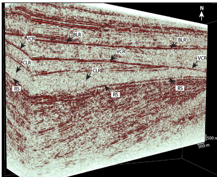
Fig. 4 Extent of the seismic volume along the West Wits Line showing strong seismic imaging of the Black Reef (BLR), Ventersdorp Contact Reef (VCR) and Roodepoort shale (RS) and the poor imaging of the Carbon Leader Reef (CLR).
