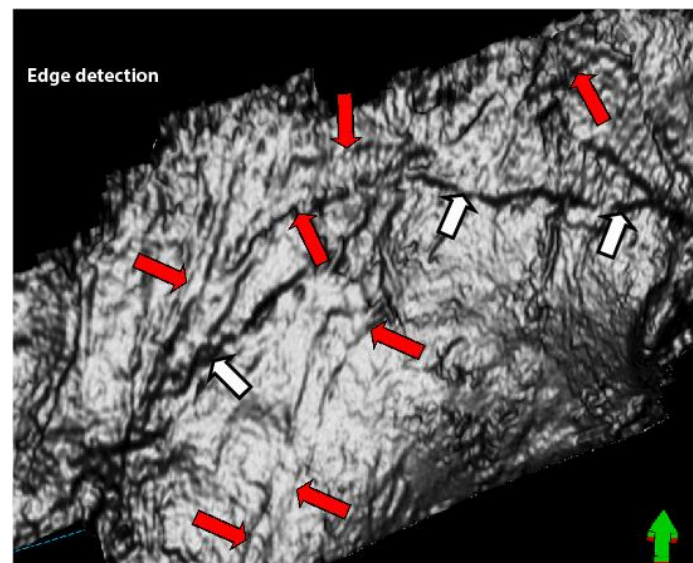
Figure 4.14 Roodepoort shale edge detection attribute map. The white arrows show faults which were clearly mapped by the dip and dip-azimuth maps in figure 14.11a and b and the red arrows show newly enhanced faults, which were not mapped by the dip-amplitude and dip-azimuth displays.
