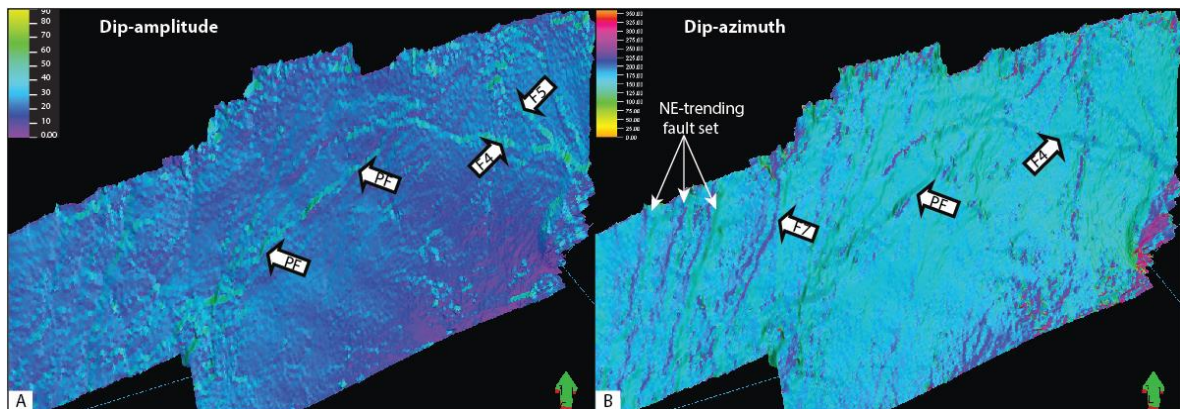
Figure 4.13 Seismic attributes computed for the Roodepoort shale horizon. (a) Dip attribute display, showing the clear mapping of the Pretorius Fault (PF) and the Fault (F4) and Fault 5 (F5) (colour bar given in degrees). (b) Dip-azimuth display, showing the extent of the PF, Fault 7 (F7) and Fault 4 (F4) (colour bar is given in degrees). The dip-azimuth map also shows the extent of some NE-trending faults on the western margin of the map.
