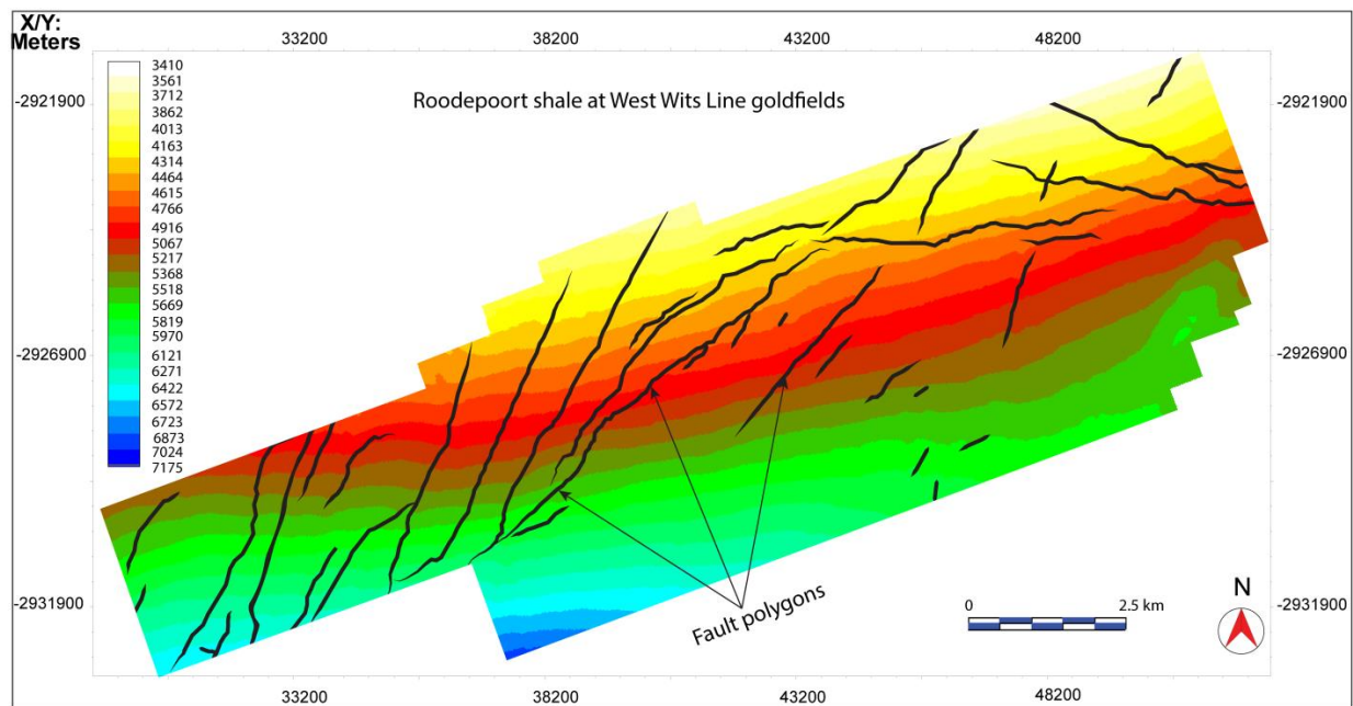
Figure 4.5 Depth structure map of the Roodepoort shale derived from manual picking. The map shows faults of various orientations that crosscut the horizon.
