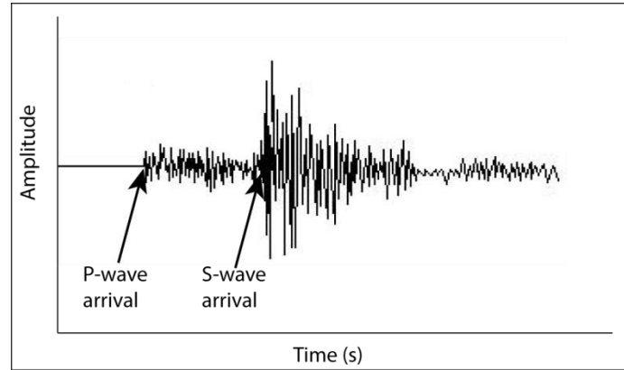
Figure 3.2 Hypothetical example of the arrival of P- and S-waves at a seismic station. The P-waves are the first waves to arrive and the next sets of waves are the S-waves which have a larger amplitude than the P-waves (after Mussett and Khan 2000).
