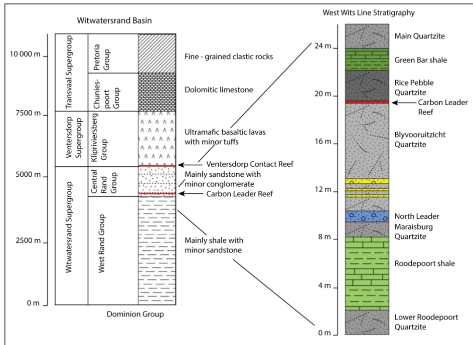
Figure 3 Generalized stratigraphic column of the Witwatersrand Basin and the West Wits Line Goldfield with particular emphasis on the CLR conglomerate and the Roodepoort shale stratigraphy (after Guy et al. 2010).
