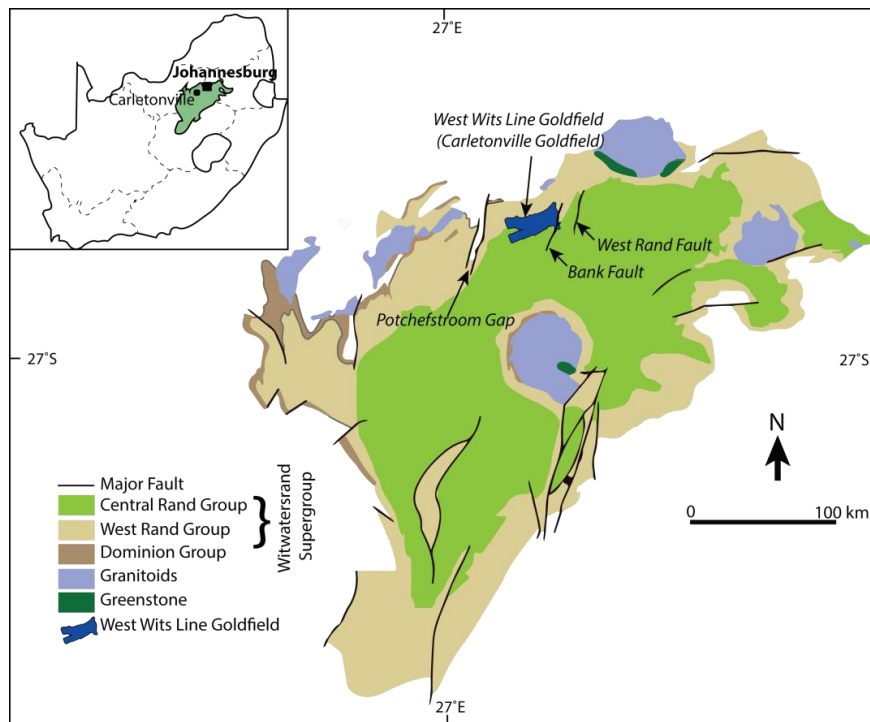
Figure 1 A simplified geological map of the Witwatersrand Basin with older sediment cover, showing the location of the West Wits Line Goldfield (Carletonville Goldfield) (after Grové and Harris 2010).
