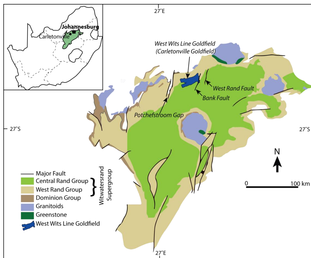
Figure 0.1 A simplified geological map of the Witwatersrand Basin showing the location of the West Wits Line goldfield (Carletonville goldfield) as well as the locations of major faults (after Grové and Harris 2010).
