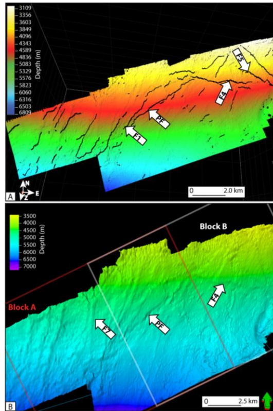
Fig. 11 Top of the West Rand surfaces obtained from (a) conventional picking and (b) smoothed top of the West Rand surface. The red square represents the boundary for Block A and the white square represents the boundary for Block B.
