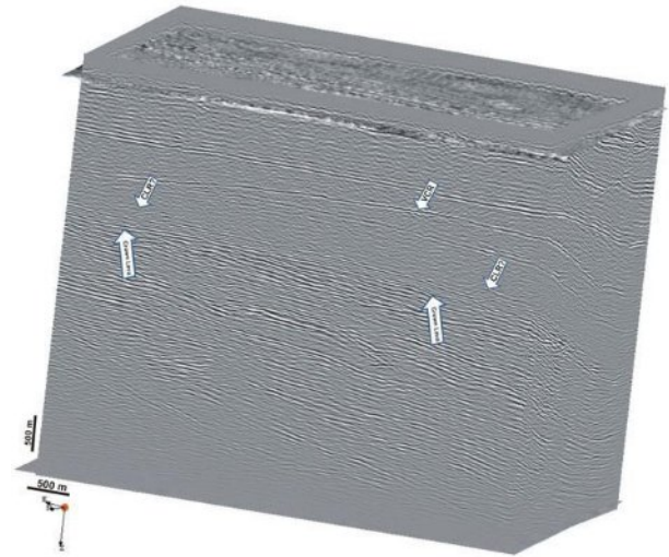
Figure 8 Seismic cube showing poor imaging of the CLR and good imaging of the VCR and Crown Lava (see Figs 1 and 2 for the location of the survey).
