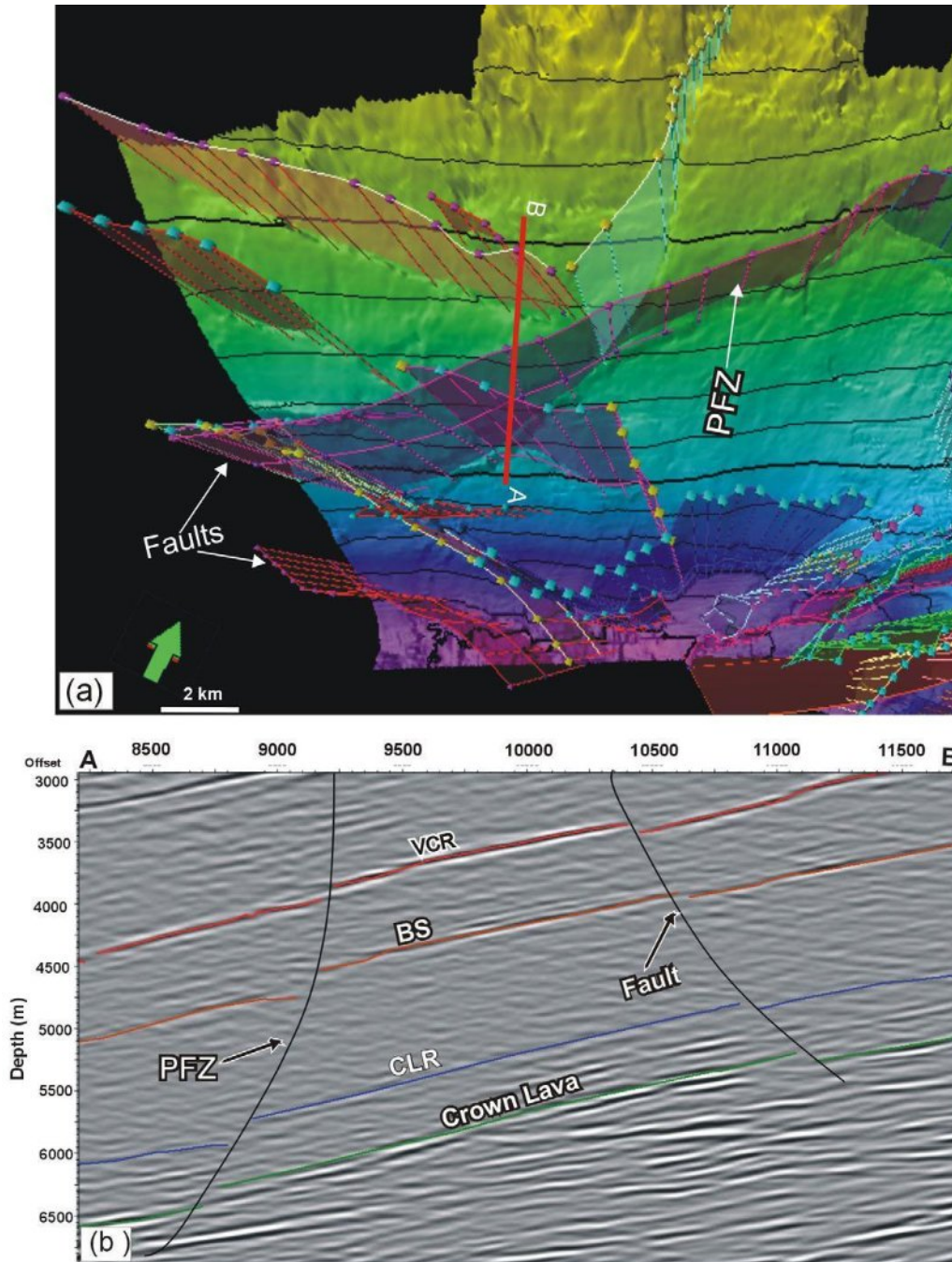
Figure 14 (a) CLR horizon-fault framework defined from the depth structure map. The model shows the stable faulted blocks, bifurcation of faults from a single plane into two branches and cross-cutting relationship between faults. (b) Seismic imaging of the major Pretorius Fault Zone (PFZ). BS: Booyens Shale.
