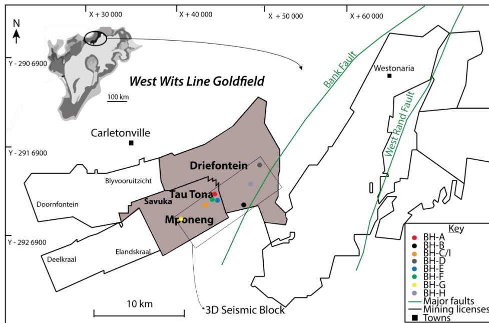
Figure 2 The map showing the location of 9 boreholes within the Anglo Gold Ashanti Ltd and Sibanye Gold Ltd mining boarders, along the West Wits Line Goldfield. Note that all the 9 boreholes lie within the 3D seismic block covering the two mines. Note that boreholes BH-C and BH-I are deflections (after Dankert and Hein 2010).
