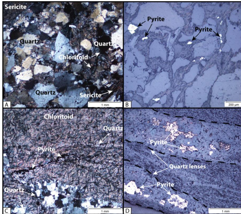
Figure 7 Thin section of the hangingwall Main Quartzite in (a) cross polarized and (b) reflected light, and the Green Bar shale in (c) cross polarized and (b) reflected light. Sulphides occur within the groundmass in the Main Quartzite (b) and the sulphides in the Green Bar shale (d) occur within the quartzite lenses.
