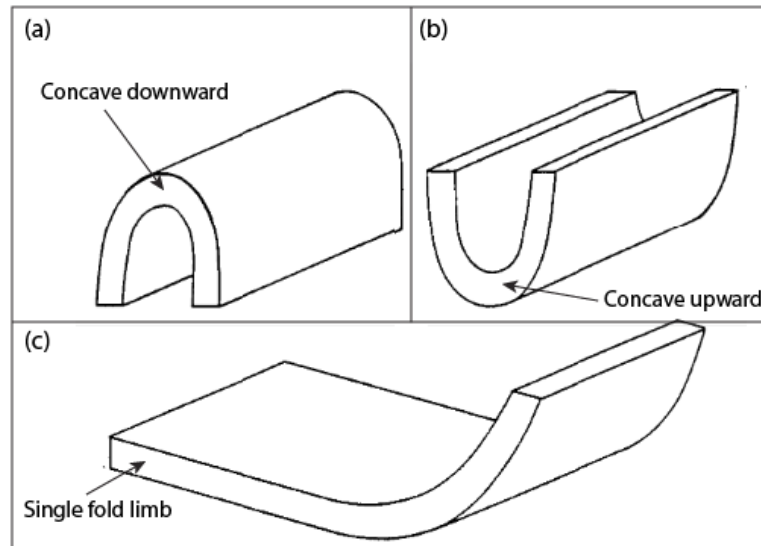
Figure 4.6 Schematic diagrams of basic fold structures. (a) Symmetrical anticline; (b) symmetrical syncline; (c) monocline. The anticline and syncline are characterized by two limbs orientated concave downward or concave upward, respectively. The monocline has only one limb (after Davis and Reynolds 1996).
