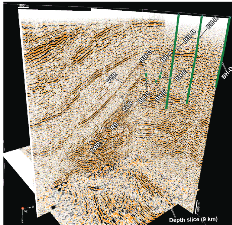
Figure 5.2 3D visualization of the migrated seismic volume covering Anglo Gold Ashanti and Sibanye Gold mines along the West Wits Line Goldfields, showing strong seismic reflectors and location of boreholes (BH-A to BH-H). VCR: Ventersdorp Contact Reef, TWR: Top of the West Rand, RS: Roodepoort shale, CLR: Carbon Leader Reef.
