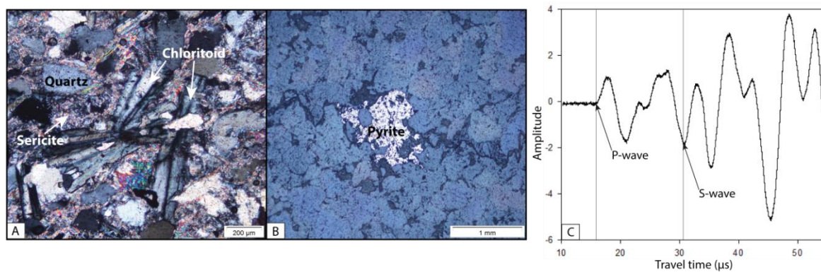
Figure 9 Thin section of the Blyvooruitzicht footwall in (a) cross polarized light and (b) reflected light. The thin sections show the dominant minerals such as quartz, chloritoid and sericite and (c) the amplitude versus travel time graph shows the response of seismic wave velocities to these dominant minerals. The amplitude versus travel time graph also shows the clear identification of the P-wave arrival time compared to the S-wave arrival time.
