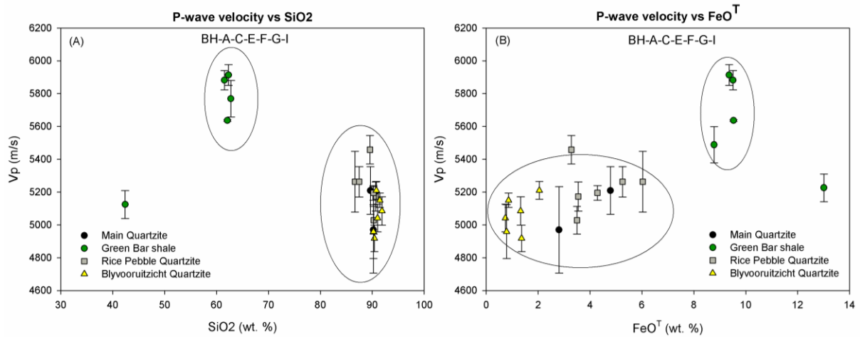
Figure 11 Graph of (a) P-wave velocity versus \text{SiO}_2 ( V_p ) and (b) P-wave velocity versus \text{FeO}^T for the Carbon Leader Reef hangingwall and footwall lithologies from borehole BH-A, BH-C, BH-E, BH-F, BH-G and BH-I. Higher P-wave velocities correspond to lower \text{SiO}_2 and higher \text{FeO} values, while lower P-wave velocities correspond to higher \text{SiO}_2 and lower \text{FeO} values. The horizontal and vertical bars indicate standard deviations obtained from multiple measurements of the same sample or from similar type samples. The calculated V_p error ranges from 0.1 to 0.3 for the measured samples.
