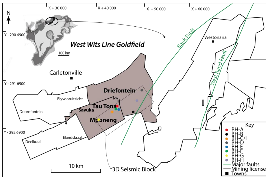
Figure 0.2 The map showing the Witwatersrand Basin and the various gold mines across the West Wits Line goldfield. The north-east trending first-order scale Bank Fault and West Rand Fault are shown. The Bank Fault cuts through the south-east margin of the Driefontein gold mine. The map also shows the locations of the 9 surface and underground boreholes used to derive samples for this study (after Dankert and Hein 2010).
