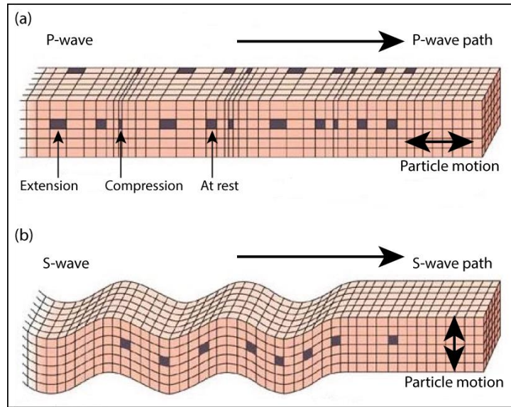
Figure 3.1 Body waves and their propagation directions. (a) Particle motion of P-waves is parallel to the direction of wave propagation. (b) Particle motion of S-waves is perpendicular to the direction of wave propagation (after Veeken 2007).
