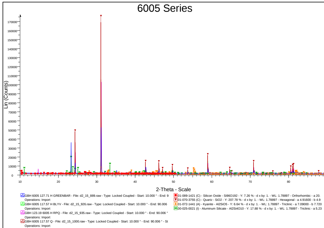
Figure 3: A stacked plot of the phase identification of the GBH 6005 samples: 127.71 H GREENBAR, 117.57 H BLYV, 123.19 H RPQ, and 117.57 Q. Phases are included at the bottom of the diagram. H: Heavy minerals; Q: Quartz.
