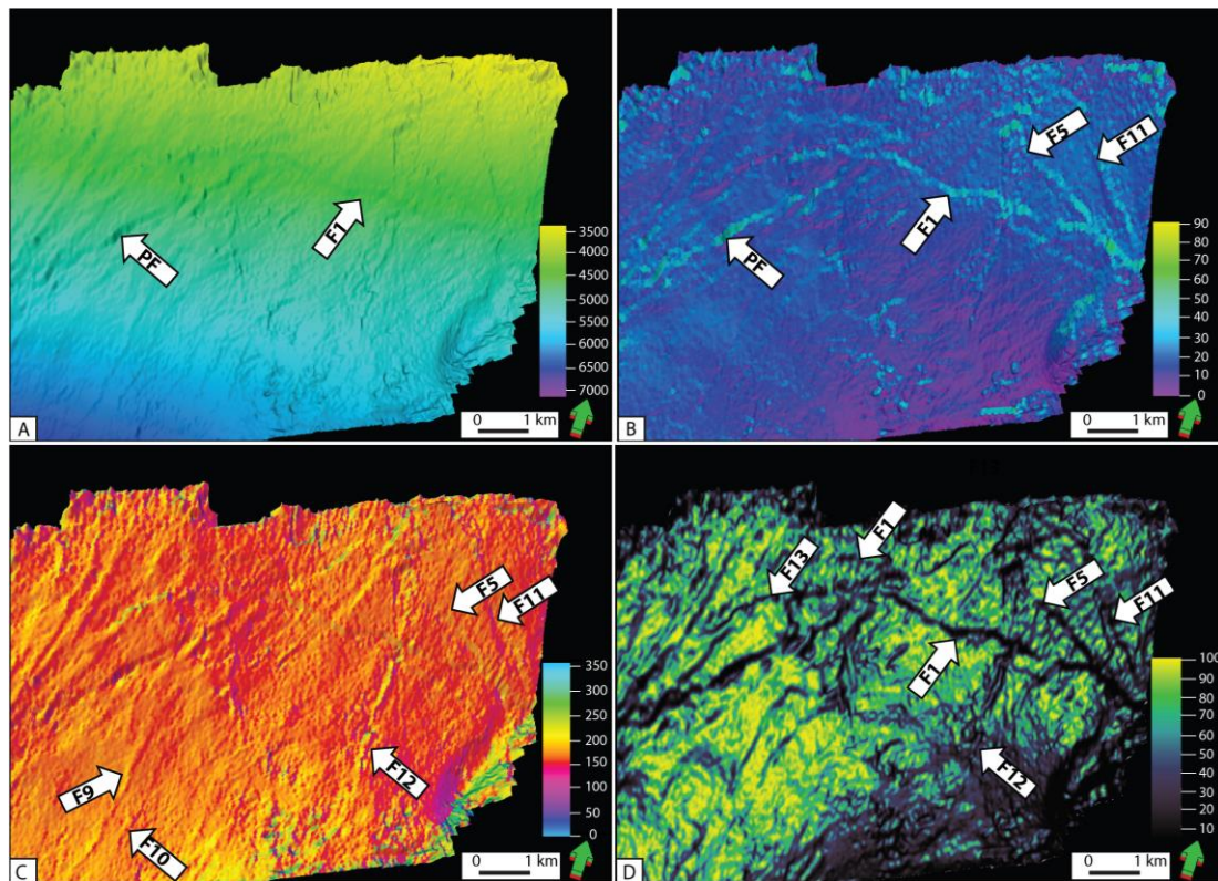
Fig. 13 Seismic attributes computed for the top of the West Rand horizon (block B). (a) The top of the West Rand smoothed surface (colour bar represents depth in metres). (b) Dip attribute display, showing the northeast trending Pretorius Fault (PF), northwest trending F1 as well as F5 and F11 (colour bar given in degrees). (c) Azimuth attribute display, showing the enhancement of the F10 and F12 (colour bar given in percentages). (d) The edge detection attribute display clearly shows the northeast trending F13 as well as the north-northeast trending F12. The edge detection map also enhances a displaced segment of F1 further north: Pretorius Fault (PF), Fault 1 (F1), Fault 5 (F5), Fault 9 (F9) and Fault 10 (F10), Fault (F10), Fault 11 (F11), Fault 12 (F12) and Fault 13 (F13).
