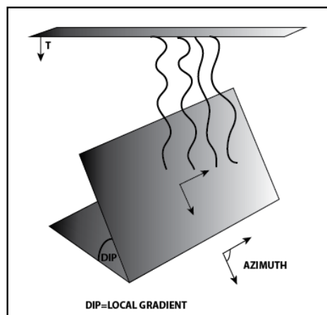
Figure 4.12 Schematic representation of how the dip and azimuth are calculated in seismic data.
