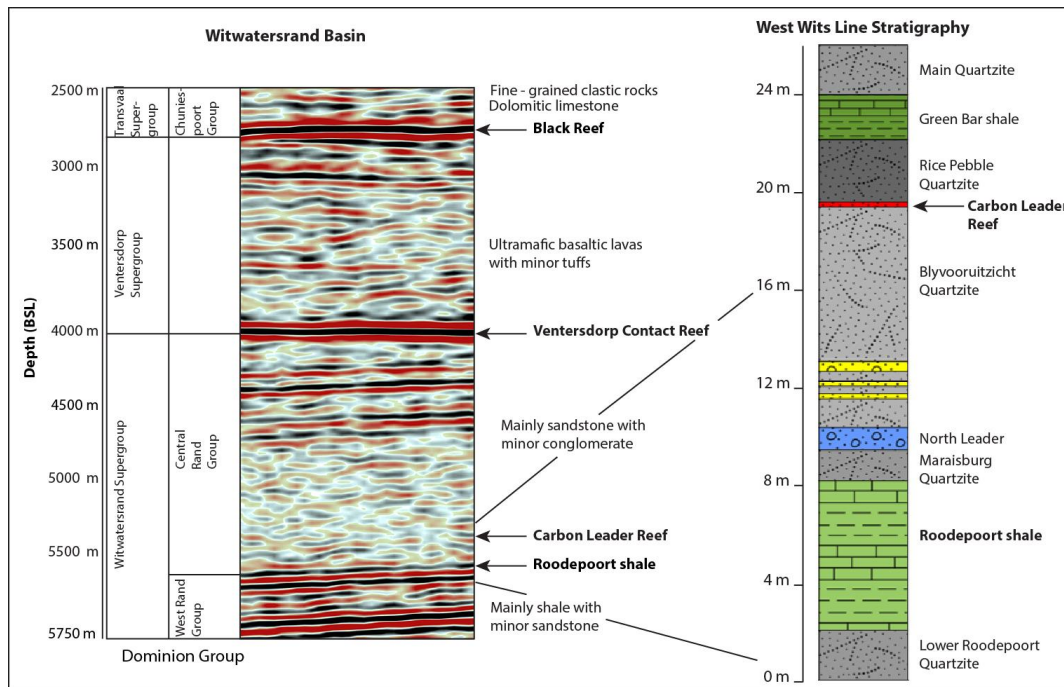
Fig. 3 Stratigraphy of the Witwatersrand Basin highlighting the location of strong seismic reflectors throughout the basin. The local stratigraphy at the base of the Central Rand Group and at the top of the West Rand Group along the West Wits Line is illustrated on the far right, as observed from borehole intersections (after Guy et al., 2010).
