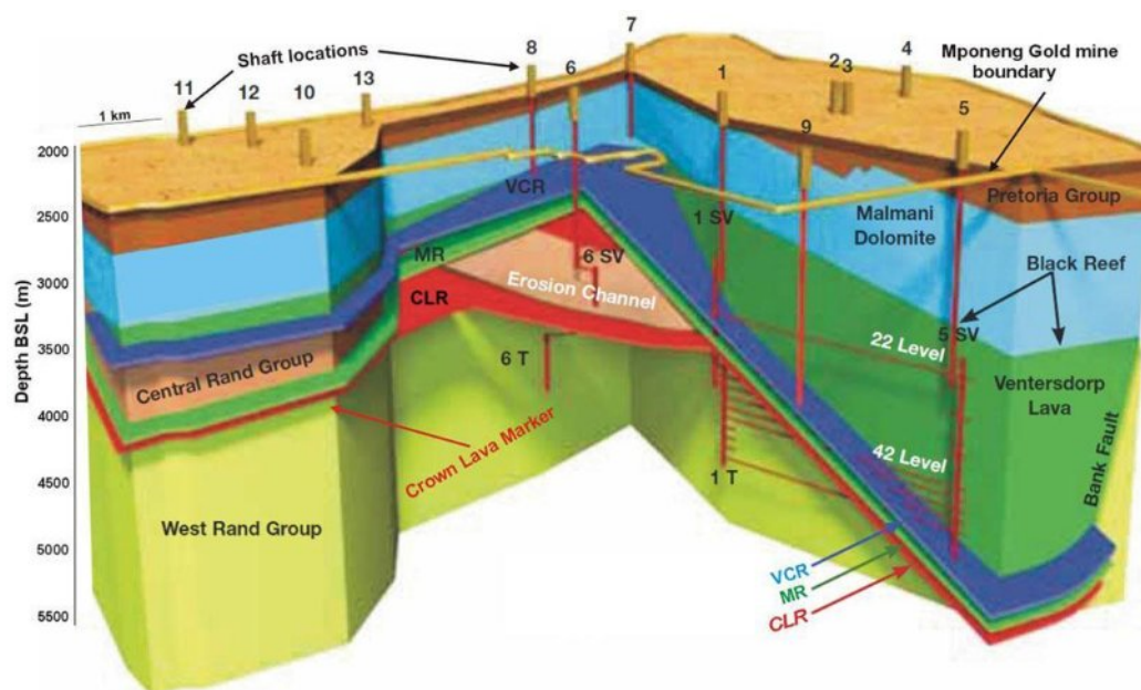
Figure 3 A 3D sketch of the mine lease showing shaft locations, mining levels and stratigraphic units of the study area. VCR: Ventersdorp Contact Reef; MR: Middelvlei Reef; CLR: Carbon Leader Reef.
