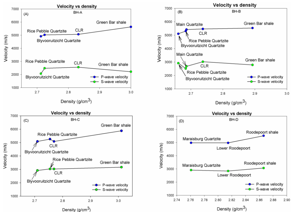
Figure 10 Graphs of P- wave and S-wave velocities obtained using the ultrasonic device at ambient stresses from (a) BH-A, (b) BH-B, (c) BH-C and (d) BH-D. Borehole BH-A to BH-C represent the Carbon Leader Reef (CLR) conglomerate intersections and borehole BH-D represents the Roodepoort shale intersection. The calculated V_p error ranges from 0.1 to 0.3 for the measured samples.
