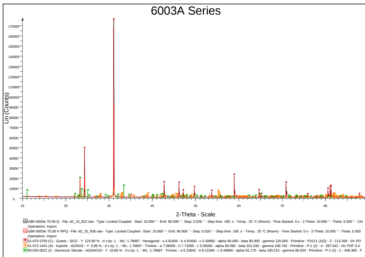
Figure 2: A stacked plot of the phase identification of the borehole GBH 6003A samples: 70.58 Q and 70.58 H RPQ. Phases are included at the bottom of the diagram. H: Heavy minerals; Q: Quartz.
