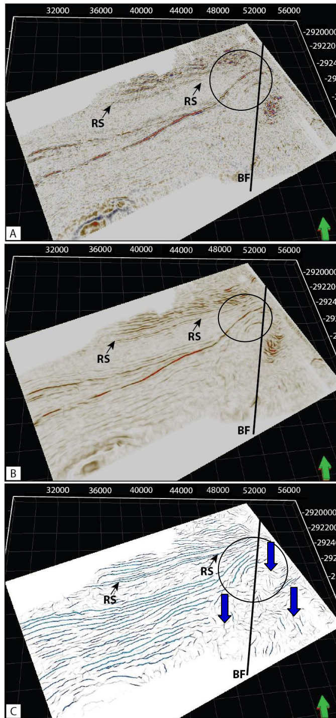
Fig. 10 Depth slices showing (a) the conventional seismic amplitude display, (b) edge enhancement display and (c) the ant-tracking attribute. Circle highlights the rollover anticline position and the blue arrows show the enhancement of fractures and minor faults. RS: Roodepoort shale, BF: Bank Fault.
