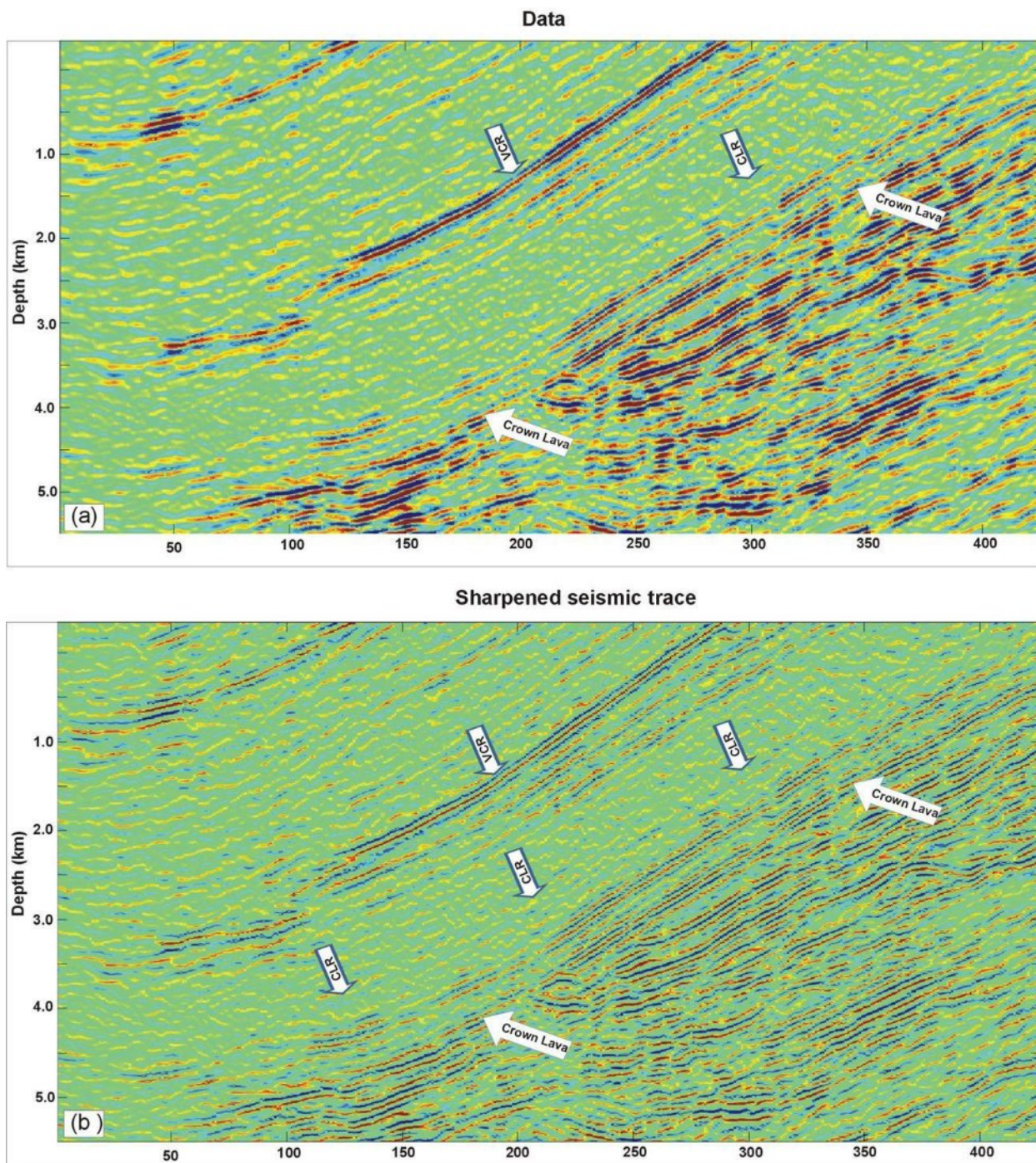
Figure 10 The comparison between an original seismic trace and sharpened trace. (a) Original seismic trace showing poor detection of the CLR. (b) The detection of Carbon Leader Reef is enhanced on the sharpened seismic trace.
