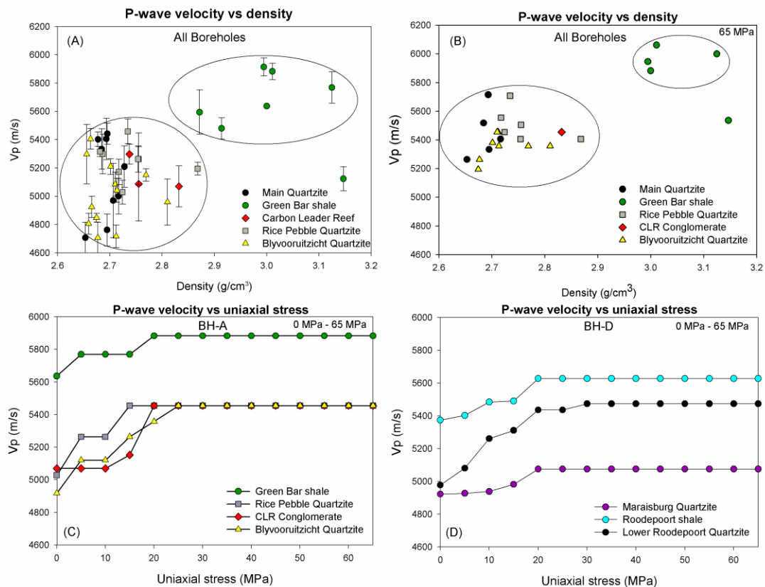
Figure 12 A comparison of P-wave velocity ( V_p ) versus density (a) ambient and (b) elevated stresses, showing an increase in velocities of the samples with increasing stress. The effect of uniaxial stress is further shown by (c) borehole BH-A and (d) BH-D where the seismic velocities increase as the stress is increased and becomes constant above ~20 - 25 MPa. The horizontal and vertical bars indicate standard deviations obtained from the measurements of similar type samples or repeated measurements. The calculated V_p error ranges from 0.1 to 0.3 m/s for the measured samples.
