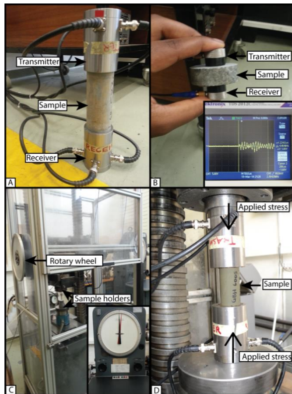
Figure 6 Ultrasonic velocity measurement apparatus at ambient (a and b) and elevated stresses (c and d). (a) Larger transducer (diameter=32 mm, 0.5 MHz) set used to measure seismic velocities for large samples (b) smaller transducer (diameter=16 mm, 0.5 MHz) set used to measure seismic velocities for smaller samples. (c) The uniaxial compressional loading is produced by hydraulic pistons that are driven by a computer controlled load holding pump. The induced load is monitored on a stress measuring gauge (insert in c). (d) The image shows the placement of the sample between the transducers positioned on pistons within the chamber.
