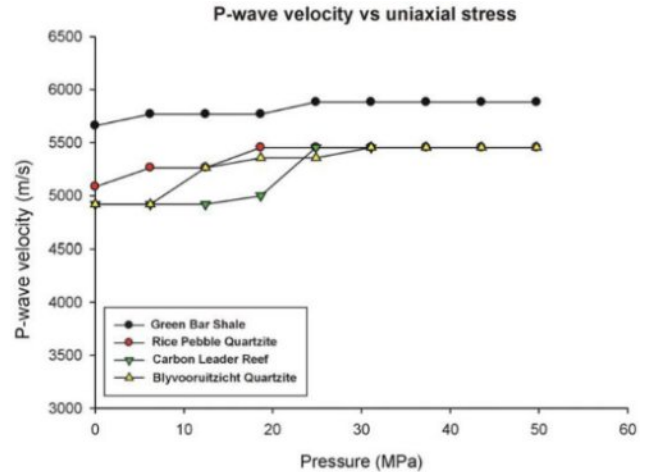
Figure 7 Effect of uniaxial stress on the P-wave velocities. The seismic velocities increase as the uniaxial stress increases and become constant above 20 MPa.
