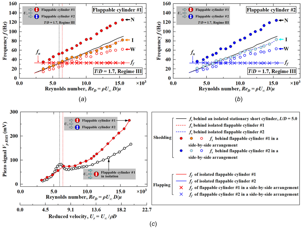
Fig. 14 Wake shedding frequency ( f_s ) and flapping frequency ( f_f ) at T/D = 1.7 , as a function of Reynolds number: (a) for flappable cylinder #1, (b) for flappable cylinder #2, and (c) piezo-signals showing amplification due to resonance
