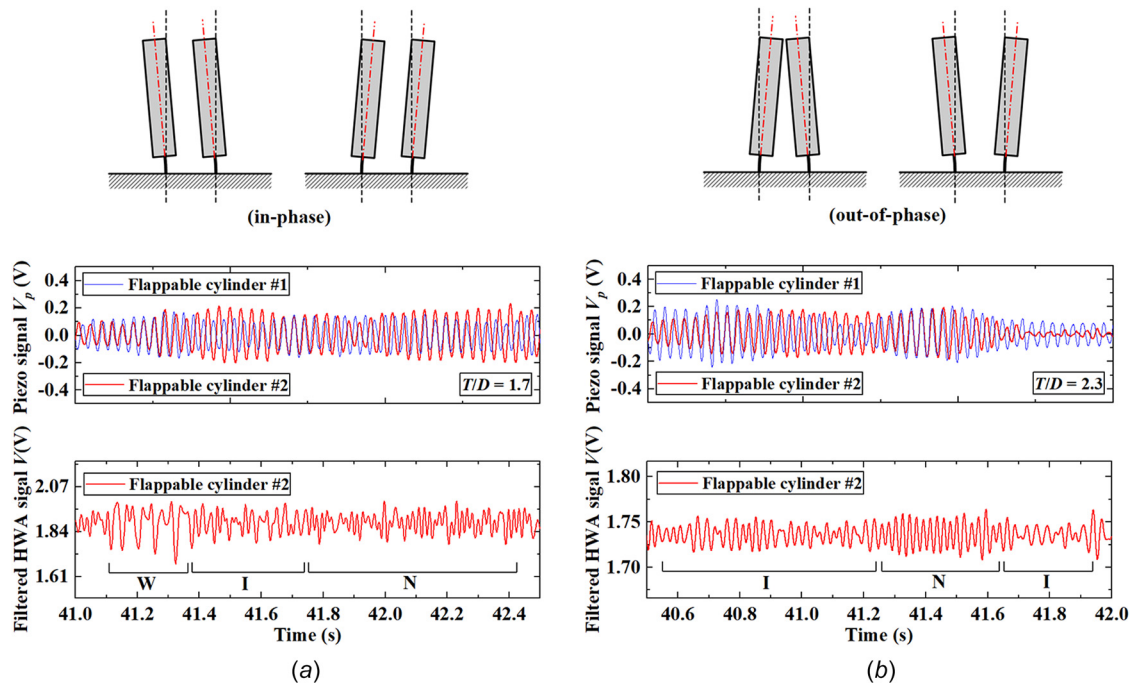
Fig. 15 Time-resolved signals from both PZT mounts attached to the base of each flappable cylinder and the corresponding switching events of wakes shed at Re_D = 6000 : (a) at T/D = 1.7 and (b) at T/D = 2.3
