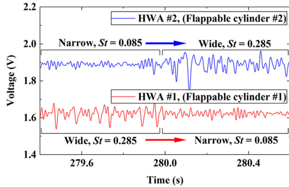
Fig. 11 Bistable wakes that switch at T/D = 1.4 and Re_D = 6000 by sampled raw voltage signals from HWA#1 showing the switching from wide (W) wakes to narrow (N) wakes, i.e., W \rightarrow N , and from HWA#2 showing the reciprocal switching from narrow (N) wakes to wide (W) wakes N \rightarrow W
