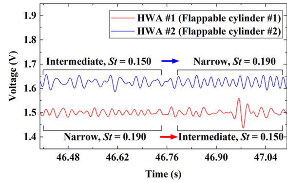
Fig. 13 Biased wakes shed at T/D = 2.3 and Re_D = 6000 by sampled raw voltage signals from HWA #1 and HWA #2, showing the biased switching mode, i.e., N \rightarrow I for flappable cylinder #1 and I \rightarrow N for flappable cylinder #2
