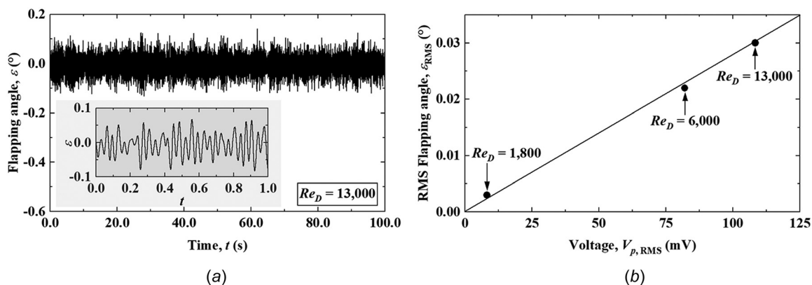
Fig. 5 Variation of an isolated cylinder flapping displacement: (a) flapping angle variation with time and (b) variation of RMS flapping angle versus PZT plate voltage
