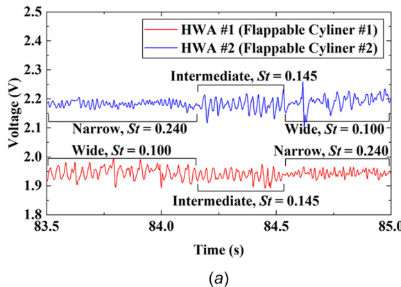
Fig. 12 Tristable wakes shed at T/D = 1.7 and Re_D = 6000 (i.e., regime III): (a) sampled raw voltage signals from HWA #1 and HWA #2, showing the full switching mode, i.e., W \rightarrow I \rightarrow N for flappable cylinder #1 and N \rightarrow I \rightarrow W for flappable cylinder #2 and (b) sampled raw voltage signals from HWA #1 and HWA #2, showing the biased switching mode, i.e., W \rightarrow I \rightarrow W for flappable cylinder #1 and N \rightarrow I \rightarrow N for flappable cylinder #2
