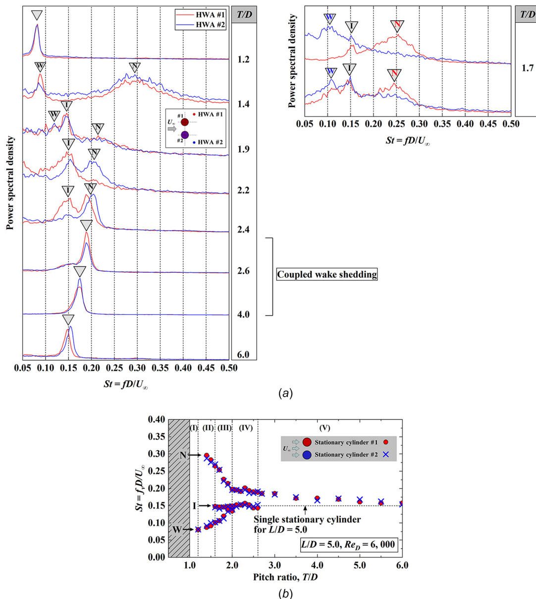
Fig. 8 Wakes shed from two short side-by-side cylinders at Re_D = 6000 : (a) power spectra from both stationary cylinders and (b) Strouhal number of both stationary cylinders varying with gap ratio ( T/D ), with a short single stationary cylinder in isolation as reference
