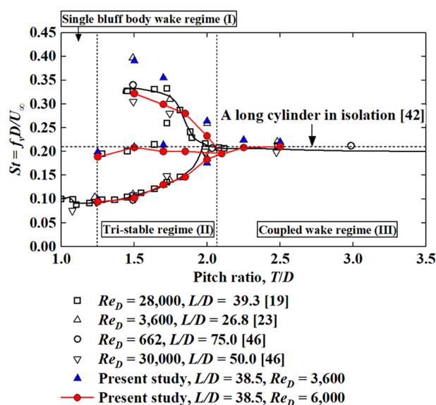
Fig. 7 Wakes shed from two long side-by-side cylinders showing Strouhal number that varies with gap ratio ( T/D ) for selected Reynolds numbers
