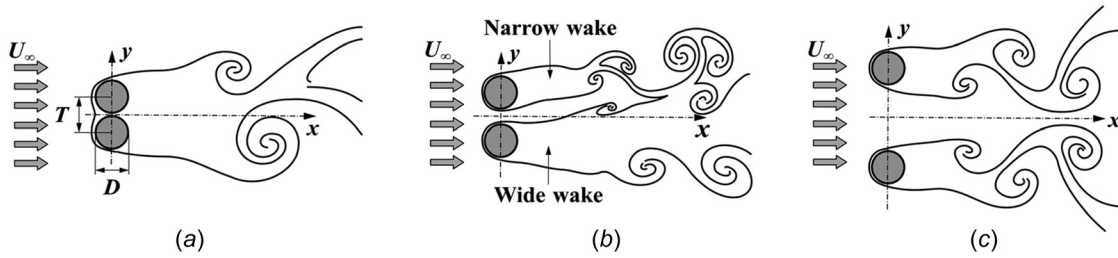
Fig. 1 Schematic representation of distinct wake regimes varying with gap ratio: (a) single bluff body wake regime, T/D < 1.1 – 1.2 [2,16–18]; (b) bistable wake regime, 1.1 – 1.2 \leq T/D \leq 2.0 – 2.2 [1,18,19]; and (c) coupled wake regime, 2.0 – 2.2 < T/D < 4.0 – 4.5 , at 30 – 48 \leq Re_D < 500,000 – 1,000,000 [2,15]
