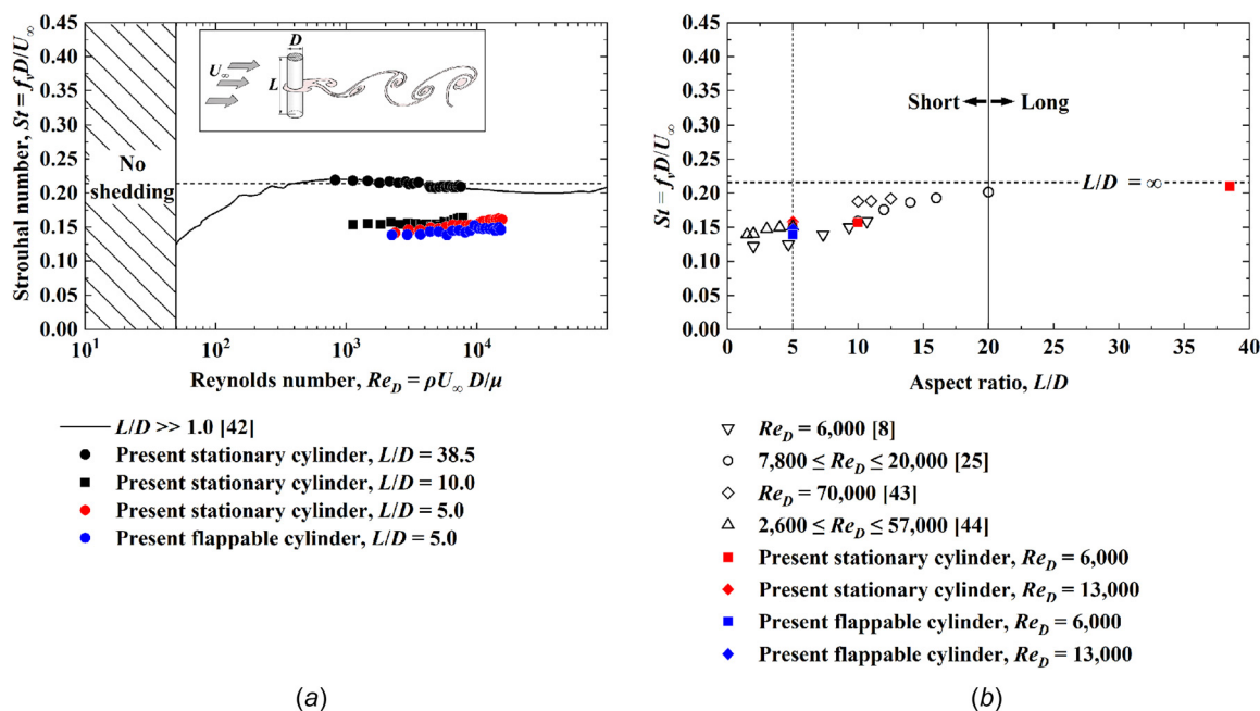
Fig. 6 Wakes shed from a cylinder in isolation: (a) Strouhal number varying with Reynolds number and (b) effect of aspect ratio on Strouhal number
