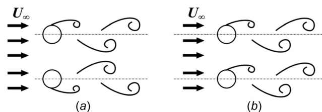
Fig. 2 Synchronized vortices shed from two long side-by-side cylinders: (a) antiphase mode and (b) in-phase mode
