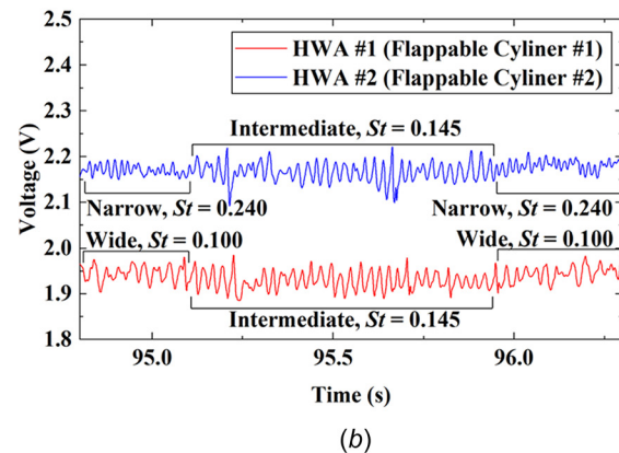
Fig. 12 Tristable wakes shed at T/D = 1.7 and Re_D = 6000 (i.e., regime III): (a) sampled raw voltage signals from HWA #1 and HWA #2, showing the full switching mode, i.e., W \rightarrow I \rightarrow N for flappable cylinder #1 and N \rightarrow I \rightarrow W for flappable cylinder #2 and (b) sampled raw voltage signals from HWA #1 and HWA #2, showing the biased switching mode, i.e., W \rightarrow I \rightarrow W for flappable cylinder #1 and N \rightarrow I \rightarrow N for flappable cylinder #2
