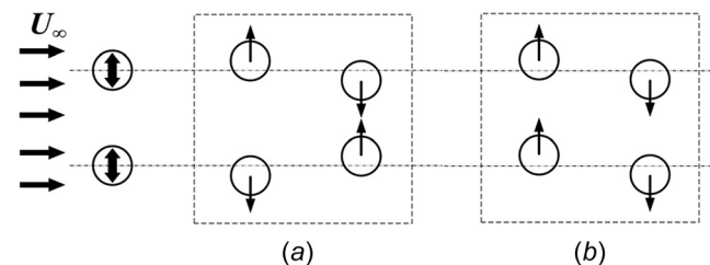
Fig. 3 Vibration modes of two long side-by-side cylinders: (a) antiphase mode and (b) in-phase mode
