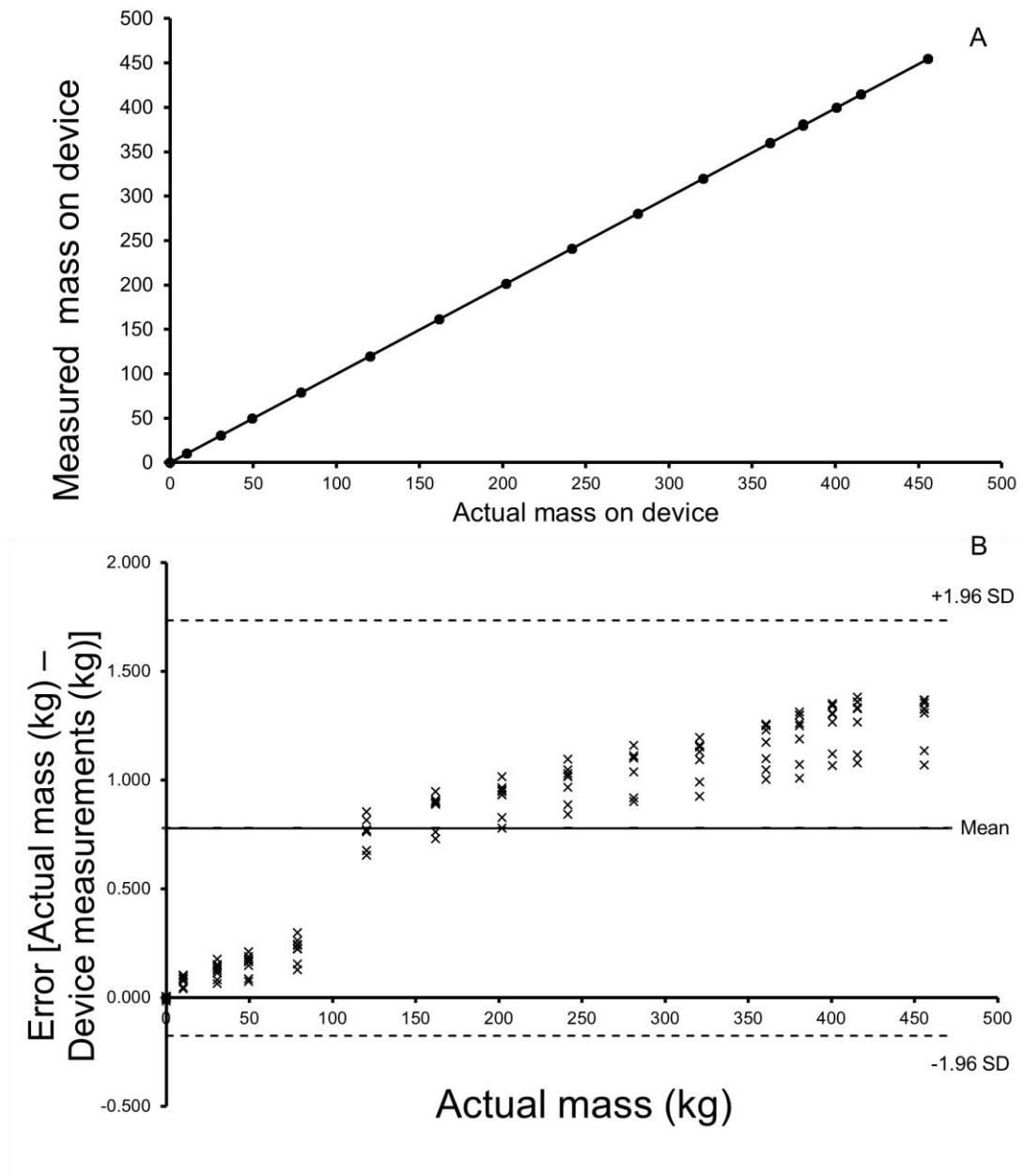
Figure 6.4: The relationship between actual force application and measured forces on the scrumming ergometer (A) and Bland-Altman Limits of agreement as a function of actual masses applied (B) for 8 trials.
