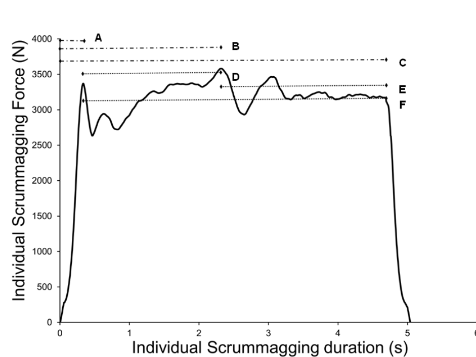
Figure 7.1: Individual scrummaging force tracing and the duration divisions: A starting force to engagement force; B starting force to peak force; C starting force to sustained force; D engagement force to peak force; E engagement force to sustained force; and F peak force to sustained force.
