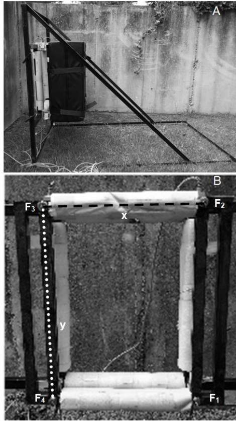
Figure 6.1: The individual scrum ergometer. A: profile of ergometer with cushion pads on the scrum plate: load cells placed between support structure and scrum plate. B: Scrum plate without cushion pads: load cells positioned and F_1 - F_4 .
