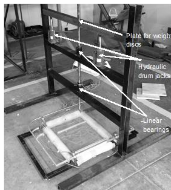
Figure 6.2: Linear vertical mass assembly used to calibrate the centre of pressure position.
