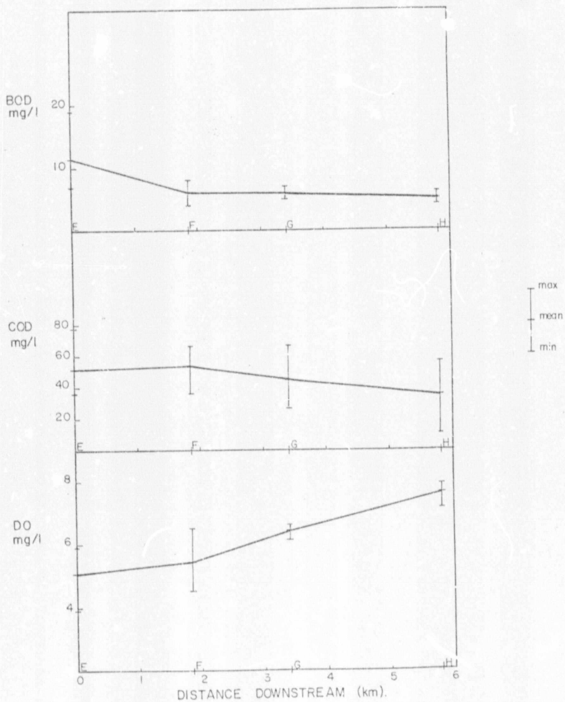
Figures :- 7.2 :- BOD, COD and DO variation with distance downstream. (Sampling survey 18 July 1978.)
