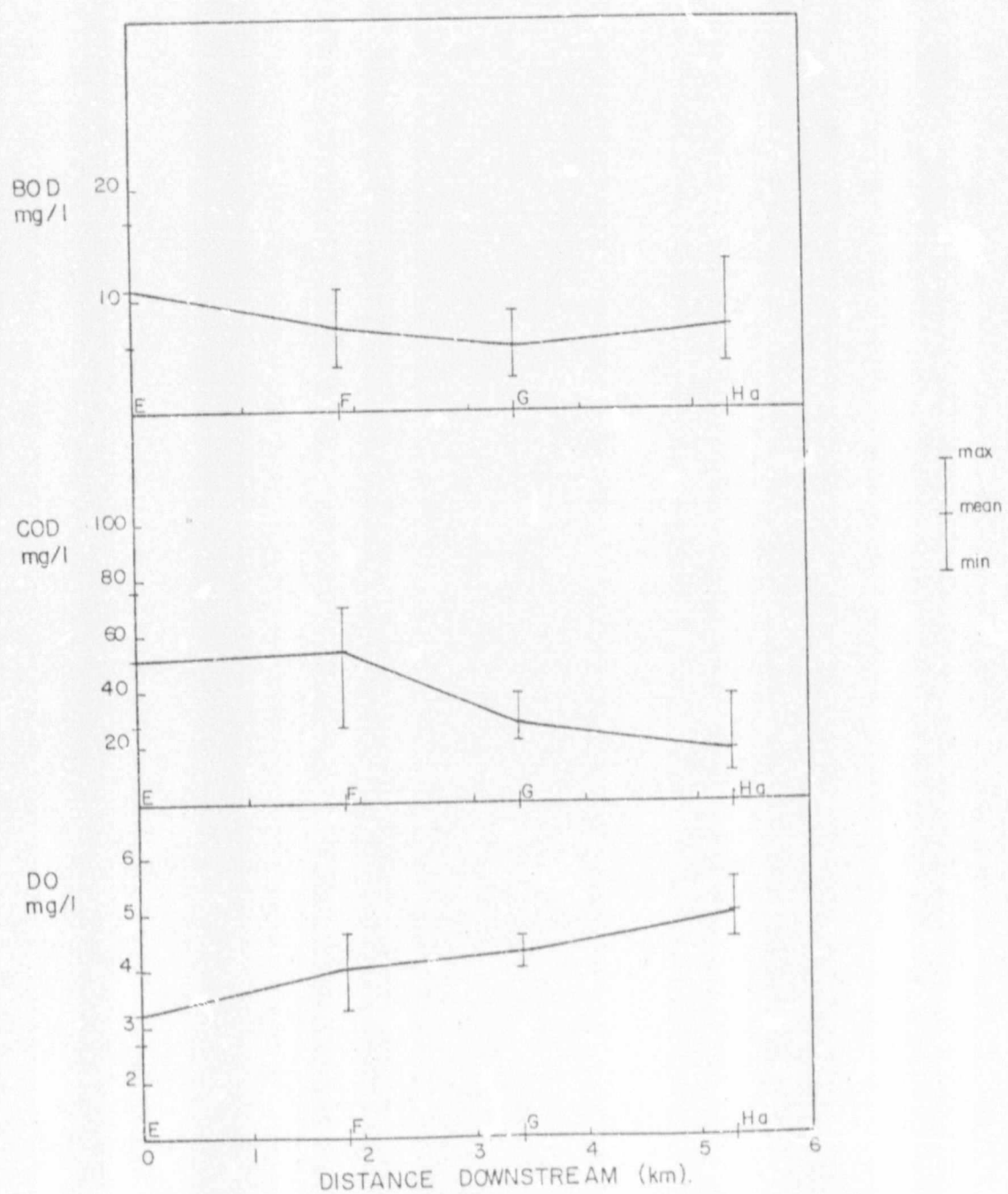
Figures :- 7.5 BOD, COD and DO variation with distance downstream. (Sampling survey 21 March 1979.)
