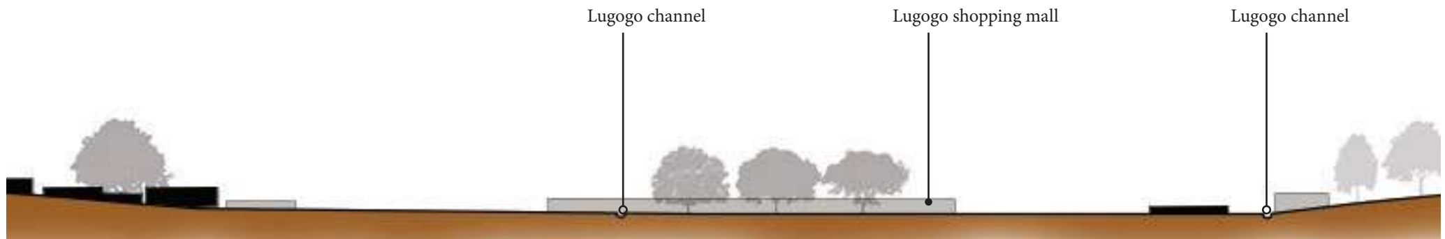
Figure 4.37: Section D-D (Author's sketch)
