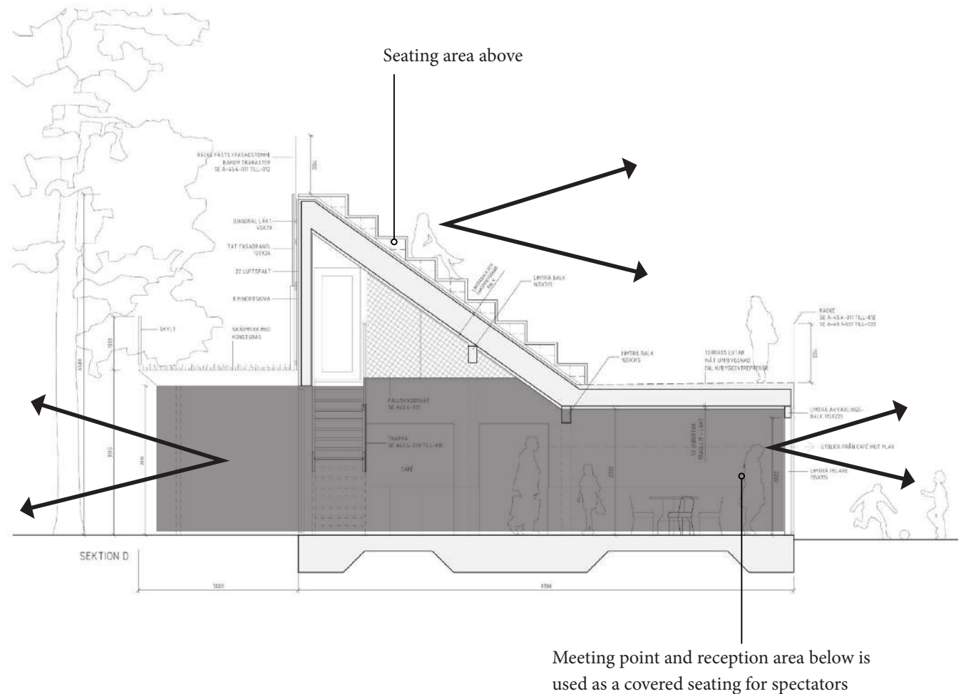
Figure 5.29: Section through the grandstand
