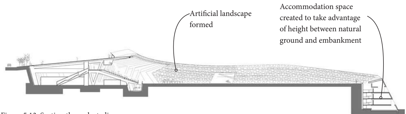
Figure 5.13: Section through stadium
