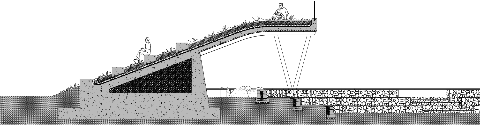
Detail 1 | Scale 1:100
