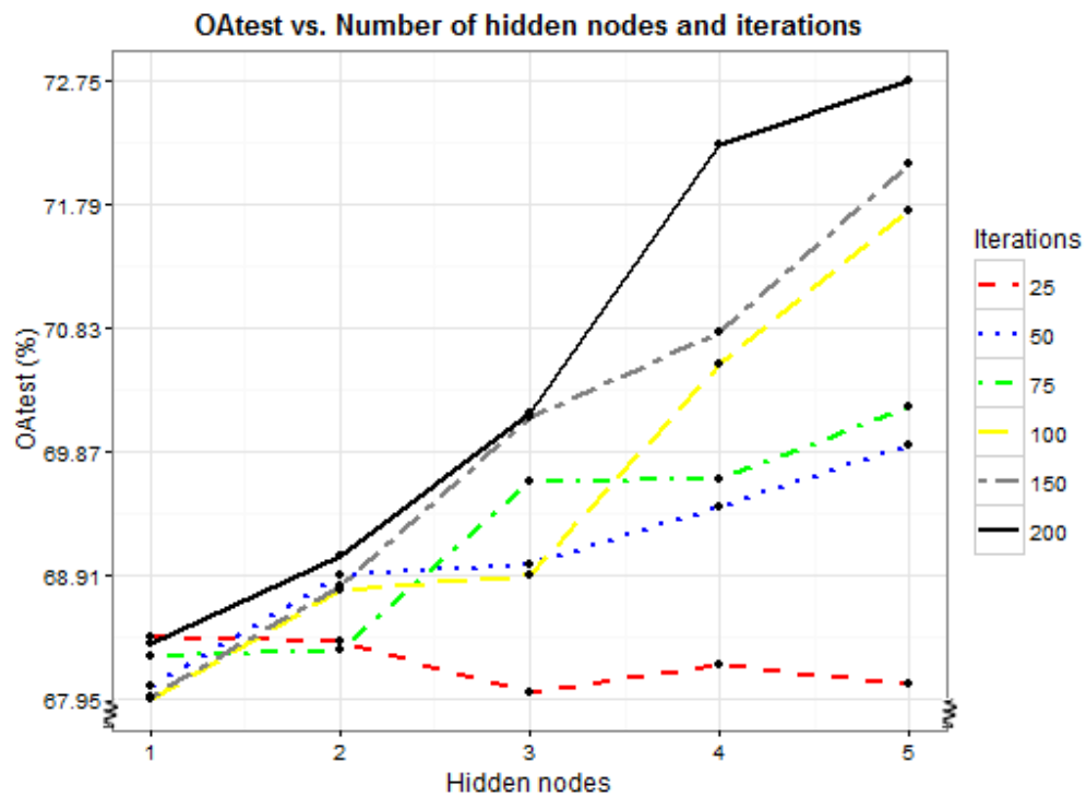
Figure 5.10: OAtest for 1-5 hidden nodes with 25-200 training iterations for the CYT/~CYT binary classifier
