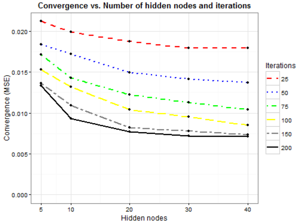
Figure 5.1: The MSE for varying the number of hidden nodes and training iterations for the cp/\sim cp binary classifier trained with Rprop
