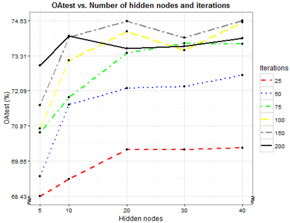
Figure 5.7: The OAtest for varying number of hidden nodes and training iterations for the CYT/ \sim CYT binary classifier trained with Rprop
