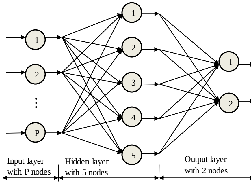
Figure 4.1: Neural network with P input, 5 hidden and 2 output nodes
