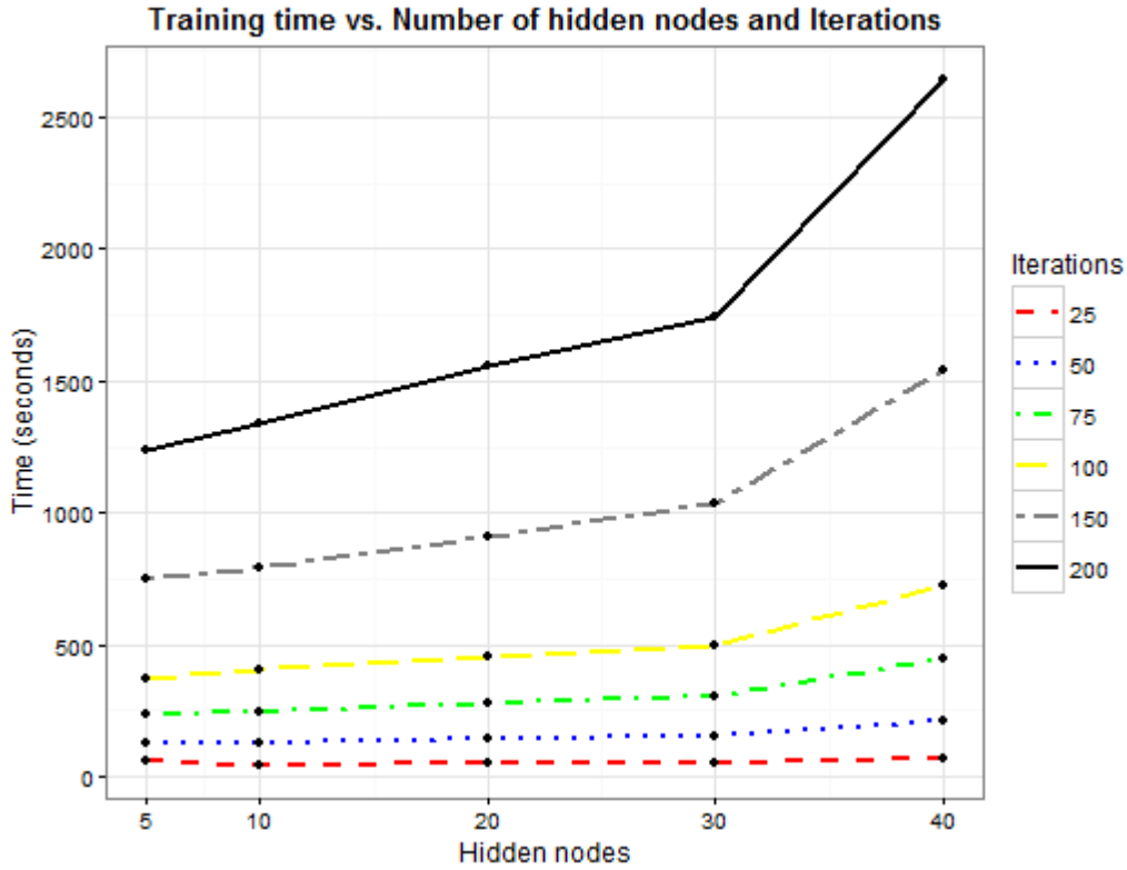
Figure 5.8: Training time (in seconds) for varying number of hidden nodes and training iterations for the CYT/ \sim CYT binary classifier trained with Rprop
