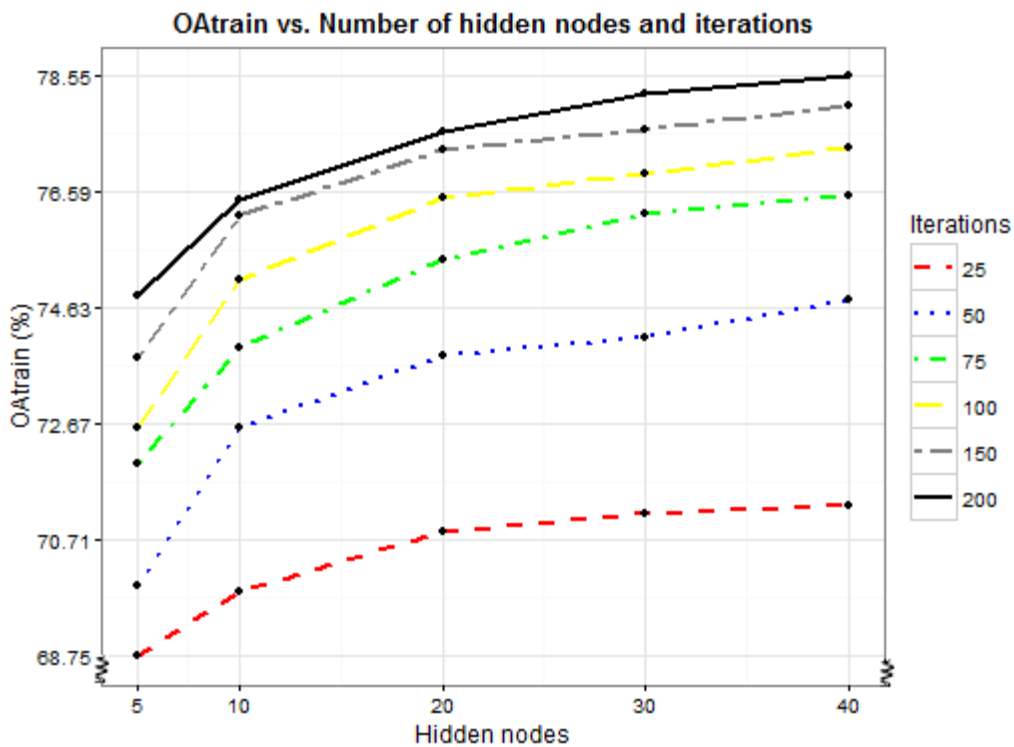
Figure 5.6: The OA train for varying number of hidden nodes and training iterations for the CYT/ \sim CYT binary classifier trained with Rprop
