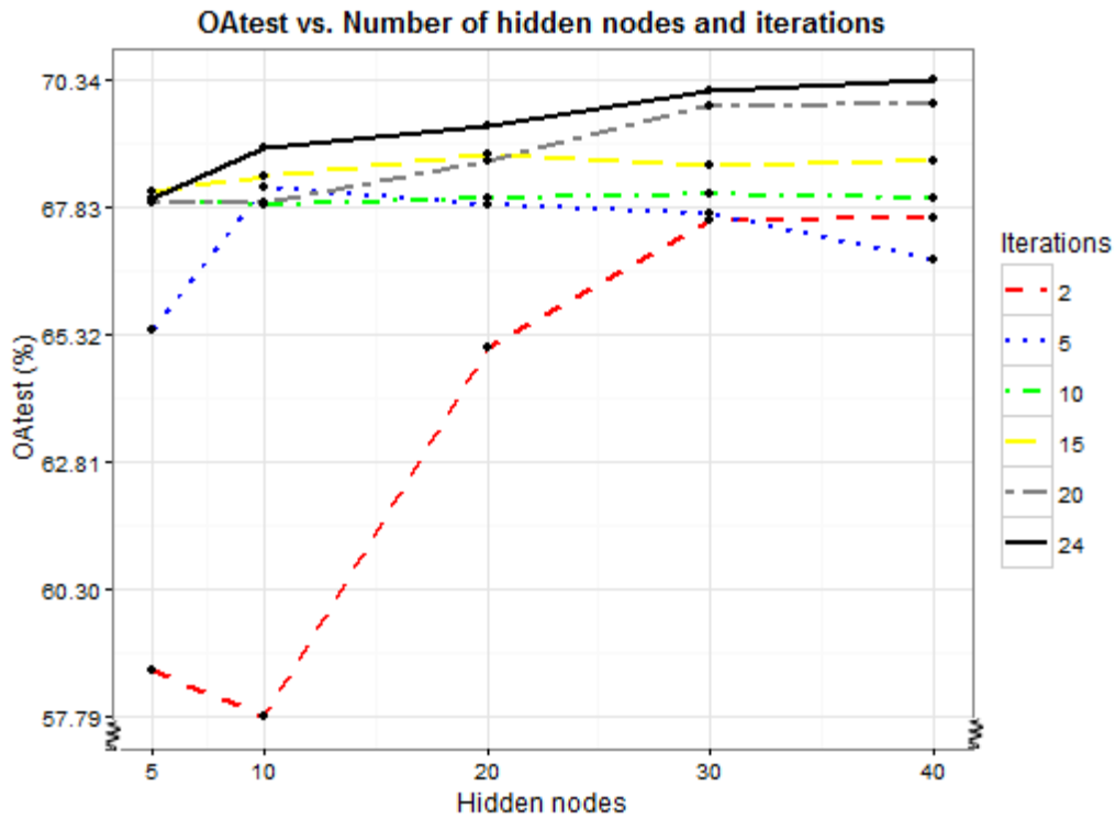
Figure 5.12: OAtest for 5-40 hidden nodes with 2-24 training iterations for the CYT/~CYT binary classifier
