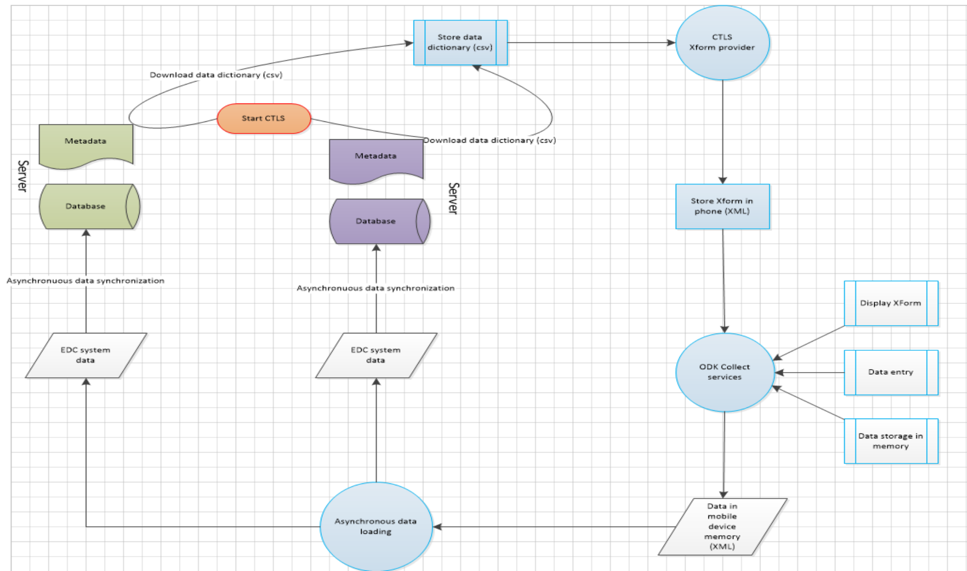
Figure 6: Architecture of CTLS
