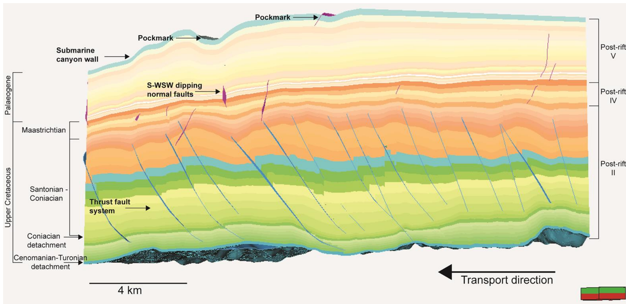
Figure 7.3. 3D model showing the stratigraphic units and their corresponding megasequences identified in the deepwater Orange Basin and the intersection of S-WSW dipping normal faults with the base of the pockmark. The continuation of the thrust faults into the Palaeogene is not visible in this view of the model. The full 3D model animation can be viewed in the attachment.
