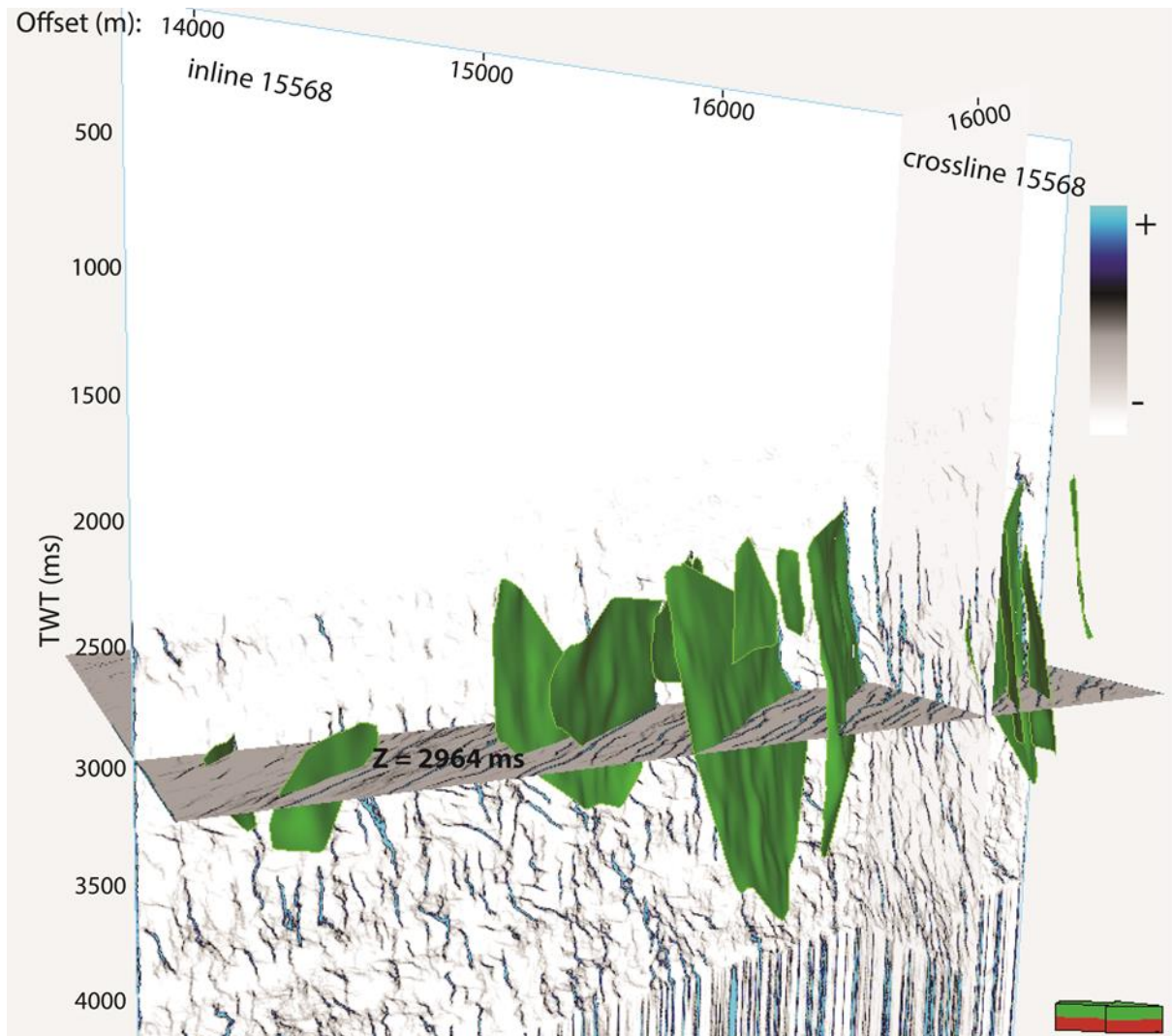
Figure 4.11. An ant tracked volume highlighting the extracted N-ENE dipping faults in green. Vertical exaggeration (VE) is 7:1.
