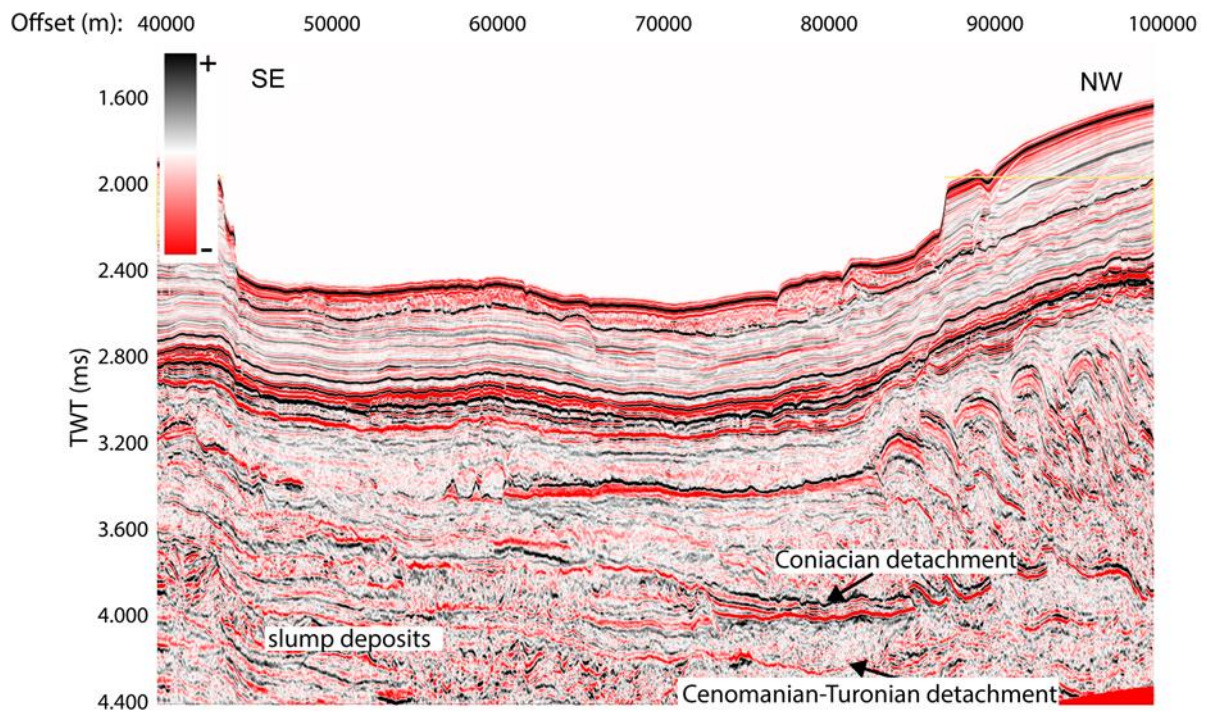
Figure 5.3. An amplitude display section showing the Coniacian and Cenomanian-Turonian detachments. The Cenomanian-Turonian detachment is terminated by a slump deposit in the south. The vertical exaggeration (VE) of the section is 17:1.
