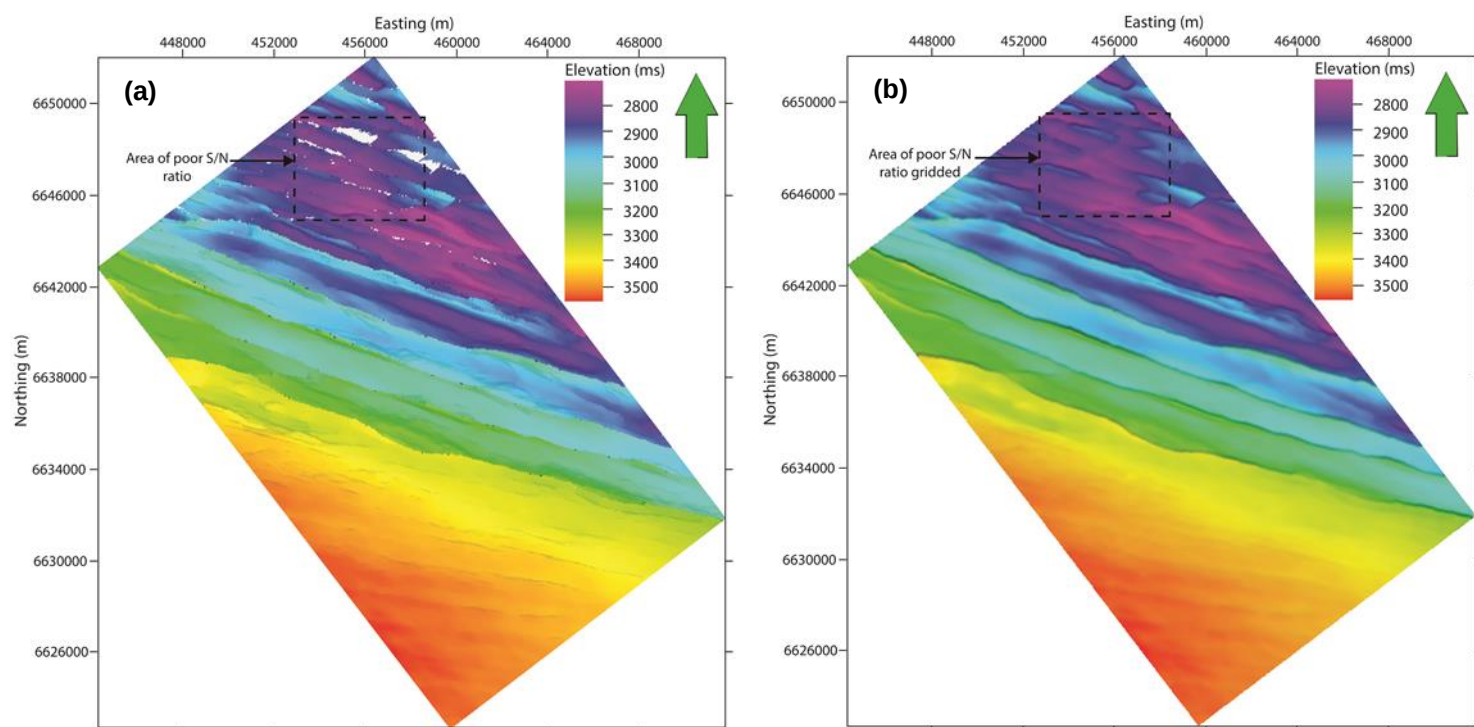
Figure 4.7. Horizon at the top of the thrust fault system (base of the Santonian) (a) before and (b) after applying the Kriging method to interpolate in structurally complex areas with sparse data. The dashed box highlights the areas that are structurally complex or have sparse data.
