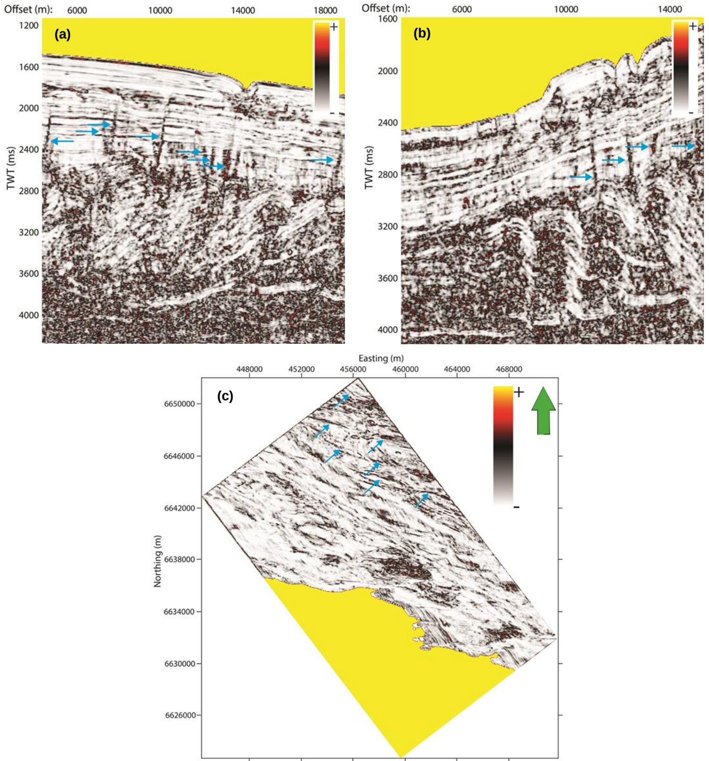
Figure 4.8. Chaos attribute applied to the (a) inline, (b) crossline and (c) time slice ( Z = 2400 ms) prior to ant tracking computation. Blue arrows indicate structures that were further enhanced by ant tracking. In (a) and (b), the darkest zones are zones with high chaoticness. These highly chaotic zones are fracture/fault zones. Sections (a) and (b) are vertically exaggerated by a factor of 7.
