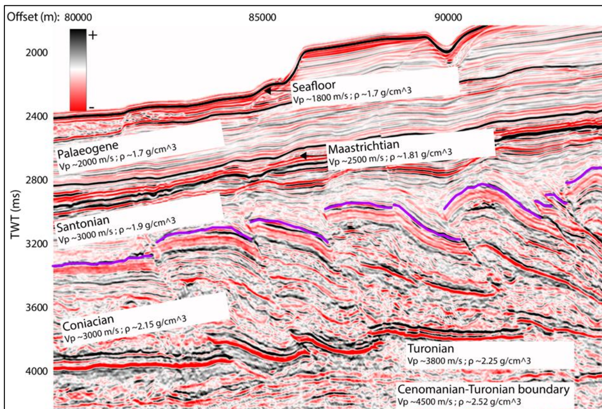
Figure 5.6. An amplitude display seismic section showing faults at the deformation front. The horizon used to measure displacement along the fault is highlighted. The vertical exaggeration (VE) of the section is 8:1.
