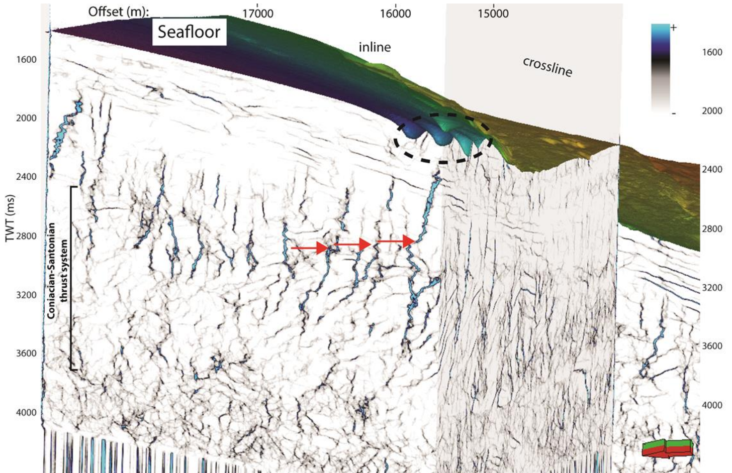
Figure 6.2. Ant tracked volume with the stereonet filter applied to detect faults dipping N-ENE. A number of faults have been highlighted above the Coniacian-Santonian thrust fault system. The normal faults indicated by the red arrows are linked to the thrust faults. The normal faults terminate in the Palaeogene. The pockmarks are shown by the dashed ellipse. Vertical exaggeration (VE) is 7:1.
