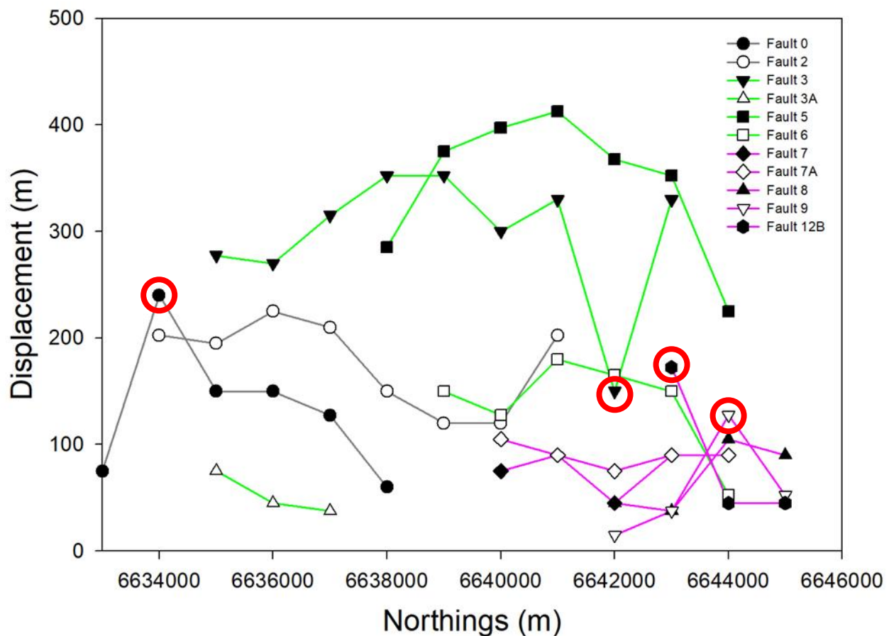
Figure 5.8. A south-to-north profile of the Coniacian to Santonian thrust fault system showing variations in vertical displacement with distance along the strike of the fault. The faults in grey occur along the deformation front; the faults in green are mapped in the inner part of the thrust fault system and the faults in pink are at the rear of the thrust fault system. Anomalous displacement measurements are indicated by the red circles.
