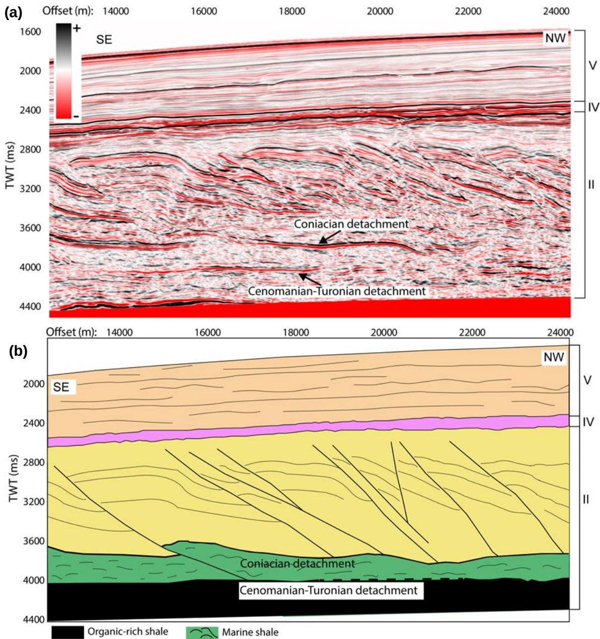
Figure 5.2. (a) An amplitude display seismic section and (b) a schematic diagram showing thrust faults attached to two basal detachment levels. The thrust faults to the NW sole into the Coniacian detachment and the thrust faults to the SE sole into the Cenomanian-Turonian detachment. Post-rift sequences II, IV and V were identified. Sections (a) and (b) are vertically exaggerated by a factor of 3.
