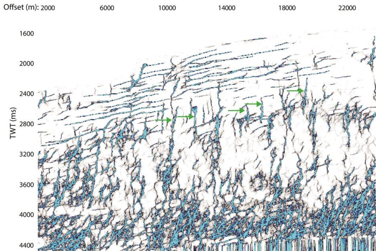
Figure 5.15. An ant tracked section of inline 15648 limited to detecting fault with a S to WSW dip direction and dip angles between 0^{\circ} and 90^{\circ} . A number of faults have been highlighted by the attribute. The faults marked by the green arrows are below the vertical resolution limit of 12 m. Vertical exaggeration (VE) is 7:1.
