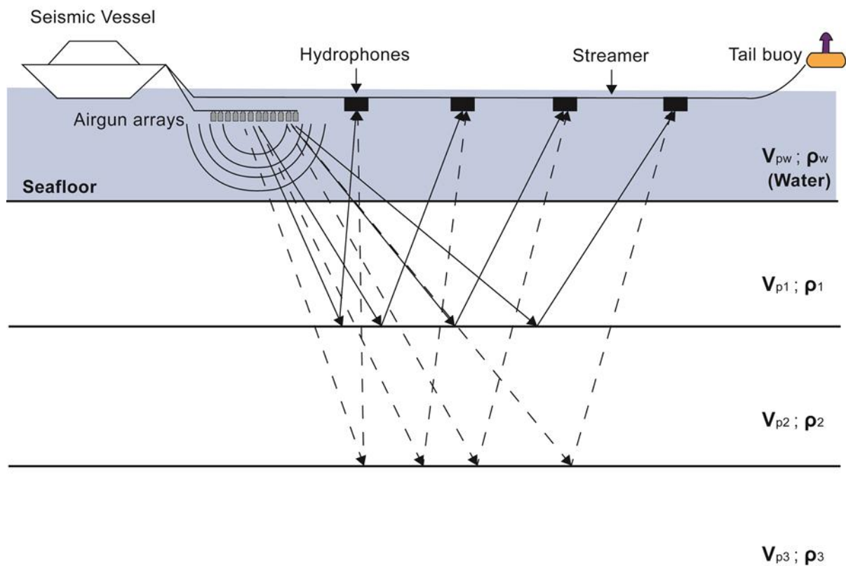
Figure 3.1. A Schematic diagram illustrating raypaths for reflections from interfaces. V_p represents the compressional waves and \rho represents the density. There is an acoustic impedance contrast across these interfaces, where V_{p2}\rho_2 > V_{p1}\rho_1 or V_{p2}\rho_2 < V_{p1}\rho_1 (After Thomas, 2015).
