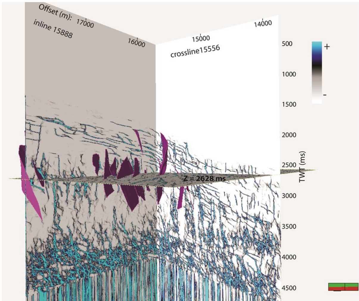
Figure 4.12. An ant tracked volume highlighting the S-WSW dipping faults in pink. Vertical exaggeration (VE) is 7:1.
