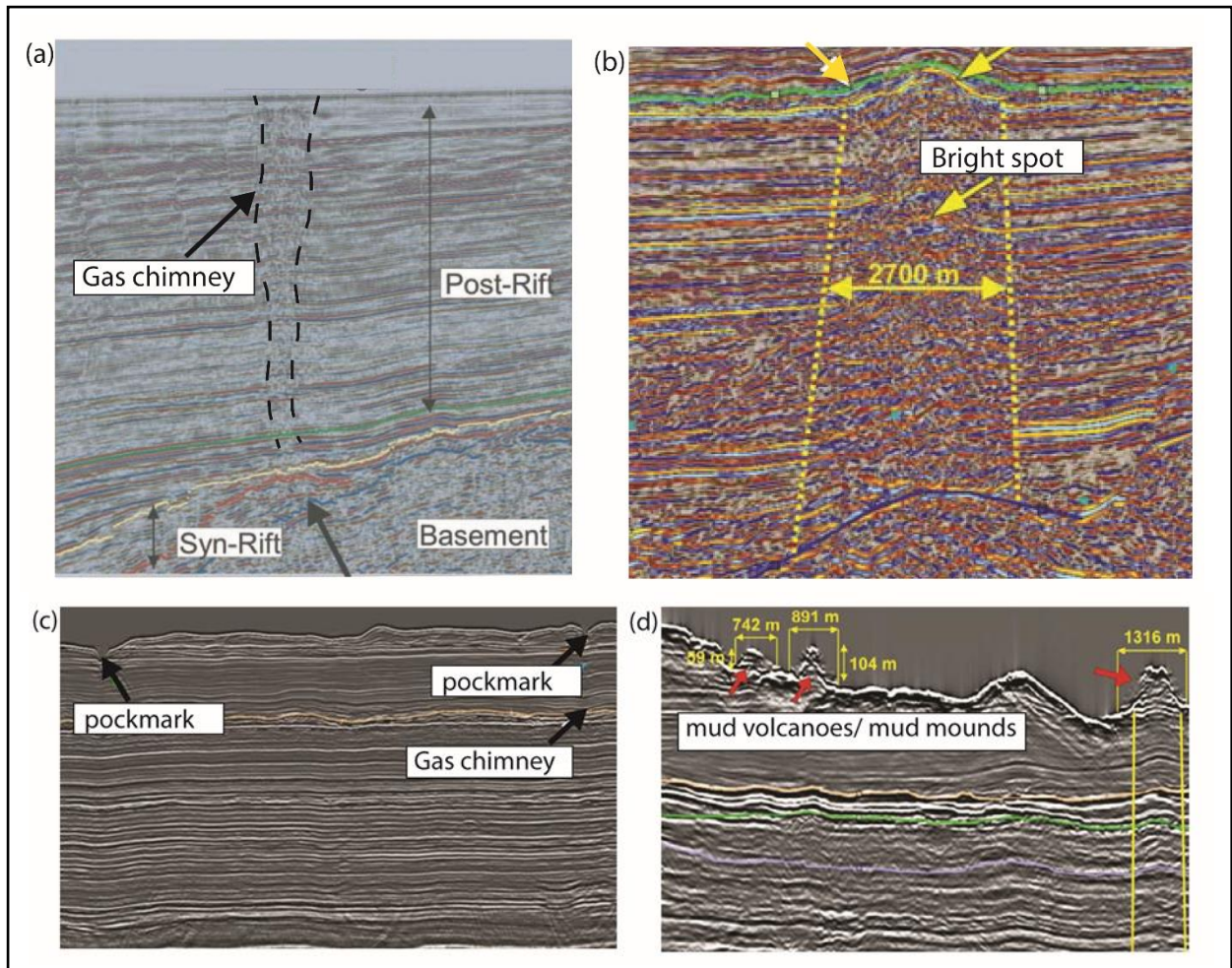
Figure 2.4. Seismic sections illustrating examples of gas escape features. (a) Gas chimney outlined by dashed black lines. (b) Yellow arrows indicating bright spots. (c) Gas chimney feeding pockmark. (d) Mud volcanoes or Mud mounds indicated by red arrows (Paton et al., 2007; Anka et al., 2014).
