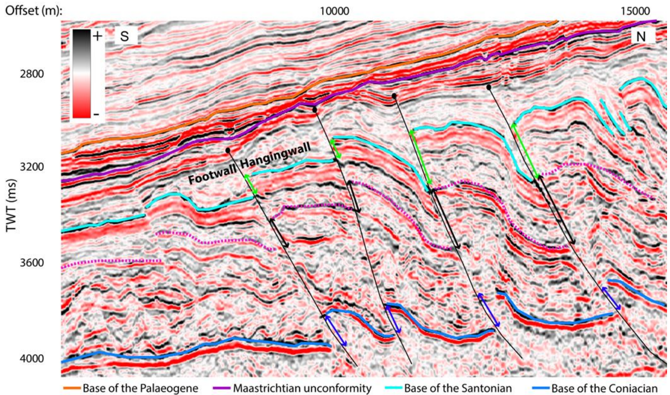
Figure 5.18. An amplitude display seismic section showing a large displacement (between the pink dotted lines) at the centre of the fault indicated by the black arrows and smaller displacement towards the detachment (indicated by the blue arrows) and fault tip (black circle) indicated by the green arrows. Faults propagate through fault limbs forming fault breakthrough folds. Both the footwall and hangingwall units are thickened, resulting in a constant thickness across dip domains. Vertical exaggeration (VE) of the section is 8:1.
