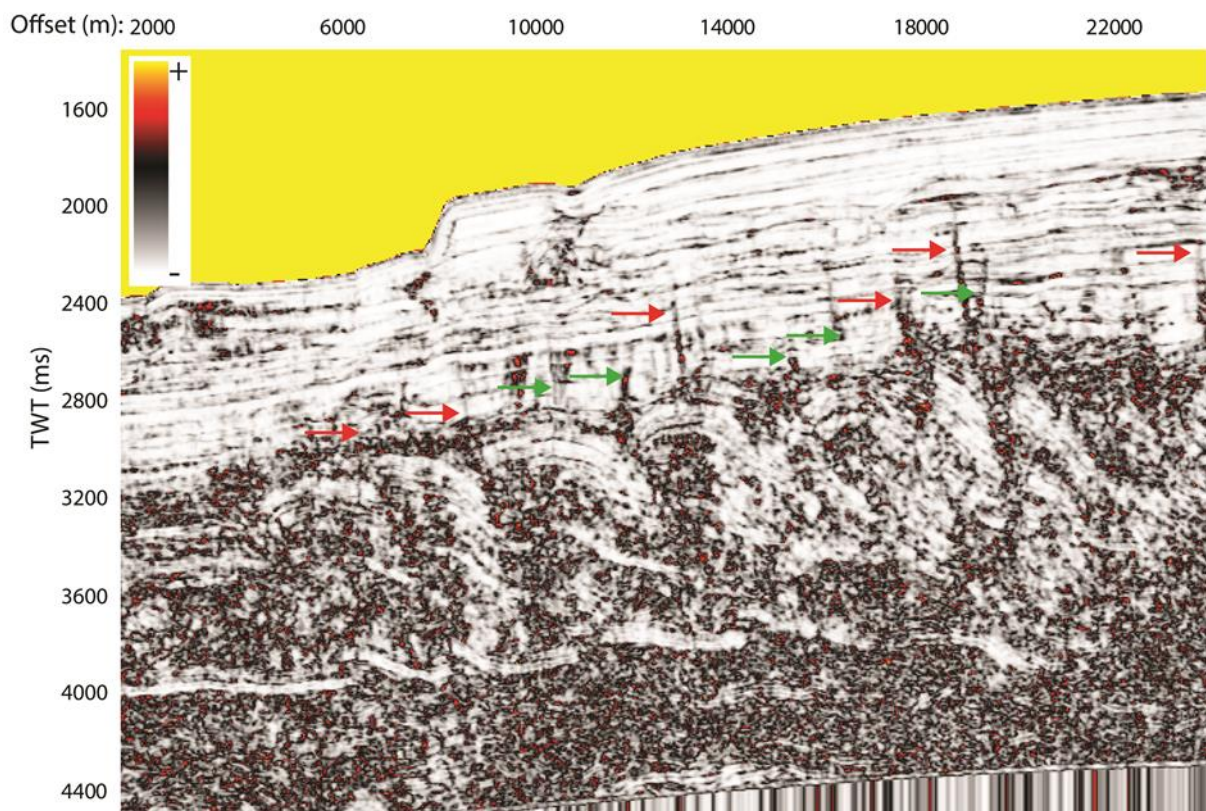
Figure 5.13. Chaos attribute applied to inline 15648 prior to ant tracking computation. The red and green arrows indicate normal faults, with fault displacement below the vertical resolution limit of 12 m, which were enhanced by the chaos attribute. Vertical exaggeration (VE) of the section is 7:1.
