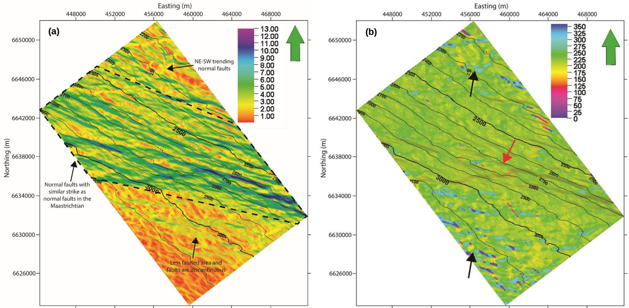
Figure 5.11. (a) A dip map of the base of the Palaeogene horizon illustrating a dense fault network trending WNW-ESE with varying dip angles along the faults in the central region of the study area (indicated by the dashed polygon). To the north, the faults are disconnected and they have a more NE-SW trend. To the south, there is less faulting and the faults are discontinuous. (b) A dip azimuth map of the base of the Palaeogene horizon illustrating faults dipping SW-WSW in the central region of the study area (indicated by the red arrow). In the northern and southern regions, the faults are dipping predominantly N to NW (indicated by the black arrows). The contour interval for (a) and (b) is 100 m.
