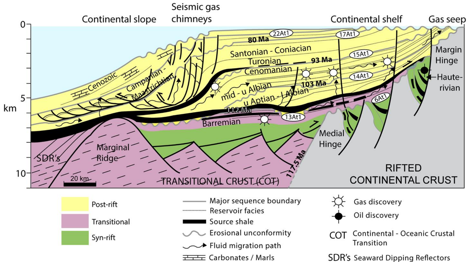
Figure 2.2. A schematic stratigraphic cross-section through the Orange Basin depocentre indicating the basin structure, sedimentary sequences and source rock intervals. 6At1, 13At1, 14At1, 15At1, 17At1 and 22At1 represent type-1 unconformities or subaerial unconformities classified by Brown et al. (1995) . 6At1 (drift onset unconformity); 13At1 (Mid-Aptian unconformity); 14At1 (Albian unconformity); 15At1 (Cenomanian unconformity); 17At1 (Maastrichtian unconformity) and 22At1 (Palaeogene unconformity) (modified from Jungslager, 1999 ).
