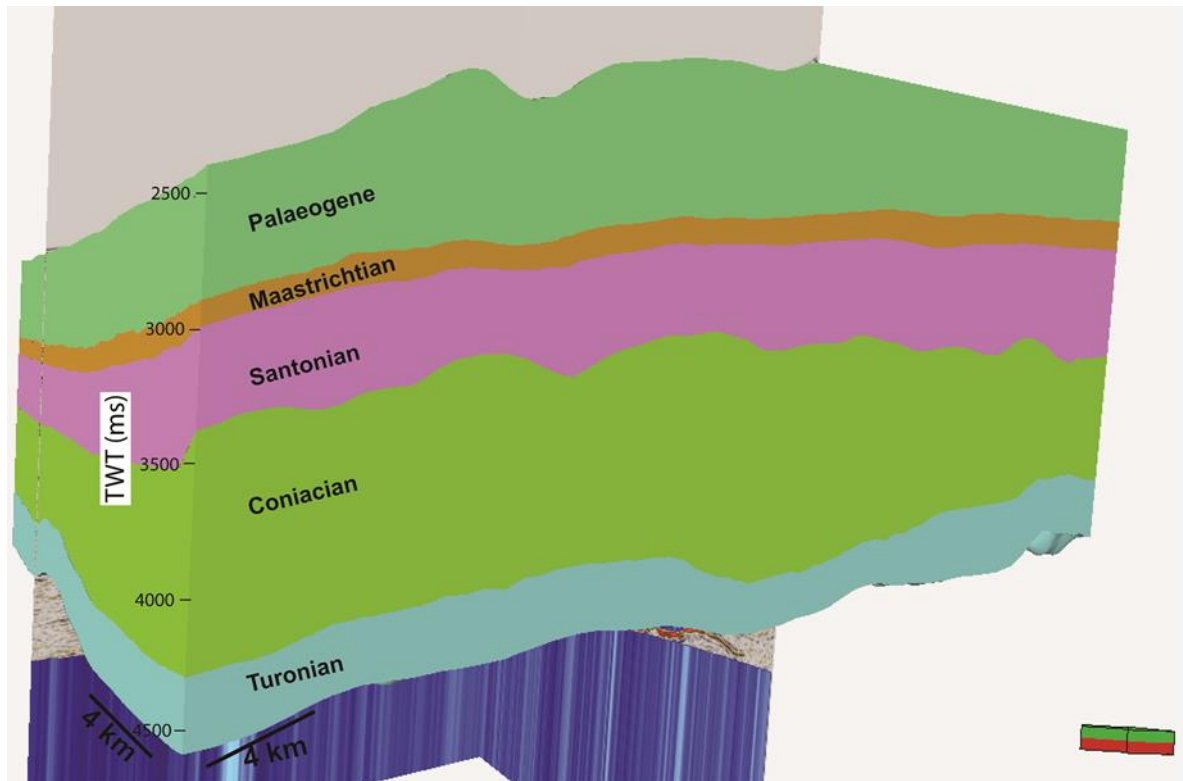
Figure 4.14. Horizons are intersected with the fault framework to create solid model. The model is divided into five zones.
