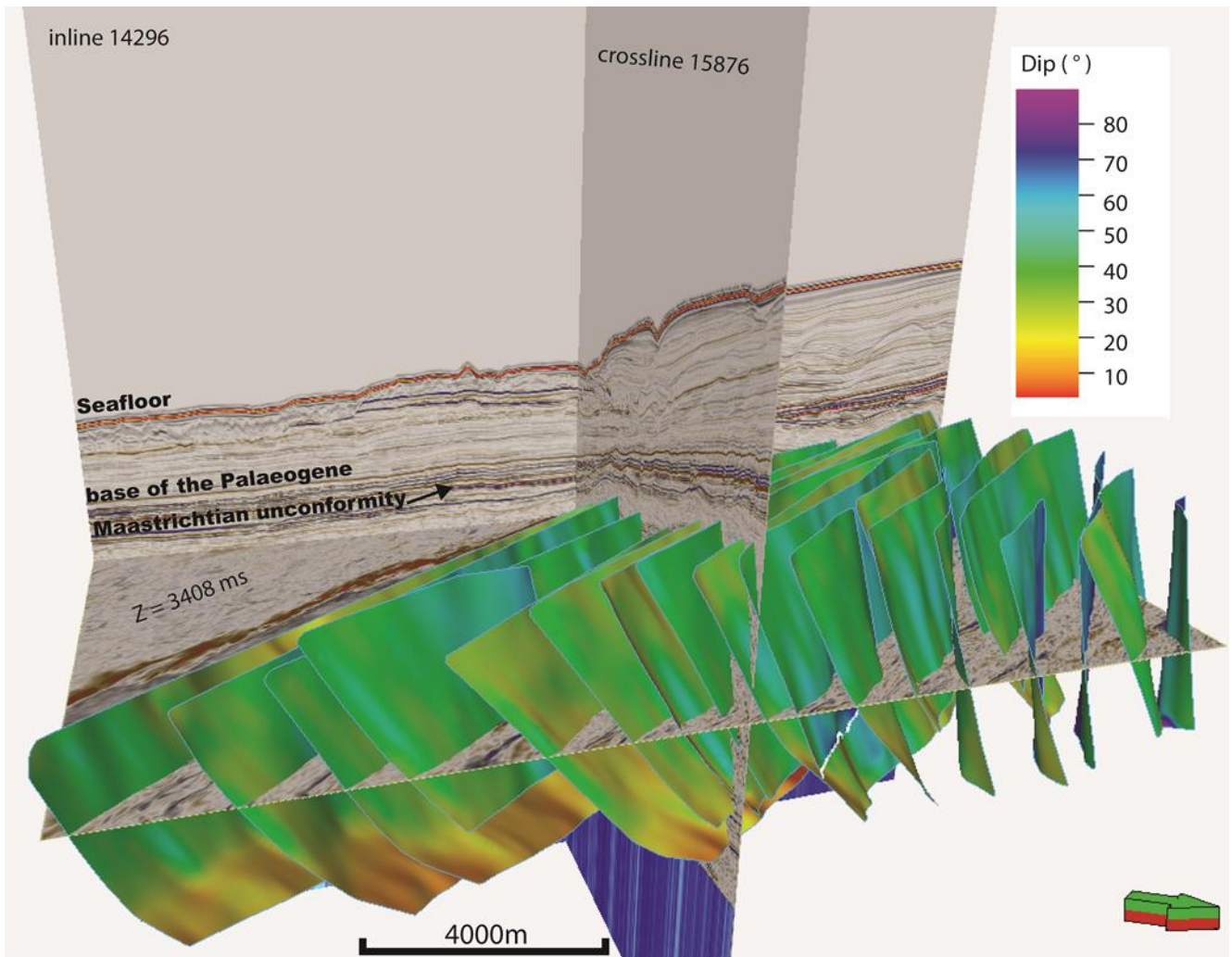
Figure 5.5. A 3D model of the thrust fault system showing variations in dip angle with depth and to the north, the faults dip steeply. The faults in the south, along the deformation front, have dip angles between 30° and 40°, and shallow to 10° with depth. In the north, the faults are dipping at high angles (60° - 70°). The vertical exaggeration (VE) is 5:1.
