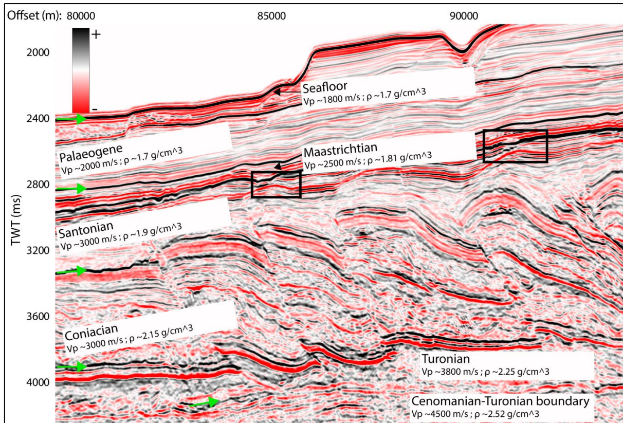
Figure 4.3. An amplitude display seismic section showing velocities (m/s) and densities ( \text{g/cm}^3 ) of the stratigraphic units. The green arrows indicate the picked interfaces that produce strong reflections. The Cenomanian-Turonian boundary is discontinuous. The black boxes highlight areas where reflectors terminate below the Maastrichtian unconformity. The vertical exaggeration (VE) of the section is 8: 1.
