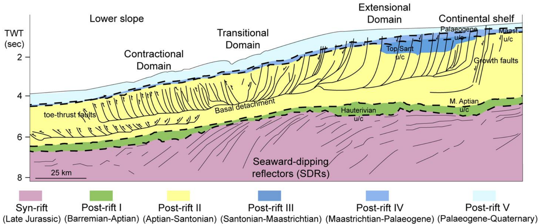
Figure 2.3. A schematic cross-section illustrating the main post-rift sequences (I-V) and the Cretaceous gravity-driven system in post-rift sequence II. The gravity-driven system is characterised by landward-dipping thrust faults and basinward-dipping growth faults that sole into a common detachment. u/c represents unconformity. The Santonian is abbreviated as Sant and the Maastrichtian as Maast (modified from de Vera et al., 2010 ).
