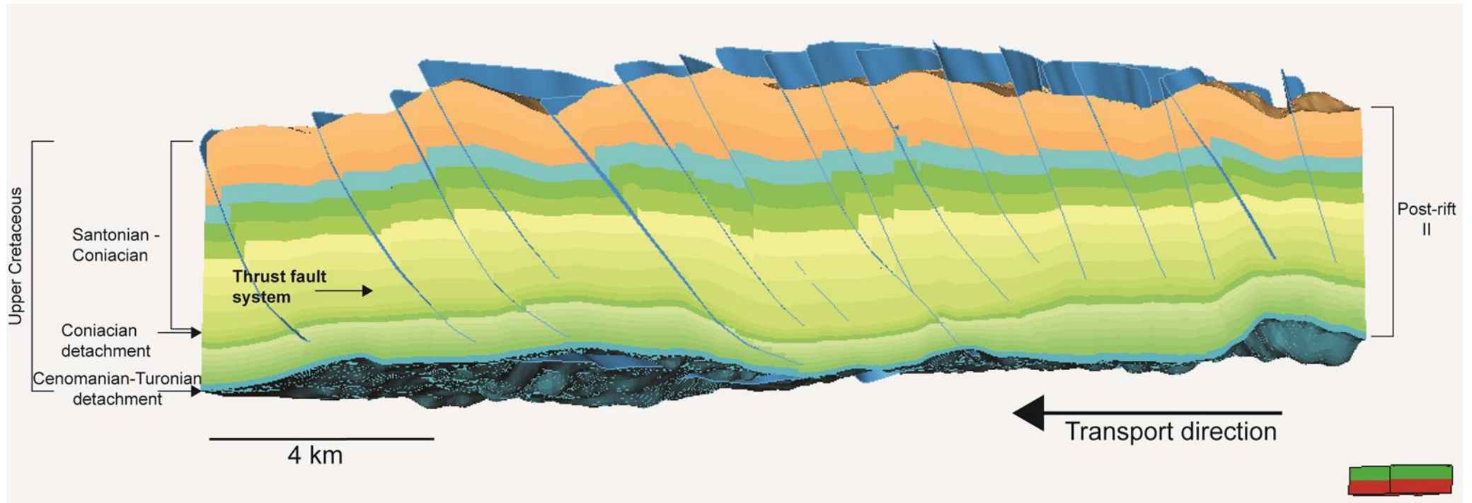
Figure 7.1. 3D model showing landward-dipping thrust faults becoming slightly curved as they attach to the Cenomanian-Turonian detachment. The thrust faults that connect to the Coniacian detachment maintain a planar geometry. The full 3D model animation can be viewed in the attachment.
