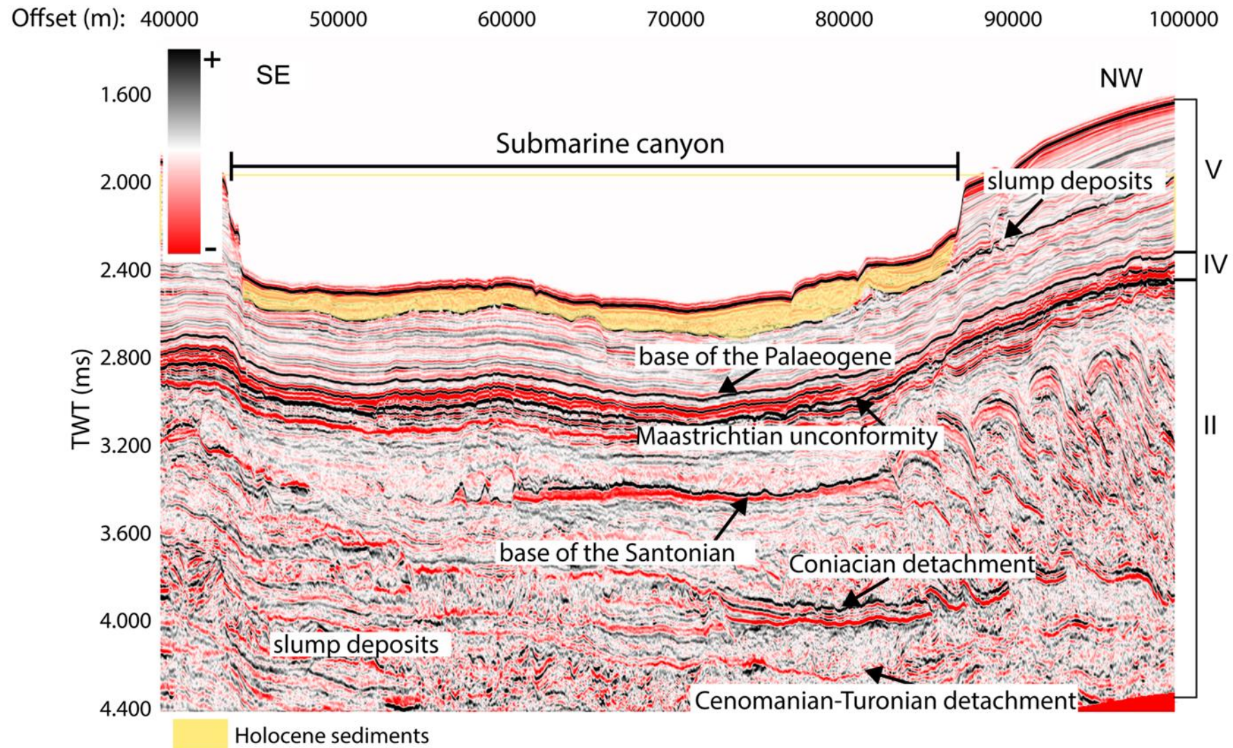
Figure 6.4. An amplitude display seismic section illustrating the structures imaged in the deepwater Orange Basin. The submarine canyon is formed above the deformation front of the thrust fault system. It has a width of 45 km and is incised to depths of approximately 650 m. The vertical exaggeration (VE) of the section is 17:1.
