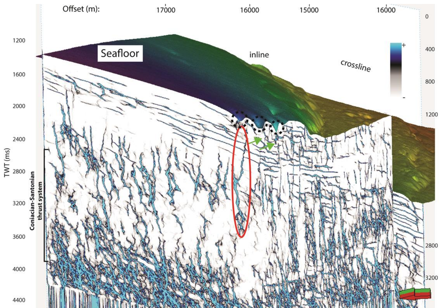
Figure 6.3. Ant tracked volume with stereonet filter applied to detect fault with a S-WSW dip direction. The green arrows indicate the termination of the S-WSW dipping normal faults below pockmarks. The red ellipse shows the connectivity between thrust fault and normal fault that propagated to the surface beneath the pockmarks (marked by black dashed circles). Vertical exaggeration (VE) is 7:1.
