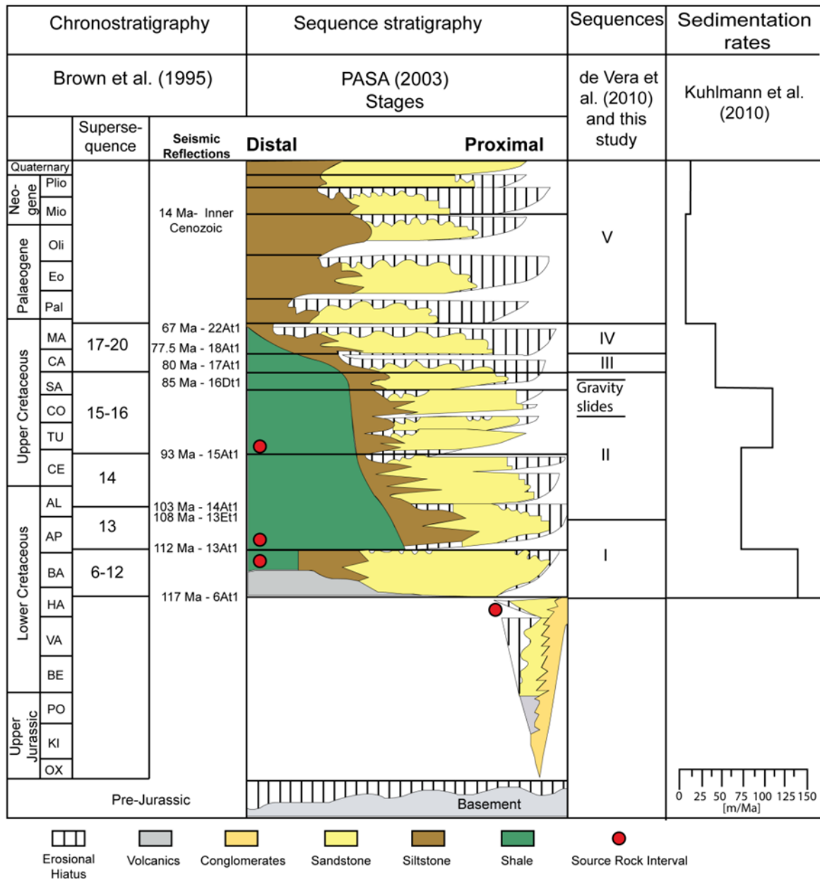
Figure 5.1. Chronostratigraphic and sequence chart for the Orange Basin illustrating major stratigraphic units and sedimentation rates. Stratigraphic units below the red line were cut from the seismic volume. 6-12, 13, 14, 15-16, 17-20 represent supersequences classified by Brown et al. (1995) . OX (Oxfordian); KI (Kimmeridgian); TI (Tithonian); BE (Berriasian); VA (Valanginian); HA (Hauterivian); BA (Barremian); AP (Aptian); AL (Albian); CE (Cenomanian); TU (Turonian); CO (Coniacian); SA (Santonian); CA (Campanian); MA (Maastrichtian); Pal (Palaeocene); Eo (Eocene); Oli (Oligocene); Mio (Miocene) and Plio (Pliocene). I – V represents the classification by de Vera et al. (2010) used to group sequences from the Hauterivian to Holocene (modified from Boyd et al., 2011 ; Loefering et al., 2013 ).
