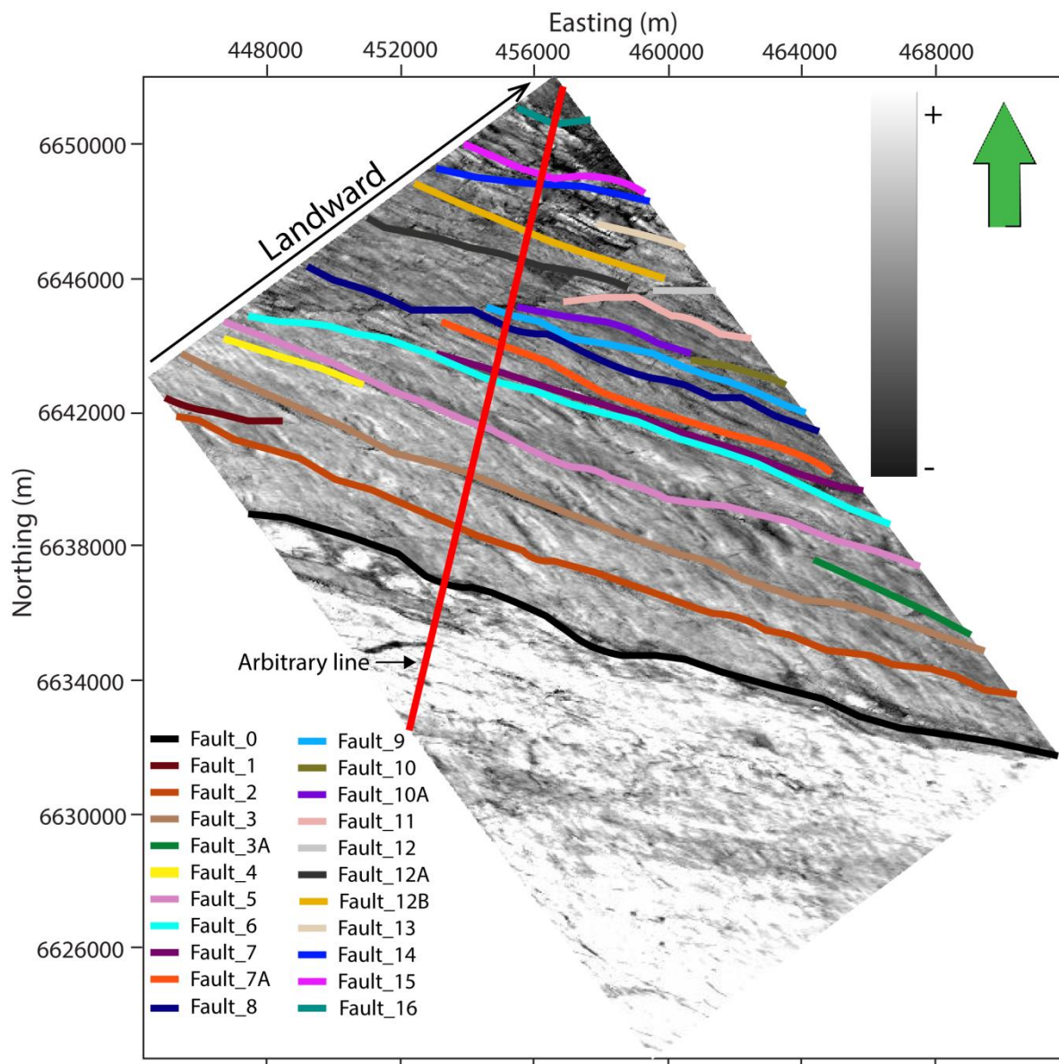
Figure 5.7. An elevation map of the horizon located at the top of the thrust fault system (base of the Santonian) (highlighted in Figure 5.6) with an overlay of thrust fault polygons. The faults are trending WNW-ESE. The red line represents an arbitrary line presented in Figure 5.9.
