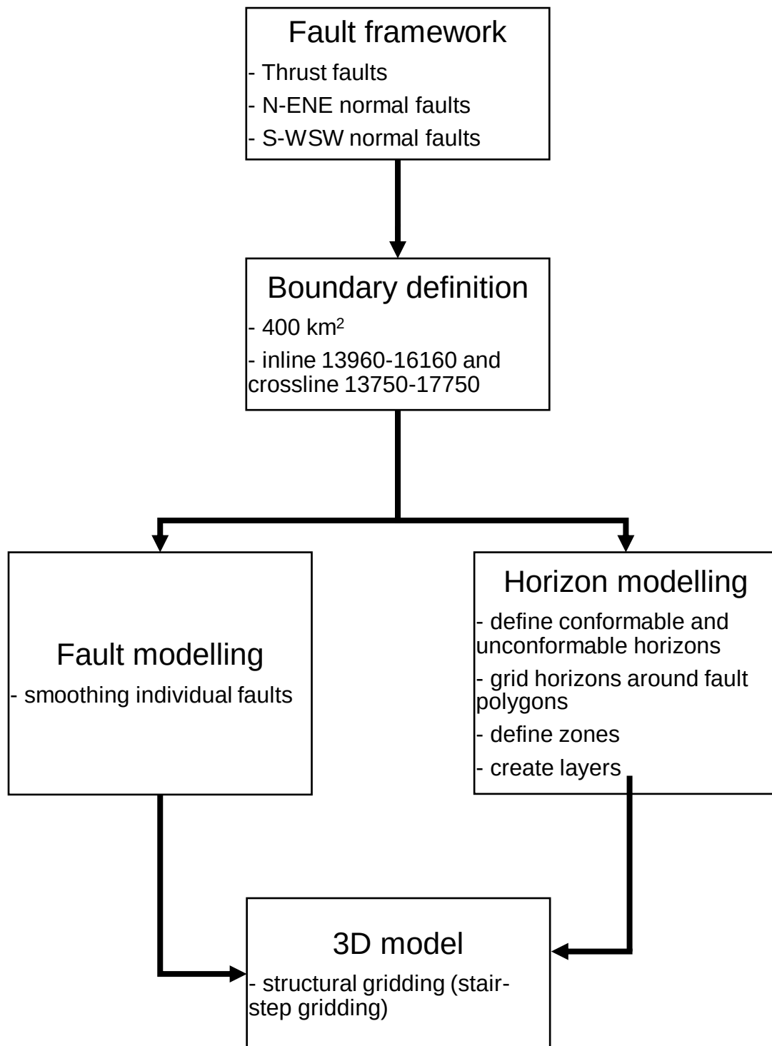
Figure 4.16. Workflow used to construct a 3D geological model of the deepwater Orange Basin.
