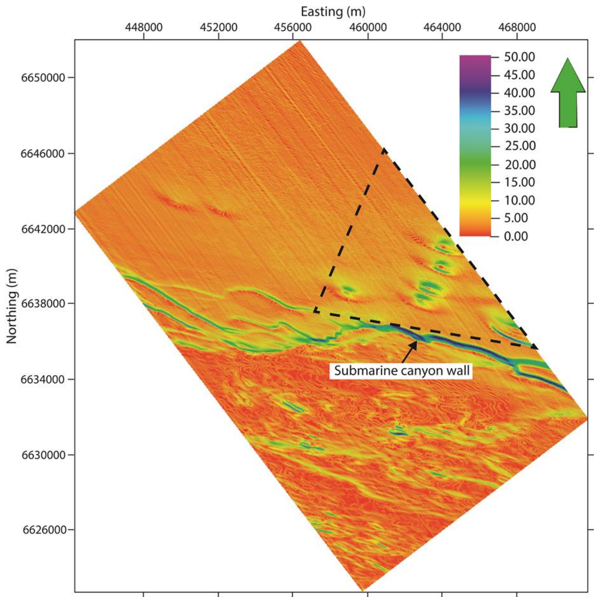
Figure 6.5. A dip map of the seafloor horizon highlighting the dip of the canyon wall and pockmarks, in the area marked by the dashed polygon.
