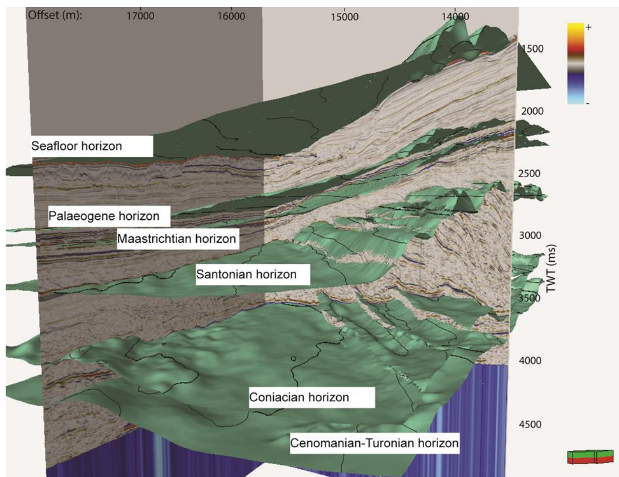
Figure 4.13. 3D seismic volume overlain with gridded horizons. The contour interval is 50 m. Vertical exaggeration (VE) is 7:1.
