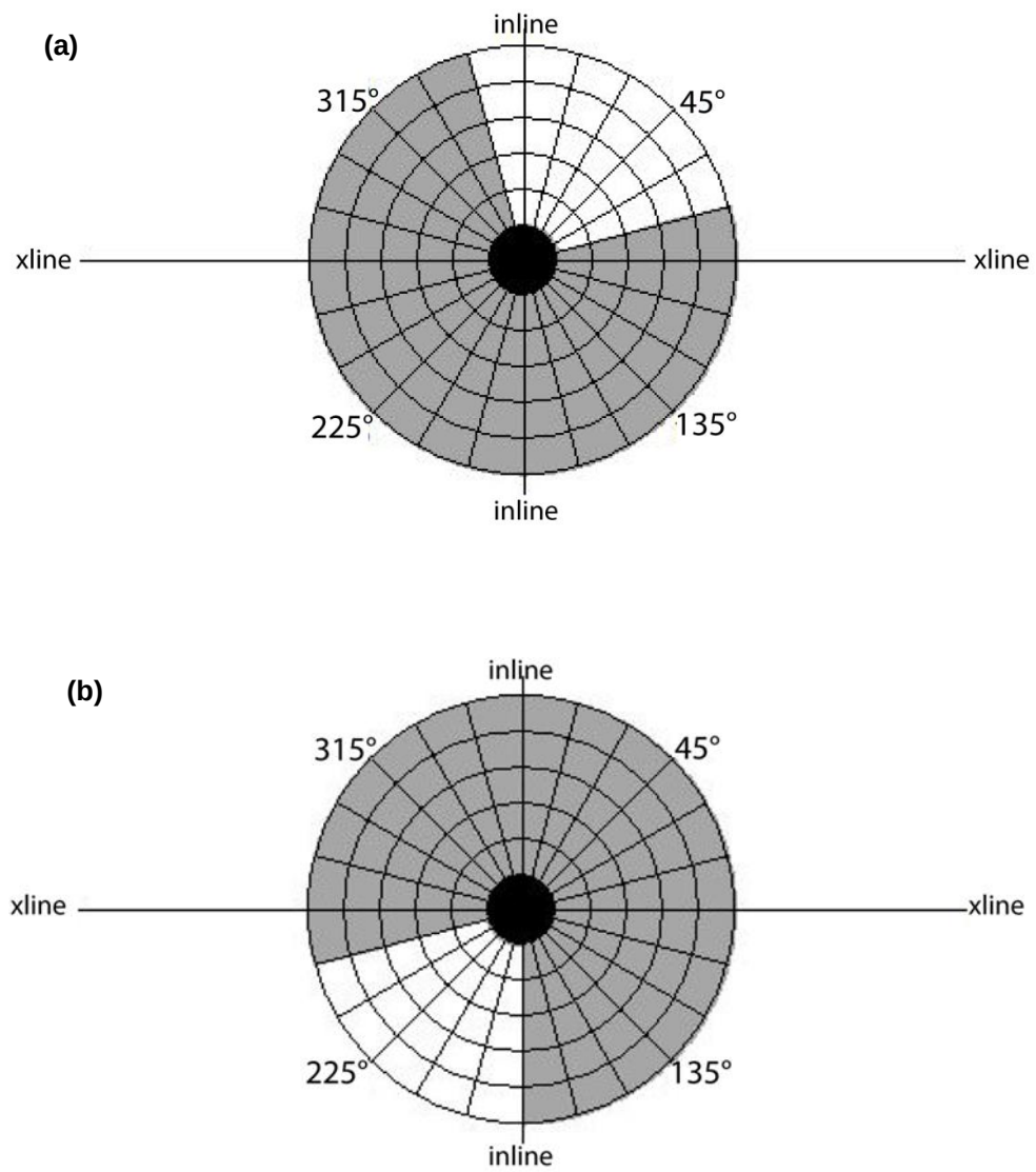
Figure 4.9. Stereonet filters used to compute ant tracking seismic cube. (a) Stereonet for normal faults dipping at 0°-90° N to ENE (b) Stereonet for normal faults dipping at 0°-90° S to WSW.
