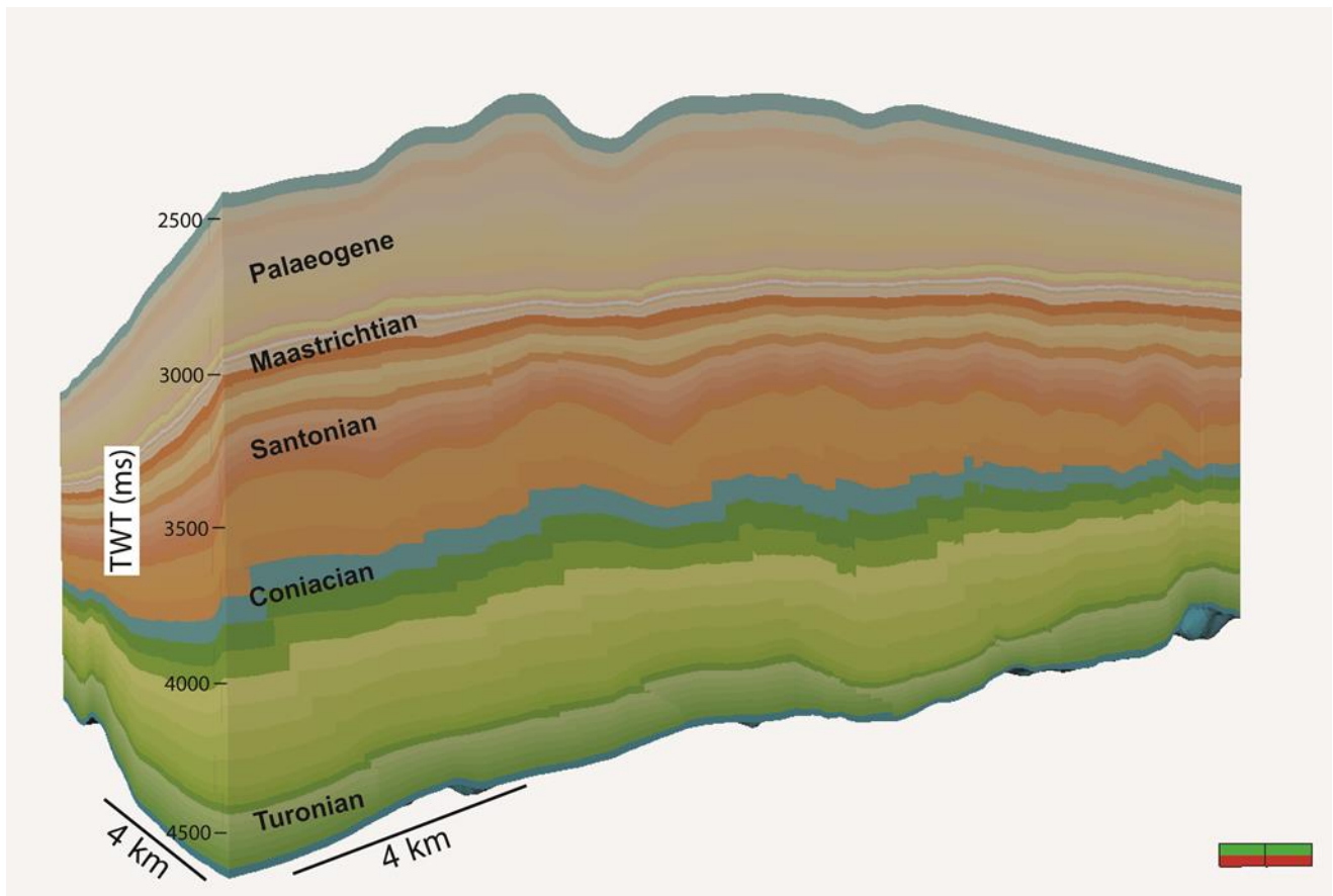
Figure 4.15. 3D model showing layering and displacement of layers due to faulting.
