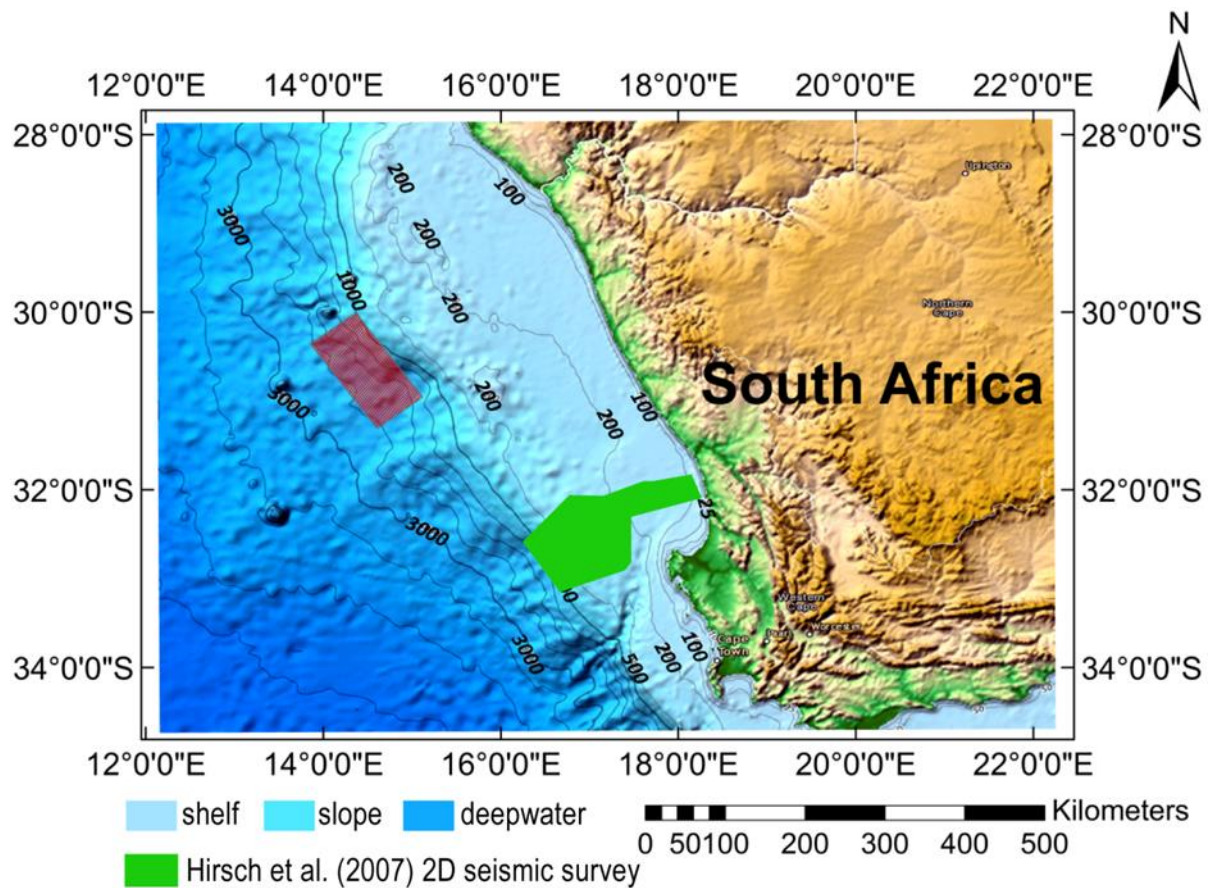
Figure 4.1. Bathymetric map superimposed with the deepwater Orange Basin licence area indicated by the red polygon. The study area covers approximately 8200 km 2 . The green polygon shows the 2D seismic survey used in a study by Hirsch et al. (2007) . Borehole data used to calculate the densities of the rocks are found within the green polygon (basemap sourced from the National Oceanic and Atmospheric Administration , https://maps.ngdc.noaa.gov/viewers/bathymetry , March, 2017)
