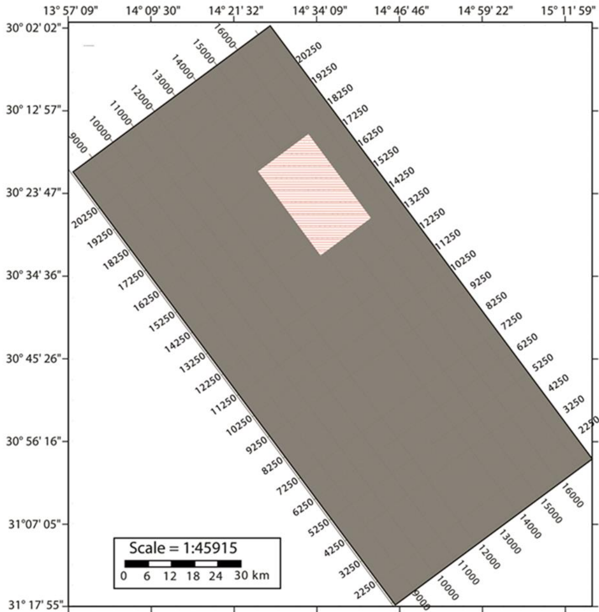
Figure 4.2. A survey map of the deepwater Orange Basin licence area showing inlines (parallel to acquisition direction) and crosslines (perpendicular to acquisition direction). The survey is 8000km 2 . The 400km 2 study area is highlighted by the red polygon.
