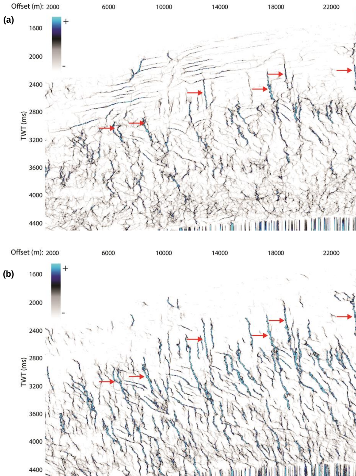
Figure 5.14. Ant tracked sections of inline 15648. These sections show the (a) first run and (b) second run of the ant tracking algorithm limited to detecting fault with a N to ENE dip direction and dip angles between 0^{\circ} and 90^{\circ} . A number of faults have been highlighted by the attribute. The faults marked by the red arrows are difficult to see on the amplitude seismic display. Section (a) and (b) are vertically exaggerated by a factor of 7.
