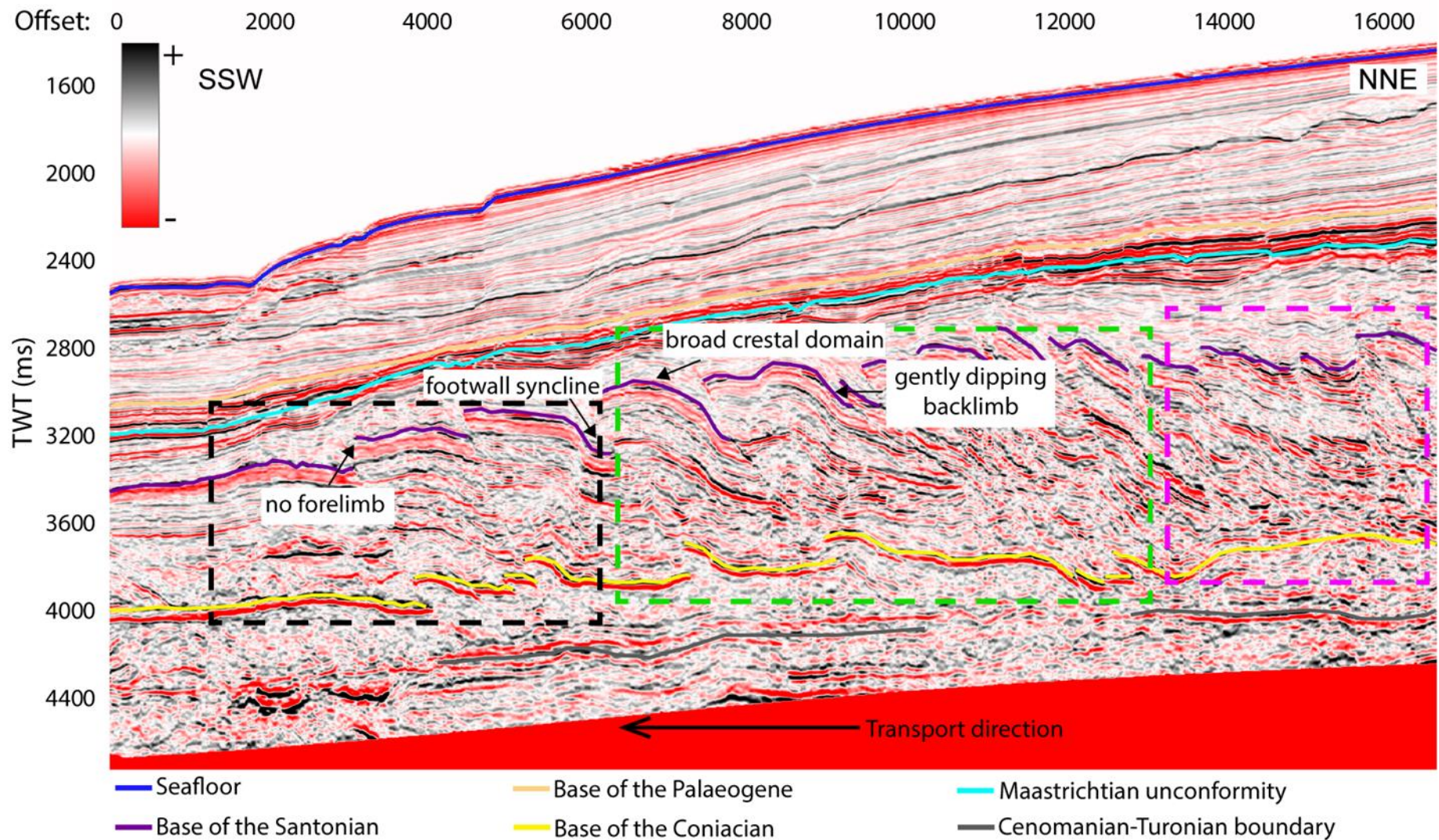
Figure 5.9. An amplitude display seismic section showing the geometry of the folds. The folds are asymmetric with backlimbs that dip gentler than the fault ramp. The backlimbs dip approximately 4^{\circ} – 24^{\circ} . The thrust faults cut through the forelimbs of the folds and the footwall synclines. The area to the north is structurally complex and highly deformed compared to the south. The black block highlights faults along the deformation front; green block highlights faults in the inner part of thrust fault system and pink block shows faults at the rear of the system. Vertical exaggeration (VE) of the section is 3:1
