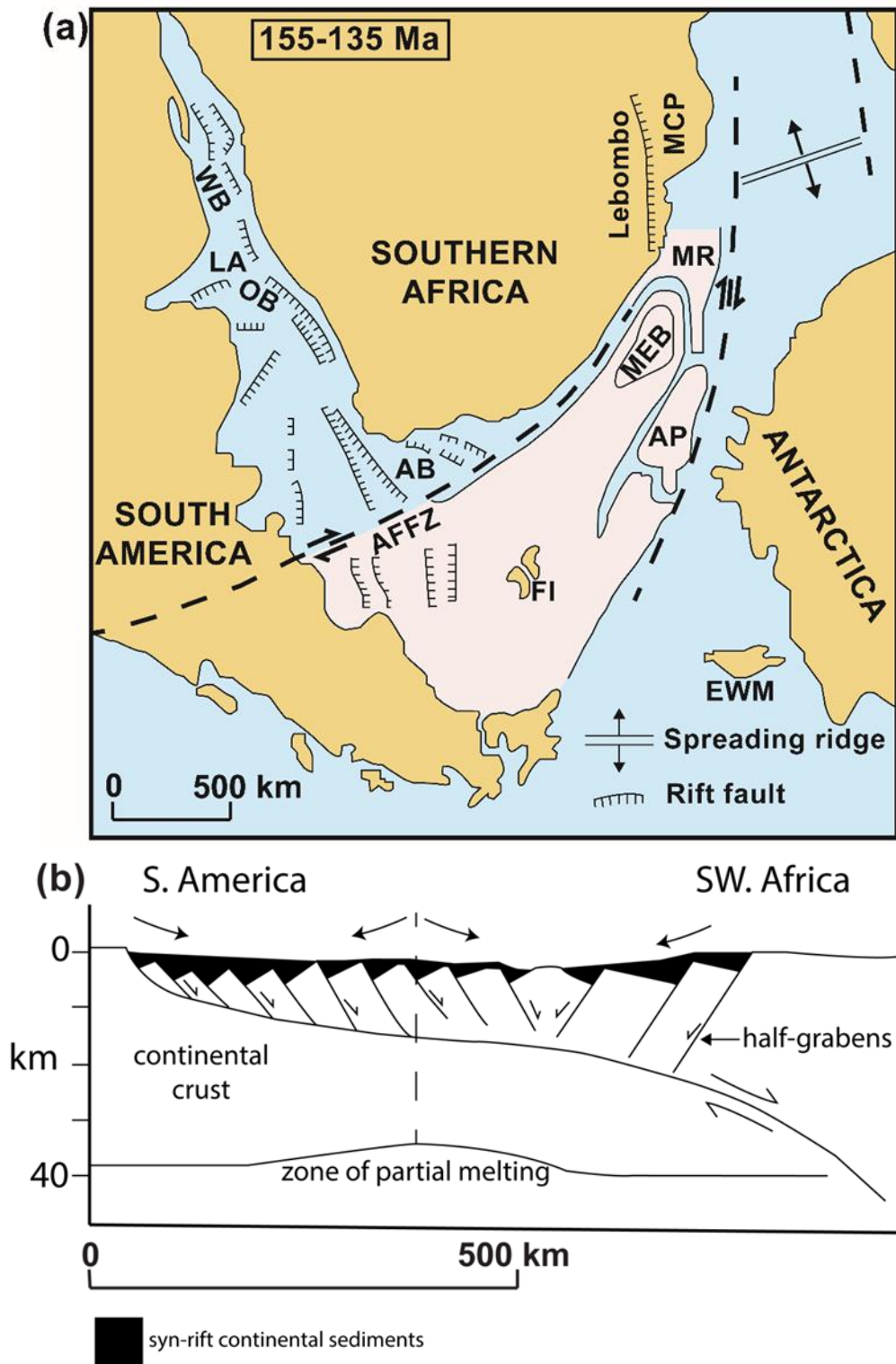
Figure 1.1. (a) Tectonic plate reconstruction illustrating rifting of South America and Africa at 155 Ma to 135 Ma. AB (Agulhas Bank); AFFZ (Agulhas-Falkland Fracture Zone); AP (Agulhas Plateau); EWM (Ellsworth Island); FI (Falkland Islands); LA (Luderitz Arch); MCP (Mozambique coastal plain); MEB (Maurice Ewing Bank); MR (Mozambique Ridge); OB (Orange Basin); WB (Walvis Basin) (after Watkeys, 2006 ). (b) A schematic diagram showing the formation of syn-rift basins in the South Atlantic. Black arrows indicate the direction of continental sediment movement (after Dingle, 1992 ).
