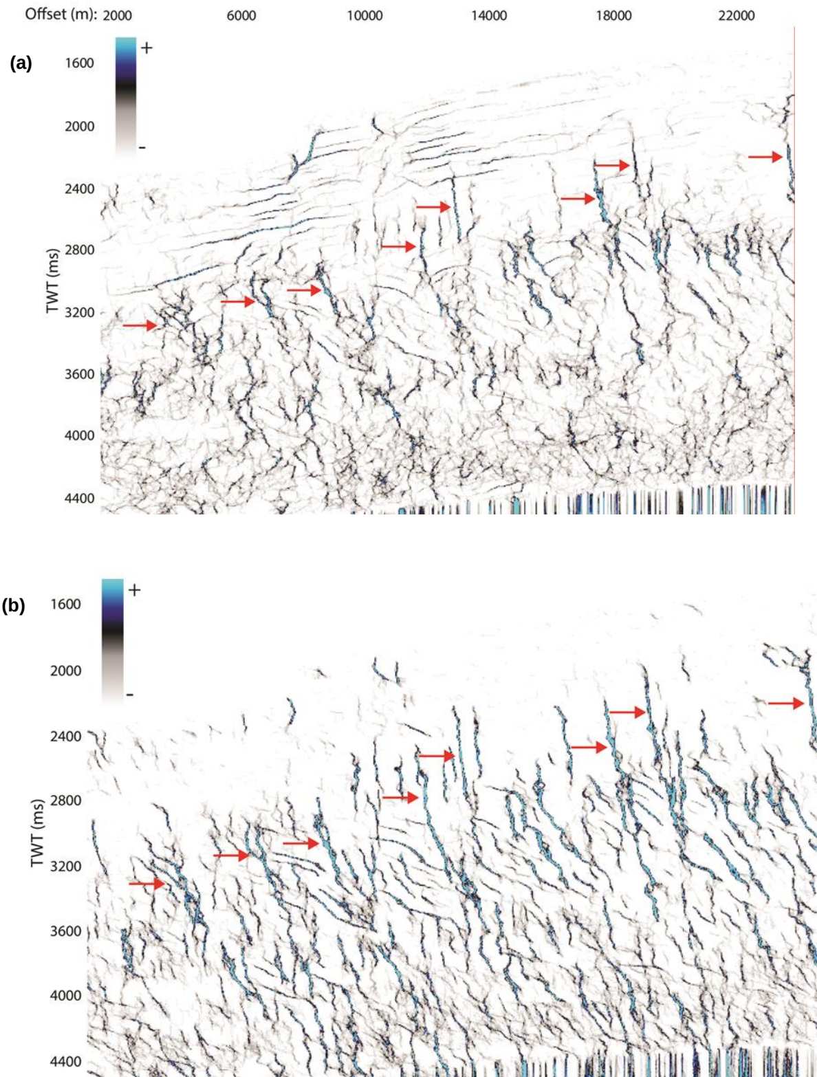
Figure 4.10. (a) An ant tracked volume of the first run with the stereonet filter applied to detect faults dipping N-ENE. The red arrows point to fault whose continuity is highlighted in the second run. (b) An ant tracked volume of the second run with the stereonet filter applied to detect faults dipping N-ENE. Sections (a) and (b) are vertically exaggerated by a factor of 7.
