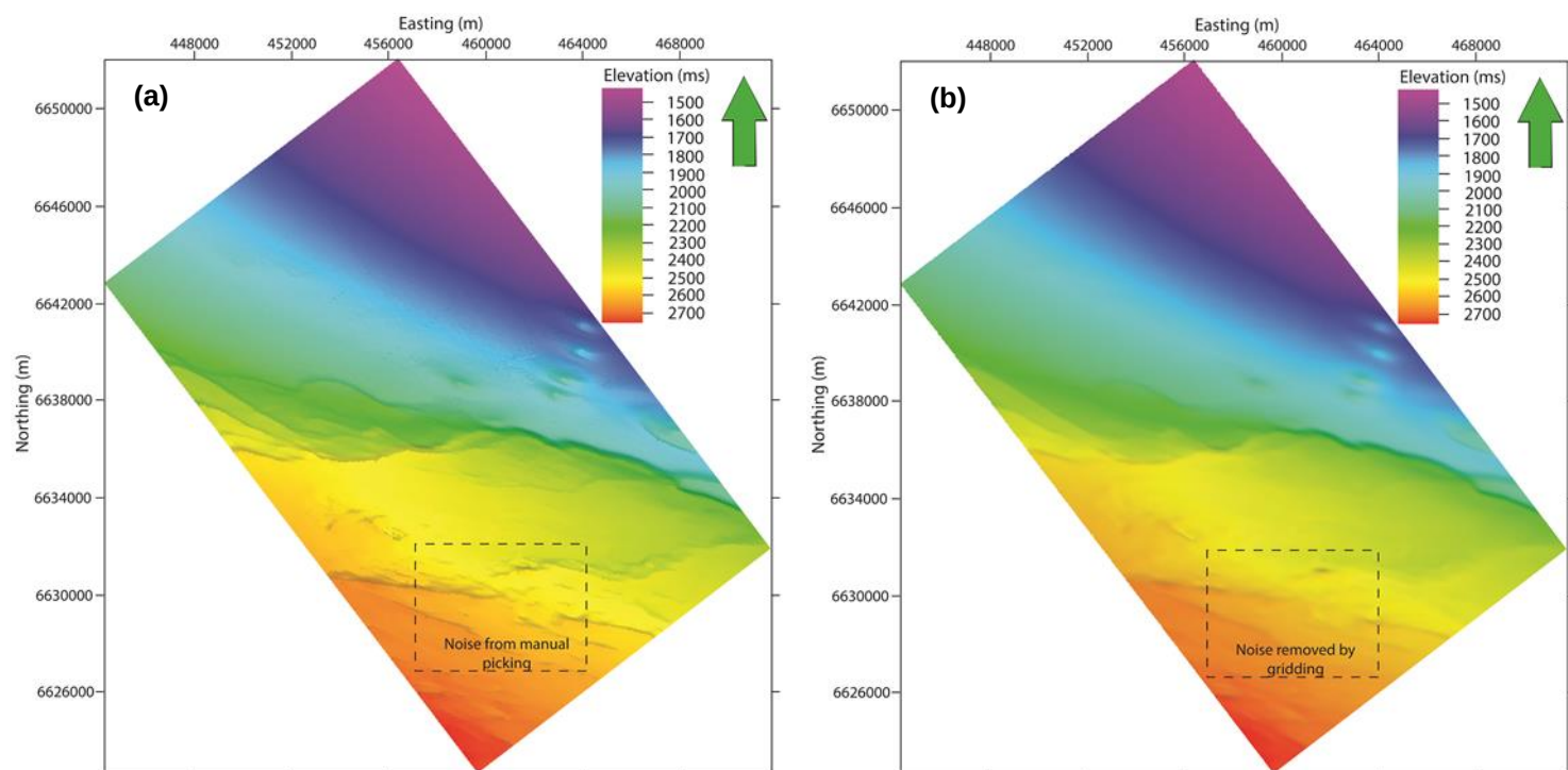
Figure 4.6. The seafloor horizon (a) before and (b) after smoothing using the Gaussian method. The dashed box highlights a structurally complex area where noise was generated by manual picking.
