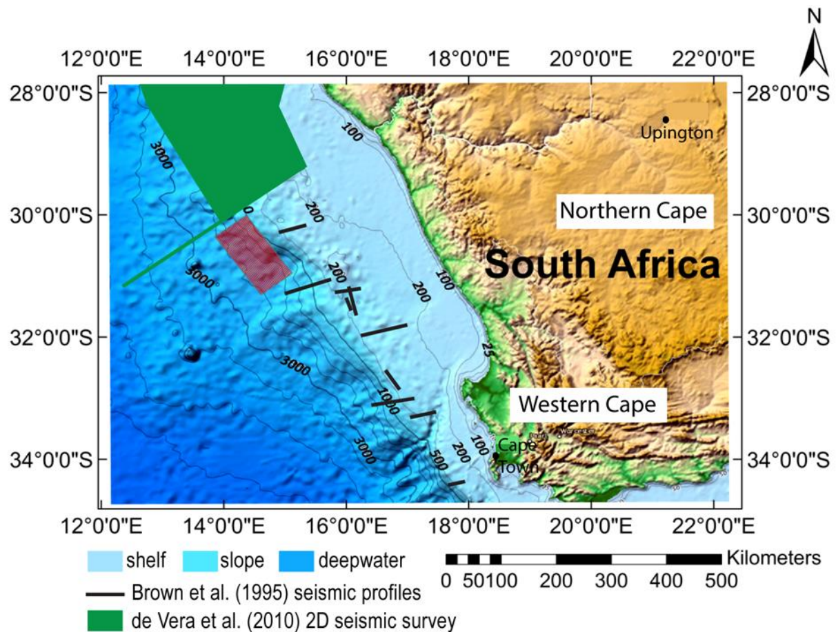
Figure 1.3. Bathymetric map superimposed with the deepwater Orange Basin 3D seismic grid shown by the red polygon. The study area covers approximately 8200 km 2 . Seismic profiles used in the study by Brown et al. (1995) are shown by the black lines. The green polygon shows the 2D seismic survey used in the study by de Vera et al. (2010). The green polygon extends out of the bathymetric map (basemap sourced from the National Oceanic and Atmospheric Administration, https://maps.ngdc.noaa.gov/viewers/bathymetry , March, 2017).
