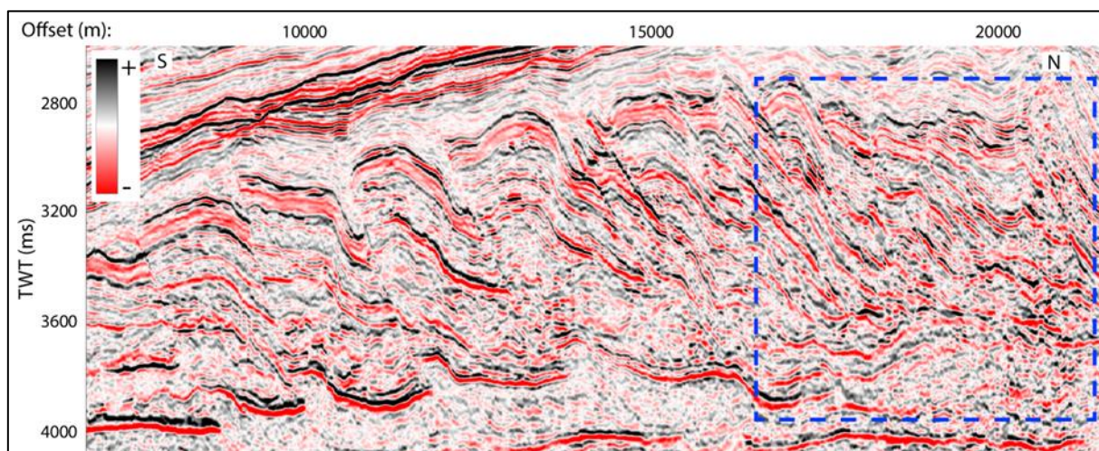
Figure 4.5. An amplitude seismic section showing the structurally complex area with low signal-to-noise ratio in the NE portion of the study area. This area is highlighted by the blue dashed box. The vertical exaggeration (VE) of the section is 8:1.
