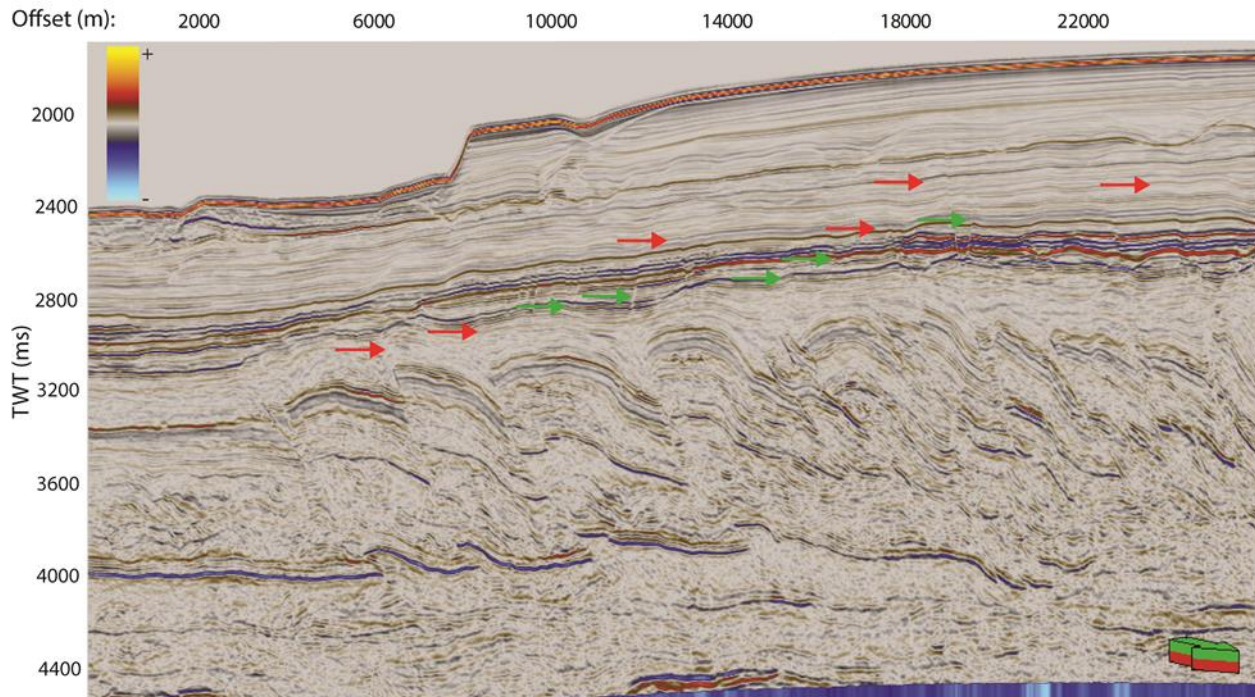
Figure 5.12. An amplitude display of inline 15648. A number of normal faults displace the Maastrichtian unconformity and base of the Palaeogene horizons. The faults indicated by the red and green arrows have displacement below the vertical resolution limit of 12 m, thus cannot be seen on the amplitude display. The vertical exaggeration (VE) of the section is 7:1.
