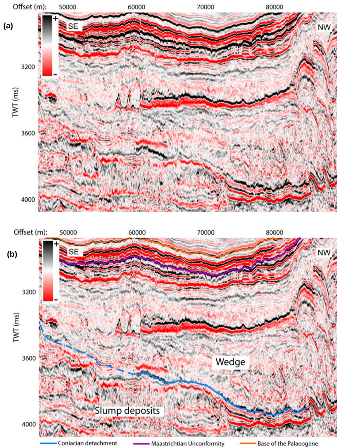
Figure 5.17. (a) Uninterpreted amplitude section. (b) Interpreted amplitude section showing the Coniacian detachment along the base of the wedge. The vertical exaggeration (VE) for (a) and (b) is 17:1
