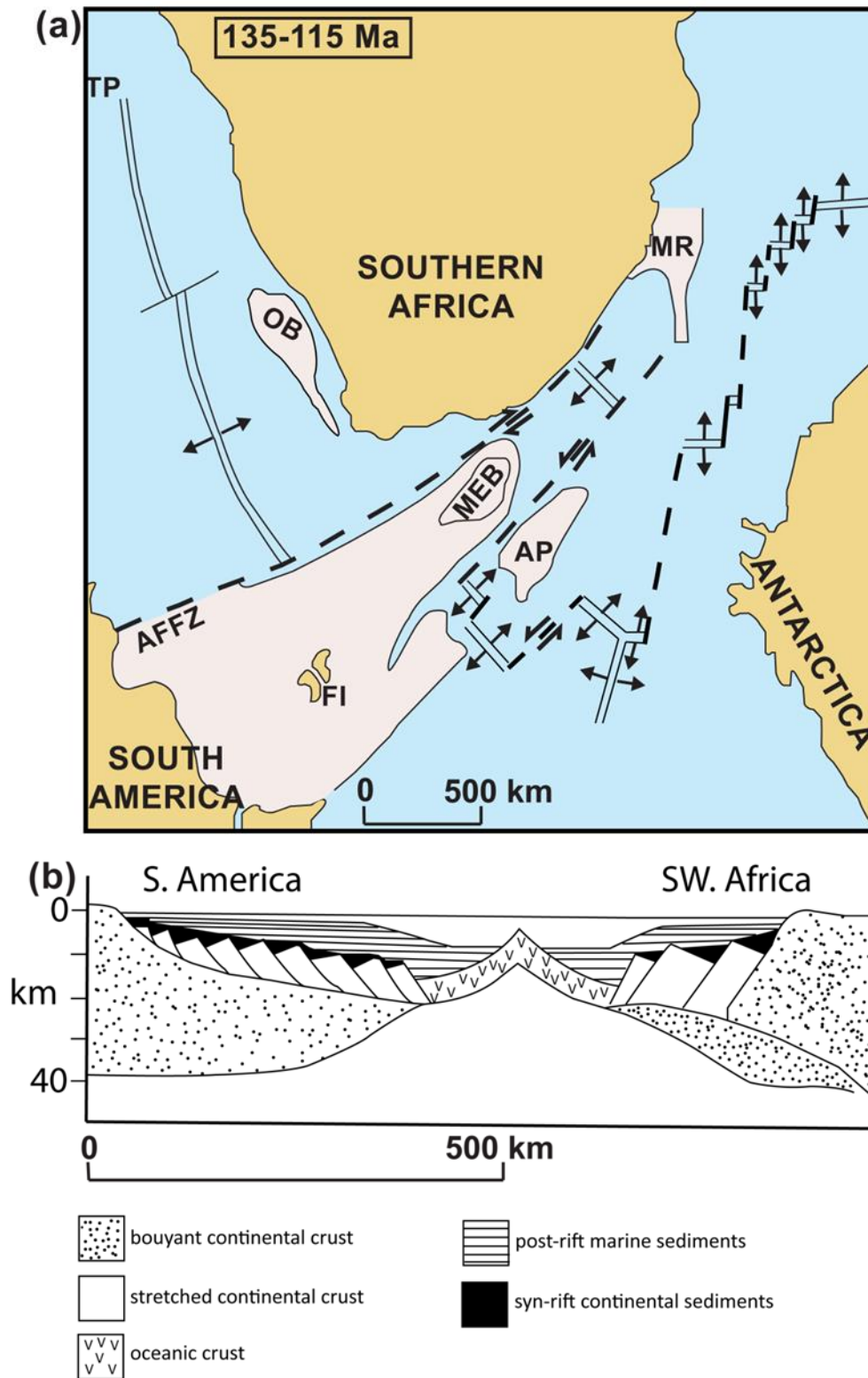
Figure 1.2. (a) Tectonic plate reconstruction illustrating drifting of South America from Africa and development of Southern Africa's passive margin. AFFZ (Agulhas-Falkland Fracture Zone); AP (Agulhas Plateau); FI (Falkland Islands); MEB (Maurice Ewing Bank); MR (Mozambique Ridge); OB (Orange Basin); TP (Tristan Plume) (after Watkeys, 2006 ). (b) A Schematic diagram showing the emplacement of continental flood basalts initiating the South Atlantic drift phase and subsequent deposition of marine sediments of the Orange Basin (after Dingle, 1992 ).
