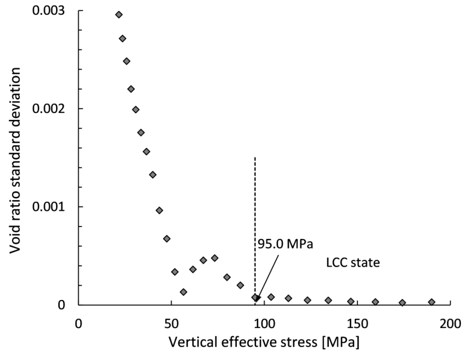
Fig. 4.18 LCC determination for the BI soil type.
