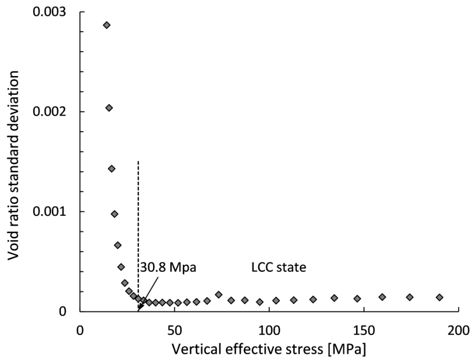
Fig. B.4 LCC determination for the SN soil type.
