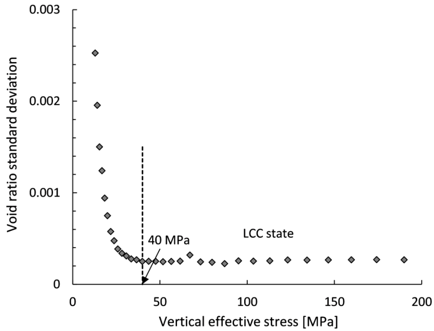
Fig. 3.19 LCC determination for the angular, broad PSD soil type.
