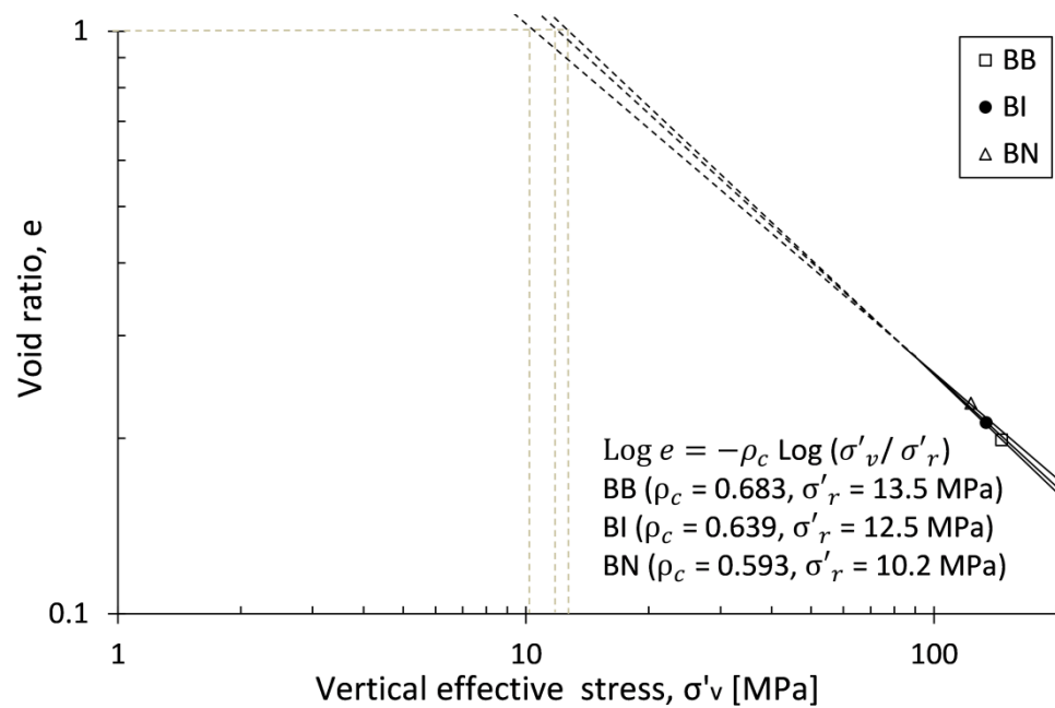
Fig. 4.22 Limiting compression curves of the beads soil types.
