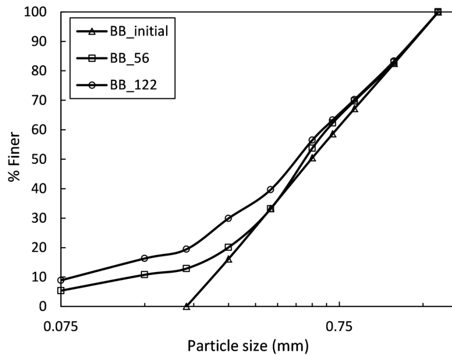
Fig. C.6 Pre and post-compression PSD curves of the BB soil type.
