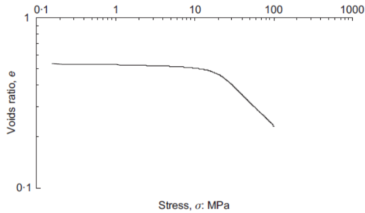
Fig. 2.4 A replot of Figure 2.3 in \log e - \log \sigma'_v space (McDowell, 2005).
