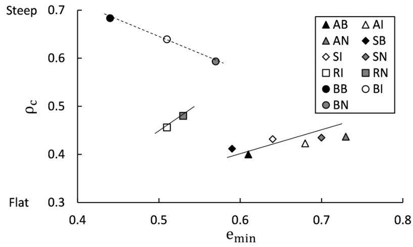
Fig. 5.6 Relationship between \rho_c and e_{\min} .
