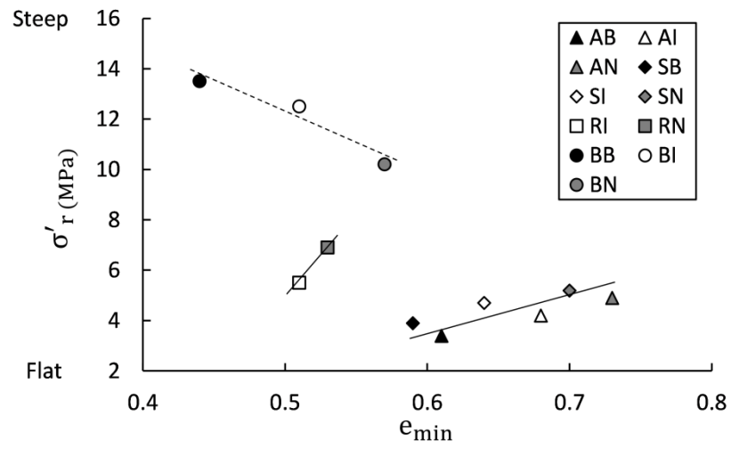
Fig. 5.8 Relationship between \sigma'_r and e_{min} .
