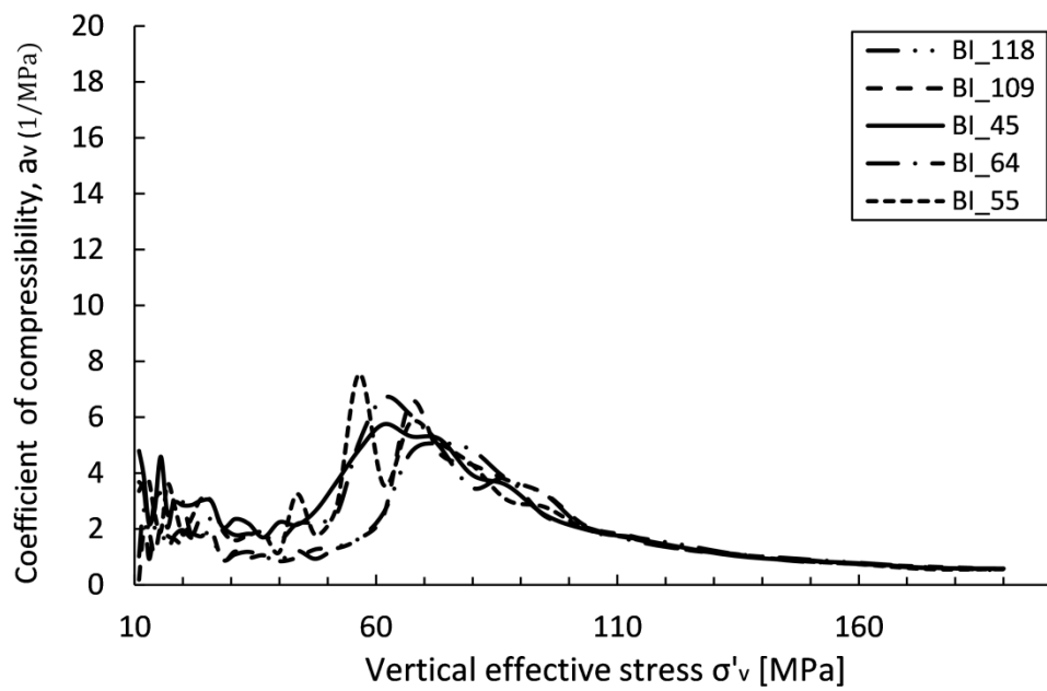
Fig. 4.9 Effect of initial relative density on compressibility for the BI soil type.
