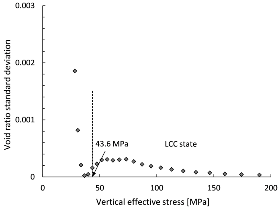
Fig. B.5 LCC determination for the RN soil type.
