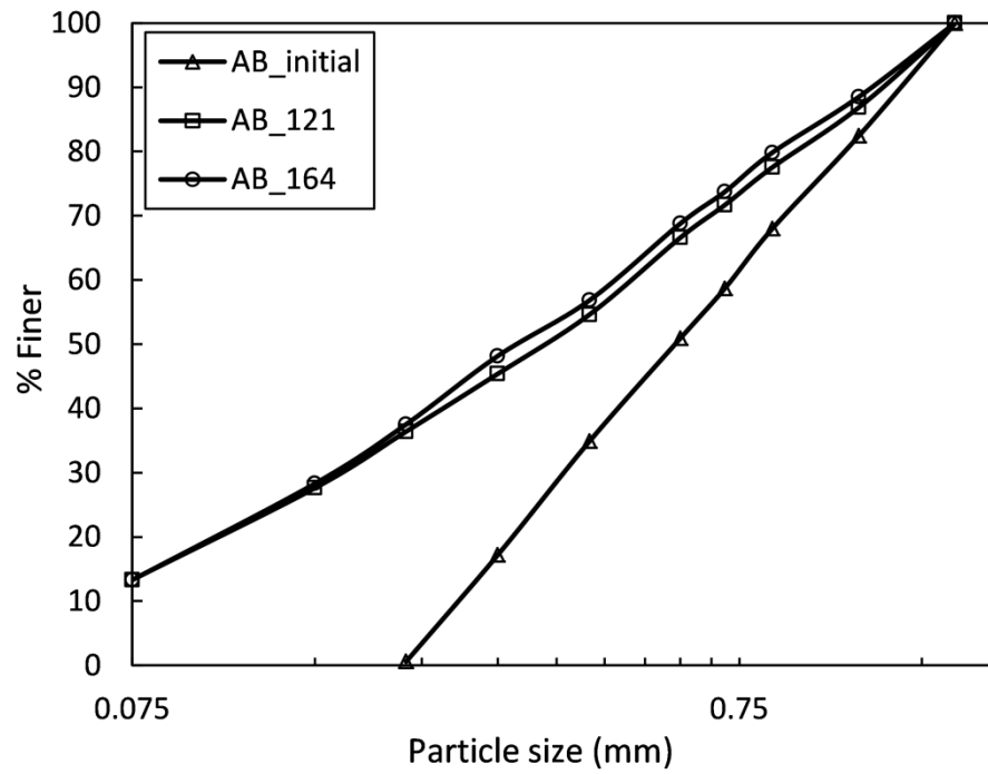
Fig. C.1 Pre and post-compression PSD curves of the AB soil type.
