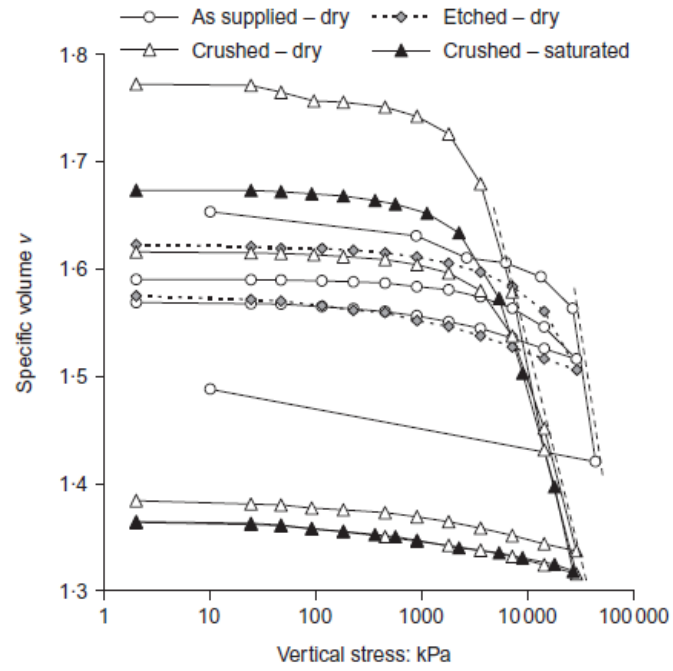
Fig. 2.8 1-D confined compression tests results of Cavarretta et al. (2010). ‘As supplied’ refers to the spherical glass ballotine particles.
