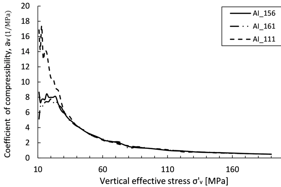
Fig. 4.6 Effect of initial relative density on compressibility for the AI soil type.
