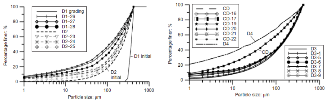
Fig. 2.5 PSD curves of Dog's bay sand. From narrowest to broadest gradation; D1, D2, D3 and D4, and CD (critical grading) (Altuhafi and Coop, 2011).
