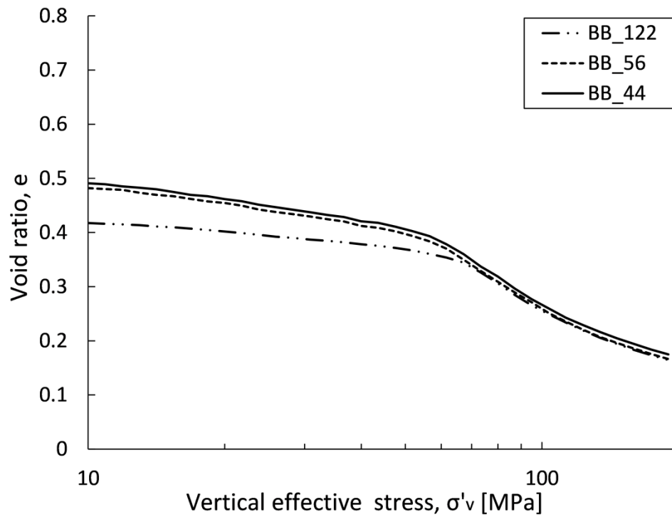
Fig. A.6 Beads broad soil type 1-D compression curves.
