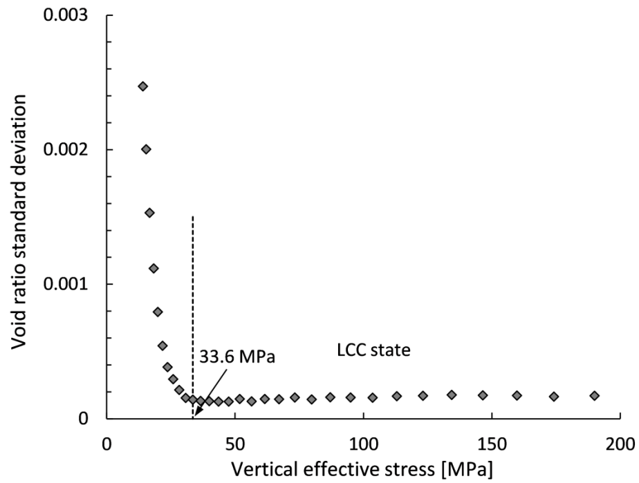
Fig. B.3 LCC determination for the SB soil type.
