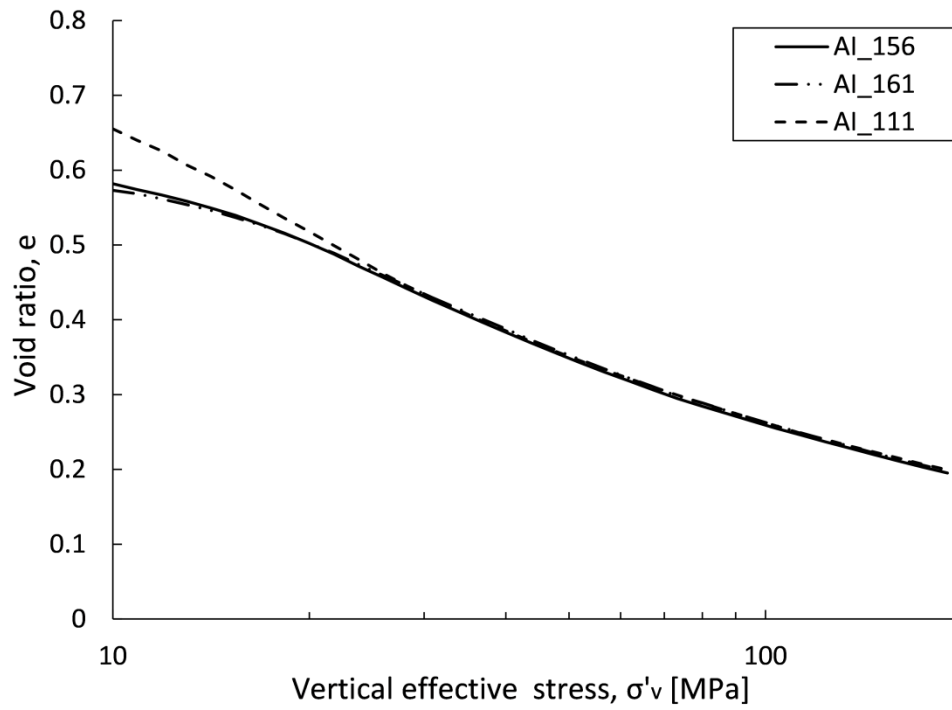
Fig. 4.2 AI soil type 1-D compression curves.
