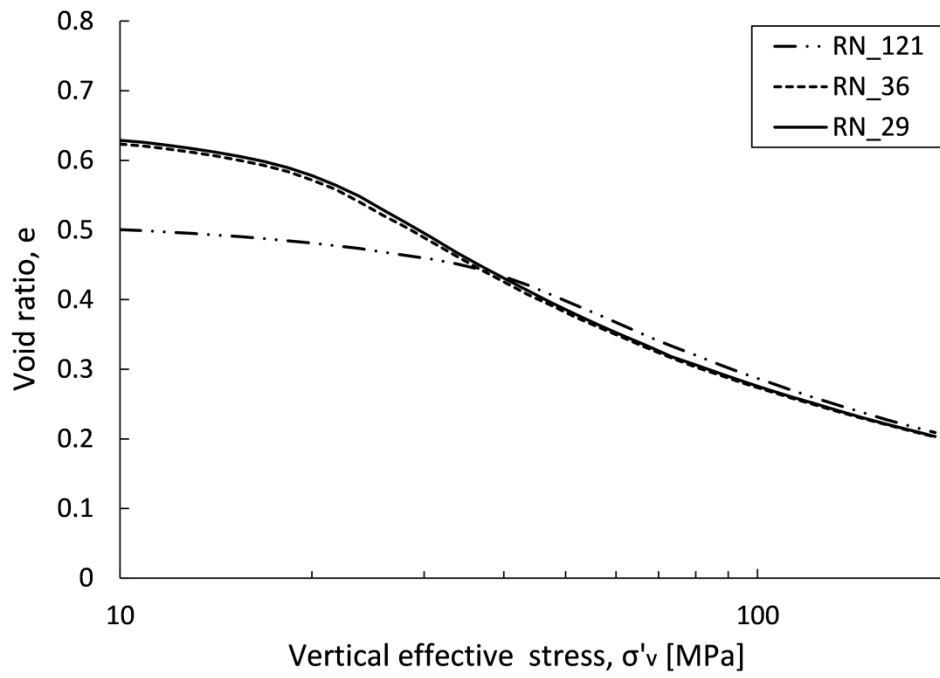
Fig. A.5 Rounded narrow soil type 1-D compression curves.
