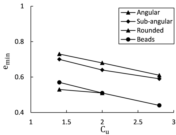
Fig. 3.13 Relationship between e_{\min} and PSD.
