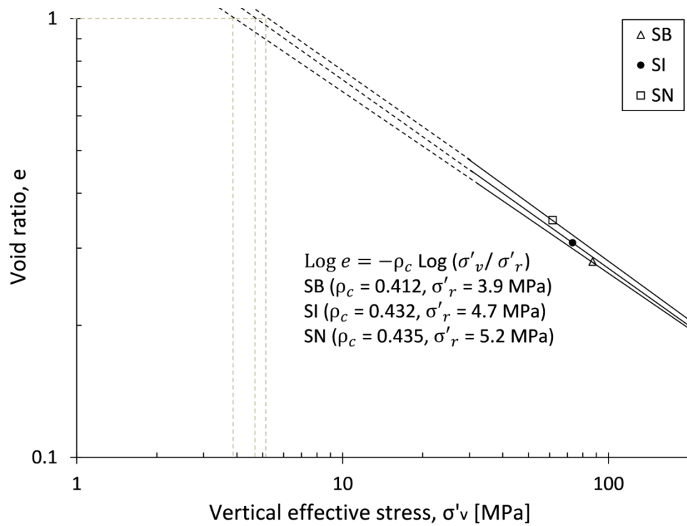
Fig. 4.20 Limiting compression curves of the sub-angular soil types.
