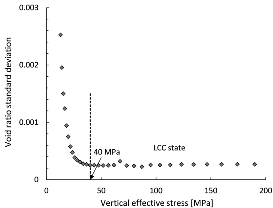
Fig. B.1 LCC determination for the AB soil type.
