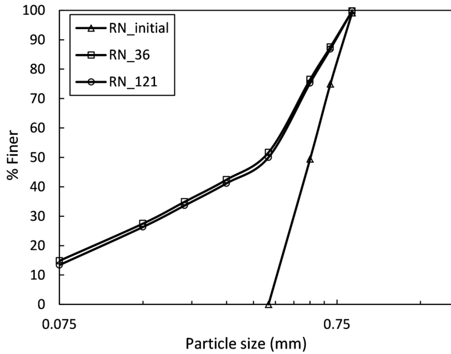
Fig. C.5 Pre and post-compression PSD curves of the RN soil type.
