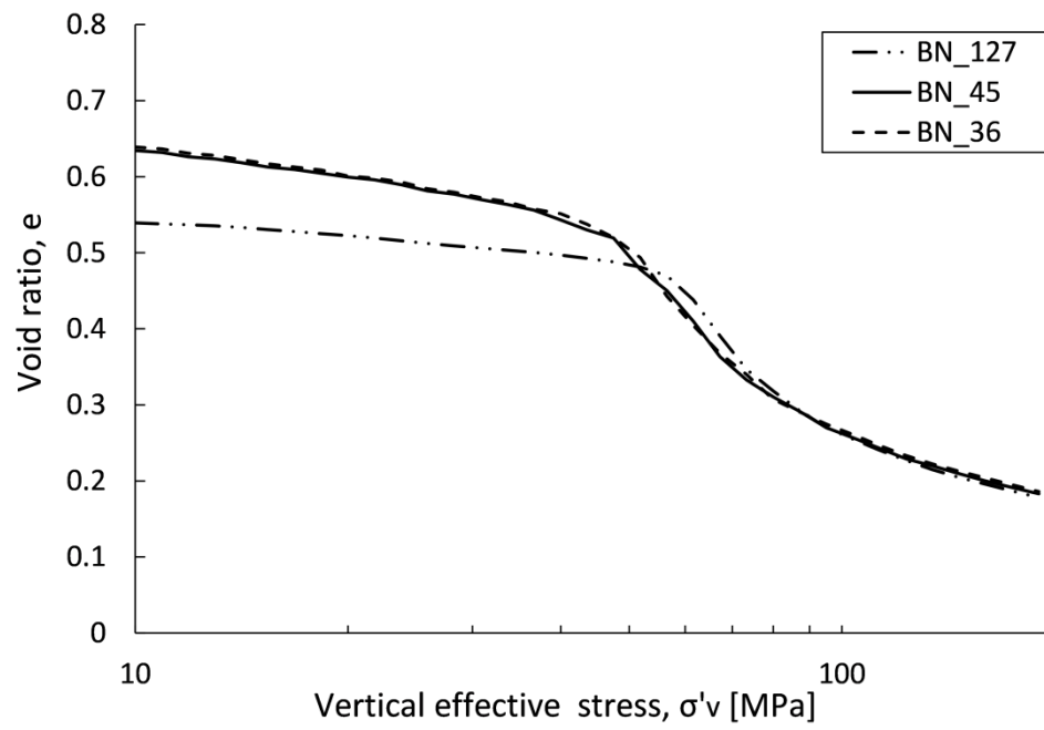
Fig. A.7 Beads narrow soil type 1-D compression curves.
