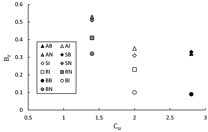
Fig. 4.29 Effect of PSD on particle breakage.
