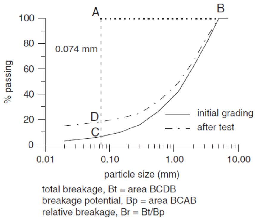
Fig. 3.20 Hardin (1985) particle breakage measurement parameters.
