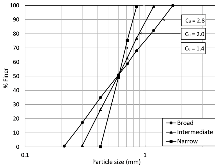
Fig. 3.8 PSD curves of the soil types tested.
