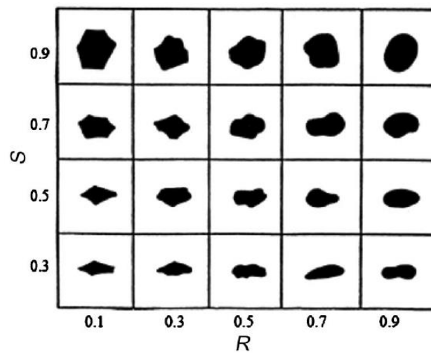
Fig. 3.10 Krumbein and Sloss (1963) Particle shape determination chart.
