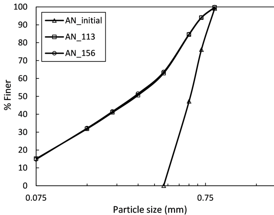
Fig. C.2 Pre and post-compression PSD curves of the AN soil type.
