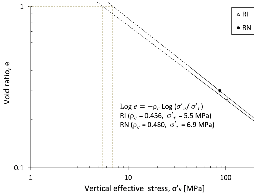
Fig. 4.21 Limiting compression curves of the rounded soil types.
