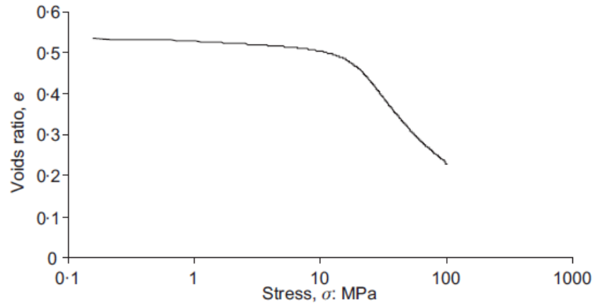
Fig. 2.3 Normal compression curve of silica sand in e - \log \sigma'_v space (McDowell, 2005) as adopted from McDowell (2002).
