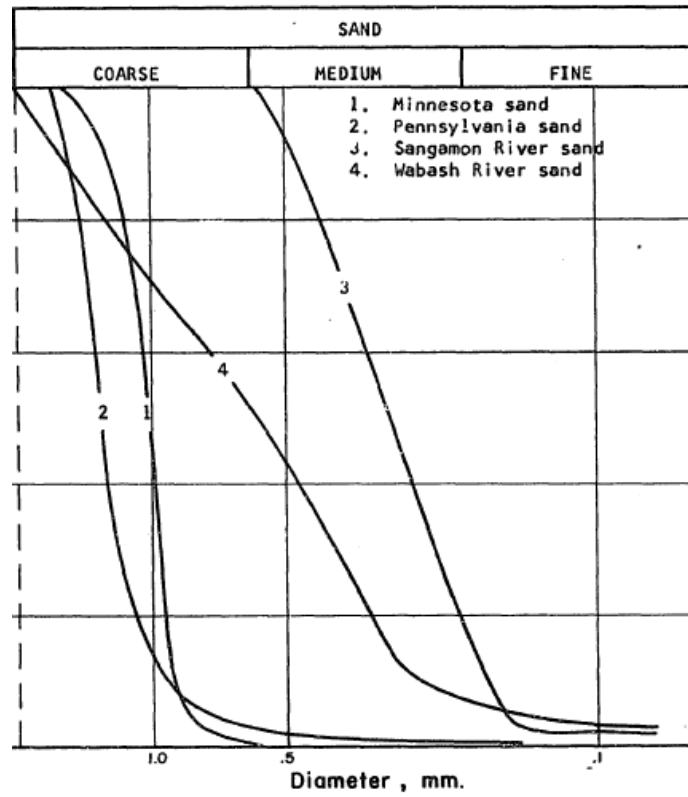
Fig. 2.1 PSD curves of the sands investigated by Hendron (1963).
