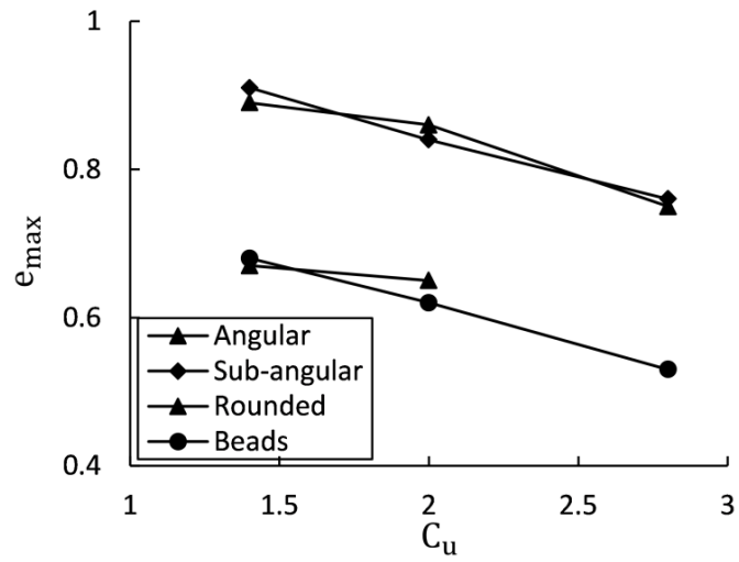
Fig. 3.12 Relationship between e_{\max} and PSD.
