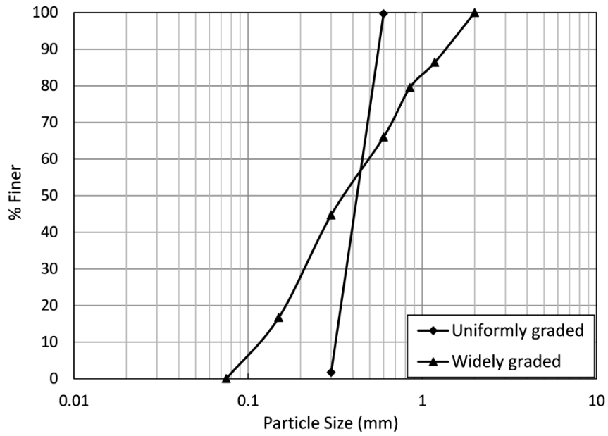
Fig. 3.4 PSD curves of the samples used for preliminary study.
