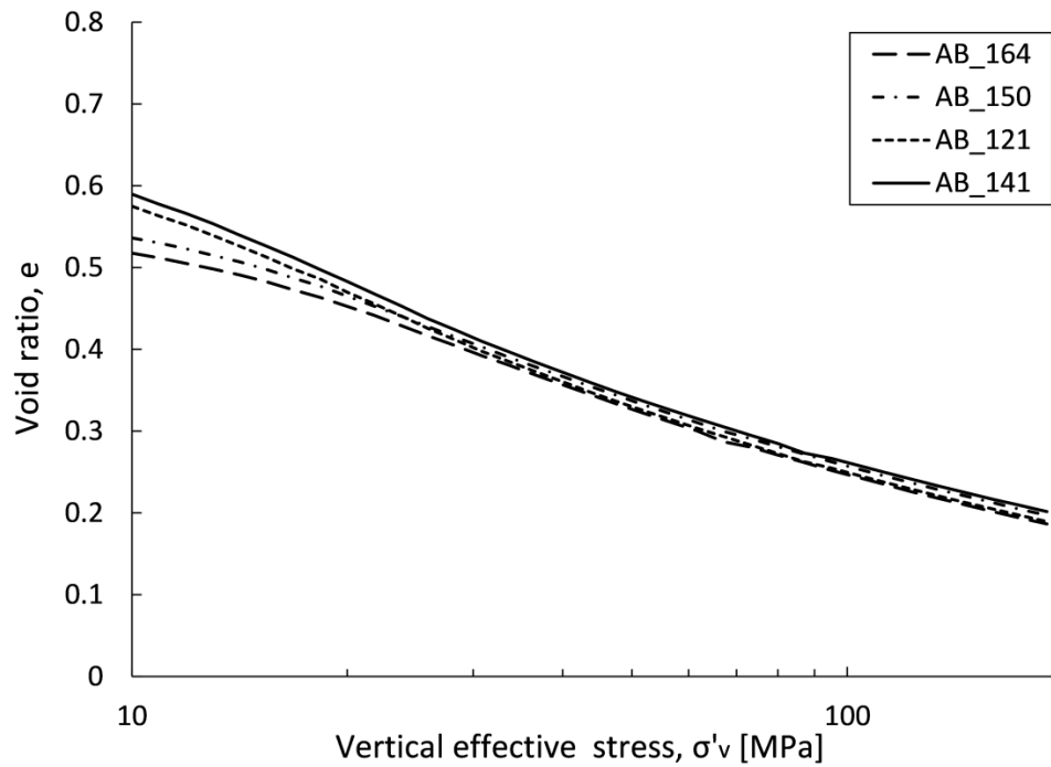
Fig. A.1 Angular broad soil type 1-D compression curves.
