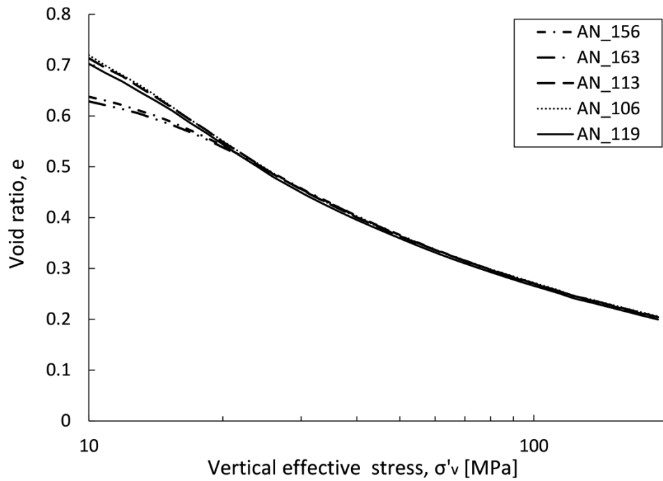
Fig. A.2 Angular narrow soil type 1-D compression curves.
