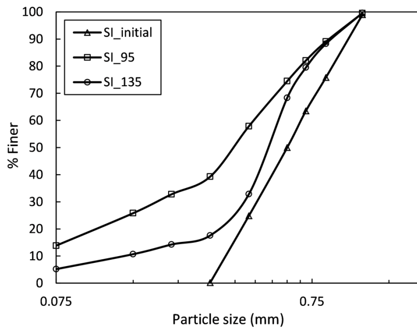
Fig. 4.26 Pre and post-compression PSD curves of the SI soil type.
