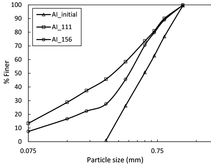
Fig. 4.25 Pre and post-compression PSD curves of the AI soil type.
