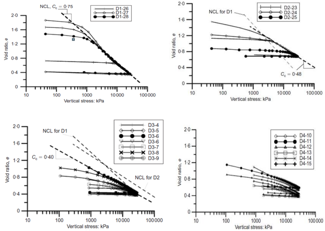
Fig. 2.6 1-D compression curves of Dog's bay sand. From narrowest to broadest gradation; D1, D2, D3 and D4 (Altuhafi and Coop, 2011).
