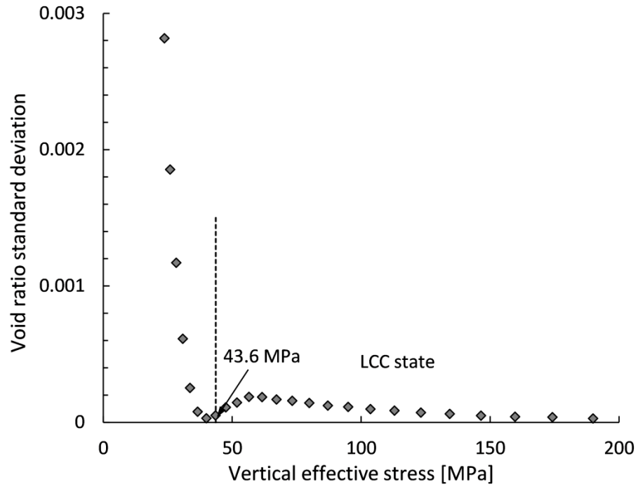
Fig. 4.17 LCC determination for the RI soil type.
