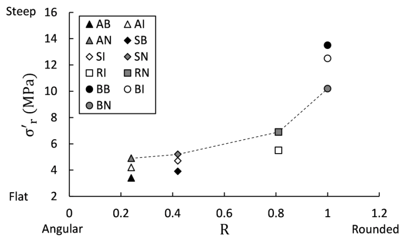
Fig. 5.4 Relationship between \sigma'_r and particle roundness.
