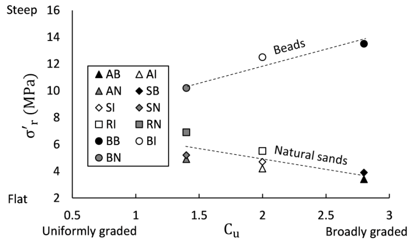
Fig. 5.2 Relationship between \sigma'_r and C_u .
