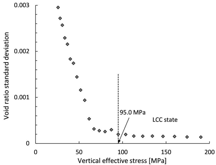
Fig. B.6 LCC determination for the BB soil type.
