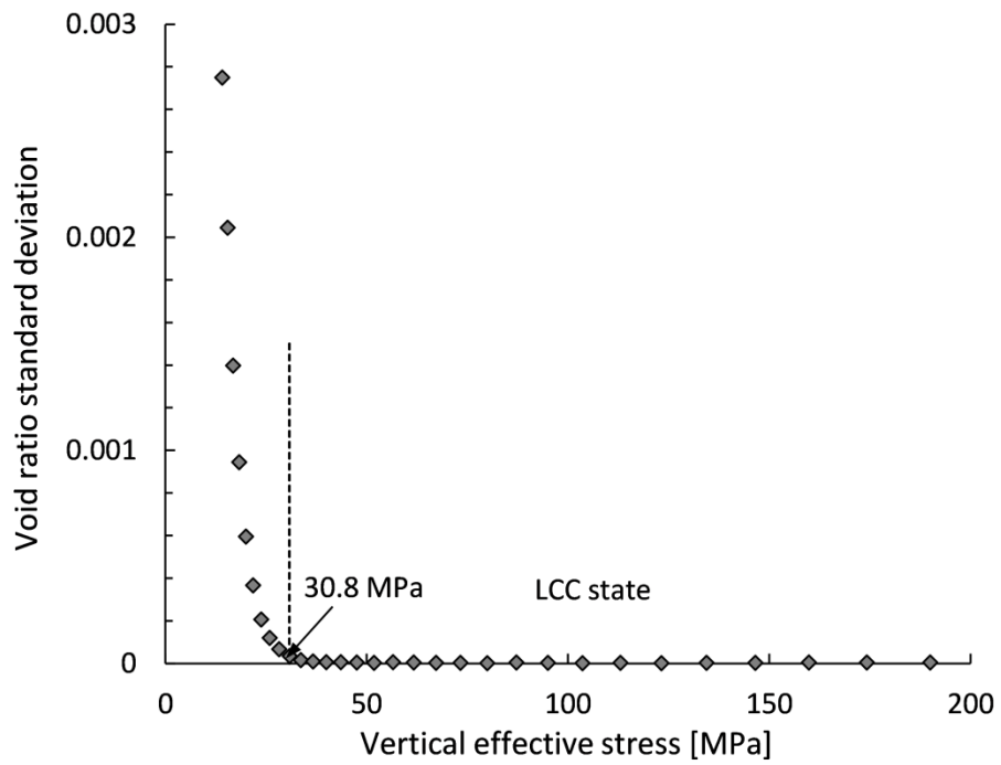
Fig. 4.16 LCC determination for the SI soil type.
