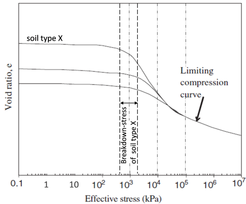
Fig. 1.1 Conceptual representation of the LCC [adopted from Uygar and Doven (2006)].
