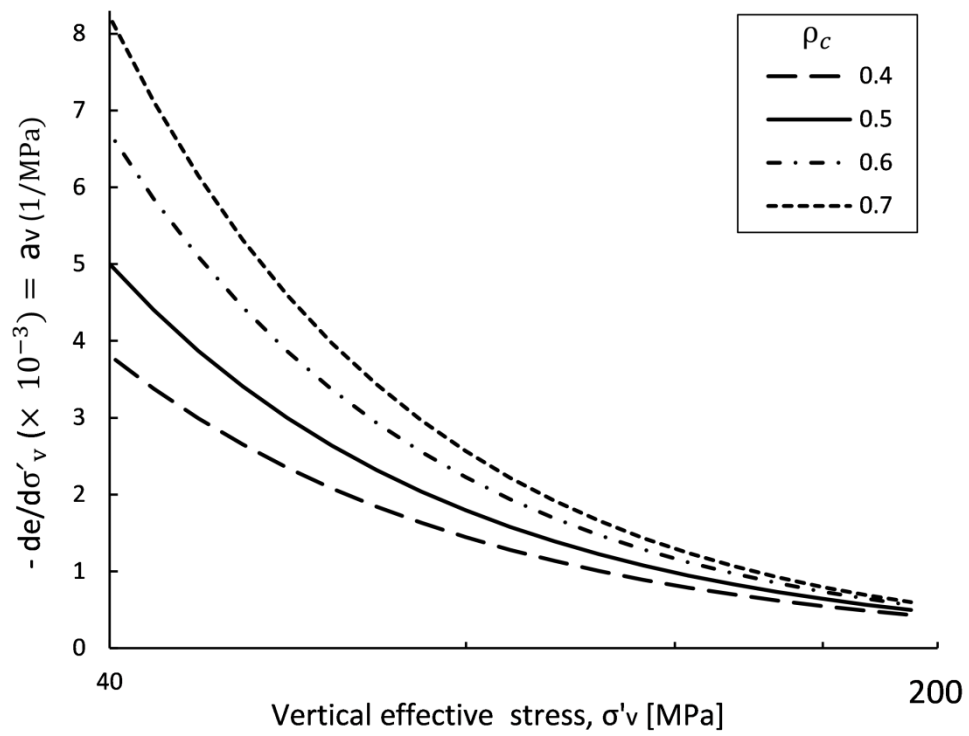
Fig. 4.24 Relationship between the LCC and compressibility.
