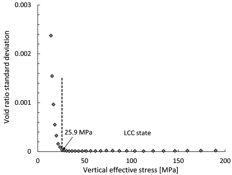
Fig. 4.15 LCC determination for the AI soil type.
