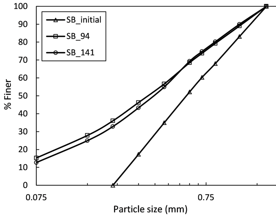
Fig. C.3 Pre and post-compression PSD curves of the SB soil type.
