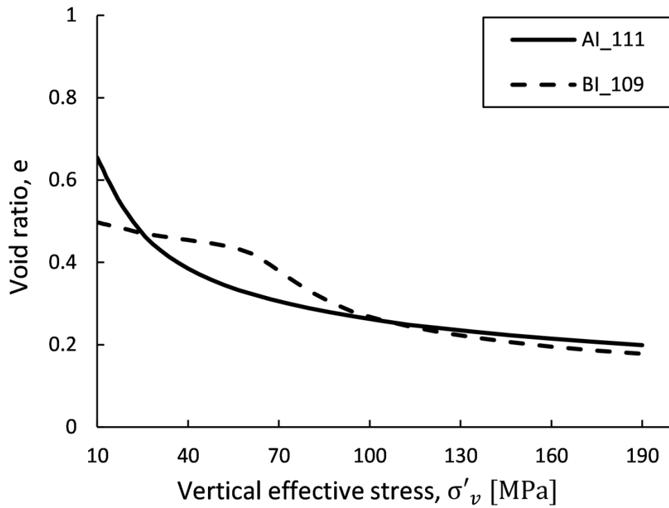
Fig. 4.1 Typical 1-D confined compression curves of the tested soil types in: (a) semi-logarithmic space; (b) double-logarithmic space; (c) natural space.
