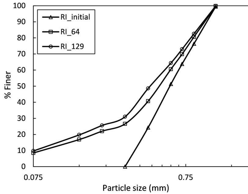
Fig. 4.27 Pre and post-compression PSD curves of the RI soil type.
