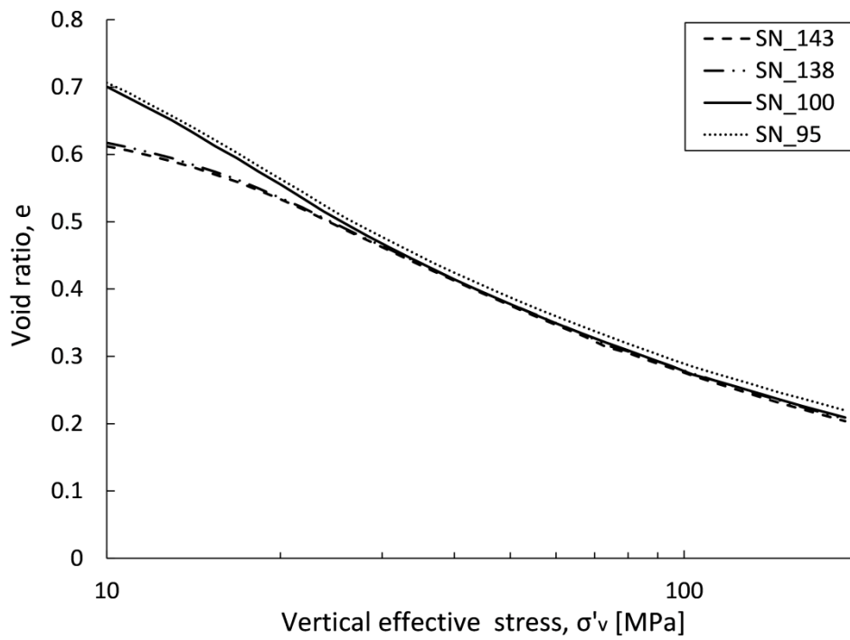
Fig. A.4 Sub-angular narrow soil type 1-D compression curves.
