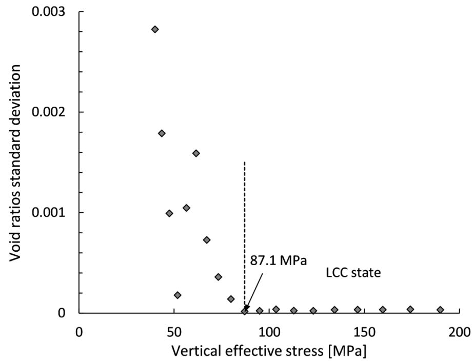
Fig. B.7 LCC determination for the BN soil type.
