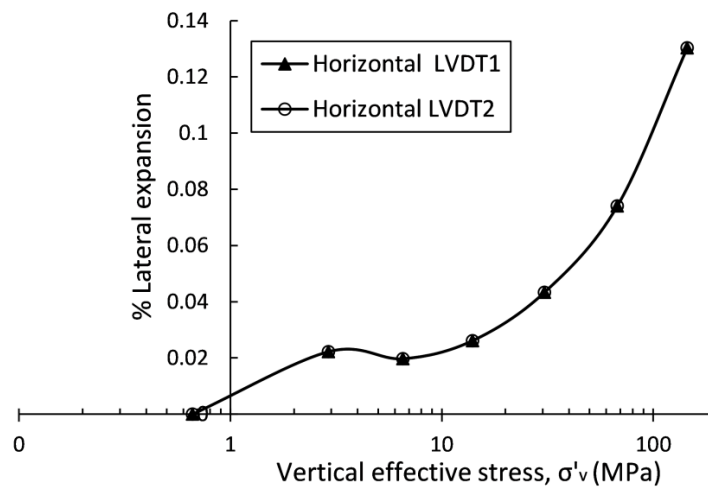
Fig. 3.16 Compression mould lateral expansion measured from two horizontal LVDTs.
