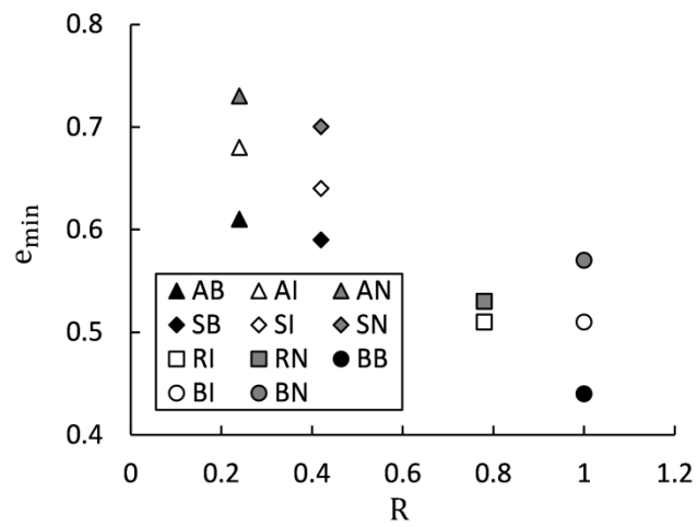
Fig. 3.15 Relationship between e_{min} and particle roundness.
