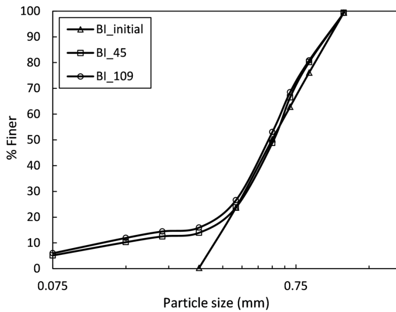
Fig. 4.28 Pre and post-compression PSD curves of the BI soil type.
