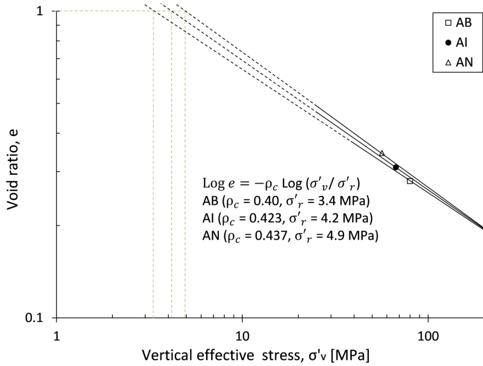
Fig. 4.19 Limiting compression curves of the angular soil types.
