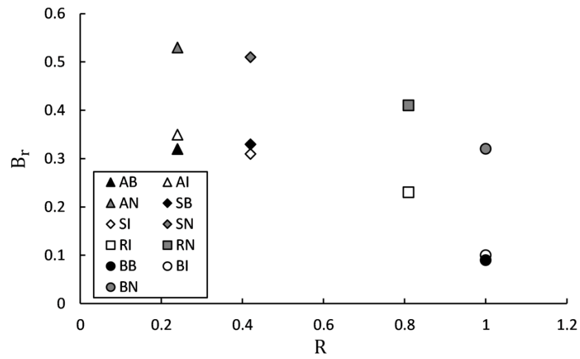
Fig. 4.30 Effect of particles roundness on particle breakage.
