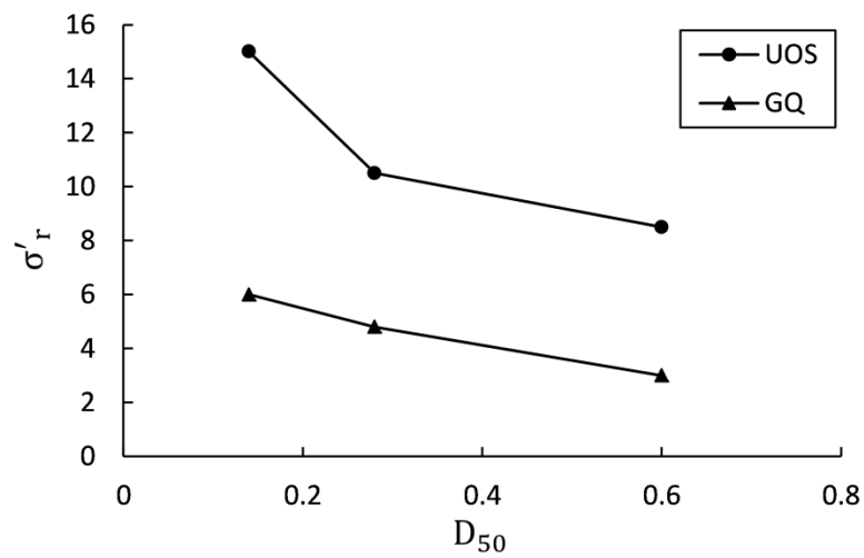
Fig. 2.7 A plot of median particle size against reference vertical effective stress; UOS, uniform Ottawa sand; GQ, ground quartz [tested by Roberts and De Souza (1958) and Roberts (1964)].
