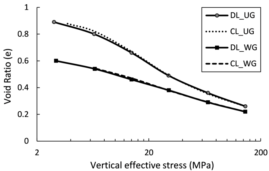
Fig. 3.5 Compression curves of the samples used for preliminary study; DL; discrete loading compression machine; CL; continuous loading compression machine; UG, uniformly graded PSD; WG, widely graded PSD.
