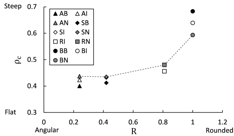
Fig. 5.3 Relationship between \rho_c and particle roundness.
