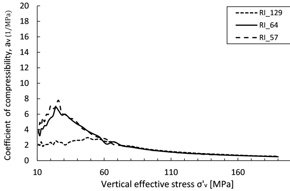
Fig. 4.8 Effect of initial relative density on compressibility for the RI soil type.
