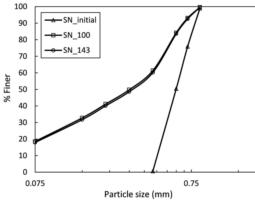
Fig. C.4 Pre and post-compression PSD curves of the SN soil type.
