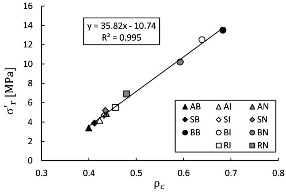
Fig. 4.23 Relationship between the LCC parameters.
