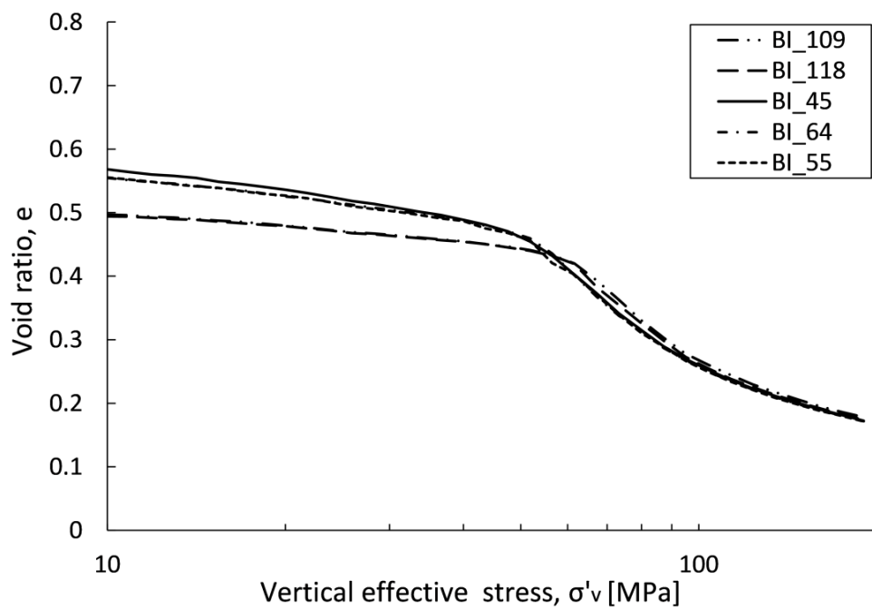
Fig. 4.5 BI soil type 1-D compression curves.
