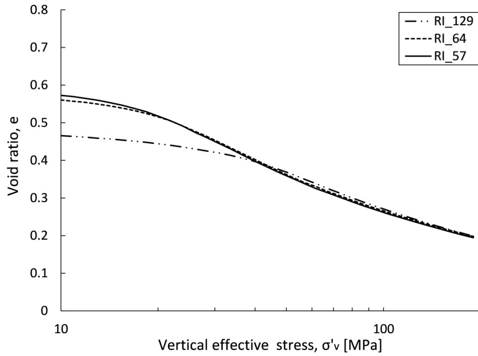
Fig. 4.4 RI soil type 1-D compression curves.
