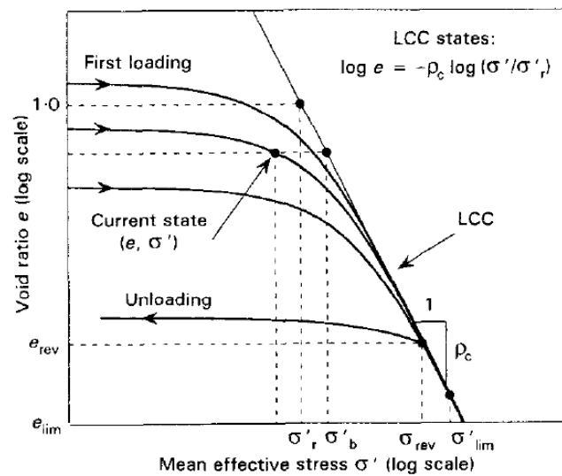
Fig. 2.2 Conceptual representation of the LCC for cohesionless soils (Pestana and Whittle, 1995).
