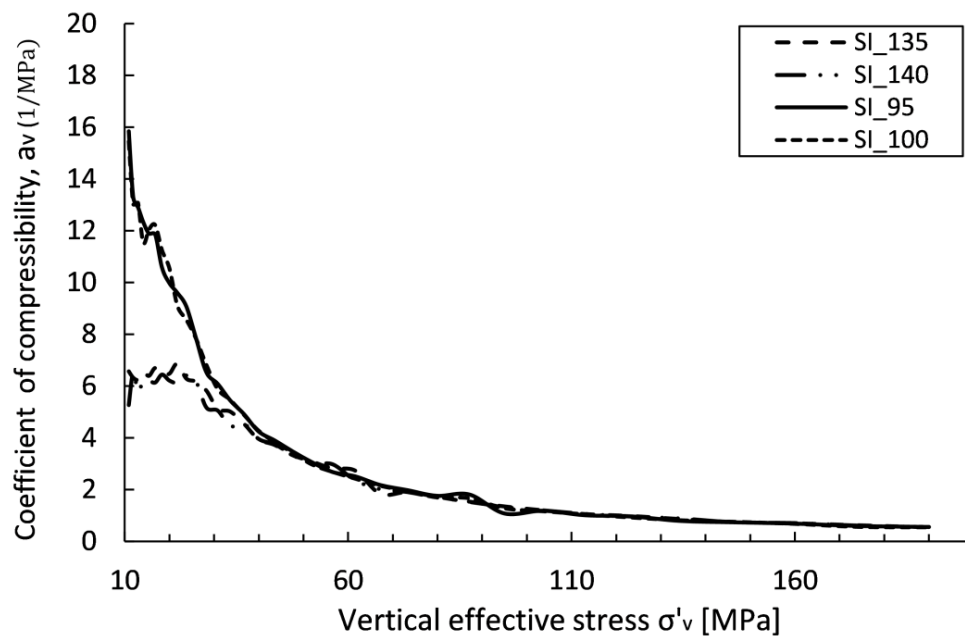
Fig. 4.7 Effect of initial relative density on compressibility for the SI soil type.
