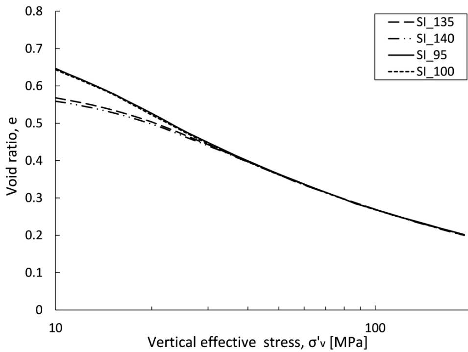
Fig. 4.3 SI soil type 1-D compression curves.
