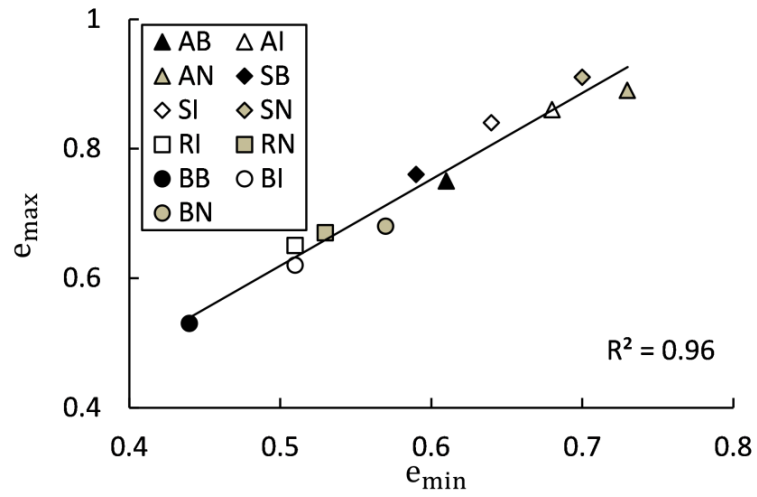
Fig. 3.11 Relation between e_{\max} and e_{\min} of the selected soil types.
