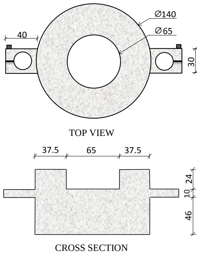
Fig. 3.3 Schematic diagram of the compression mould vessel (all dimensions are in mm).
