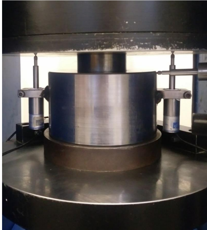
Fig. 3.1 Compression mould placed in the compression machine and with the three displacement transducers in place.
