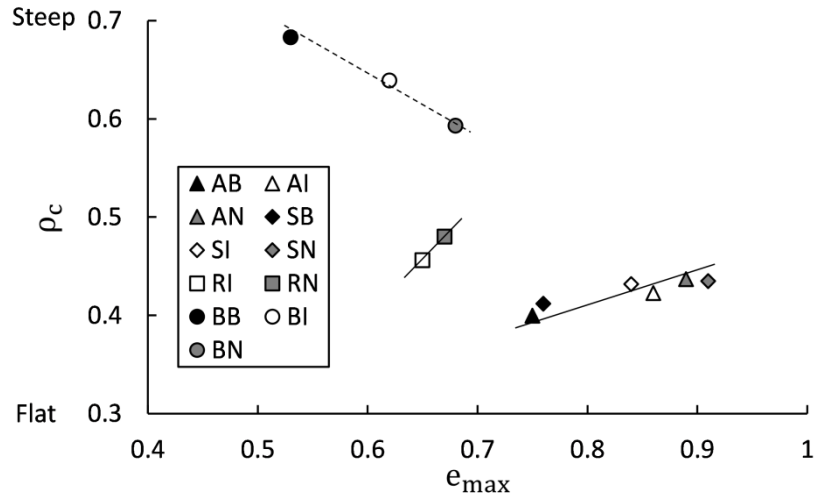
Fig. 5.5 Relationship between \rho_c and e_{\max} .
