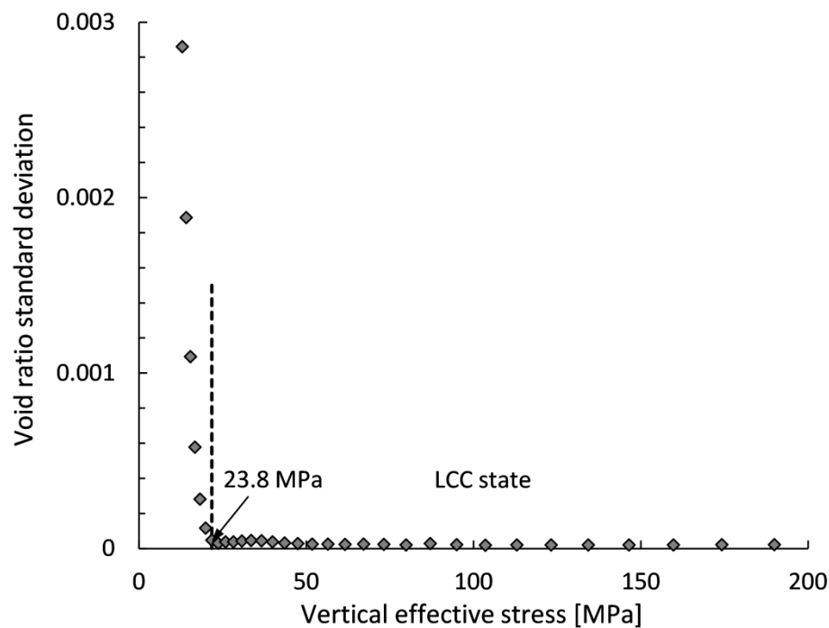
Fig. B.2 LCC determination for the AN soil type.
