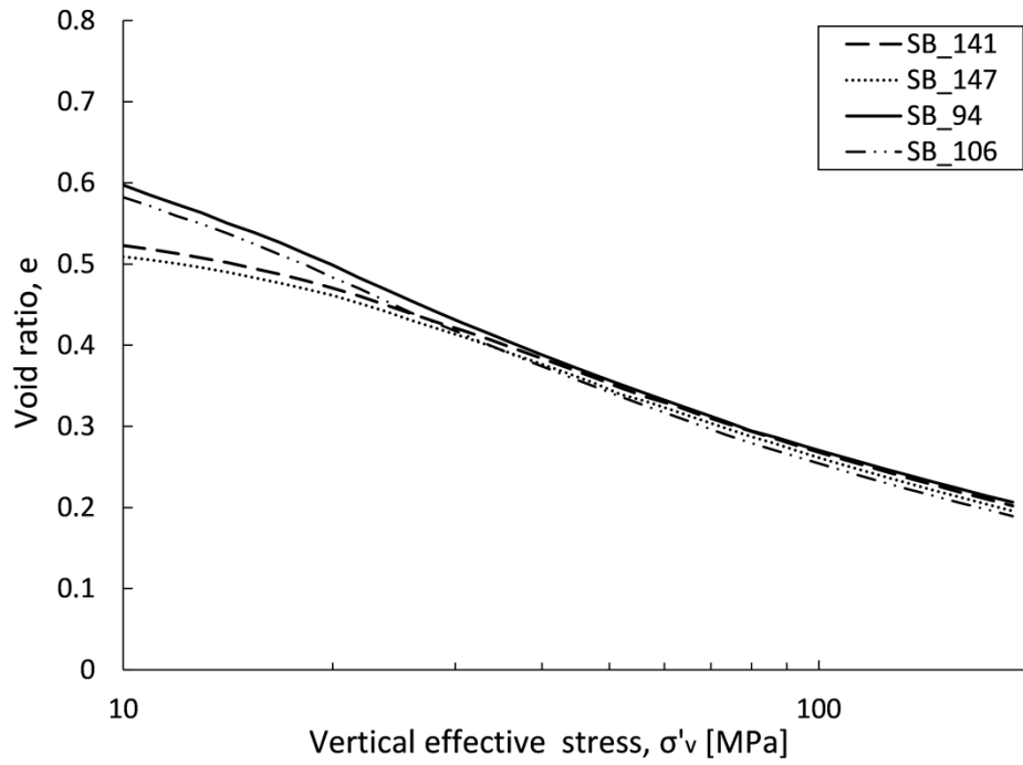
Fig. A.3 Sub-angular broad soil type 1-D compression curves.
