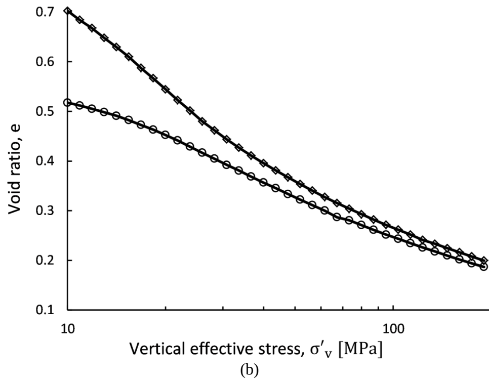
Fig. 3.18 Illustration of the approach used in defining the 1-D compression curve obtained herein; (a) initial data points (b) refined 35 data points.
