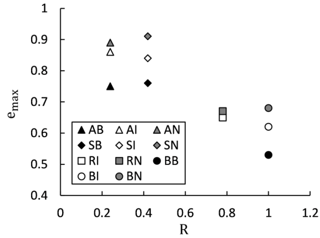
Fig. 3.14 Relationship between e_{max} and particle roundness.
