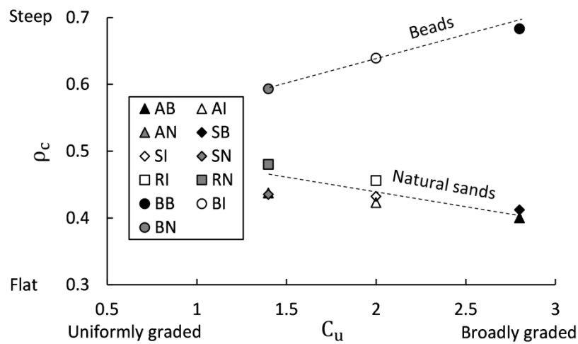
Fig. 5.1 Relationship between \rho_c and C_u .
