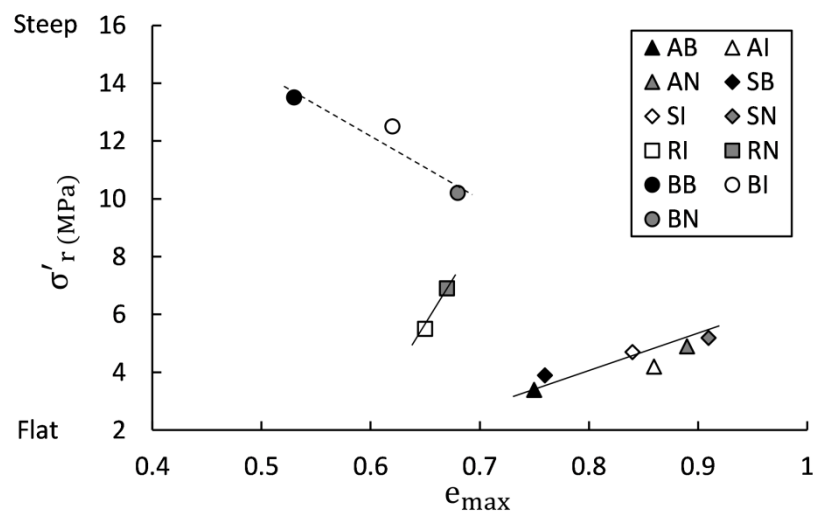
Fig. 5.7 Relationship between \sigma'_r and e_{\max} .
