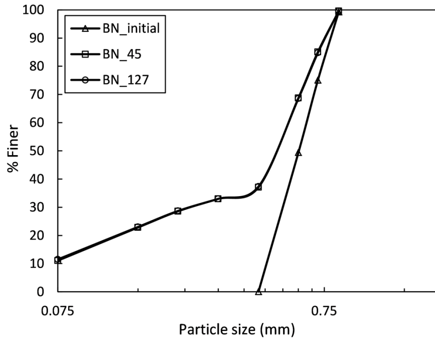
Fig. C.7 Pre and post-compression PSD curves of the BN soil type.
