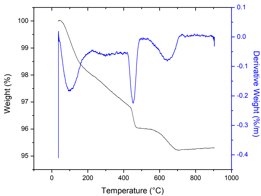
Figure C18: TGA/DTA curves for FA-75 -28
