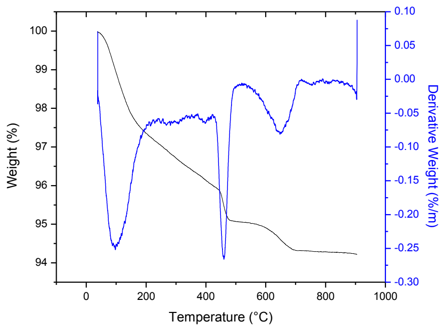
Figure C40: TGA/DTA curves for SF-60 -3
