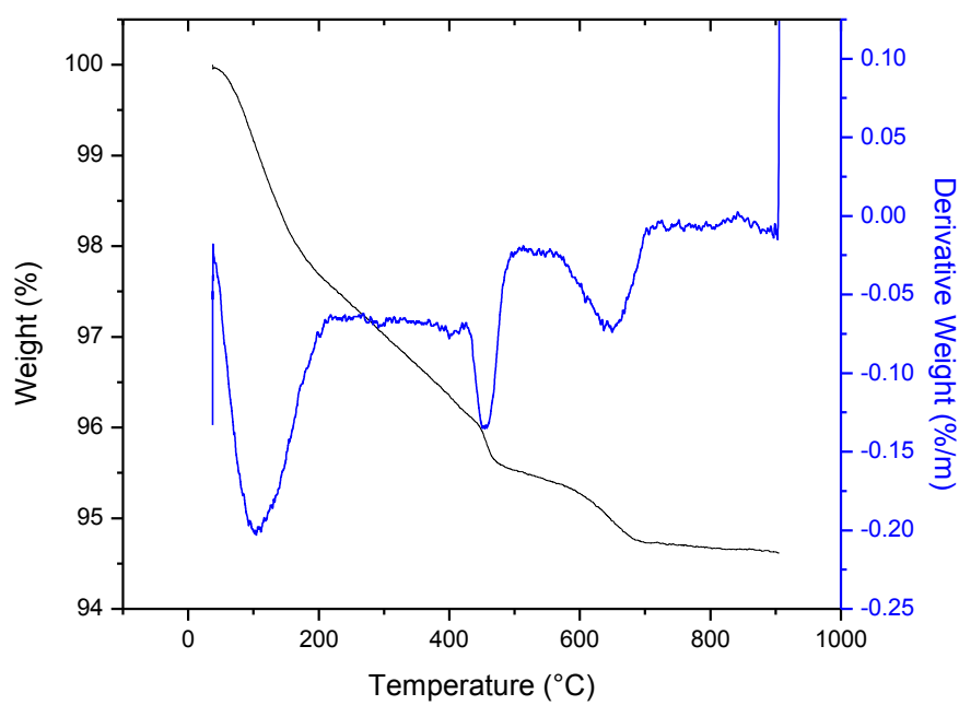
Figure C27: TGA/DTA curves for CC-50 -28
