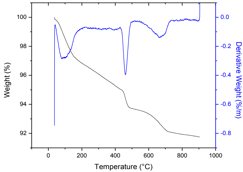
Figure C1: TGA/DTA curves for PC-40 -3
