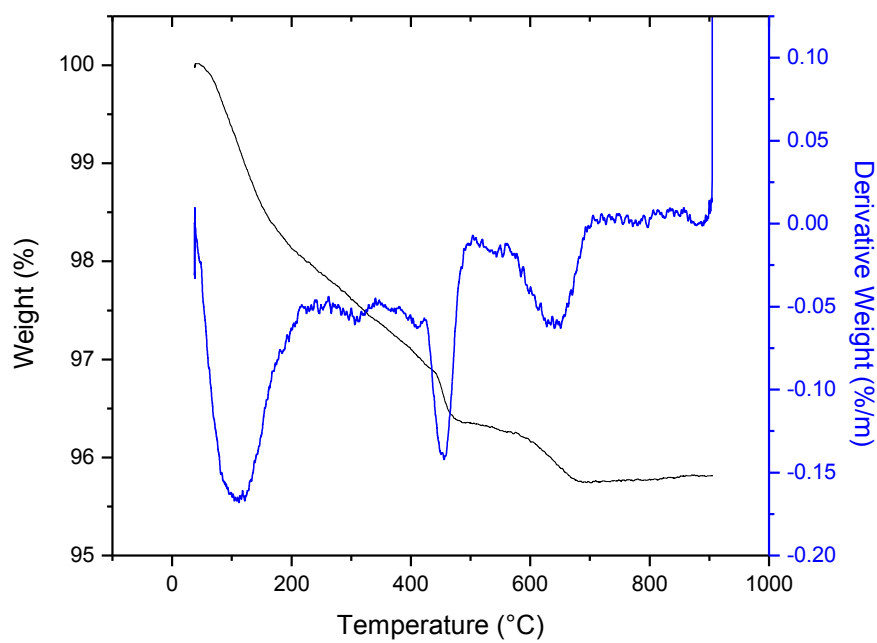
Figure C25: TGA/DTA curves for SL-50 -3
