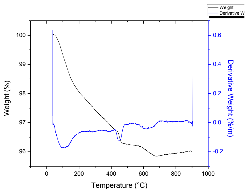
Figure C24: TGA/DTA curves for SL-40 -28
