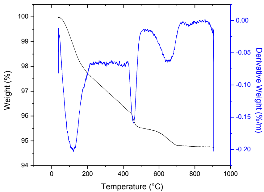
Figure C23: TGA/DTA curves for CC-40 -7
