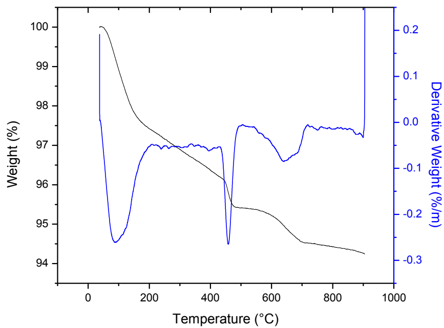
Figure C34: TGA/DTA curves for SF-40 -3
