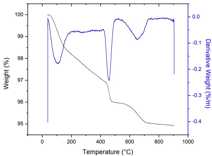
Figure C10: TGA/DTA curves for PC-75 -3
