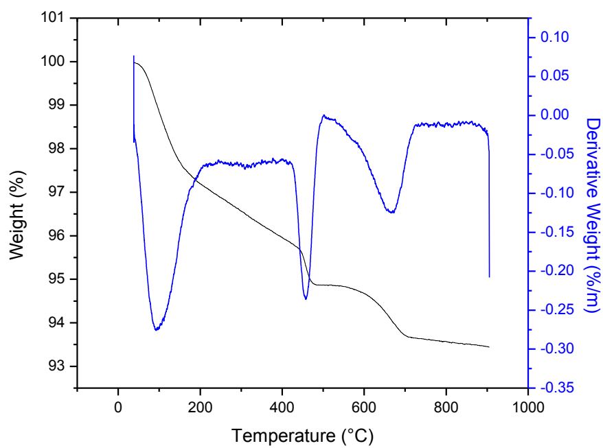
Figure C44: TGA/DTA curves for SF-75 -7
