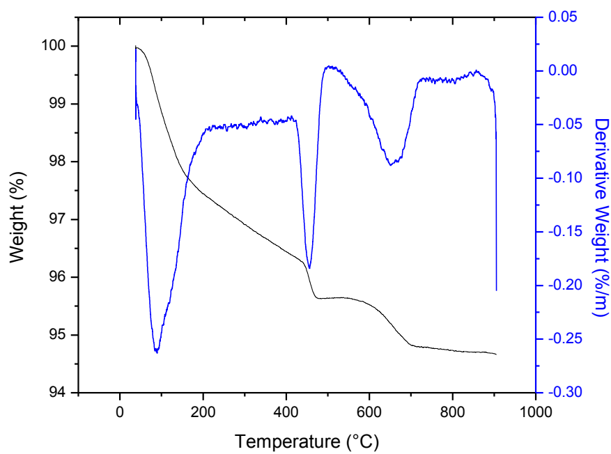
Figure C43: TGA/DTA curves for SF-75 -3
