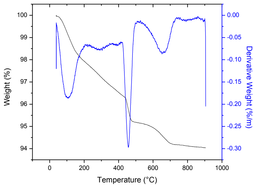
Figure C11: TGA/DTA curves for PC-75 -7
