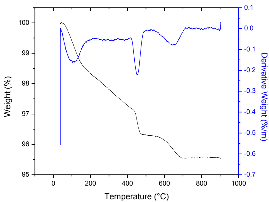
Figure C16: TGA/DTA curves for FA-50 -3
