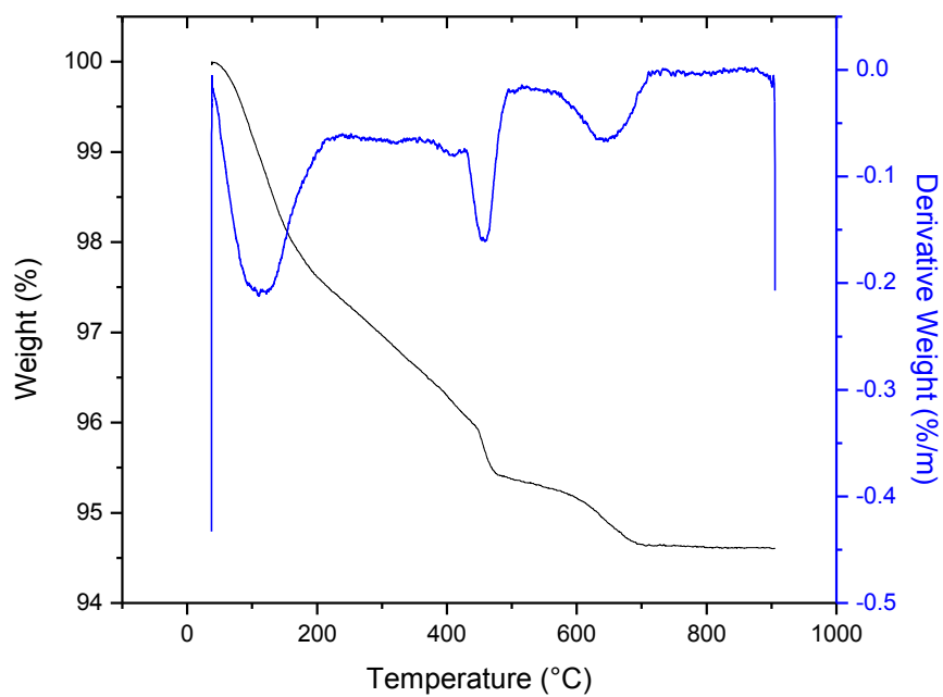
Figure C22: TGA/DTA curves for CC-40 -3
