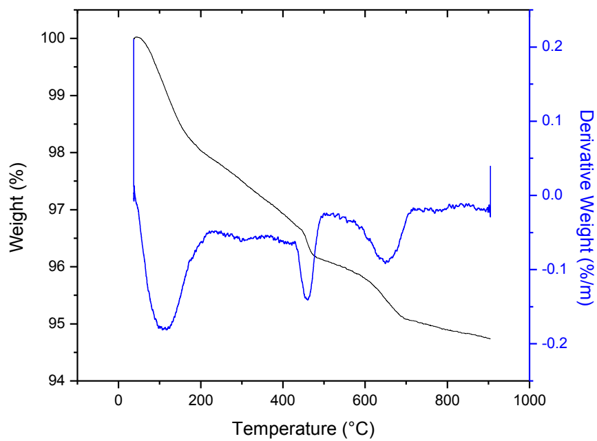
Figure C30: TGA/DTA curves for SL-60 -28
