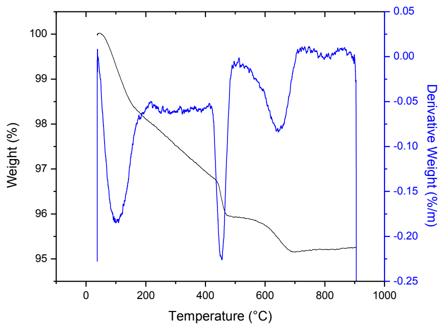
Figure C17: TGA/DTA curves for FA-50 -7
