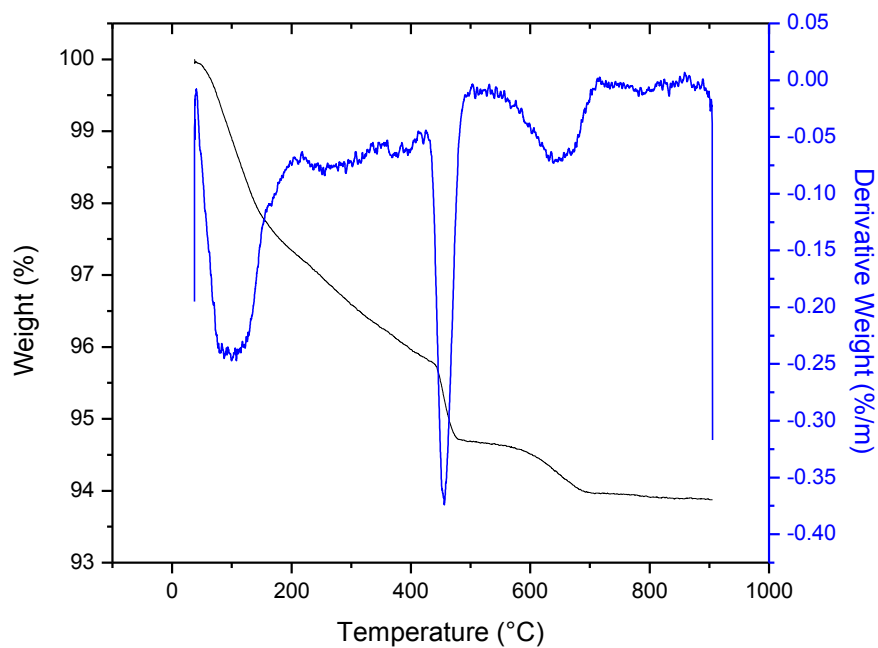
Figure C7: TGA/DTA curves for PC-60 -3
