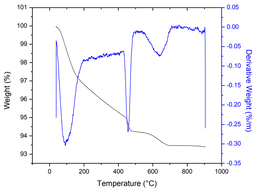
Figure C36: TGA/DTA curves for SF-40 -28
