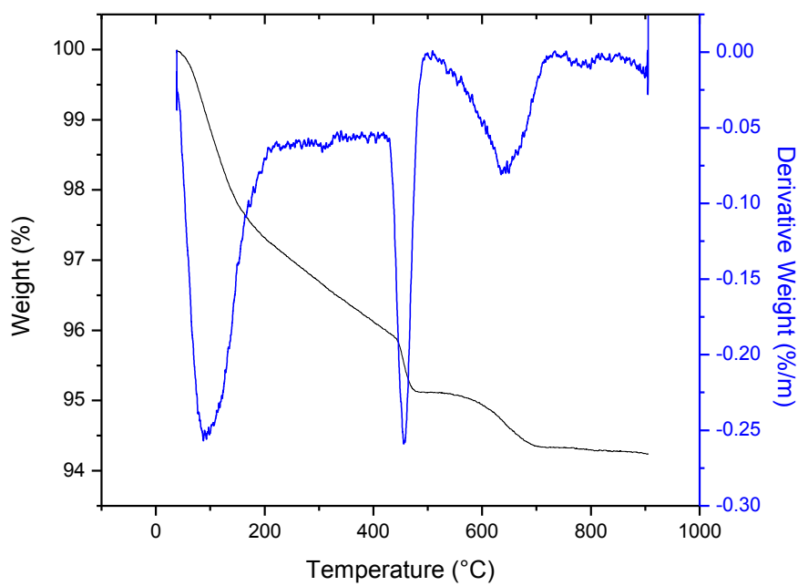
Figure C39: TGA/DTA curves for SF-50 -28
