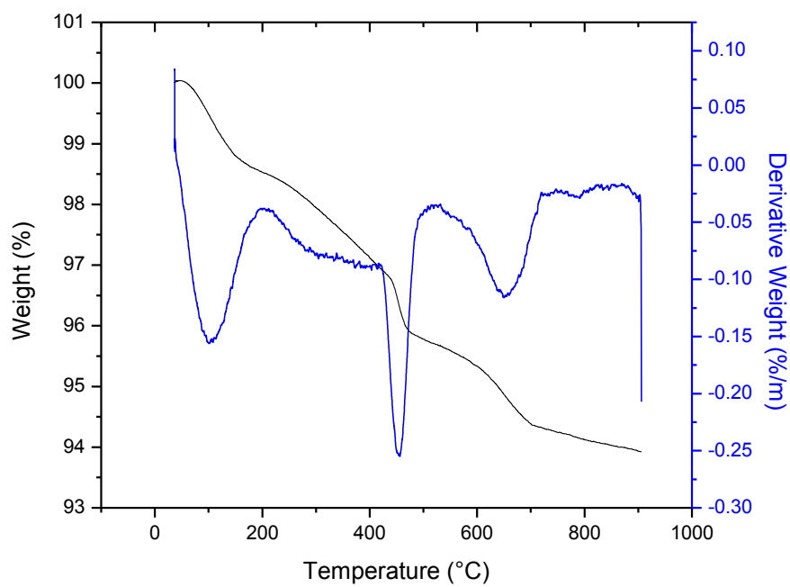
Figure C20: TGA/DTA curves for FA-60 -7
