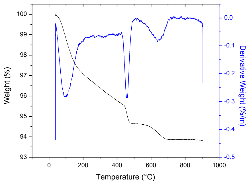
Figure C42: TGA/DTA curves for SF-60 -28
