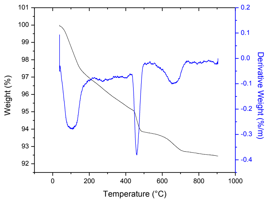
Figure C9: TGA/DTA curves for PC-60 -28
