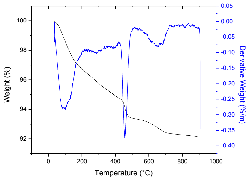
Figure C2: TGA/DTA curves for PC-40 -7
