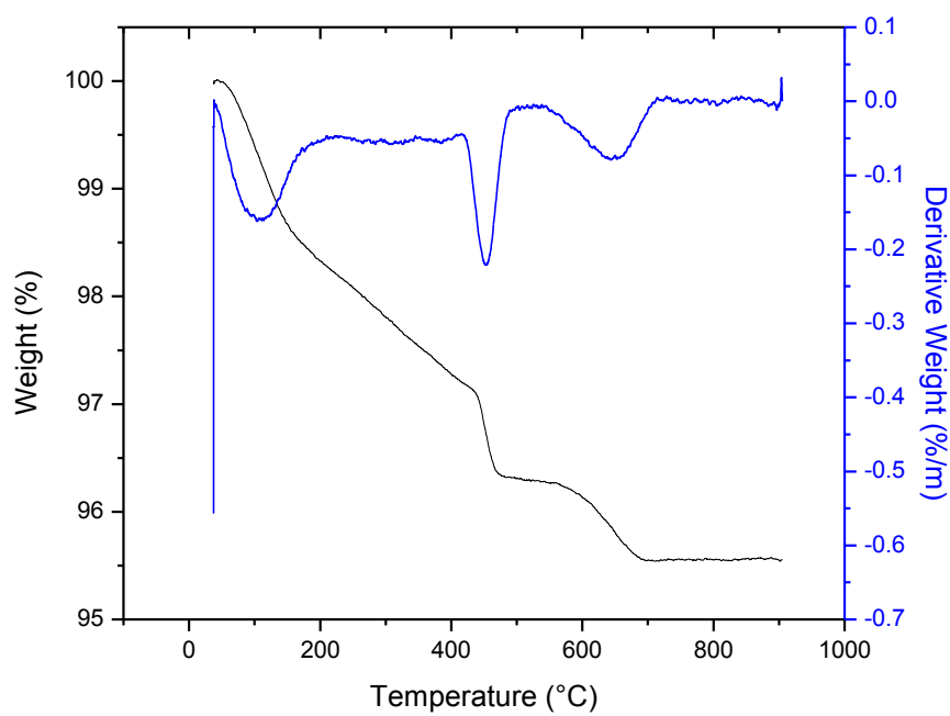
Figure C16: TGA/DTA curves for FA-75 -3
