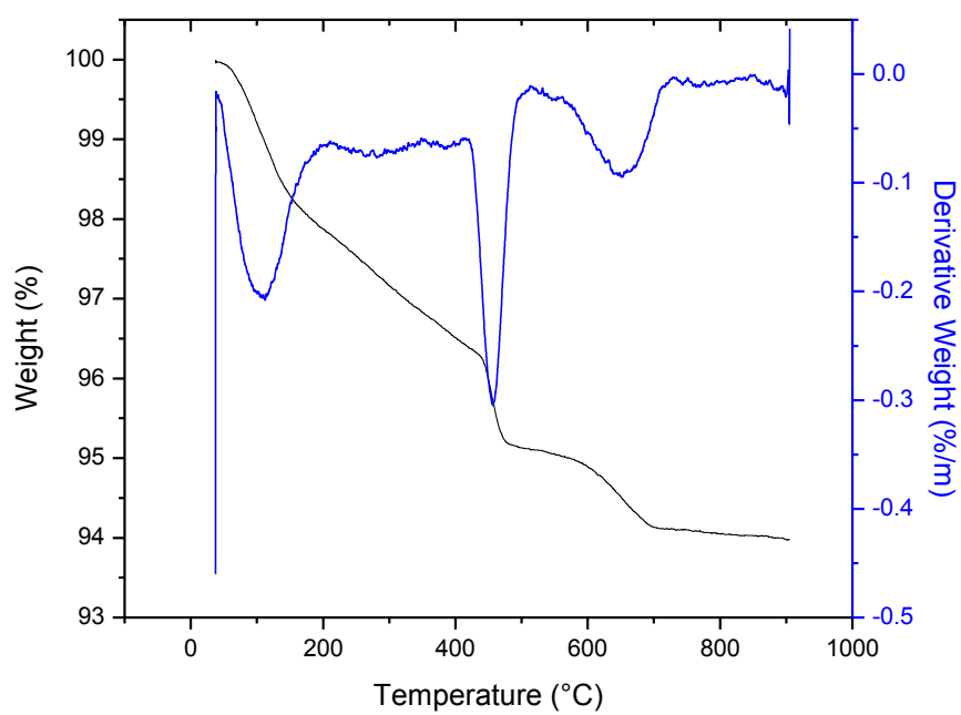
Figure C12: TGA/DTA curves for PC-75 -28
