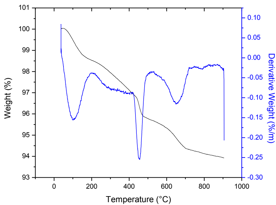
Figure C14: TGA/DTA curves for FA-40 -7
