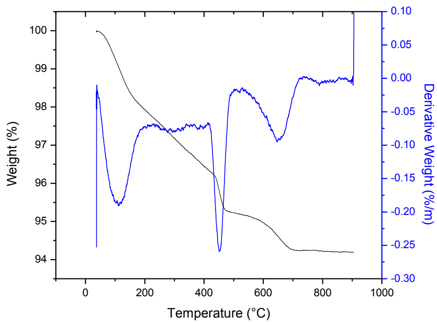
Figure C15: TGA/DTA curves for FA-40 -28
