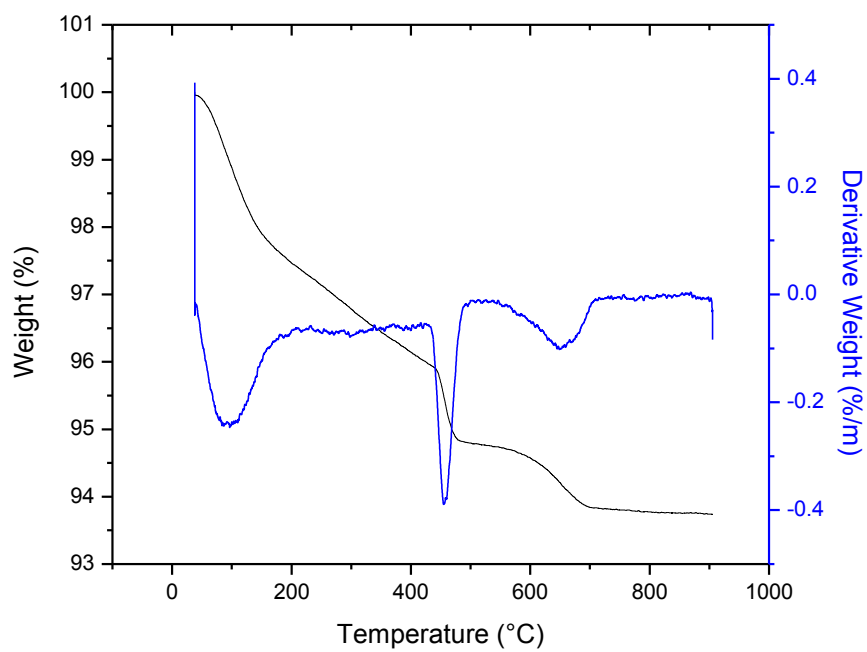
Figure C4: TGA/DTA curves for PC-50 -3
