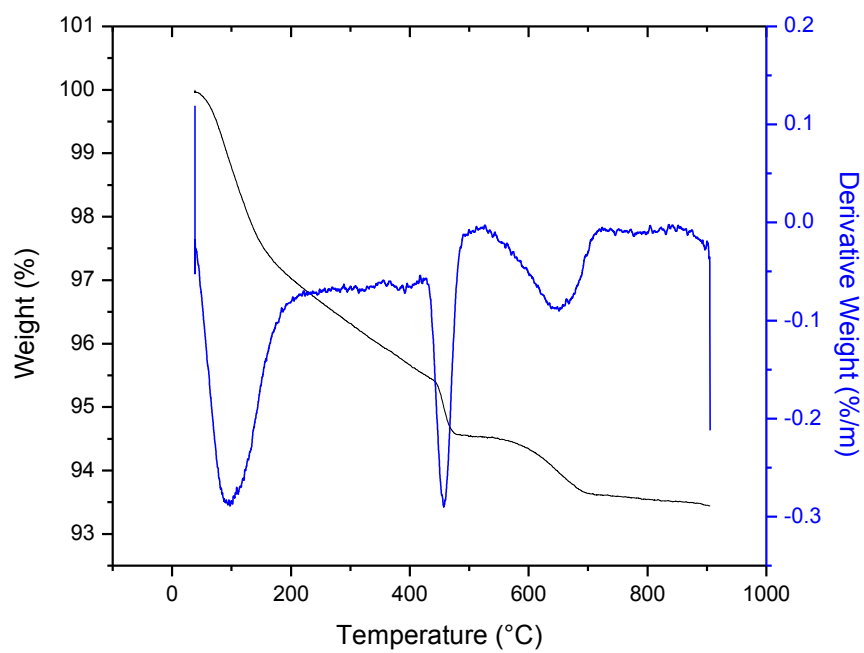
Figure C38: TGA/DTA curves for SF-50 -7
