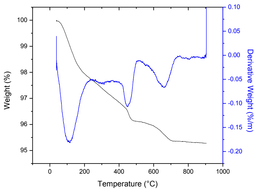
Figure C33: TGA/DTA curves for CC-75 -28
