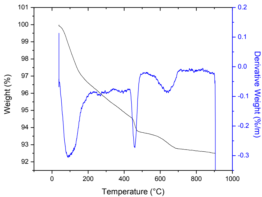
Figure C35: TGA/DTA curves for SF-40 - 7
