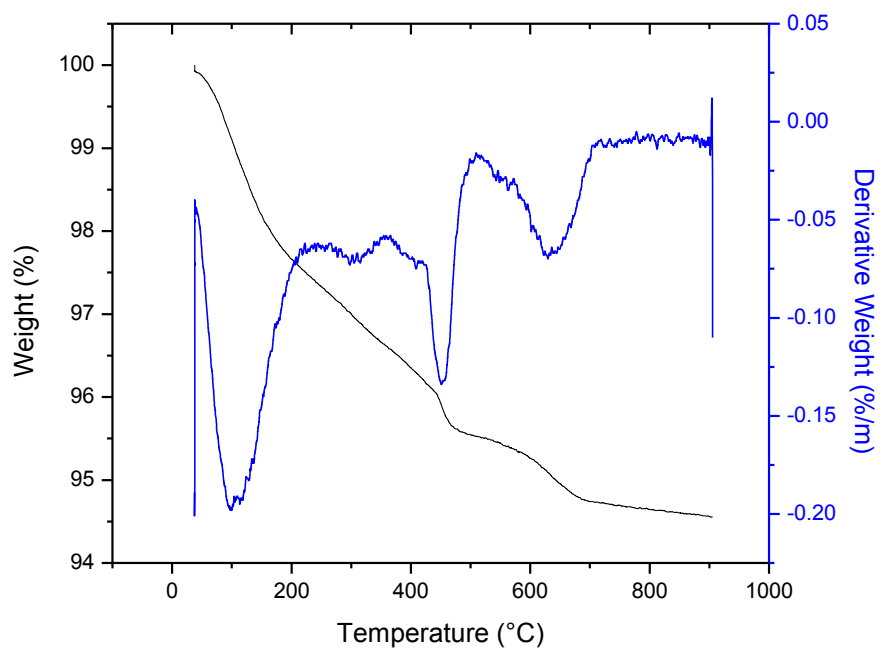
Figure C29: TGA/DTA curves for SL-60 -7
