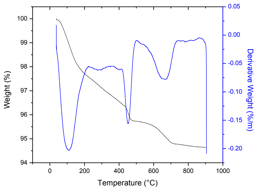
Figure C32: TGA/DTA curves for CC-75 -7
