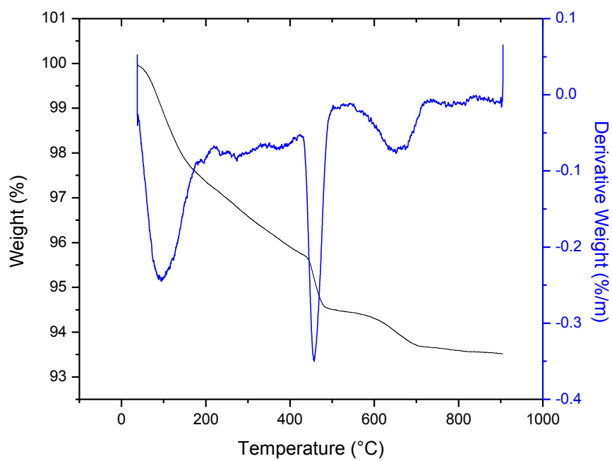
Figure C5: TGA/DTA curves for PC-50 -7
