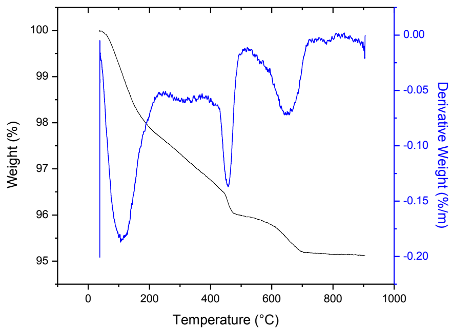
Figure C28: TGA/DTA curves for CC-60 -3
