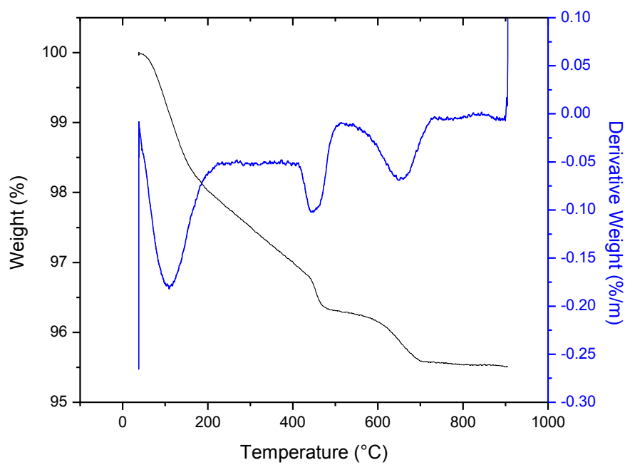
Figure C31: TGA/DTA curves for CC-75 -3
