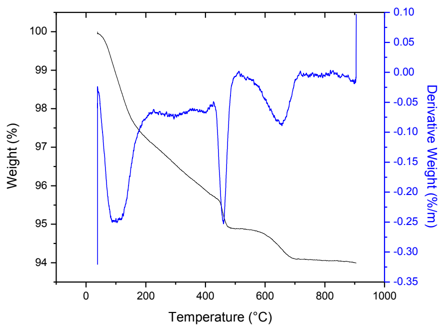
Figure C37: TGA/DTA curves for SF-50 -3
