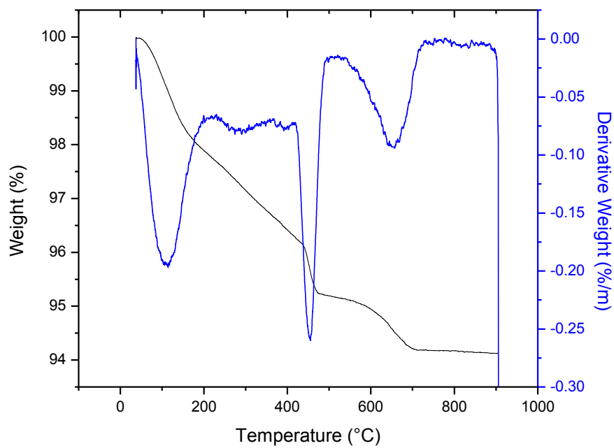
Figure C13: TGA/DTA curves for FA-40 – 3
