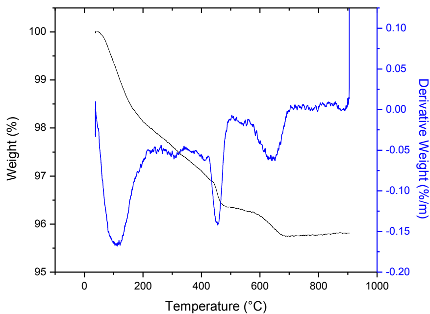
Figure C25: TGA/DTA curves for CC-50 -3
