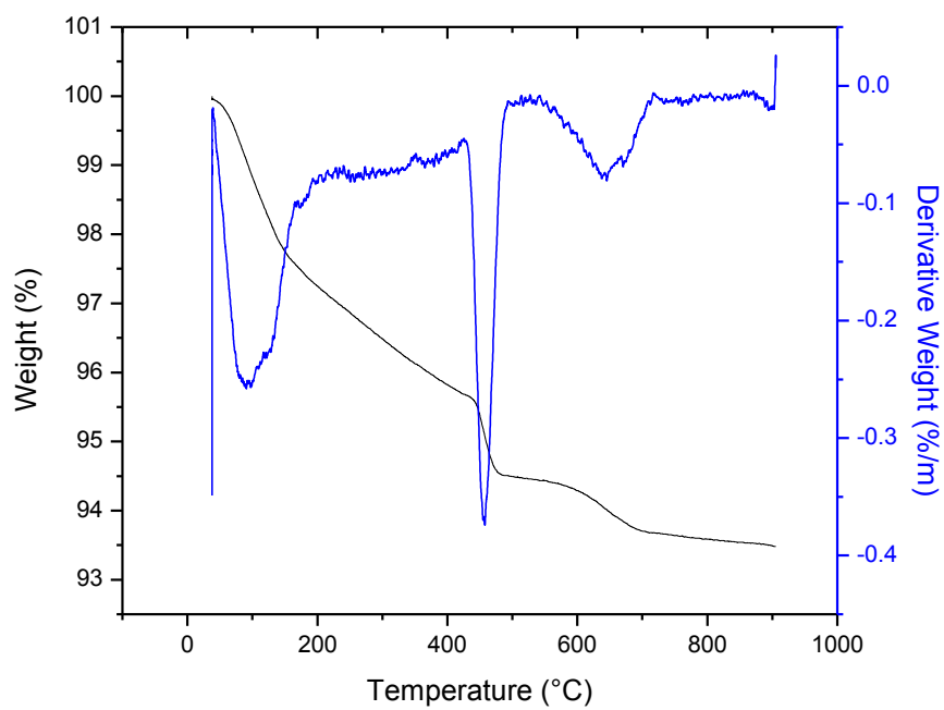
Figure C8: TGA/DTA curves for PC-60 -7
