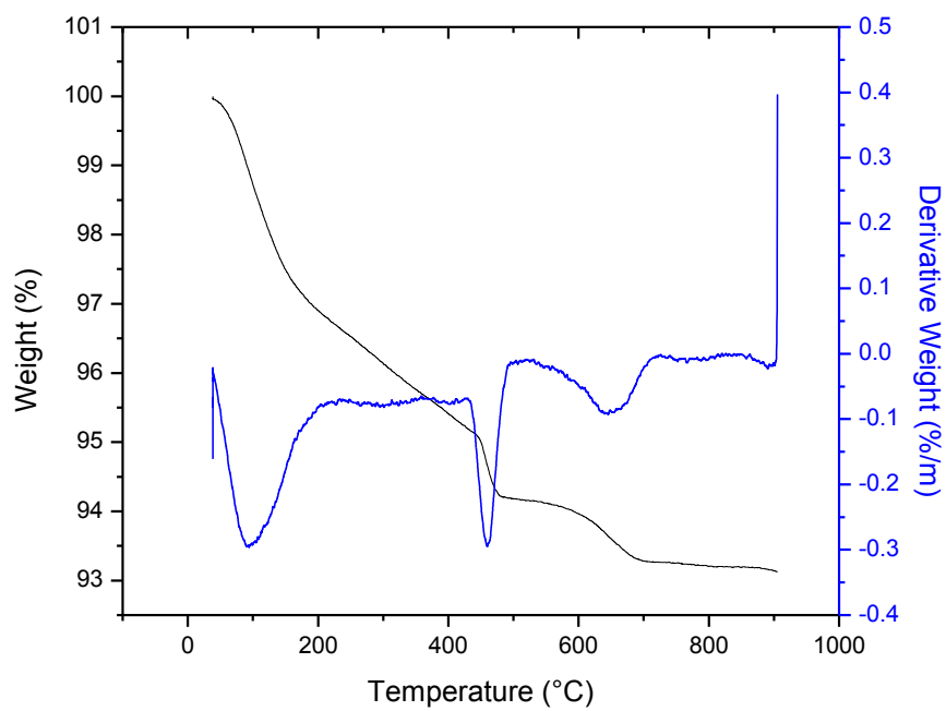
Figure C41: TGA/DTA curves for SF -60 -7
