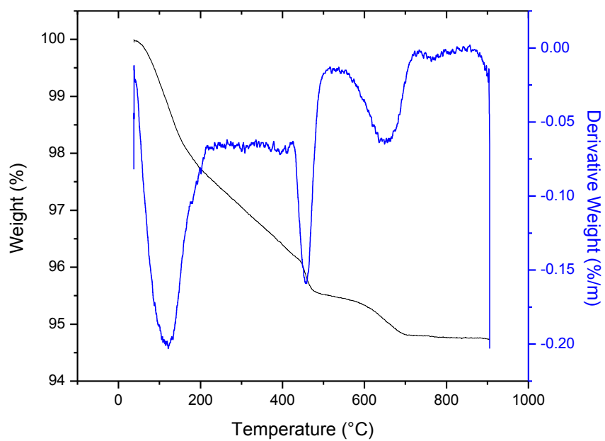
Figure C23: TGA/DTA curves for SL-40 -7
