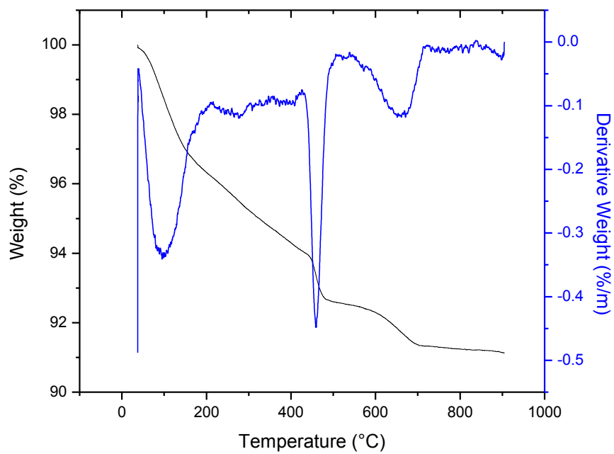
Figure C3: TGA/DTA curves for PC-40 -28
