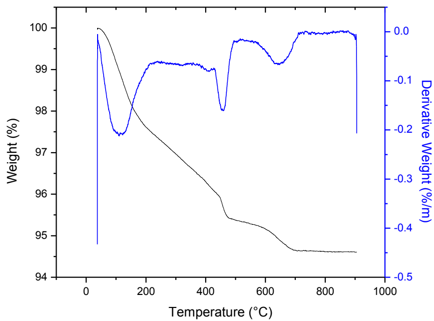
Figure C22: TGA/DTA curves for SL-40 -3
