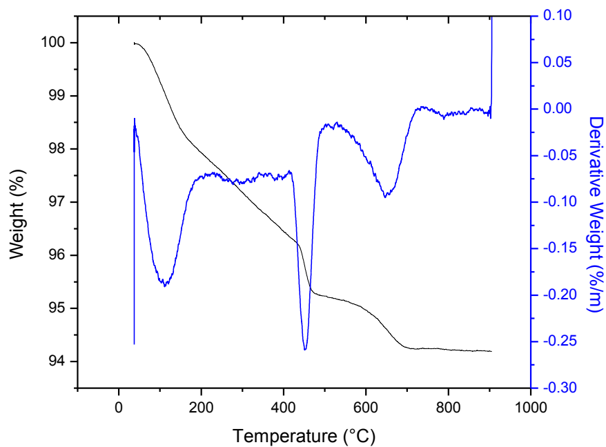
Figure C21: TGA/DTA curves for FA-60 -28
