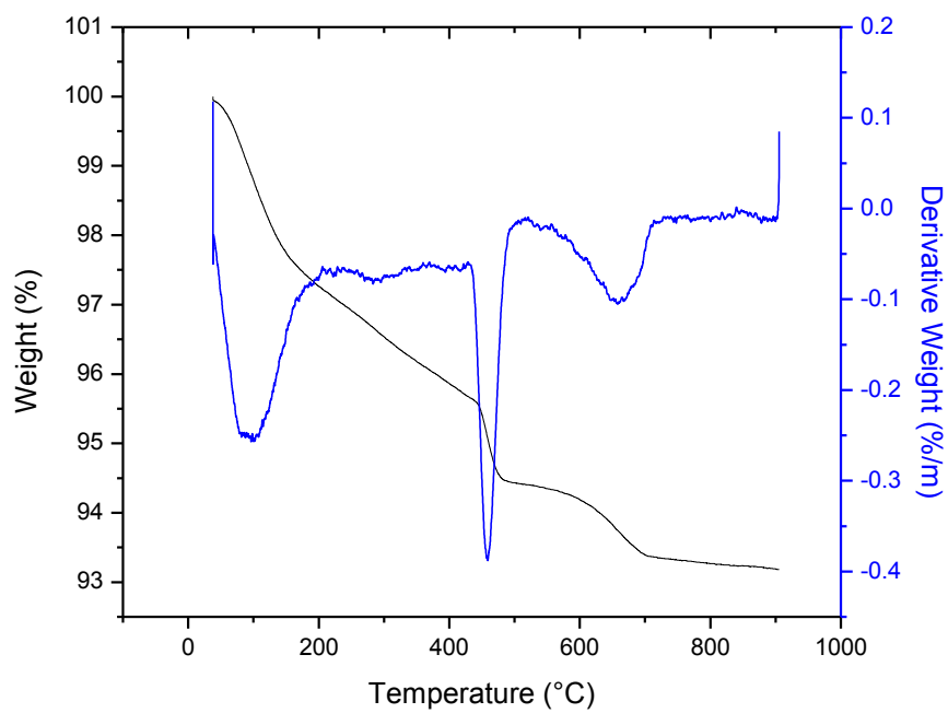
Figure C6: TGA/DTA curves for PC-50 -28
