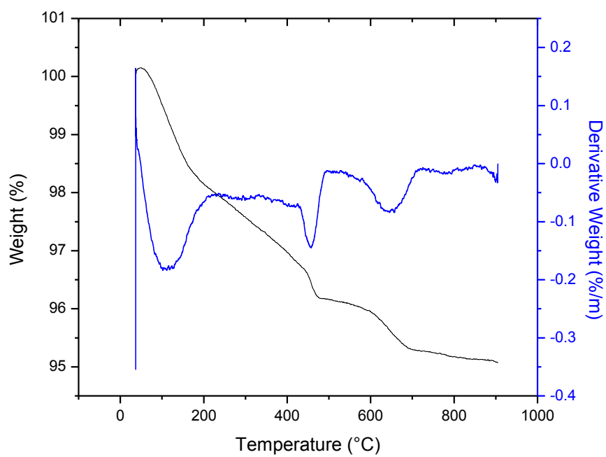
Figure C26: TGA/DTA curves for SL-50 -7
