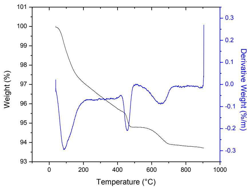
Figure C45: TGA/DTA curves for SF-75 -28
