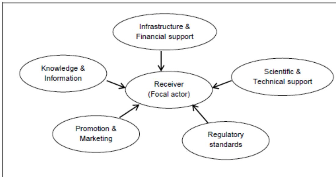
Figure 4.9: Actor contributions
