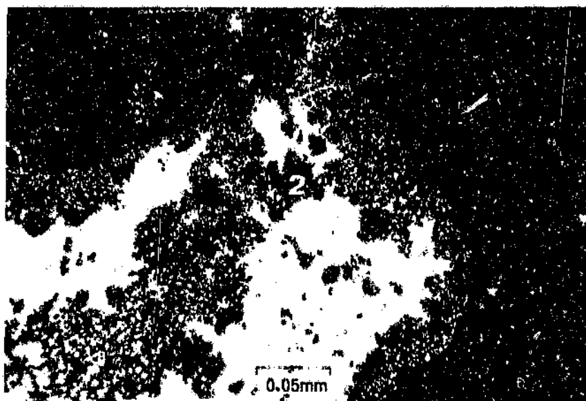
Figure 5.8: Stibnite (Sb) being replaced firstly by chalcocite (1) and/or native antimony (1) and thereafter by metacinnabarite and/or fahlors (2), in a second generation gangue, SPD-083, 221m, (120 X, reflected light).
