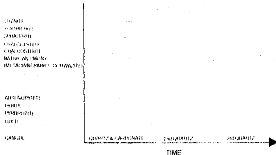
Figure 5.26: Ore paragenesis of the "A" Zone mineralization, Signal Hill area.
