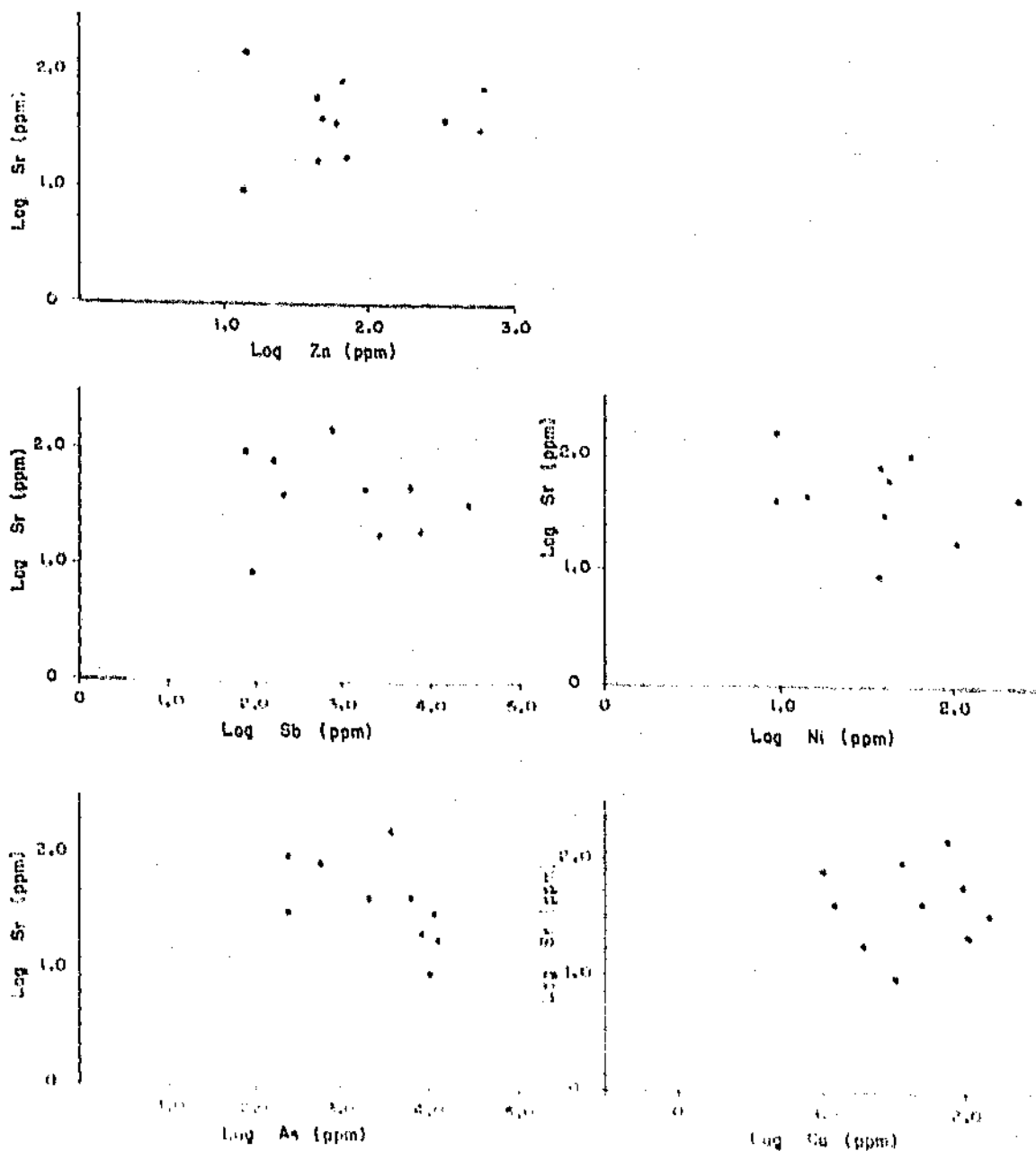
Figure 6.10: Variation diagrams for As, Sb, Zn, Ni and Cu with Sr, samples are listed in Appendix IV.
