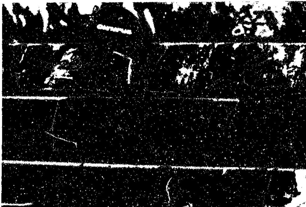
Figure 3.20: Quartz wacke's matrix partially replaced by carbonatization, SPD-066, 75m.
