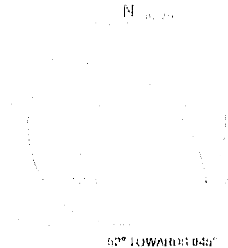
Figure 4.12: Cyclographic trace shows the cleavage dipping at 62° towards 045°.
