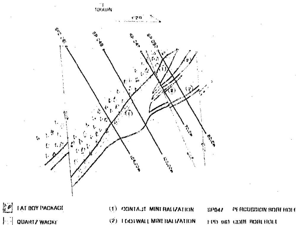
Figure 5.1 : Cross-section showing both the Contact mineralization and the Footwall mineralization, along the line 9875 E ("A" Zone grid).
