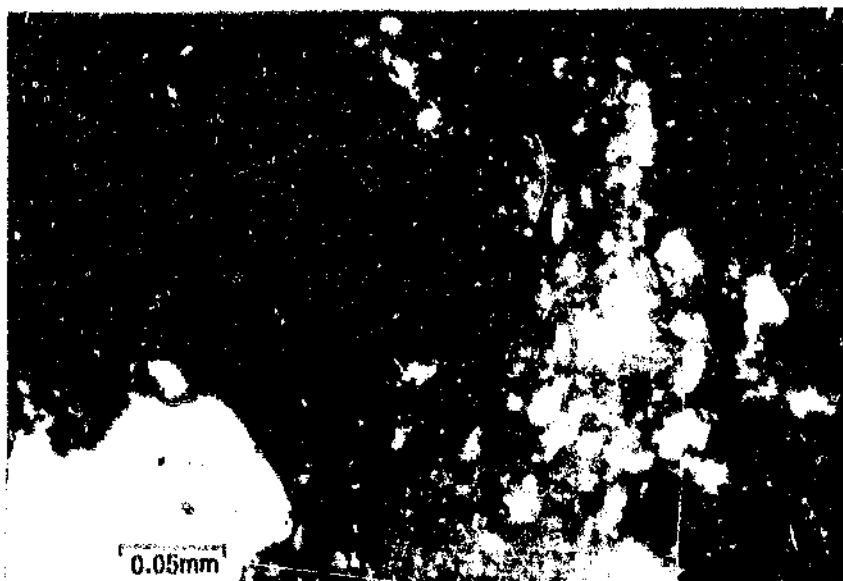
Figure 5.19: Brocciated early sphalerite in a quartz-carbonate, first generation gangue material, thereafter affected by a later tectonic event and the associated second gangue generation and the growth of arsenopyrite, SD-003, 55m (320 X, reflected light)
