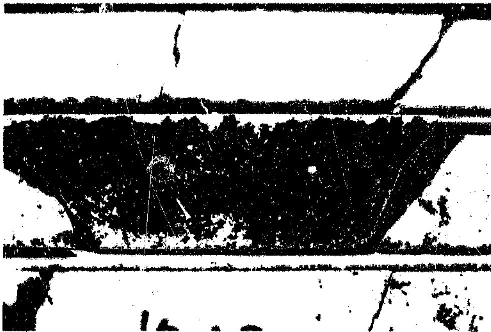
Figure 5.6: Silicified quartz wacke, tectonically brecciated and thereafter altered by the precipitation of pyrite and arsenopyrite by mineralizing fluids, SPB-003, sample 10426.
