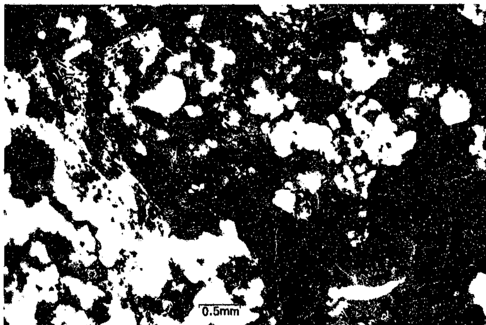
Figure 5.23: Footwall vein with stibnite-berthierite-sphalerite mineralization. The gangue is composed almost exclusively of quartz, SPD-083, 220m, (25 X, + Nic).
