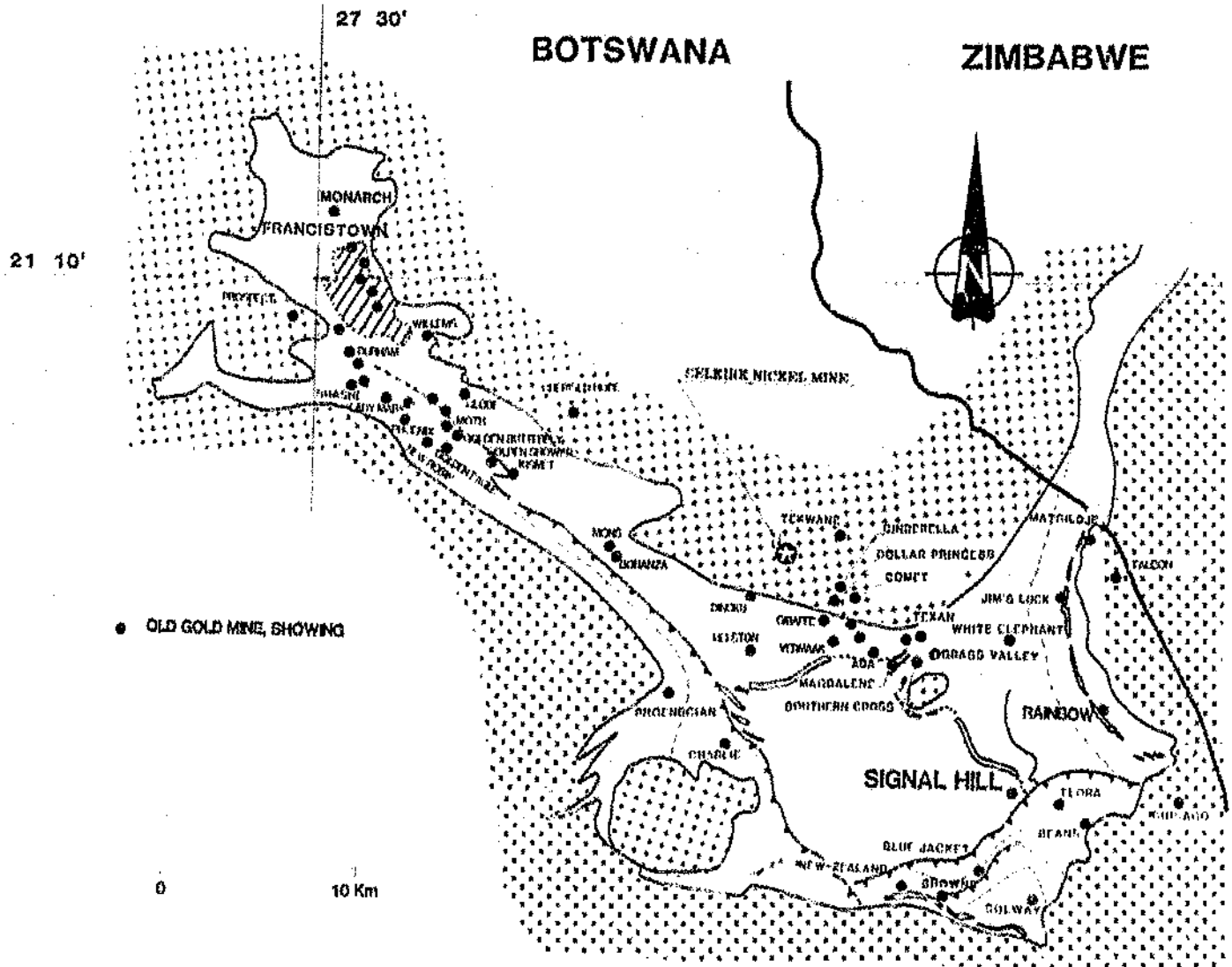
Figure 1.3: Location of Selkirk nickel mine and old gold mines and showings, Tati schist belt, modified after Key (1976).
