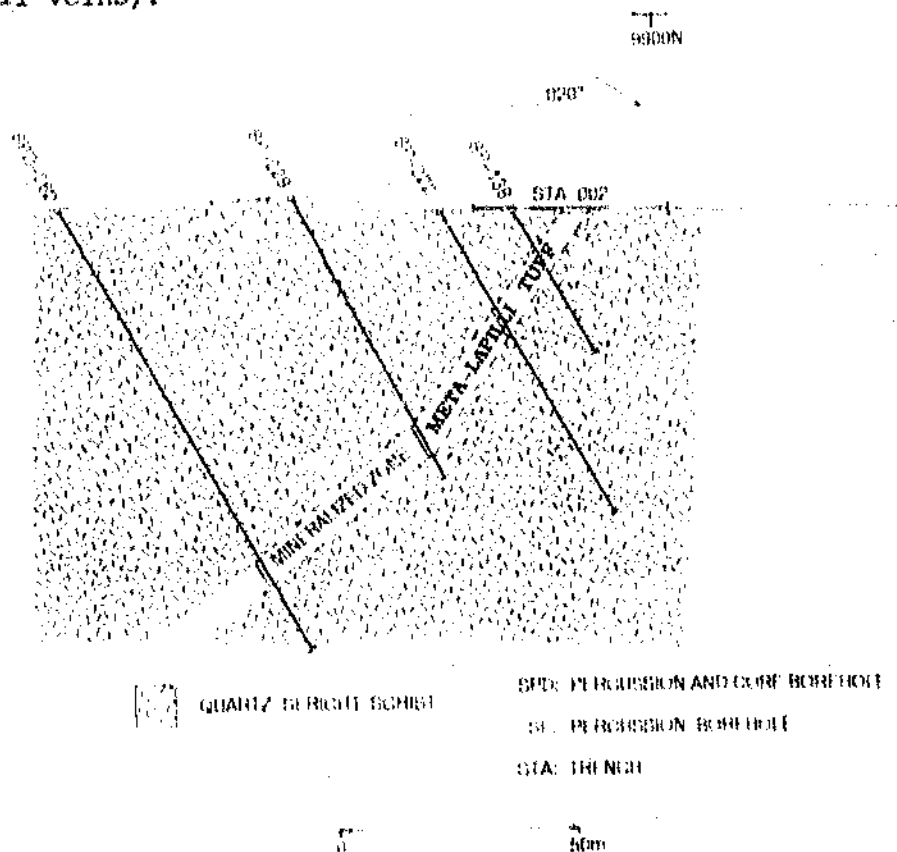
Figure 5.7: Cross section through the "F" Zone, the section is located along line 11285E (Appendix IX).
