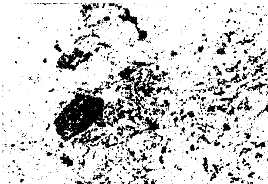
Figure 3.14: Very rare zircon within a quartz wacke, SD-077, 64m, 200 X.
