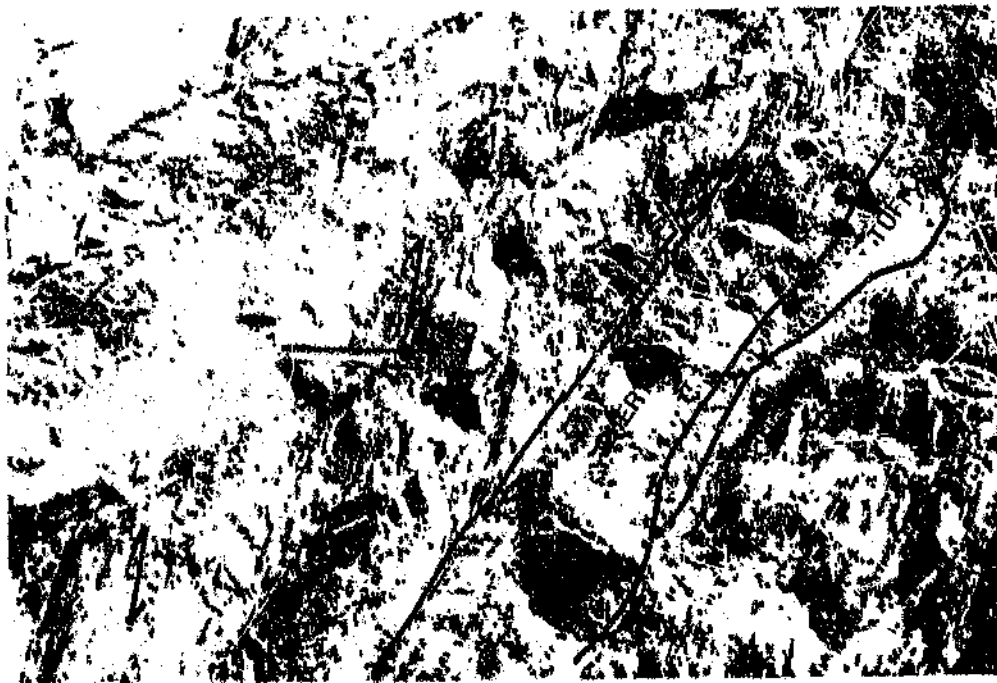
Figure 2.6: Rock succession showing light-grey and well-banded chert units with felsic meta-tuff. A basal chert unit (1) shows an erosive contact infilled with meta-tuff material (2). The felsic meta-tuff contains the well-developed regional schistosity.
