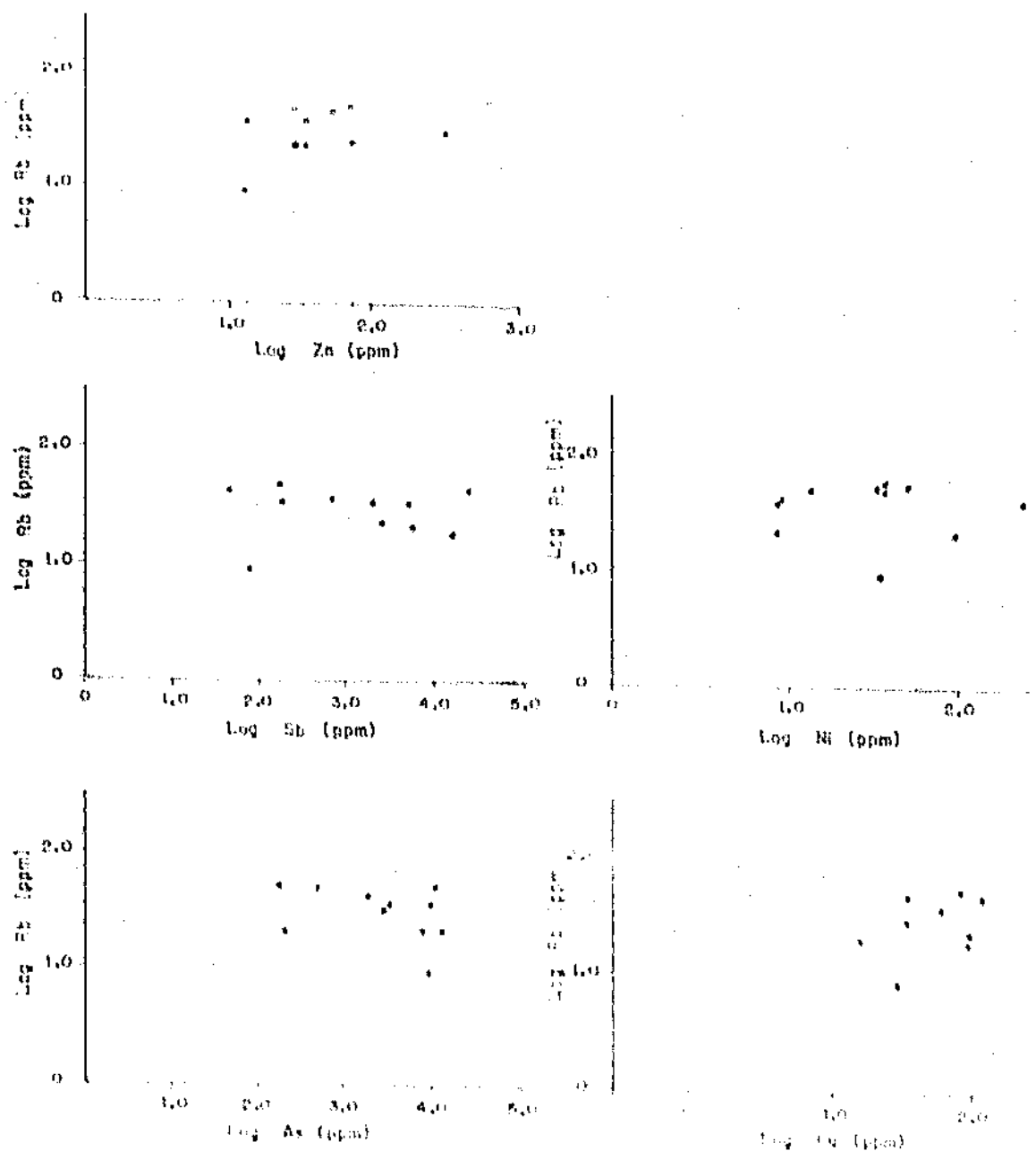
Figure 6.11: Variation diagrams for As, Sb, Zn, Ni and Cu with Rb, samples are listed in Appendix IV.
