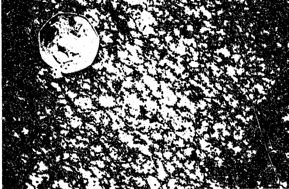
Figure 2.7: Highly deformed granitoid rock located at the contact between the New Zealand batholith and the Matsiloje Formation (Appendix VII).
