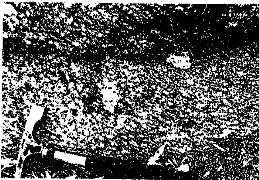
Figure 2.10: Sheared granodiorite rock located at the margin of the Hill View pluton, see Appendix VII.
