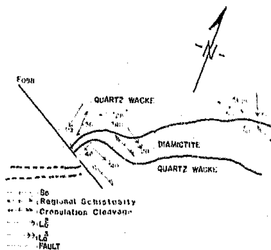
Figure 4.8: Figure showing structural relationship at the "A" Zone, between S0, S2, the normal fault F098 and the crenulation cleavage.
