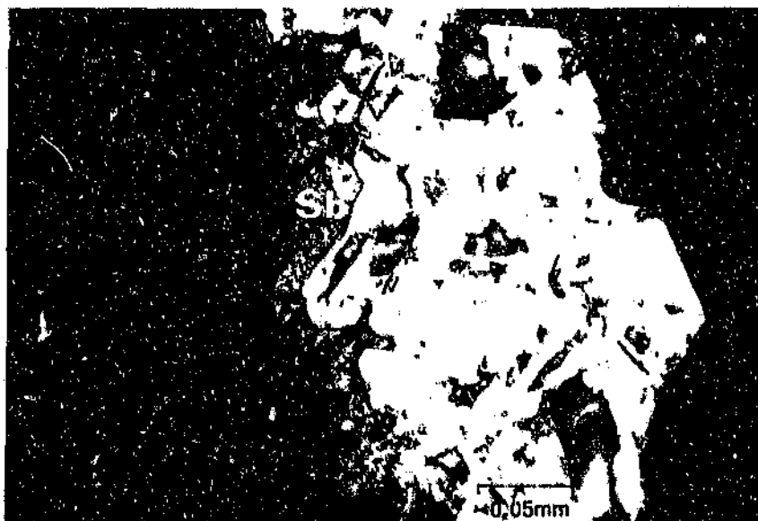
Figure 5.15: Stringer of remobilized stibnite located adjacent to a pyrite crystal, SPD-083, 221m, (320X, reflected light).
