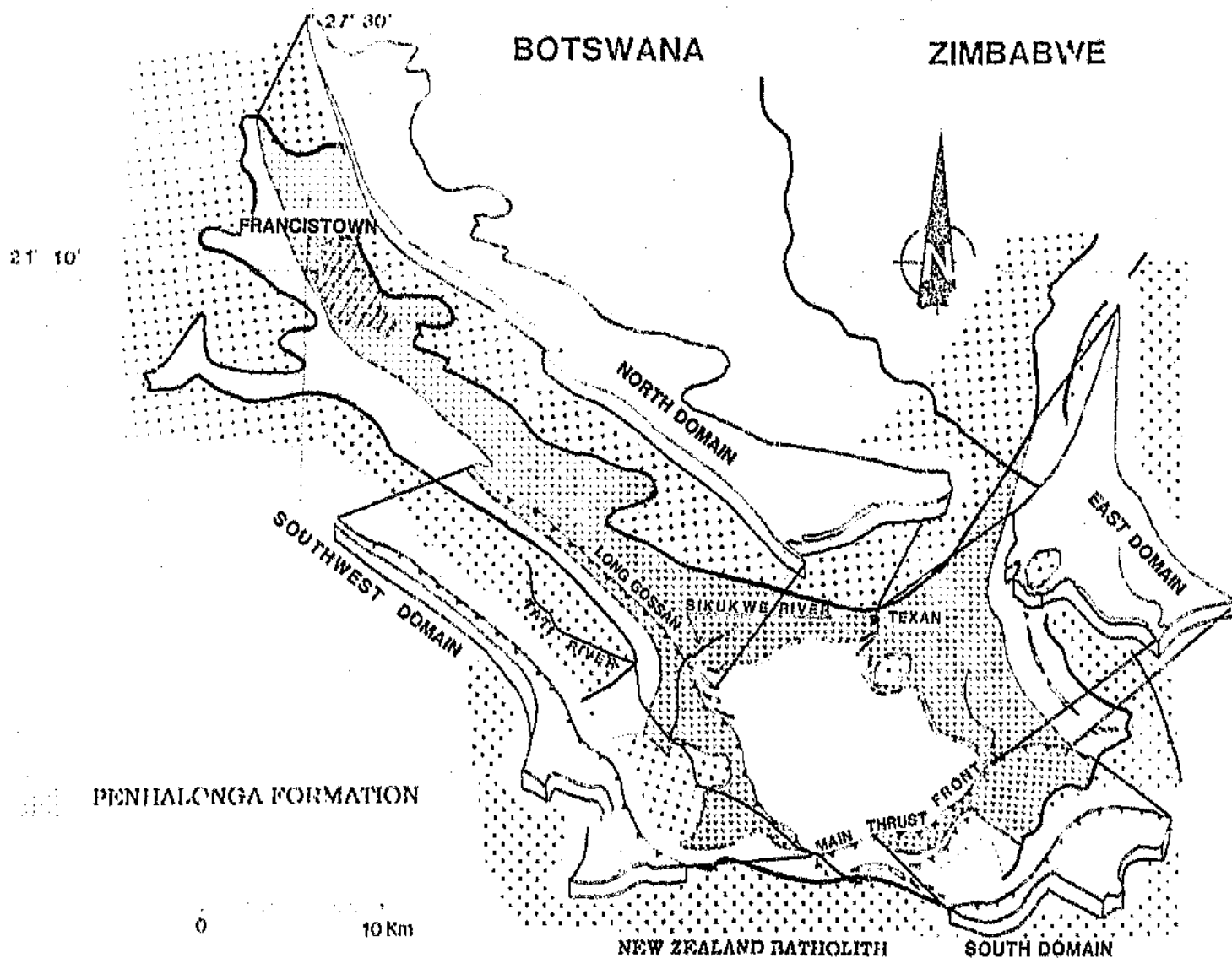
Figure 2.3 : Subdivision into four distinct structural domains of the Penhalonga Formation.
