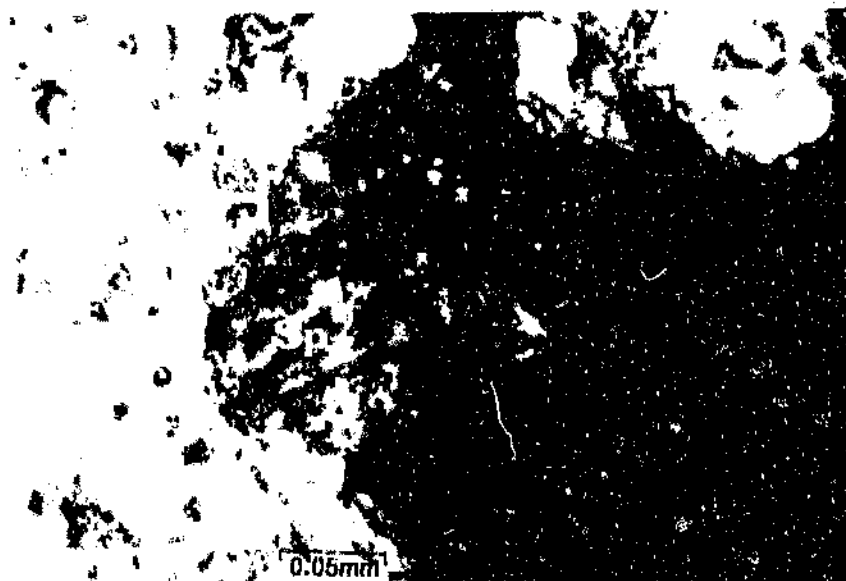
Figure 5.17: Brecciated early sphalerite (Sp) cut off by a late pyrite crystal (Py). Assemblage occurs within the second gangue generation, SD-107, 126m, (320 X, reflected light).
