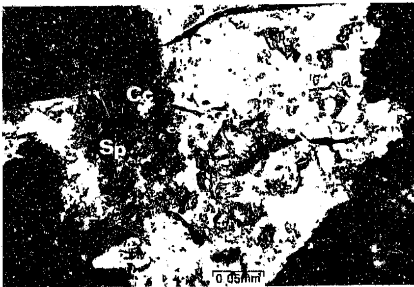
Figure 5.12: Stibnite (Sb) and berthierite (Be) (replaced by chalcostibite and/or native antimony) in close relationship with sphalerite (Sp) and chalcopyrite (Cc), SPD-083, 255m, (320 X, reflected light).
