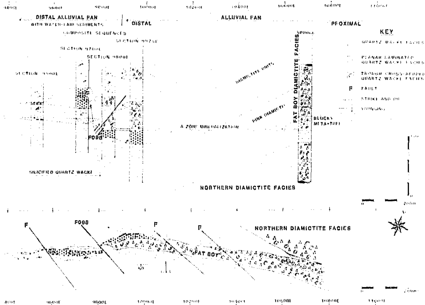
Figure 3.11: Figure showing the composite sequences and surface geology of the "A" Zone. Composite sequences were constructed from data from boreholes and trenches along each sections.
