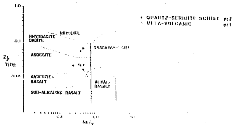
Figure 6.2: Zr/TiO_2 - Nb/Y plot showing the classification of the volcanic rocks of the upper Penhalonga Formation (after Floyd and Winchester, 1978).
