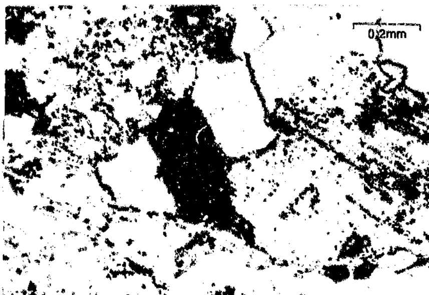
Figure 3.13: Rare twinned plagioclase crystal associated with quartz fragments in a quartz-sericite matrix, SP-077, 62m, 100 X, X nic.
