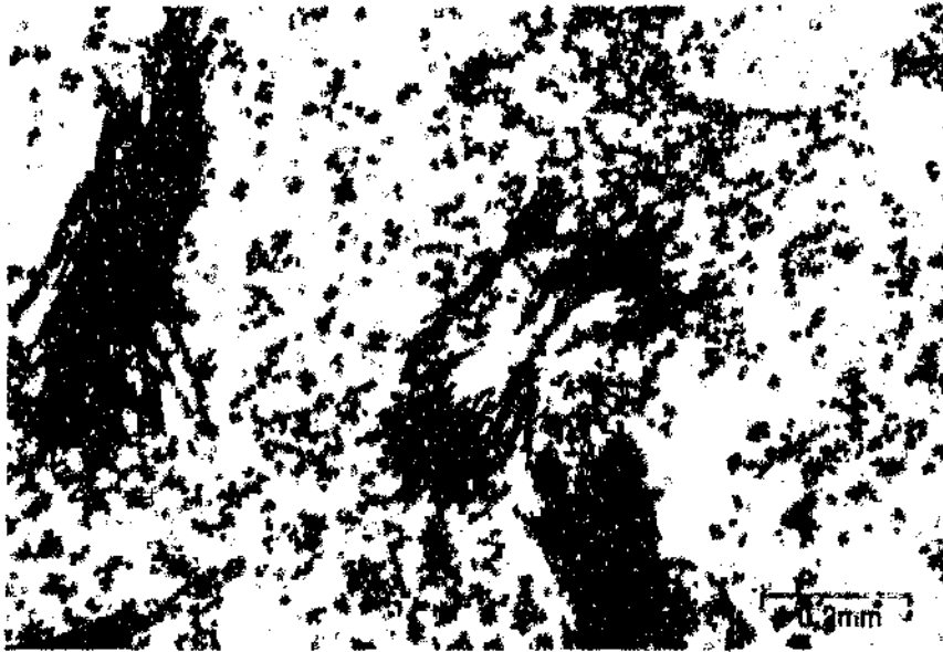
Figure 3.41: Porphyroblast of epidote being replaced by iron oxide, STD-061, 53m, 100 X.
