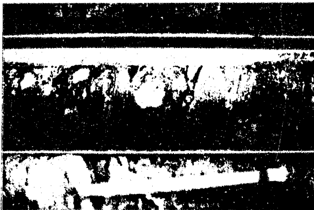
Figure 3.18: Diamictite showing sub-angular quartz and ironstone clasts and sub-angular to angular and flattened volcanic fragments in a fine carbonated matrix. The sediment is matrix supported, 69B-003, 1976.
