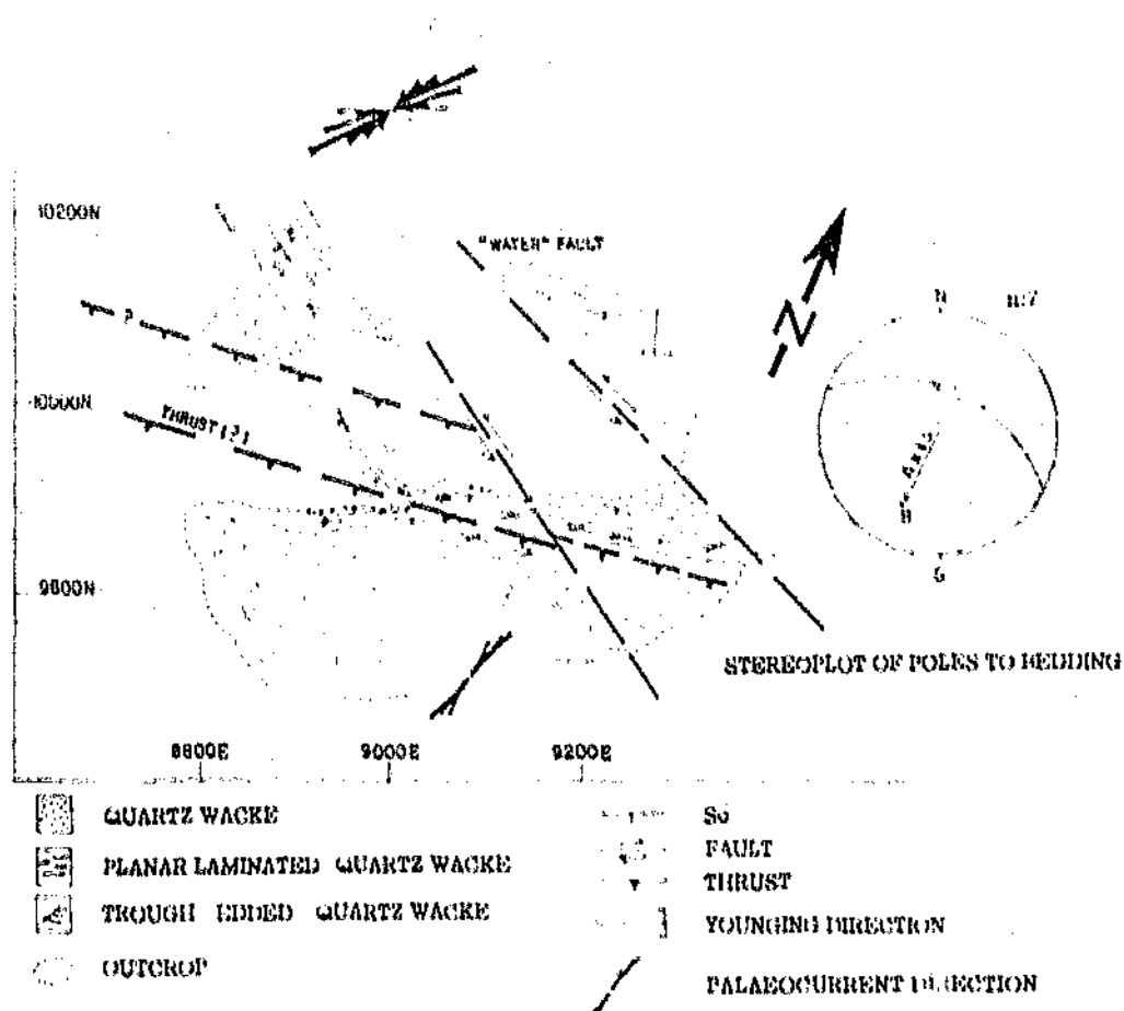
Figure 4.2: Detail of the antiform located approximately 1 Km west of the "A" Zone.
