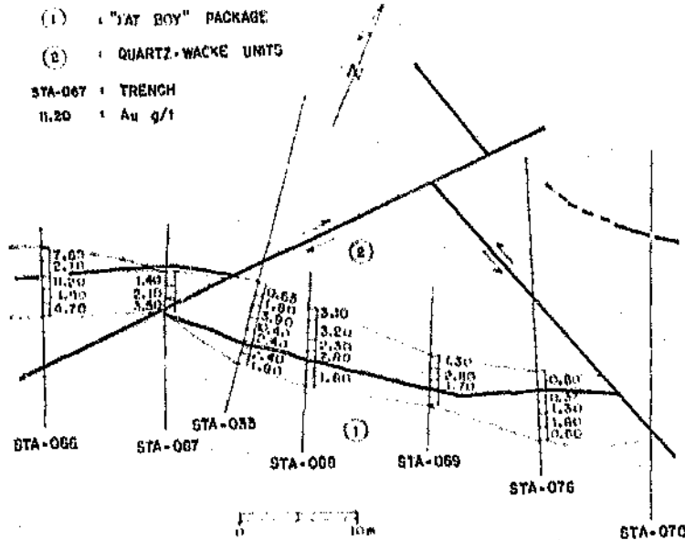
Figure 5.2: Distribution of gold within the "A" Zone ore body. The ore body is defined by a cut-off grade of 0.5 Au g/t.
