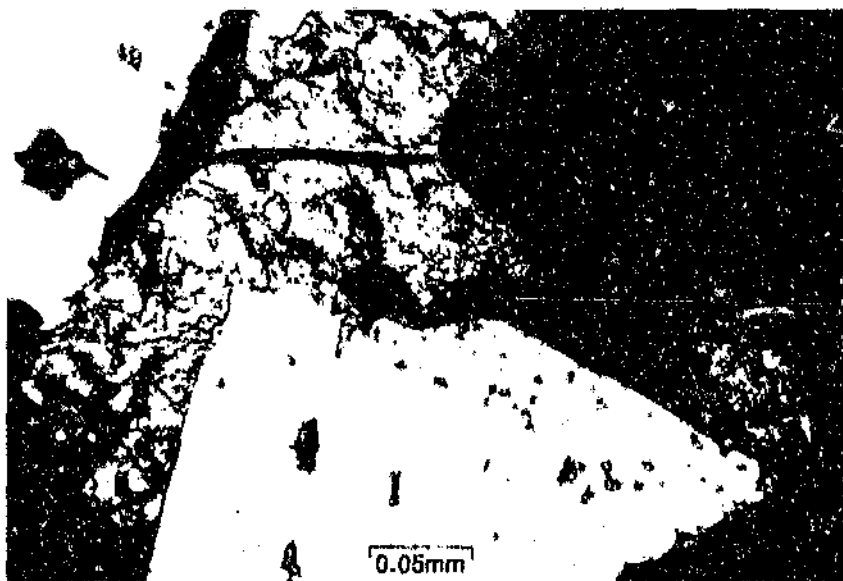
Figure 5.13: Stibnite (Sb) affected by a later tectonic event (fractures infill by the second generation of gangue material) and the growth of late euhedral arsenopyrite (Apy), SP-003, 221m, (320 X, reflected light).
