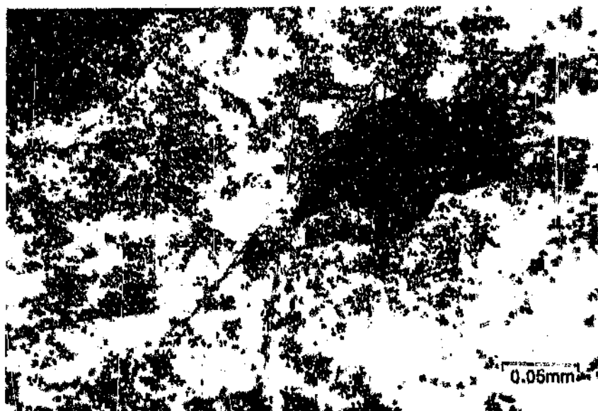
Figure 5.9: Stibnite (Sb) with inclusions of native antimony (1) and/or chalcocite (1) (high reflectance, white, top left) SPD-083, 220m, sample 10310 (120 X, reflected light).
