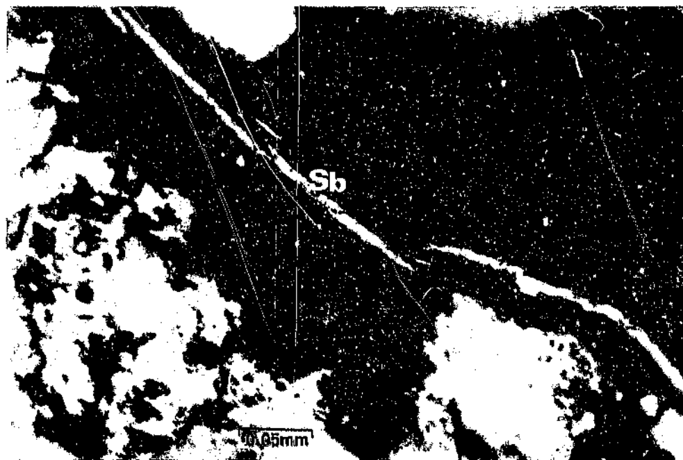
Figure 5.11: Remobilized stibnite as fine stringers in fractures created by a later tectonic event. sphalerite (Sp) occurs at the bottom left. SPD-083, 221m, (320 X, reflected light).
