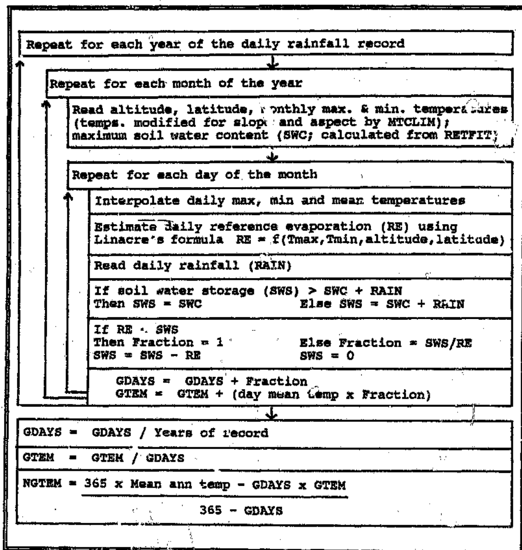
Figure 5.3: Schematic representation of the water balance model used to generate the indices of growth days (GDAYS), growth temperature (GTEM) and no-growth temperature (NGTEM), and including the effects of soil moisture properties.
