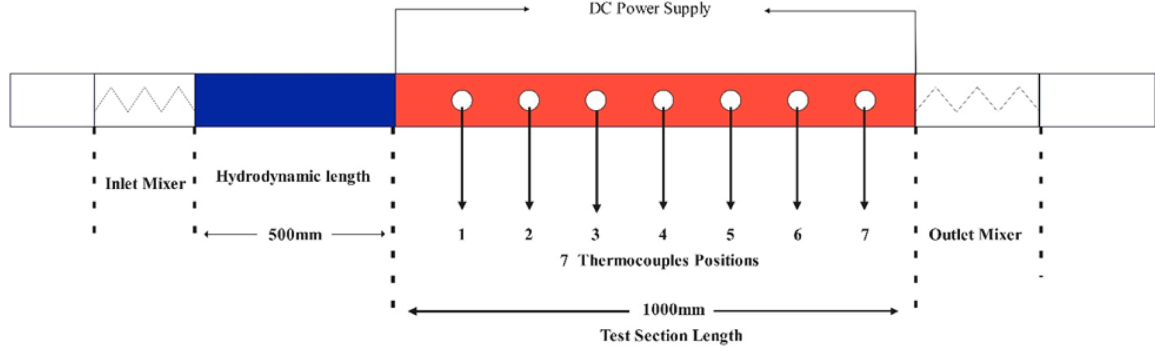
Fig. 6. Schematic diagram of test section.
