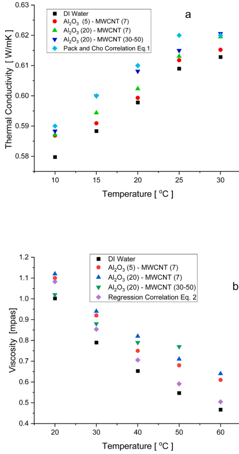
Fig. 3. a) Thermal conductivity and b) Viscosity of hybrid nanofluids.
