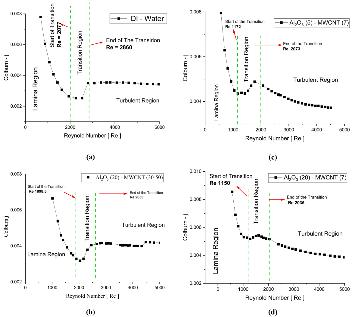
Fig. 11. Colburn-J factor versus Re for identification of lamina, transition, and turbulent regions for (a) DI water, (b) \text{Al}_2\text{O}_3 (20) – MWCNT(30–50), (c) \text{Al}_2\text{O}_3 (5) – MWCNT(<7), (d) \text{Al}_2\text{O}_3 (20) – MWCNT(<7).
