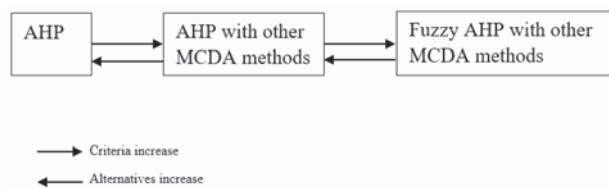
Figure 5—Impact of different combinations of MCDA methods on criteria and alternatives
