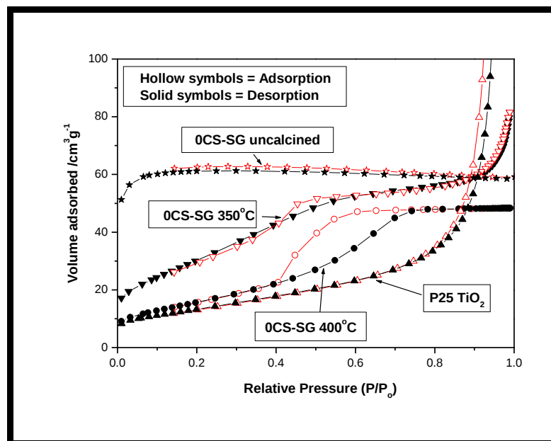
Figure 4.22 Nitrogen adsorption-desorption isotherms of calcined (350 °C) P25 TiO 2 , uncalcined 0CS-SG, and calcined 0CS-SG (at 350 and 400 °C)
