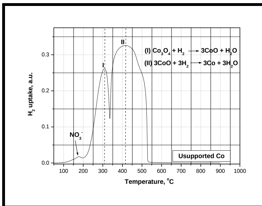
Figure 5.7 TPR of uncalcined unsupported cobalt oxide precursor
