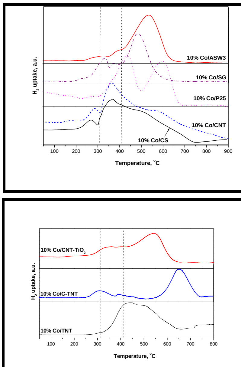
Figure 5.10 H 2 -TPR of calcined supported cobalt catalysts
