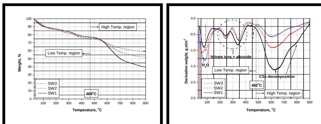
Figure 4.33 TGA (left) and DTG (right) of uncalcined SW1, SW2 and SW3
