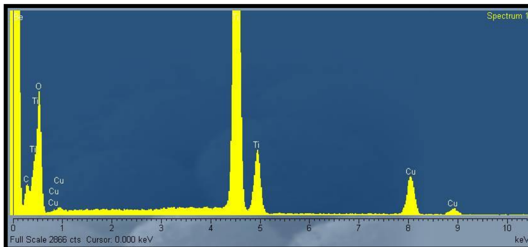
Figure 4.27 EDX spectrum corresponding to the F-CS surface coverage by TiO 2 shown in Fig. 4.25 (f). C and Ti were detected; the Cu signal corresponds to the Cu grid substrate used for TEM analysis.
