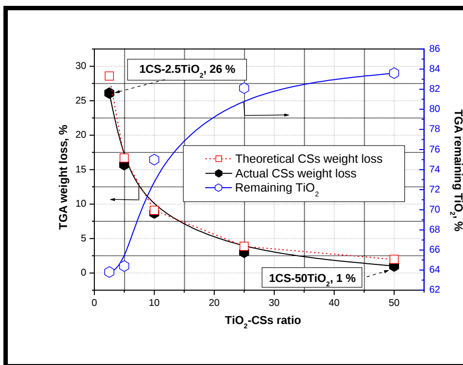
Figure 4.13 Analysis of CSs weight loss and residue TiO 2 for the composite samples as a function of CS-TiO 2 composite ratio. Data were obtained from TGA measurements.
