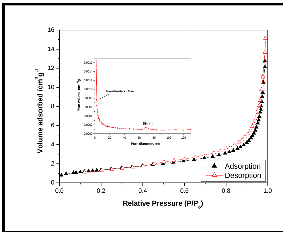
Figure 4.21 Nitrogen adsorption-desorption isotherm and its BJH pore size distribution curve ( inset ) of F-CS
