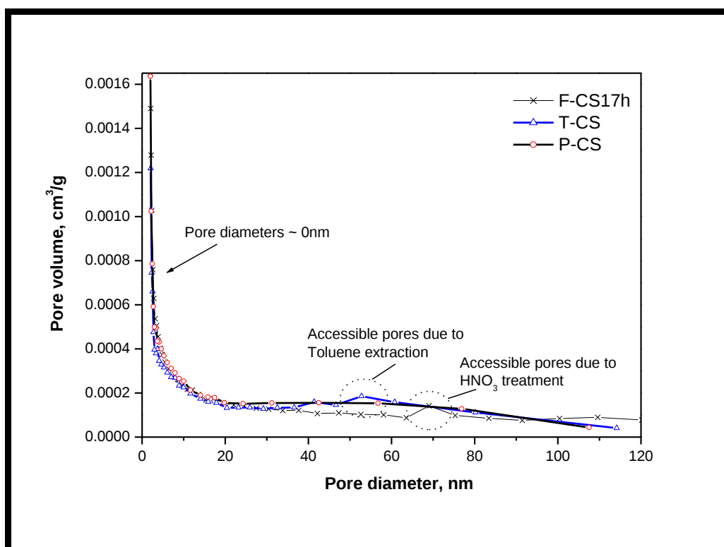
Figure 3.15 BJH pore size distributions (calculated from the adsorption arms of N_2 isotherms) of P-CS, T-CS and F-CS17h
