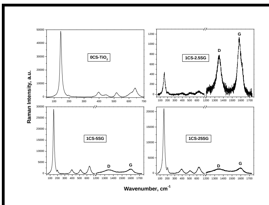
Figure 4.20 Raman spectra of calcined bulk 0CS-SG (calcined at 400 °C) and calcined CS-TiO 2 composites prepared by conventional sol-gel with ratios of: 1CS-2.5SG, 1CS-5SG and 1CS-25SG (calcined at 400 °C).
