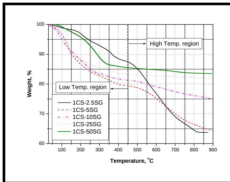
Figure 4.11 TGA uncalcined 1CS-2.5SG, 1CS-5SG, 1CS-10SG, 1CS-25SG and 1CS-50SG
