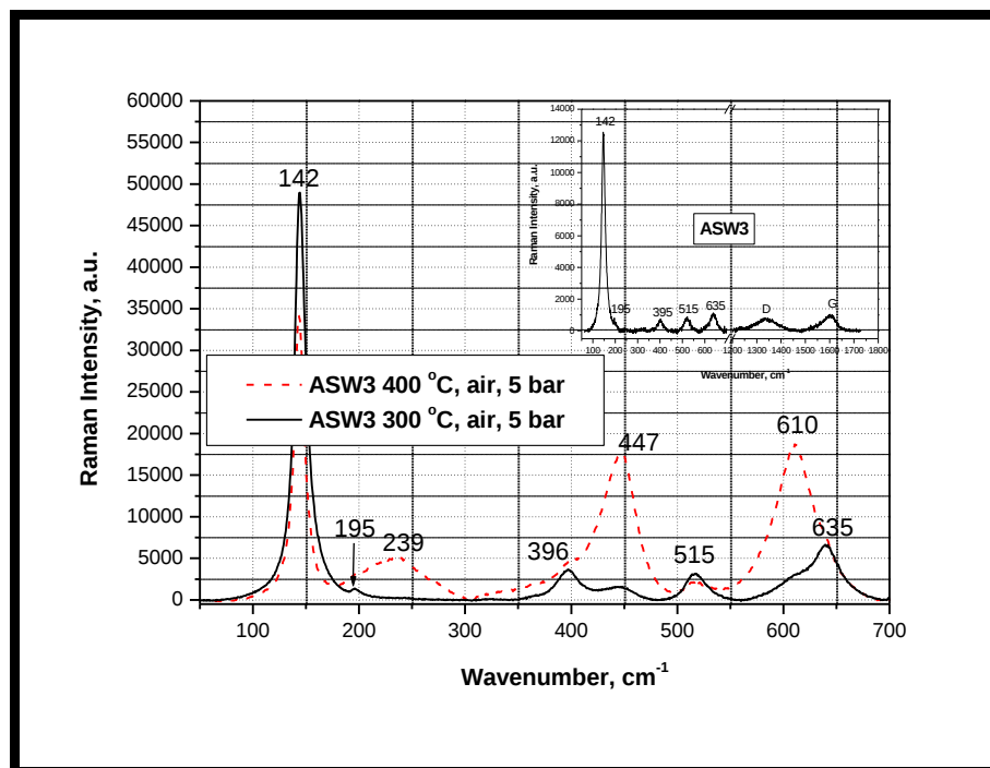
Figure 4.31 Raman spectra of \text{TiO}_2 residue from combusted ASW3 composite sample. Samples were combusted in air at 5 bar for 6h at: (a) 300 °C and, (b) 400 °C. Raman spectra of bulk uncombusted ASW3 is shown on the inset .
