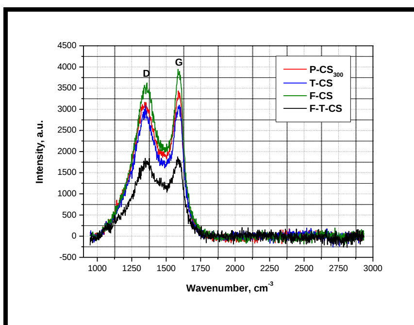
Figure 3.12 Raman spectra of P-CS produced at 300 mL/min, T-CS, F-CS and F-T-CS
