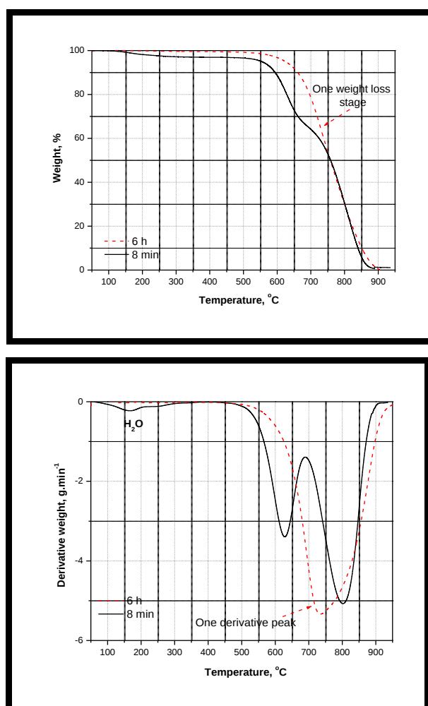
Figure 3.10 TGA ( top ) of P-CS left in the quartz reactor for 8 min and 6 h with their respective DTG ( bottom ) curves
