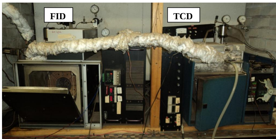
Figure 2.9 Gas chromatography one fitted with FID and the other with a TCD detector
