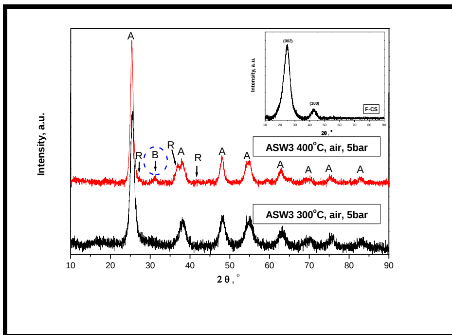
Figure 4.30 XRD patterns of \text{TiO}_2 residues from combusted ASW3 composite material where A = anatase phase, B = brookite and R = rutile phase. Samples were combusted in air at 5 bar for 6h at: 300 °C and at 400 °C, respectively. XRD pattern of the F-CS is shown on the inset .
