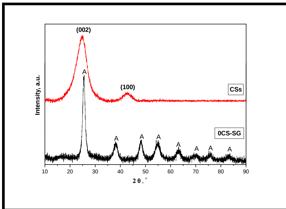
Figure 4.16 XRD patterns of calcined sol-gel derived \text{TiO}_2 (0CS-SG) and F-CS. The peaks marked with (A) and (002, 100) correspond to \text{TiO}_2 (anatase) and CSs, respectively
