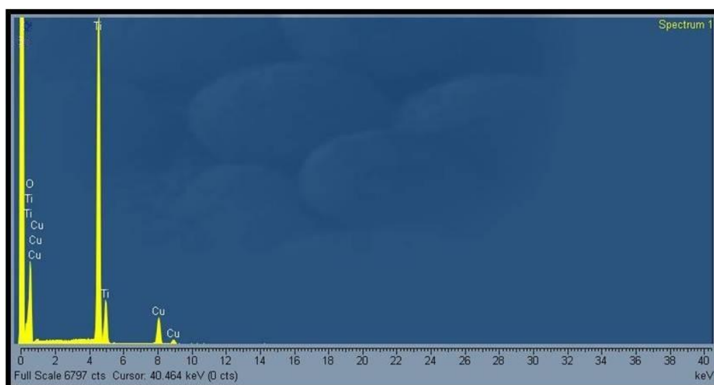
Figure 4.29 EDX spectrum of \text{TiO}_2 residue corresponding to sample (b) in Fig. 4.28
