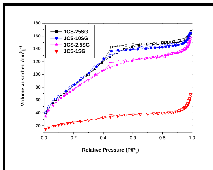
Figure 4.23 Nitrogen adsorption-desorption isotherms of 1CS-1SG, 1CS-2.5SG, 1CS-10SG, and 1CS-25SG
