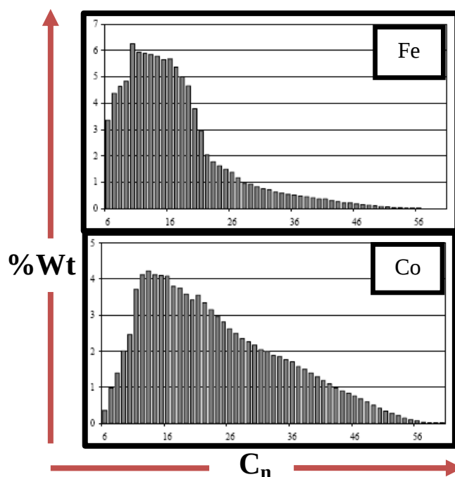
Figure 1.5 Product distribution with iron and cobalt based catalysts [31]
