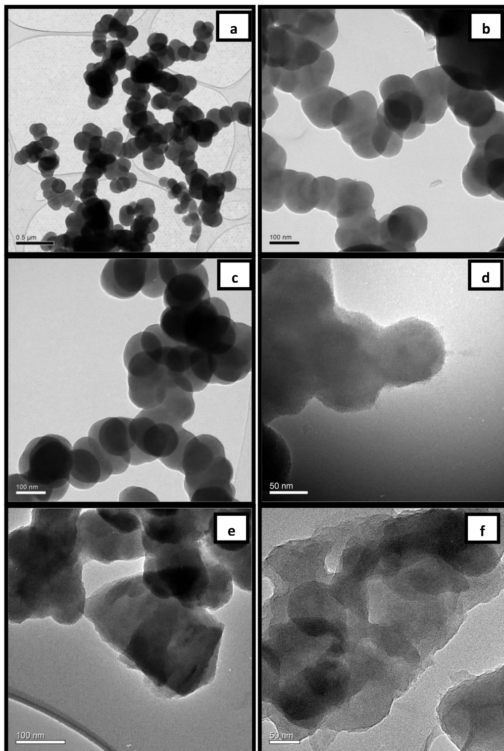
Figure 3.14 TEM micrographs of CSs: (a) P-CS, (b) T-CS, (c) F-CS17h, (d) F-CS24h, (e) F-CS30h and (f) F-CS40h
