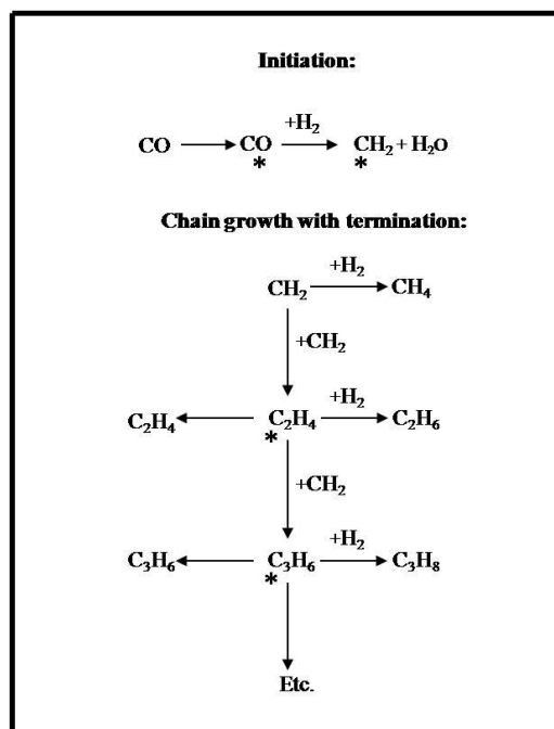
Figure 1.3 Simple FT stepwise growth process (where ‘*’ symbolises a surface). Adapted from [24]
