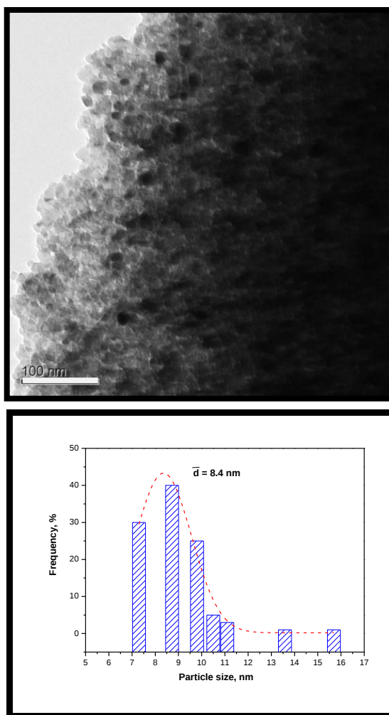
Figure 4.4 TEM image of pure TiO 2 ( top ) and particle size distribution ( bottom ) prepared without the presence of CSs by a conventional sol-gel method. (Solid line = particle size distribution histogram, and dashed line = Gaussian distribution).
