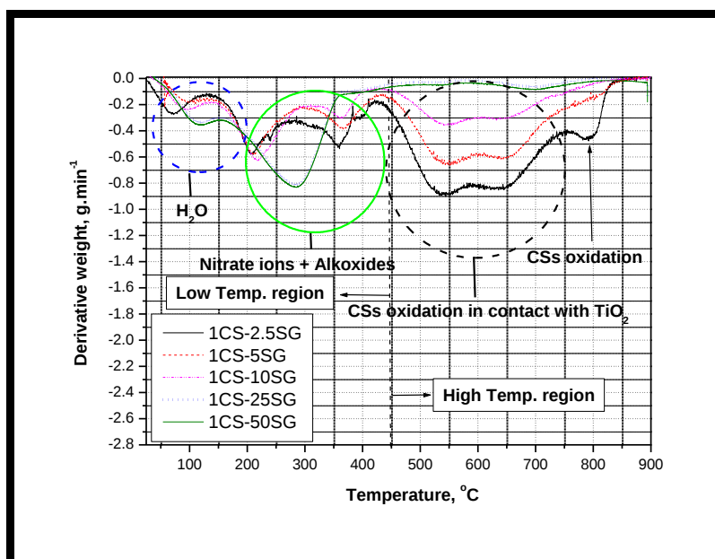
Figure 4.12 DTG of uncalcined 1CS-2.5SG, 1CS-5SG, 1CS-10SG, 1CS-25SG and 1CS-50SG
