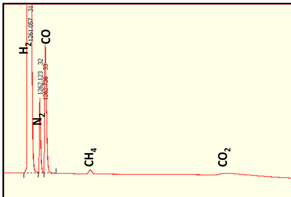
Figure 2.12 A typical product and unreacted syngas spectrum using TCD-GC
