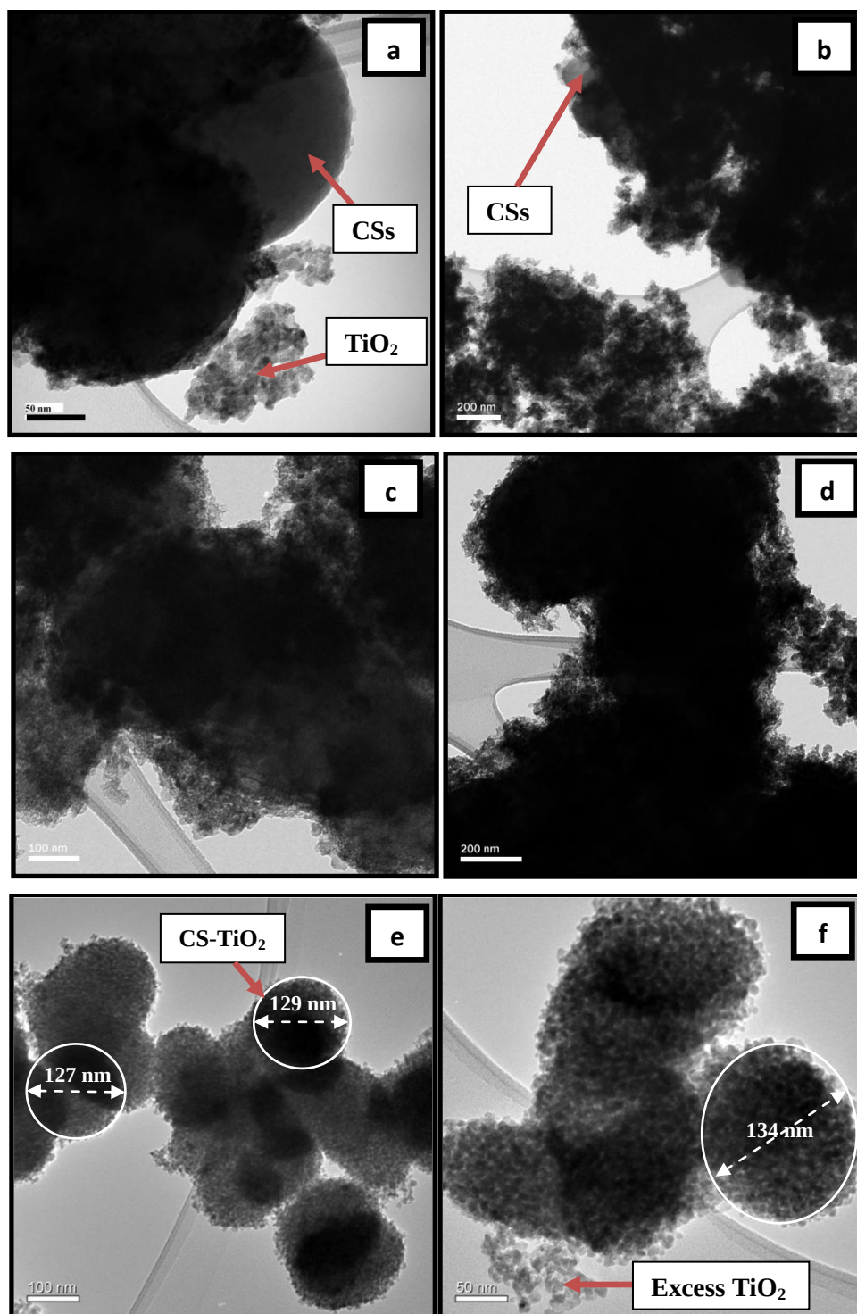
Figure 4.25 TEM images of CS-TiO 2 composites prepared by a surfactant wrapping sol-gel method, for: (a) A1, (b) A3, (c) SW1, (d) SW3, (e) ASW1 and (f) ASW3, where (A = acid treated but not surfactant wrapped CSs, SW1 = surfactant wrapped, but not acid treated CSs, ASW = acid treated and surfactant wrapped CSs ). 1 and 3 represents the number sol-gel coating cycles
