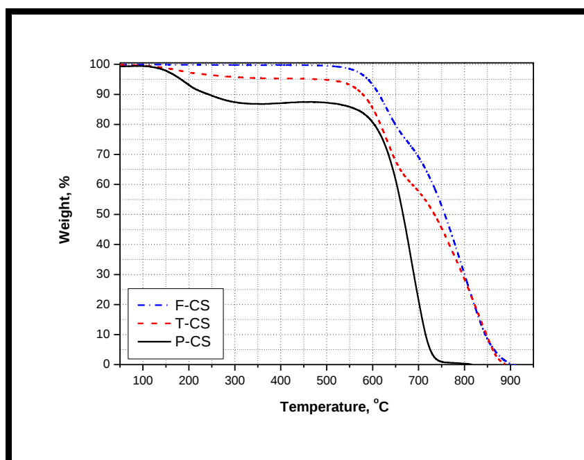
Figure 3.13 TGA of P-CS, soxhlet extracted CSs and F-CS
