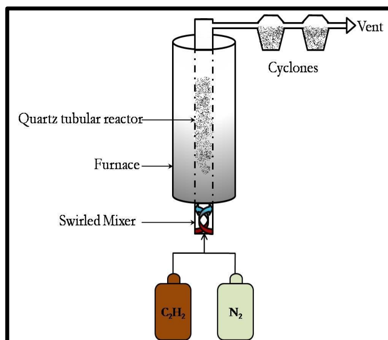
Figure 3.2 Schematic representation of a vertically positioned swirled floating chemical vapour deposition reactor setup.
