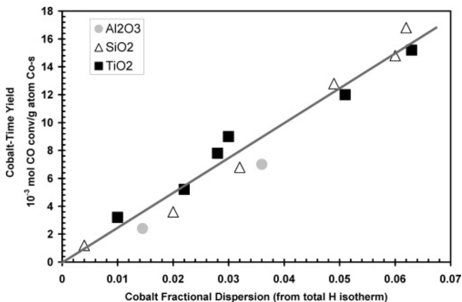
Figure 5. 1 Cobalt time yield for a variety of \text{Co}/\text{Al}_2\text{O}_3 , \text{Co}/\text{SiO}_2 and \text{Co}/\text{TiO}_2 supported catalysts. Adapted from [9].
