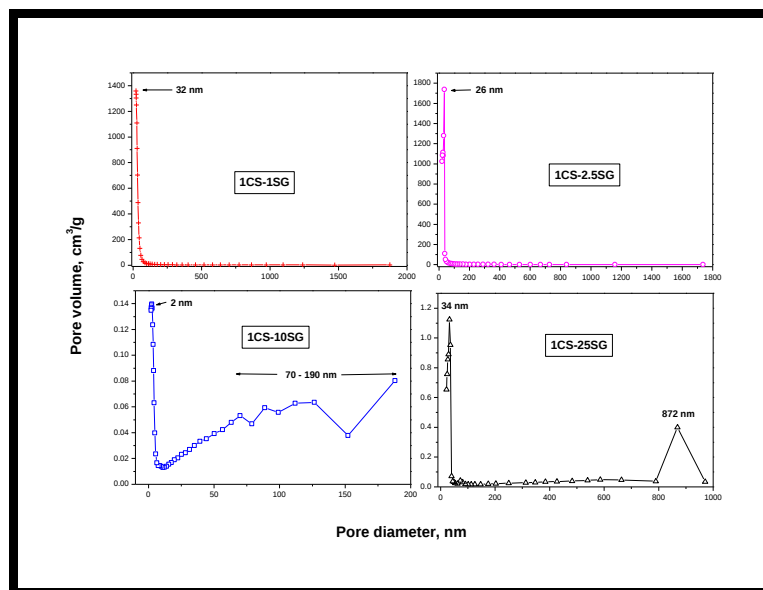
Figure 4.24 BJH pore size distributions (calculated from the adsorption arms of N_2 isotherms) of 1CS-1SG, 1CS-2.5SG, 1CS-10SG, and 1CS-25SG
