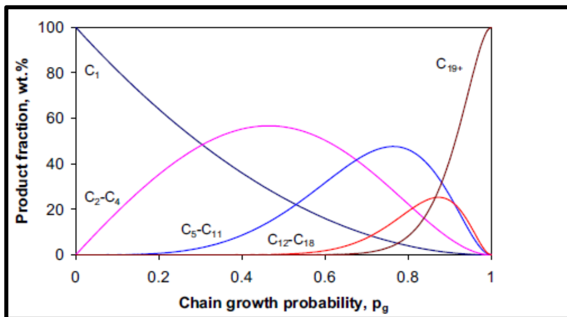
Figure 1.4 Theoretical FTS product distribution of products produced by the Anderson-Schulz-Flory model as a function of chain growth probability [30]
