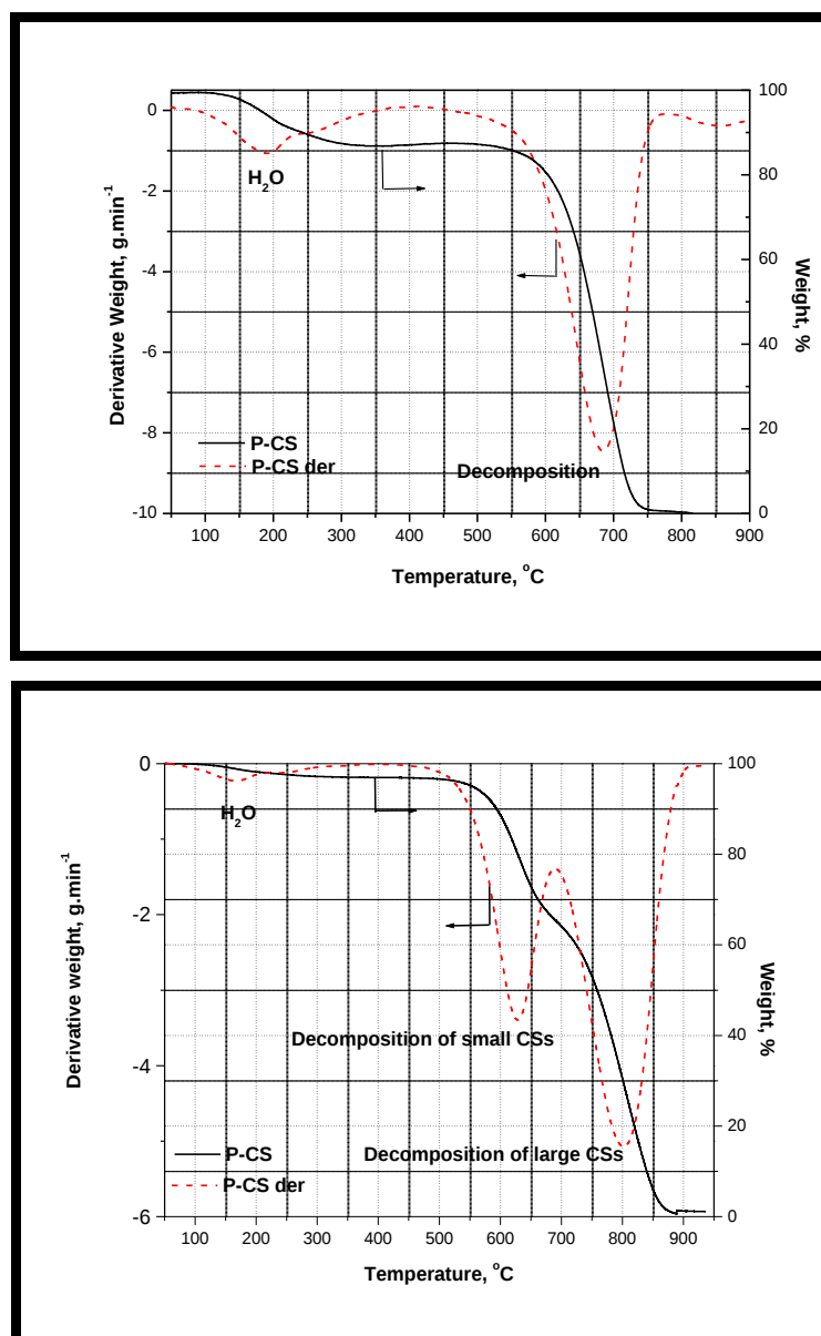
Figure 3.8 TGA and DTG of P-CS left in the quartz reactor for: 4 min ( top ) and 8 min ( bottom )
