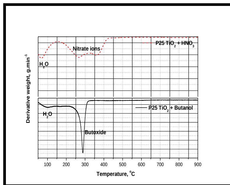
Figure 4.10 DTG of P25 TiO 2 mixed with HNO 3 and P25 TiO 2 mixed with butanol
