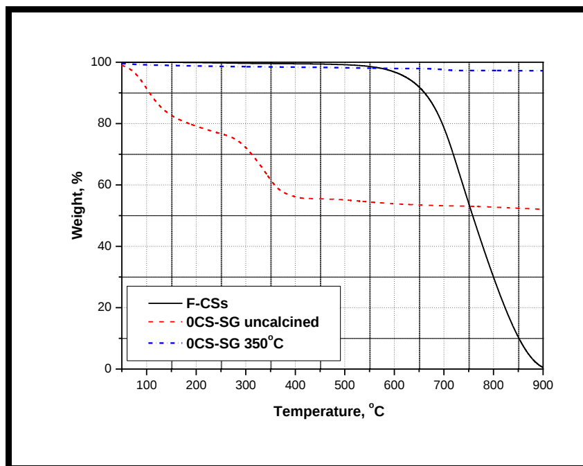
Figure 4.7 TGA profiles of the F-CS, uncalcined 0CS-SG and the calcined 0CS-SG (350 °C) samples
