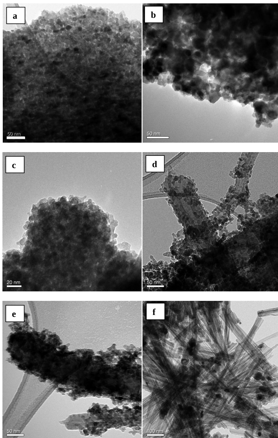
Figure 5.3 TEM images showing cobalt dispersed at different supports: (a) 10%Co/SG, (b) 10%Co/P25, (c) 10%Co/ASW3, (d) 10%Co/CNT, (e) 10%Co/CNT-TiO 2 and (f) 10%Co/TNT
