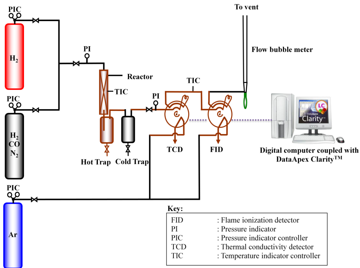
Figure 2.8 A schematic diagram for the reactor system
