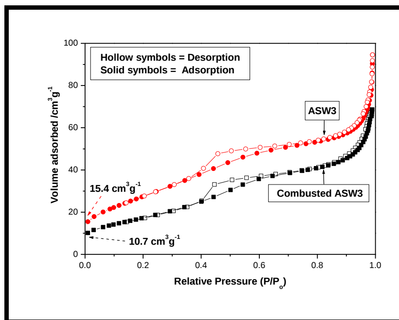
Figure 4.35 Nitrogen adsorption-desorption isotherms of uncombusted ASW3 composite, calcined in air (300 °C, 6 h, 1 bar) and TiO 2 residue from combusted ASW3 at 400 °C in air 6h 5 bar
