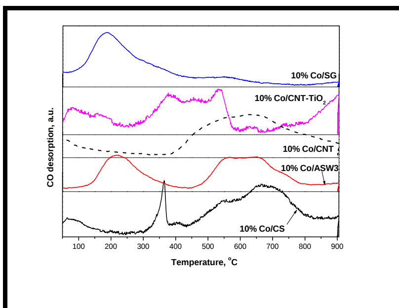
Figure 5.12 CO-TPD of calcined supported cobalt catalysts
