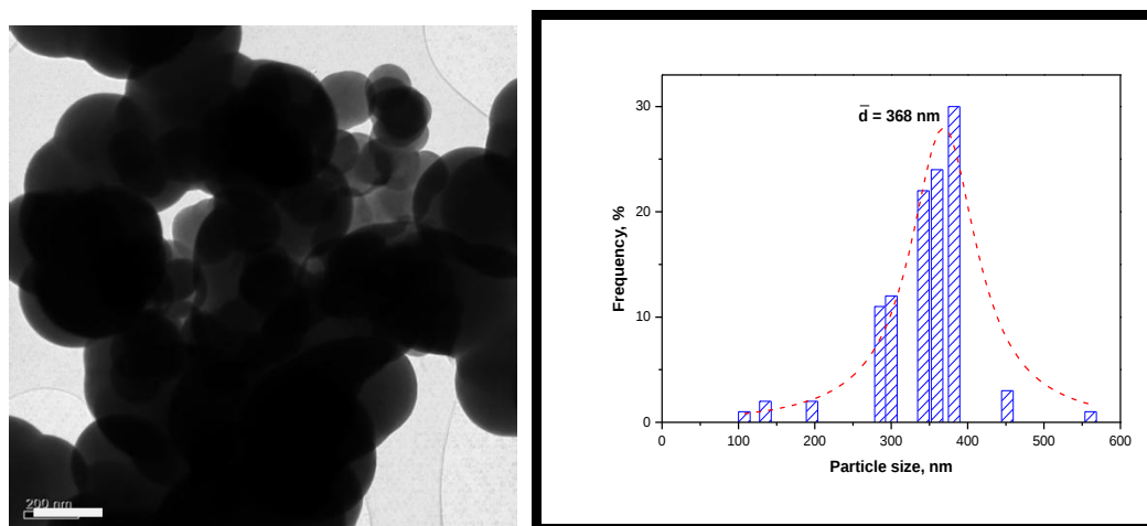
Figure 3.9 TEM image and particle size distribution (solid line = particle size distribution histogram, and dashed line = Gaussian distribution) of CSs sample that was annealed for 6 h in CVD
