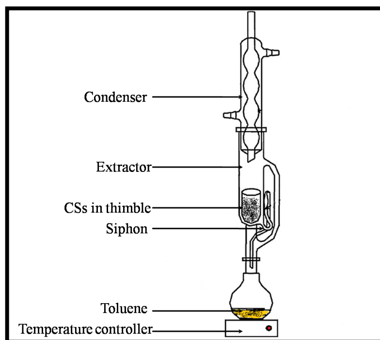
Figure 3.4 Schematic representation of conventional soxhlet extraction set-up for the purification of CSs
