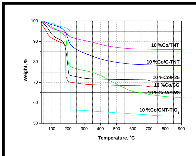
Figure 5.6 TGA profiles for the 10%Co/P25, 10%Co/SG, 10%Co/ASW3, 10%Co/CNT-TiO 2 , 10%Co/TNT and 10%Co/C-TNT catalysts in air atmosphere before calcination
