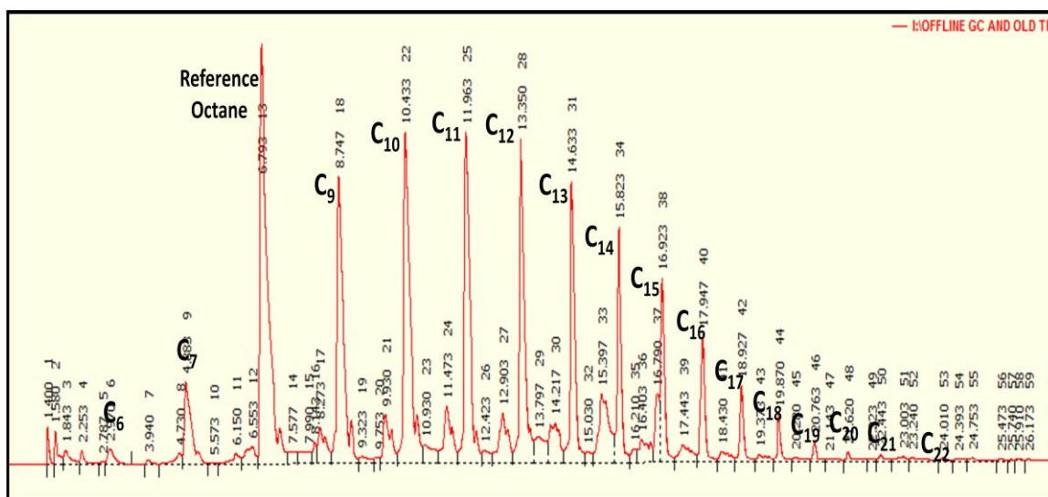
Figure 2.14 A typical FT spectrum (spiked with octane 1L) for gaseous products obtained from an FID-GC (only major peaks are labeled here).
