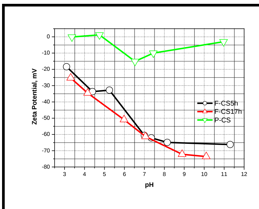
Figure 3.18 Zeta potential of P-CS, F-CS5h and F-CS17h suspensions as a function of pH
