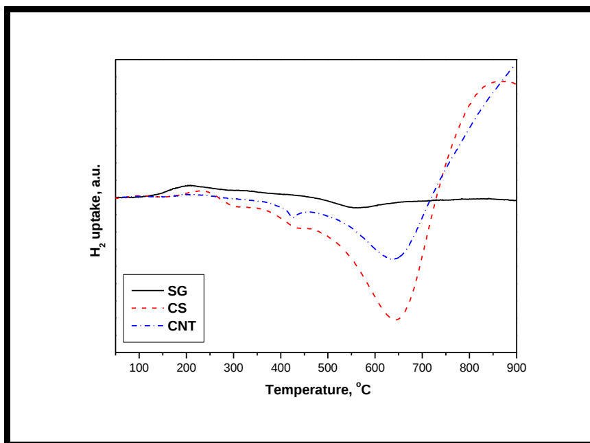
Figure 5.8 H 2 -TPR of SG, CS and CNT
