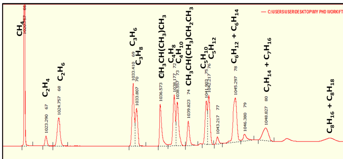
Figure 2.13 A typical FT spectrum for gaseous products obtained from an FID-GC.
