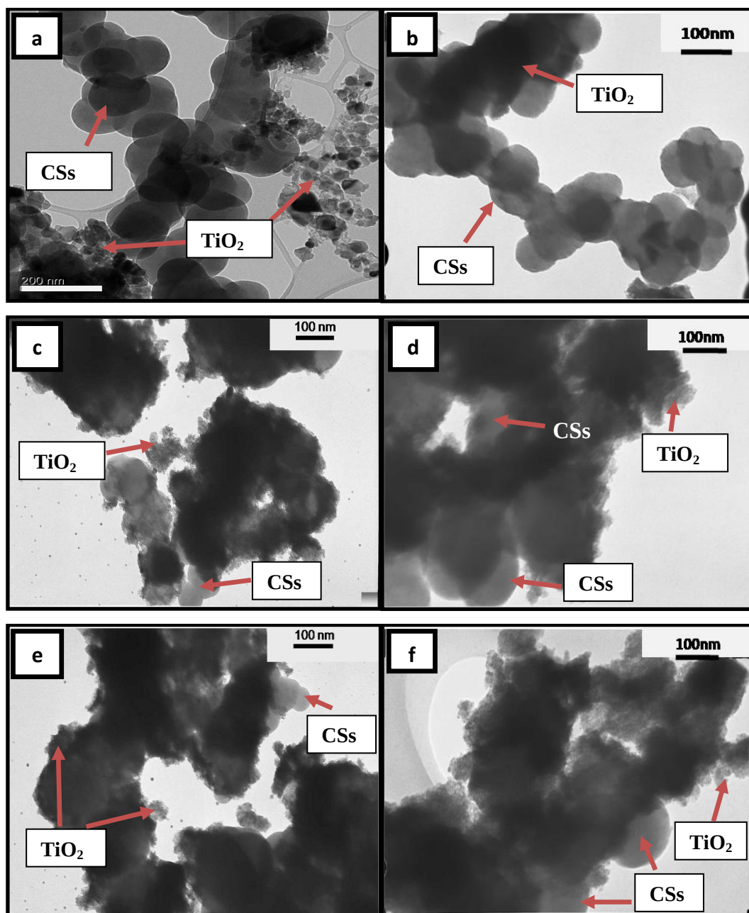
Figure 4.5 TEM images of CS- \text{TiO}_2 composites prepared by a conventional sol-gel method: (a) 1CS-1SG, (b) 1CS-2.5SG, (c) 1CS-5SG, (d) 1CS-10SG, (e) 1CS-25SG and (f) 1CS-50SG
