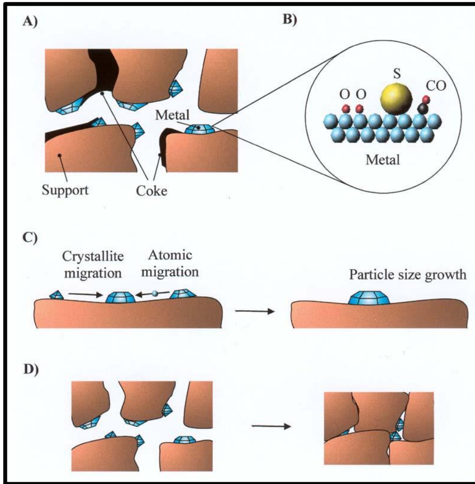
Figure 1.6 Deactivation mechanisms: (A) coke formation, (B) poisoning, (C) sintering of active metal particles and (D) sintering and solid-solid phase transitions and encapsulation of active metal particles [56]
