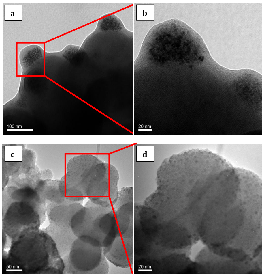
Figure 5.2 (a) and (b) TEM images of 10%Co/F-CS1h indicating cobalt crystallites forming aggregated clusters (cluster size ~ 81 nm based on 50 clusters); (c) and (d) 10%Co/F-CS17h indicating well dispersed cobalt particles on the surface (cobalt particle size ~ 4 nm based on 80 particles)
