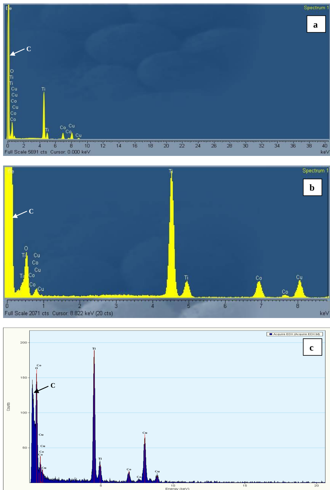
Figure 5.4 (a), (b) and (c) EDX spectra corresponding to the surface coverage shown in Fig. 5.3 (a), (c) and (e), respectively. C and Ti were detected; the Cu signal corresponds to the Cu grid substrate used in the TEM analysis.
