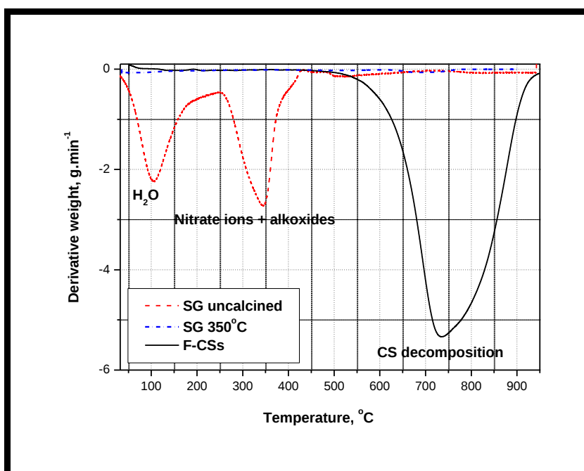
Figure 4.8 DTG of F-CS, uncalcined 0CS-SG and the calcined 0CS-SG
