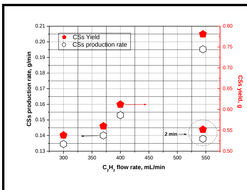
Figure 3.6 Rate of CS growth as a function of C_2H_2 flow rate
