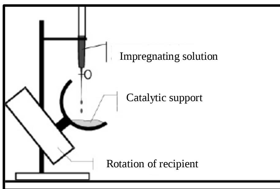
Figure 1.7 Schematic representation of experimental set up for incipient wetness impregnation. Adapted from [53]
