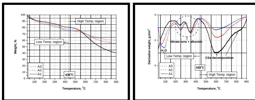
Figure 4.32 TGA (left) and DTG (right) of uncalcined A1, A2 and A3
