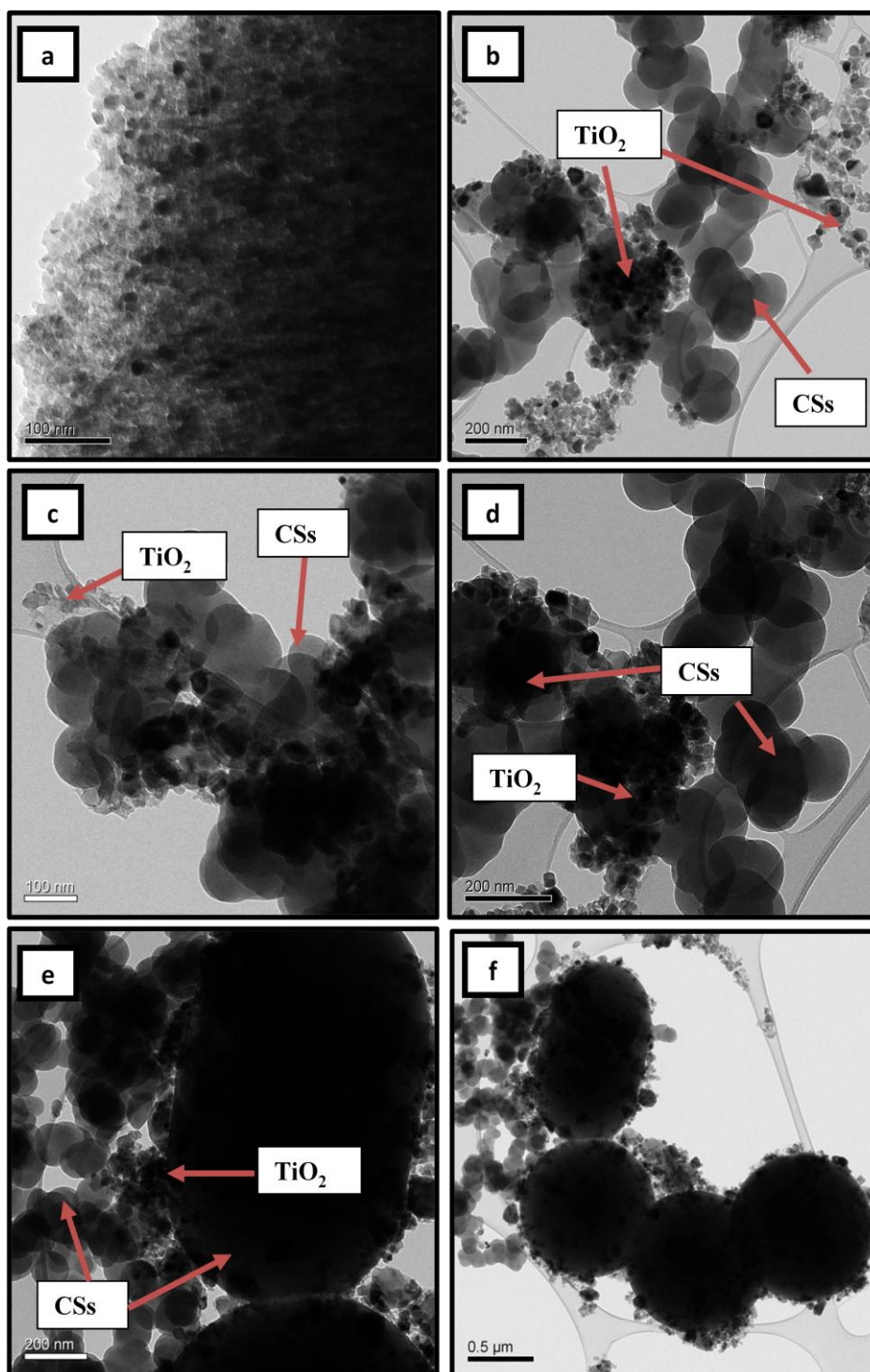
Figure 4.36 TEM images of carbon coated titania materials (C-TiO 2 ) prepared by CVD: (a) C0-TiO 2 , (b) C5-TiO 2 , (c) C30-TiO 2 , (d) C60-TiO 2 , (e) C120-TiO 2 and (f) C240-TiO 2
