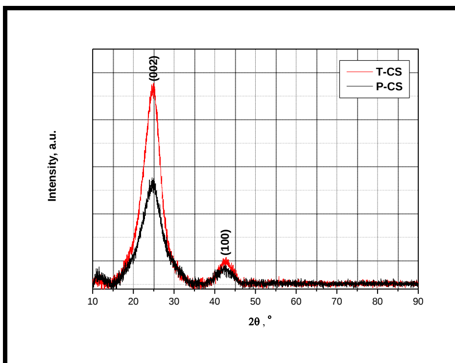
Figure 3.11 XRD patterns of P-CS and T-CS
