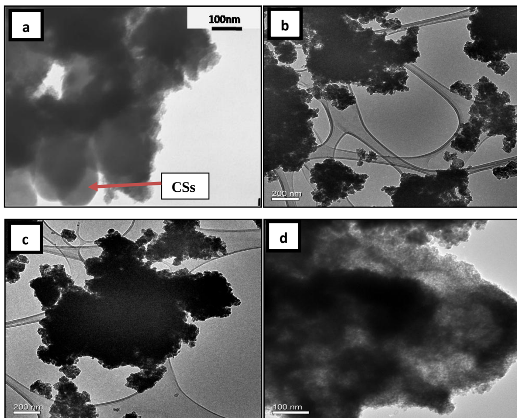
Figure 4.15 TEM images of 1CS-10SG samples after calcination at: (a) 1 bar 350 °C for 6 h; (b) 1 bar 350 °C for 13 h; (c) 5 bar 350 °C for 6 h; and (d) 5 bar 400 °C for 6 h
