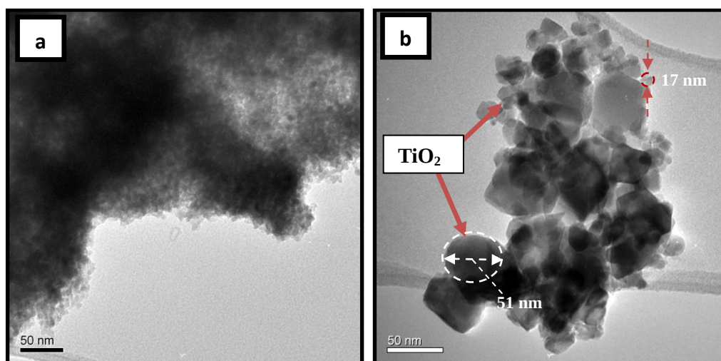
Figure 4.28 TEM images of \text{TiO}_2 residue from combusted ASW3 composite. Samples were combusted in air at 5 bar for 6h at: (a) 300 °C and, (b) 400 °C
