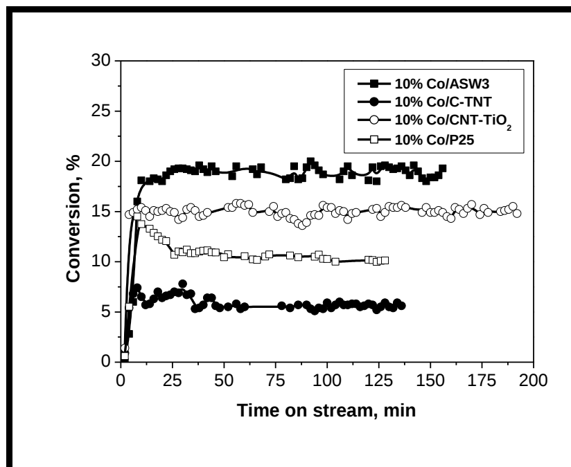
Figure 5.14 CO conversion with time on stream for 10%Co/ASW3, 10%Co/CNT-TiO 2 , 10%Co/P25 and 10%Co/C-TNT
