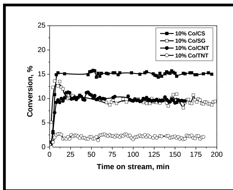
Figure 5.13 CO conversion with time on stream for 10%Co/CS, 10%Co/SG, 10%Co/CNT and 10%Co/TNT
