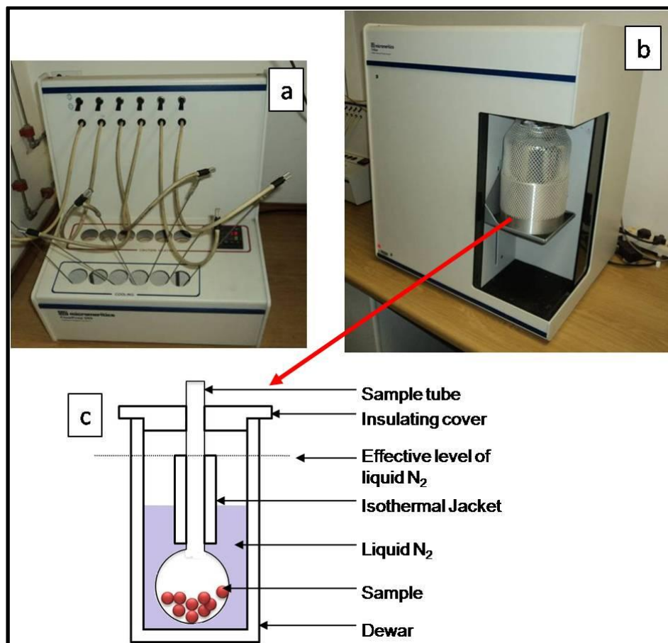
Figure 2.4 (a) Micromeritics Flow Prep 060, (b) Micromeritics Tristar 3000 and (c) liquid N_2 coolant Dewar depicting the Isothermal Jacket TM method of maintaining the cold/warm volume ratio in the sample tube
