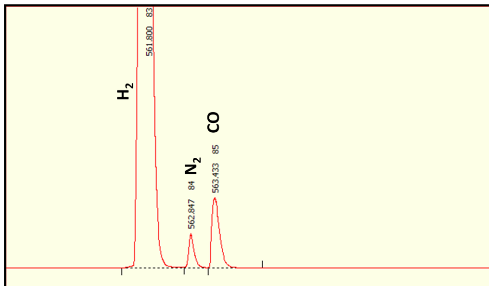
Figure 2.11 A typical spectrum for the synthesis gas (bypass) using TCD-GC
