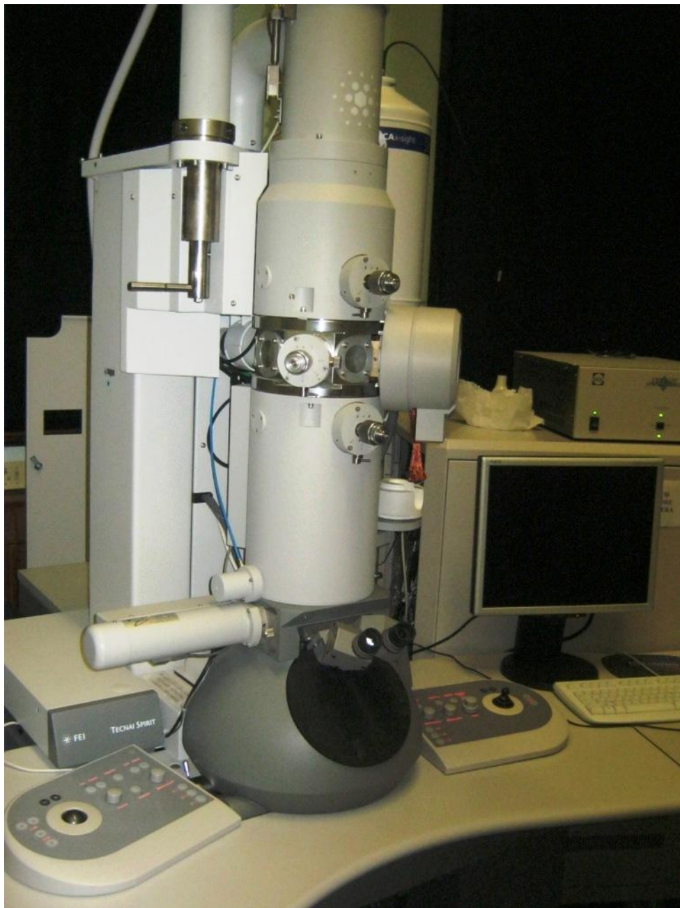
Figure 2.2 TEM FEI Technai Spirit G 2
