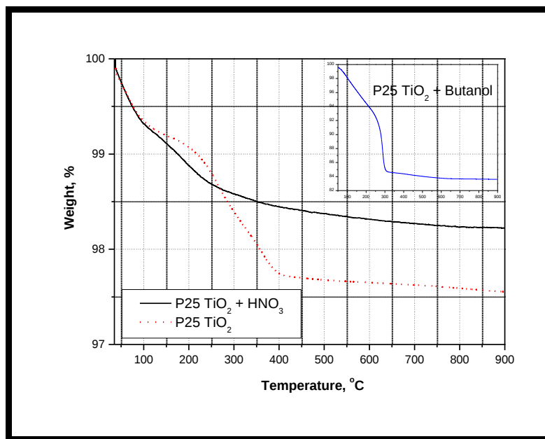
Figure 4. 9 TGA of P25 TiO 2 , P25 TiO 2 mixed with HNO 3 , and P25 TiO 2 mixed with butanol ( inset )
