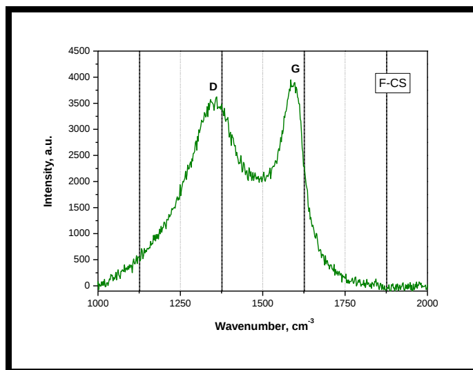
Figure 4.19 Raman spectra of calcined F-CS produced, showing D and G-Bands
