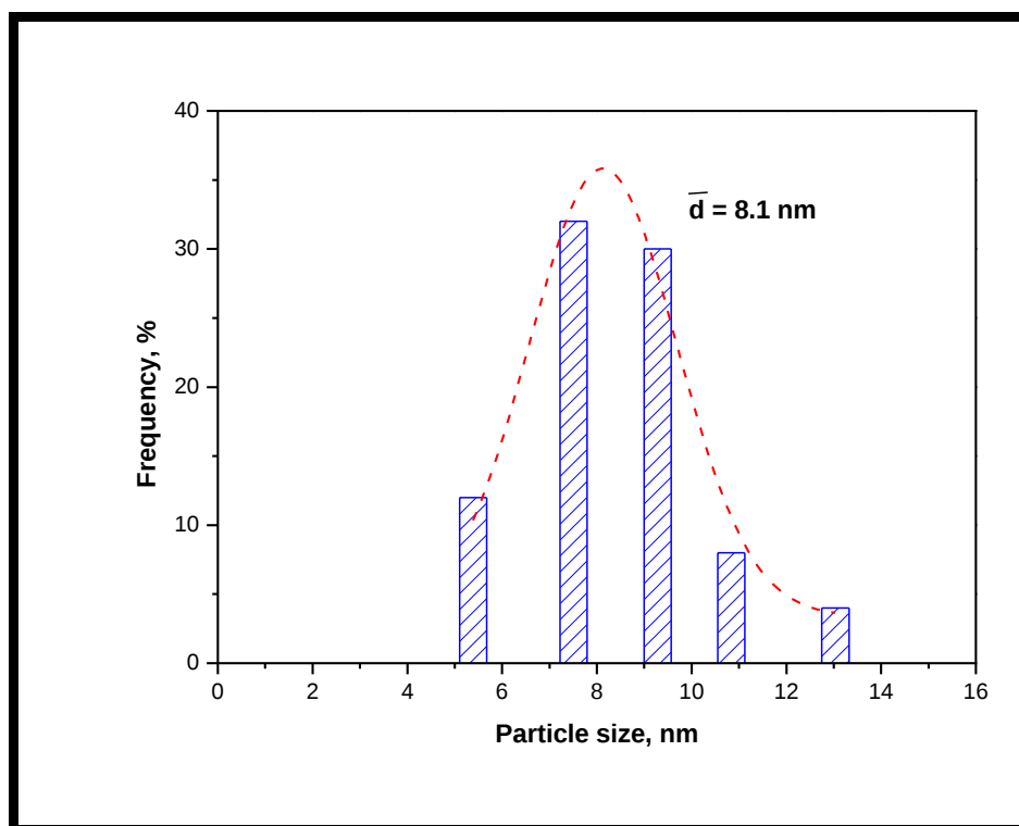
Figure 4.26 Particle size distribution of \text{TiO}_2 in ASW3 (solid line = particle size distribution histogram, and dashed line = Gaussian distribution) prepared by a surfactant wrapping sol-gel method
