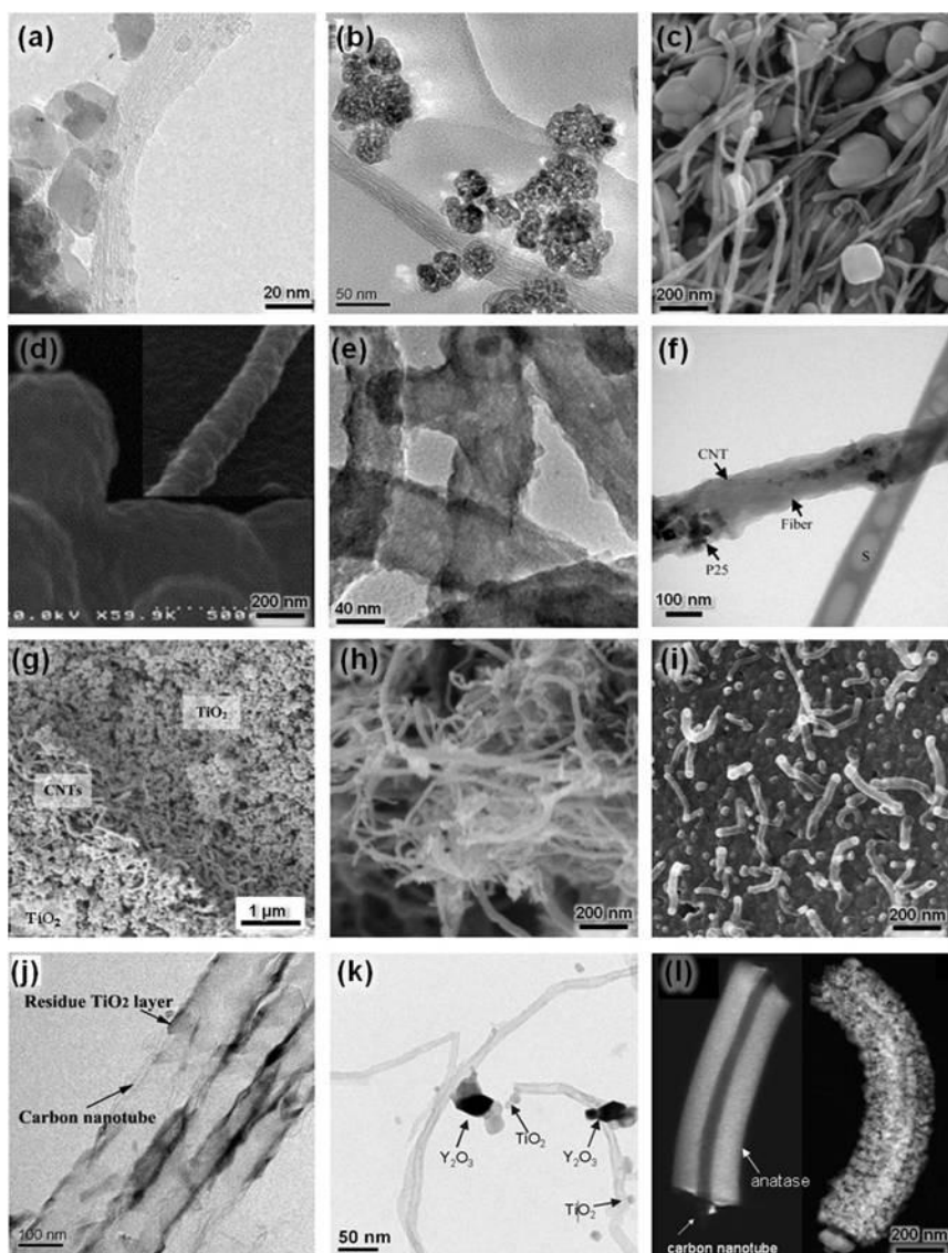
Figure 1.8 CNT- \text{TiO}_2 composites. (a) \text{TiO}_2 nanoparticles on SWCNTs [102], (b) \text{TiO}_2 nanoparticles on MWCNTs [103], (c) SWCNTs on \text{TiO}_2 nanoparticles [104], (d) \text{TiO}_2 coated SWCNTs [105], (e) \text{TiO}_2 coated MWCNTs [106], (f) CNT and \text{TiO}_2 embedded in polymer nanofibres [107], (g) laminate composite films [108], (h) intermixed CNTs and \text{TiO}_2 nanotubes [109], (i) MWCNTs grown or deposited on bulk \text{TiO}_2 [110], (j) CNTs grown in \text{TiO}_2 nanotube arrays [111], (k) yttrium treated CNT- \text{TiO}_2 [112] and (l) \text{TiO}_2 nanotube arrays produced via sacrificial CNT templates [113]. Adapted from [114]
