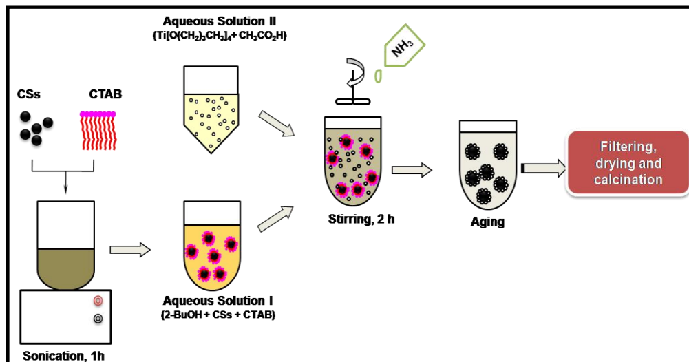
Figure 4.3 A schematic representation of the CS-TiO 2 composite prepared via the surfactant wrapping sol-gel method.
