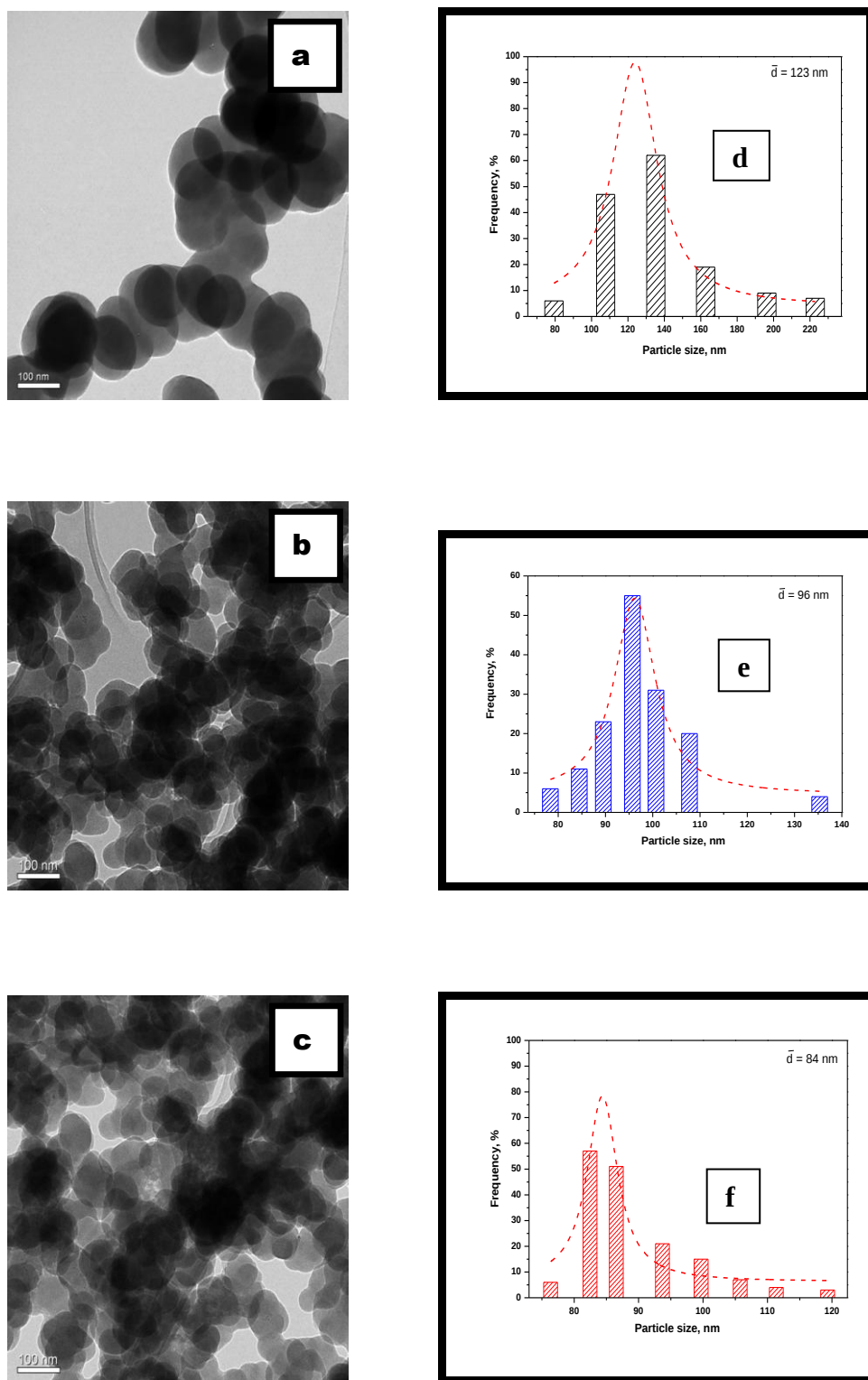
Figure 3.5 TEM images of P-CS prepared at different C_2H_2 flow rates with their corresponding particle size distributions (solid line = particle size distribution histogram, and dashed line = Gaussian distribution): (a) and (d) 300 mL/min; (b) and (e) 400 mL/min; and (c) and (f) 545 mL/min
