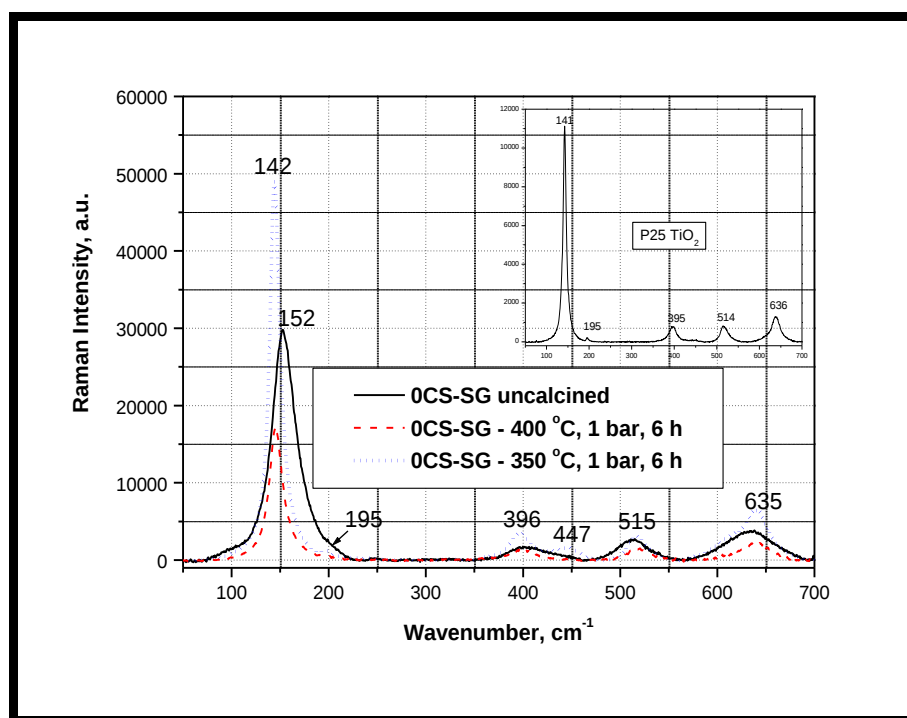
Figure 4.18 Raman spectra of uncalcined OCS-SG sample; and of calcined OCS-SG samples at: 1 bar 350 °C for 6 h, and 1 bar 400 °C for 6 h. Raman spectra of bulk commercial TiO 2 material (P25 TiO 2 ) is shown on the inset .
