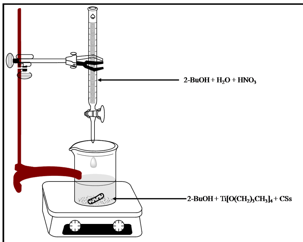
Figure 4.2 A schematic representation of the set up used for the preparation of CS- \text{TiO}_2 composites by the conventional sol-gel method. Adapted from [46]
