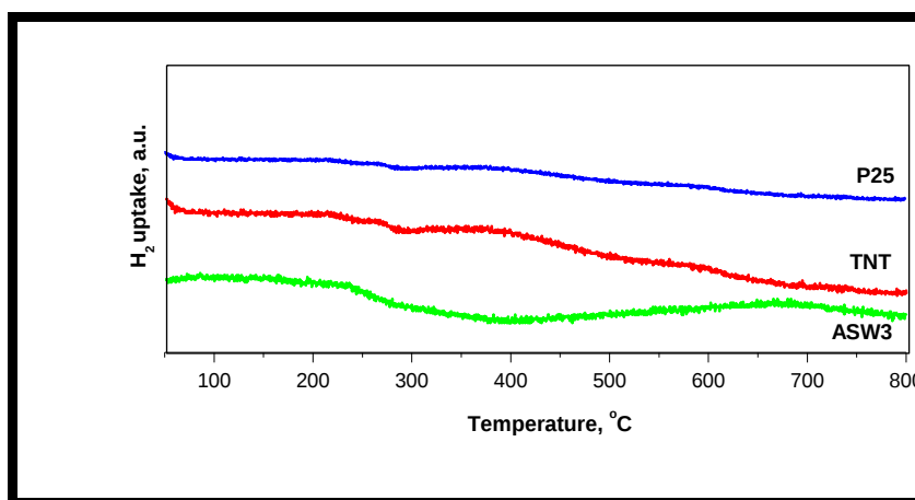
Figure 5.9 H 2 -TPR of P25, TNT and ASW3
