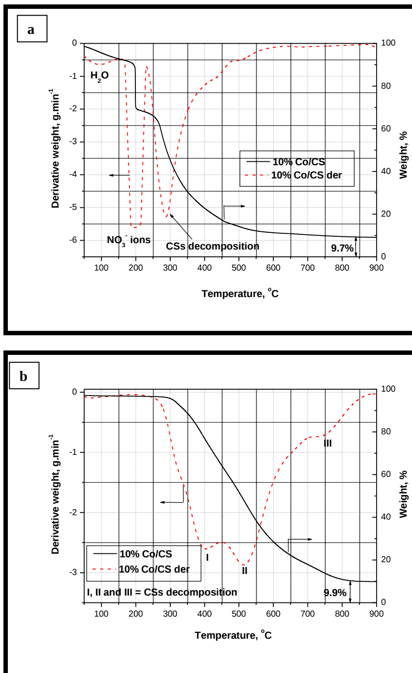
Figure 5.5 TGA and DTA profiles for the 10%Co/CS catalyst in air atmosphere; (a) before calcination and (b) after heating in N 2 (220 °C, 150 min)
