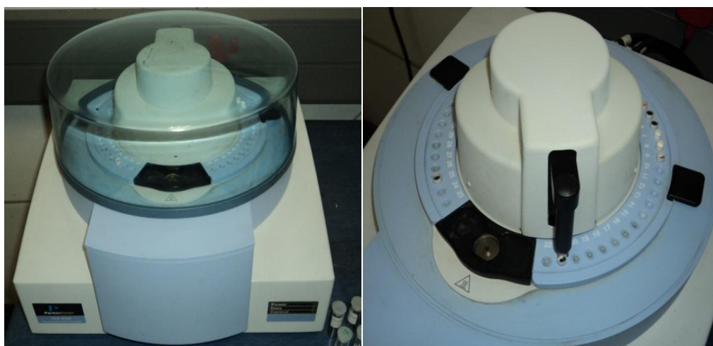
Figure 2.3 Perkin Elmer STA 4000 thermogravimetric analyzer coupled to an auto sampler: (left) manual-single sample analysis and (right) an autosampler-multiple samples analysis (with an autosampler arm in operation)
