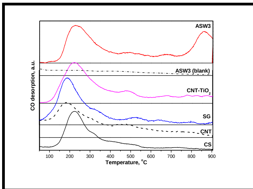
Figure 5.11 CO-TPD of calcined supports; i.e. ASW3, CNT-TiO 2 , CNT, SG and CS
