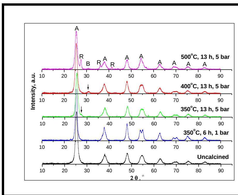
Figure 4.17 XRD patterns of calcined sol-gel derived composite materials, where A = anatase phase, B = brookite and R = rutile phase.
