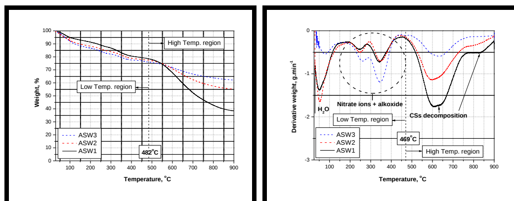
Figure 4.34 TGA (left) and DTG (right) of uncalcined ASW1, ASW2 and ASW3
