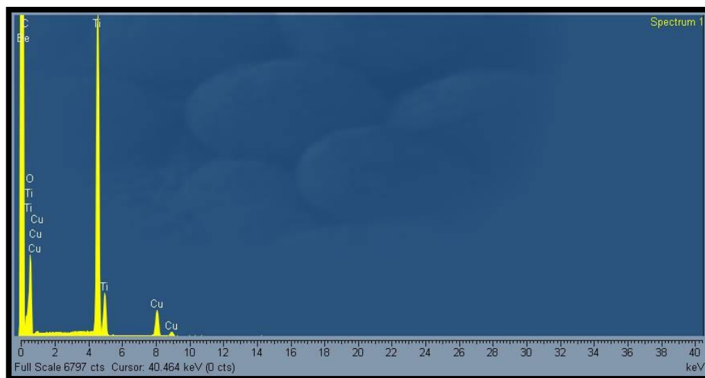
Figure 4.6 EDX spectrum corresponding to the surface coverage shown in Fig. 4.5(c). C and Ti were detected; the Cu signal corresponds to the Cu grid substrate for TEM analysis.
