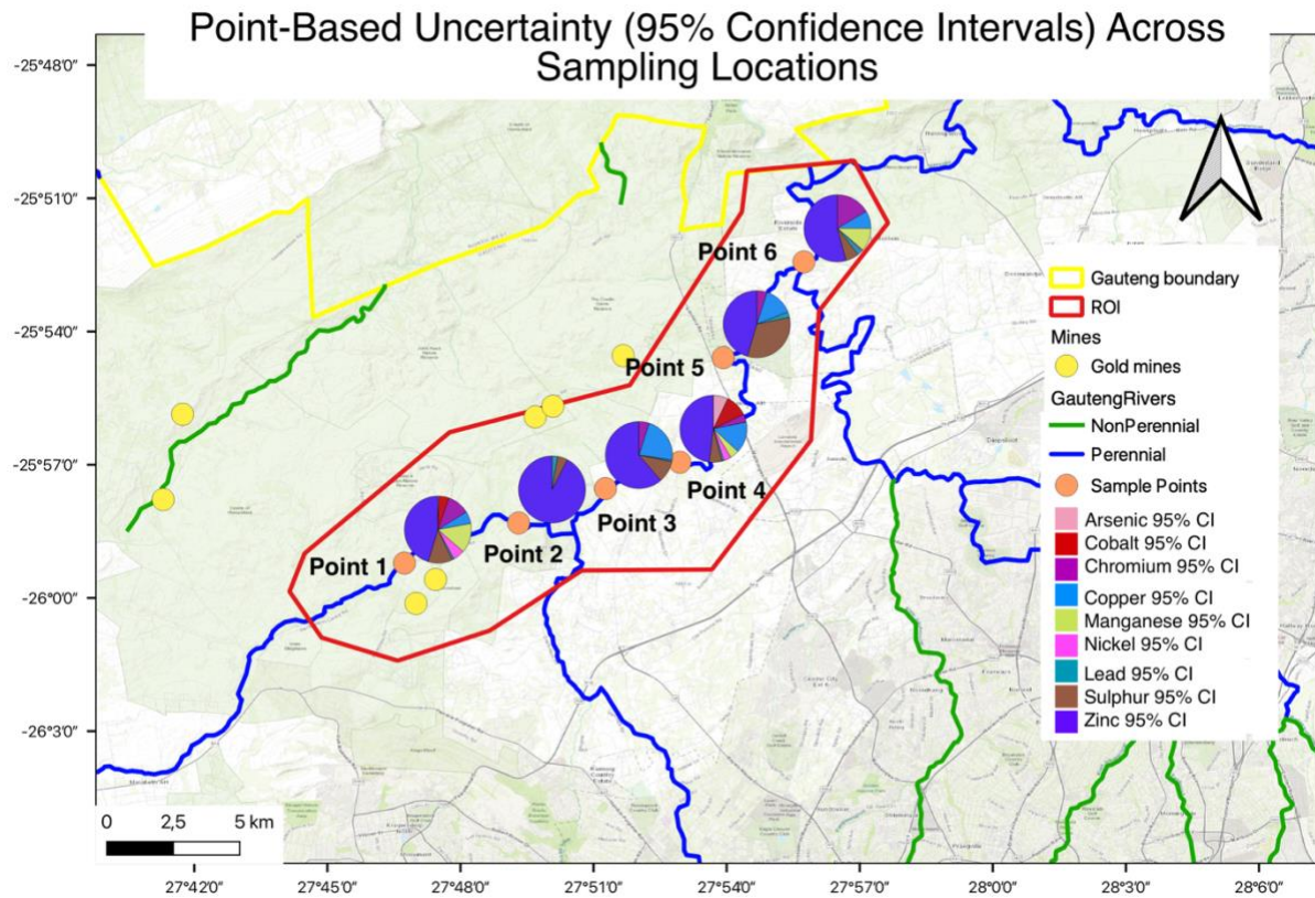
Figure 8: Point based uncertainty map across all sample sites
