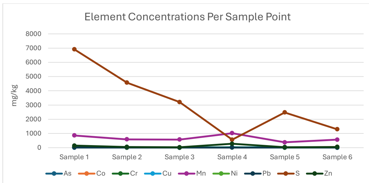
Figure 7: Mean element concentrations over each sample site
