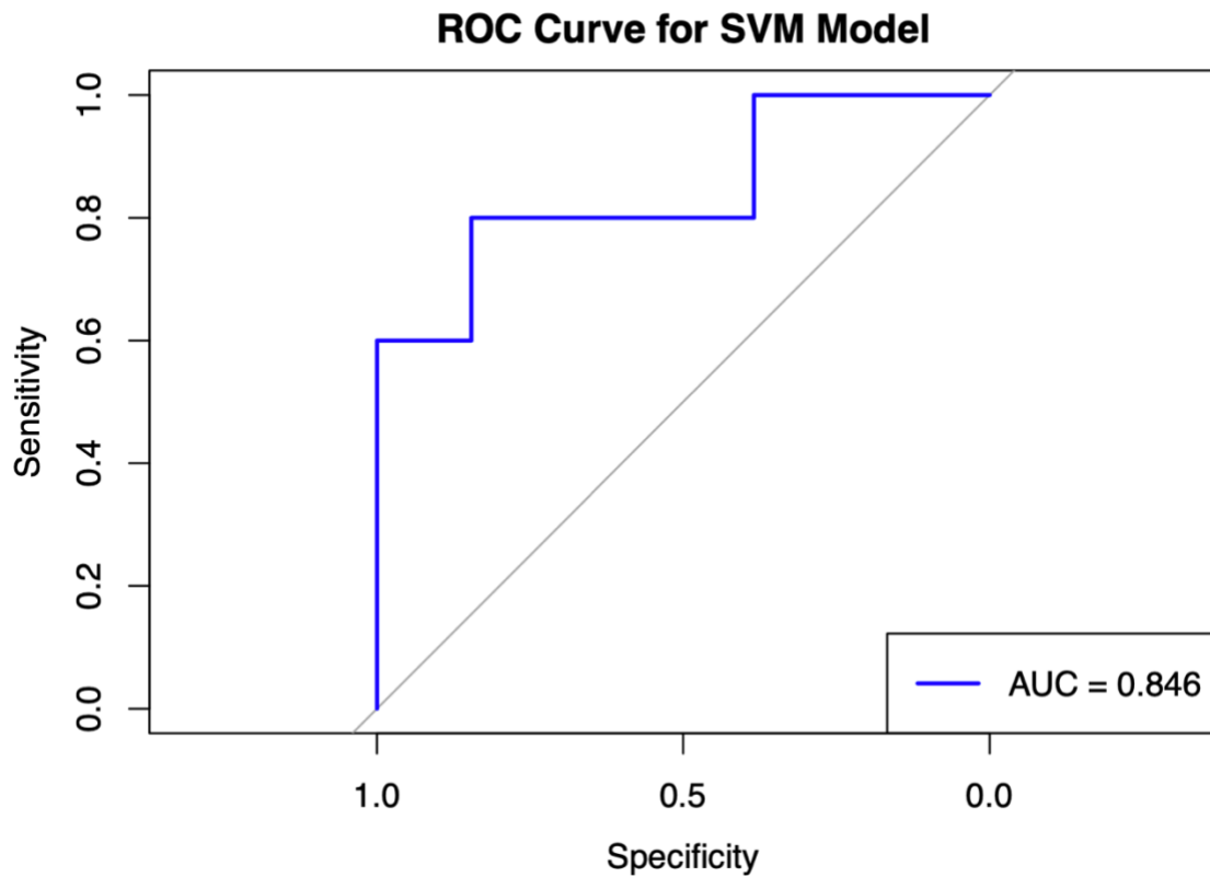
Figure 11: ROC curve and AUC value for predictive accuracy of SVM model
