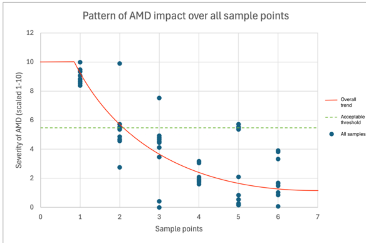
Figure 9: General trend in AMD impact over all sample sites
