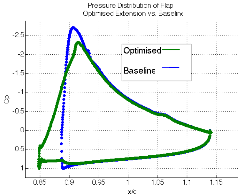
Figure 5.23: Pressure distribution of TC12 high lift configuration optimised solution with smoothed geometry vs. baseline at 8.09 degrees in Fluent, SA turbulence model, Re 2.95 Million
