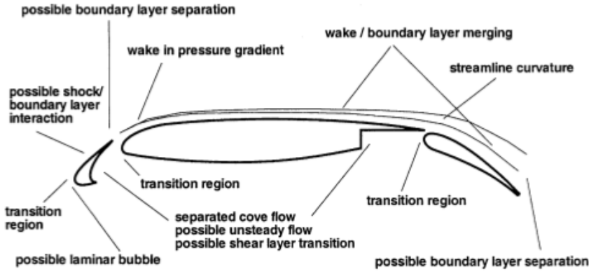
Figure 2.5: Challenges inherent in multi-element flow field prediction ( Rumsey and Ying, 2002 )
