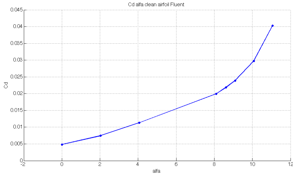
Figure 4.29: C_d vs. \alpha for TC12 in clean configuration compared to experiments, Re = 2.95 Million, transition-SST turbulence model
