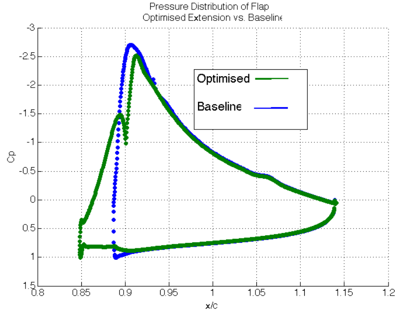
Figure 5.18: Pressure distribution at flap of TC12 high lift configuration optimised solution vs. baseline in Fluent SA turbulence model, 8.09 degrees, Re 2.95 million
