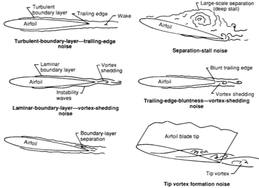
Figure 2.7: Five different types of airfoil self noise
