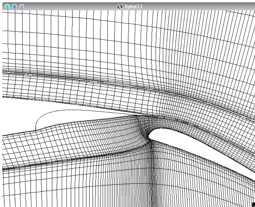
Figure B.4: Grid at spoiler cove for the TC12 profile high lift configuration in MSES
