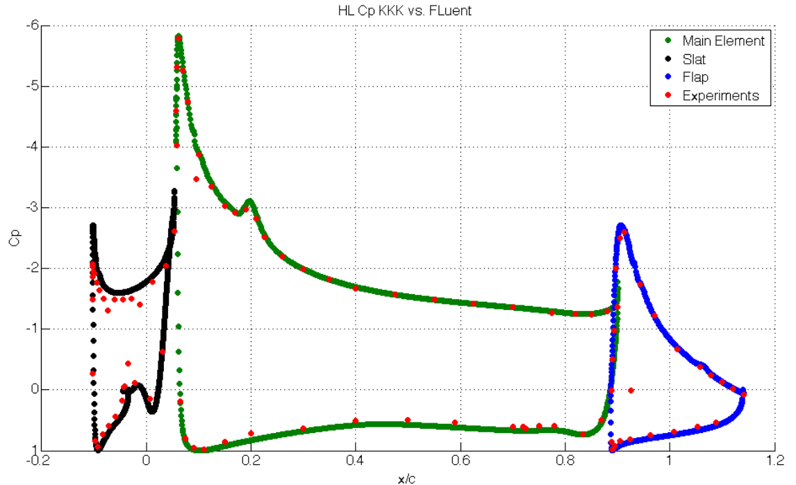
Figure 4.54: Pressure distribution for TC12 profile in high lift configuration, k-omega SST turbulence model, 8.09 degrees, Re 2.95 million
