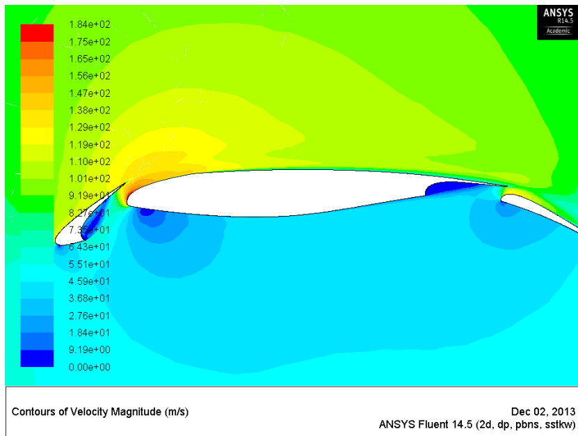
Figure 4.47: Velocity contours for TC12 profile in high lift configuration, k-omega SST turbulence model, 8.09 degrees, Re 2.95 million
