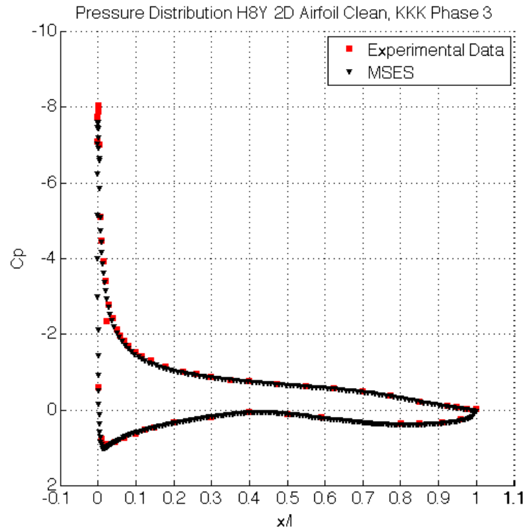
Figure 4.6: Pressure distribution of TC12 profile in clean configuration at Re 9.06 million, angle of attack 8.1 Degrees
