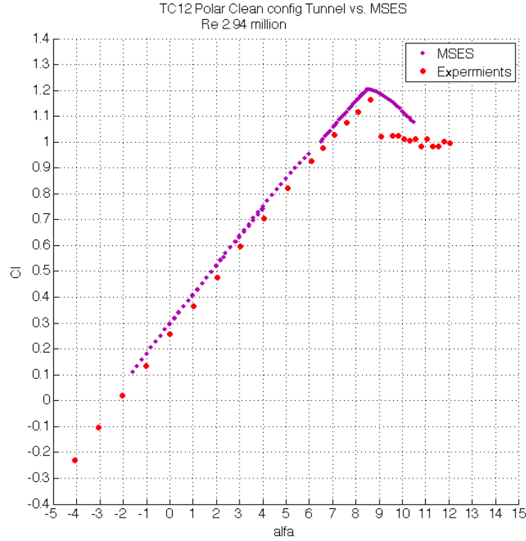
Figure 4.3: C_l vs. \alpha for TC12 profile in clean configuration at Re 2.94 Million, MSES
