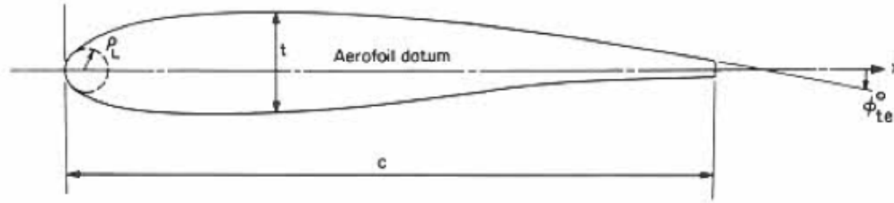
Figure 4.12: ESDU definitions associated with basic airfoil geometry
