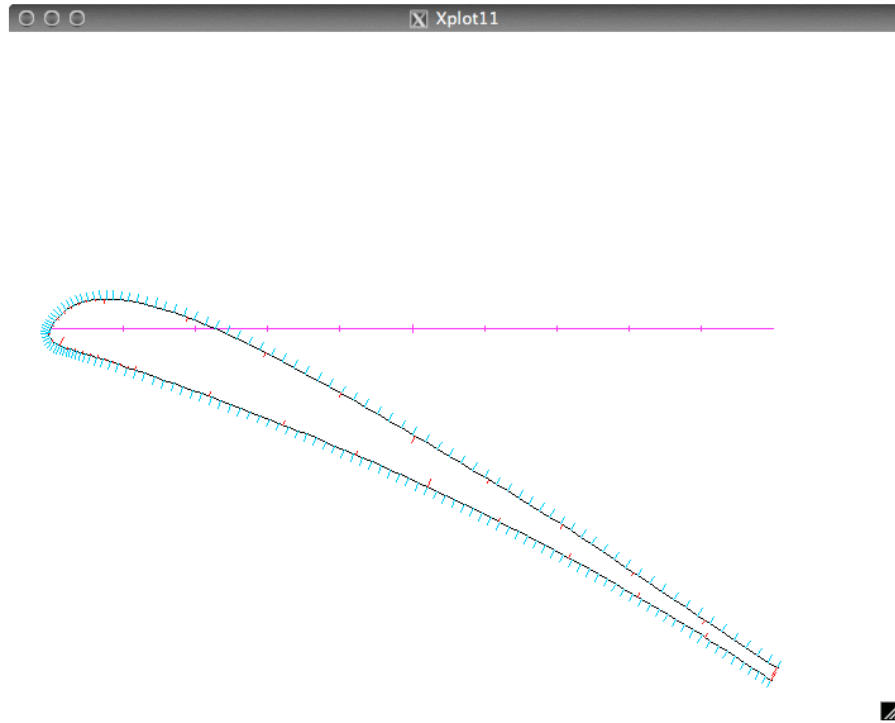
Figure B.8: Flap panelling for the TC12 profile high lift configuration in MSES
