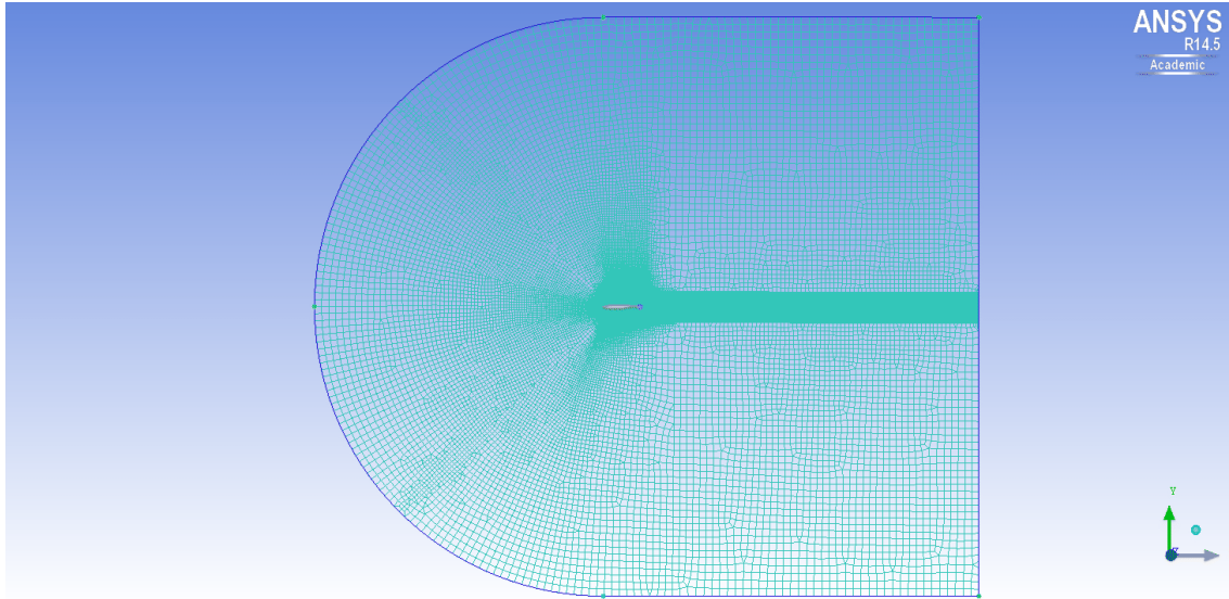
Figure 4.21: TC12 profile clean configuration airfoil mesh (full view)
