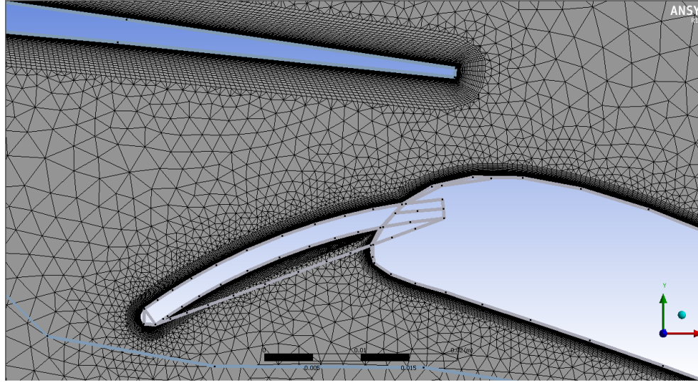
Figure 6.8: Mesh of DesignXplorer MOGA optimised solution
