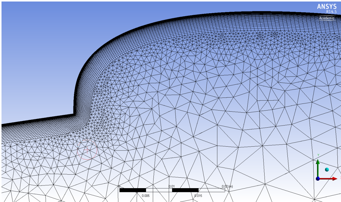
Figure 4.34: Mesh at the cove region of the main element TC12 profile in high lift configuration
