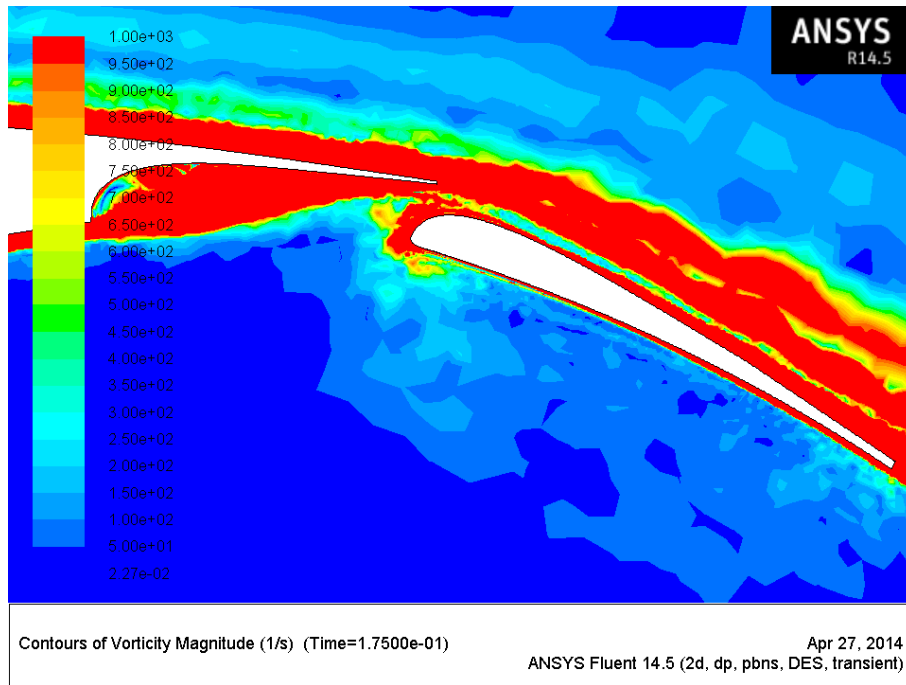
Figure 7.9: Vorticity between 0 - 1 000 near the trailing edge of the TC12 profile in high lift configuration at 8.09 degrees angle of attack using the DES turbulence model
