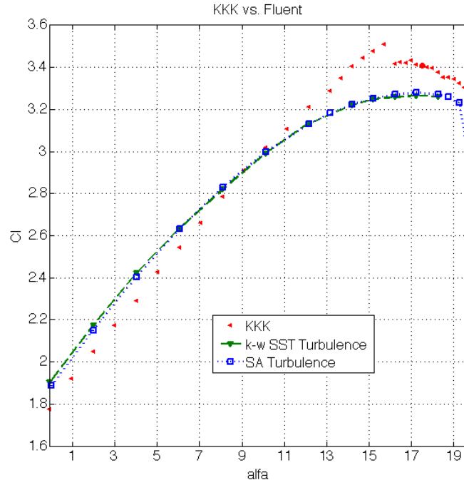
Figure 4.48: C_l vs. \alpha for TC12 profile in high lift configuration, Re 2.95 million vs. KKK windtunnel data
