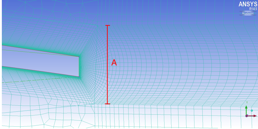
Figure 4.20: Boundary layer mesh at the trailing Edge of TC12 profile clean configuration
