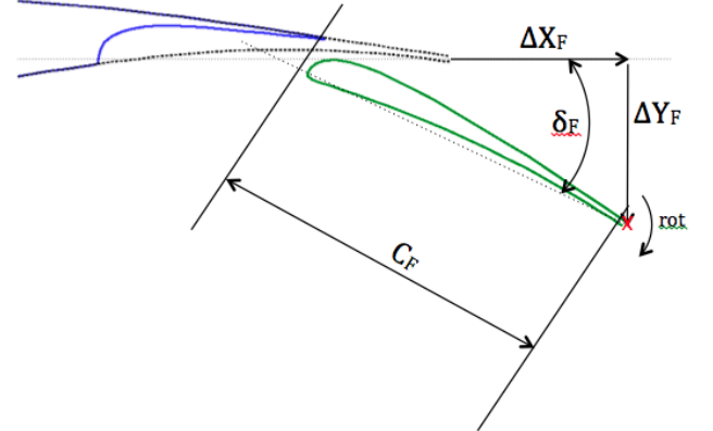
Figure 3.3: Fowler flap motion of TC12 profile in high lift configuration
