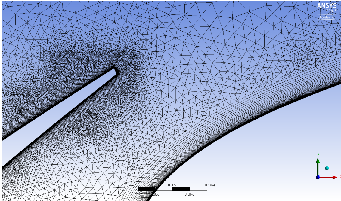
Figure 4.32: Mesh at the region between TC12 profile in high lift configuration, slat trailing edge and main element leading edge
