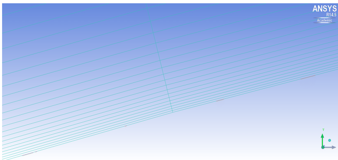
Figure 4.19: Boundary layer mesh close to surface of TC12 profile clean configuration
