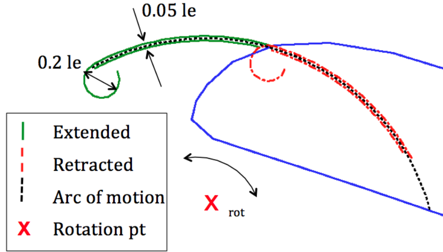
Figure 5.3: Constrained optimisation variables
