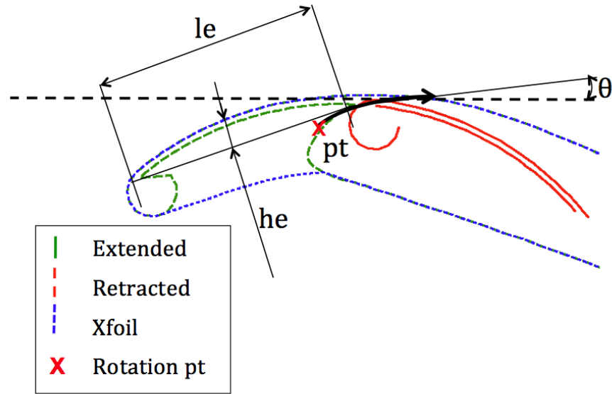
Figure 5.5: Geometry of solution of zero order flap optimisation
