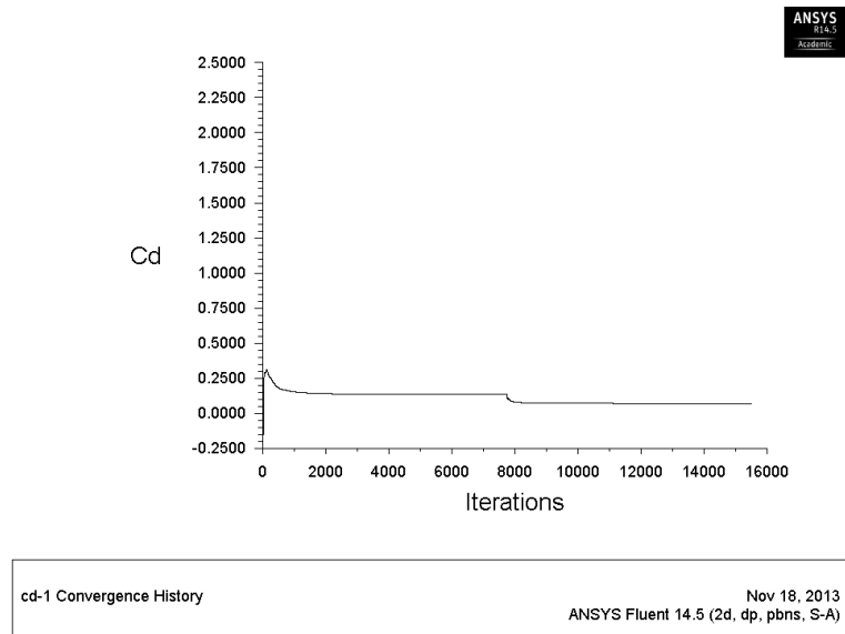
Figure 4.41: Convergence of drag coefficient residuals for TC12 high lift configuration mesh, SA turbulence model
