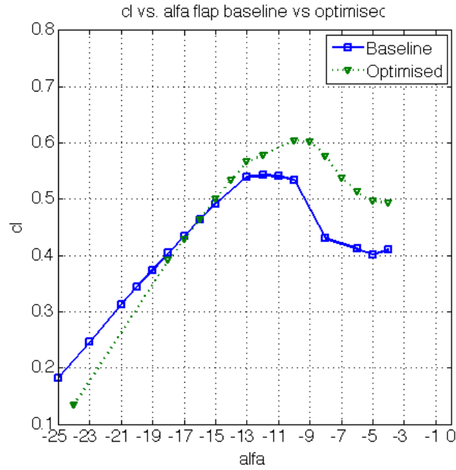
Figure 5.6: C_l vs. \alpha of TC12 flap optimised solution vs baseline in XFOIL
