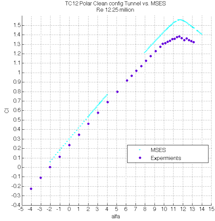
Figure C.4: C_l vs. \alpha for TC12 profile in clean configuration, Re 12.25 million, MSES
