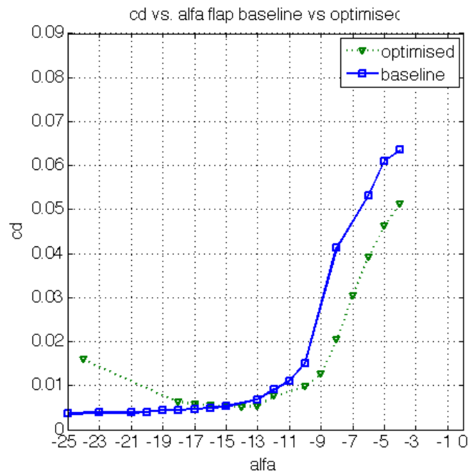
Figure 5.7: C_d vs. \alpha of TC12 flap optimised solution vs baseline in XFOIL
