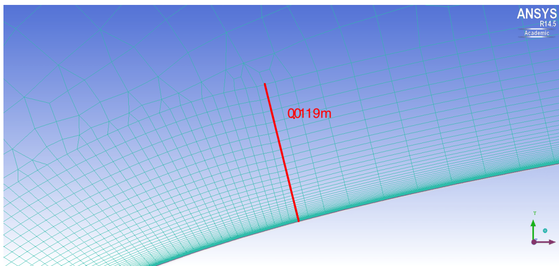
Figure 4.18: Boundary layer mesh of TC12 profile clean configuration
