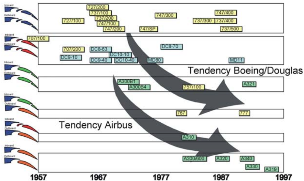
Figure 2.3: Development of trailing edge high lift systems on airliners (Reckzeh, 2003)
