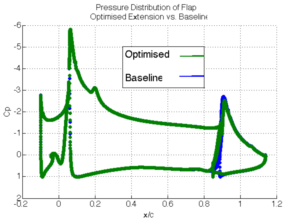
Figure 5.17: Pressure distribution of tc12 high lift configuration optimised solution vs. baseline in Fluent SA turbulence model, 8.09 degrees, Re 2.95 million
