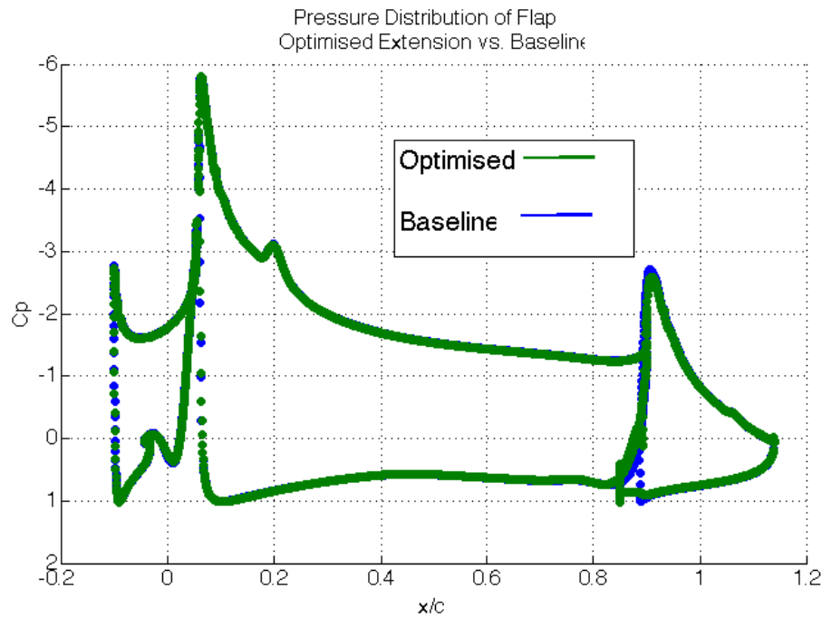
Figure 6.12: Pressure distribution of TC12 high lift configuration at 8.09 degrees DesignXplorer optimised solution vs. baseline in Fluent, Re 2.95 million, SA turbulence model
