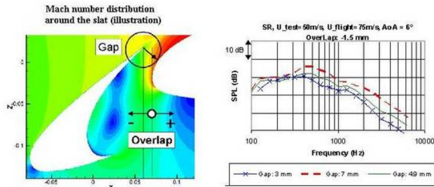
Figure 2 - Slat gap reduction impact on airfoil noise measured on a 2d profile at 50m/s and 6^\circ of angle-of-attack
