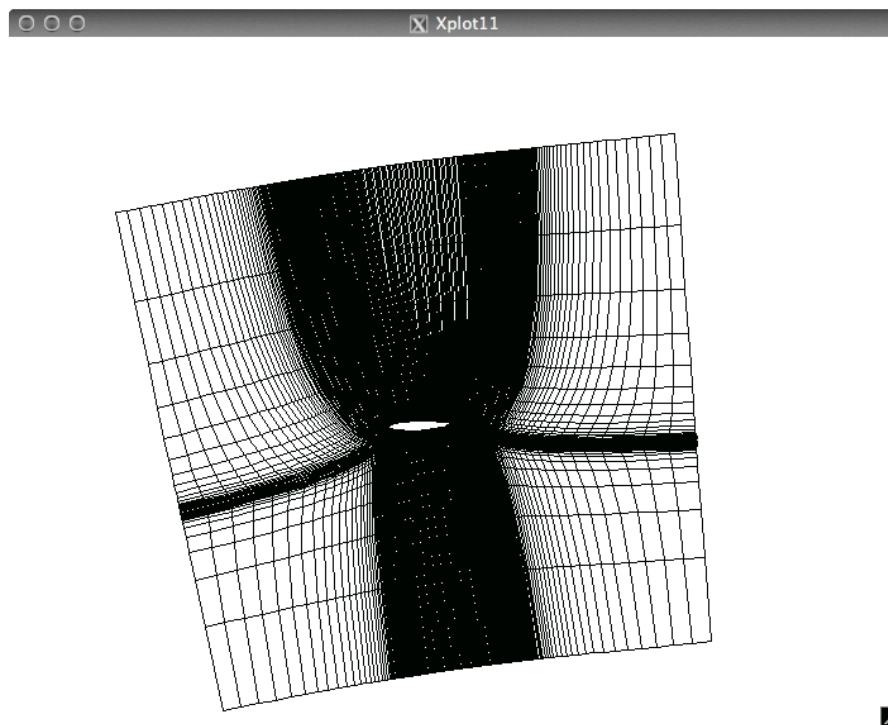
Figure B.1: Full view of grid for the TC12 profile in high lift configuration in MSES
