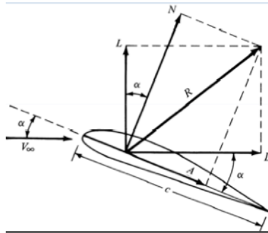
Figure 4.15: Diagram explaining conventions in equations (4.14) and (4.15)
