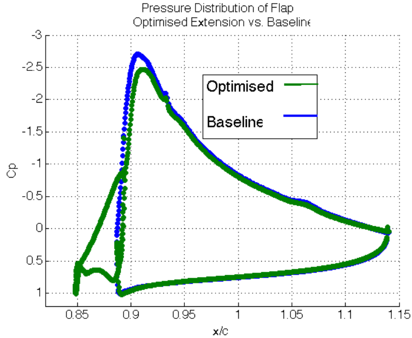
Figure 5.26: Pressure distribution of TC12 high lift configuration optimised solution with slot (flap alone) at 8.09 degrees vs. baseline in Fluent, SA turbulence model, Re 2.95 Million
