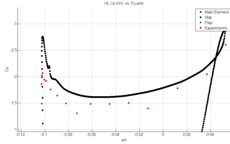
Figure 4.52: Pressure distribution at slat for TC12 profile in high lift configuration, SA turbulence model vs. windtunnel data, 8.09 degrees Re 2.95 million
