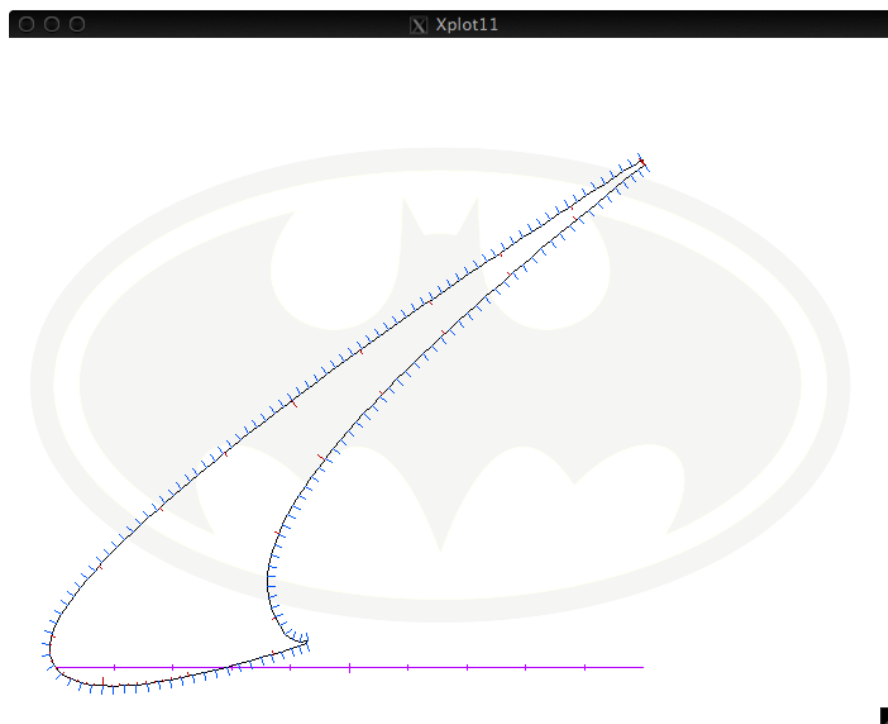
Figure B.6: Slat panelling for the TC12 profile in high lift configuration in MSES
