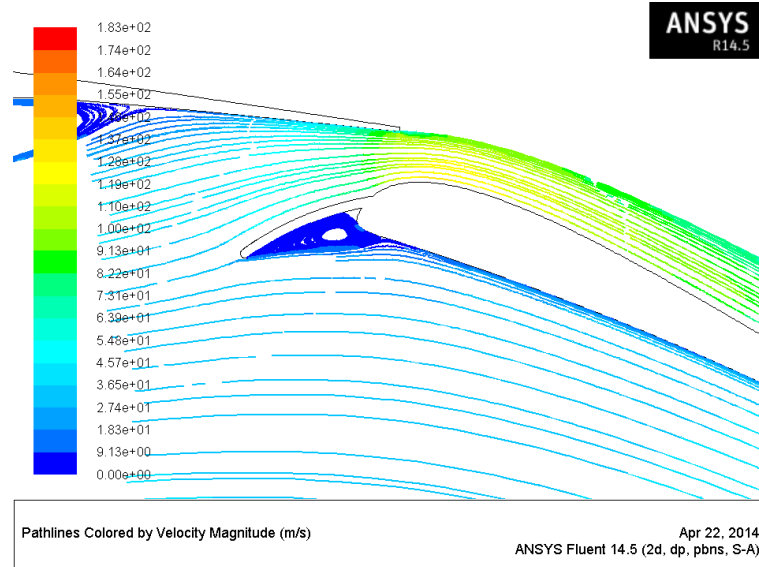
Figure 6.15: Streamlines showing recirculation region of the DesignXplorer optimised concept
