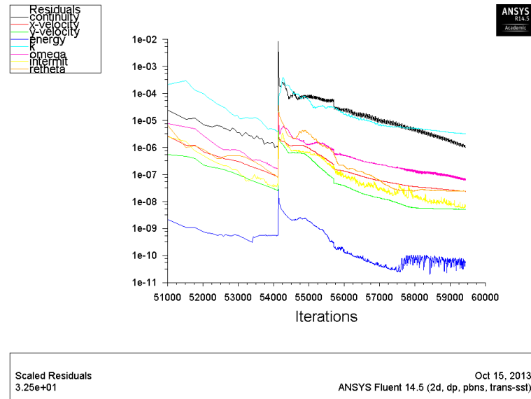
Figure 4.25: Second Order Convergence of Fluent Results for the TC12 Clean Airfoil at 8.1051 degrees
