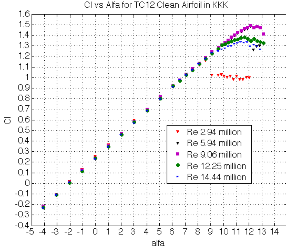
Figure 4.1: Coefficient of lift against angle of attack for TC12 profile in clean configuration, KKK experiments
