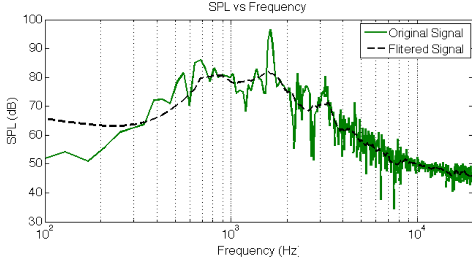
Figure 7.11: Sound spectrum for the TC12 profile in high lift configuration at 8.09 degrees angle of attack using the DES turbulence model
