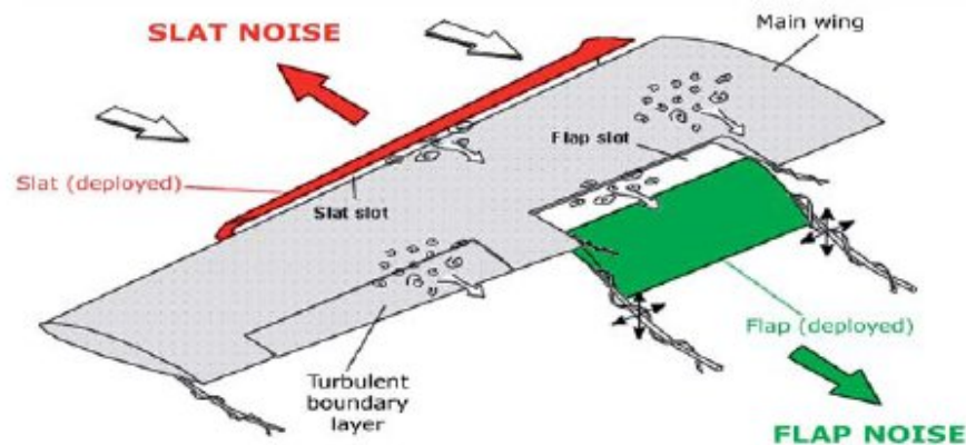
Figure 2.10: Noise sources examined during the VALIANT project
