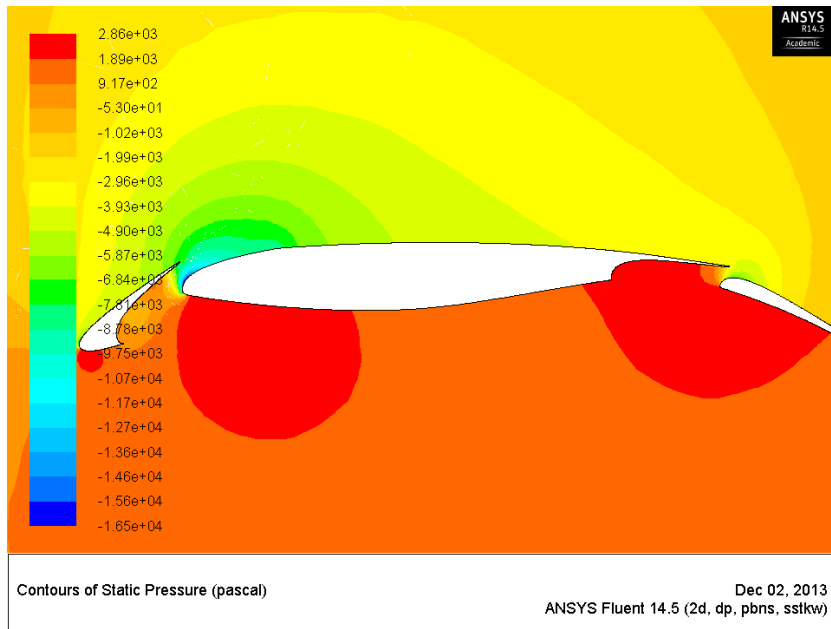
Figure 4.46: Pressure distribution for TC12 profile in high lift configuration, k-omega SST turbulence model, 8.09 degrees, Re 2.95 million
