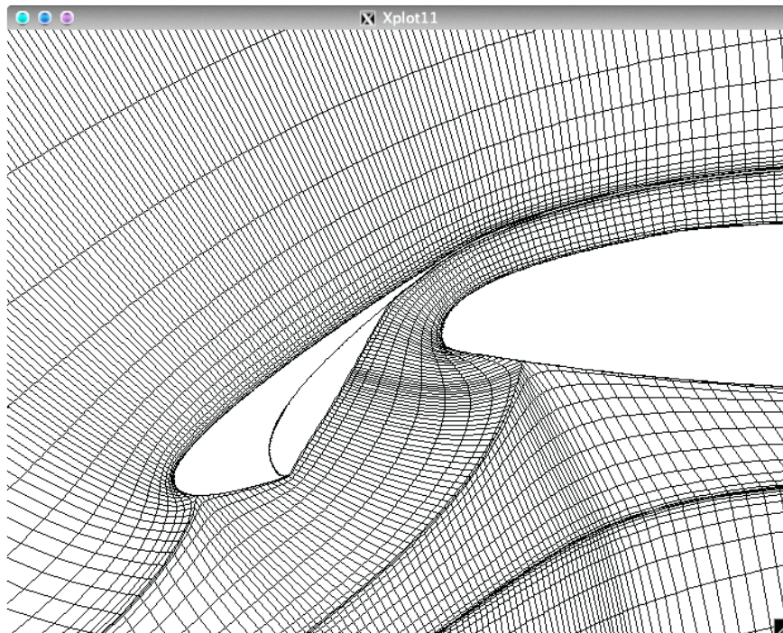
Figure B.3: Grid at slat cove for the TC12 profile high lift configuration in MSES
