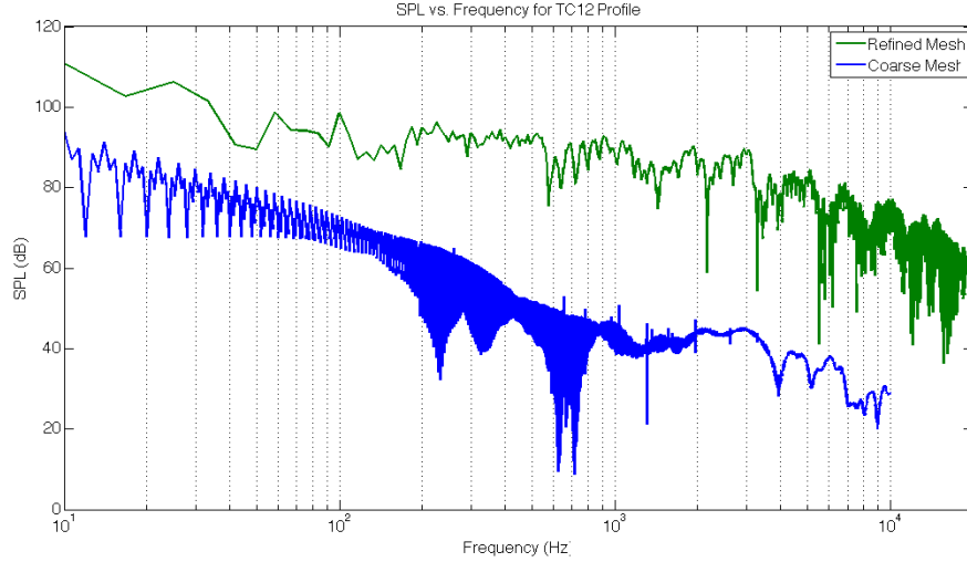
Figure 7.6: Sound spectrum for the TC12 profile in high lift configuration at 8.09 degrees angle of attack using the SA turbulence model
