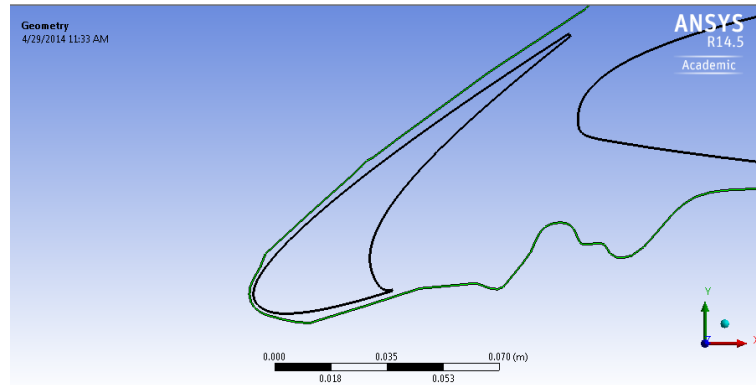
Figure 7.2: Integration region around TC12 profile in high lift configuration for acoustic calculations at slat
