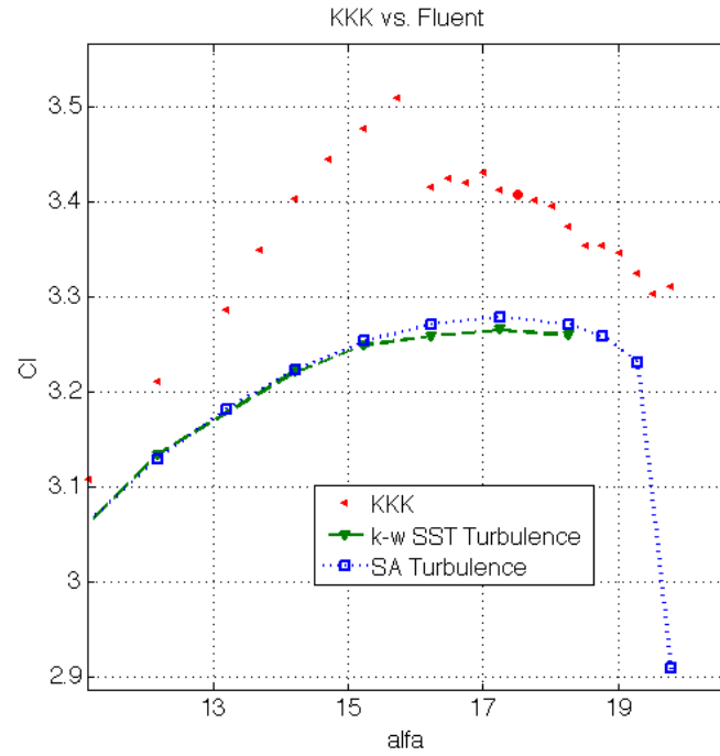
Figure 4.49: C_l vs. \alpha showing stall for TC12 profile in high lift configuration, Re 2.95 million vs. KKK windtunnel data
