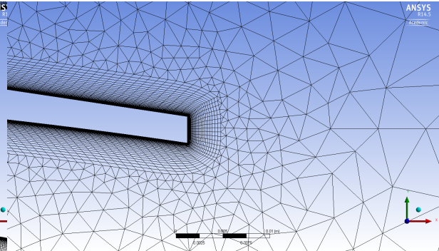
Figure D.4: Mesh for TC12 profile clean configuration trailing edge, ANSYS mesher
