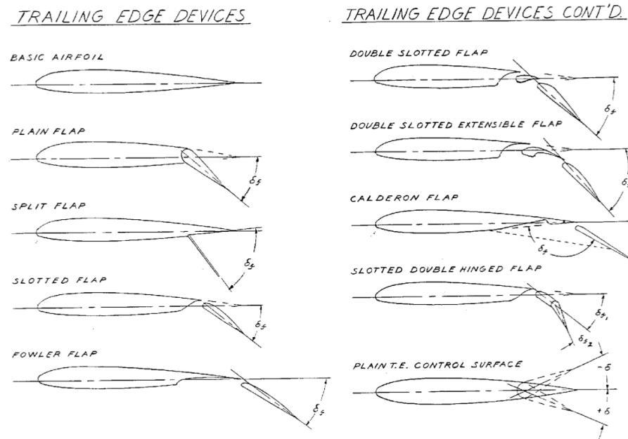
Figure 2.1: Drawings of various trailing edge high lift devices
