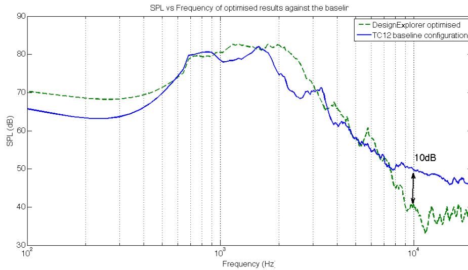
Figure 7.16: Filtered sound spectrum for the optimised TC12 profile in high lift configuration against the baseline at 8.09 degrees angle of attack using the DES turbulence model
