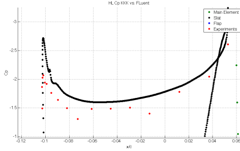
Figure 4.55: Pressure Distribution at slat for TC12 profile in high lift configuration, k-omega SST turbulence model vs. windtunnel data, 8.09 degrees, Re 2.95 million
