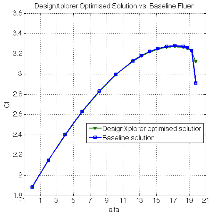
Figure 6.9: C_l vs. \alpha of TC12 profil in high lift configuration DesignXplorer optimised solution vs. baseline in fluent sa turbulence model, Re 2.95 million
