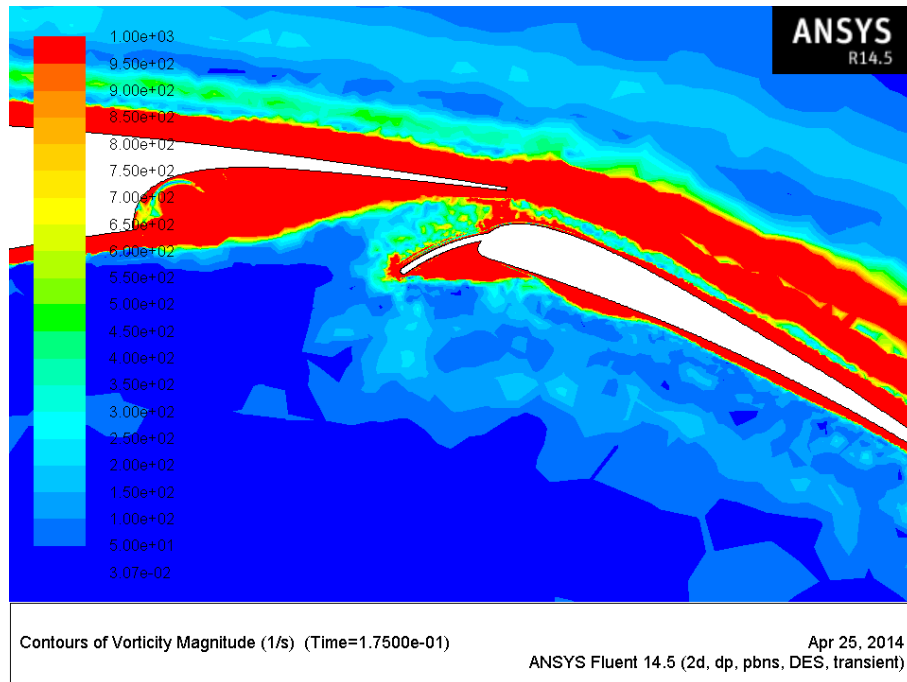
Figure 7.12: Vorticity between 0 - 1 000 near the trailing edge of the DesignXplorer optimised TC12 profile in high lift configuration at 8.09 degrees angle of attack using the DES turbulence model
