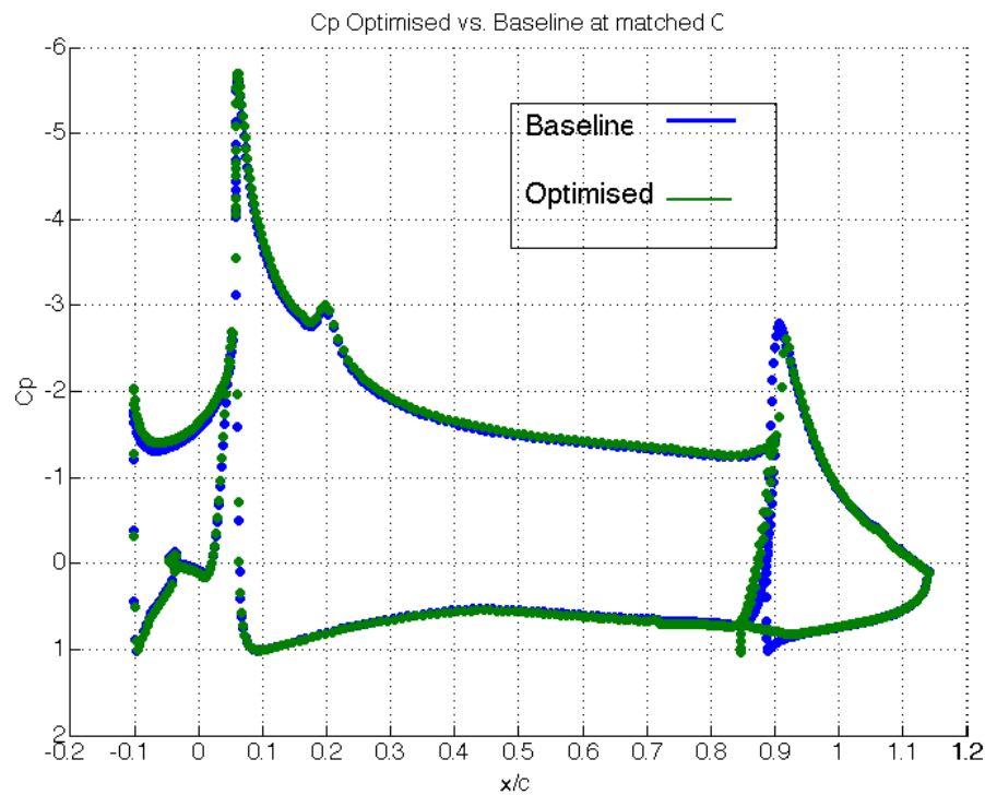
Figure 5.11: Pressure distribution of TC12 profile in high lift configuration optimised solution vs. baseline in MSES, baseline matched C_l , Re 2.95 Million
