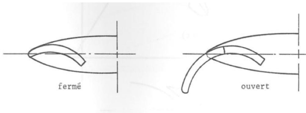
Figure 3.6: Betz flap, Modification De La Forme Dun Profil (1980)
