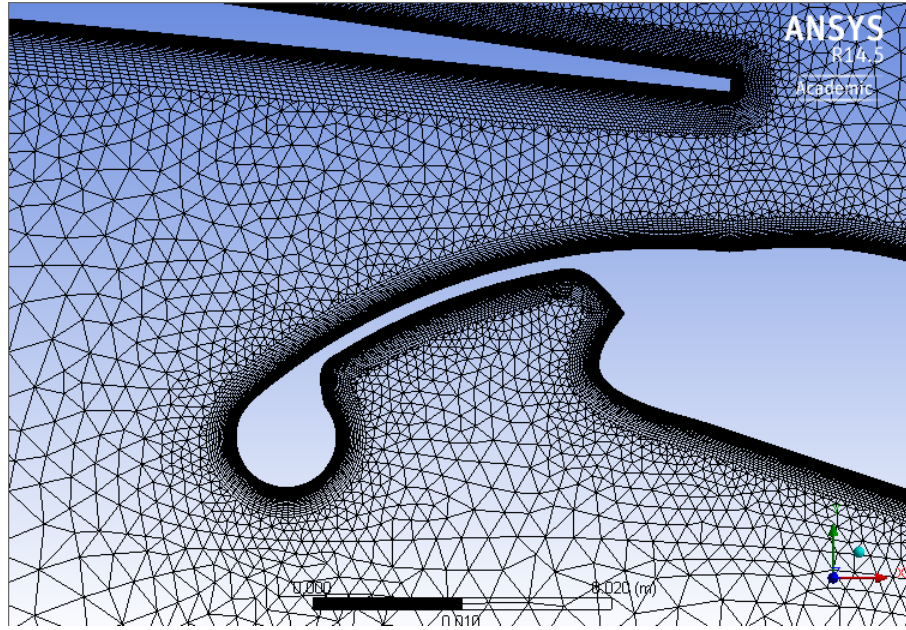
Figure 5.13: Mesh at the leading edge of the TC12 flap showing the implementation of the new concept
