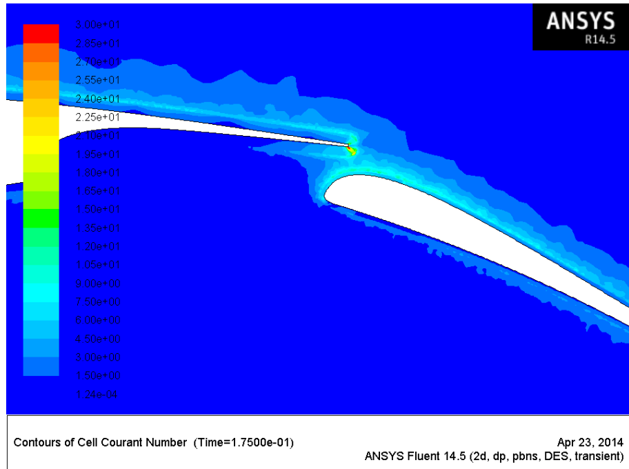
Figure 7.8: Courant numbers at each cell at the trailing edge of the TC12 profile in high lift configuration at 8.09 degrees angle of attack using the DES turbulence model
