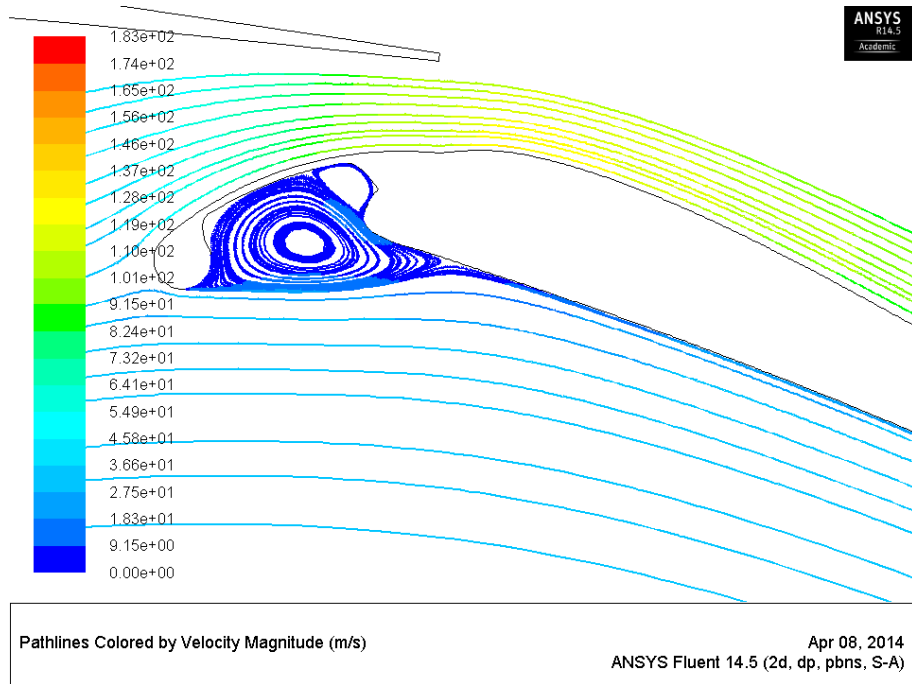
Figure 5.19: Streamlines around trailing edge of zero order optimised flap extension showing the Coanda effect
