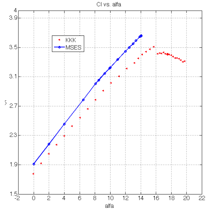
Figure 4.10: C_l vs. \alpha for TC12 profile in high lift configuration at Re 2.95 Million, MSES
