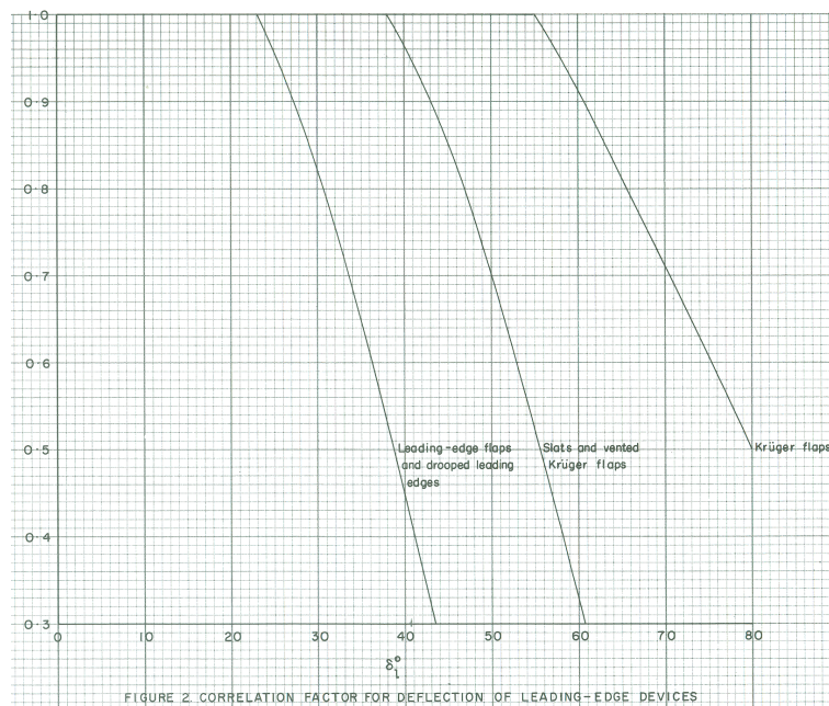
Figure A.2: Figure 2 from ESDU 85033
