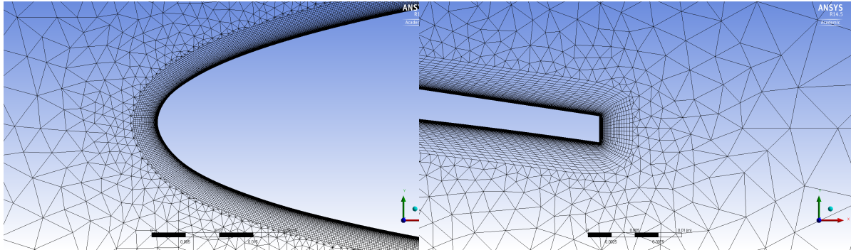
Figure D.3: Mesh for TC12 profile clean configuration leading edge, ANSYS mesher
