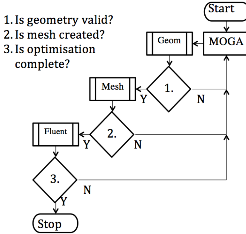
Figure 6.1: System diagram of MOGA optimisation in Ansys DesignXplorer
