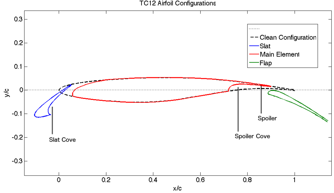
Figure 3.1: Schematic of TC12 profile in high lift configuration
