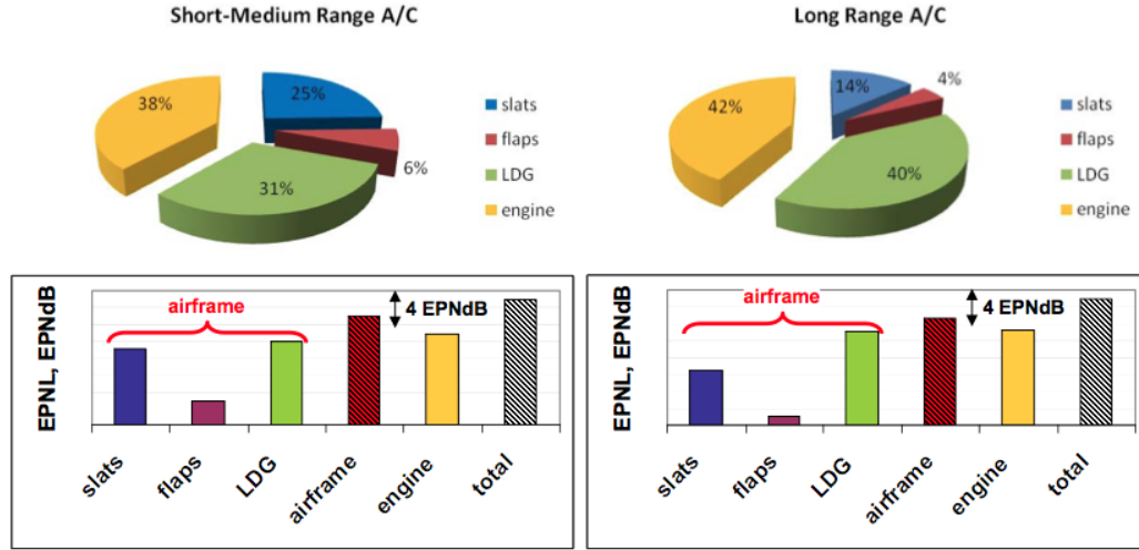
Figure 2.6: Aircraft noise levels by component during approach (Dobrzynski, 2008)
