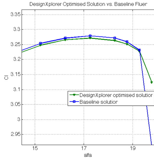
Figure 6.10: C_l vs. \alpha at stall of TC12 profile in high lift configuration DesignXplorer optimised solution vs. baseline in Fluent, SA turbulence model, Re 2.95 million
