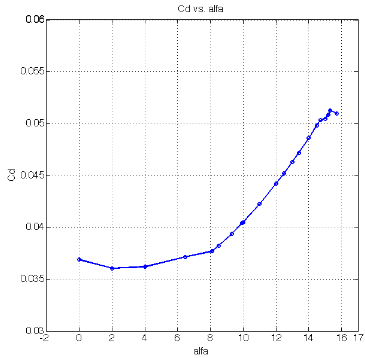
Figure 4.11: C_d vs. \alpha for TC12 profile in high lift configuration in MSES
