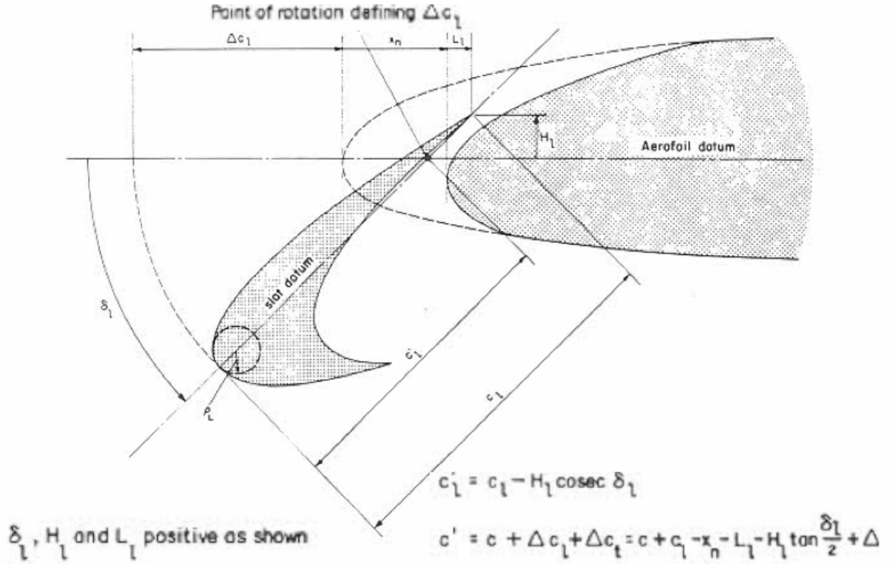
Figure 4.13: ESDU definitions associated with slats
