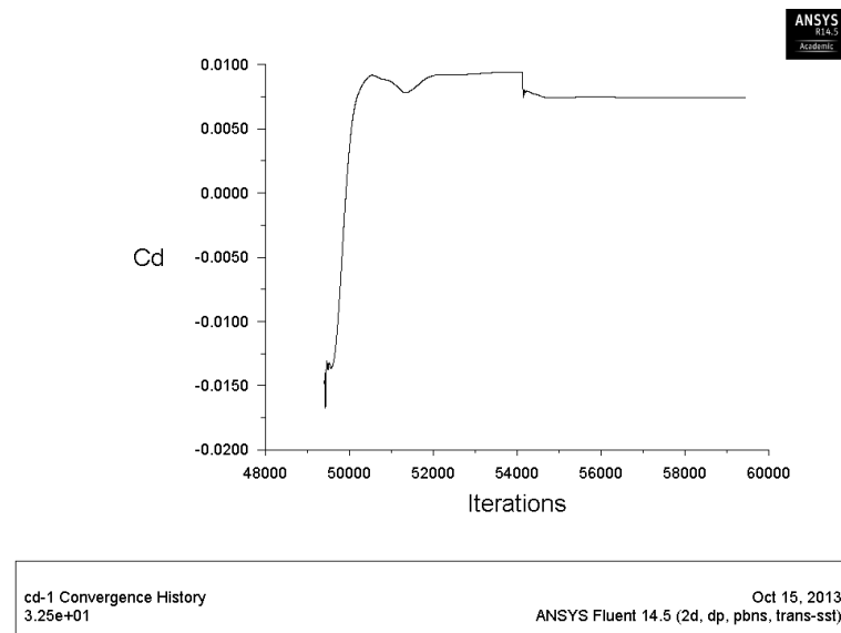
Figure 4.26: Coefficient of Drag convergence for the TC12 profile in clean configuration at 8.1051 degrees
