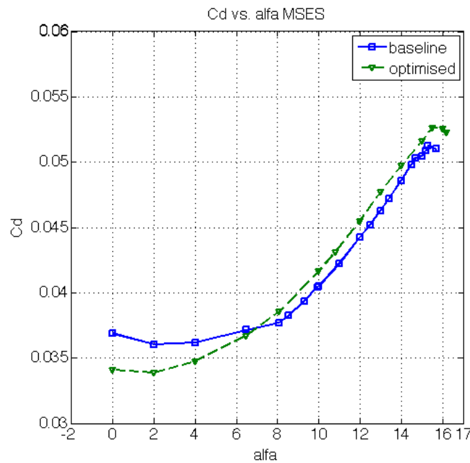
Figure 5.10: C_d vs. \alpha of TC12 profile in high lift configuration optimised solution vs baseline in MSES
