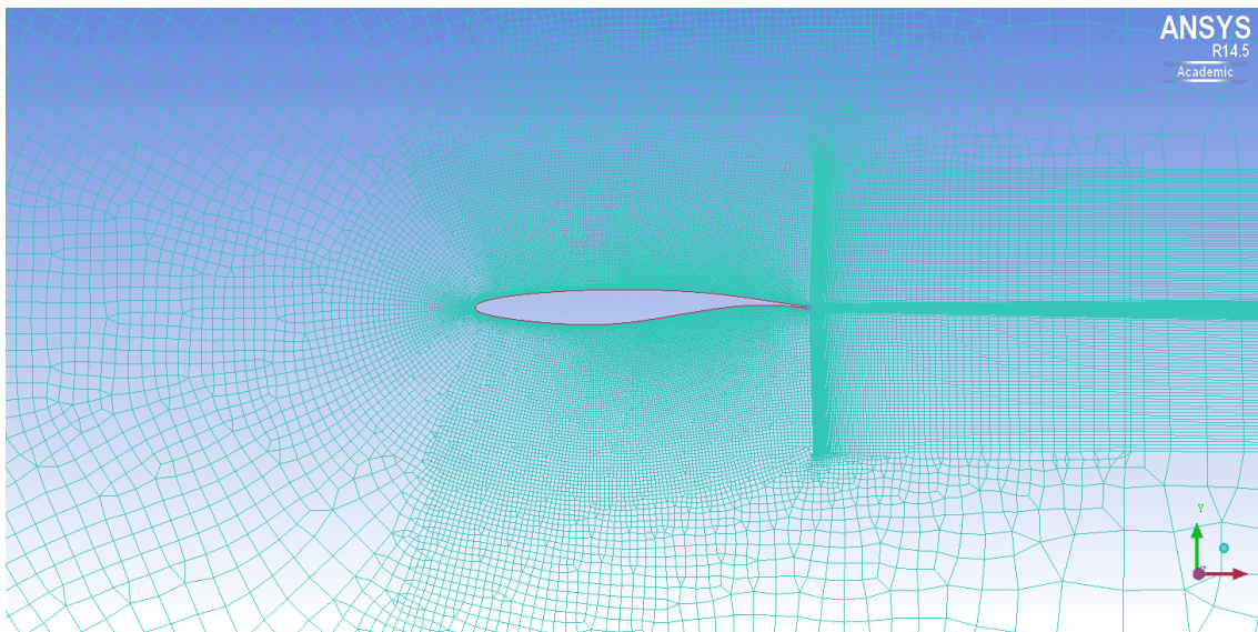
Figure 4.22: TC12 profile clean configuration airfoil mesh close Up on airfoil
