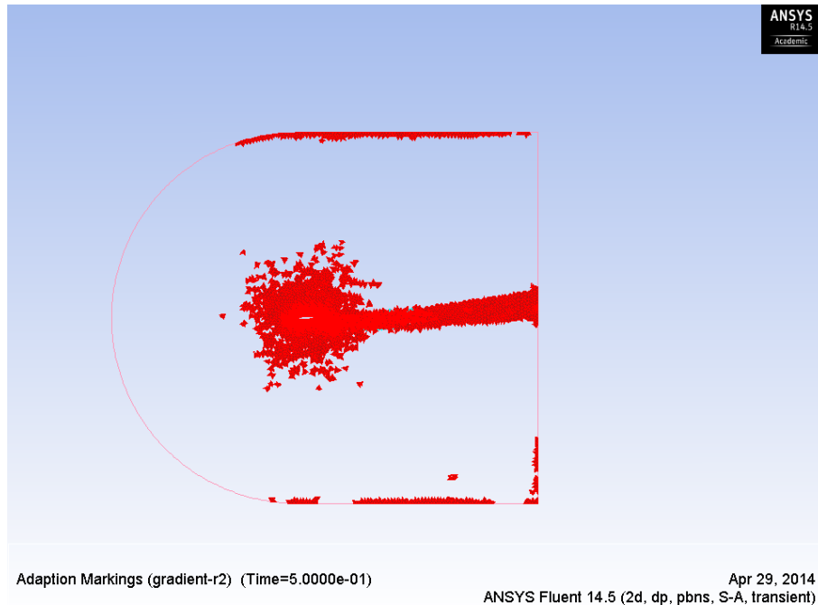
Figure 7.4: Mesh refinements for SA turbulence model acoustic simulations
