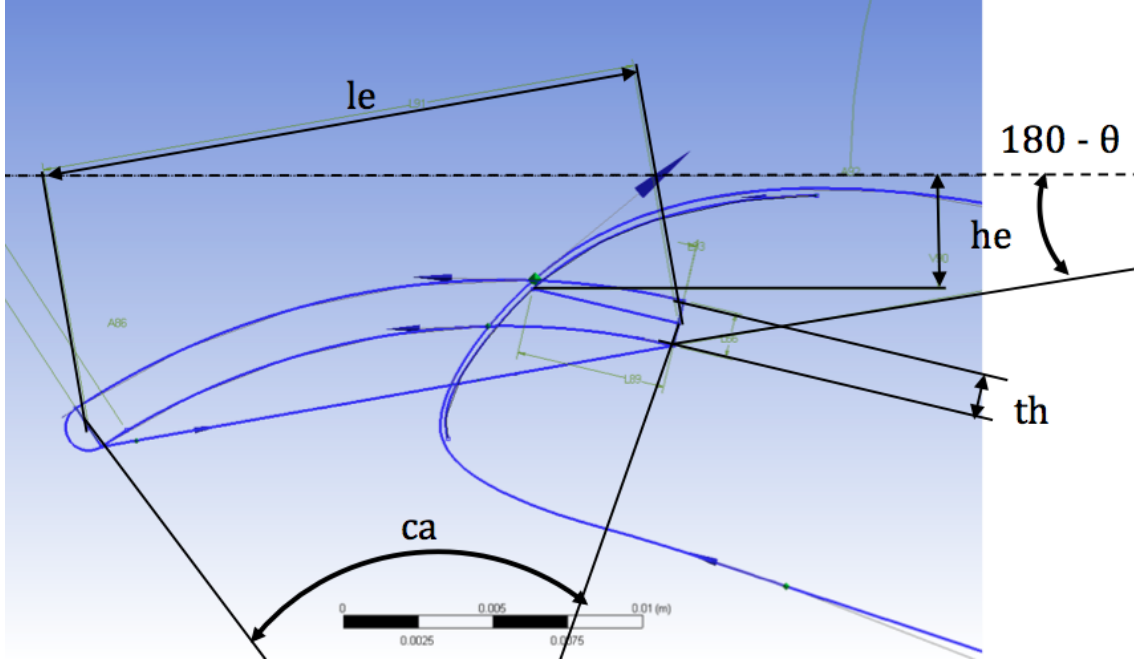
Figure 6.2: Parameterisation of flap extension concept in DesignXplorer
