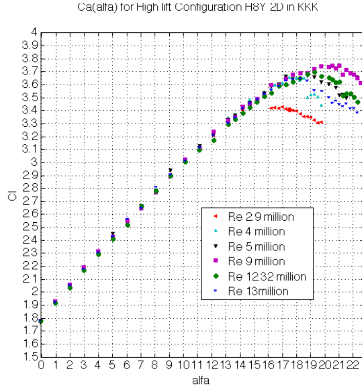
Figure 4.2: Coefficient of lift against angle of attack for TC12 profile in high lift configuration, KKK experiments
