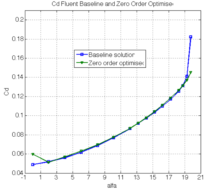
Figure 5.16: Cd vs. alfa of TC12 high lift configuration zero order optimised solution vs. baseline in Fluent SA turbulence model, Re 2.95 Million
