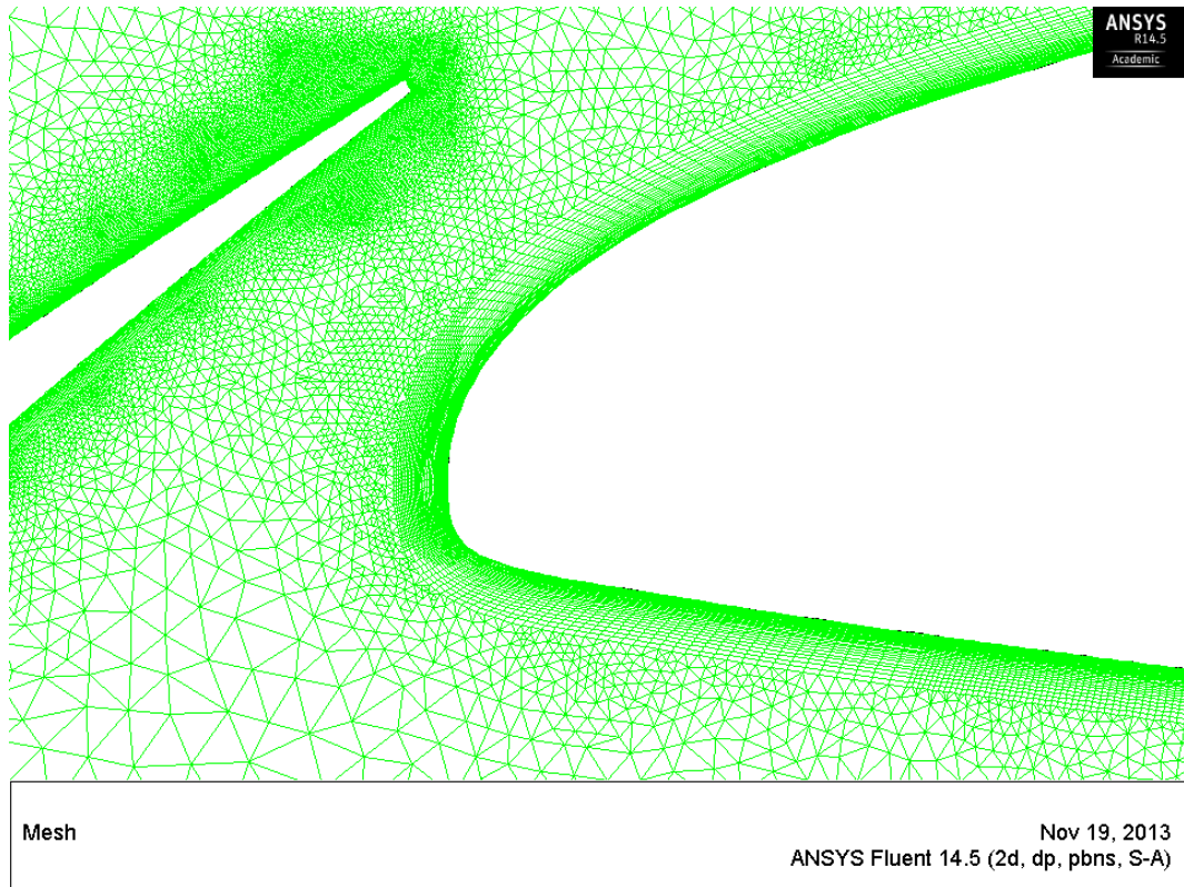
Figure 4.39: Adapted region of mesh for TC12 profile in high lift configuration
