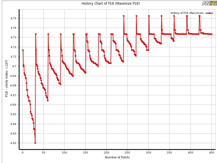
Figure 6.5: Convergence history of DesignXplorer MOGA optimisation of TC12 profile
