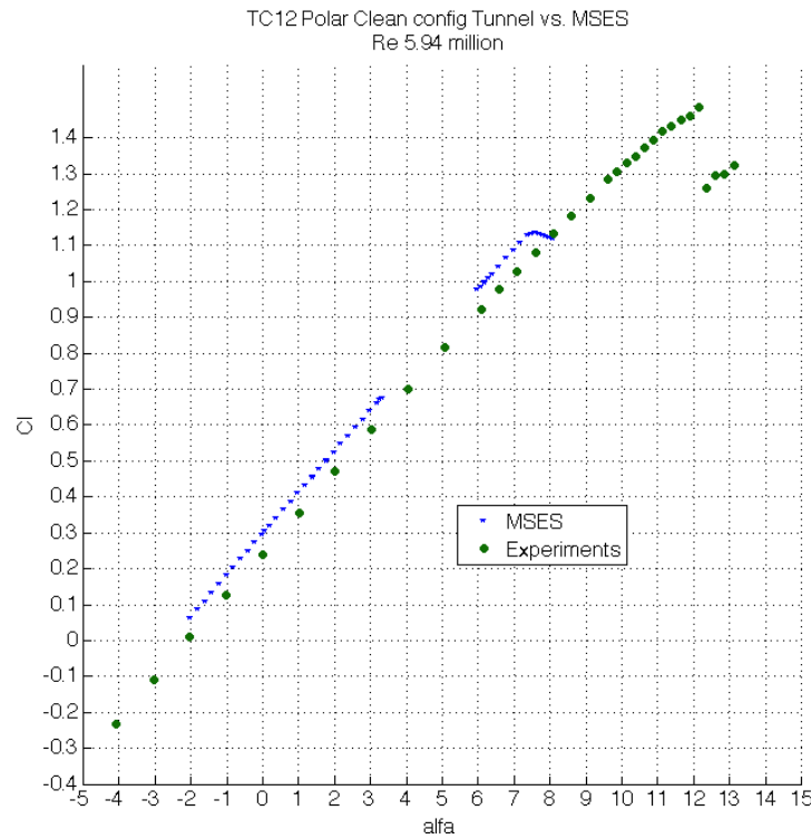
Figure C.2: C_l vs. \alpha for TC12 profile in clean configuration, Re 5.94 million, MSES
