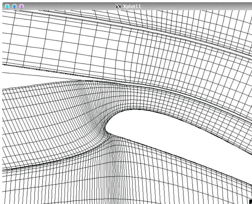
Figure B.5: Grid at leading edge of flap for the TC12 profile in high lift configuration in MSES
