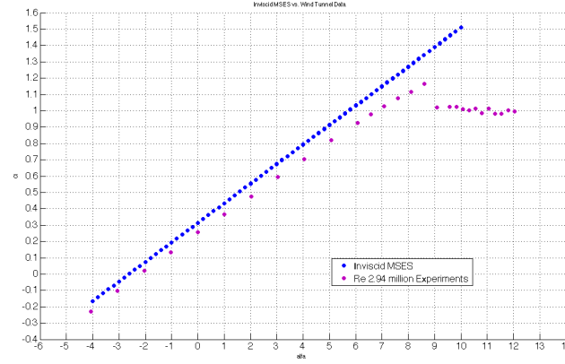
Figure C.1: C_l vs. \alpha for TC12 profile in clean configuration, inviscid, MSES
