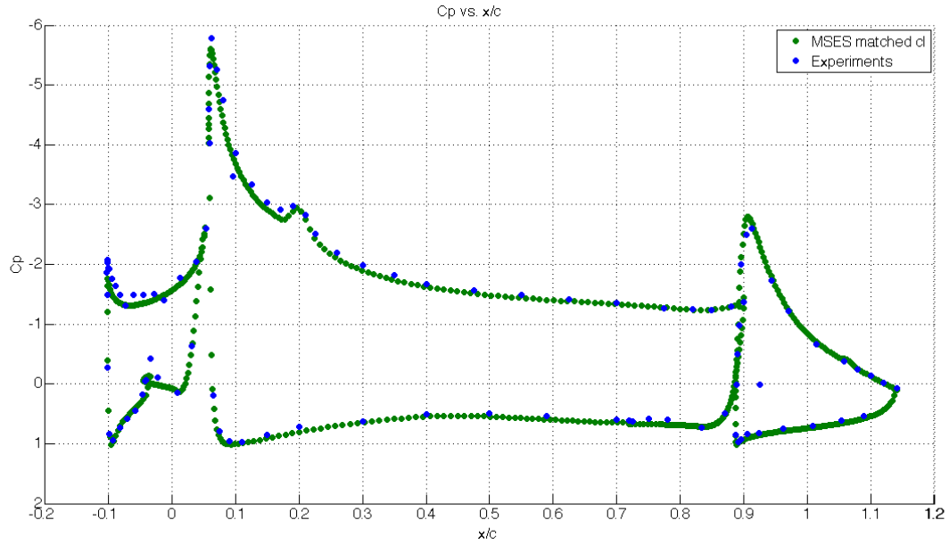
Figure 4.9: Pressure distribution for TC12 high lift at matched Cl 2.879
