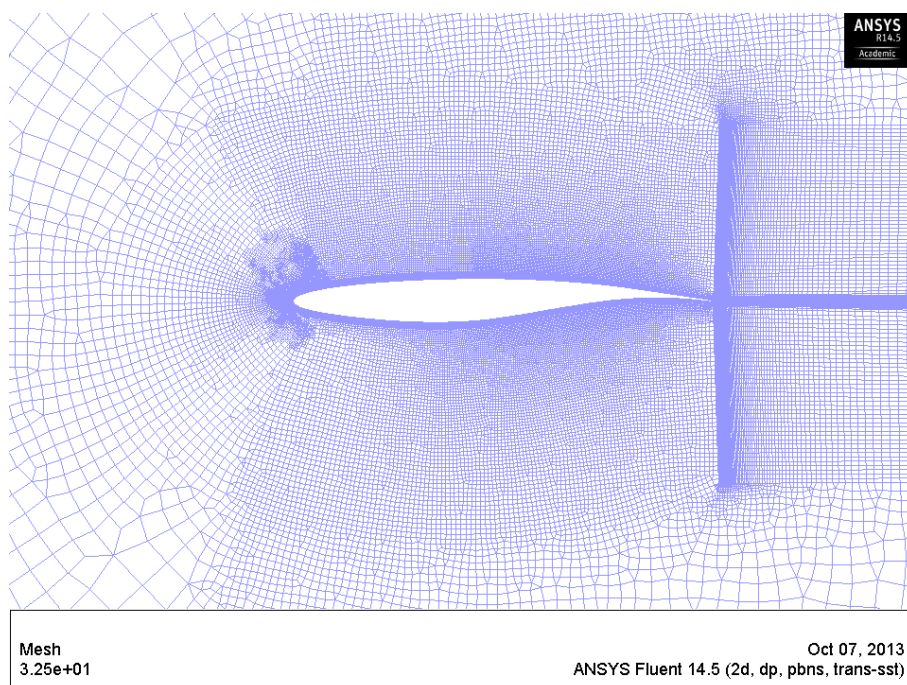
Figure 4.23: Mesh adaptations for TC12 profile clean configuration
