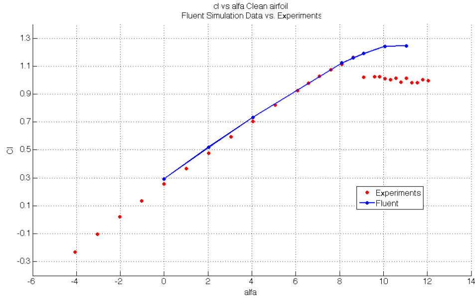
Figure 4.28: C_l vs. \alpha for TC12 in clean configuration compared to experiments, Re = 2.95 Million, transition-SST turbulence model
