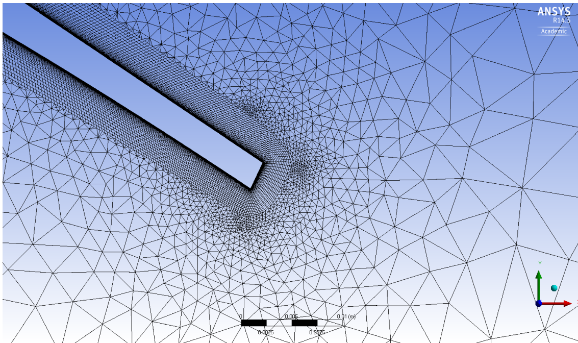
Figure 4.36: Close up of flap trailing edge mesh TC12 profile in high lift configuration
