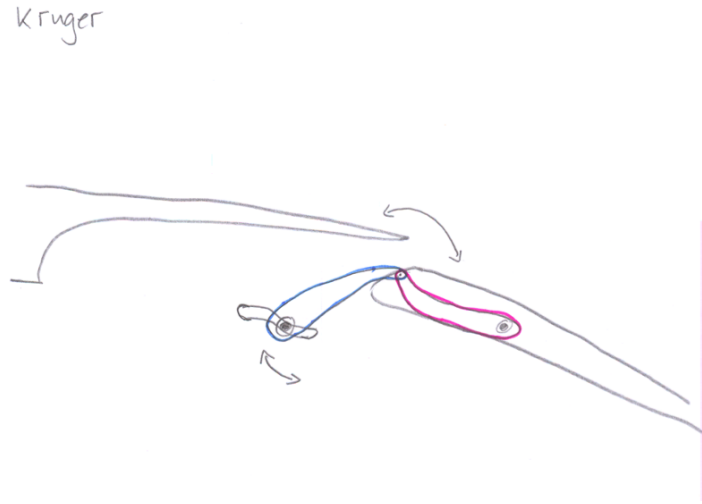
Figure 8.3: Unpowered Krueger flap predesign concept
