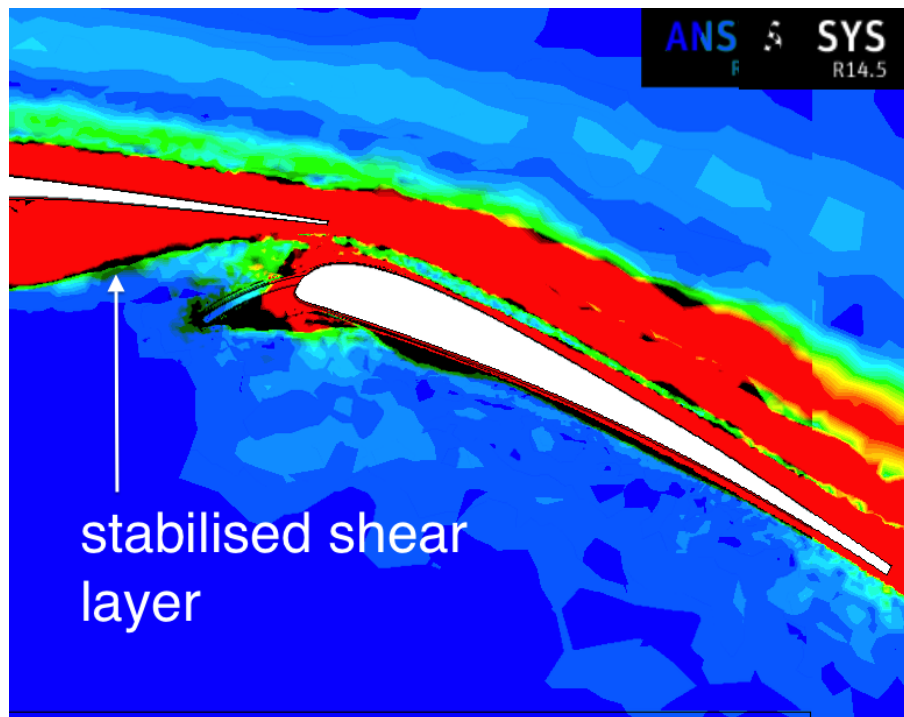
Figure 7.13: Vorticity between 0 - 1 000 near the trailing edge comparing the TC12 profile in high lift configuration compared to the DesignXplorer optimised solution at 8.09 degrees angle of attack using the DES turbulence model
