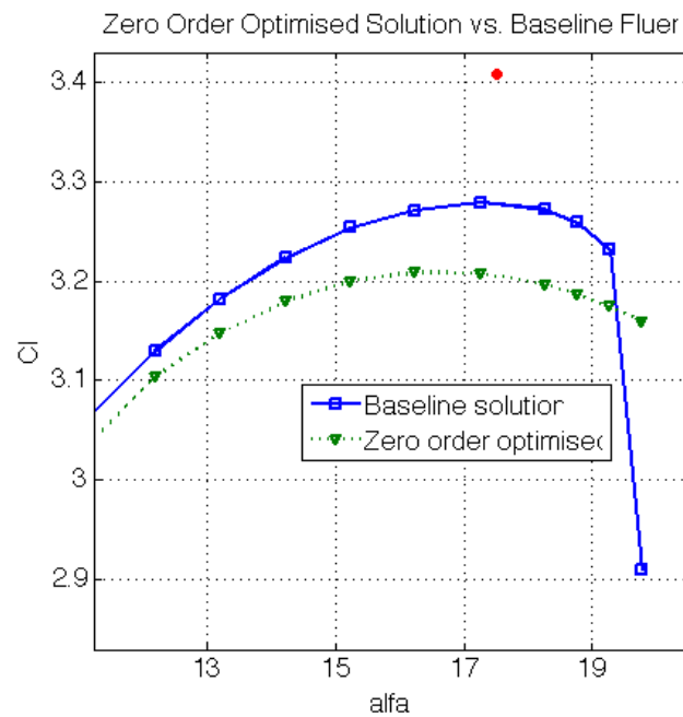
Figure 5.15: C_l vs. \alpha of TC12 high lift configuration at stall zero order optimised solution vs. baseline in Fluent SA turbulence model, Re 2.95 Million
