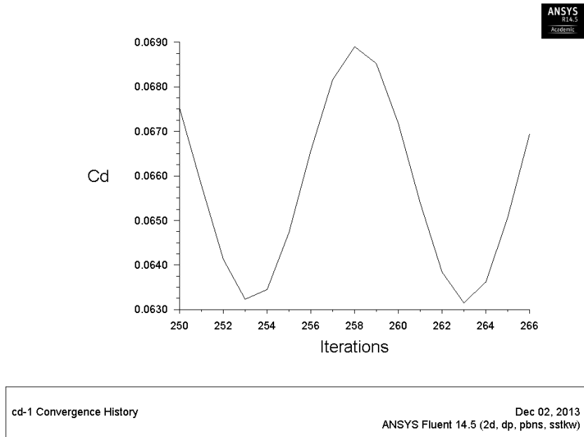
Figure 4.45: Excerpt of value of drag residuals for TC12 profile in high lift configuration, k-omega SST turbulence model, 8.09 degrees, Re 2.95 million
