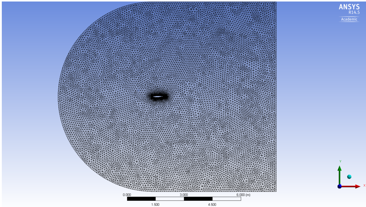
Figure D.1: Mesh for the TC12 profile clean configuration in ANSYS mesher
