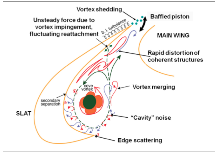
Figure 2.8: Suspected slat noise sources ( Choudhari et al., 2012 )
