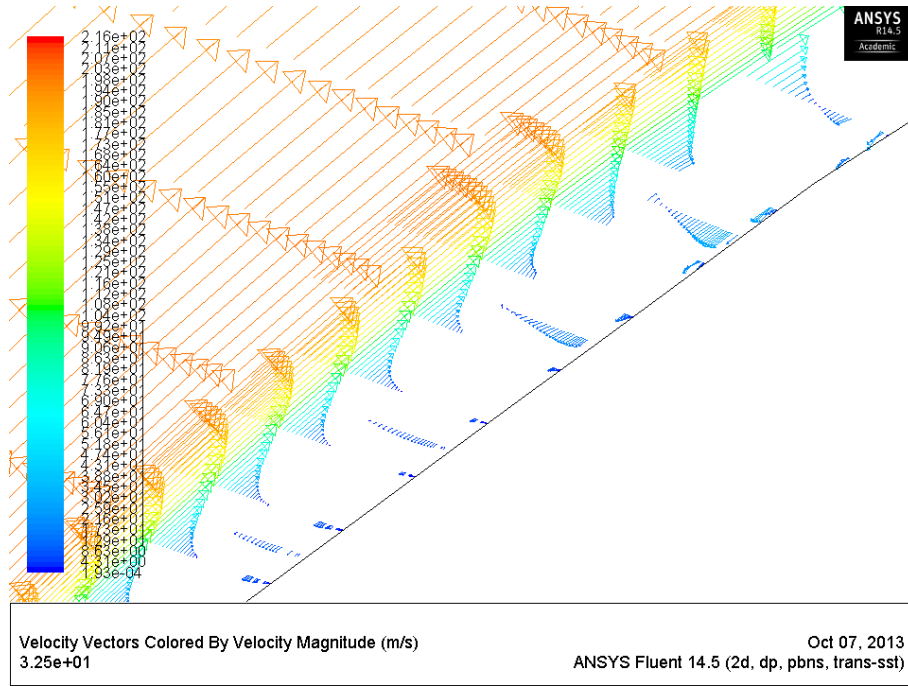
Figure 4.27: Separations at the leading edge of TC12 profile in clean configuration
