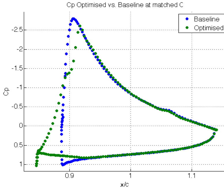
Figure 5.12: Pressure distribution of TC12 high lift configuration flap at 8.09 degrees optimised solution vs. baseline in MSES, baseline matched C_l , Re 2.95 million
