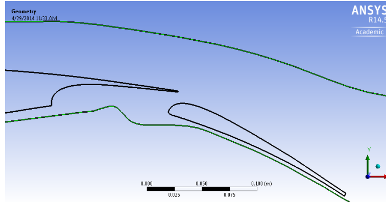
Figure 7.3: Integration region around TC12 profile in high lift configuration for acoustic calculations at flap
