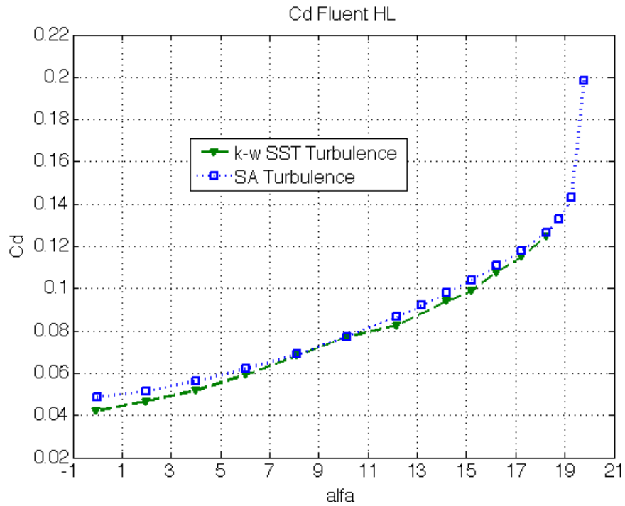
Figure 4.50: C_d vs. \alpha for TC12 profile in high lift configuration, Re 2.95 million
