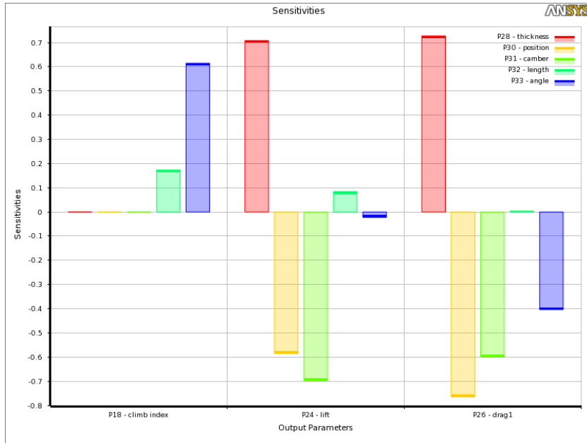
Figure 6.6: Sensitivity analysis of input parameters to output parameters of DesignXplorer MOGA optimisation of TC12 profile
