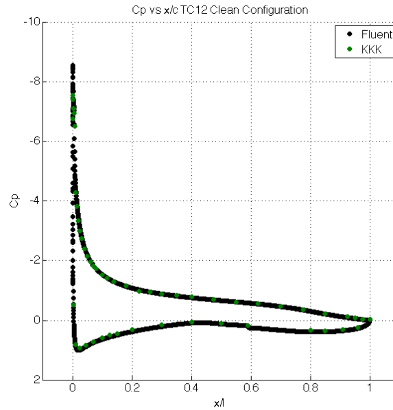
Figure 4.30: Pressure distributions of TC12 profile in clean configuration at 8.1 degrees, Fluent vs. Experiments
