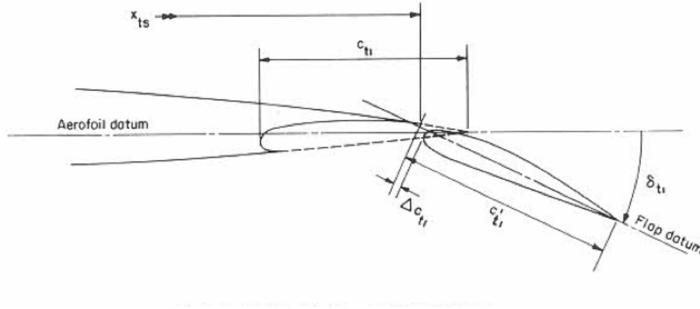
Figure 4.14: ESDU definitions associated with slotted flaps
