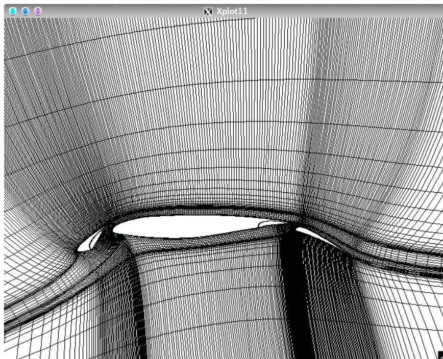
Figure B.2: View of grid close to airfoil for the TC12 in profile high lift configuration in MSES
