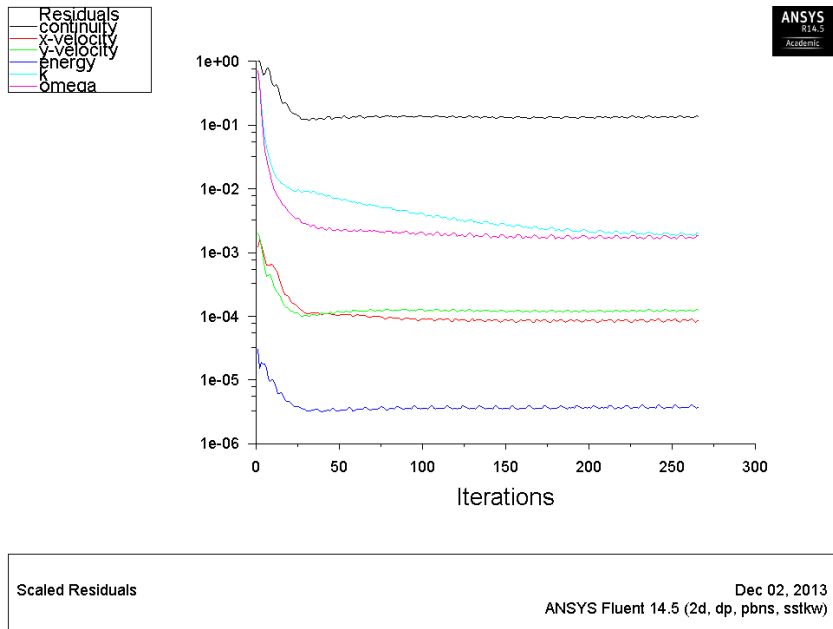
Figure 4.44: Scaled residuals of TC12 profile in high lift configuration, k-omega SST turbulence model, 8.09 degrees, Re 2.95 million
