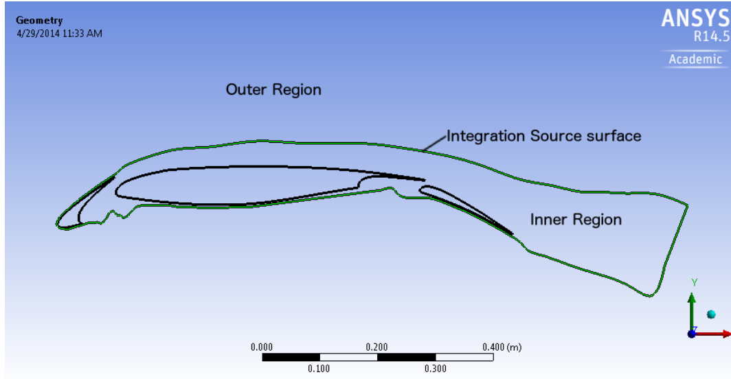
Figure 7.1: Integration region around TC12 profile in high lift configuration for acoustic calculations
