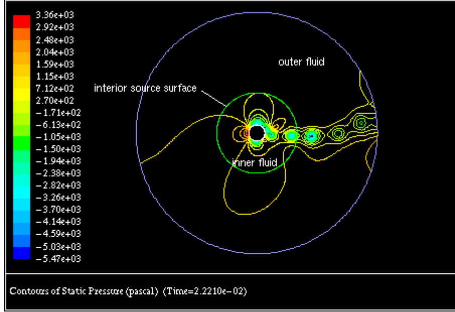
Figure 2.11: Source surfaces as implemented in ANSYS Fluent for FWH solutions ( ANSYS Fluent online user guide , 2013)
