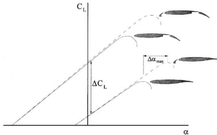
Figure 1.1: Effect of flaps and slats on lift ESDU 85033: Increments in Aerofoil Maximum Lift Coefficient due to Deployment of Various High Lift Devices (1992)
