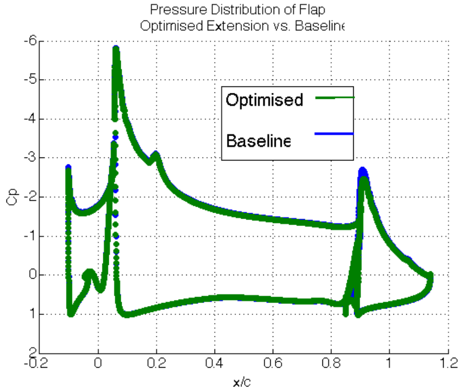
Figure 5.25: Pressure distribution of TC12 high lift configuration optimised solution with slot vs. baseline at 8.09 degrees in Fluent, SA turbulence model, Re 2.95 Million
