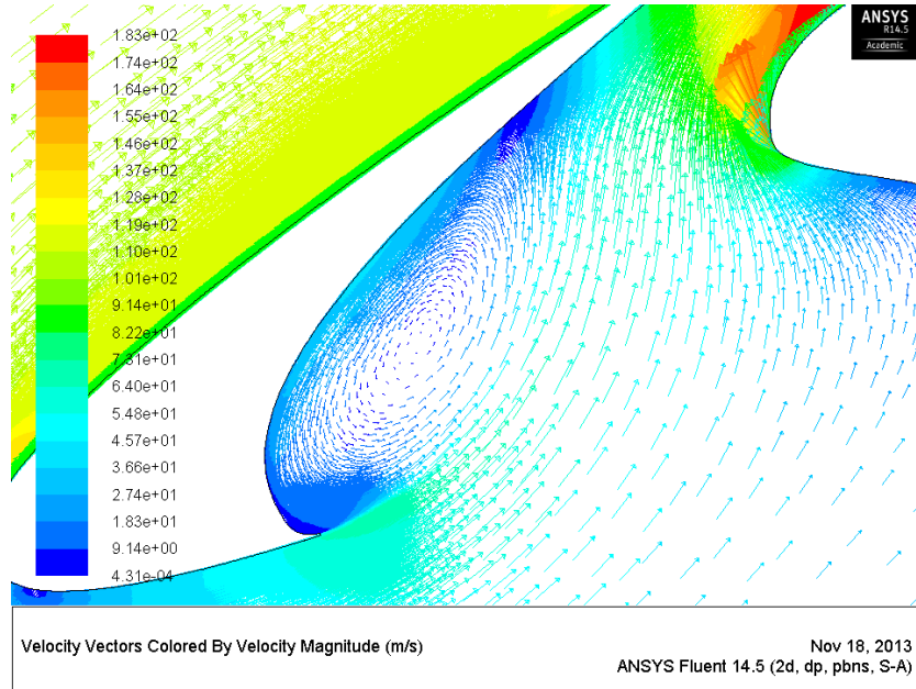
Figure 4.43: Recirculation at slat cove of TC12 profile in high lift configuration, SA turbulence model, 8.09 degrees, Re 2.95 million
