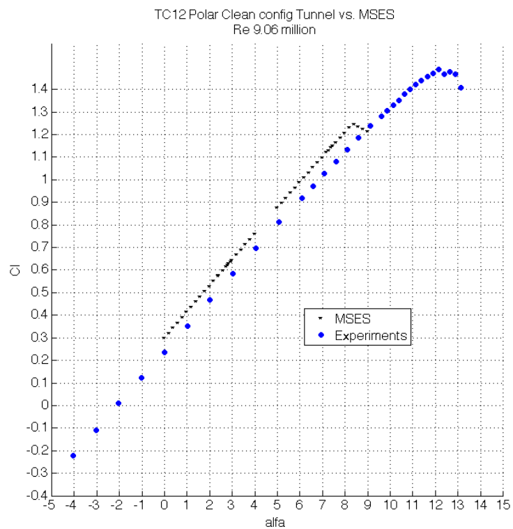
Figure C.3: C_l vs. \alpha for TC12 profile in clean configuration, Re 9.06 million, MSES
