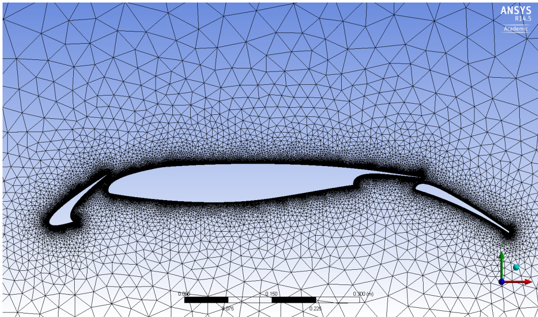
Figure 4.38: Mesh close up of airfoil for TC12 profile in high lift configuration
