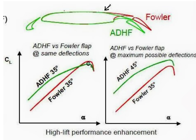
Figure 2.2: Advanced drooped hinge flap lift compared to a conventional fowler flap ( The ADHF “advanced dropped hinge flap” patented by Airbus onboard the A350 XWB, 2013 )
