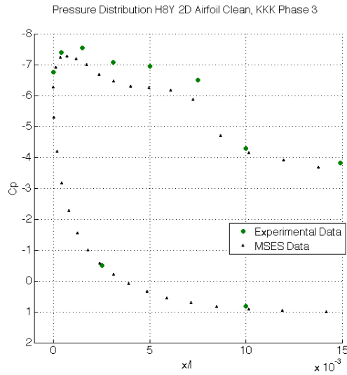
Figure 4.5: Pressure distribution (peak) of TC12 profile in clean configuration at Re 2.94 million, angle of attack 8.11 degrees
