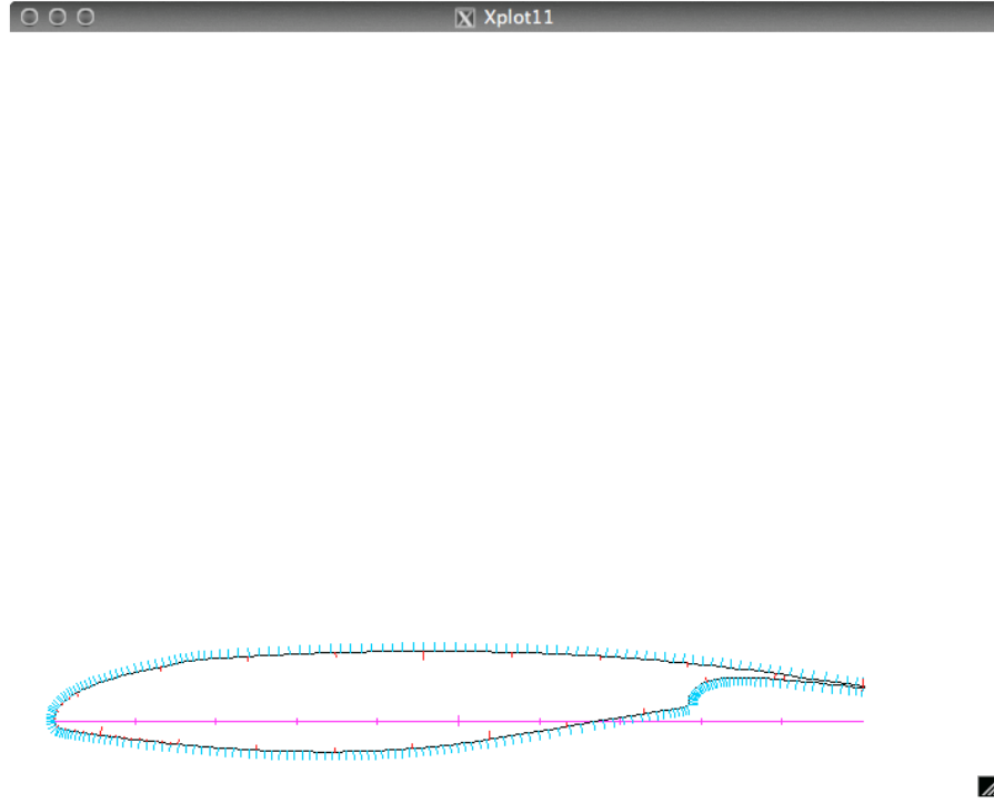
Figure B.7: Main element panelling for the TC12 profile in high lift configuration in MSES
