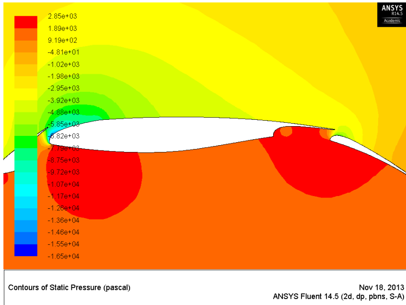
Figure 4.42: Pressure contours for TC12 profile in high lift configuration, SA turbulence model, 8.09 degree, Re 2.95 million
