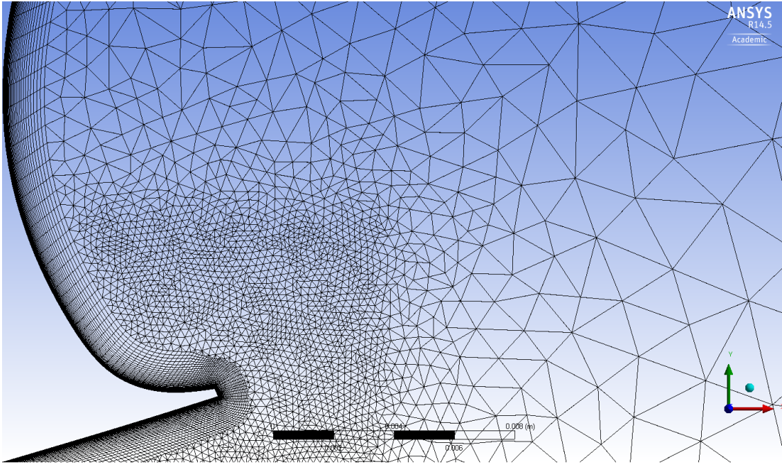
Figure 4.33: Mesh at the cove region of the slat TC12 profile high lift configuration
