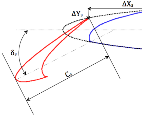
Figure 3.2: Slat motion of TC12 profile in high lift configuration
