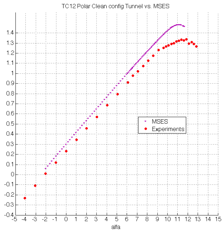
Figure C.5: Cl vs. \alpha for TC12 profile in clean configuration, Re 14.44 million, MSES
