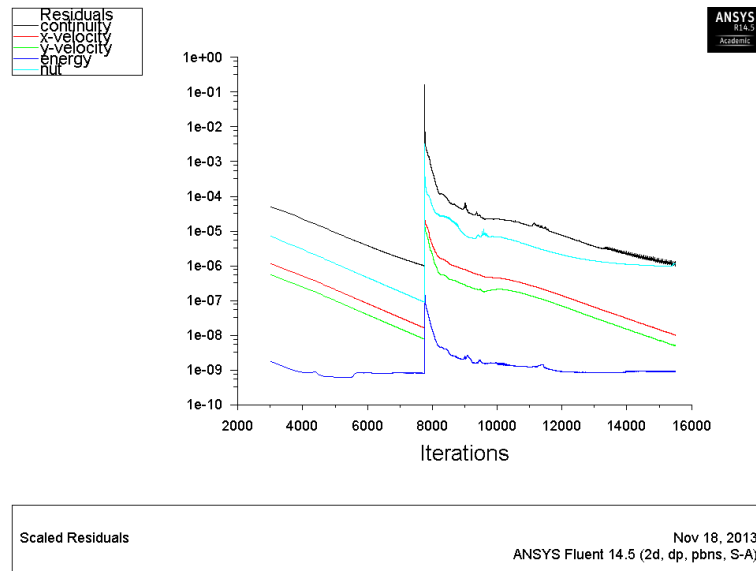
Figure 4.40: Scaled residuals for TC12 high lift configuration mesh, SA turbulence model
