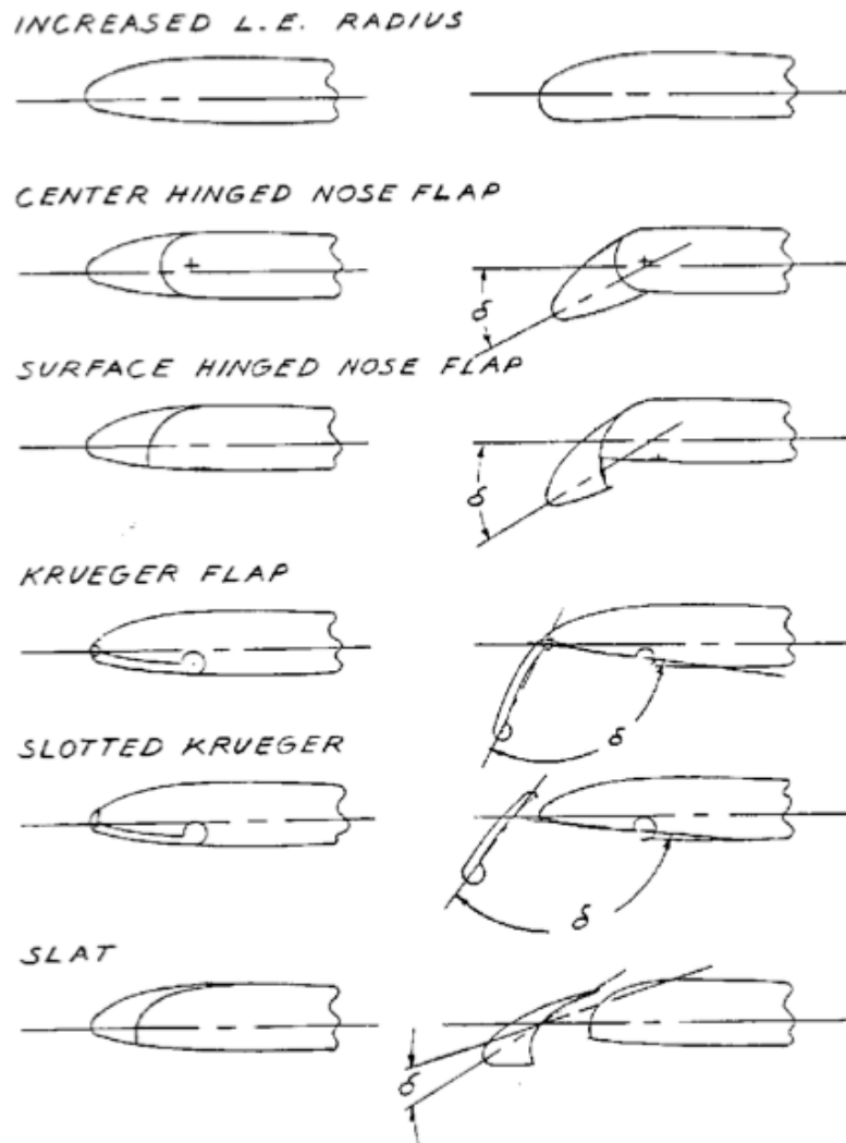
Figure 2.4: Drawings of various leading edge high lift devices
