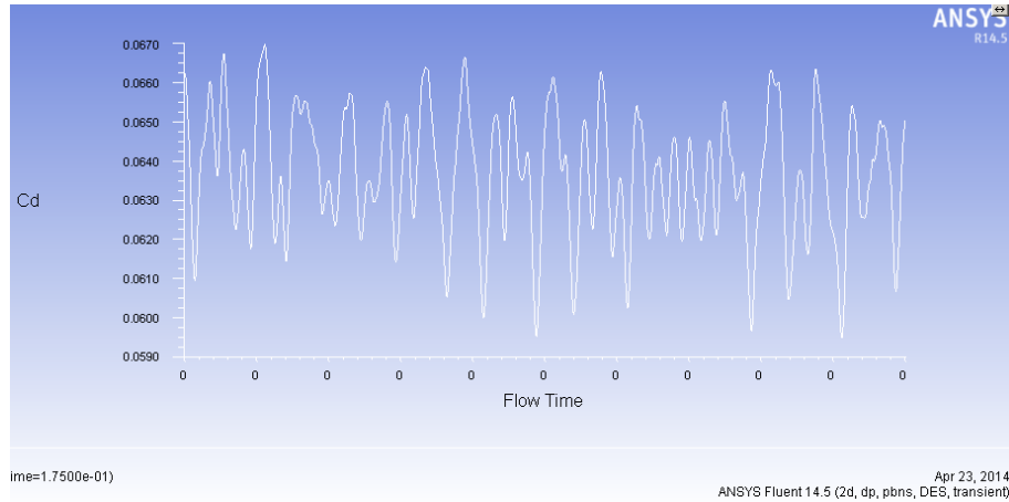
Figure 7.7: Fluctuation of drag during last 1 000 iterations of the TC12 profile in high lift configuration at 8.09 degrees angle of attack using the DES turbulence model
