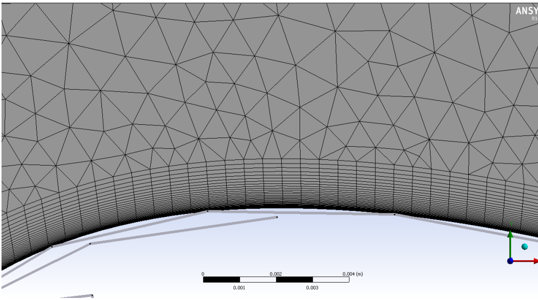
Figure 6.4: Boundary layer sizing of mesh for DesignXplorer optimisation of TC12 high lift profile
