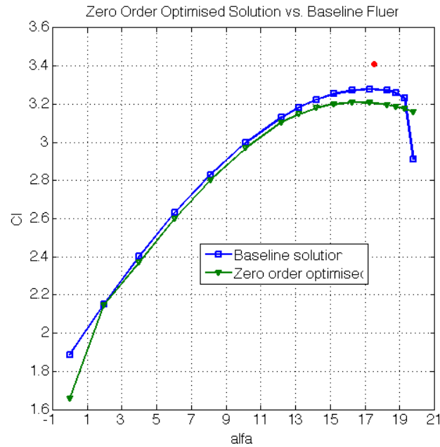
Figure 5.14: C_l vs. \alpha of TC12 high lift configuration zero order optimised solution vs. baseline in Fluent SA turbulence model, Re 2.95 Million
