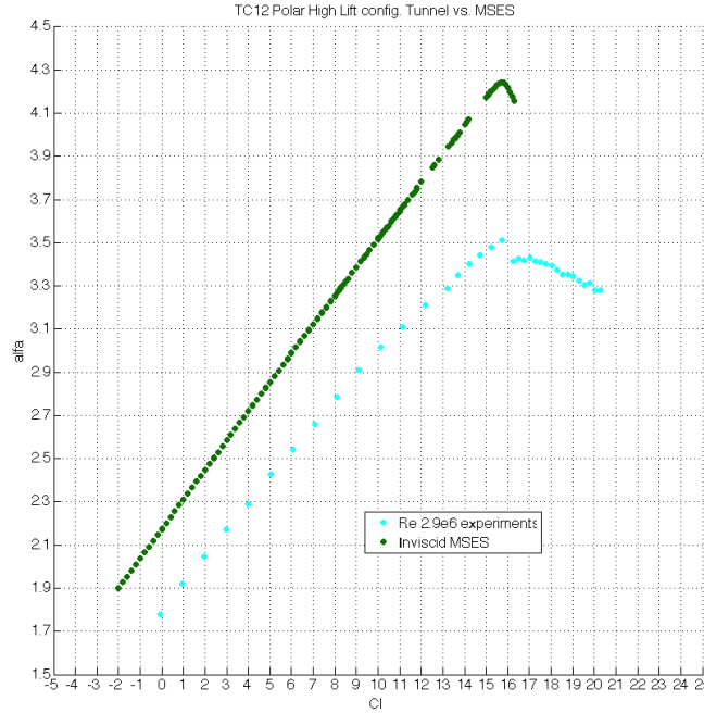
Figure 4.8: Comparison of inviscid MSES results with wind tunnel Re 2.9 million
