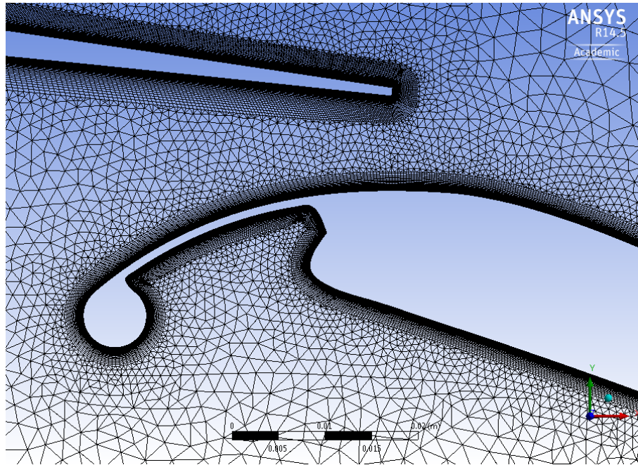
Figure 5.21: Mesh at the leading edge of the TC12 flap showing the meshing around the smoothed concept
