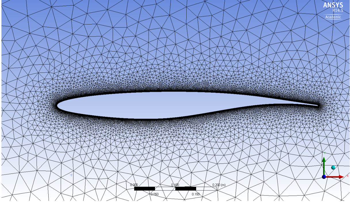
Figure D.2: Mesh for the TC12 profile in clean configuration, ANSYS mesher (zoomed in)
