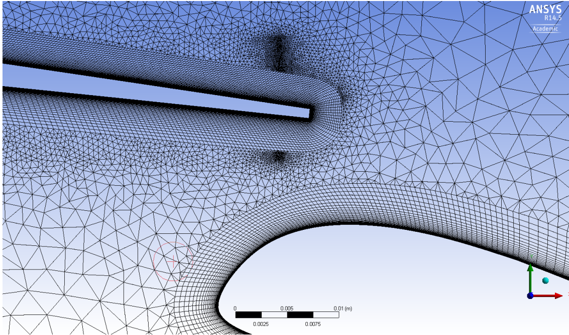
Figure 4.35: Mesh between the spoiler and the flap TC12 profile in high lift configuration
