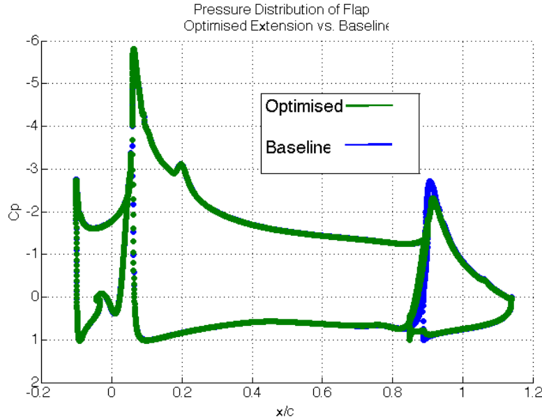
Figure 5.22: Pressure distribution of TC12 high lift configuration optimised solution with smoothed geometry vs. baseline at 8.09 degrees in Fluent, SA turbulence model, Re 2.95 Million
