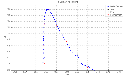
Figure 4.53: Pressure distribution peak for TC12 profile in high lift configuration, SA turbulence model vs. windtunnel data, 8.09 degrees Re 2.95 million
