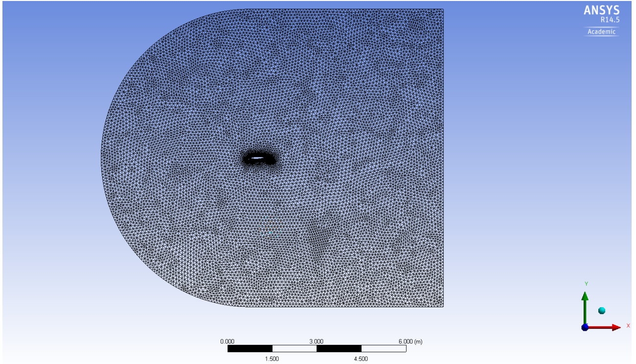
Figure 4.37: Mesh outer block for TC12 profile in high lift configuration
