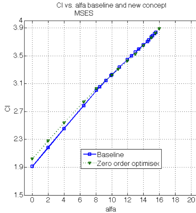
Figure 5.9: C_l vs. \alpha of TC12 profile in high lift configuration optimised solution vs baseline in MSES
