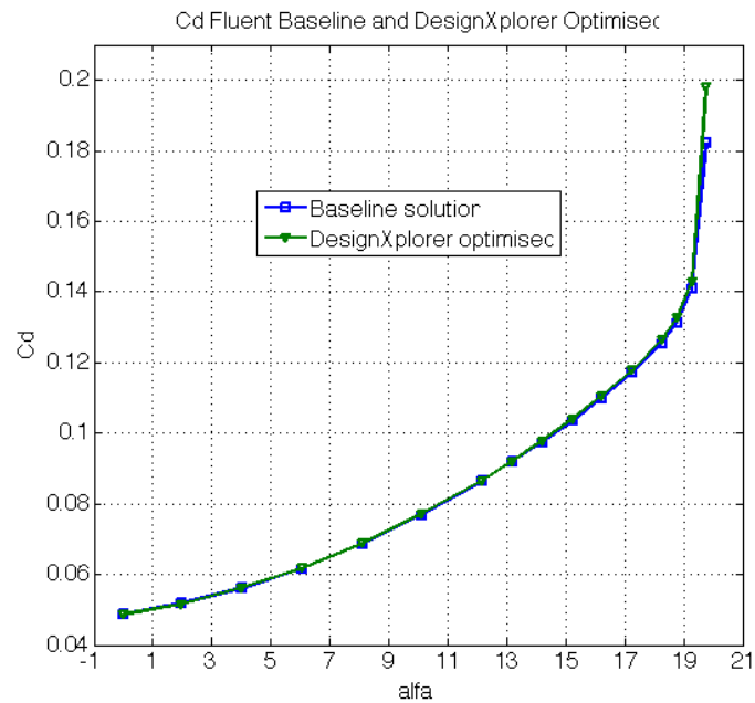
Figure 6.11: C_d vs. \alpha of TC12 profile in high lift configuration DesignXplorer optimised solution vs. baseline in Fluent SA turbulence model, Re 2.95 million
