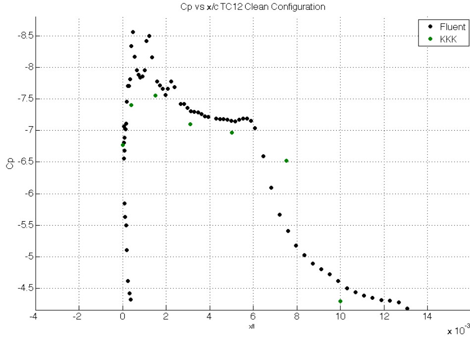
Figure 4.31: Pressure Distributions of TC12 profile in clean configuration zoomed in at separation bubble, Fluent vs. experiments
