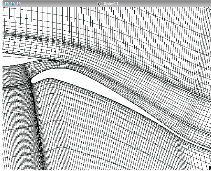
Figure 5.8: Gridding at the flap for the zero order optimised extension
