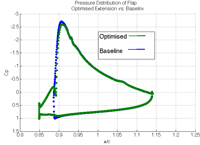
Figure 6.13: Pressure distribution of TC12 high lift configuration flap at 8.09 degrees DesignXplorer optimised solution vs. baseline in Fluent, Re 2.95 million, SA turbulence model
