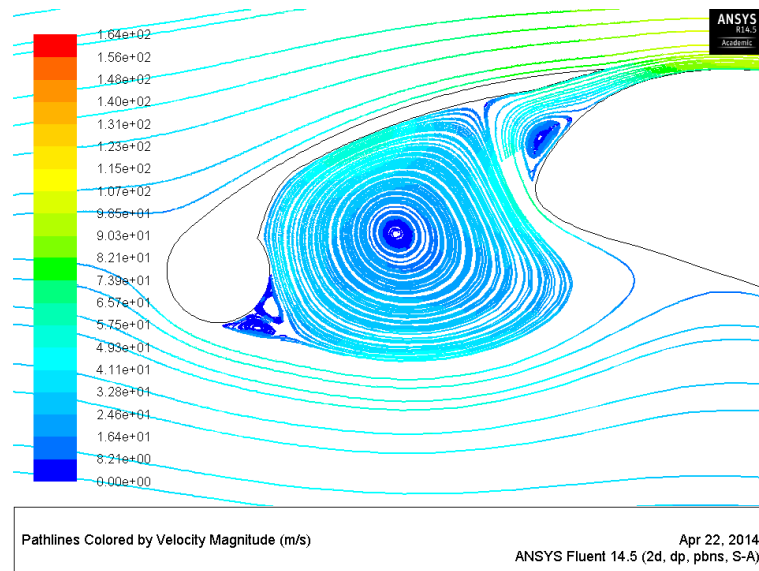
Figure 5.27: Recirculation regions on new concept extension with slot
