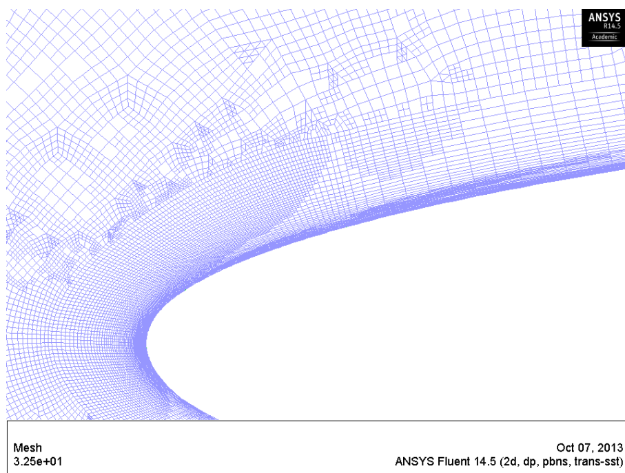
Figure 4.24: Mesh adaptations of TC12 profile clean configuration within the boundary layer at the leading edge
