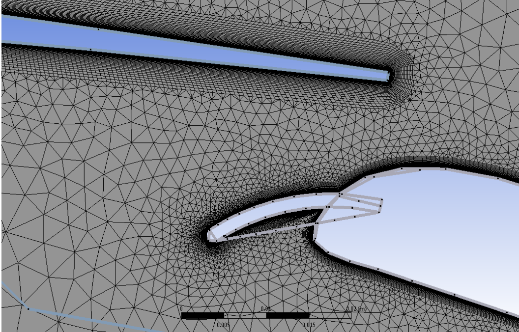
Figure 6.3: Example of an automatically generated mesh for DesignXplorer optimisation of TC12 high lift profile
