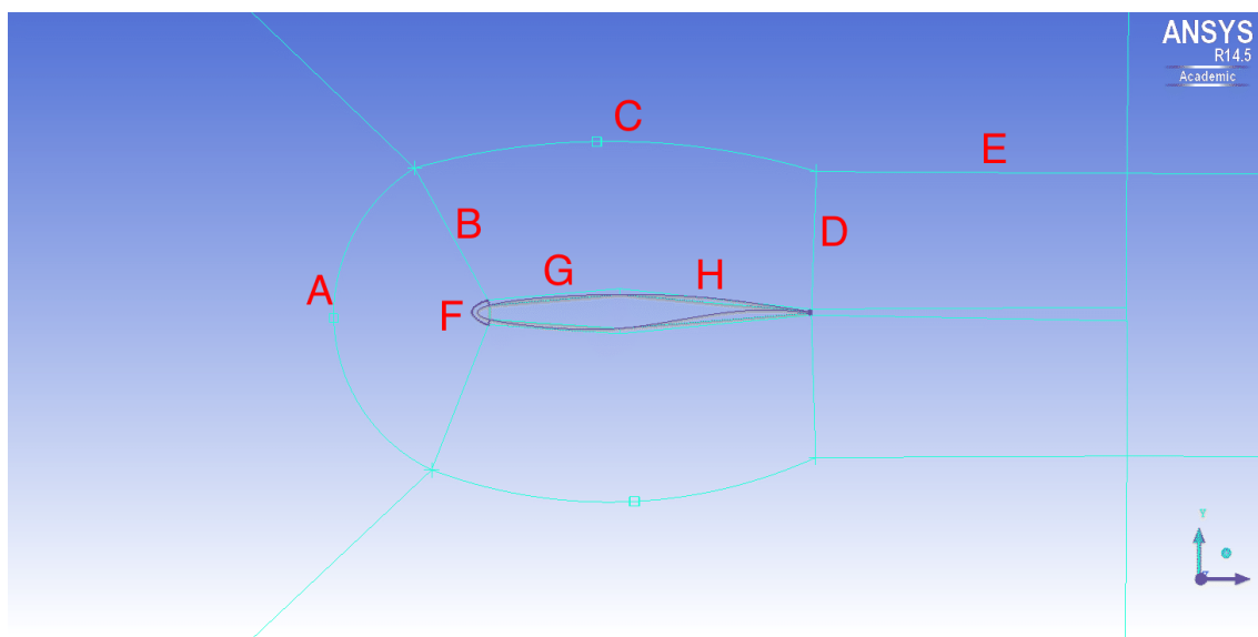
Figure 4.17: Close up of blocking of TC12 profile clean configuration mesh
