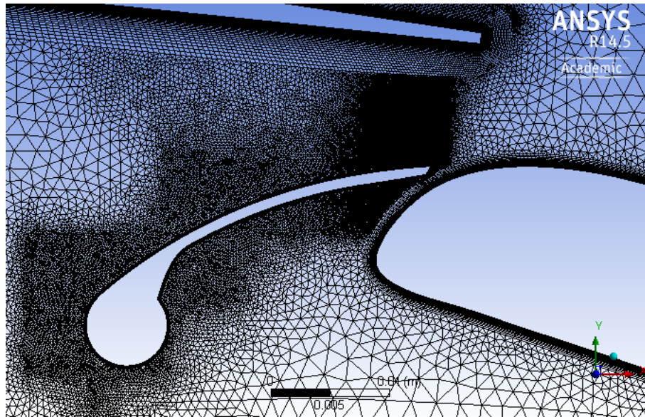
Figure 5.24: Mesh at the leading edge of the TC12 flap showing the meshing around the slotted concept
