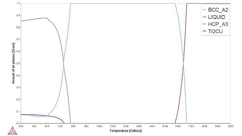
Figure 4.41: Phase proportion diagram for Ti-8Ta-1.5Mo-1.5Zr. Figure 4.42: Phase proportion diagram for Ti-8Ta-1.5Mo-1.5Zr-1Cu. Figure 4.43: Phase proportion diagram for Ti-8Ta-1.5Mo-1.5Zr-3Cu.
