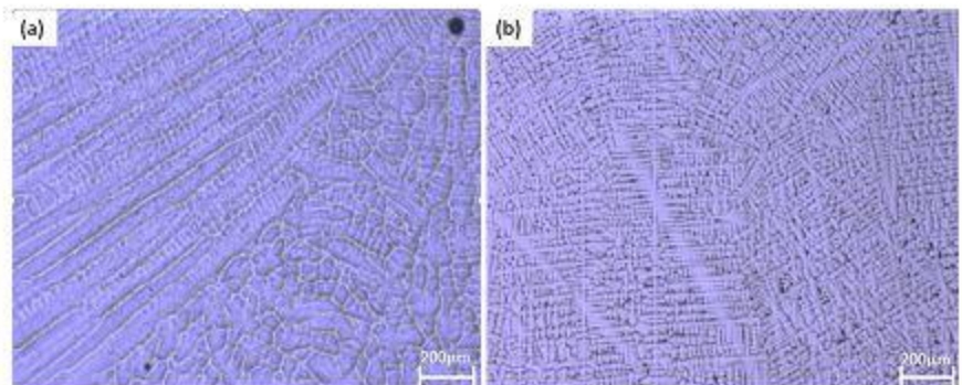
Figure 6: Optical micrographs of as-cast: (a) Ti-2Ta-8Mo-8Sn and (b) Ti-2Ta-8Mo-8Sn-5Cu (wt%) showing mainly a cored dendritic structure, with small proportions (Ti,Cu)
