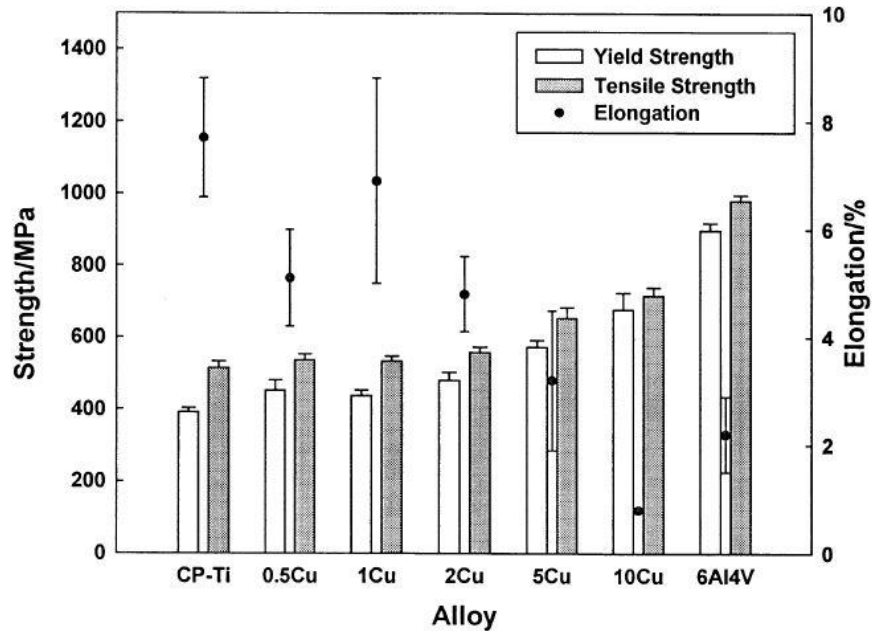
Figure 2.17: Tensile strength, yield strength, and elongation of Ti alloys (Kikuchi et al., 2003).
