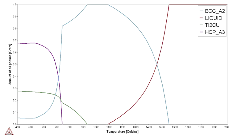
Figure 4.49: Phase proportion diagram for Ti-8Zr-4Ta-2Mo-5Cu.
