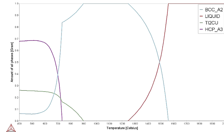
Figure 4.20: Phase proportion diagram for Ti-8Nb-4Zr-10Cu.
