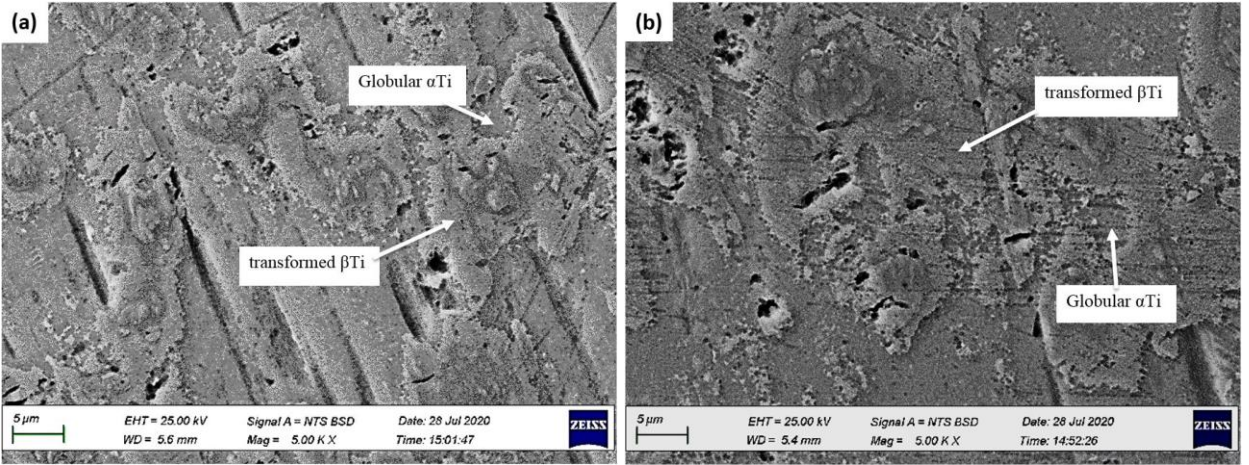
Figure 5.27: SEM-BSE images of as-received Ti-10.1Ta-1.7Nb-1.6Zr deformed at 10 s -1 strain rate: (a) 850°C and (b) 950°C.
