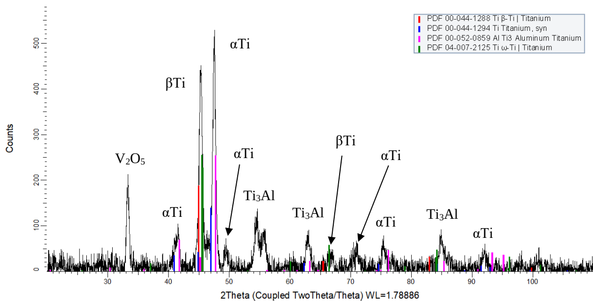
Figure 5.2: XRD analysis of the wrought Ti-6Al-4V (wt%) alloy (Bodunrin, 2018), showing \alpha Ti and \beta Ti peaks shifted due to alloying.
