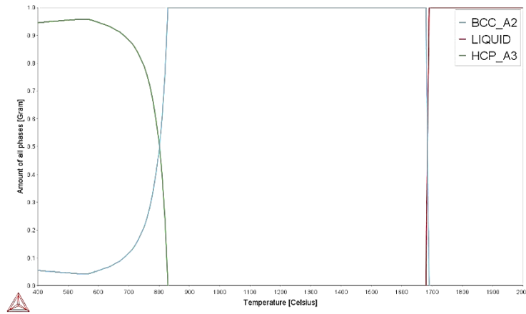
Figure 4.36: Phase proportion diagram for Ti-6Ta-2Zr-1.5Mo.
