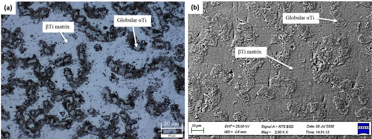
Figure 5.3: As-received Ti-10.1Ta-1.7Nb-1.6Zr (wt%): (a) Optical micrograph and (b) SEM-BSE image.
