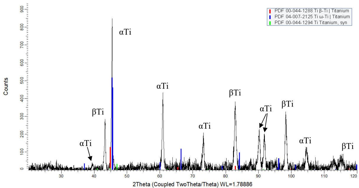
Figure 5.29: XRD analysis of the as-received Ti-10.1Ta-1.7Nb-1.6Zr deformed at 950°C and 10 s -1 strain rate, showing mainly αTi with βTi peaks, shifted by alloying.
