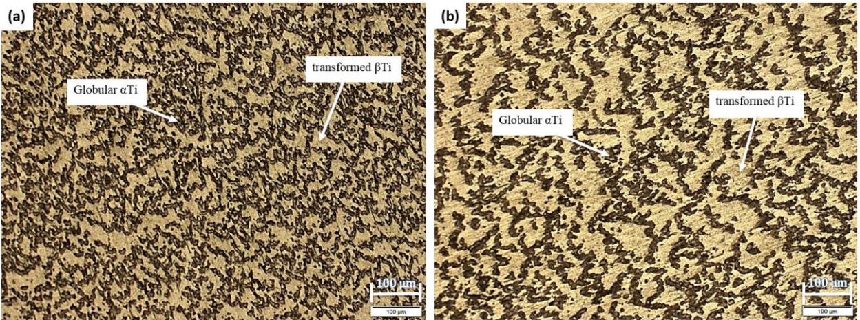
Figure 5.26: Optical micrographs of as-received Ti-10.1Ta-1.7Nb-1.6Zr deformed at 10 s -1 strain rate: (a) 850°C and (b) 950°C.
