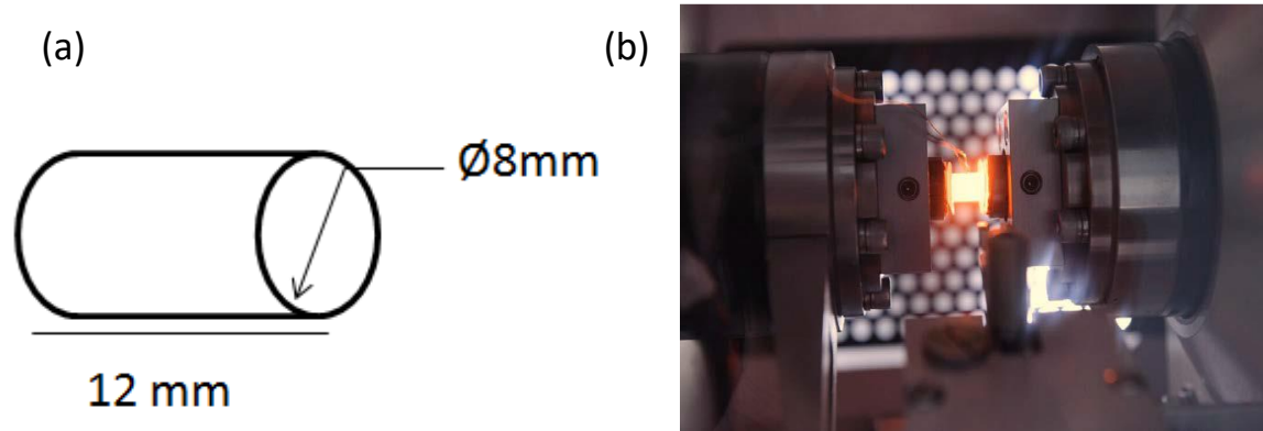
Figure 3.2: Hot compression testing: (a) test sample and (b) testing in the Gleeble 3500 ® (Bodunrin, 2018).
