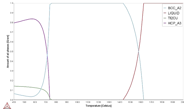
Figure 4.74: Phase proportion diagram for Ti-10Ta-8Zr-5Cu.
