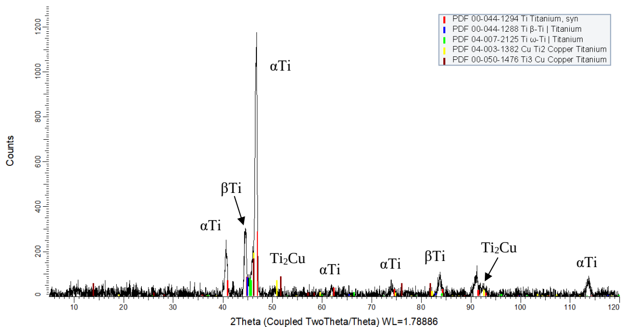
Figure 5.8: XRD analysis of the as-cast Ti-6Nb-4Zr-5Cu (wt%) alloy, showing mainly shifted \alpha Ti peaks, with some Ti_2Cu .
