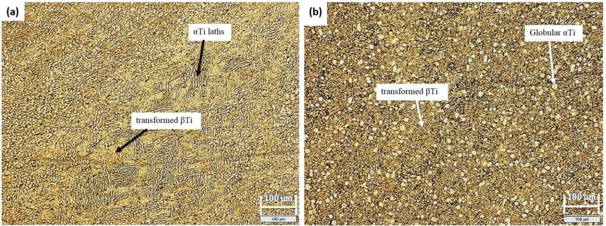
Figure 5.14: Optical micrographs of as-received Ti-6Al-4V (wt%) deformed at 0.1 s -1 strain rate: (a) 850°C and (b) 950°C.
