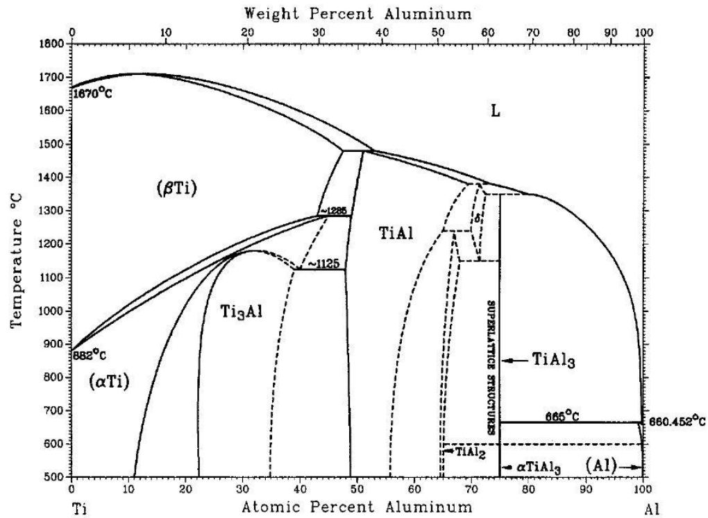
Figure 2.3: Ti-Al phase diagram (Massalski, 1990).
