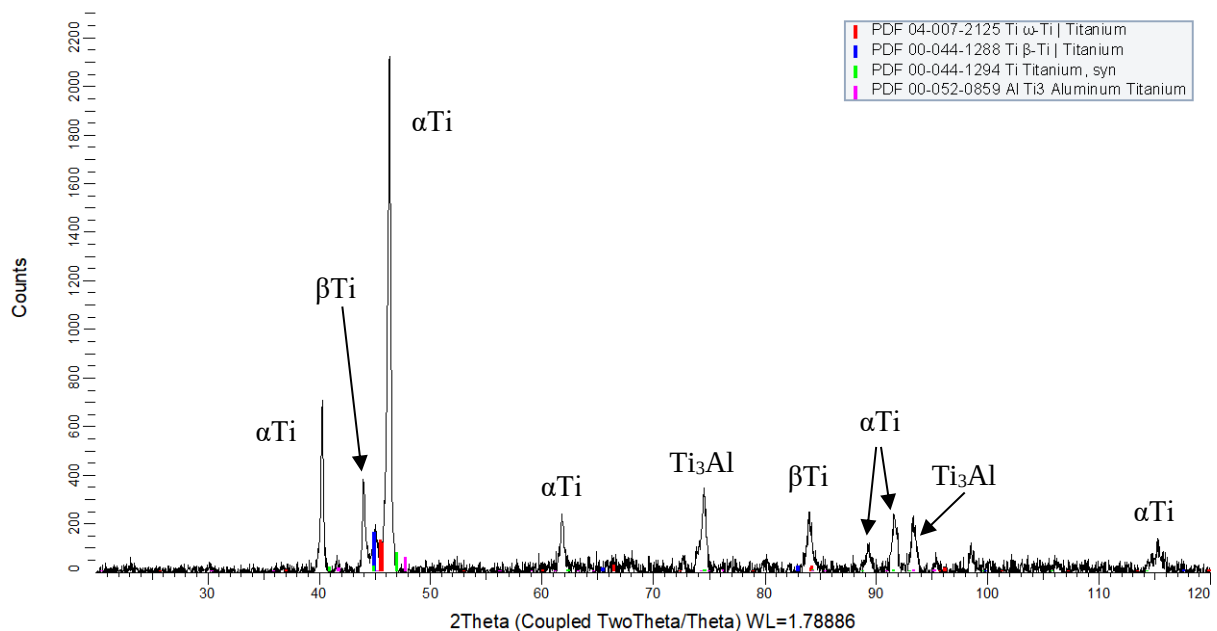
Figure 5.16: XRD analysis of the as-received Ti-6Al-4V deformed at 850°C and 0.1 s -1 strain rate, showing \alpha Ti and \beta Ti peaks shifted by alloying.
