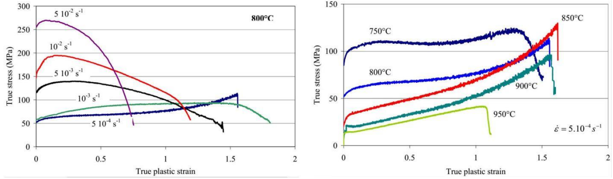
Figure 2.20: Tensile stress-strain curves of Ti-6Al-4V at 5 \times 10^{-2} - 5 \times 10^{-4} \text{ s}^{-1} and 750-950°C from a Gleeble 3800® (Vanderhasten, 2008).
