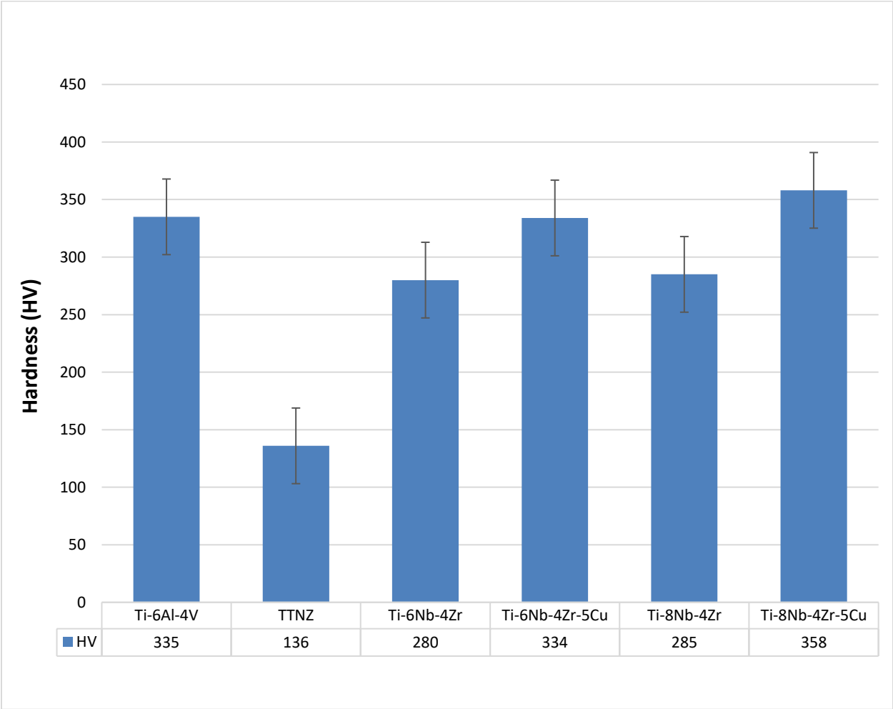
Figure 5.13: Mean Vickers hardness of the investigated alloys.
