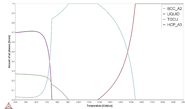
Figure 4.65: Phase proportion diagram for Ti-6Zr-4Nb-10Cu.
