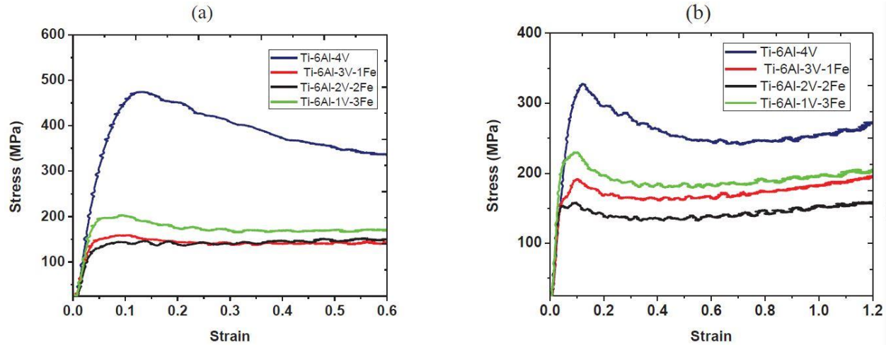
Figure 2.25: Compressive engineering stress-strain curves of as-cast Ti-6Al-xV-yFe at a strain of (a) 0.6 and (b) 1.2, from a Gleeble 3500 ® (Bodunrin et al., 2017).
