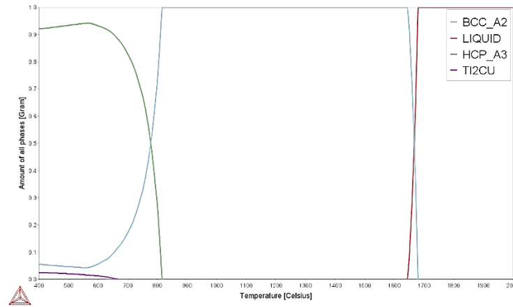
Figure 4.37: Phase proportion diagram for Ti-6Ta-2Zr-1.5Mo-1Cu.
