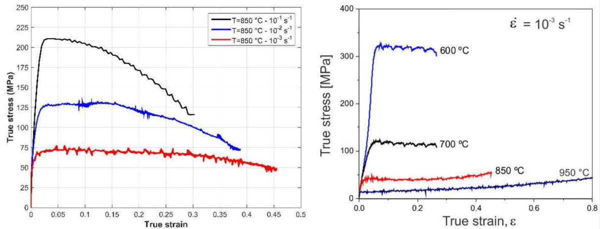
Figure 2.21: Tensile stress-strain curves of Ti-6Al-4V at 600-950°C and 10^{-1} - 10^{-3} \text{ s}^{-1} strain rate from a Gleeble 3800® (Dos Santos, 2017).
