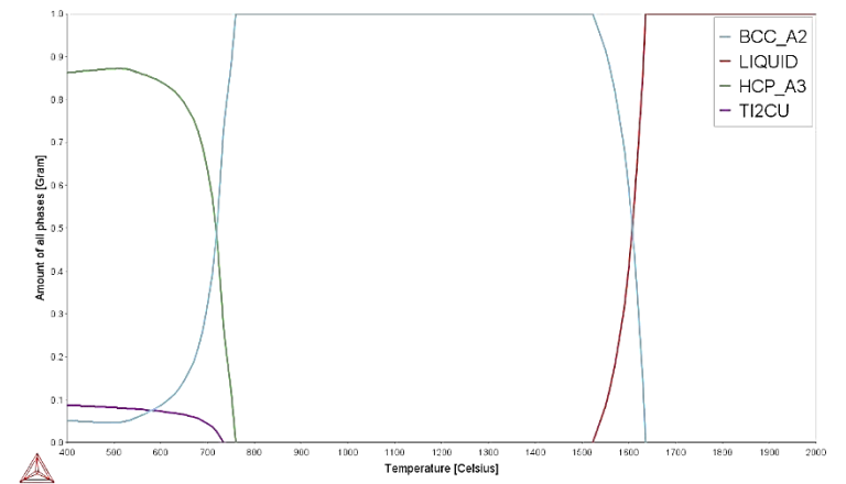
Figure 4.46: Phase proportion diagram for Ti-8Zr-4Ta-2Mo. Figure 4.47: Phase proportion diagram for Ti-8Zr-4Ta-2Mo-1Cu. Figure 4.48: Phase proportion diagram for Ti-8Zr-4Ta-2Mo-3Cu.
