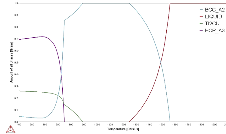
Figure 4.55: Phase proportion diagram for Ti-3.5Ta-3Nb-3Zr-10Cu.
