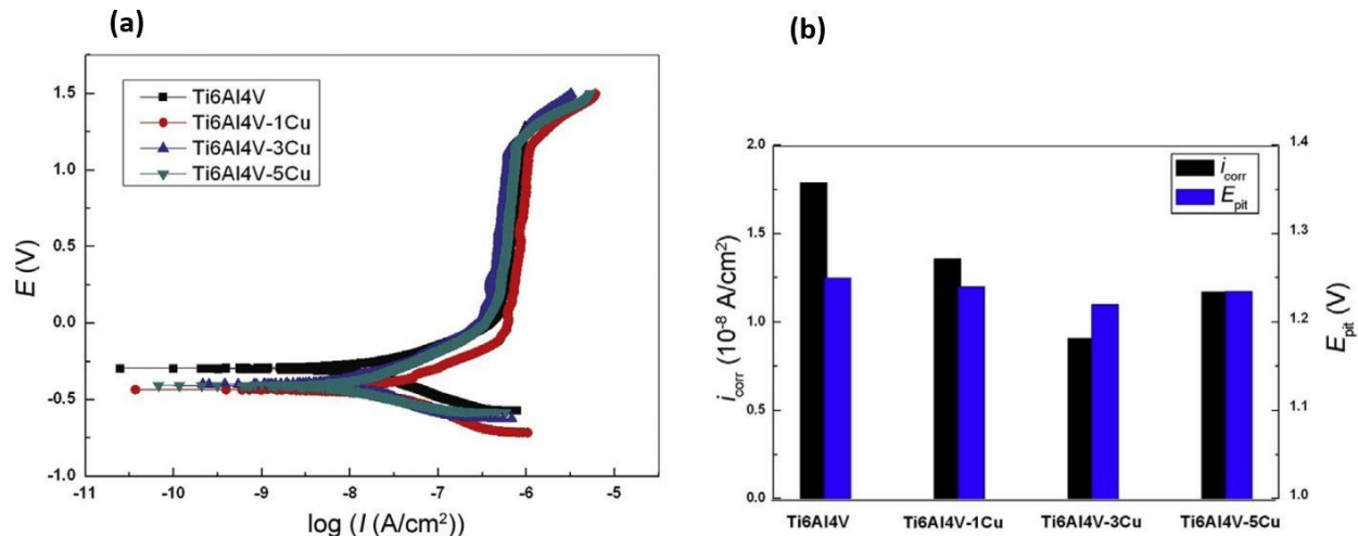
Figure 2.18: Corrosion studies of Ti-6Al-4V-xCu: (a) Potential polarisation and (b) Electrochemical corrosion currents and pitting potentials (Ren et al., 2014).
