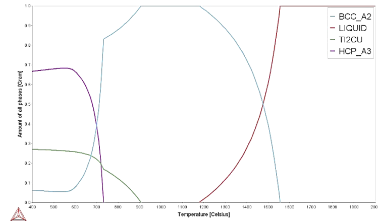
Figure 4.30: Phase proportion diagram for Ti-6Zr-4Ta-4Nb-10Cu.
