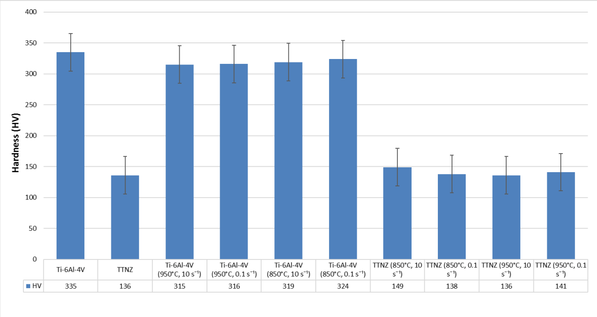
Figure 5.31: Mean Vickers hardness of the as-received and deformed Ti-6Al-4V and Ti-10.1Ta-1.7Nb-1.6Zr alloys.
