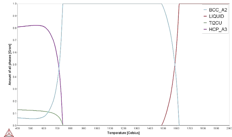
Figure 4.24: Phase proportion diagram for Ti-6Nb-2Zr-1.7Ta-5Cu. Figure 4.25: Phase proportion diagram for Ti-6Nb-2Zr-1.7Ta-10Cu.
