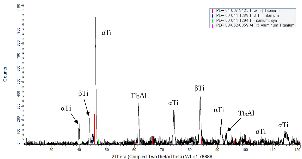
Figure 5.17: XRD analysis of the as-received Ti-6Al-4V deformed at 950°C and 0.1 s -1 strain rate, showing \alpha Ti and \beta Ti peaks shifted by alloying.
