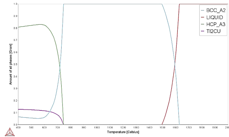
Figure 4.59: Phase proportion diagram for Ti-4.5Nb-4Ta-1.5Zr-5Cu.
