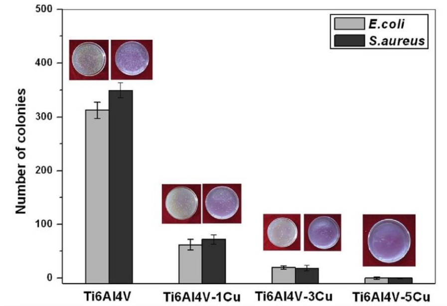
Figure 2.11: Numbers of bacterial colonies after co-culturing with Ti-6Al-4V-xCu alloys (Ren et al., 2014).
