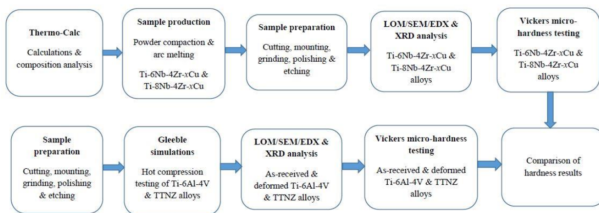
Figure 3.1: Flow diagram showing the experimental procedure for the project.
