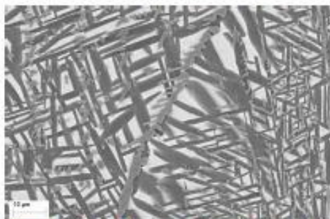
Figure 3. SEM-BSE image of TTNZ + 10 wt% Cu: light ( \beta Ti), dark ( \alpha Ti) and medium contrast Ti 2 Cu.
