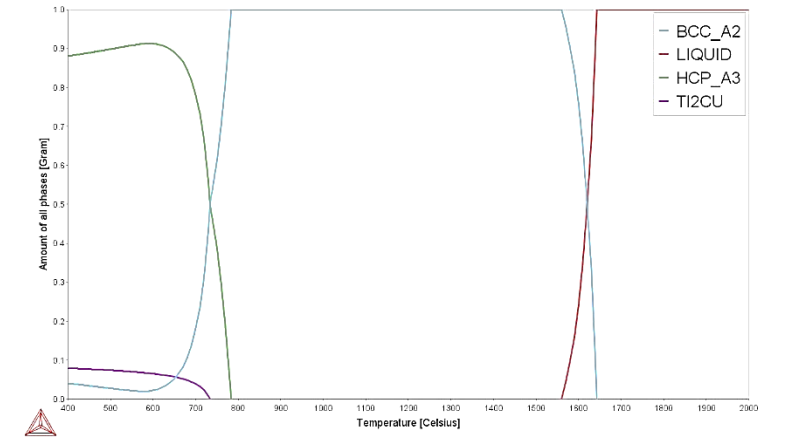
Figure 4.53: Phase proportion diagram for Ti-3.5Ta-3Nb-3Zr-3Cu.
