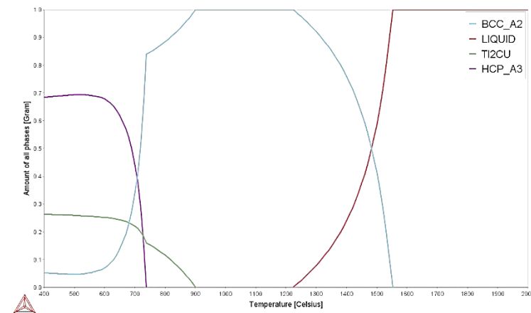
Figure 4.15: Phase proportion diagram for Ti-6Nb-4Zr-10Cu.
