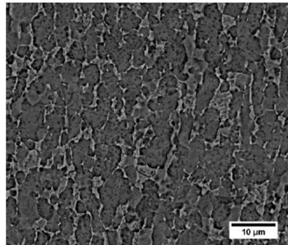
Figure 2.23: Microstructures of deformed Ti-6Al-4V at 700°C and 850°C for 10^{-3} \text{ s}^{-1} strain rate (dark phase is \alpha and light is \beta ) (Dos Santos, 2017).
