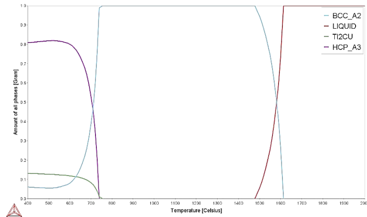
Figure 4.19: Phase proportion diagram for Ti-8Nb-4Zr-5Cu.
