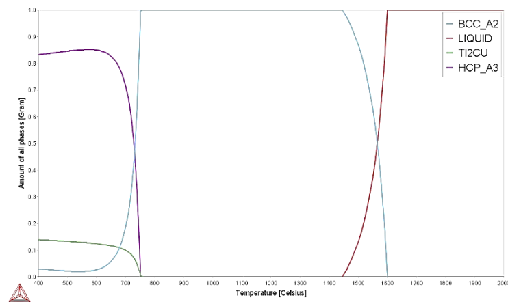
Figure 4.64: Phase proportion diagram for Ti-6Zr-4Nb-5Cu.
