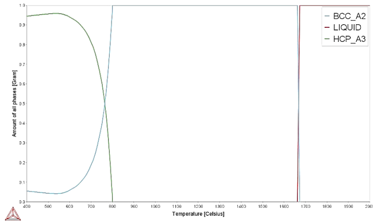
Figure 4.26: Phase proportion diagram for Ti-6Zr-4Ta-4Nb.
