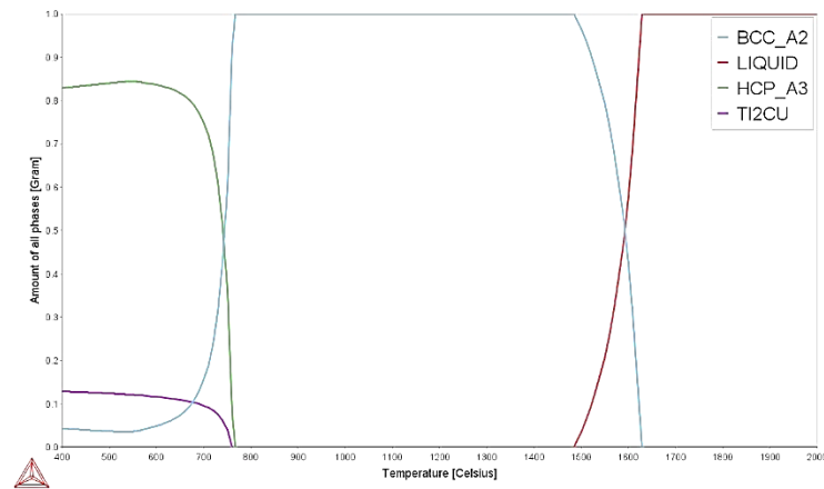
Figure 4.34: Phase proportion diagram for Ti-4Ta-1.8Zr-1.5Mo-5Cu.
