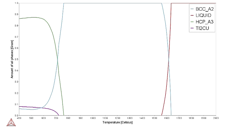
Figure 4.18: Phase proportion diagram for Ti-8Nb-4Zr-3Cu.
