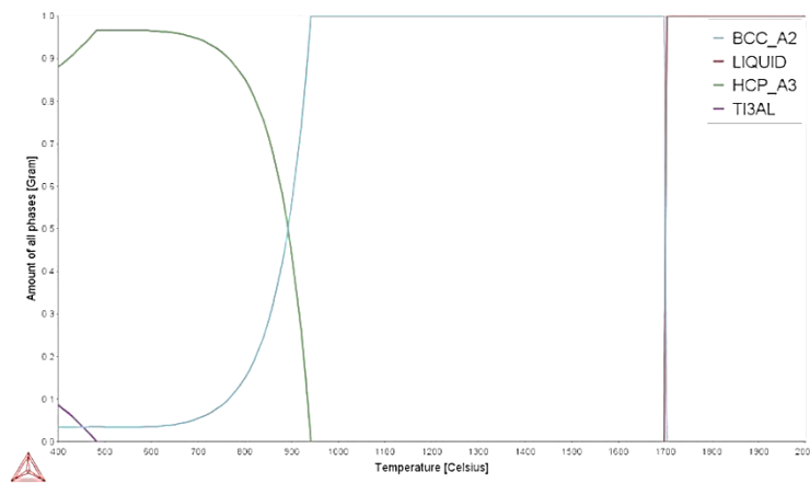
Figure 4.1: Phase proportion diagram for Ti-6Al-4V (wt%).
