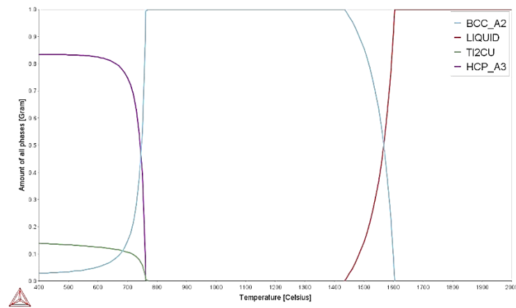
Figure 4.69: Phase proportion diagram for Ti-6Zr-2Mo-5Cu.
