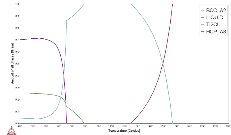
Figure 4.35: Phase proportion diagram for Ti-4Ta-1.8Zr-1.5Mo-10Cu.
