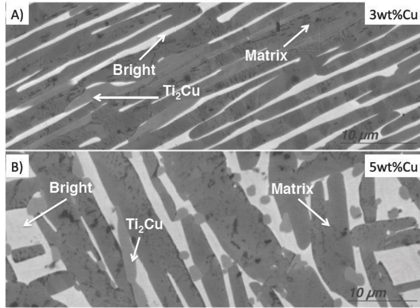
Figure 2.15: Microstructures of: (A) Ti-10.1Ta-1.7Nb-1.6Zr-3Cu and (B) Ti-10.1Ta-1.7Nb-1.6Zr-5Cu (wt%) showing Ti_2Cu (Fowler et al., 2019d).
