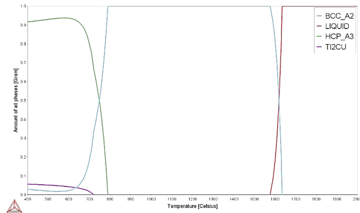
Figure 4.62: Phase proportion diagram for Ti-6Zr-4Nb-1Cu.
