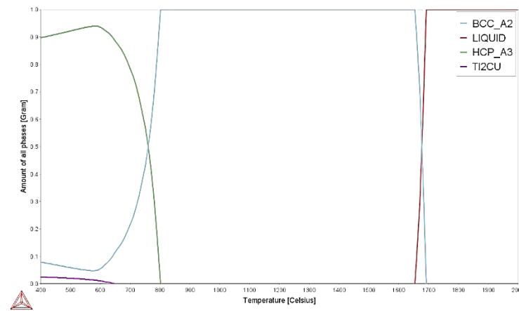
Figure 4.6: Phase proportion diagram for Ti-10.1Ta-1.7Nb-1.6Zr. Figure 4.7: Phase proportion diagram for Ti-10.1Ta-1.7Nb-1.6Zr-1Cu. Figure 4.8: Phase proportion diagram for Ti-10.1Ta-1.7Nb-1.6Zr-3Cu.
