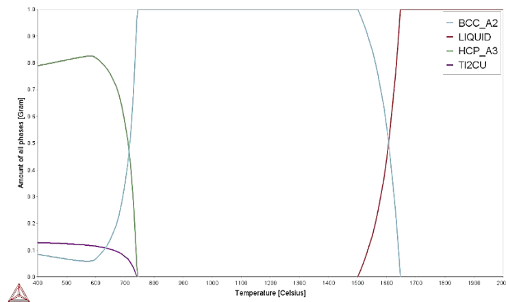
Figure 4.9: Phase proportion diagram for Ti-10.1Ta-1.7Nb-1.6Zr-5Cu.
