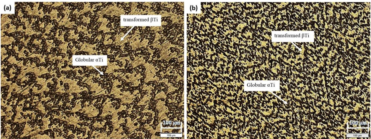
Figure 5.22: Optical micrographs of as-received Ti-10.1Ta-1.7Nb-1.6Zr deformed at 0.1 s -1 strain rate: (a) 850°C and (b) 950°C.
