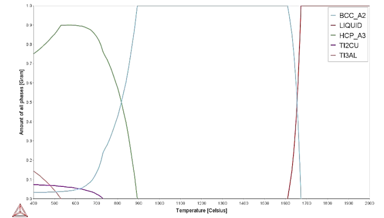
Figure 4.3: Phase proportion diagram for Ti-6Al-4V-3Cu (wt%).
