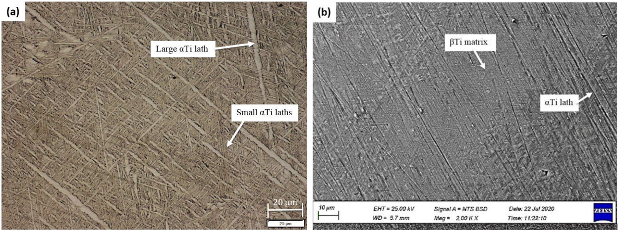
Figure 5.5: As-cast Ti-6Nb-4Zr (wt%): (a) Optical micrograph and (b) SEM-BSE image.
