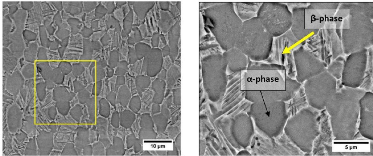
Figure 2.24: Microstructures of deformed Ti-6Al-4V at 950°C for 10^{-3} \text{ s}^{-1} strain rate (Dos Santos, 2017).
