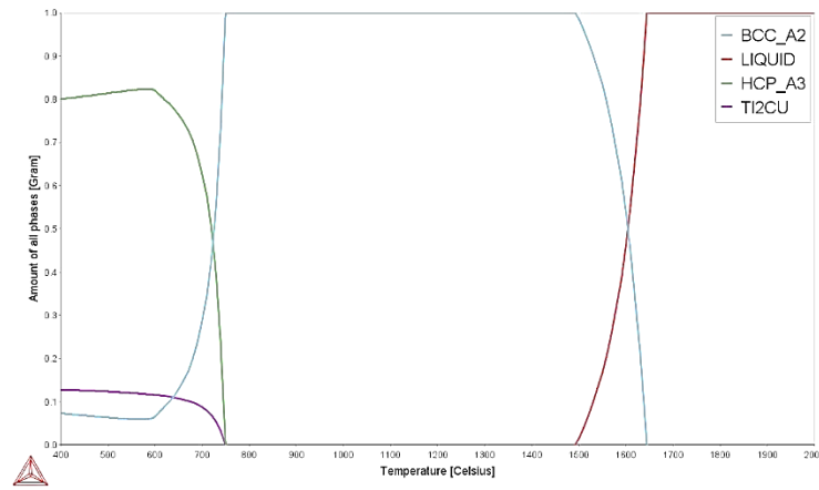
Figure 4.44: Phase proportion diagram for Ti-8Ta-1.5Mo-1.5Zr-5Cu. Figure 4.45: Phase proportion diagram for Ti-8Ta-1.5Mo-1.5Zr-10Cu.
