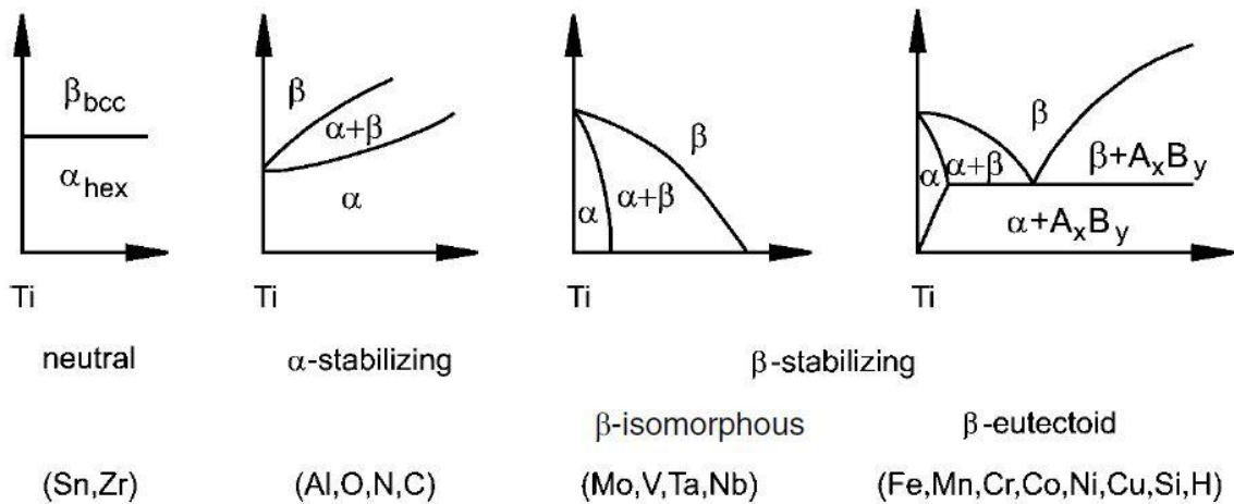
Figure 2.2: Schematic Ti phase diagrams showing the effects of selected alloying elements (Leyens & Peters, 2003).
