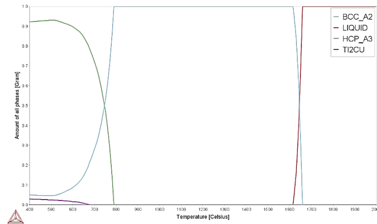
Figure 4.46: Phase proportion diagram for Ti-8Zr-4Ta-2Mo. Figure 4.47: Phase proportion diagram for Ti-8Zr-4Ta-2Mo-1Cu. Figure 4.48: Phase proportion diagram for Ti-8Zr-4Ta-2Mo-3Cu.
