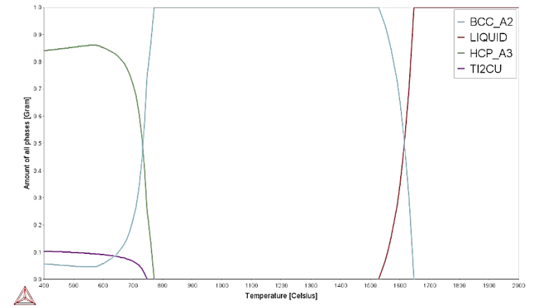
Figure 4.38: Phase proportion diagram for Ti-6Ta-2Zr-1.5Mo-3Cu.
