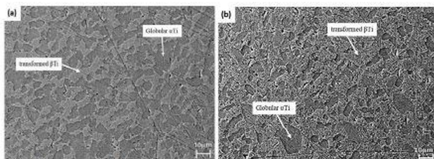
Figure 8: SEM-BSE images of Ti-6Al-4V deformed at 0.1 s -1 strain rate at: (a) 850 °C and (b) 950 °C, showing βTi matrix (light contrast) and αTi globules (dark contrast)
