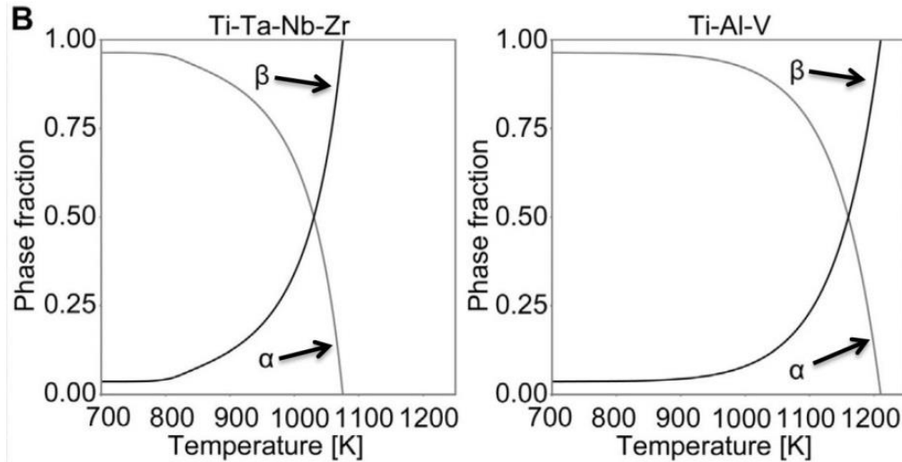
Figure 2.8: Phase proportion diagrams for Ti-10.1Ta-1.7Nb-1.6Zr and Ti-6Al-4V (wt%) (Stenlund et al., 2015).
