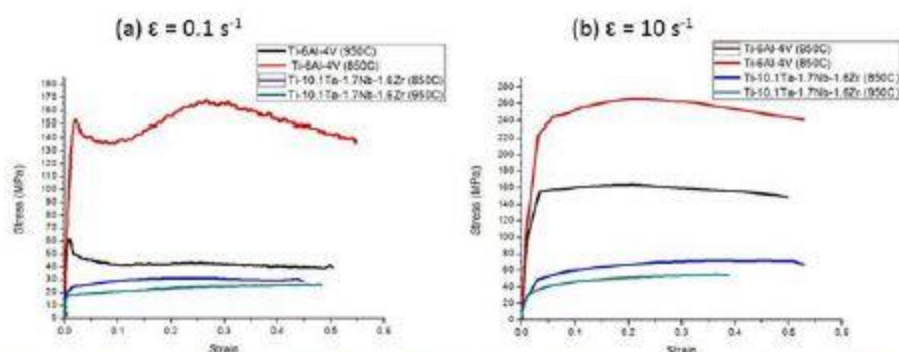
Figure 7: Stress-strain curves of the as-received Ti-6Al-4V and Ti-10.1Ta-1.7Nb-1.6Zr (wt%) alloys deformed at 850 °C and 950 °C, at: (a) 0.1 s -1 and (b) 10 s -1 strain rates
