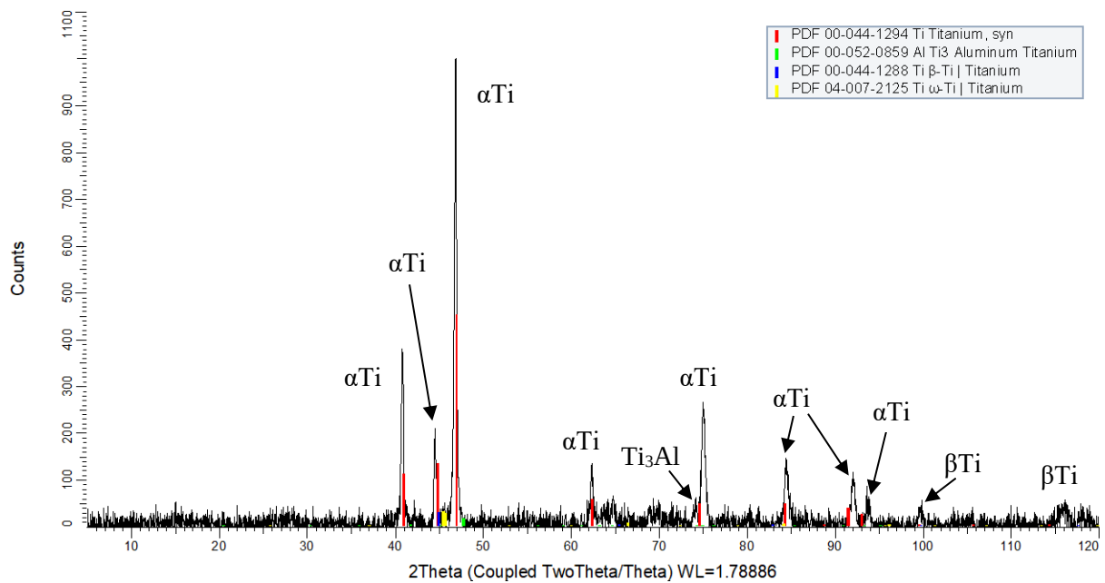
Figure 5.20: XRD analysis of the as-received Ti-6Al-4V deformed at 850°C and 10 s -1 strain rate, showing \alpha Ti and \beta Ti peaks shifted by alloying.
