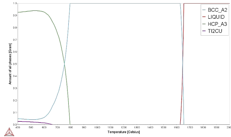
Figure 4.12: Phase proportion diagram for Ti-6Nb-4Zr-1Cu.
