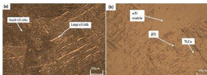
Figure 3: Optical micrographs of as-cast: (a) Ti-8Nb-4Zr showing clusters of \alpha Ti laths within prior \beta Ti grains and (b) Ti-8Nb-4Zr-5Cu (wt%) showing \beta Ti, \alpha Ti and \text{Ti}_3\text{Cu} phases
