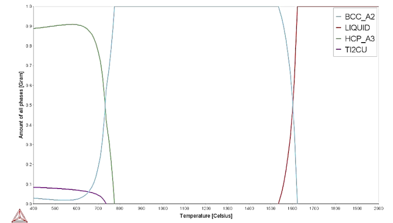
Figure 4.63: Phase proportion diagram for Ti-6Zr-4Nb-3Cu.
