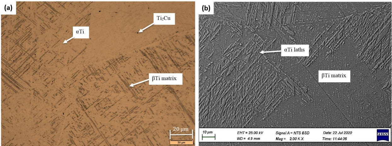
Figure 5.10: As-cast Ti-8Nb-4Zr-5Cu (wt%): (a) Optical micrograph and (b) SEM-BSE image.
