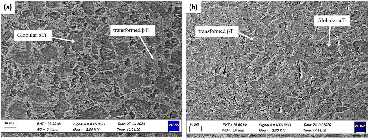
Figure 5.19: SEM-BSE images of as-received Ti-6Al-4V deformed at 10\text{ s}^{-1} strain rate: (a) 850°C and (b) 950°C.
