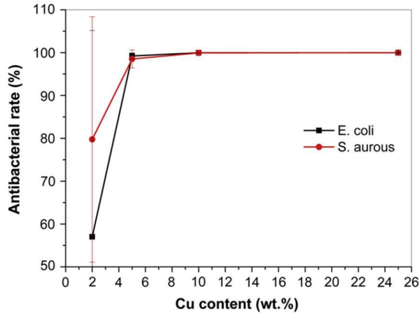
Figure 2.12: Antibacterial rate of Ti-Cu alloys against E. coli and S. aureus at different Cu content (Liu et al., 2014a).
