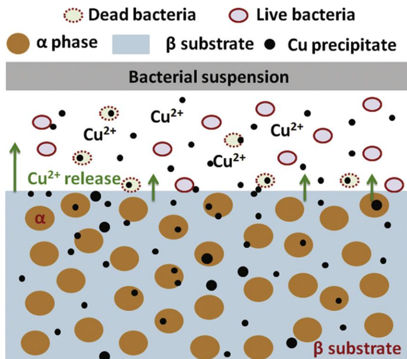
Figure 2.13: Schematic illustration of the antibacterial mechanism of Ti-Cu alloys (Ma et al., 2015).
