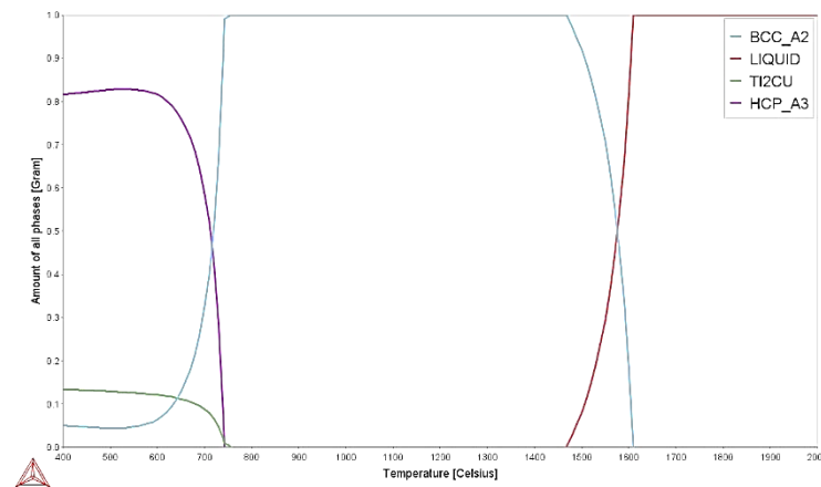
Figure 4.14: Phase proportion diagram for Ti-6Nb-4Zr-5Cu.
