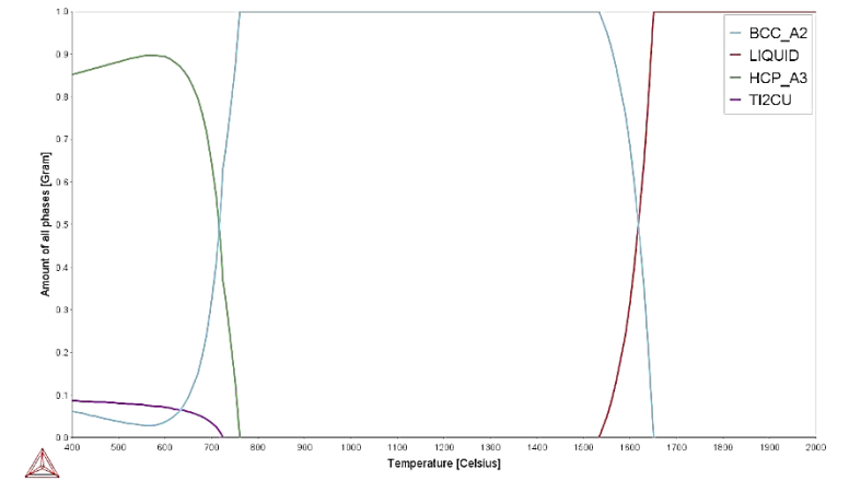
Figure 4.73: Phase proportion diagram for Ti-10Ta-8Zr-3Cu.
