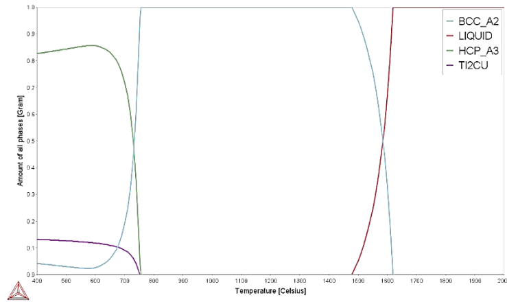
Figure 4.54: Phase proportion diagram for Ti-3.5Ta-3Nb-3Zr-5Cu.
