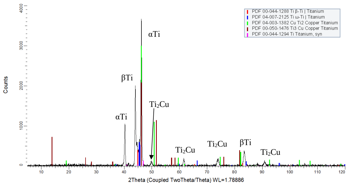
Figure 5.12: XRD analysis of the as-cast Ti-8Nb-4Zr-5Cu (wt%) alloy, showing \alpha Ti, and small \beta Ti peaks shifted by alloying and Ti_2Cu .
