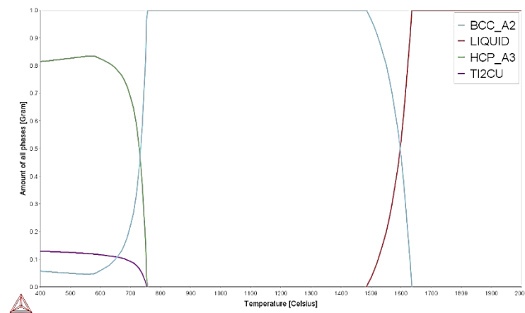
Figure 4.39: Phase proportion diagram for Ti-6Ta-2Zr-1.5Mo-5Cu.
