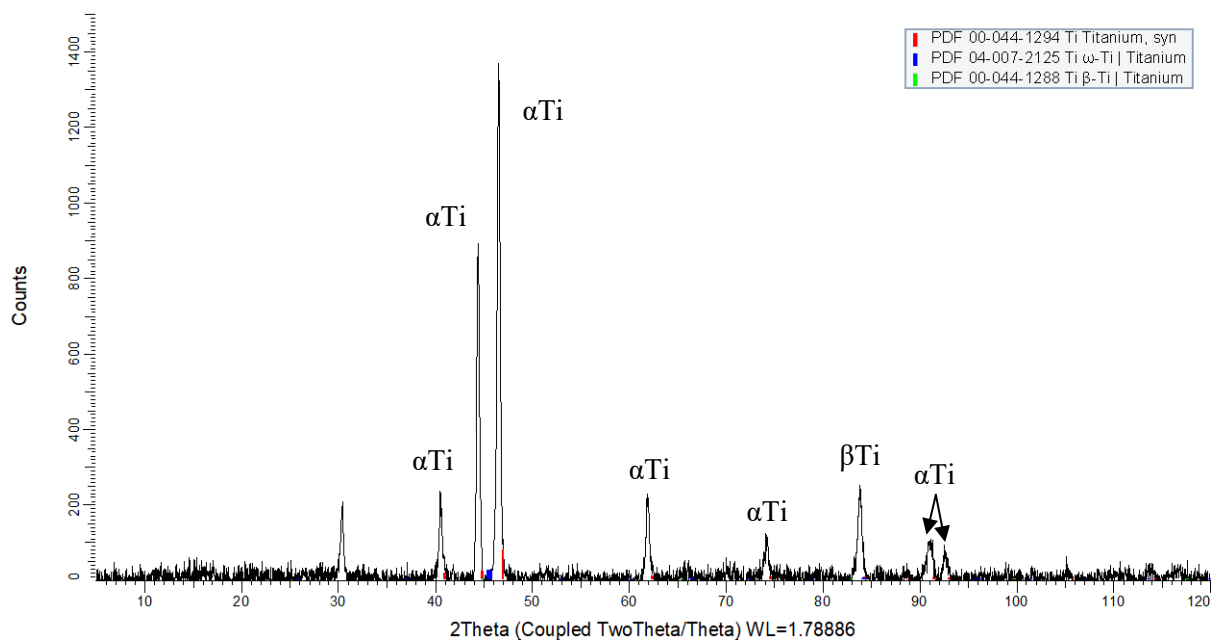
Figure 5.24: XRD analysis of the as-received Ti-10.1Ta-1.7Nb-1.6Zr deformed at 850°C and 0.1 s -1 strain rate, showing mainly αTi with βTi peaks, shifted by alloying.
