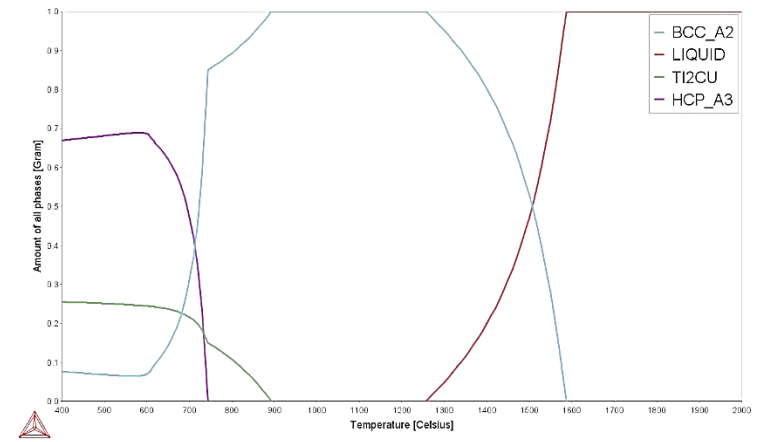
Figure 4.44: Phase proportion diagram for Ti-8Ta-1.5Mo-1.5Zr-5Cu. Figure 4.45: Phase proportion diagram for Ti-8Ta-1.5Mo-1.5Zr-10Cu.
