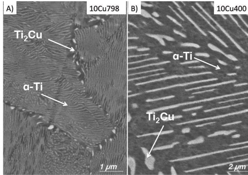
Figure 2.14: Microstructures of Ti-10Cu (wt%): (A) after rapid quenching from 798^\circ\text{C} and (B) after ageing at 400^\circ\text{C} (Fowler et al., 2019b).
