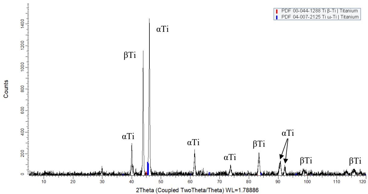
Figure 5.28: XRD analysis of the as-received Ti-10.1Ta-1.7Nb-1.6Zr deformed at 850°C and 10 s -1 strain rate, showing mainly αTi with βTi peaks, shifted by alloying.
