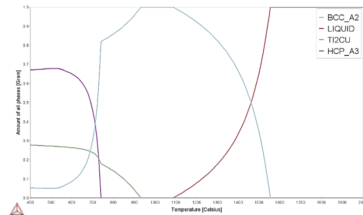
Figure 4.50: Phase proportion diagram for Ti-8Zr-4Ta-2Mo-10Cu.
