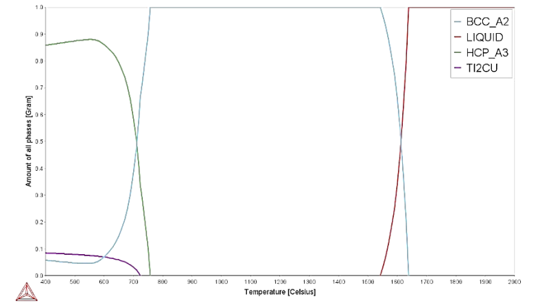
Figure 4.28: Phase proportion diagram for Ti-6Zr-4Ta-4Nb-3Cu.
