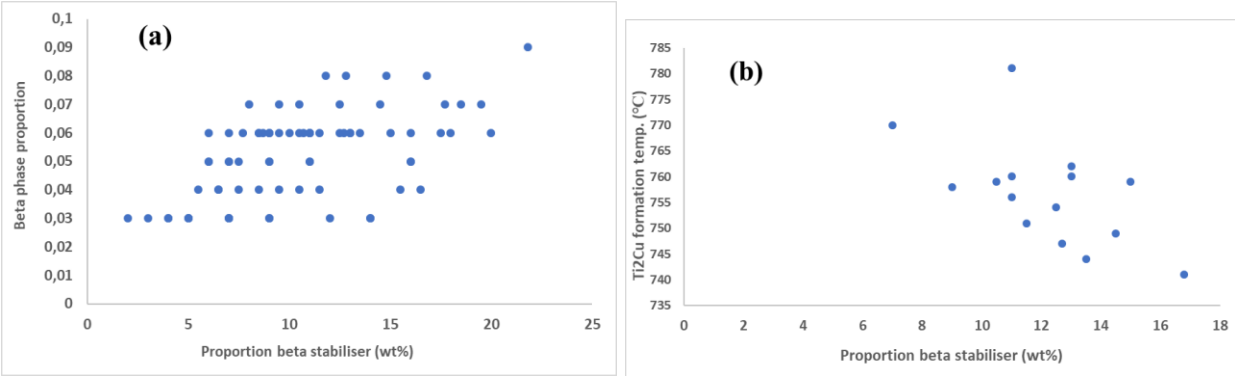
Figure 4.77: Effect of beta-stabilisers on: (a) beta phase proportions at 400°C and (b) Ti 2 Cu formation temperatures.
