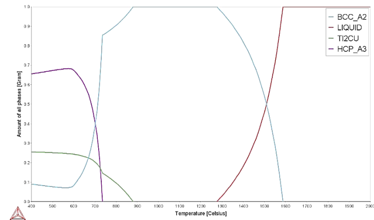
Figure 4.10: Phase proportion diagram for Ti-10.1Ta-1.7Nb-1.6Zr-10Cu.
