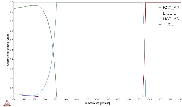
Figure 4.52: Phase proportion diagram for Ti-3.5Ta-3Nb-3Zr-1Cu.
