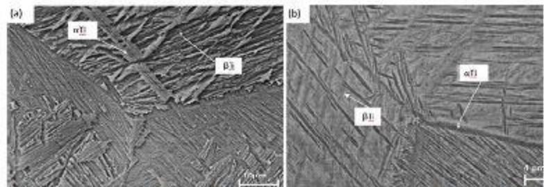
Figure 5: SEM-BSE images of as-cast: (a) Ti-6Ta-1.5Zr-0.2Ru (wt%) showing light contrast plate-like αTi, and (b) Ti-6Ta-1.5Zr-0.2Ru-5Cu showing parallel αTi laths growing from prior βTi grain boundaries
