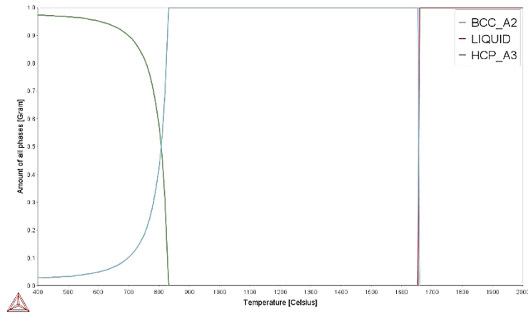
Figure 4.66: Phase proportion diagram for Ti-6Zr-2Mo.
