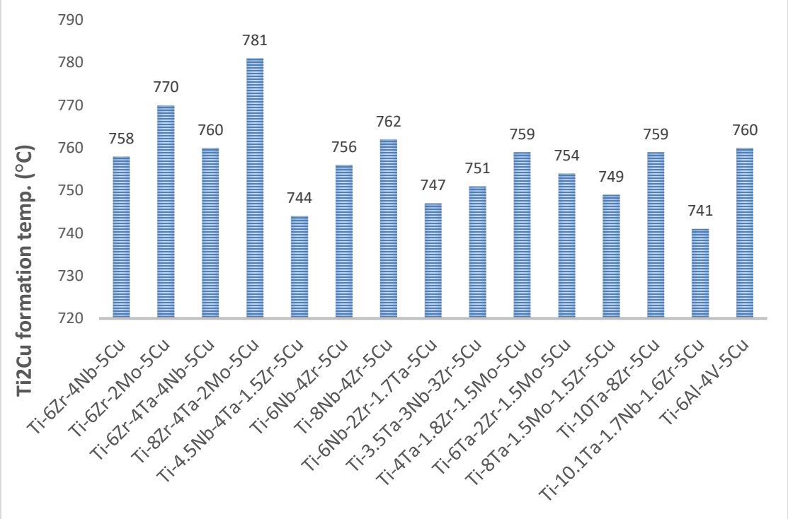
Figure 4.76: Ti 2 Cu formation temperatures of the different titanium compositions.
