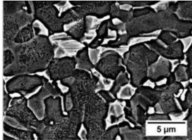
Figure 2.22: Starting microstructure of Ti-6Al-4V (dark phase is \alpha and light is \beta ) (Dos Santos, 2017).
