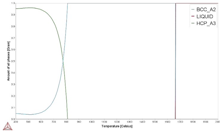
Figure 4.11: Phase proportion diagram for Ti-6Nb-4Zr.
