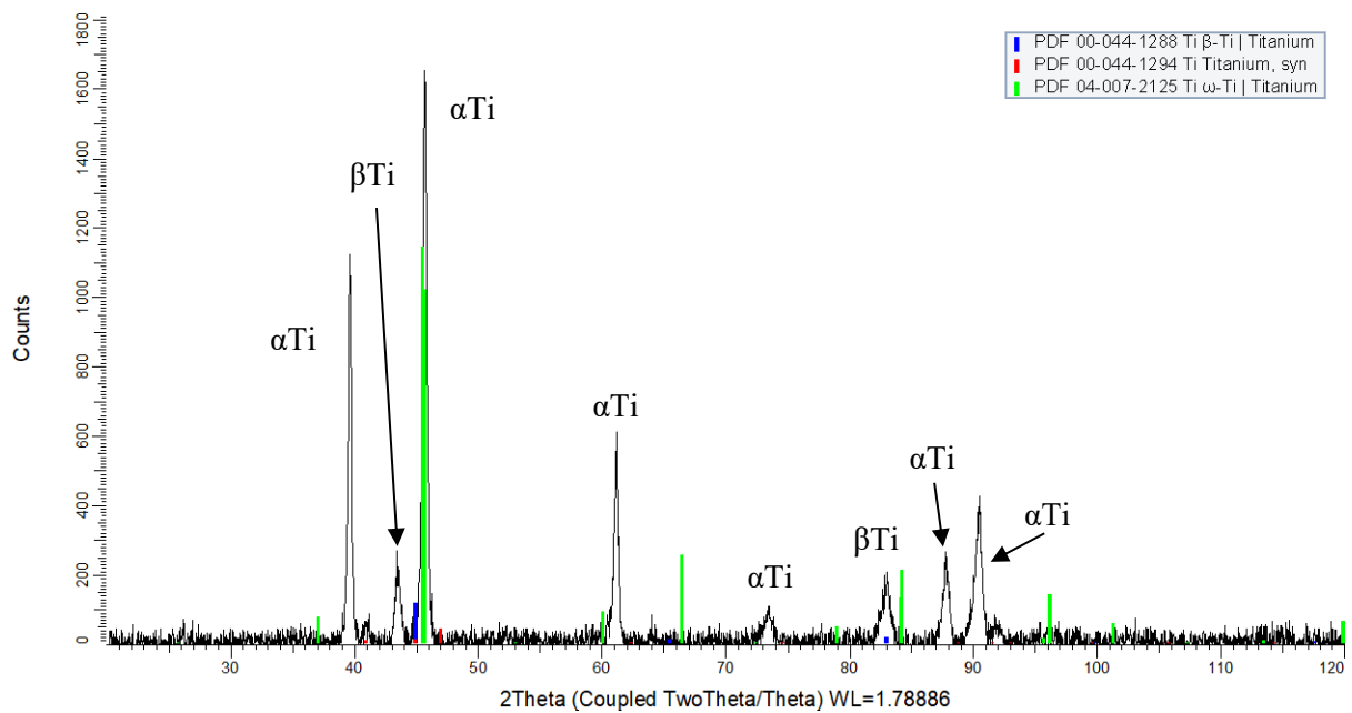
Figure 5.11: XRD analysis of the as-cast Ti-8Nb-4Zr (wt%) alloy, showing peaks for \alpha Ti, and small peaks for \beta Ti shifted by alloying.
