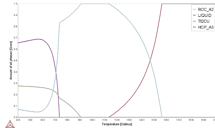
Figure 4.75: Phase proportion diagram for Ti-10Ta-8Zr-10Cu.
