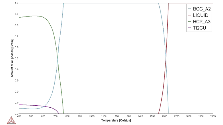
Figure 4.13: Phase proportion diagram for Ti-6Nb-4Zr-3Cu.
