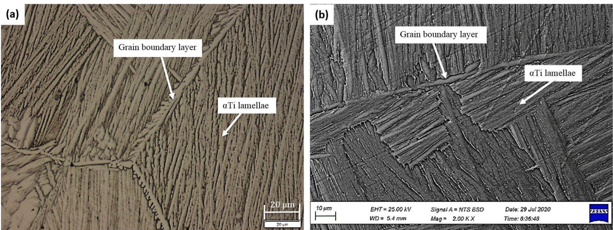
Figure 5.1: As-received Ti-6Al-4V (wt%): (a) Optical micrograph and (b) SEM-BSE image.
