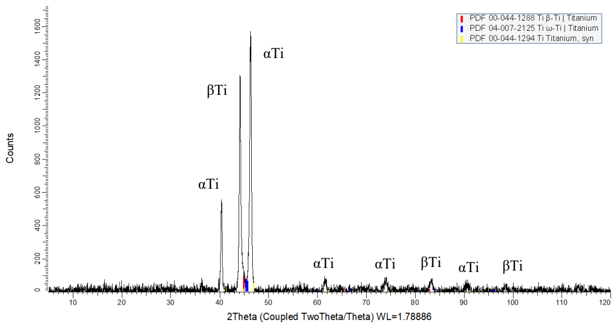
Figure 5.7: XRD analysis of the as-cast Ti-6Nb-4Zr (wt%) alloy, showing mainly shifted \alpha Ti peaks due to alloying.
