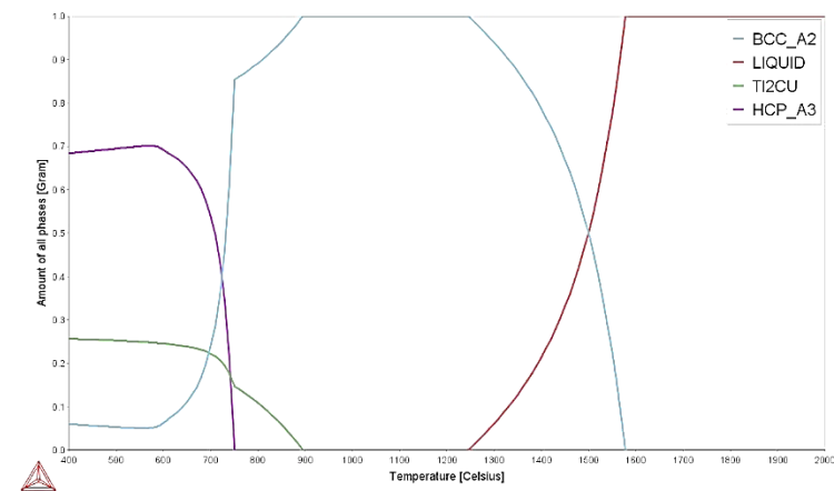
Figure 4.40: Phase proportion diagram for Ti-6Ta-2Zr-1.5Mo-10Cu.
