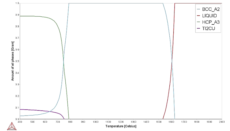
Figure 4.68: Phase proportion diagram for Ti-6Zr-2Mo-3Cu.
