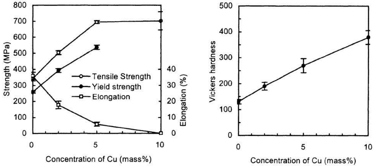
Figure 2.16: Mechanical properties of cast Ti-xCu ( x = 2, 5 and 10 wt%) alloys (Takahashi et al., 2002).
