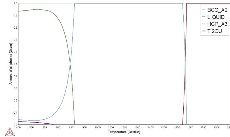
Figure 4.31: Phase proportion diagram for Ti-4Ta-1.8Zr-1.5Mo. Figure 4.32: Phase proportion diagram for Ti-4Ta-1.8Zr-1.5Mo-1Cu. Figure 4.33: Phase proportion diagram for Ti-4Ta-1.8Zr-1.5Mo-3Cu.
