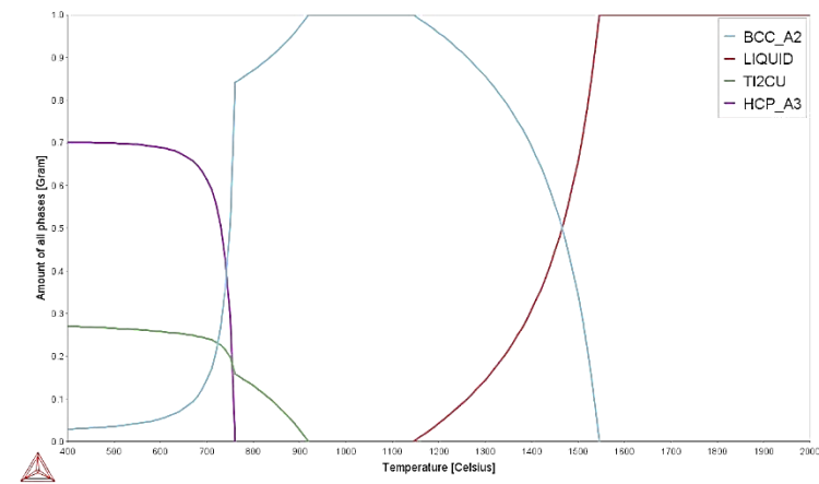
Figure 4.70: Phase proportion diagram for Ti-6Zr-2Mo-10Cu.
