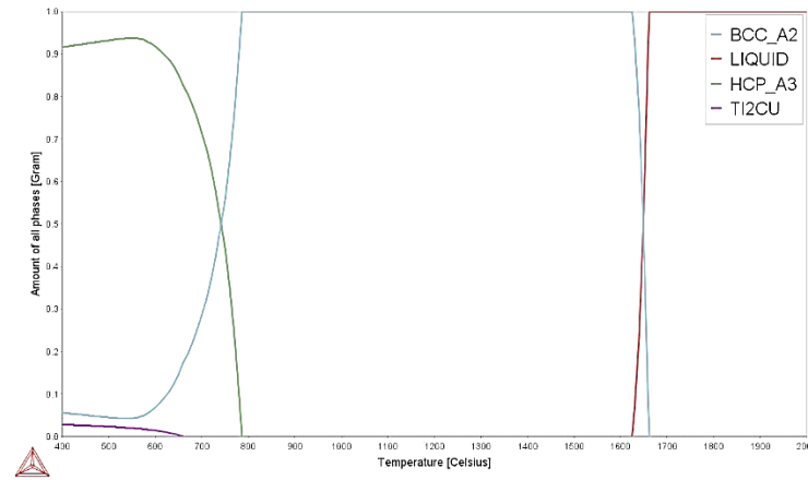
Figure 4.27: Phase proportion diagram for Ti-6Zr-4Ta-4Nb-1Cu.
