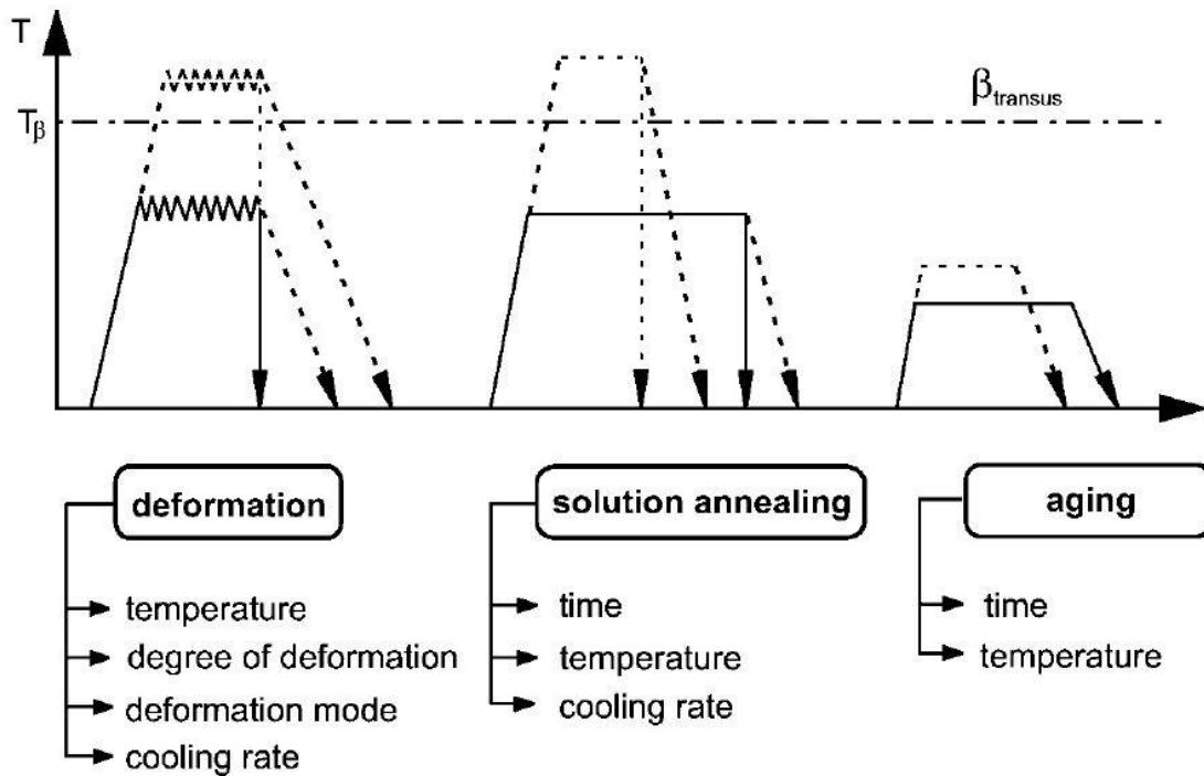
Figure 2.5: Schematic diagram showing thermomechanical treatment of titanium alloys (Leyens & Peters, 2003).
