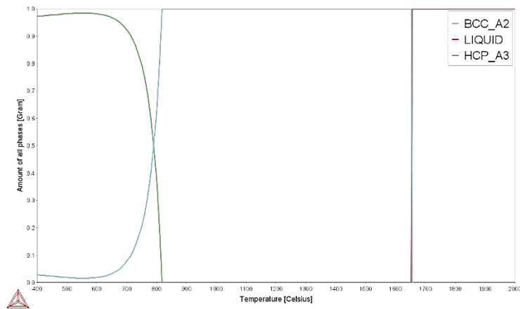
Figure 4.61: Phase proportion diagram for Ti-6Zr-4Nb.
