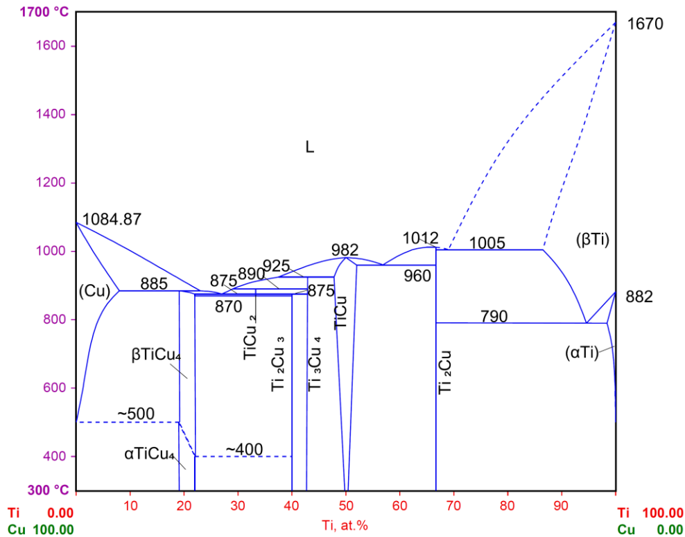
Figure 2.10: Assessed phase diagram of the Cu-Ti binary system, showing congruent formation of Ti_2Cu without Ti_3Cu (Ansara et al., 2021).
