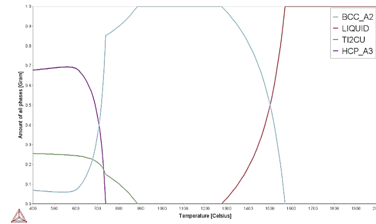
Figure 4.60: Phase proportion diagram for Ti-4.5Nb-4Ta-1.5Zr-10Cu.
