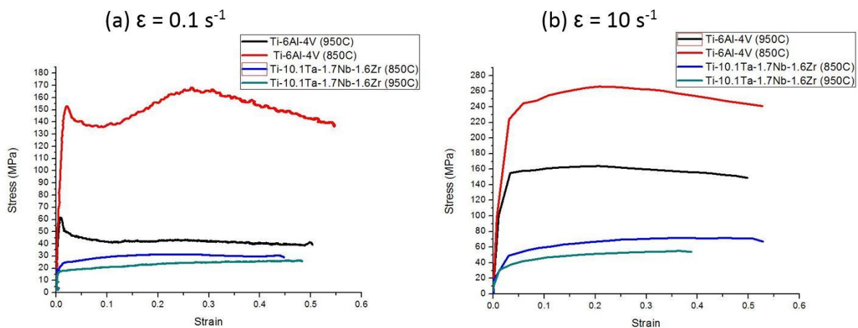
Figure 5.30: Stress-strain curves of the as-received Ti-6Al-4V and Ti-10.1Ta-1.7Nb-1.6Zr (wt%) alloys deformed at 850°C and 950°C, and (a) 0.1 s -1 and (b) 10 s -1 strain rates.
