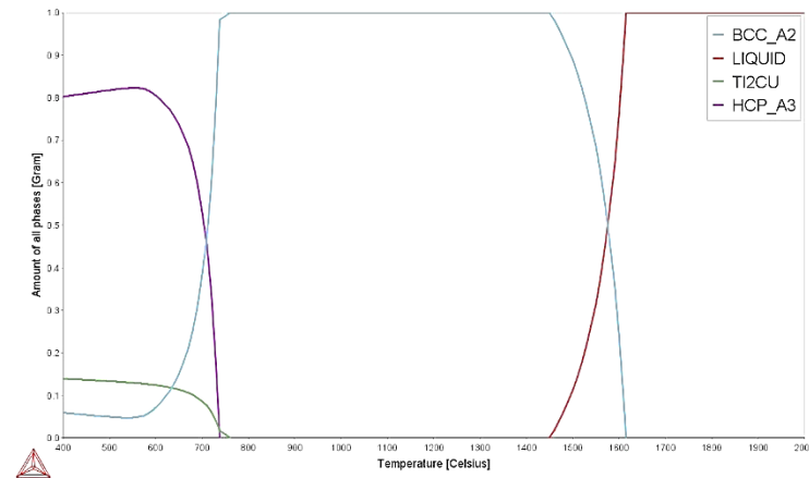
Figure 4.29: Phase proportion diagram for Ti-6Zr-4Ta-4Nb-5Cu.
