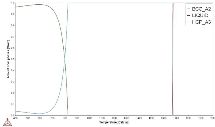
Figure 4.51: Phase proportion diagram for Ti-3.5Ta-3Nb-3Zr.
