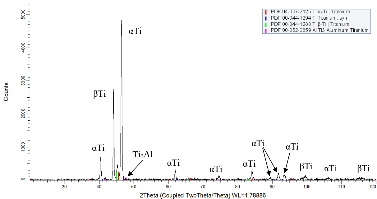
Figure 5.21: XRD analysis of the as-received Ti-6Al-4V deformed at 950°C and 10 s -1 strain rate, showing \alpha Ti and \beta Ti peaks shifted by alloying.
