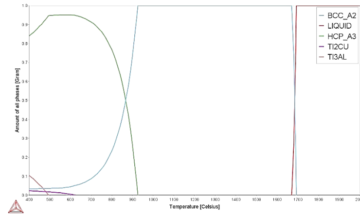
Figure 4.2: Phase proportion diagram for Ti-6Al-4V-1Cu (wt%).
