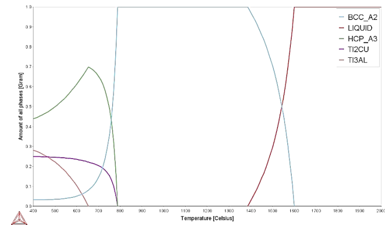
Figure 4.5: Phase proportion diagram for Ti-6Al-4V-10Cu (wt%).
