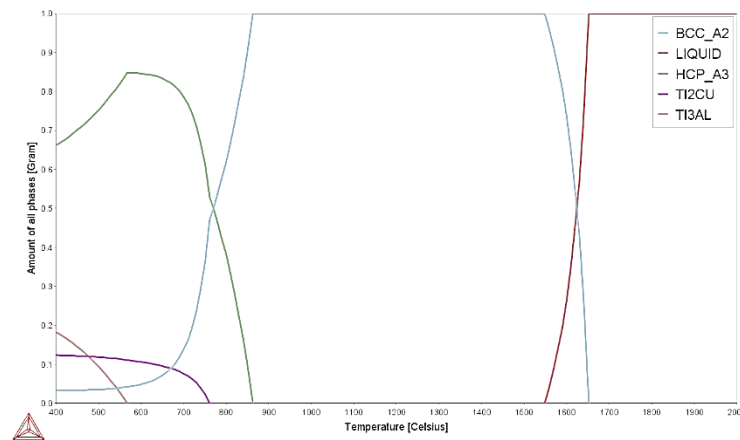
Figure 4.4: Phase proportion diagram for Ti-6Al-4V-5Cu (wt%).
