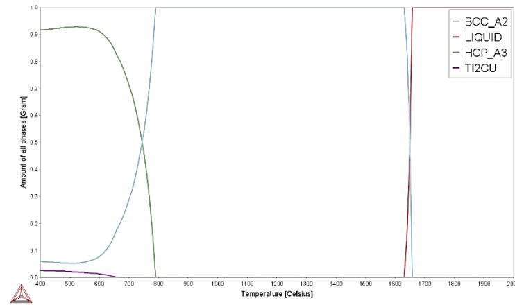
Figure 4.17: Phase proportion diagram for Ti-8Nb-4Zr-1Cu.
