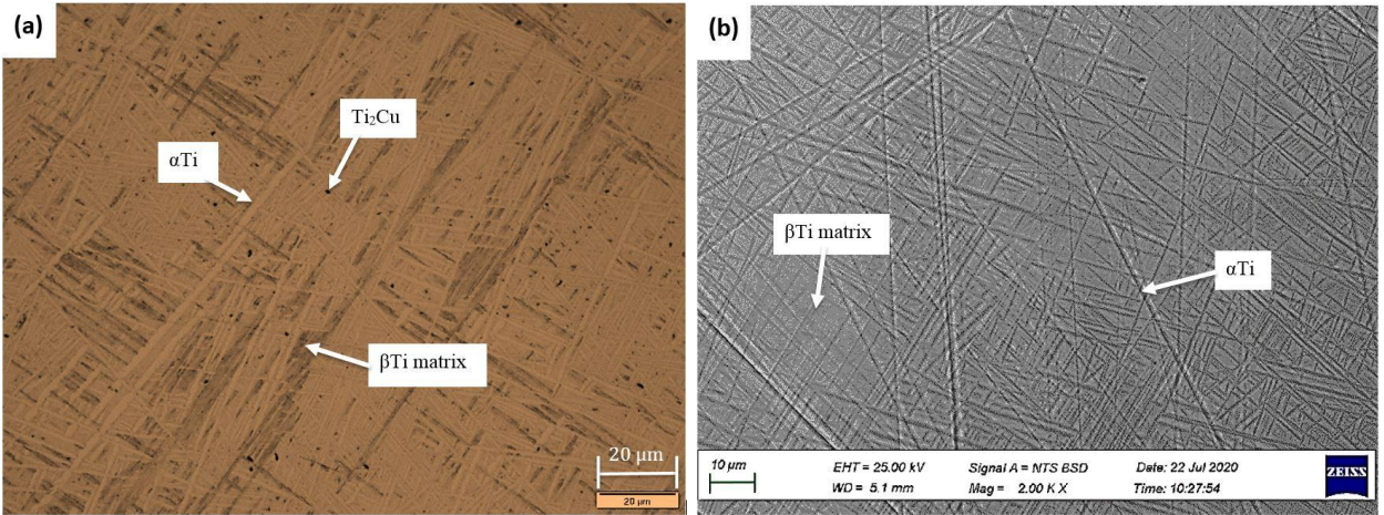
Figure 5.6: As-cast Ti-6Nb-4Zr-5Cu (wt%): (a) Optical micrograph and (b) SEM-BSE image.
