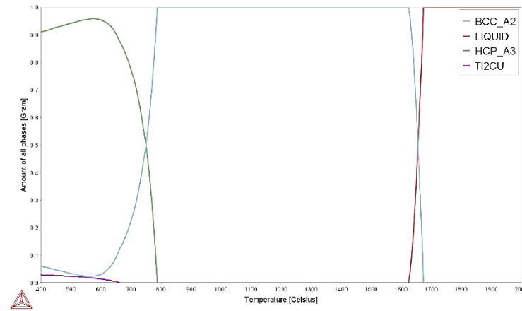
Figure 4.72: Phase proportion diagram for Ti-10Ta-8Zr-1Cu.
