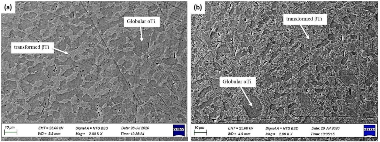
Figure 5.15: SEM-BSE images of as-received Ti-6Al-4V (wt%) deformed at 0.1 s -1 strain rate: (a) 850°C and (b) 950°C.
