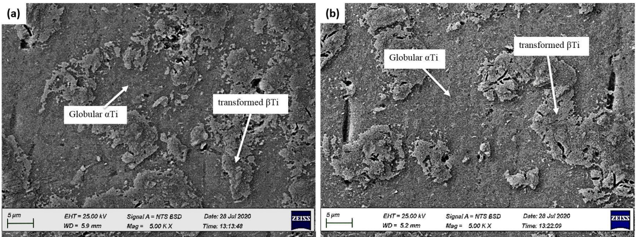
Figure 5.23: SEM-BSE images of as-received Ti-10.1Ta-1.7Nb-1.6Zr deformed at 0.1 s -1 strain rate: (a) 850°C and (b) 950°C.
