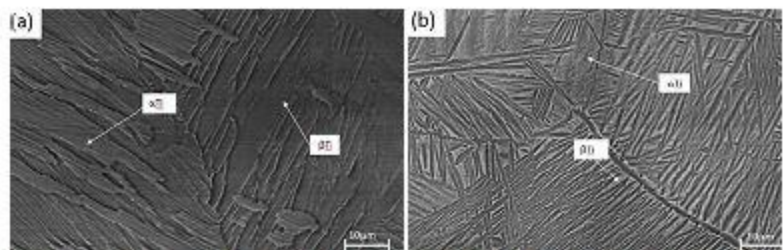
Figure 4: SEM-BSE images of as-cast: (a) Ti-6Ta-1.5Zr (wt%) and (b) Ti-6Ta-1.5Zr-5Cu showing thick and thin (αTi) lamellae, growing from prior βTi grain boundaries
