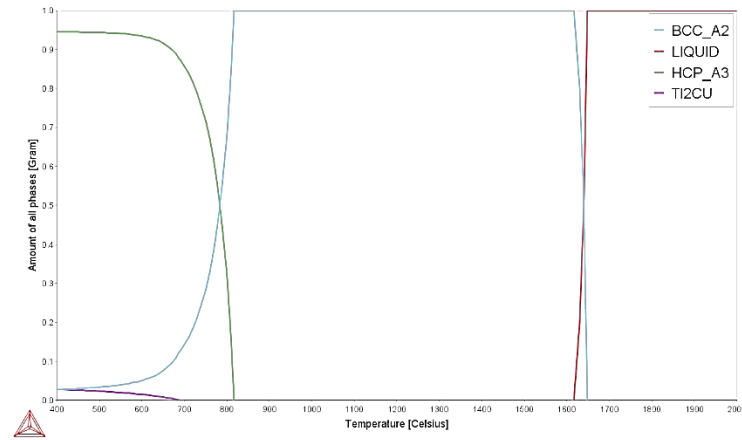
Figure 4.67: Phase proportion diagram for Ti-6Zr-2Mo-1Cu.
