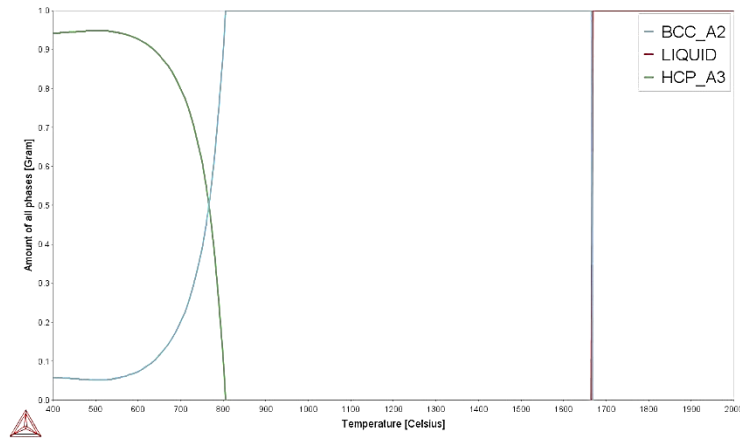
Figure 4.16: Phase proportion diagram for Ti-8Nb-4Zr.
