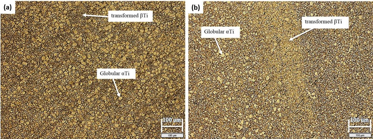
Figure 5.18: Optical micrographs of as-received Ti-6Al-4V deformed at 10\text{ s}^{-1} strain rate: (a) 850°C and (b) 950°C.
