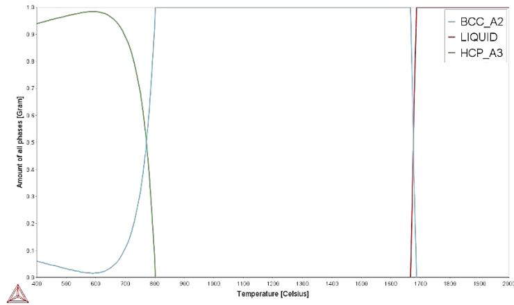
Figure 4.71: Phase proportion diagram for Ti-10Ta-8Zr.
