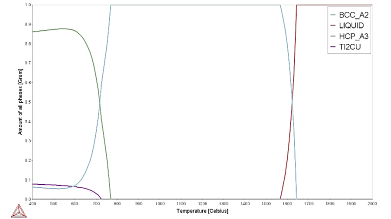
Figure 4.21: Phase proportion diagram for Ti-6Nb-2Zr-1.7Ta. Figure 4.22: Phase proportion diagram for Ti-6Nb-2Zr-1.7Ta-1Cu. Figure 4.23: Phase proportion diagram for Ti-6Nb-2Zr-1.7Ta-3Cu.
