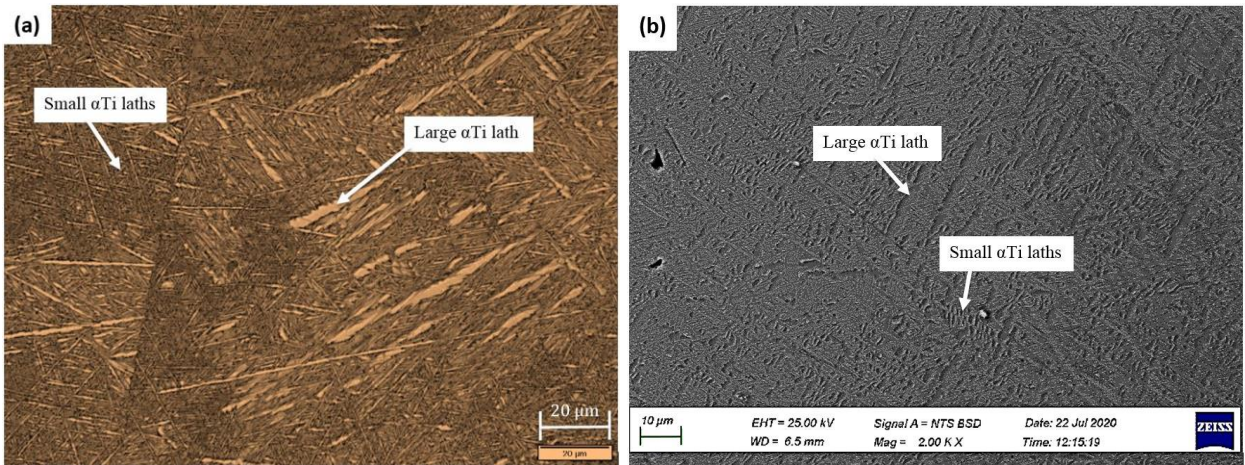
Figure 5.9: As-cast Ti-8Nb-4Zr (wt%): (a) Optical micrograph and (b) SEM-BSE image.
