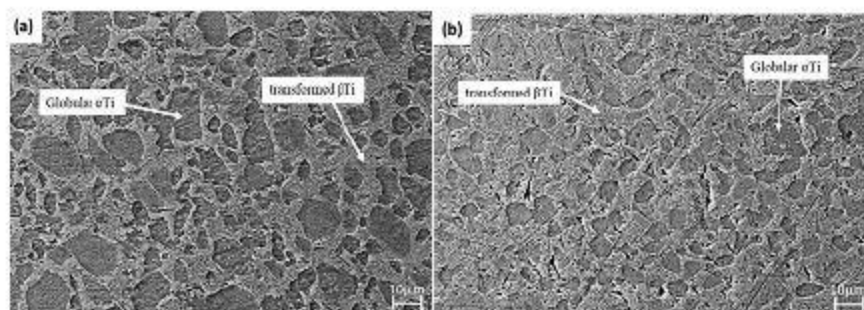
Figure 9: SEM-BSE images of Ti-6Al-4V (wt%) deformed at 10 s -1 strain rate at: (a) 850 °C and (b) 950 °C, showing βTi-matrix (light contrast) and αTi globules (dark contrast)
