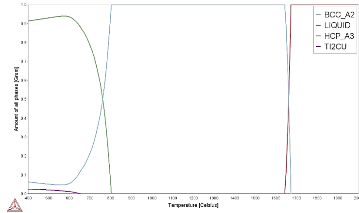
Figure 4.56: Phase proportion diagram for Ti-4.5Nb-4Ta-1.5Zr. Figure 4.57: Phase proportion diagram for Ti-4.5Nb-4Ta-1.5Zr-1Cu. Figure 4.58: Phase proportion diagram for Ti-4.5Nb-4Ta-1.5Zr-3Cu.
