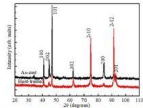
Figure 2. XRD patterns of the as-cast and heat treated Ti-Ta-Cu-Nb-Zr alloy, showing only alpha-Ti.
