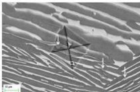
Figure 2. SEM-BSE image of TTNZ + 3 wt% Cu, showing a hardness indentation with light ( \beta Ti), dark ( \alpha Ti) and medium contrast Ti 2 Cu (shown by arrows).
