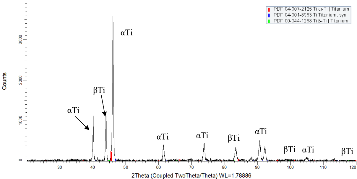
Figure 5.4: XRD analysis of the as-received Ti-10.1Ta-1.7Nb-1.6Zr (wt%) (TTNZ) alloy, showing mainly shifted \alpha Ti peaks due to the alloying.
