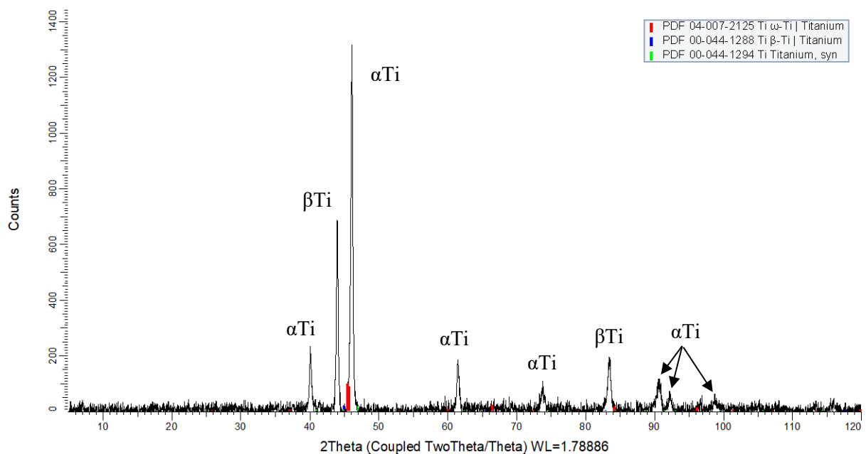
Figure 5.25: XRD analysis of the as-received Ti-10.1Ta-1.7Nb-1.6Zr deformed at 950°C and 0.1 s -1 strain rate, showing mainly αTi with βTi peaks, shifted by alloying.
