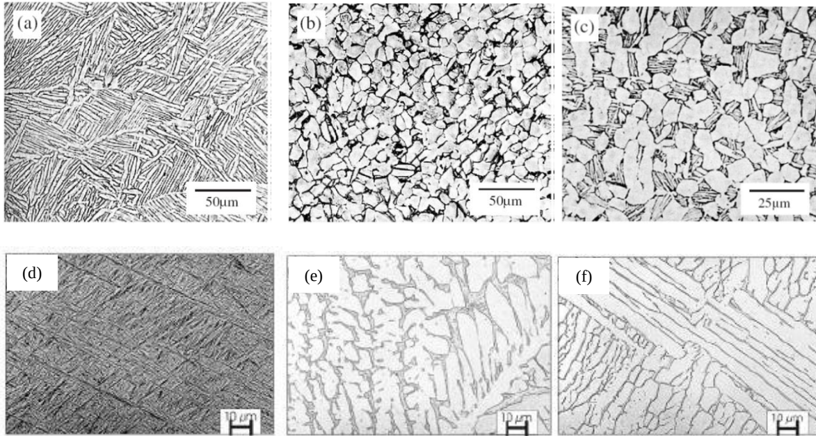
Figure 2.6: Optical micrographs showing different Ti-6Al-4V microstructures: (a) lamellar, (b) equiaxed and (c) bimodal (Rack & Qazi, 2006), and after slow cooling (50°C/h) and water quenching from (d) 1050°C, (e) 800°C and (f) 650°C. Light areas are \alpha phase, dark areas are \beta phase (Leyens & Peters, 2003).
